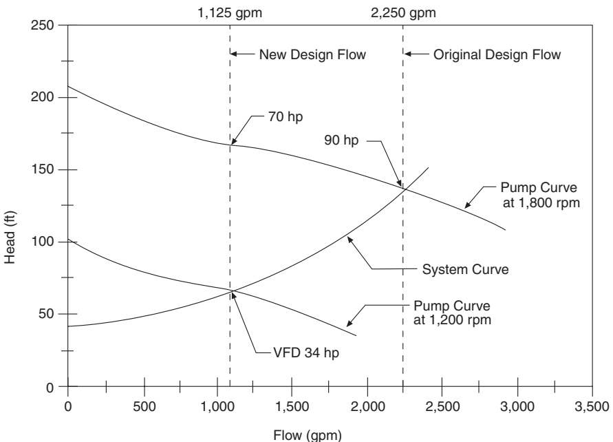
Fig. 30–11. Comparison of flows and loads for throttling valve versus VFDs
