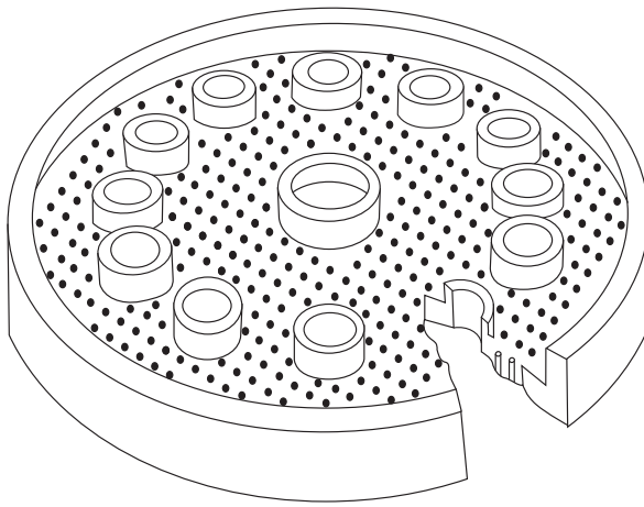
Orifice-type Distributor
