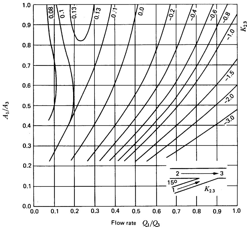
Fig. 26-14. Combining flow—branch angle 15^\circ —loss coefficient K_{23} (Source: Reference 7; courtesy of the BHR Group Limited)
