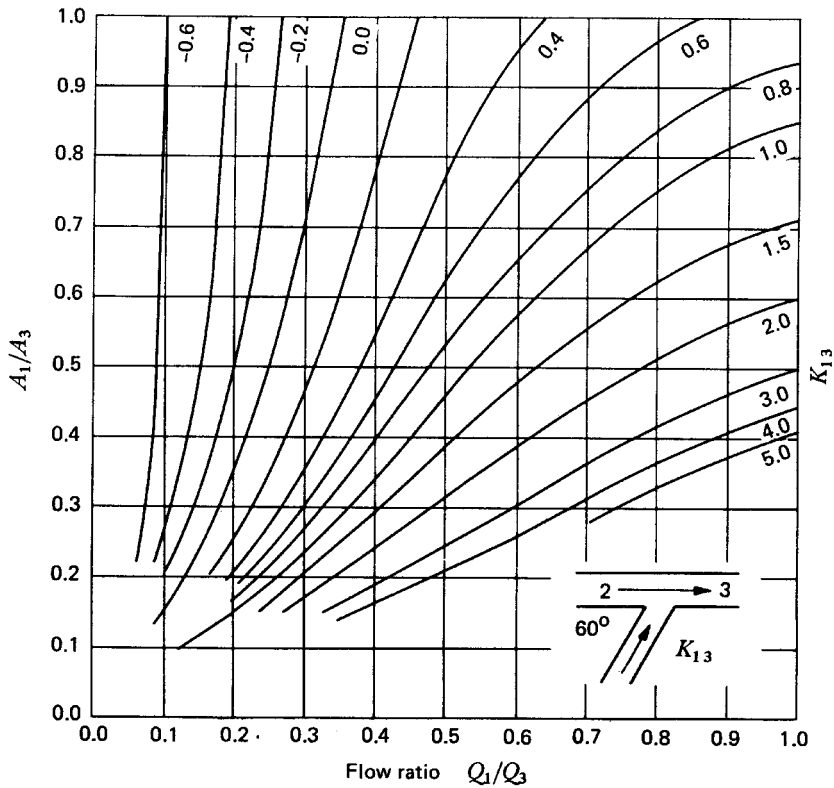
Fig. 26-19. Combining flow—branch angle 60^\circ —loss coefficient K_{13} (Source: Reference 7; courtesy of the BHR Group Limited)
