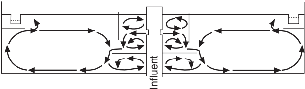
B. Flow Pattern in Baffled Circular Clarifier
