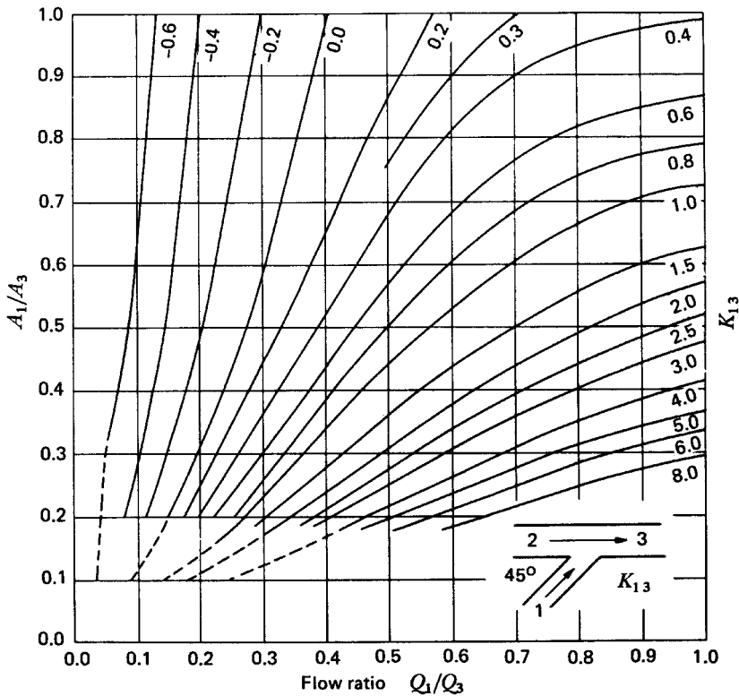
Fig. 26-17. Combining flow—branch angle 45°—loss coefficient K_{13} (Source: Reference 7; courtesy of the BHR Group Limited)
