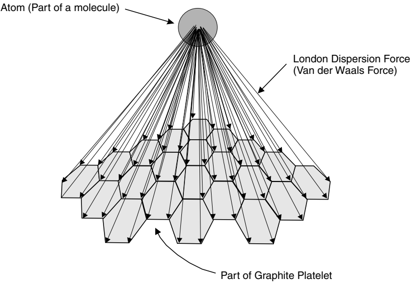
(b) Adsorption Force Between Molecule and Platelet
