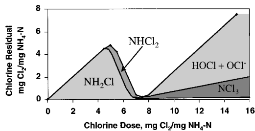
Fig. 19–4. Theoretical breakpoint curve (chlorine and ammonia)
