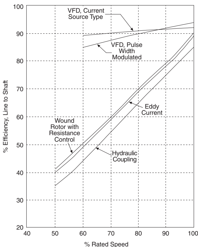
Fig. 30–10. Comparative efficiencies of variable-speed drives ( Source: Reference 10) (Adapted from Journal AWWA , Vol. 72, No. 6 (June 1980), by permission. Copyright © 1980, American Water Works Association.)
