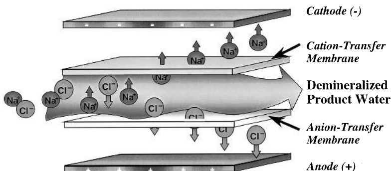
Fig. 15–18. A schematic of typical electrodialysis membrane (Courtesy of Ionics)
