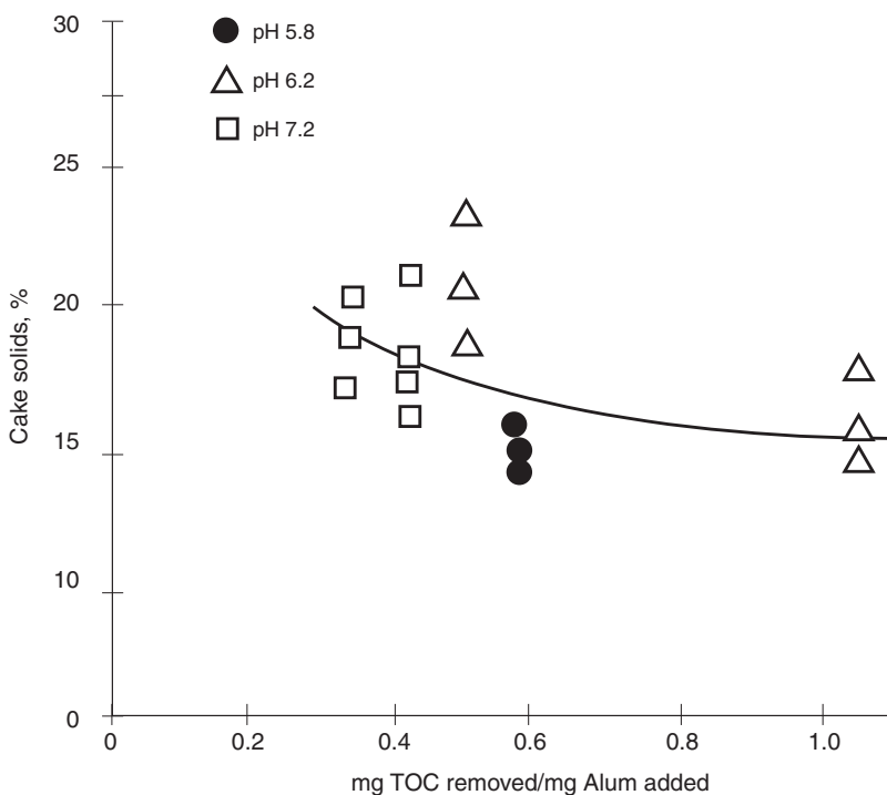
Fig. 23-2. Variations in alum sludge cake solids concentrations as a function of organic content ( Source: Reference 22) (Reprinted from Journal AWWA , Vol. 81, No. 5 (May 1989), by permission. Copyright © 1989, American Water Works Association.)
