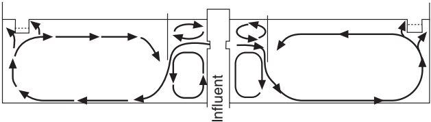
A. Flow Pattern in Conventional Circular Clarifier
