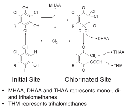
Fig. 3–2. Preferred model of THM and HAA formation following chlorination of NOM (Source: Reference 17)
