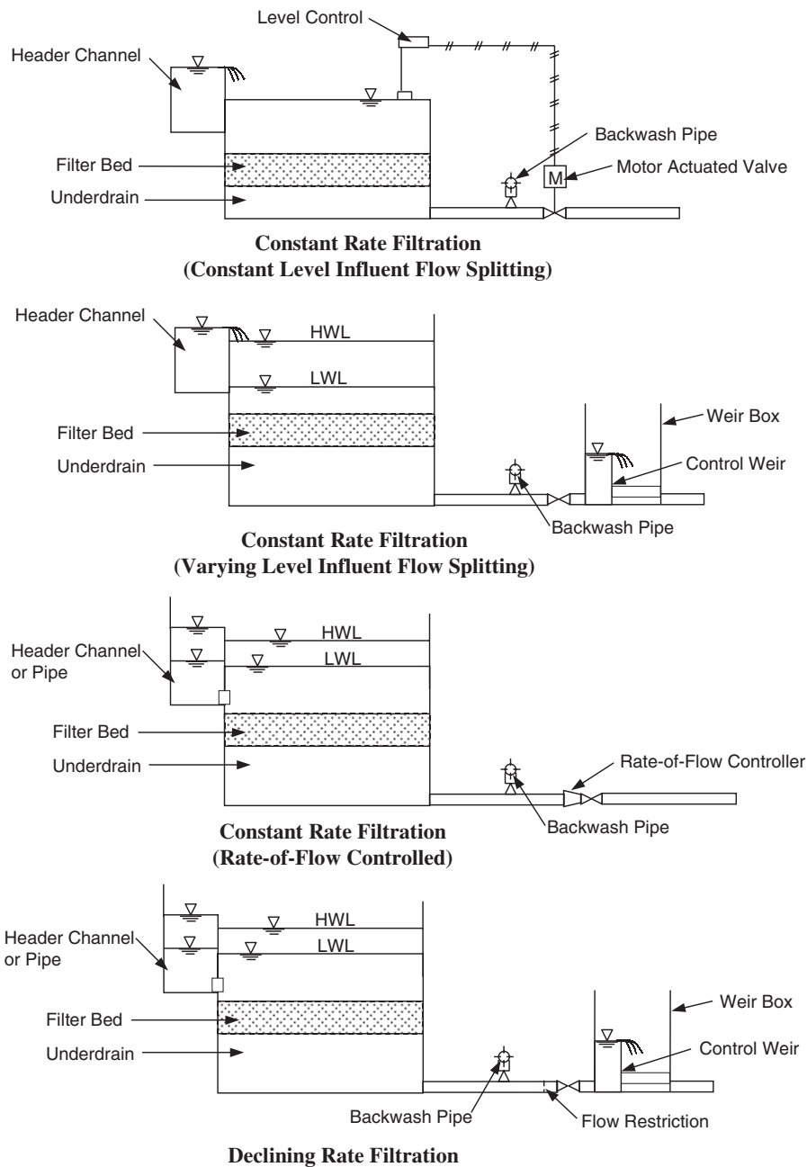
Fig. 12-11. Potential options for operating gravity filters
