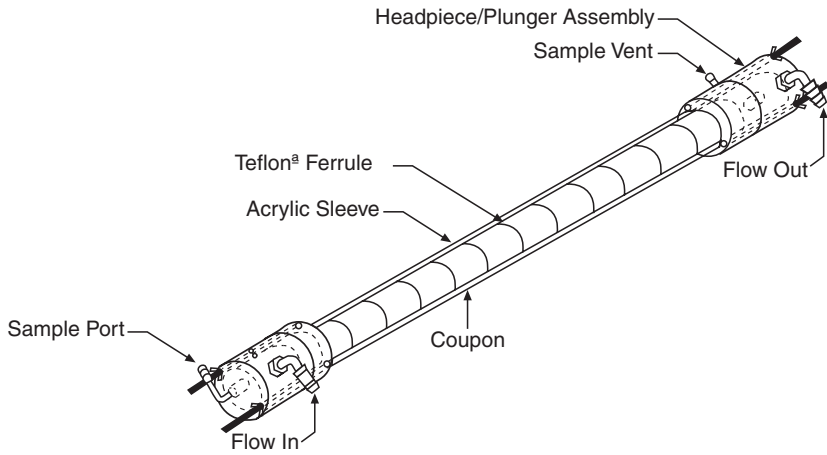
Modified ISWS Coupon Sleeve (University of Washington) Mounting up to 10 Pipe Segment Coupons
