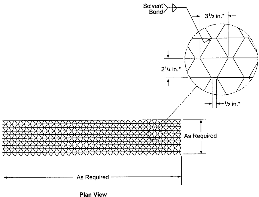
Fig. 11-14. Plan view of modular tube construction (Courtesy of Enviropax, Inc.)
