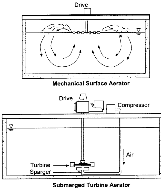
Fig. 9-43. Schematic of a mechanical aeration process
