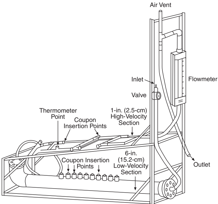
WRC Corrosion Rig with Low- and High-Flow Sections (Uses Flat Coupon Held on an Insulating Stem)
