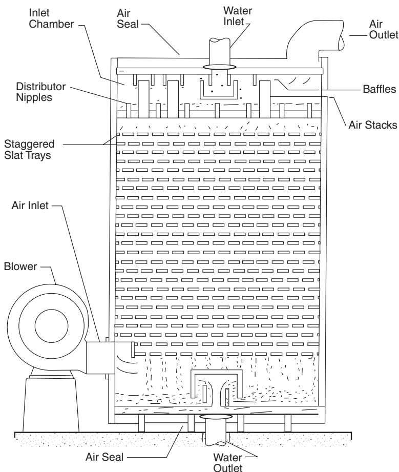
Fig. 9-40. Multiple tray aeration system
