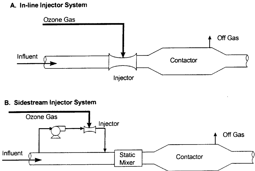
Fig. 19–15. Sidestream ozone injection system
