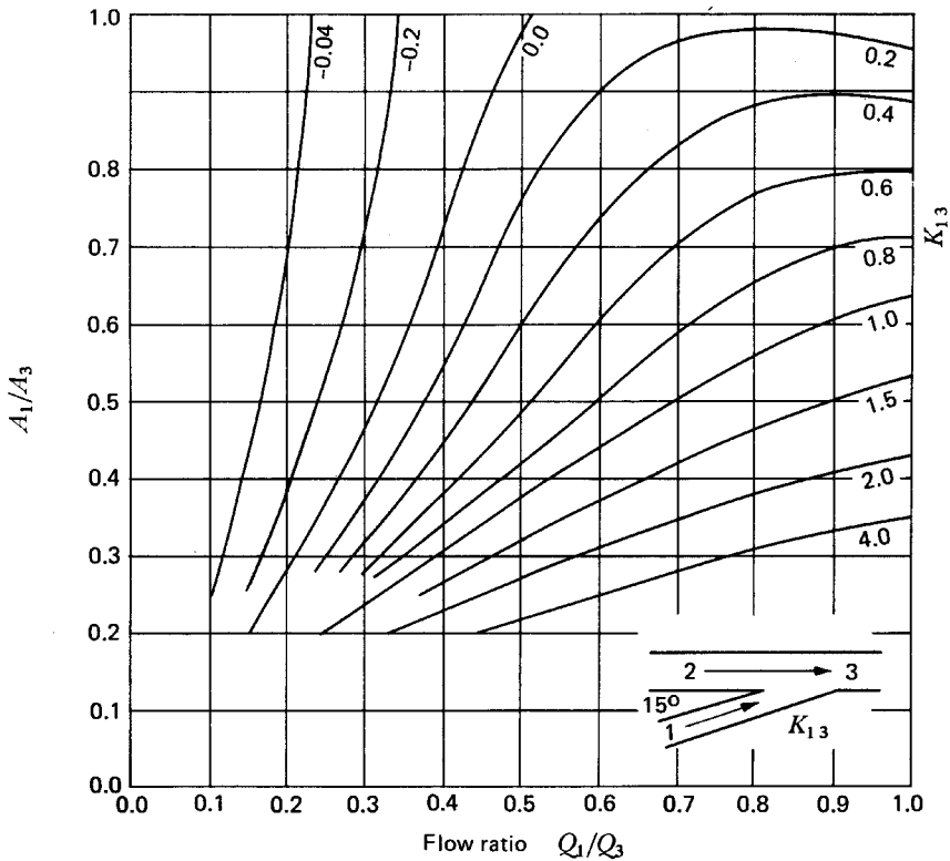
Fig. 26-13. Combining flow—branch angle 15^\circ —loss coefficient K_{13} (Source: Reference 7; courtesy of the BHR Group Limited)
