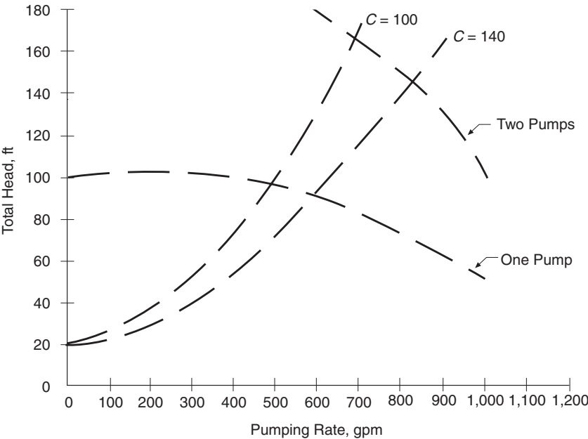
Fig. 29–15. System curve for pumps in series
