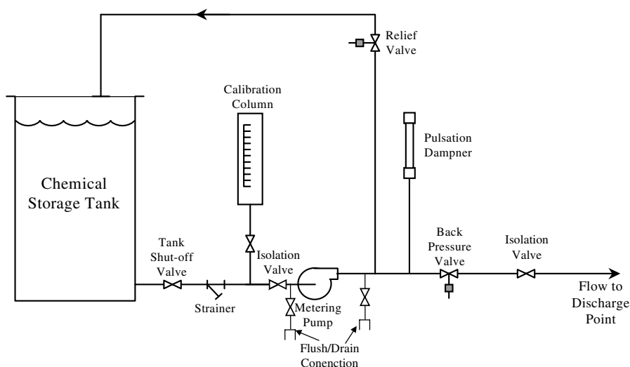
Fig. 19-3. Sodium hypochlorite feed system
