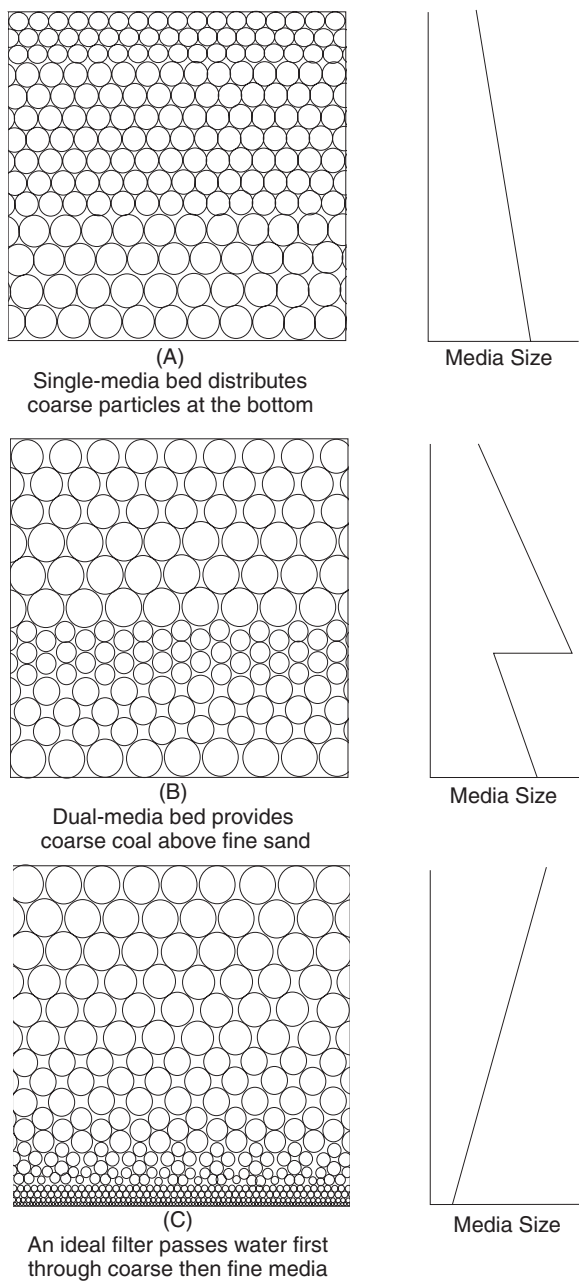
Fig. 12–2. Graphical representation of various media designs
