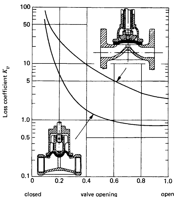
Fig. 26-27. Diagrams valve loss coefficients ( Source: Reference 7; courtesy of the BHR Group Limited)
