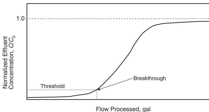
Fig. 17-5. Typical breakthrough curve
