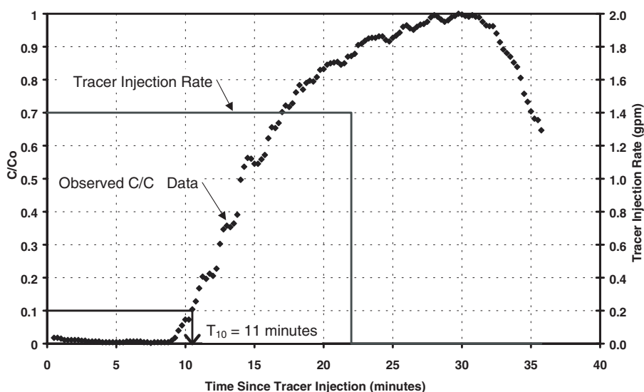
Fig. 26-43. Step-feed tracer curve
