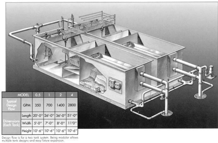
Fig. 25–15. Schematic of Actifloc package water treatment plant setup (Courtesy of USFilter/ Kruger)
