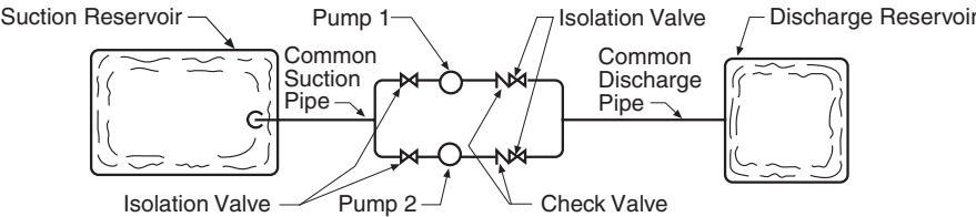
Fig. 29–12. Parallel pumps
