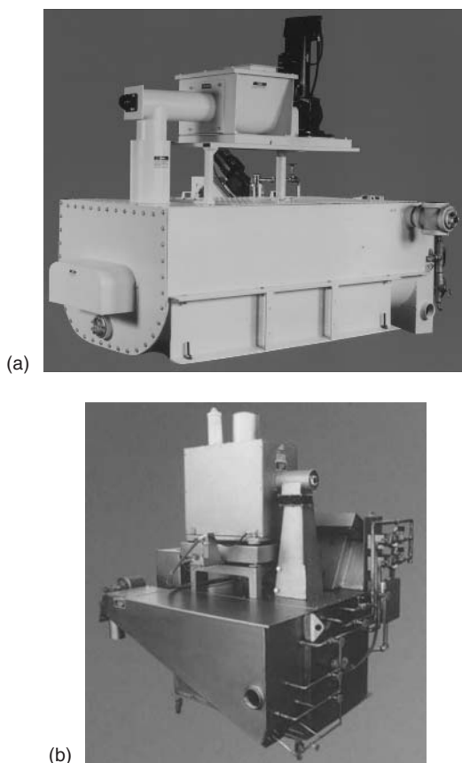
Fig. 24-19. (a) Photo of paste-type lime slaker (Courtesy of USFilter/Wallace and Tiernan); (b) Photo of detention-type slaker (Courtesy of Penn Process/Omega)
