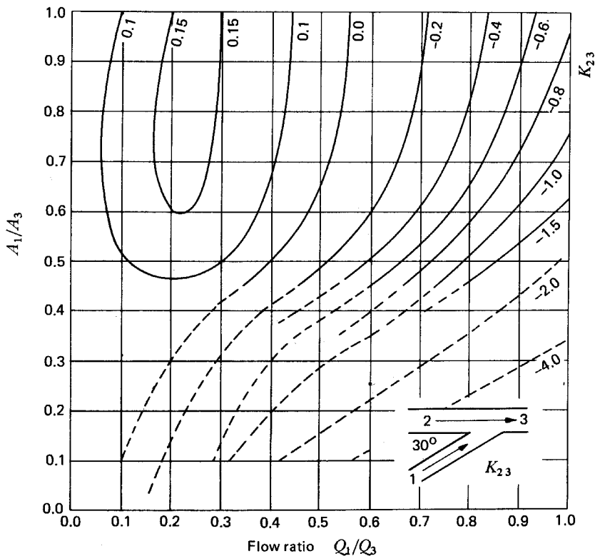
Fig. 26-16. Combining flow—branch angle 30^\circ —loss coefficient K_{23} (Source: Reference 7; courtesy of the BHR Group Limited)
