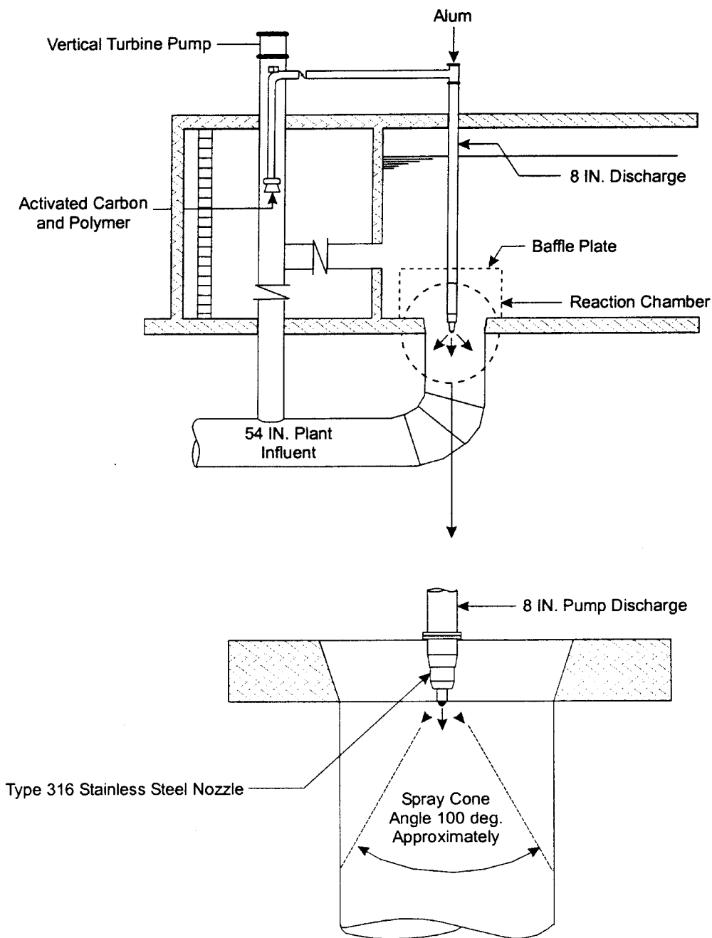
Fig. 10-8. Typical flash mixing facility (Source: Reference 44. Reprinted from Water Treatment Plant Design , 3d ed., by permission. Copyright © 1998, American Water Works Association and American Society of Civil Engineers.)
