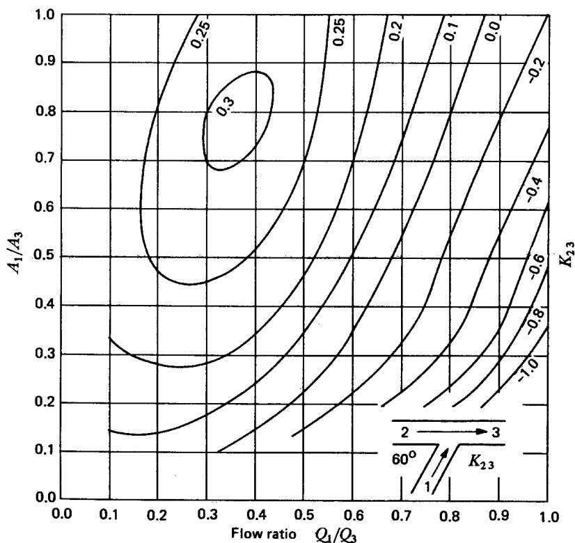
Fig. 26–20. Combining flow—branch angle 60^\circ —loss coefficient K_{23} (Source: Reference 7; courtesy of the BHR Group Limited)
