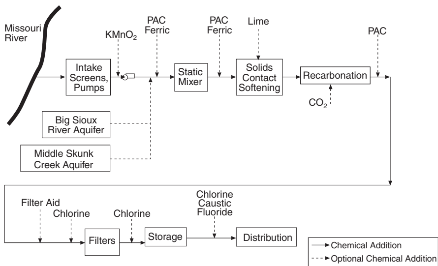
Fig. 17-14. Sioux Falls water treatment plant flow schematic
