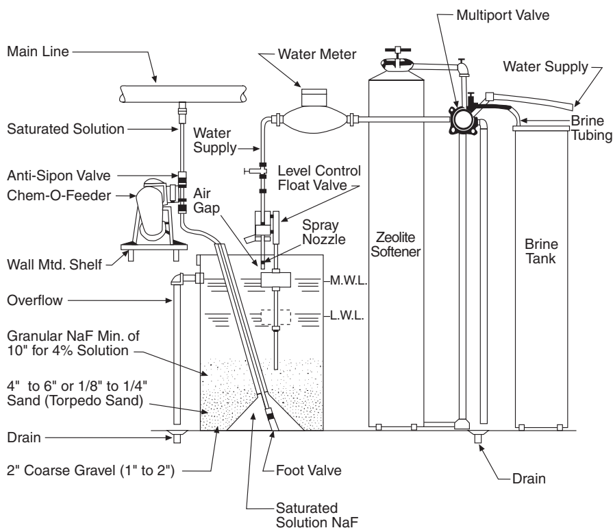
Fig. 20-5. Downflow saturator
