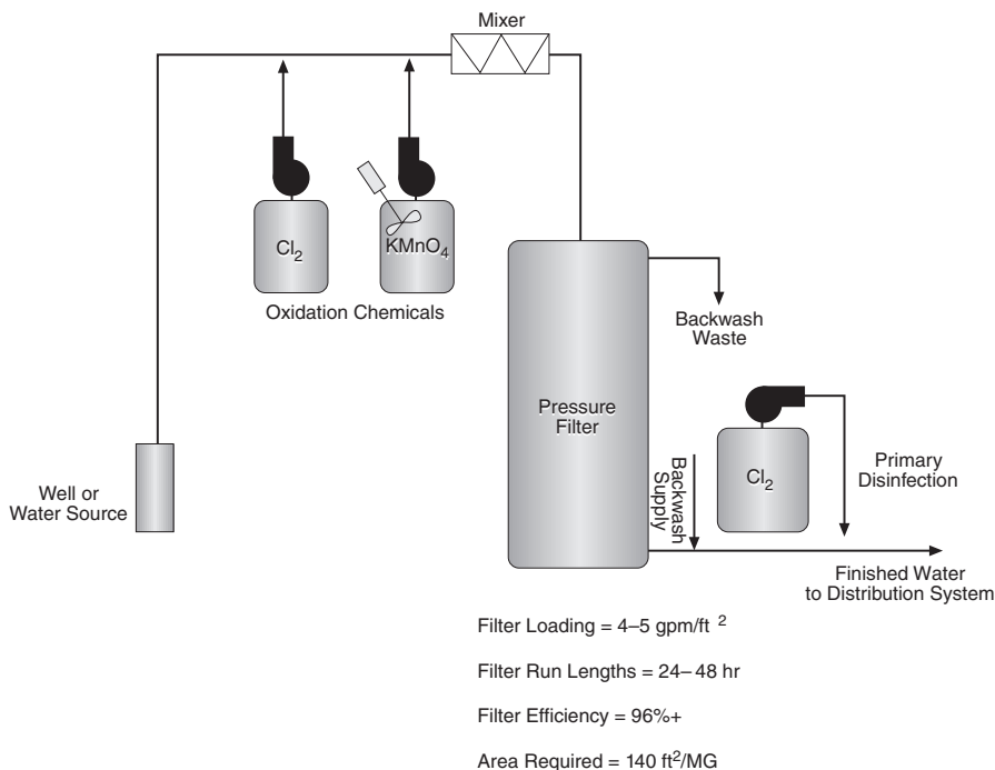
Fig. 14-2. Prechlorination system for removal of iron and manganese
