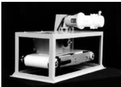
Fig. 24-13b. Gravimetric feeder (Courtesy of Inflico Degremont, Inc.)
