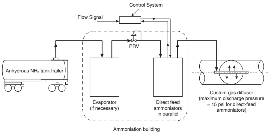
Fig. 19–6. Anhydrous ammonia direct feed system ( Source: Reference 1)
