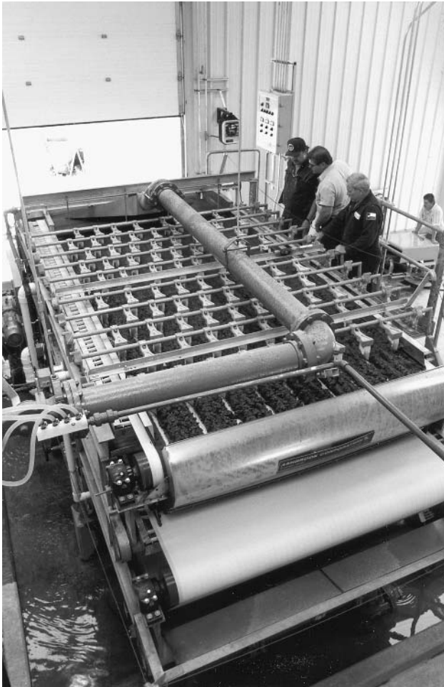
Fig. 23–17. Belt press installation at Cedar Park, Texas, water-treatment plant (Courtesy of Ashbrook-Simon-Hartley)
