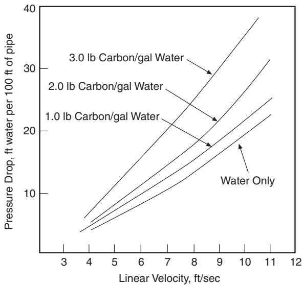
Fig. 17-41. Pressure drop of carbon-water slurries (2-inch pipe) (Courtesy of Calgon Carbon Corporation)
