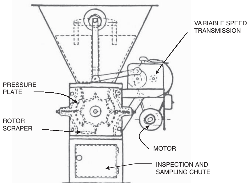
Fig. 24-10. Positive-displacement rotary feeder (Source: Reference 7)
