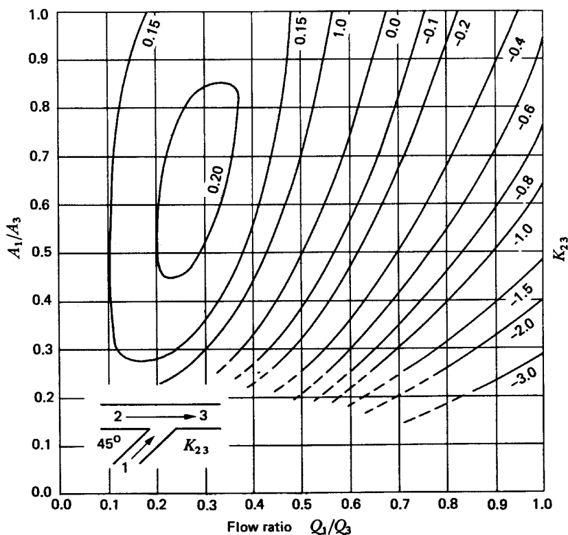
Fig. 26–18. Combining flow—branch angle 45^\circ —loss coefficient K_{23} (Source: Reference 7; courtesy of the BHR Group Limited)
