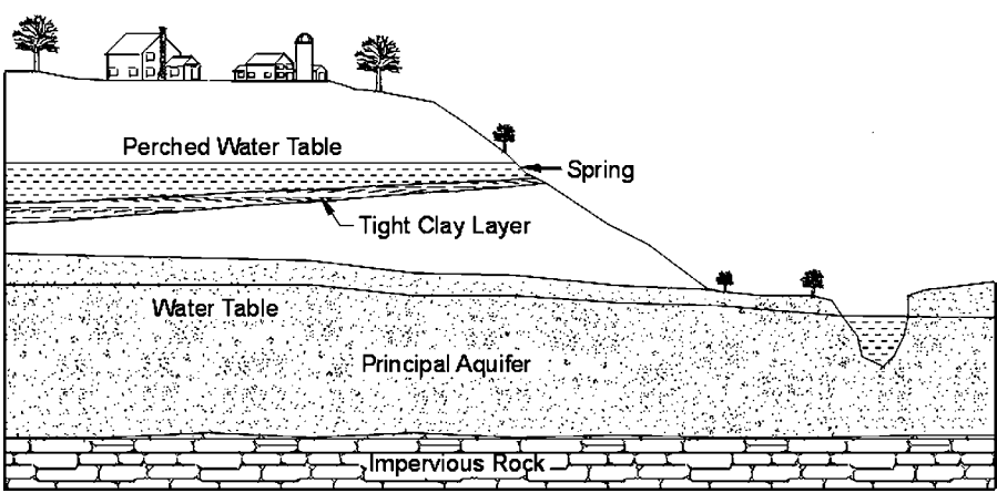
Fig. 8-16. Perched water table (Courtesy of US Filter/Johnson Sceeens)
