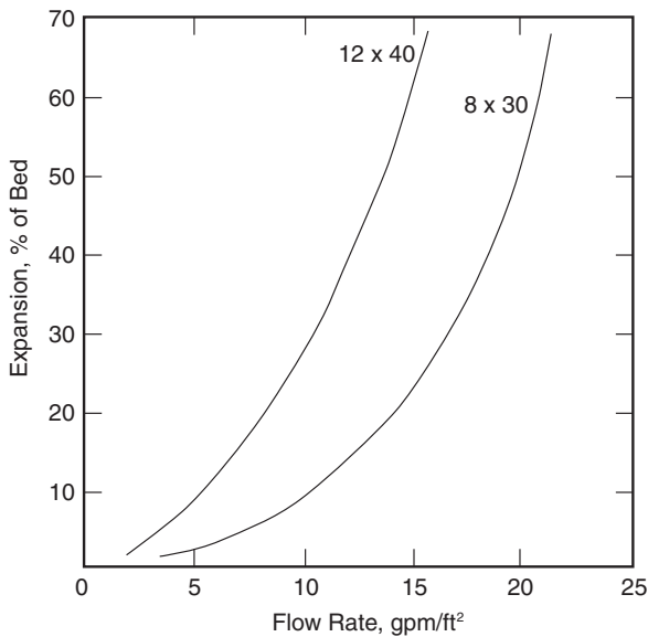
Fig. 17-4. Expansion of carbon bed at various flow rates. Carbon: 12 × 40, 8 × 30; liquid: water at 22°C ( Source: Reference 10; courtesy of Calgon Carbon Corporation)
