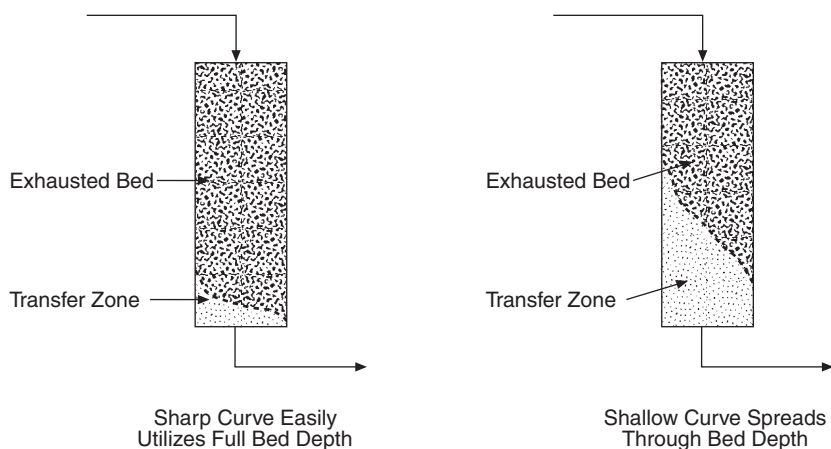
Fig. 17-7. Breakthrough curve shape determines effectiveness of adsorption
