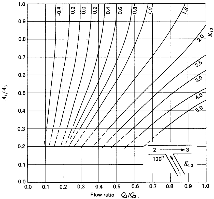
Fig. 26-23. Combining flow—branch angle 120^\circ —loss coefficient K_{13} (Source: Reference 7; courtesy of the BHR Group Limited)
