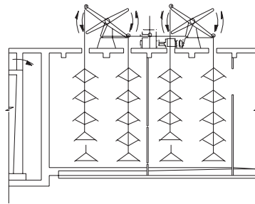
g) Walking beam flocculator
