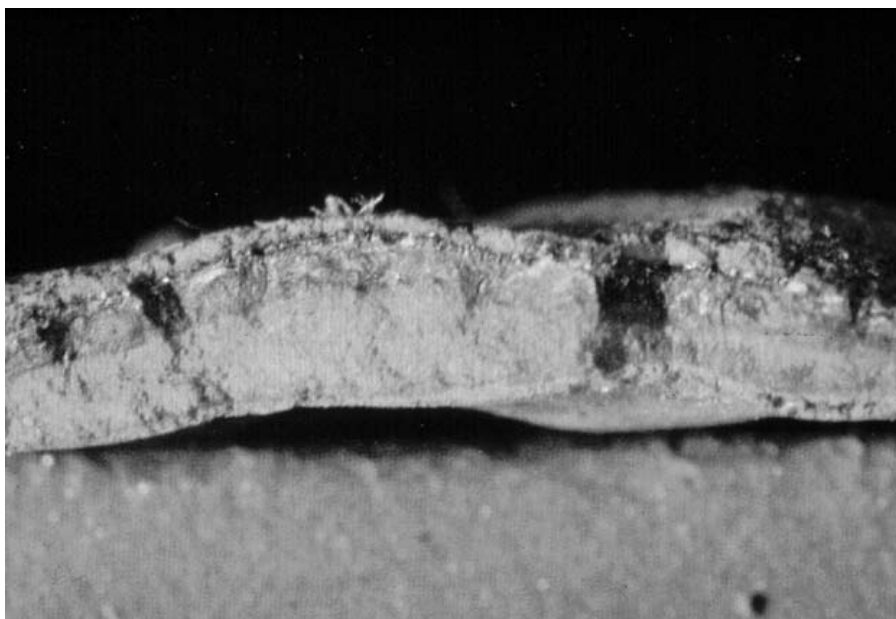
Fig. 21-8. Corrosion scale cross-section on an unlined cast-iron pipe
