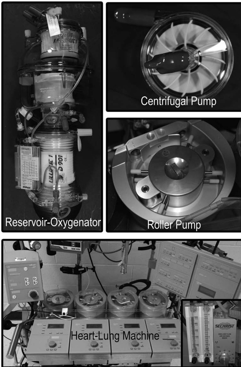
Figure 18.2 Heart-Lung Machine
