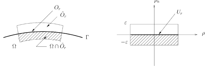
Figure 8.2.1: The tubular neighbourhood of O_r
