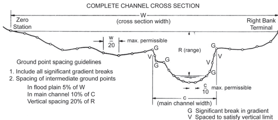
FIGURE 3.7 Example of a riverine cross-section survey. Elevations are measured at all significant breaks in gradient and at intermediate points depending on the width and depth of the river. SOURCE: FEMA (2003).
