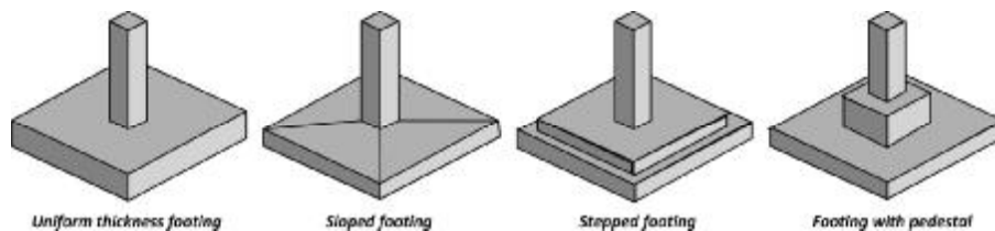
Fig. 14.5.3.6—Types of spread footings.
