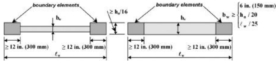
Fig. 11.1.5.2—Boundary element dimensions.
