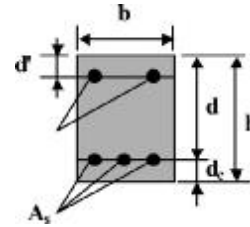
Fig. 8.4.6—Section with tension and compression reinforcement.
