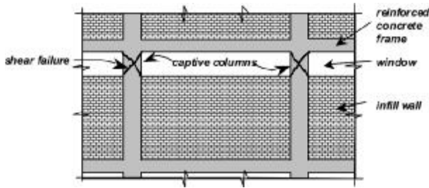
Fig. 11.2.3.1—Captive or short column effect.
