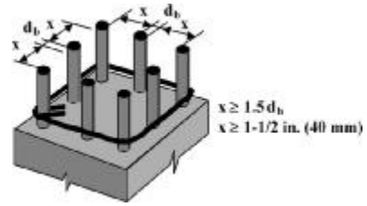
Fig. 10.4.2.6—Clear spacing between longitudinal bars in columns.
