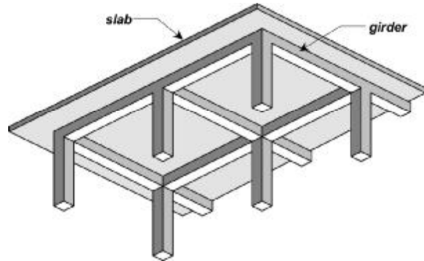
Fig. 6.1.2.1—Slab-on-girder floor system.
