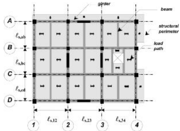
Fig. 3.3.2—Typical floor structural layout.
