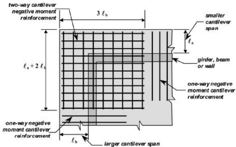
Fig. 7.6.3.4—Negative moment reinforcement in two-way slab cantilevers.
