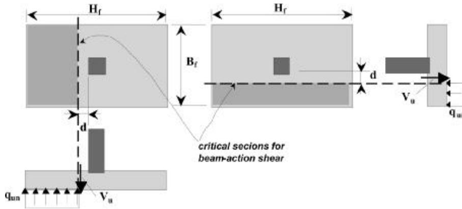
Fig. 14.5.5.7—Tributary areas for beam-action shear.
