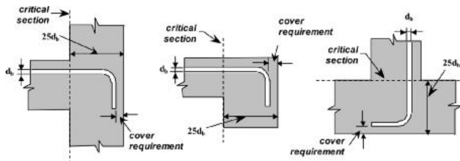
Fig. 5.8.3—Minimum standard hook anchorage distance.
