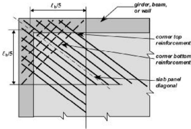
Fig. 7.3.8—Slab corner reinforcement.
