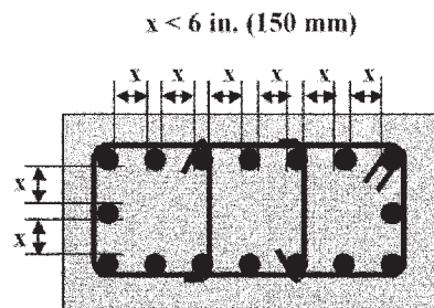
Fig. 10.4.3.2a—Horizontal tie arrangement.
