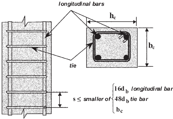
Fig. 10.4.3.2b—Vertical spacing of ties.
