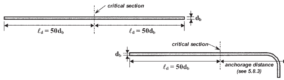
Fig. 5.8.1.1—Development length for reinforcing bars.
