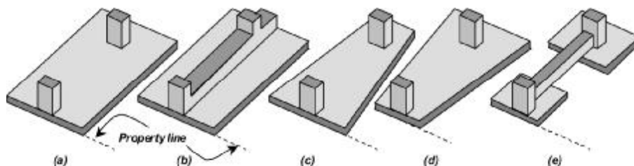
Fig. 14.7.1—Types of combined footings.
