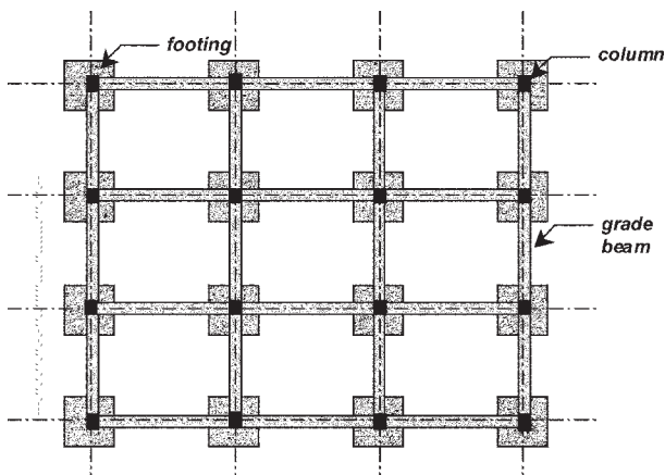
Fig. 14.12.1.1b—Grid of grade beams.
