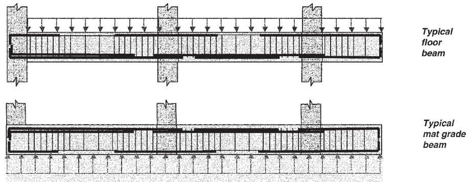
Fig. 14.10.3.1—Reinforcement layout for beams.
