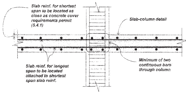
Fig. 9.4.1—Slab reinforcement detail.
