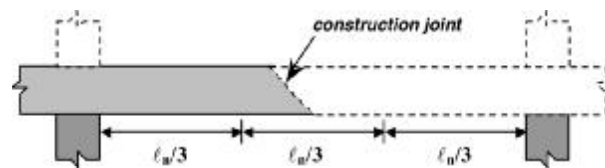
Fig. 16.4.6.2—Construction joints in slabs, girders, and beams.
