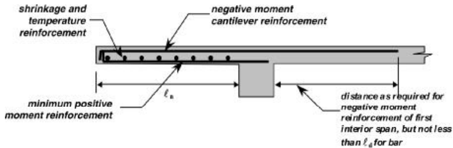
Fig. 7.6.3.1—Reinforcement for slab cantilevers.
