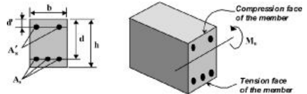
Fig. 8.4.9.3—Design dimensions for moment strength: sections with compression reinforcement.
