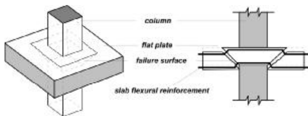
Fig. 6.1.4.1—Punching shear failure.
