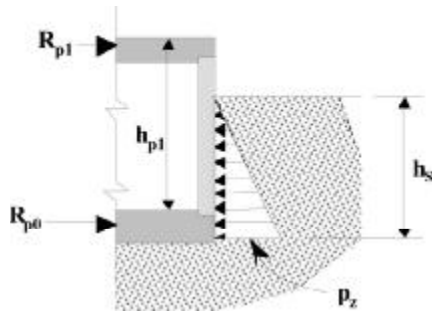
Fig. 4.13.2.3—Lateral reaction due to soil pressure.
