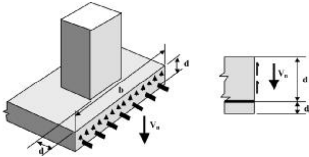
Fig. 9.5.5—Beam-action shear strength in solid slabs.
