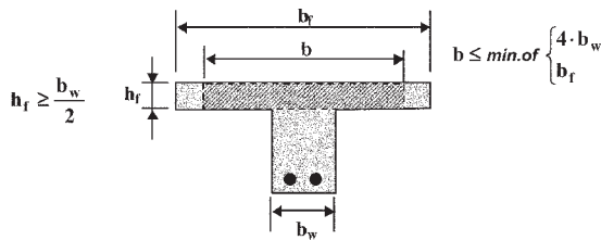
Fig. 8.4.10.3—Effective flange width for isolated T-beams.
