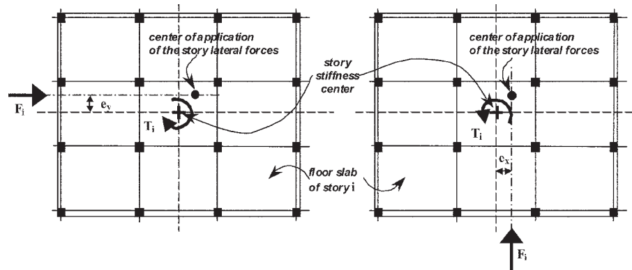
Fig. 4.13.5—Story torsion.
