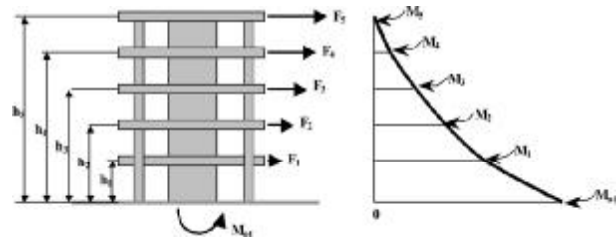
Fig. 4.13.4—Overturning moment calculation.
