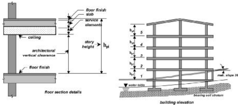
Fig. 3.3.3—General structural layout in elevation
