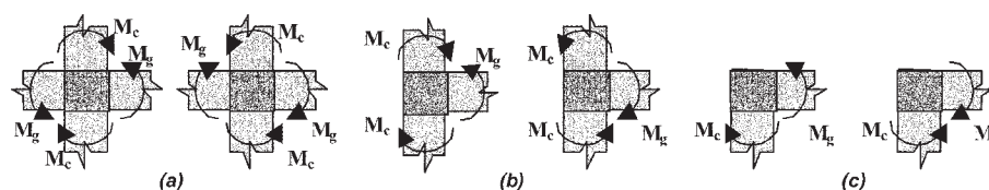
Fig. 11.1.3.3—Minimum moment strength of columns.
