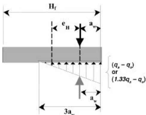
Fig. 14.5.7.5—Soil pressure with uplift.
