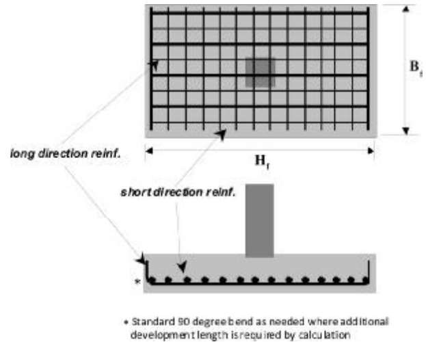
Fig. 14.5.4.7—Distribution of reinforcement in rectangular spread footings.
