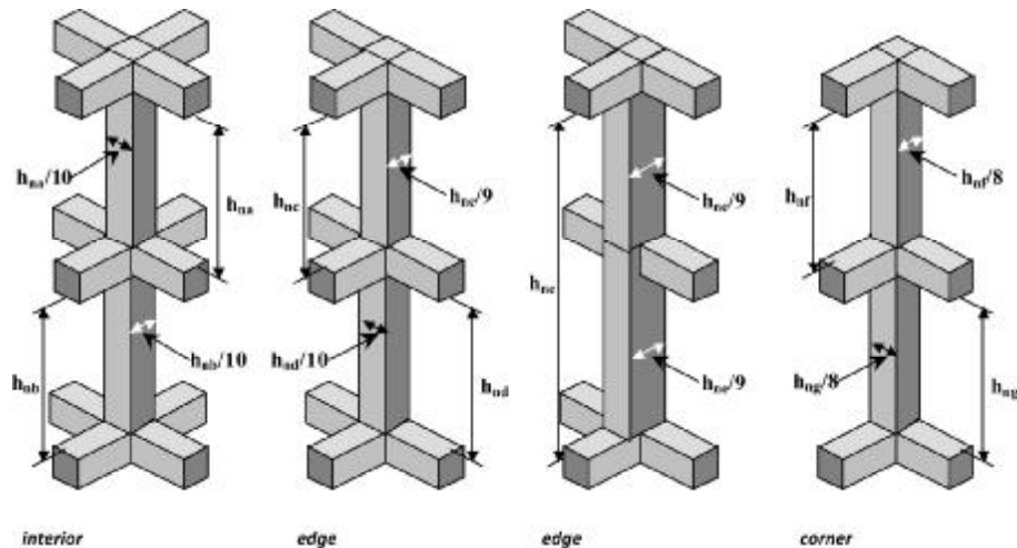
Fig. 10.3.3.1—Lateral restraint for columns.
