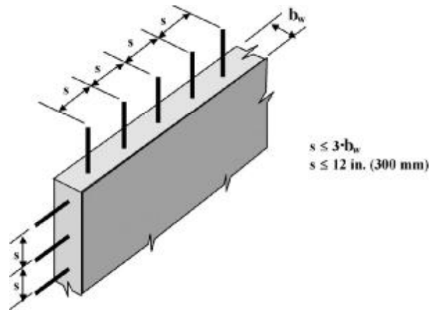
Fig. 12.4.2—Reinforcement spacing in reinforced concrete walls.
