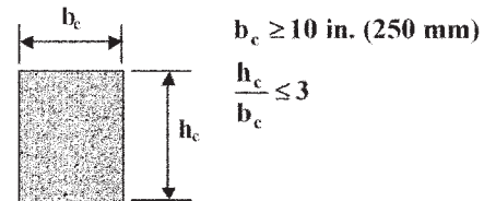
Fig. 10.3.2.1—Minimum cross-sectional dimensions for rectangular columns.
