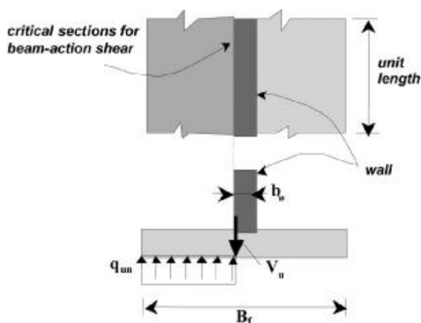
Fig. 14.6.2.2—Beam-action shear in wall footings.
