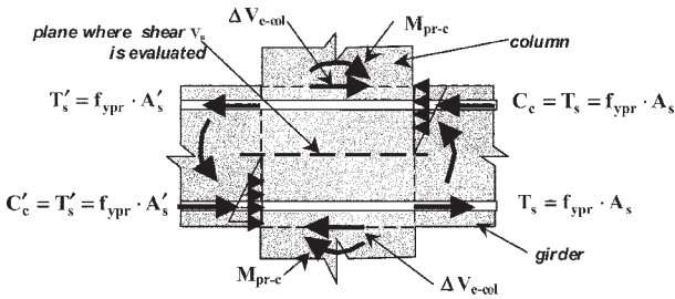
Fig. 11.1.4.4a—Joint shear determination.
