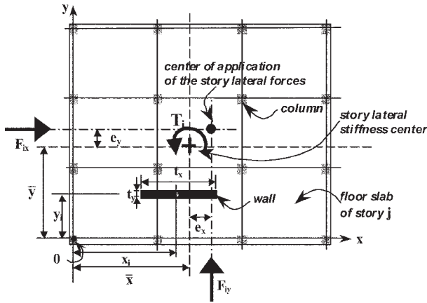
Fig. 4.14.5—Calculation of the story lateral stiffness center.
