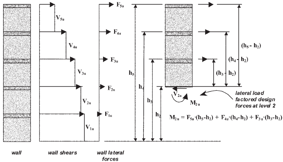
Fig. 12.2.3—Calculation of factored lateral force moments.
