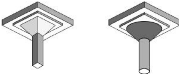
Fig. 6.1.4.3c—Column capital and drop panel.
