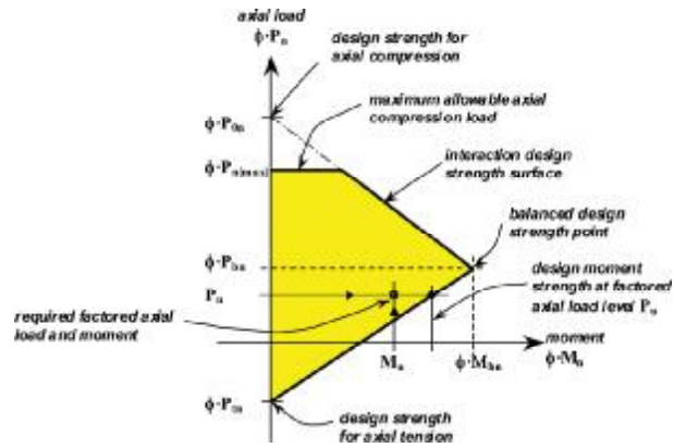
Fig. 5.12.6—Interaction diagram for (\phi M_n, \phi P_n) .
