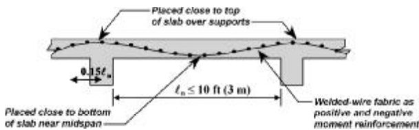
Fig. 7.3.9—Welded wire reinforcement in short one-way spans.
