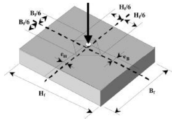
Fig. 14.5.7.3—Location of the resultant to avoid footing uplift.
