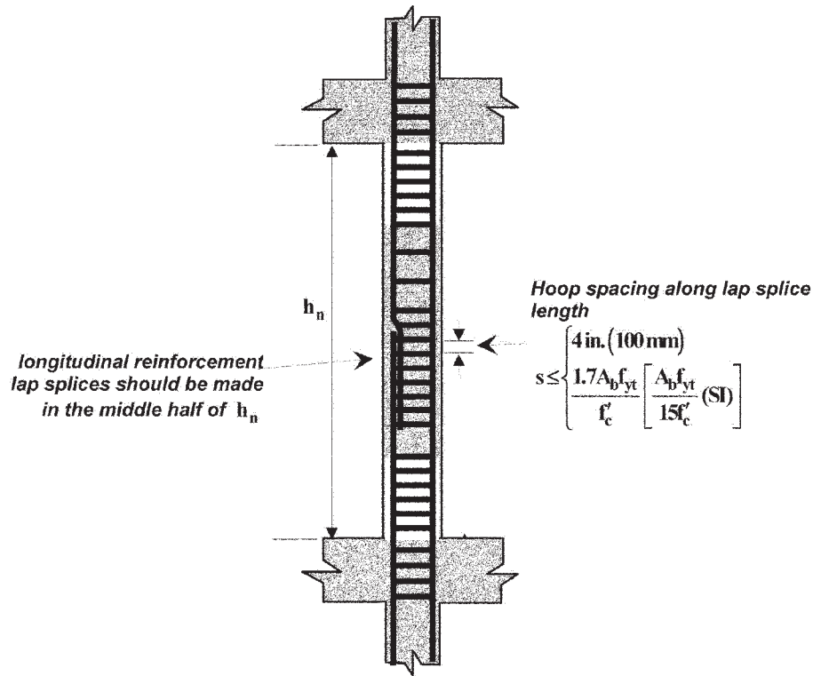
Fig. 11.1.3.4c—Confinement hoop spacing in columns for splices.
