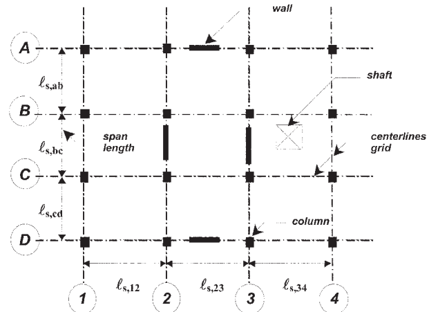
Fig. 3.3.1—General structural layout in plan.
