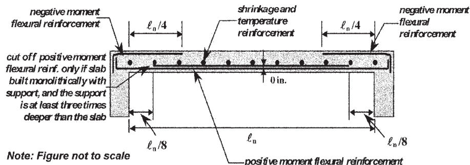
Fig. 7.7.3.1—Reinforcement for single-span one-way slabs.
