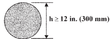
Fig. 10.3.2.2—Minimum cross-sectional dimension for circular columns.
