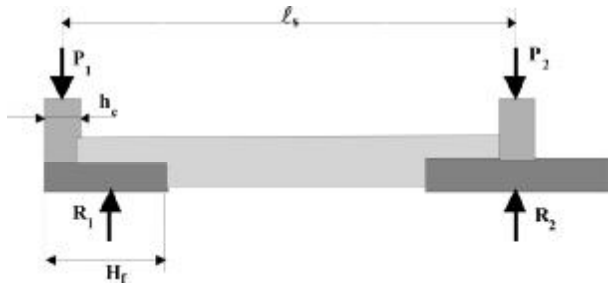
Fig. 14.7.2.1—Combined footing loads, reactions, and dimensions.
