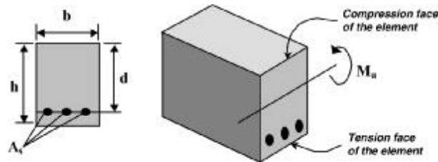
Fig. 5.11.3—Design dimensions for design moment strength.
