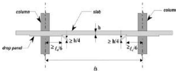
Fig. 6.1.4.3d—Minimum dimensions for drop panels.
