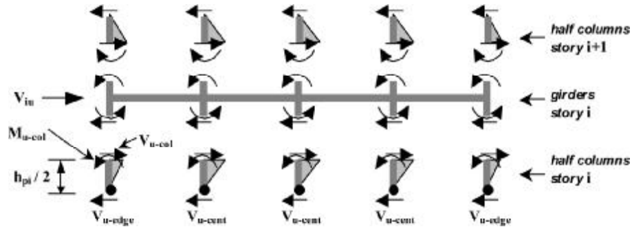
Fig. 4.15.4.2a—Column lateral shears and moments in frames.
