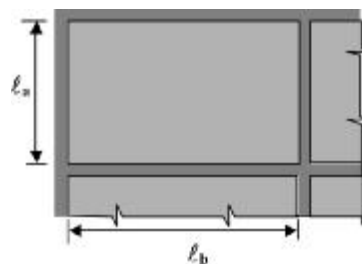
Fig. 7.9.2g—Corner panel of two-way slabs supported on girders, beams, or reinforced concrete walls.
