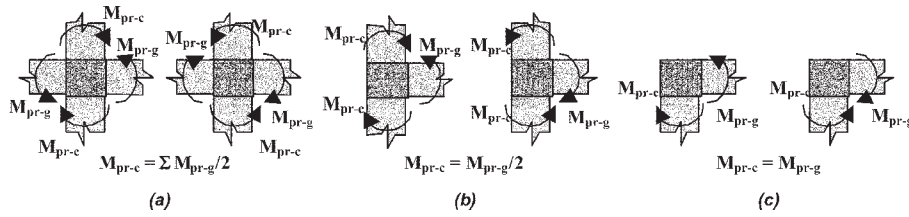
Fig. 11.1.3.6b—Maximum M_{pr} for columns required for column shear \Delta V_c .
