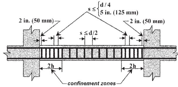
Fig. 11.1.2.3—Confinement stirrup spacing.
