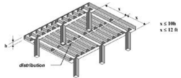
Fig. 6.1.3.2—Distribution ribs.
