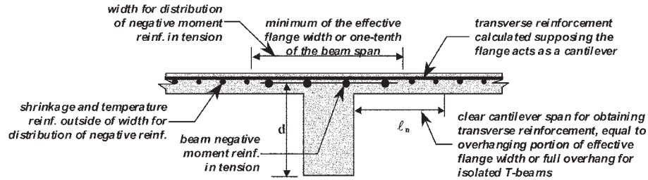
Fig. 8.4.11.1—Reinforcement in T-beam flanges.
