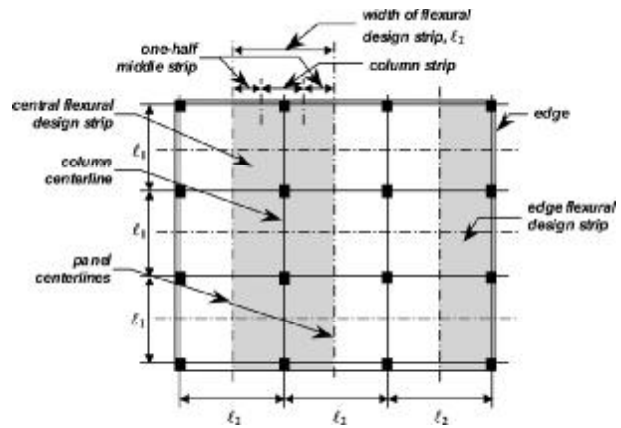
Fig. 9.8.1.1a—Definition of design strips.
