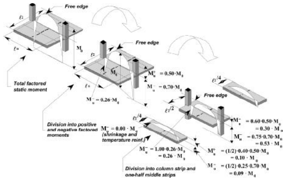
Fig. 9.8.1.1c—Factored moments: exterior spans.
