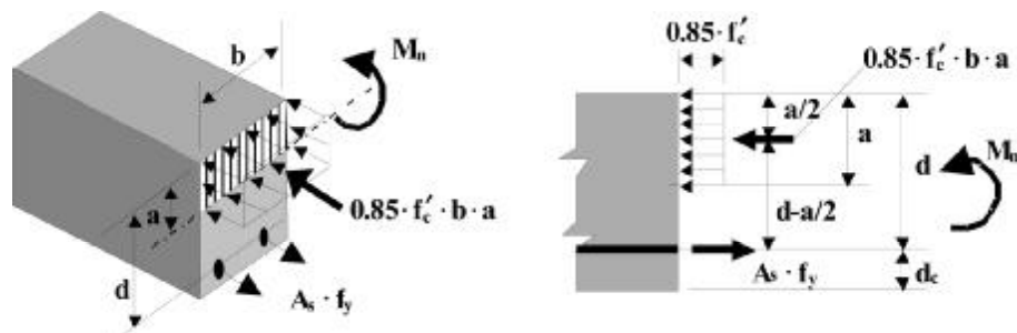
Fig. 5.11.4.1—Flexural nominal moment strength.
