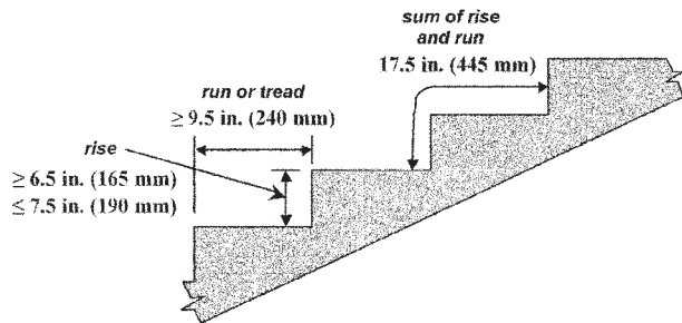
Fig. 13.1.3.3—Maximum step rise and minimum step rise and thread in stairways.
