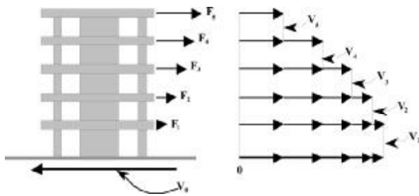
Fig. 4.13.3—Story shear and base shear calculation.
