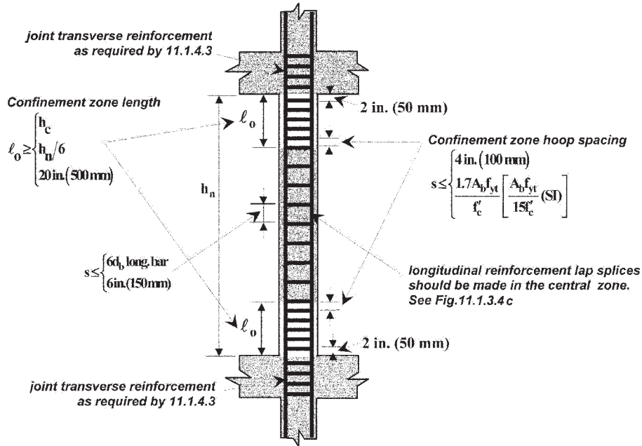
Fig. 11.1.3.4a—Confinement hoop spacing in columns.
