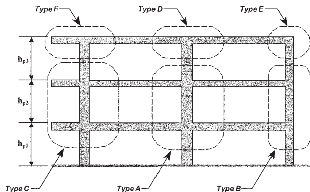
Fig. 8.7.6.3—Joint types for determination of column moments.
