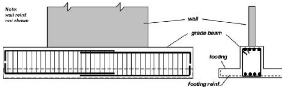
Fig. 14.6.4b—Wall footing grade beam reinforcement layout.
