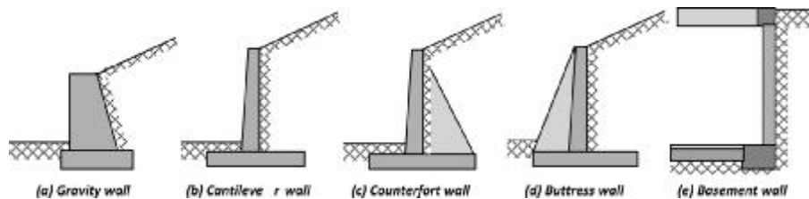
Fig. 14.11.1—Types of retaining walls.
