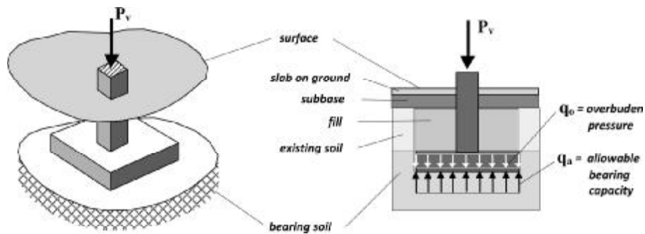
Fig. 14.5.2.1—Loads acting on footings.
