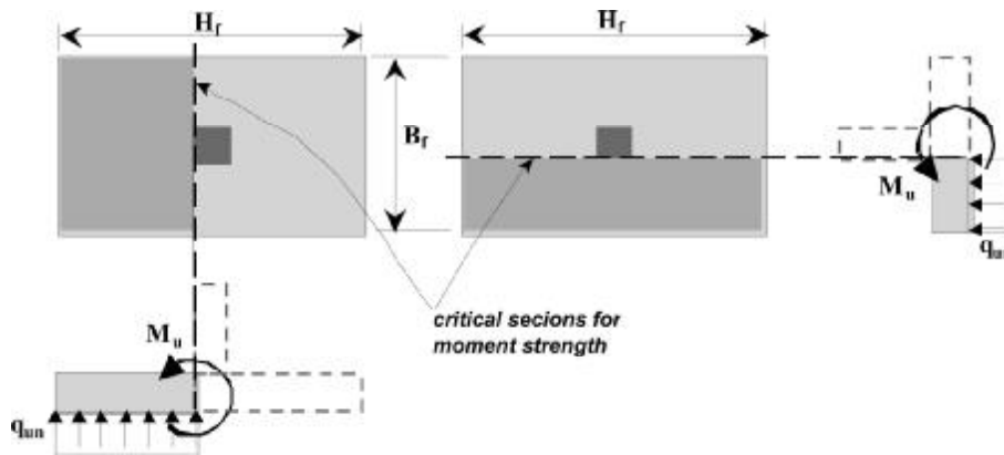
Fig. 14.5.6.1—Critical sections for moments.
