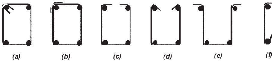
Fig. 8.5.2a—Typical stirrup shapes for girders and beams.
