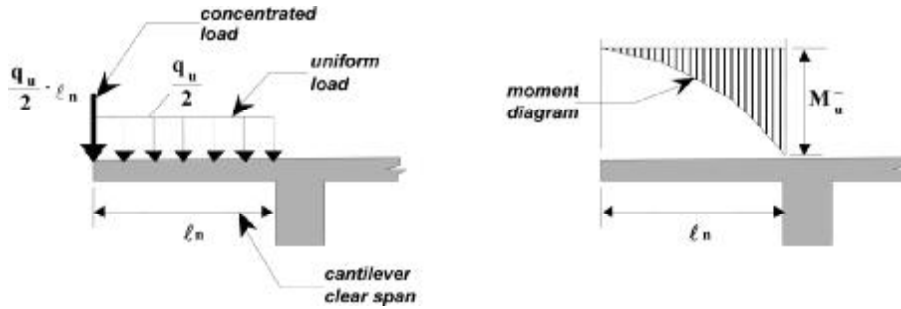
Fig. 7.6.2—Calculation of negative moment at slab cantilevers.
