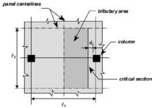
Fig. 9.7.2—Tributary area for beam-action shear.
