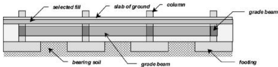
Fig. 14.12.1.1a—Location of grade beams.
