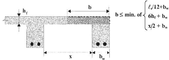
Fig. 8.4.10.2—Effective flange width for T-beams with slab on one side only
