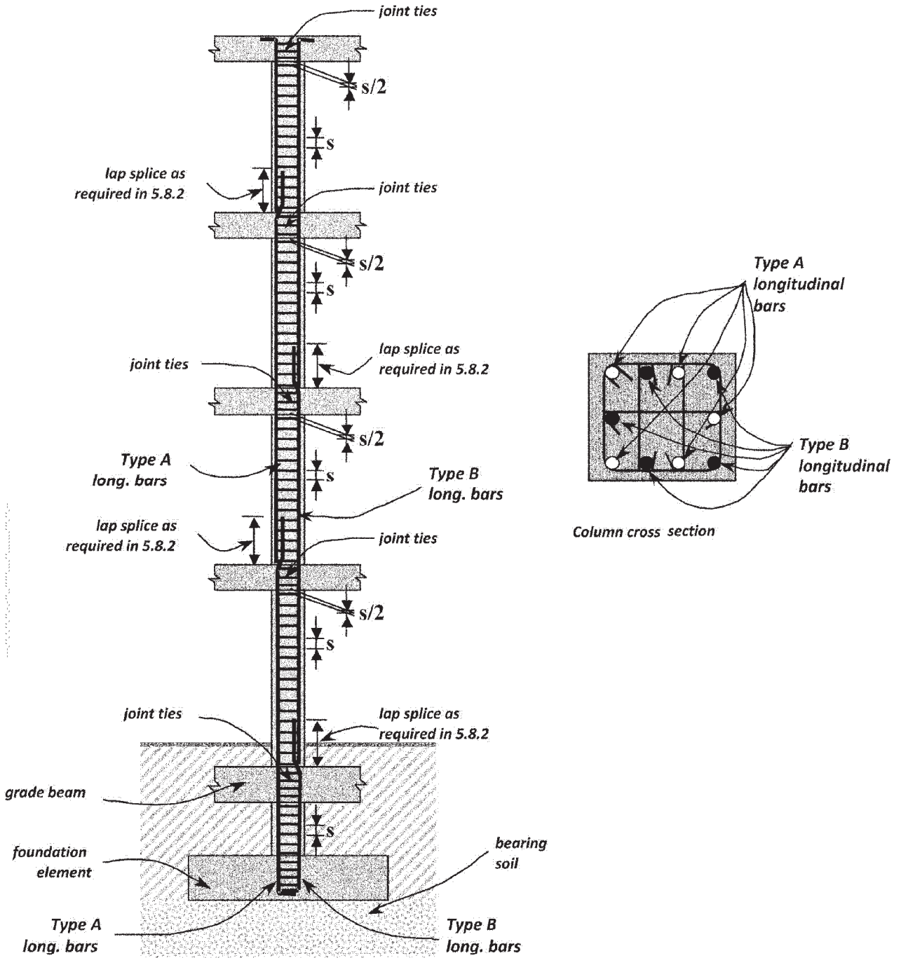
Fig. 10.4.2.8a—Typical column reinforcement layout.
