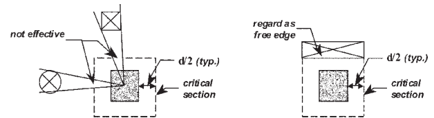
Fig. 9.3.9.3—Effect of openings in the slab.
