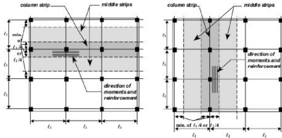
Fig. 9.3.2—Column and middle strips.
