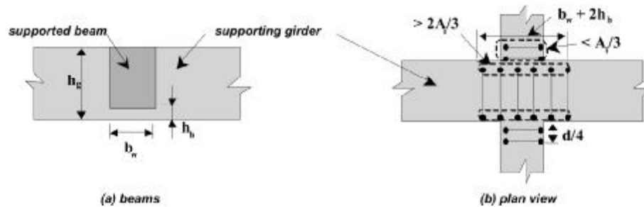
Fig. 8.5.5—Hanger reinforcement.
