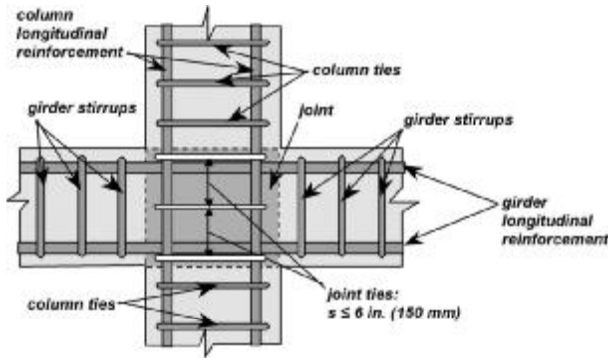
Fig. 10.4.3.4—Column ties in column-girder joints.
