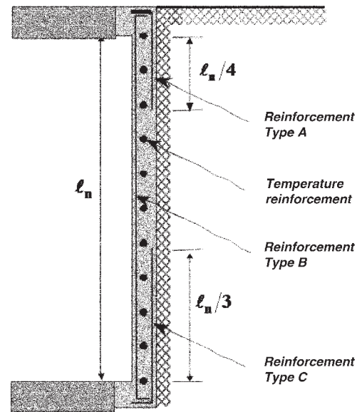
Fig. 14.11.12—Design moments and reinforcement for basement walls.
