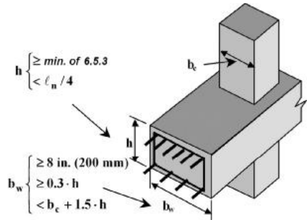
Fig. 8.7.2.2—Limits on girder depth and width.
