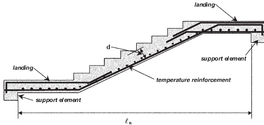
Fig. 13.1.4.3—Typical reinforcement details.
