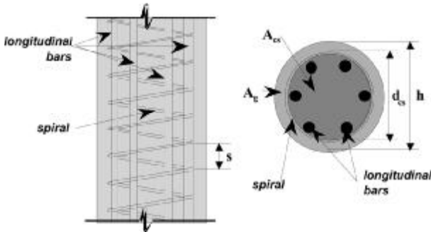
Fig. 10.4.3.3—Spiral reinforcement of column.
