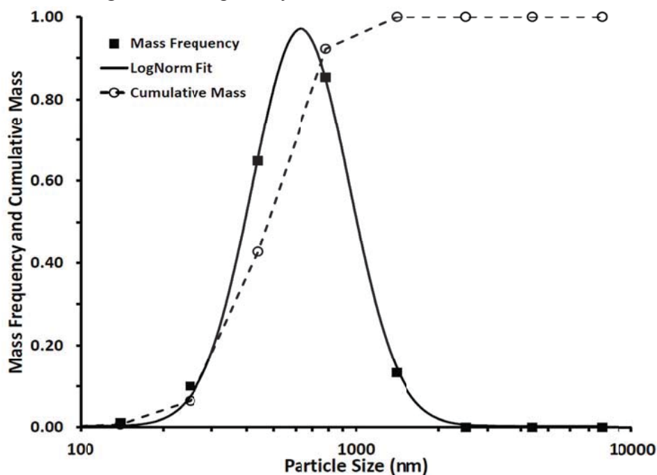
FIGURE 3-2 Mass frequency and cumulative mass distributions derived from impactor particle size distribution measurement of e-cigarette 1.
