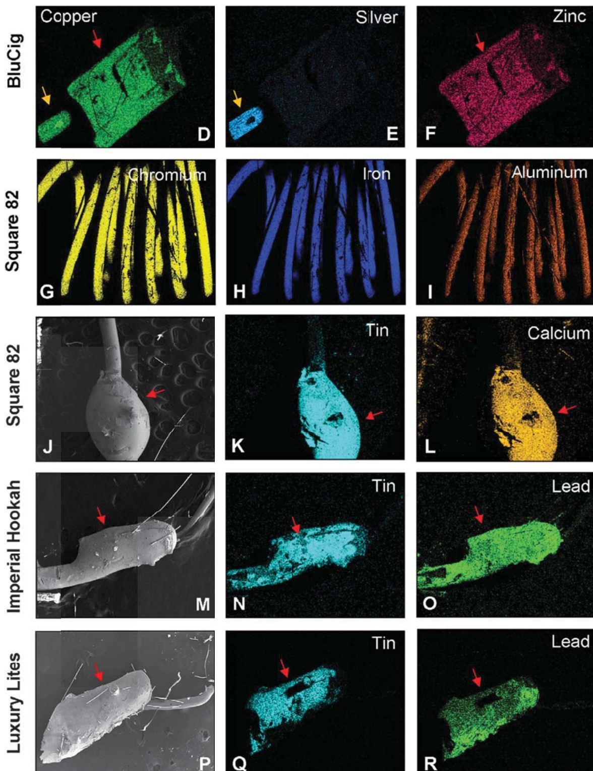
FIGURE 5-3 Scanning electron microscopy and energy dispersive X-ray spectroscopy analysis of disposable EC/EH wires and joints. SOURCE: Williams et al., 2017.
