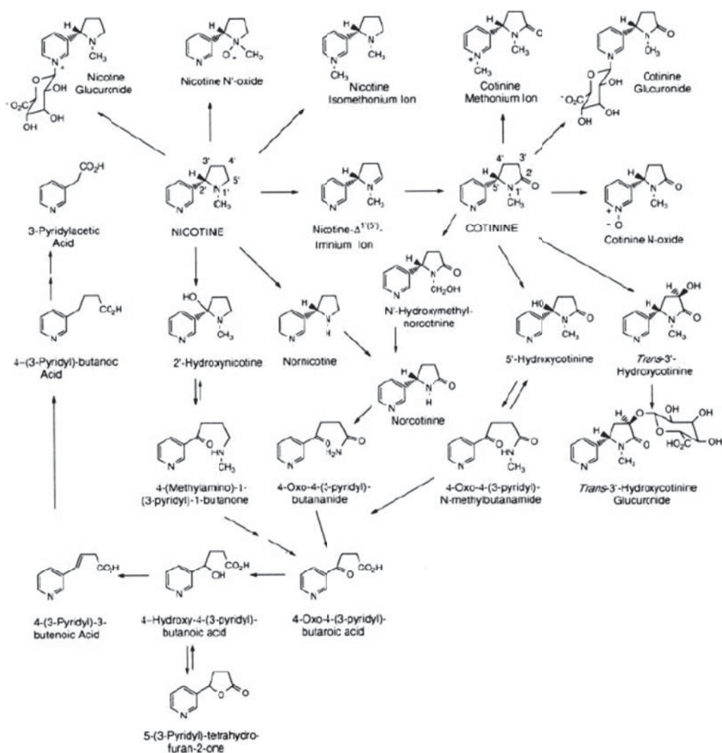
FIG. 5. Pathways of nicotine metabolism.
