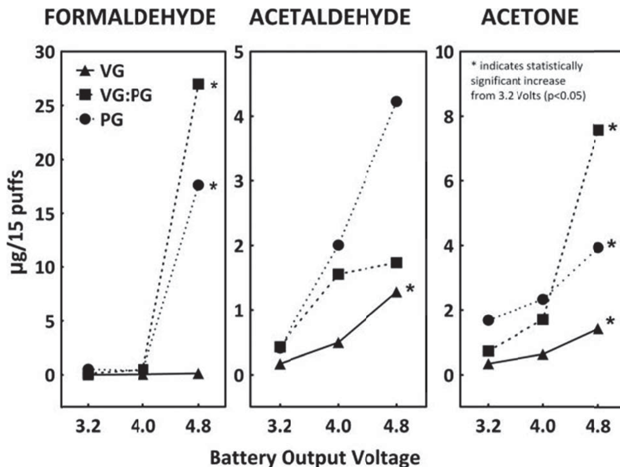
FIGURE 5-2 Effects of nicotine solvent and battery output voltage on levels of carbonyl compounds released from electronic cigarettes ( \mu\text{g}/15 puffs; n = 3 ; puff duration 1.8 s, puff volume 70ml, puff intervals 17 s).
