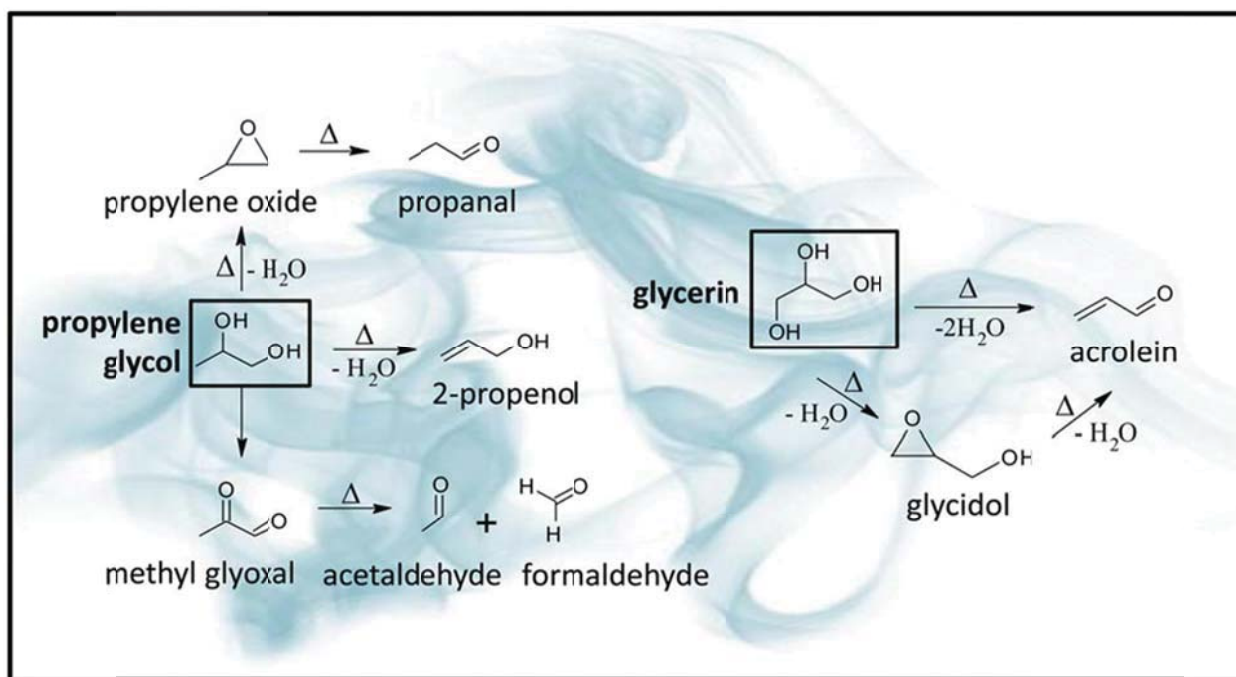
FIGURE 5-1 Postulated pathways and byproducts formed during thermal dehydration of propylene glycol and glycerin.
