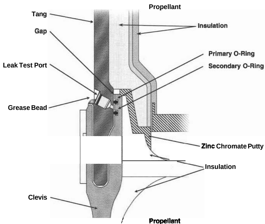
Exhibit 111 Cross section showing the leak test port
