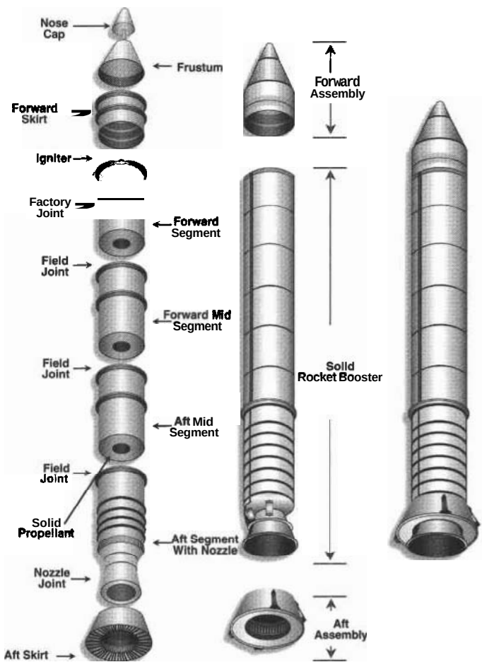
Exhibit I. Solid rocket booster (SRB)
