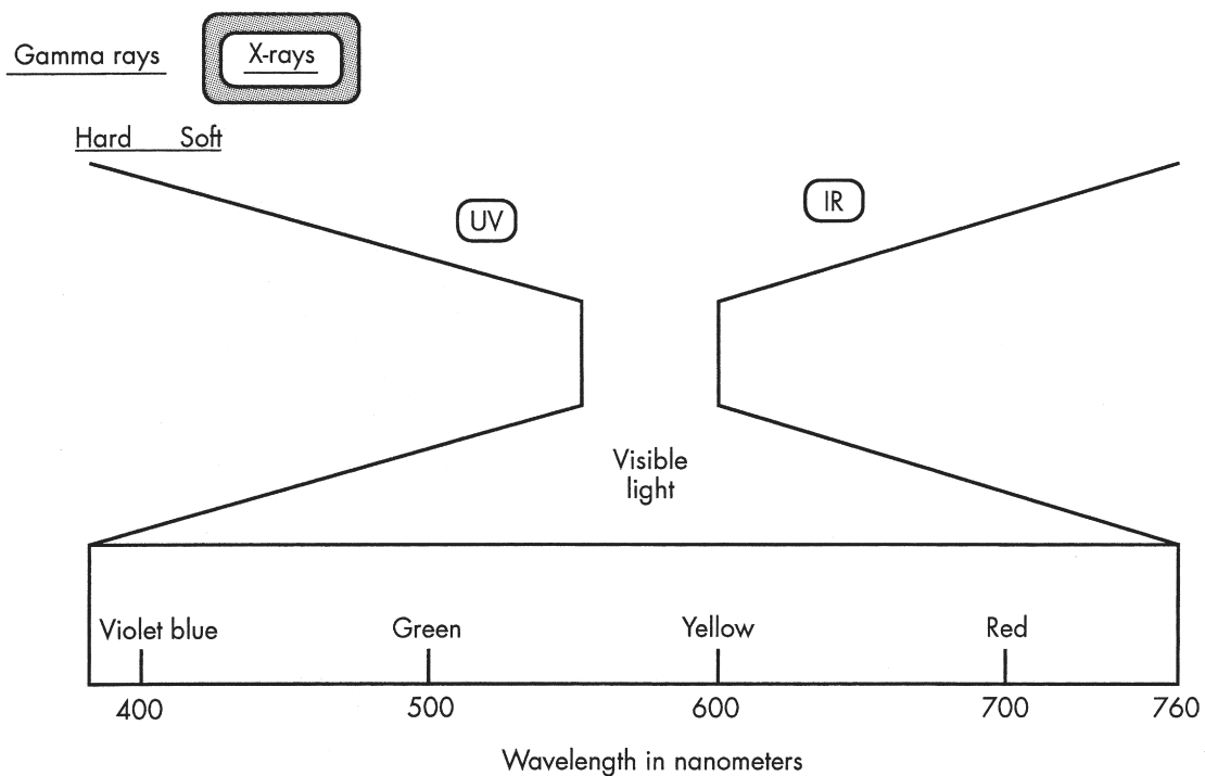
FIGURE 5-1 ■ Electromagnetic spectrum.
