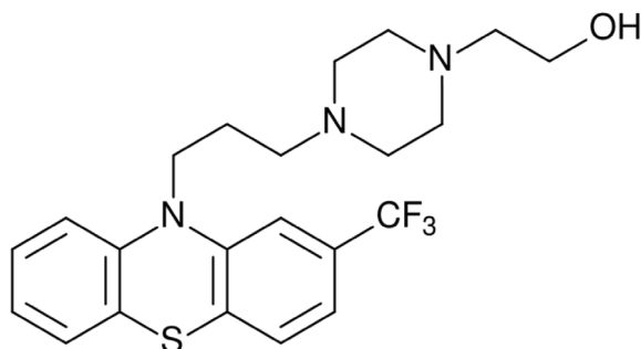
Fig. 1. Chemical structure of Fluphenazine
