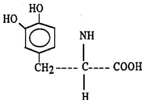
Fig. 3. Chemical structure of L-DOPA
