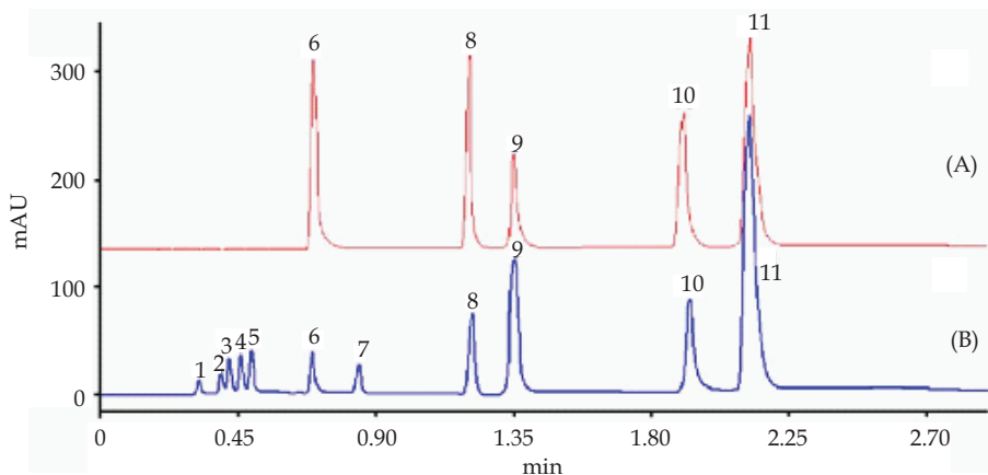
Fig. 4. Chromatogram of mixed standard compounds (A) and standardized chromatographic fingerprint of 10 batches Rhizoma Coptidis samples obtained by UPLC-PAD method at 350 nm(B)
