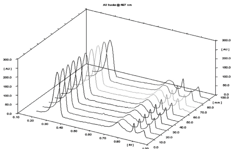
Fig. 12. Selectivity of the method. Peak 1 (from left to right): L-DOPA; peak 2: Carbidope (dopa-decarboxylase inhibitor)
