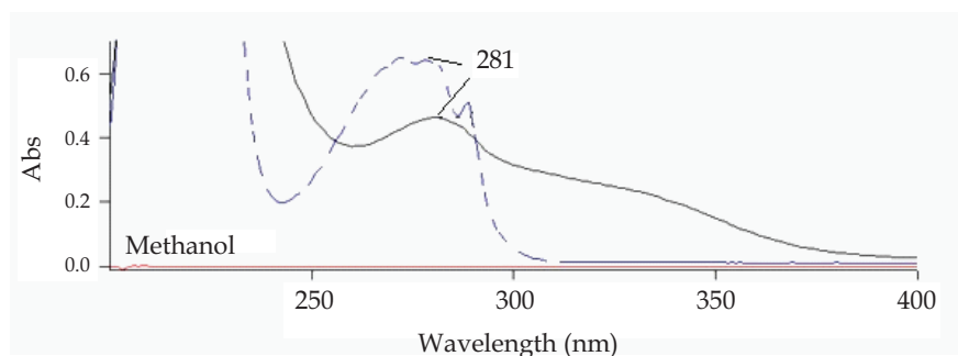
Fig. 7. Selectivity of the method developed with 22µg/mL Yoimbine as reference, (---), in relation to the alkaloid fraction of the aqueous extract of Himatanthus sp at 30 µg/mL (—) and to solvent methanol, observed from 200nm to 400nm (absorbance vs wavelength)
