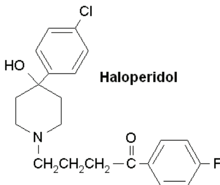
Fig. 2. Chemical structure of Haloperidol
