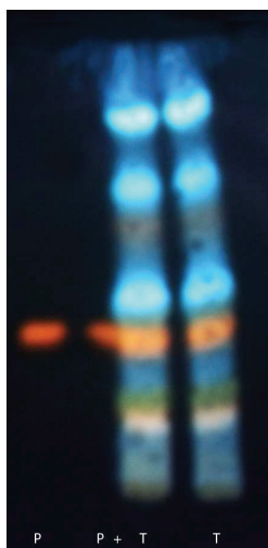
Fig. 6. TLC analysis of the tincture of Calendula officinalis L. Eluent I: ethyl acetate; formic acid; acetic acid; water (100:11:11:26); developer: NP/PEG 4000. Observation under light UV 365 nm; P- rutin standard ; T- Calendula tincture (Nunes, 2008; Nunes et al., 2009)
