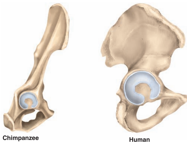
Figure 8.8 Chimpanzee and Human Hip Bones. Lateral views of the right hip bone. The human ilium forms a more bowl-like greater pelvis and is expanded posteriorly (toward page left) so that the gluteus maximus muscle produces an effective backswing of the thigh during the stride.
