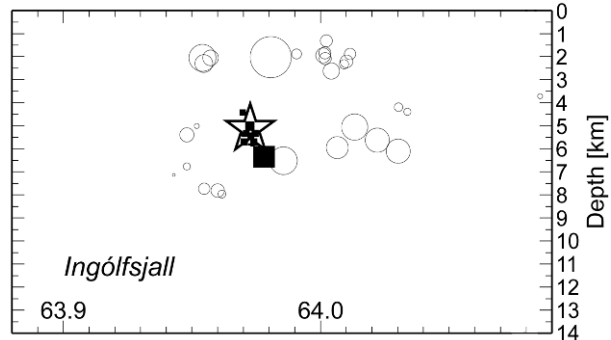
Figure 4.36. Earthquakes on a north–south cross-section along the fault of the first part of the earthquake (i.e., the eastern fault). The horizontal axis shows latitude in degrees north. Circles are aftershocks. Squares represent the 39 densely distributed foreshocks that occurred in a single hour close to the hypocenter which is indicated by a star.
