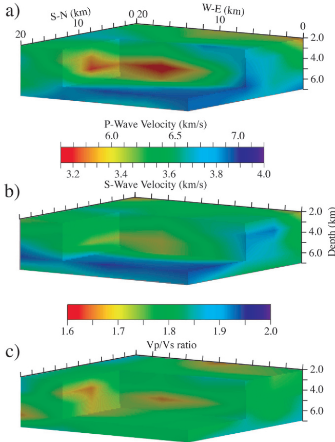
Figure 3.7. A three-dimensional view of velocities below a 20 \times 20 km rectangular area of the Hengill volcanic complex at the western end of the SISZ. Because of the higher microseismic activity below this area, resolution is better than in the adjacent SISZ as a whole (as demonstrated in Figure 3.6). Spatial variations of P , V_p , are shown in (a), S velocities in (b), and the V_p/V_s ratio in (c). The greater reduction in P velocity than S velocity is well demonstrated in the velocity ratios. The view is from the northwest (from Tryggvason et al. , 2002).
