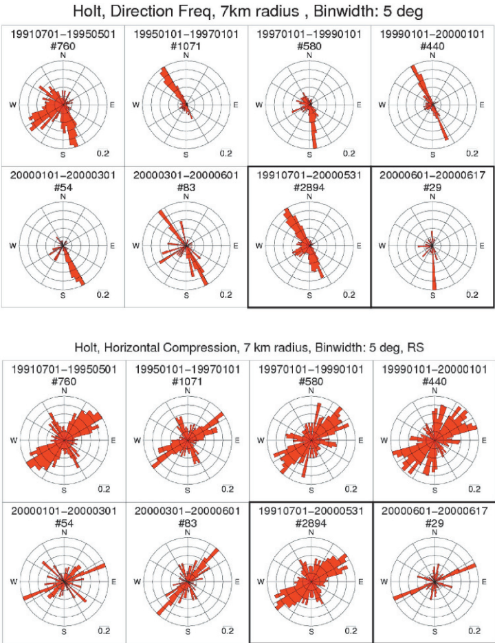
Figure 4.19. ( Upper ) Rose diagrams expressing the frequency of directions of micro-earthquakes as seen from the hypocenter of the developing June 17 earthquake. The first six diagrams are for various periods from 1991 to June 1, 2000. The diagrams inside the dark frames denote, respectively, the frequency of directions for the whole period and the frequency of directions during the last 16 days before the June 17 earthquake, when they were very close to the NS fault plane. ( Lower ) The frequency of horizontal compressions (HC) calculated from the fault plane solutions of individual micro-earthquakes. The HCs calculated here are by definition 45^\circ from fault planes. The first six diagrams are for various periods from 1991 to June 1, 2000. The last two (in the dark frames) denote respectively the whole period and the last 16 days before the June 17 earthquake. For most of the time HCs strike 50\text{--}55^\circ east from north. During the last period a 65\text{--}70^\circ strike is most frequent. So a rotation of around 15^\circ to the right is seen in the fault planes of the micro-earthquakes when they move above the main fault. This could possibly express en echelon cracks, striking 15^\circ —above and oblique to the 5^\circ east-of-north strike-slip—on the deeper part of the main fault (modified from Stefánsson and Gudmundsson, 2005). Each rose involves a 5^\circ angle, 0.2 is the fraction of the radius length in the diagrams, and # indicates the number of earthquakes used in the solution.
