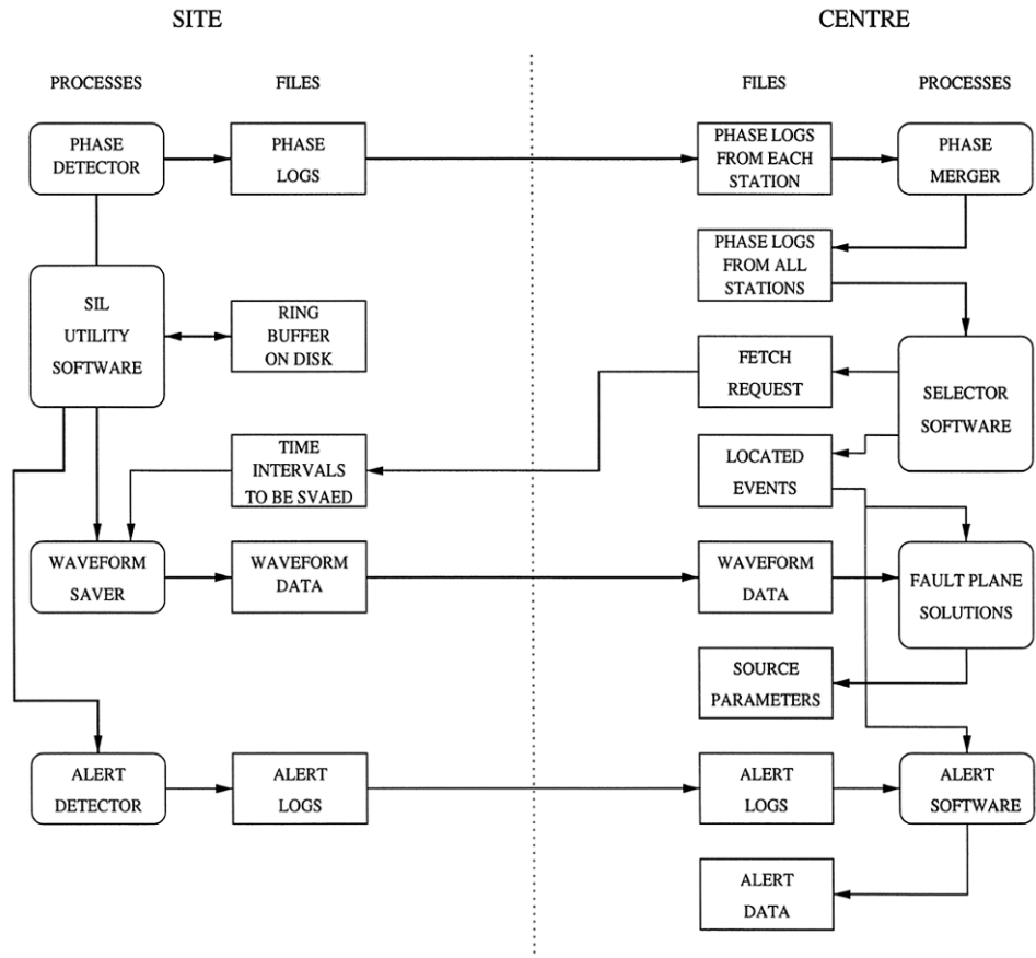
Figure 3.10. Flow chart of SIL processing. A phase detector in the computer at a remote seismic station produces phase logs that are transferred to the center. At the center a program merges phases from all stations into one file which is input to the “selector” software. The selector software defines the possible seismic events of earthquakes through a phase association procedure and determines time intervals of waveform data to be retrieved from the remote stations. At the remote stations a net saver program copies the data from the ring buffer system to local files and transfers them to the center. The alert software works in parallel with the acquisition system using information from the selector software and from the alert detector at each site (from Bóðvarsson et al. , 1999).
