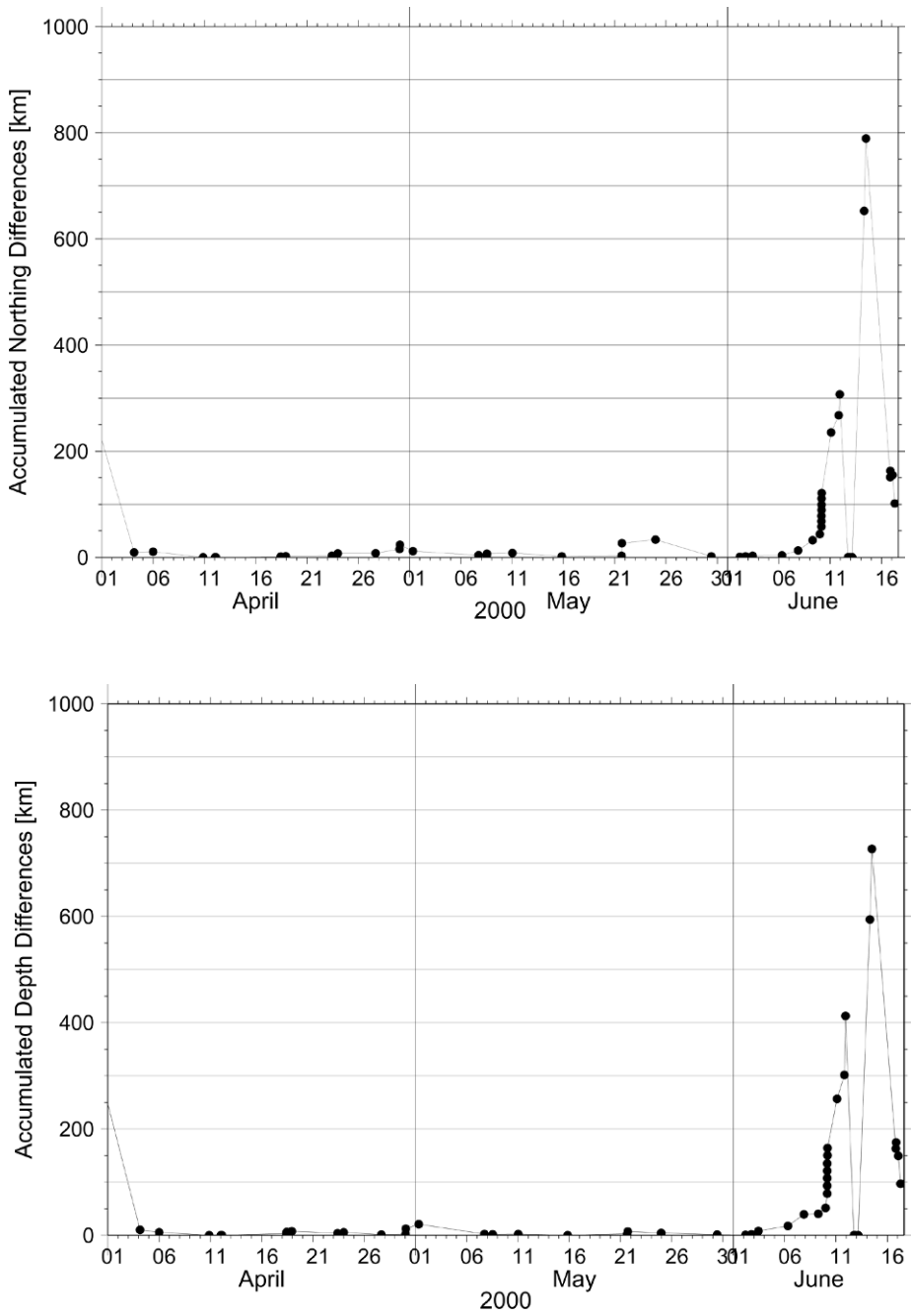
Figure 4.23. Same as Figure 4.22 , but here the cumulative sums have been normalized by dividing by the number of micro-earthquakes in a 20 km wide strip outside the 5 km wide fault strip (i.e., normalized by the surrounding background seismicity).
