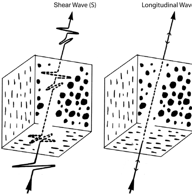
Figure 4.30. ( Left ) A seismic shear wave comes from below and through a cube that has many fluid-filled cracks. Wave motion is perpendicular to the ray path. It splits into a faster and a slower component because the velocity in different directions in the cube varies. Stress applied from outside deforms the cracks, makes them fatter or thinner, and thus changes the time difference between the two components. ( Right ) A longitudinal wave, a P -wave, goes through the cube. Its wave motion is along the ray path, as indicated by small back and forth arrows, and thus it does not split up. Therefore, a P -wave is not as useful as a shear wave at sensing stress-induced velocity changes in its wave path.
