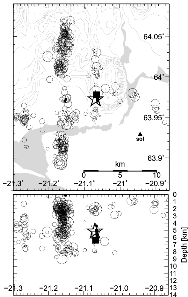
Figure 4.35. ( Upper ) A geographic view of the area where the May 2008 earthquake occurred (see for comparison Figure 4.34 ). The gray parts show the ocean in the south and the Ölfusá river flowing toward it. The earthquake occurred near the western end of the SISZ on two main faults which are shown by two north–south rows of mainly small aftershock epicenters. ( Lower ) An east–west cross-section at various depths of their sources. Circles are aftershocks in the two days following the earthquake, while squares are foreshocks one day before it. Foreshocks occurred almost entirely at the hypocenter of the earthquake, which is marked by a star obscuring the foreshocks. The north–south fault where the earthquake started (i.e., the eastern fault) was indicated as 9 km long by the aftershocks. The western fault, which started to slip just a few seconds after the first, is 4 km farther west and is 20 km long. The long fault could be considered two or three different faults, but as they are almost in the same north–south direction, I prefer to regard them as three segments of the same western fault. Some earthquakes on an old north–south fault even farther west are probably not part of the earthquake itself, rather they should be considered as being triggered by it.
