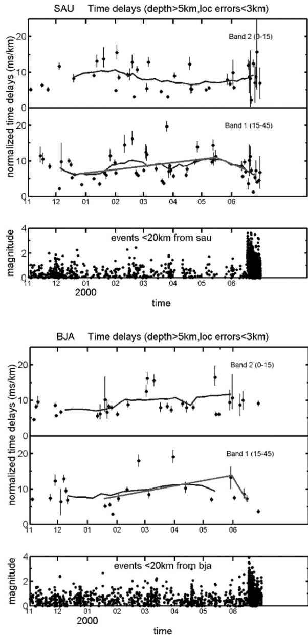
time delays in Band 1 showing the time trend of SWS time delays interpreted as stress accumulation. Station SAU (a) is within a few kilometers of the epicenter of the initial 2000 earthquake and (b) BJA is within 50 km. The bottom panels are the magnitudes of small earthquakes within 20 km of each station. Increased seismic activity marks the onset of the June 17, 2000 earthquake. A couple of weeks before the large earthquake occurred, the Band 1 trace in both panels indicated stress relaxation (called by the author, crack coalescence).
