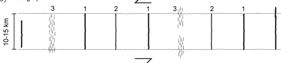
Figure 6.2. (a) The distribution of micro-earthquakes before large earthquakes at places labeled 2, resembling the real seismicity in the SISZ from 1991 to 2000 before the large 2000 earthquakes (Chapter 4). (b) The situation in the future long after the earthquakes. The high pore fluid pressures (at 2) around the epicenters have been released, but areas of renewed microearthquake activity (3) have been created, reflecting renewed buildup of high pore fluid pressures at new places in response to steadily ongoing plate motion.
