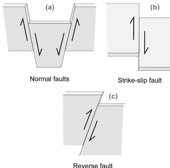
Figure 2.5. The main types of earthquake faults. (a) Normal fault shown in cross-section through the crust, typical direction of faults in tensional regions like rift zones (such as those in Iceland). Normal faults, at 45^\circ slope from the surface as in the figure, prevail where the vertical stress component is larger than the horizontal components of stress, and the fault is created between the maximum stress, the vertical stress, and the minimum horizontal stress across the fault (this is frequently described as horizontal tension in the direction of the lowest stress). (b) Strike slip fault (horizontal view), vertical fault in the figure, is created where both the largest and the smallest stress components are horizontal. Strike slip faults are typical of nearly vertical boundaries of plates which slip horizontally towards each other, such as the transform faults or transform zones that are found in the main earthquake zones in Iceland. The slip shown by the arrows is right-lateral, indicating that if you stand at one side of the fault you see the other side move to the right. This is also often named “dextral”. The opposite slip would be left-lateral also often named “sinistral”. (c) Reverse fault , as demonstrated in the figure, both horizontal components of stress are larger than the vertical, typical of the thrust faulting that occurs at plate collision, such as in the Himalayas and subduction of ocean crust below the continental crust.
