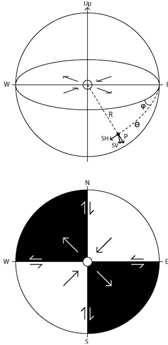
Figure 2.6. The focal sphere. P -waves oscillating along the ray of the wave ( R ) and cause push or pull on the surface. The amplitudes of the two components of the S -wave are indicated in the figure (i.e., the S_H that is perpendicular to the ray R from the source and along the surface, and the S_V component that is perpendicular to R and along the plane that the ray has with the vertical). Observations are plotted on the surface of the focal sphere after they have been corrected for ray path effect at a point that has spherical coordinates \varphi and \theta . The circle below denotes the stereographic projection of the lower part of the focal sphere on the horizontal surface. White denotes areas where the pull of P is observed, while black denotes areas where the push of P is observed. Nodal planes are between these areas. This is a simple case where both nodal planes are vertical, and thus they are presented as straight lines in this projection.
