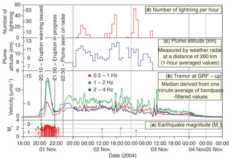
Figure 7.4. Signals shortly before the eruption and following it. Time is Universal Time Coordinated. Micro-earthquakes originating from the volcano and tremors at the closest seismic station (GRF) are shown in the two bottom rows. Height of ash plume and number of eruption-related lightning flashes are shown in the two upper rows (Vogfjörð et al. , 2005).
