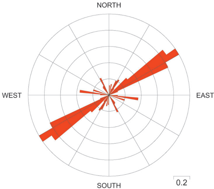
Figure 4.38. A rose diagram of the frequency of horizontal compressions in the fault plane solutions of each of the 39 foreshocks an hour before the earthquake. Frequency is counted within an angle of 15^\circ . The main direction is very stable at around 59^\circ east of north. This implies that almost all foreshocks had slips along small fault segments striking 14^\circ east of north.
