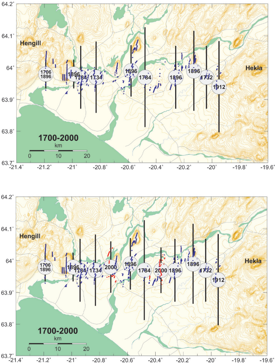
Figure 4.7. Earthquakes in the SISZ since 1700: (a) before the 2000 earthquakes and (b) where both the 2000 earthquakes are included. The earthquakes are arranged side by side and have right-lateral slip on north–south faults. Fault epicenters and magnitudes (Stefánsson et al. , 1993; Clifton and Einarsson, 2005) are estimated from historical data, and fault lengths are from Roth (2004).
