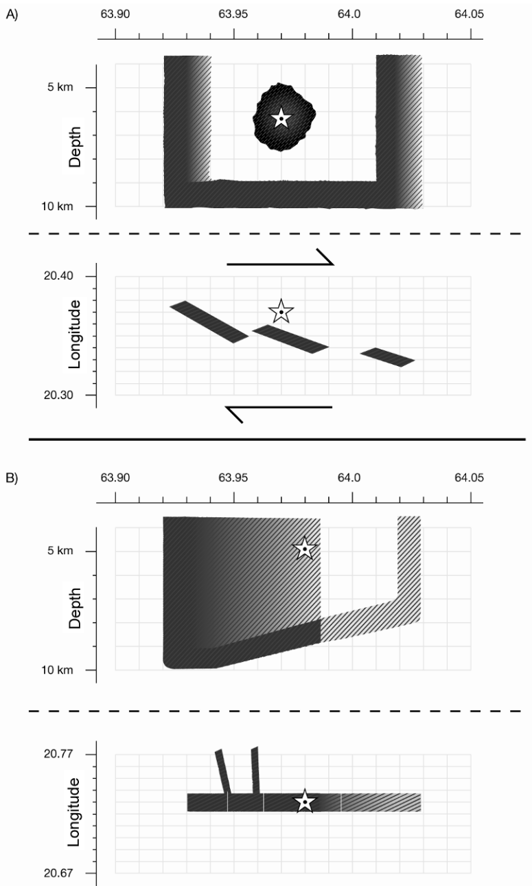
Figure 4.4. Some features of the two faults (black means dense seismic activity, gray and white less activity): A) is the June 17, 2000 earthquake fault, and B) the June 21, 2000 fault, in vertical (resp. horizontal) view, as expressed by the distribution of aftershocks (Figures 4.2 and 4.3). Comparison has also been made with deformation modeling and modeling based on strong motion data (as expressed in Figure 4.2).
