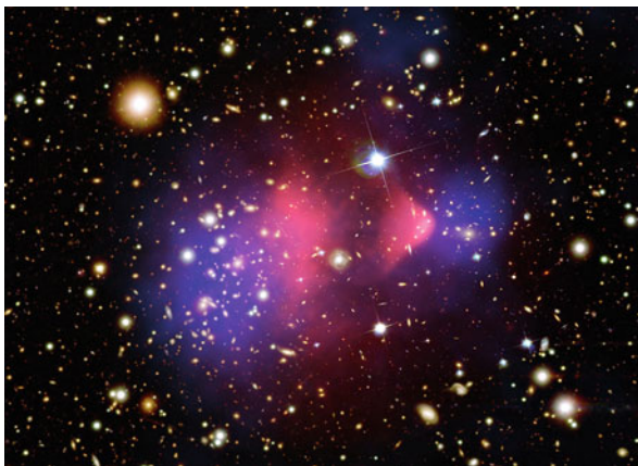
Fig. 5.22 The Bullet cluster. This composite optical and X-ray image reveals the locations of dark matter ( diffuse light grey ) and hot gas ( dark grey at image center ) after two galactic clusters have collided. (Image courtesy of NASA)
