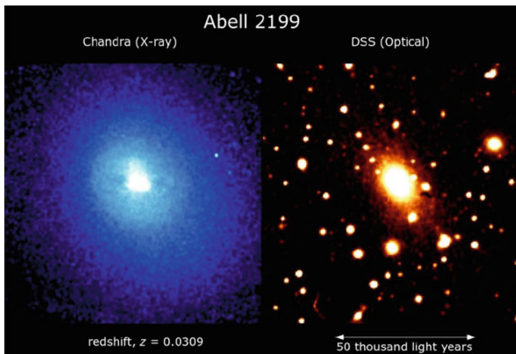
Fig. 4.10 Chandra spacecraft X-ray image ( left ) of the cluster Abell 2199. The strong X-ray emission indicates that the intracluster medium is very hot, with a temperature of millions of degrees. A detailed comparison of the Chandra X-ray data with the optical data ( image to the right ) indicates that most of the cluster’s baryonic mass is in the intracluster gas rather than in the visible stars. (Image courtesy of NASA)
