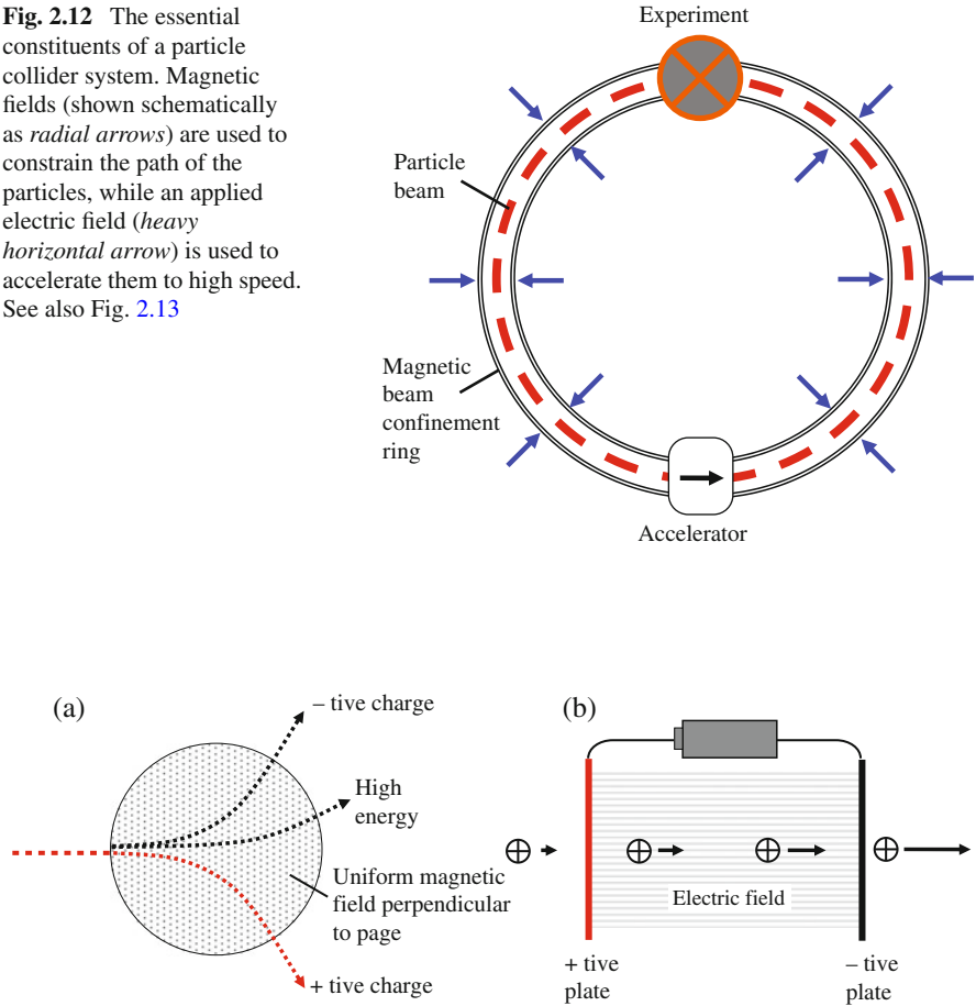
Fig. 2.13 (a) The effect of a magnetic field upon the motion of a charged particle. Positively charged particles will have paths curved in the opposite direction to negatively charged ones, and the greater the energy of the particle the smaller is its curvature. In this diagram the magnetic field is imagined to be coming out of the page towards the reader. (b) The particle accelerating effect of an electric field. The arrow length indicates the increasing speed of the particle
