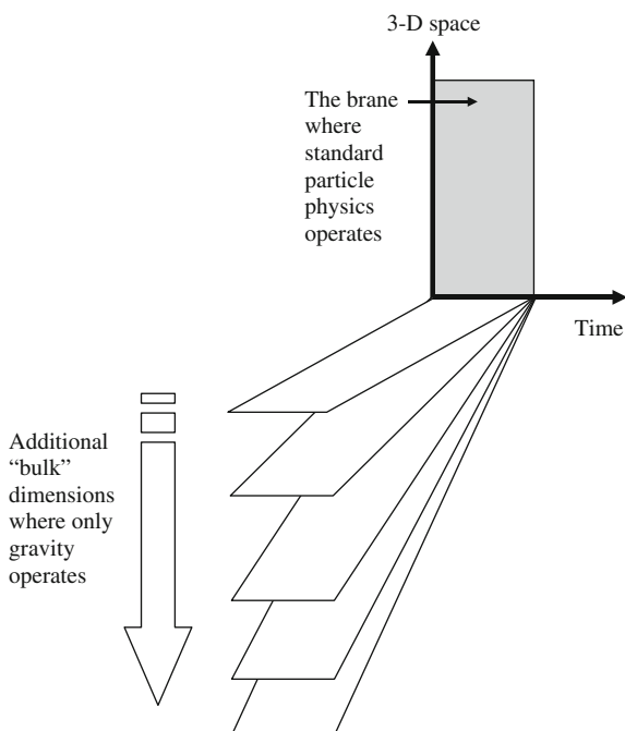
Fig. 7.15 A schematic, minds-eye, view of the idea behind extra dimensions. The vertical ( shaded ) plane is “the brane,” and this is where you and I live and experience the world, and it is also where experimental physics can be performed. The additional planes represent the “bulk” dimensions over which gravity operates. Note that the compaction and curvature of the bulk dimensions are not illustrated in this diagram
