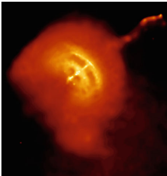
Fig. 7.4 Chandra X-ray satellite image of the Vela pulsar. The neutron star located at the core of this supernova remnant is spinning once every 89 ms. (Image courtesy of NASA)
