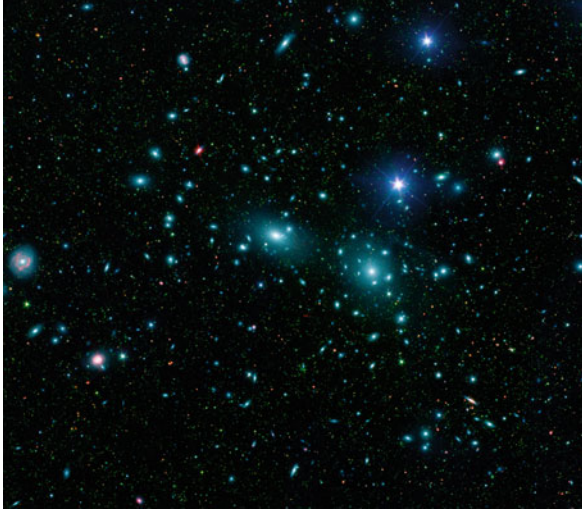
Fig. 5.9 The Coma cluster of galaxies is situated some 321 million light years distant from us and contains over 1,000 galaxies. (Image courtesy of NASA)
