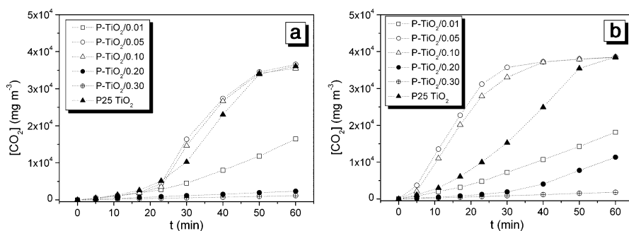
Fig. 12.13 Formation of \text{CO}_2 on bare (Degussa P25) and P- \text{TiO}_2 samples as a function of irradiation time at an initial relative humidity of (a) 0% and (b) 74% [46]
