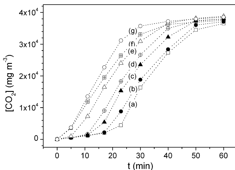
Fig. 12.15 Kinetic curves of \text{CO}_2 formation on P-TiO 2 /0.05 at different initial relative humidities: (a) 0%, (b) 12%, (c) 25%, (d) 37%, (e) 49%, (f) 62%, and (g) 74% [46]
