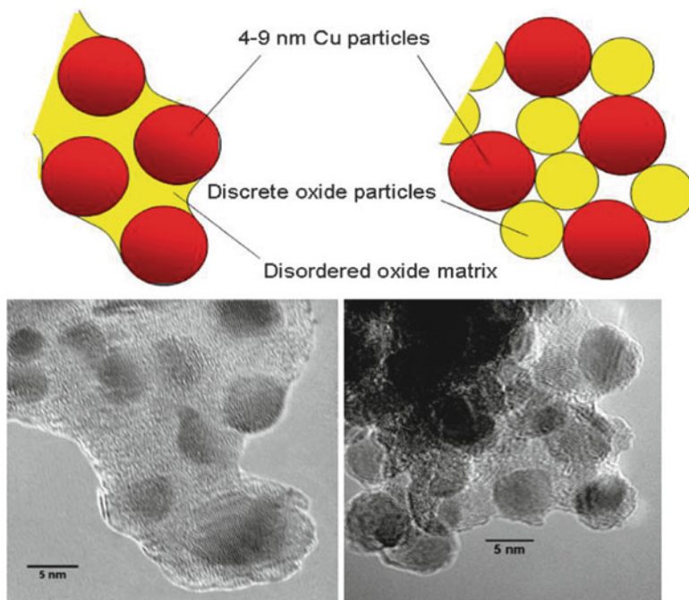
Fig. 5.4 Scheme and TEM micrographs of the microstructure of differently prepared Cu/ZnO/Al 2 O 3 catalyst with the same composition and similar Cu particle sizes; adapted from [42]
