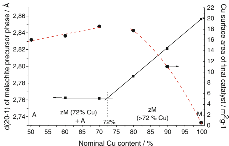
Fig. 5.6 Lattice contraction in the direction perpendicular to the (20\bar{1}) planes of zincian malachite as a measure of Zn incorporation in the precursor phase and \text{SA}_{\text{Cu}} of the final Cu/ZnO catalyst as a function Cu content (phase composition: M malachite, zM zincian malachite, A aurichalcite); adapted from [66]
