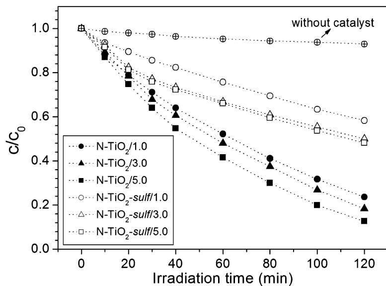
Fig. 12.19 Phenol degradation curves under UV-rich illumination using different N-doped \text{TiO}_2 catalysts [47]
