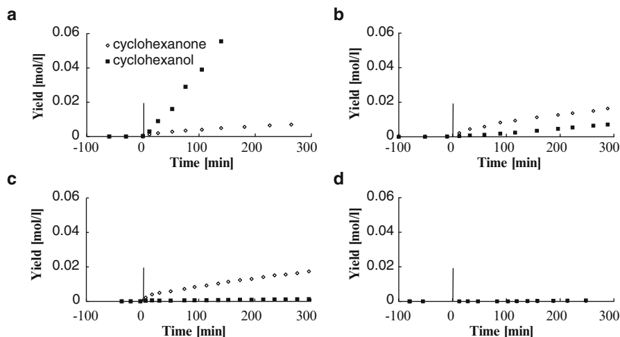
Fig. 13.9 Effect of the experimental conditions on the cyclohexanone and cyclohexanol amounts produced over Hombikat TiO 2 in photocatalytic oxidation of cyclohexane. (a) Quartz reactor, no catalyst (pure photolysis); (b) Quartz reactor, with catalyst (1 g/l of TiO 2 , combination of photolysis and photocatalysis); (c) Pyrex reactor with catalyst (1 g/l of TiO 2 , excluding photolysis); and (d) Pyrex reactor, no catalyst. Light was switched on at t = 0 min [14]
