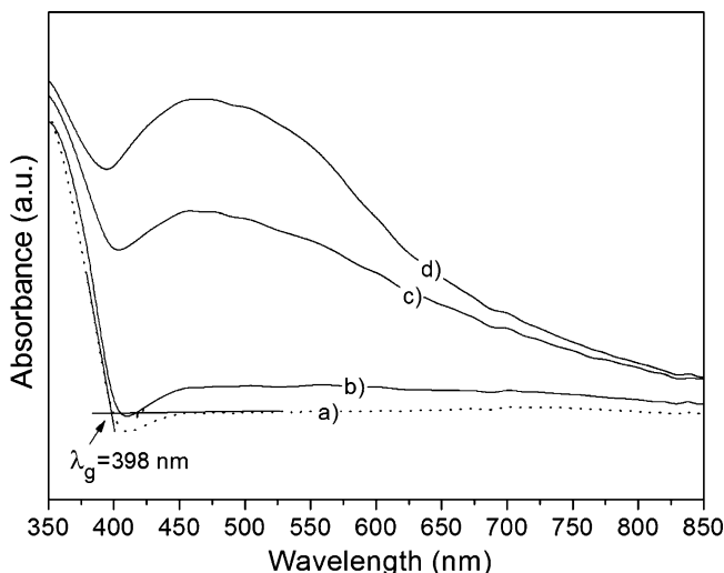
Fig. 12.22 Diffuse reflectance UV-Vis spectra of (a) unmodified P25 \text{TiO}_2 (b) \text{Ag-TiO}_2/0.1 wt%, (c) \text{Ag-TiO}_2/0.5 wt%, and (d) \text{Ag-TiO}_2/1.0 wt% [11]
