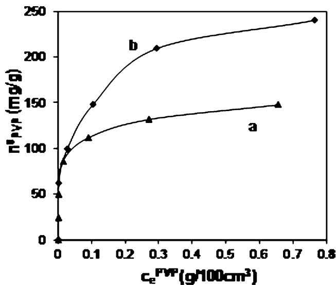
Fig. 11.32 Adsorption isotherms of (a) PVP (b) PVP-protected Pd NPs in aqueous solution on Na montmorillonite (see [59])
