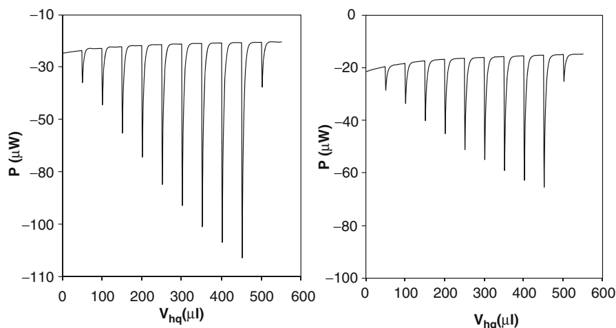
Fig. 11.11 (a) Typical enthalpogram of the formation of Ag NPs, [Ag^+]/[hq] = 14 ( 10 \times 50 \mu\text{l} 1 mM hydroquinone solution is added to 1.75 \text{ cm}^3 4 mM AgNO_3 and 0.25 \text{ cm}^3 10 mM Na citrate) (see [41]). (b) Typical enthalpogram of the mixing of the components ( 10 \times 50 \mu\text{l} 1 mM hydroquinone solution is added to 1.75 \text{ cm}^3 water and 0.25 \text{ cm}^3 10 mM Na citrate) (see [41])
