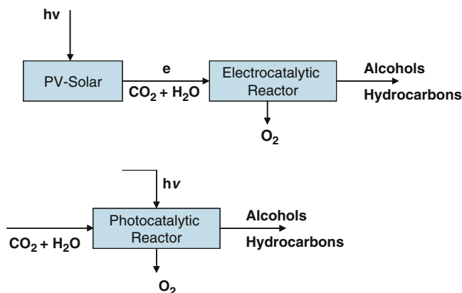
Fig. 13.1 Process options for artificial photosynthesis. ( Top ) Photovoltaic conversion of light into electricity, followed by electrocatalytic fuel generation. ( Bottom ) Photocatalytic process, which requires only one reactor and allows for gas-phase process operation
