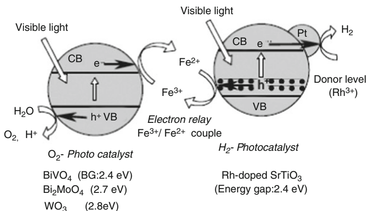
Fig. 13.5 Representation of a Z-scheme process, mediated by the Fe 2+ /Fe 3+ couple. Over oxides such as BiVO 4 , Bi 2 MoO 4 , and WO 3 O 2 evolution is thermodynamically feasible, while Rh 3+ -doped, Pt-promoted SrTiO 3 is very effective in visible-light-induced H 2 evolution. Copied from [35]
