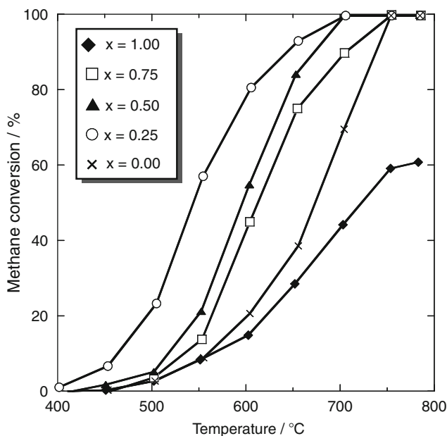
Fig. 8.8 Light-off curves over \text{Ce}_{1-x}\text{Zr}_x\text{O}_2 mixed oxide catalysts prepared via sol-gel technique with aging time = 50 h calcined at 500^\circ\text{C} . Gas mixture contains 2.0% \text{CH}_4 , 21.0% \text{O}_2 , and balance He. Total flow 100 ml/min [44]
