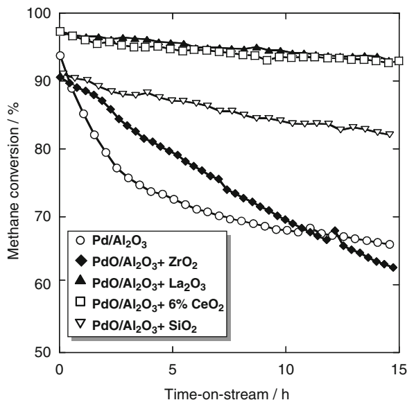
Fig. 8.4 Influence of promoters on catalyst durability—conversion versus time on stream [32]
