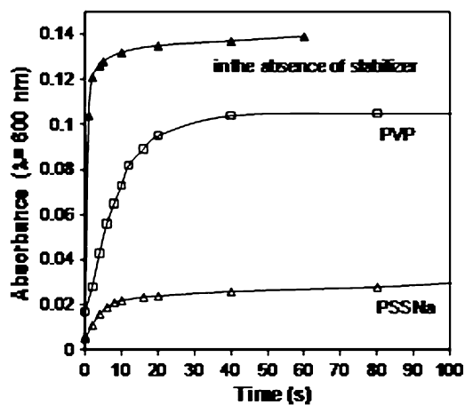
Fig. 11.3 Absorbance ( \lambda = 600 nm) versus time curves of Pd NPs stabilized by PVP and PSSNa ( c_{\text{stabilizer}} = 0.5 g/100 \text{cm}^3 and c_{\text{Pd}^{2+}} = 0.038 mmol/dm ^3 ) (see [52])
