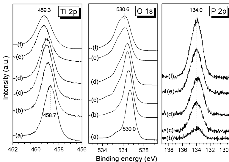
Fig. 12.4 High-resolution XP spectra of the Ti 2p , O 1s , and P 2p regions on (a) Degussa P25, (b) P- \text{TiO}_2/0.01 , (c) P- \text{TiO}_2/0.05 , (d) P- \text{TiO}_2/0.10 , (e) P- \text{TiO}_2/0.20 , and (f) P- \text{TiO}_2/0.3 [46]
