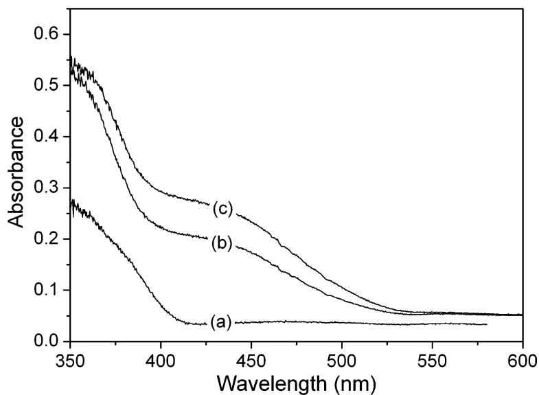
Fig. 12.18 Diffuse reflectance UV-Vis spectra of (a) nondoped \text{TiO}_2 , (b) \text{N-TiO}_2/1.0 , and (c) \text{N-TiO}_2/5.0 [47]
