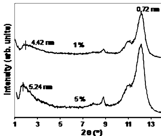
Fig. 11.34 XRD patterns of 1 and 5 wt% Ag/kaolinite prepared by photochemical reduction (see [60])
