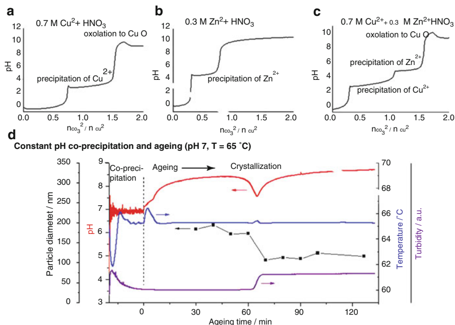
Fig. 5.5 Precipitation titration curves relevant for the co-precipitation of Cu/ZnO/ \text{Al}_2\text{O}_3 catalyst precursors at 338 K using aqueous \text{Na}_2\text{CO}_3 as precipitation agent (a–c, adapted from [65]); preparation log of corresponding constant pH co-precipitation (d), adapted from [66]
