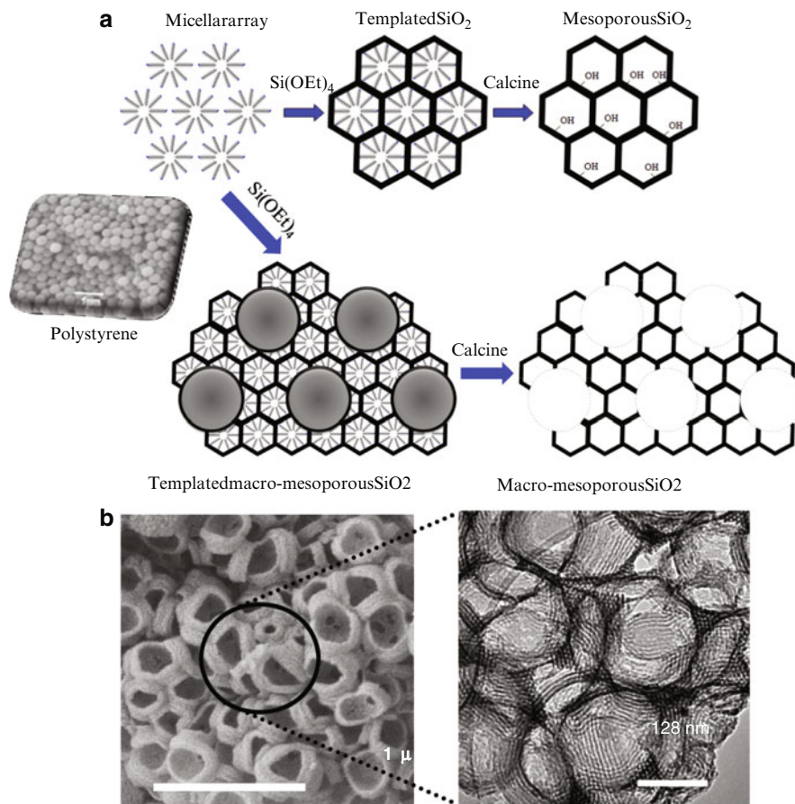
Scheme 7.8 (a) Liquid crystal templating route to form mesoporous silica and combined physical templating method using polystyrene microspheres to introduce a macropore network; (b) SEM of macroporous–mesoporous SBA-15 showing macropore network and TEM showing interconnecting mesopores
