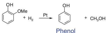
Scheme 7.24 Model reactions to study bio-oil upgrading [207]
