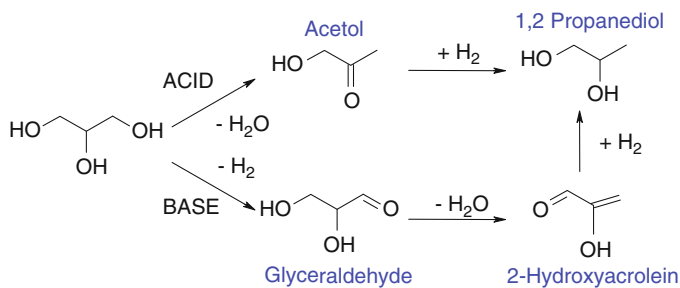
Scheme 7.15 Effect of acid or basic conditions on hydrogenolysis pathways
