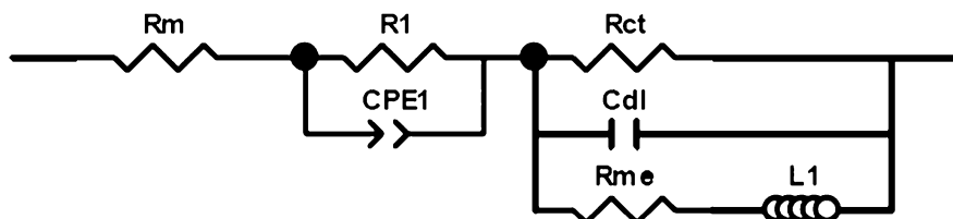
Fig. 10.9 Equivalent circuit (EQC) for the CH 3 OH oxidation reaction in the anode layer of a DMFC
