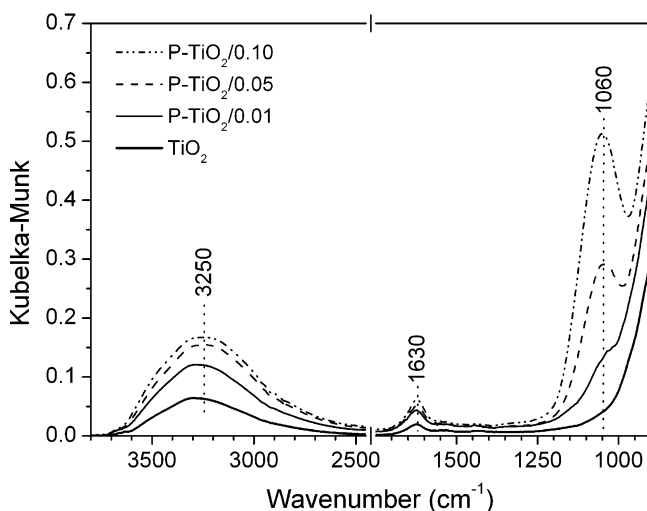
Fig. 12.3 DRIFT spectra of pure \text{TiO}_2 and different P- \text{TiO}_2 samples [52]
