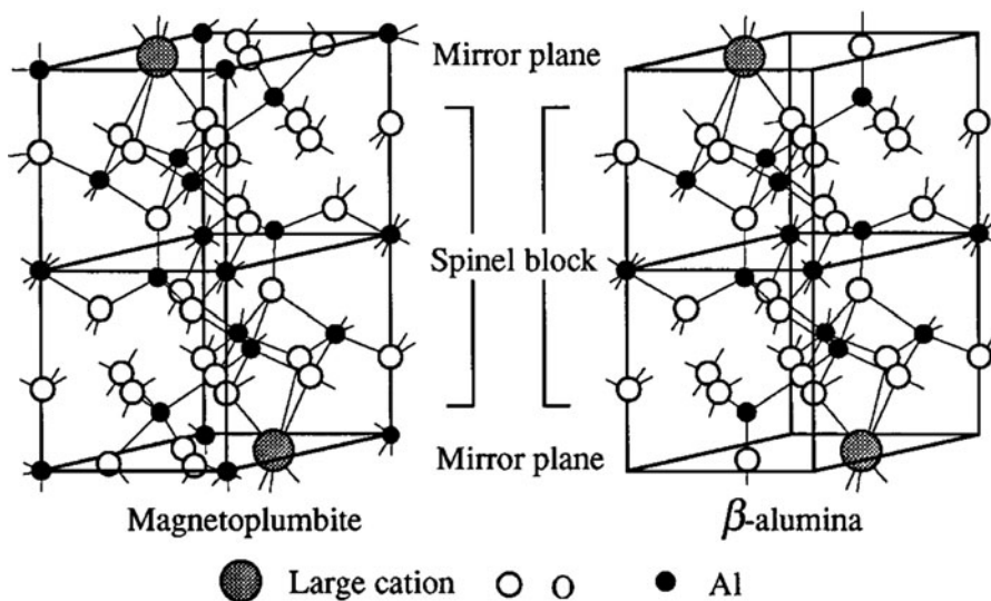
Fig. 8.11 Crystal structure of magnetoplumbite and \beta -alumina [79]
