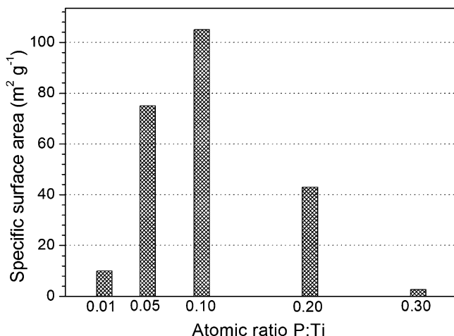
Fig. 12.7 Effect of phosphate modification on the specific surface area of \text{TiO}_2 [46]
