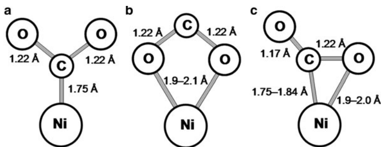
Fig. 3.6 Schematic representation of the three coordination geometries of adsorbed CO 2 : (a) pure carbon coordination, (b) pure oxygen coordination, (c) mixed carbon–oxygen coordination. CO 2 coordination modes and indicated structural parameters from Reprinted with permission from reference [81]. Copyright (1986) by Elsevier
