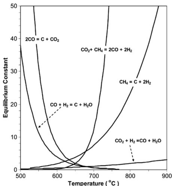
Fig. 3.5 Equilibrium constants of reactions occurring during the dry reforming of methane, as a function of temperature Reprinted with permission from reference [61]. Copyright (2007) by Elsevier
