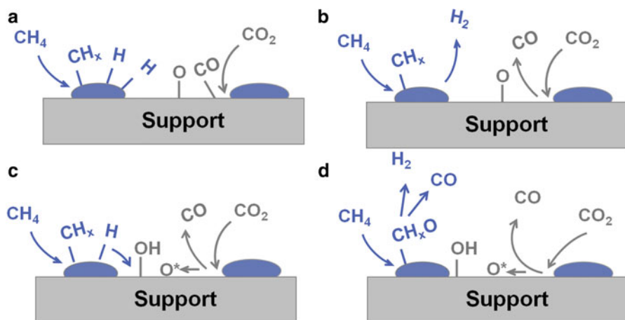
Fig. 3.7 Reaction steps for the dry reforming of methane. (a) Adsorption and dissociation of \text{CH}_4 and \text{CO}_2 on the metal and the metal–support interface, respectively. (b) \text{CO} and \text{H}_2 desorption are fast steps. (c) Surface hydroxyls are formed from hydrogen and oxygen spillover. (d) Surface oxygen species or hydroxyls oxidize the hydrogen-depleted surface methyl-like species ( \text{S}_1\text{--CH}_x ), forming \text{S}_1\text{--CH}_x\text{O} species and finally \text{CO} and \text{H}_2
