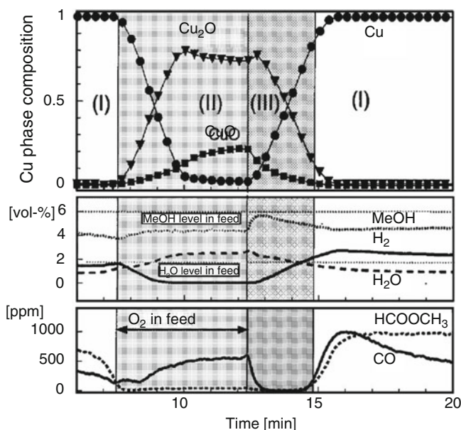
Fig. 5.8 Evolution of Cu phase composition of a Cu/ZnO catalyst during oxygen addition cycles into steam reforming feed at 523 K. Phase analysis was based on the corresponding X-ray absorption near edge structure (XANES) spectra. The two lower sections of the graph depict the evolution of the gas-phase in percent and ppm, respectively. Three transitions in bulk and gas-phase composition are marked: (I) copper metal during steam reforming, (II) oxidation of Cu, (III) and re-reduction of Cu oxide. Reprinted from [118] with permission from Elsevier
