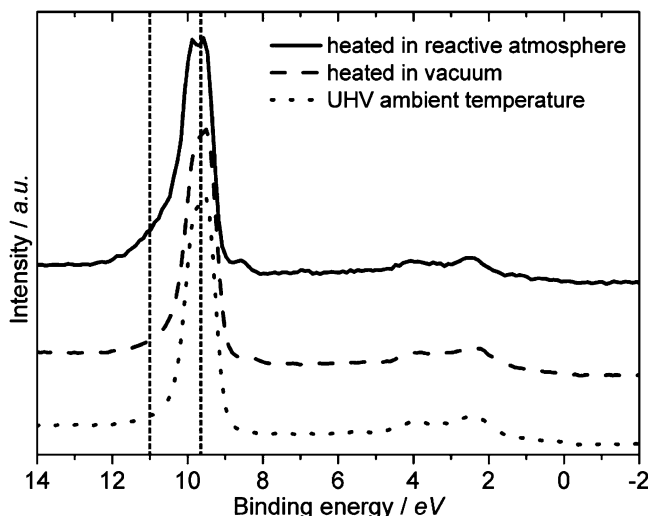
Fig. 5.18 XPS valence band spectra of ZnPd: UHV conditions at ambient temperature ( dotted line ), in situ after heating to 573 K in UHV and subsequent switching to reactive atmosphere (0.2 mbar methanol/H 2 O at a 1:1 ratio, dashed line ), and in situ after heating to 573 K in reactive atmosphere ( full line ). Photon energy is set to 237 eV for all spectra
