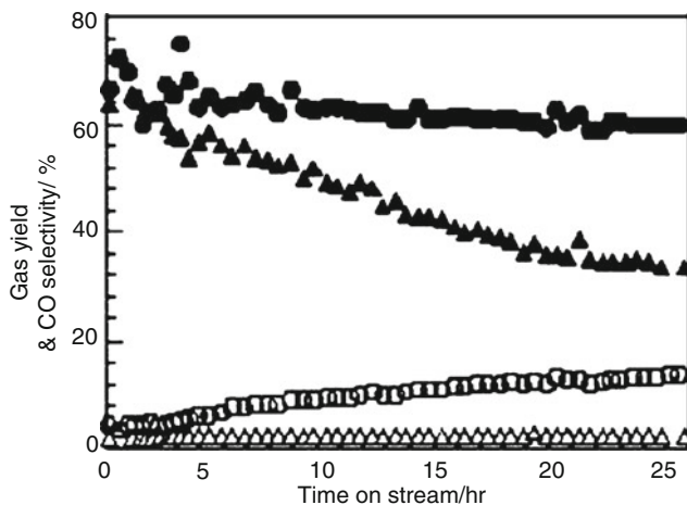
Fig. 5.14 Activity (solid symbols) and CO selectivity (open symbols) of Pd/ZnO (circles) and a commercial Cu/ZnO catalyst (triangles). Reprinted from [170], Copyright 2006, with permission from Elsevier
