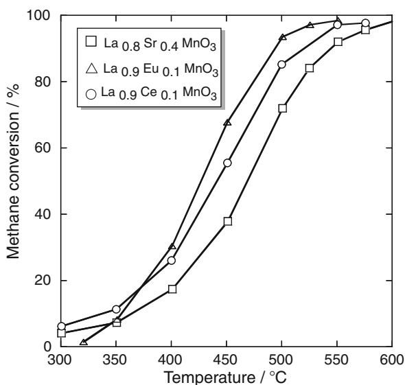
Fig. 8.9 Activity comparison data under standard reaction conditions [62]
