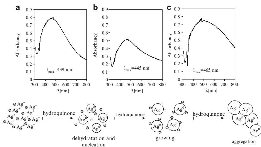
Fig. 11.15 Schematic picture and UV-Vis spectra of the formation of Ag NPs (a) [\text{Ag}^+]/[\text{hq}] = 14 , (b) [\text{Ag}^+]/[\text{hq}] = 21 , and (c) [\text{Ag}^+]/[\text{hq}] = 35 (see [41])
