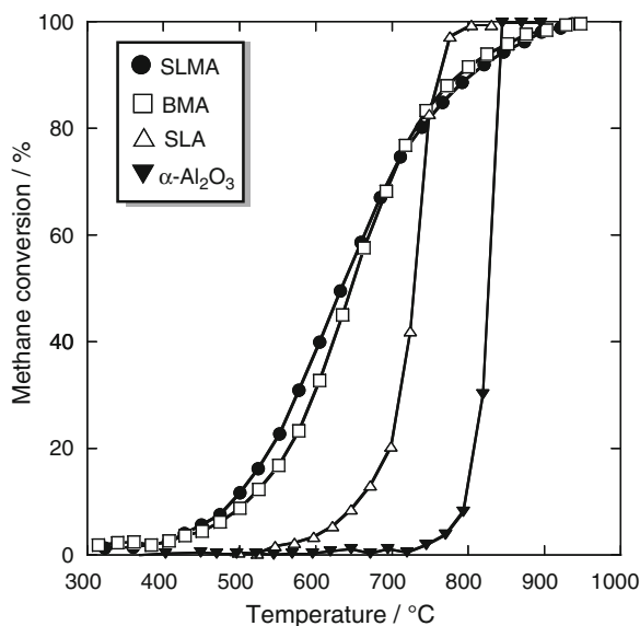
Fig. 8.12 Catalytic combustion of methane over hexaaluminate materials and \alpha - \text{Al}_2\text{O}_3 : (filled circle) \text{Sr}_{0.8}\text{La}_{0.2}\text{MnAl}_{11}\text{O}_{19-\alpha} prepared via alkoxide hydrolysis (SLMA); (open square) \text{BaMnAl}_{11}\text{O}_{19-\alpha} (BMA); (open triangle) \text{Sr}_{0.8}\text{La}_{0.2}\text{Al}_{12}\text{O}_{19-\alpha} (SLA); and (filled inverted triangle) \alpha - \text{Al}_2\text{O}_3 . Reaction conditions: \text{CH}_4 , 1 vol.%; air 99 vol.%; space velocity: 48,000 \text{ h}^{-1} [82]
