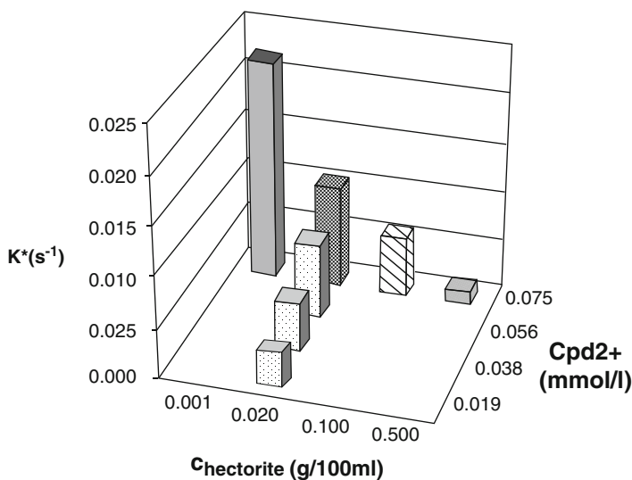
Fig. 11.20 Rate constants at different hectorite and precursor concentration (see [52])
