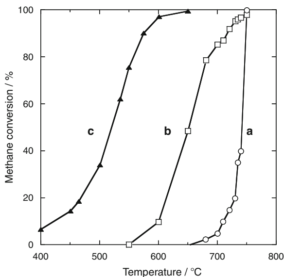
Fig. 8.13 Catalytic methane combustion experiments. Catalytic methane oxidation activity: (a) sol-gel-derived conventional BHA, (b) reverse microemulsion-derived BHA nanoparticles, (c) reverse microemulsion-derived \text{CeO}_2 -BHA nanocomposite. The reactant stream consisted of 1 vol.% \text{CH}_4 in air; space velocity: 60,000 \text{ h}^{-1} [86]
