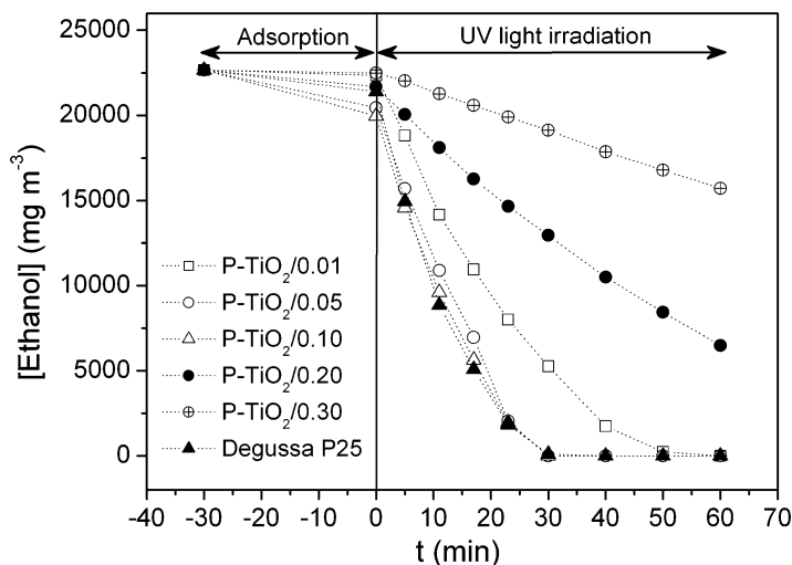
Fig. 12.11 Photodegradation of ethanol on Degussa P25 TiO 2 and various P-TiO 2 samples under dry initial conditions [46]
