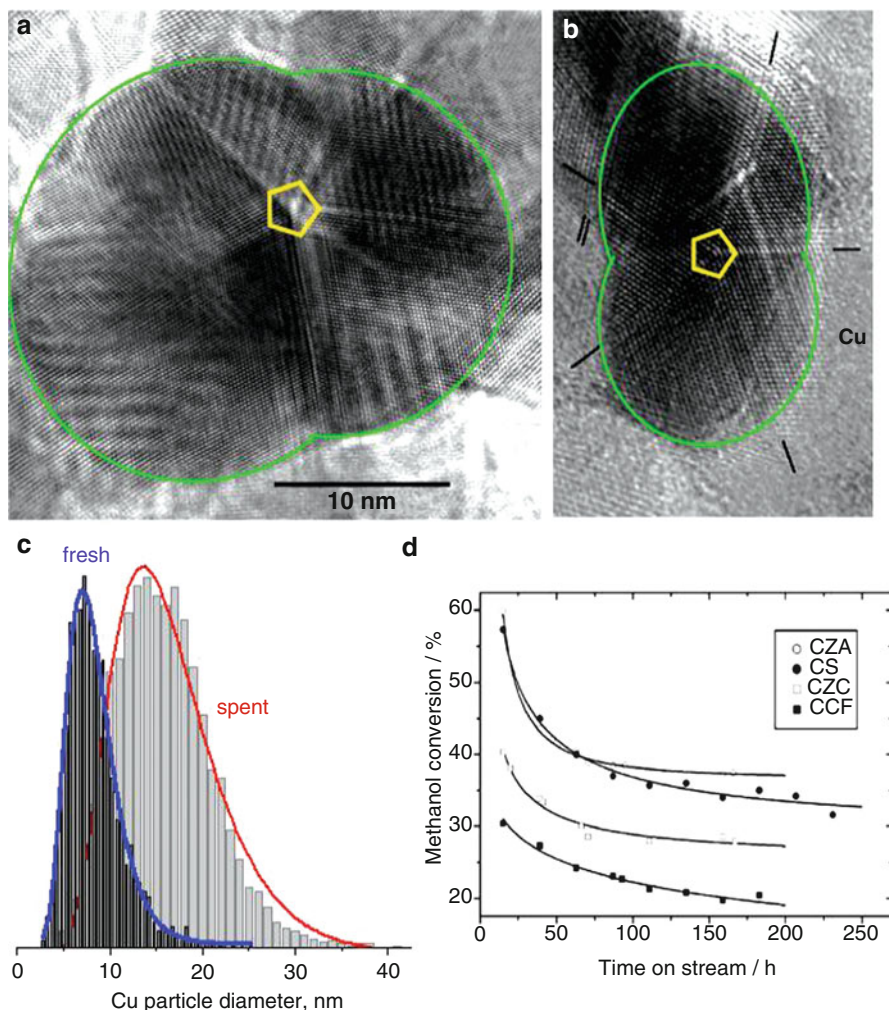
Fig. 5.3 HRTEM images of Cu/ZnO/Al 2 O 3 catalyst used in methanol synthesis (a and b); evolution of the particle size distribution during reaction (c); and loss in methanol conversion with time on stream for different Cu-based catalysts during MSR at 493 K, 1 bar, MeOH:H 2 O = 1:1 (d, CZA: 0.5 g Cu/ZnO/Al 2 O 3 , CS: 2.0 g Cu/SiO 2 , CZC: 1.0 g Cu/ZrO 2 /CeO 2 , CCF: 2.5 g Cu/Cr 2 O 3 /Fe 2 O 3 , reprinted from [37] with permission from Elsevier)
