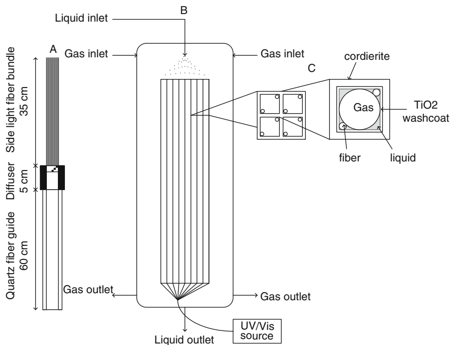
Fig. 13.10 Scheme of the internally illuminated monolith reactor setup, consisting of a ceramic monolith with square channels, on the walls of which the catalyst ( \text{TiO}_2 ) is coated and in which two optical fibers are inserted and located in the corners of the channels. The detail shows the construction of the optical fiber bundle
