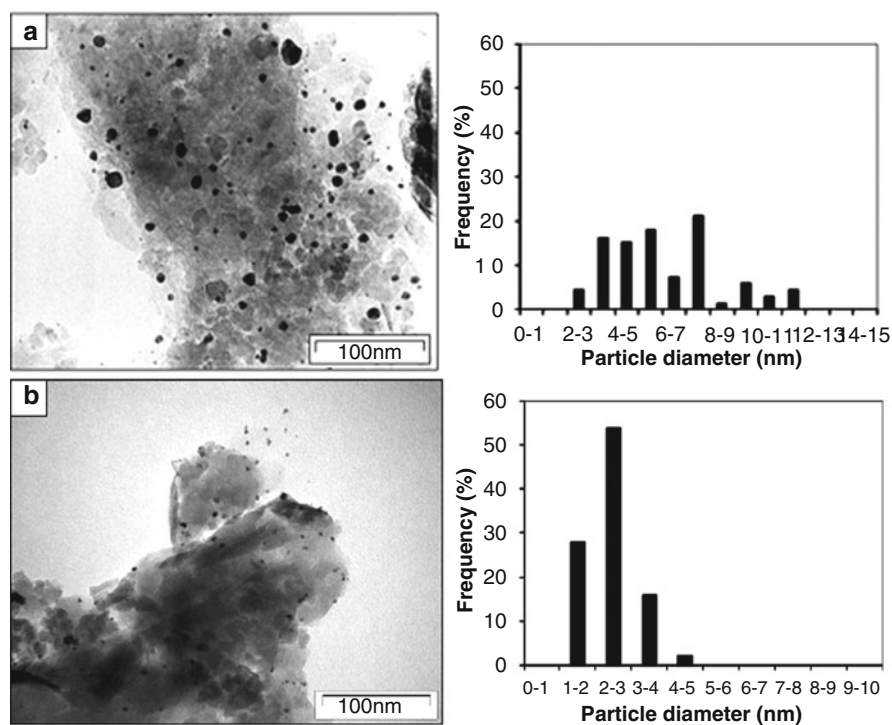
Fig. 11.28 TEM micrograph and size distribution of Pd/montmorillonites (a) PVPPdM1, d_{\text{ave.}} = 5.9 nm, and (b) PVPPdM4, d_{\text{ave.}} = 2.8 nm (see [49])
