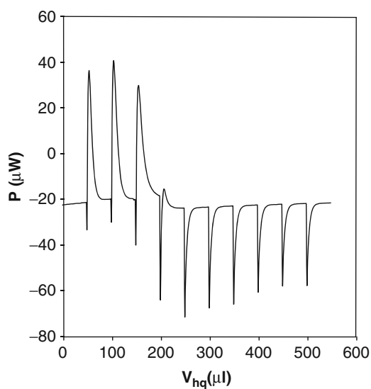
Fig. 11.12 Enthalpogram of the formation of larger, aggregated NPs, [Ag^+]/[hq] = 0.875 ( 10 \times 50 \mu\text{l} 40 mM hydroquinone solution is added to 1.75 \text{ cm}^3 10 mM AgNO_3 and 0.25 \text{ cm}^3 10 mM Na citrate) (see [41])
