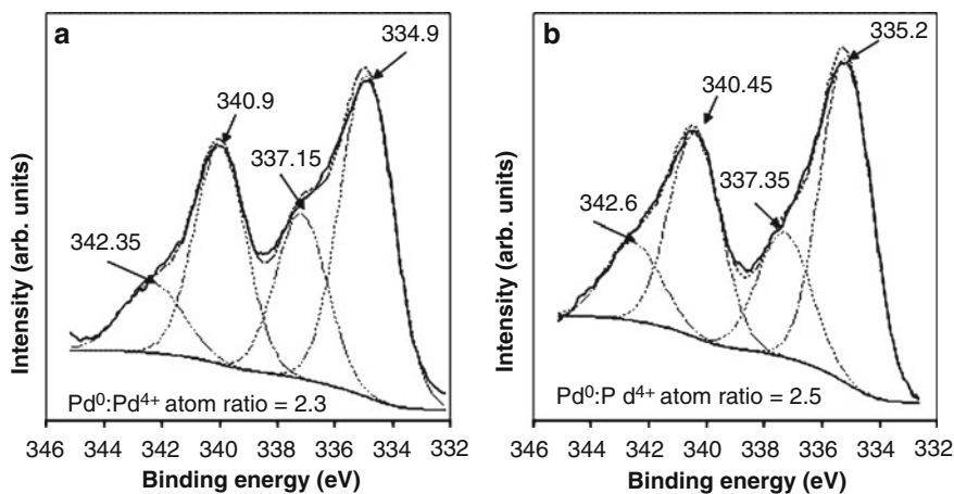
Fig. 11.37 XPS Pd3d spectra of (a) Pd/montmorillonite and (b) Pd/kaolinite samples (see [59])
