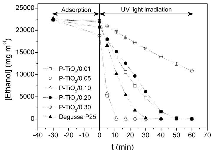
Fig. 12.12 Photodegradation of ethanol on Degussa P25 \text{TiO}_2 and various P- \text{TiO}_2 samples at 74% initial relative humidity [46]
