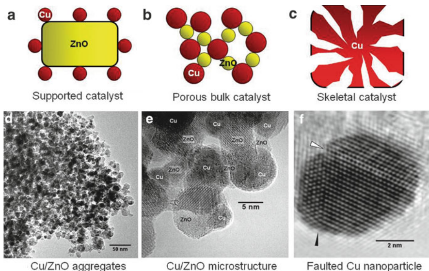
Fig. 5.2 Schemes of different catalyst microstructures (a–c) and transmission electron micrographs of a Cu/ZnO/(Al 2 O 3 ) catalyst (d and e). In the high-resolution image (f) planar defects of the Cu-nanoparticles like twin boundaries (black arrow) and stacking faults (white arrow) can be seen
