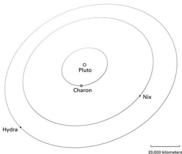
Orbits of the moons of Pluto (Wil Tirion)
