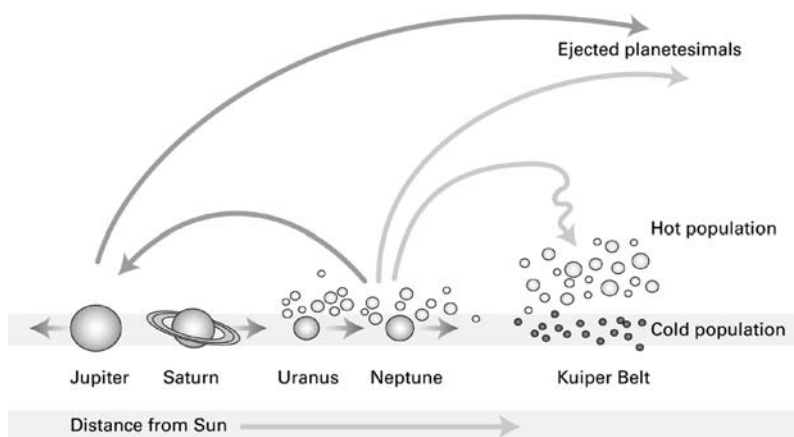
Diagram showing the process of planetesimal ejection and planet migration (Wil Tirion)
