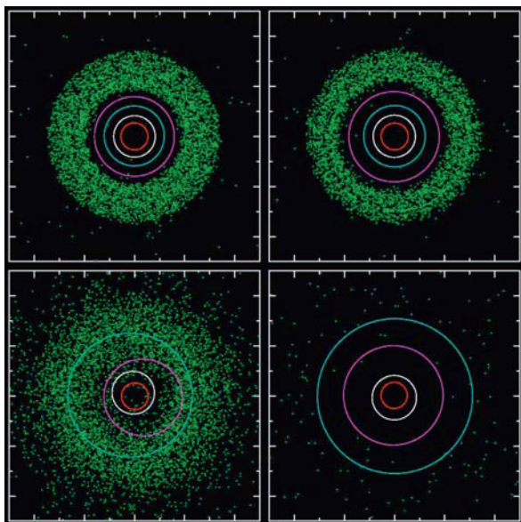
Scenes from a computer simulation of the solar system's early evolution according to the Nice model. Planets migrate, planetesimals are scattered away, and Uranus and Neptune swap orbits (Courtesy Alessandro Morbidelli)
