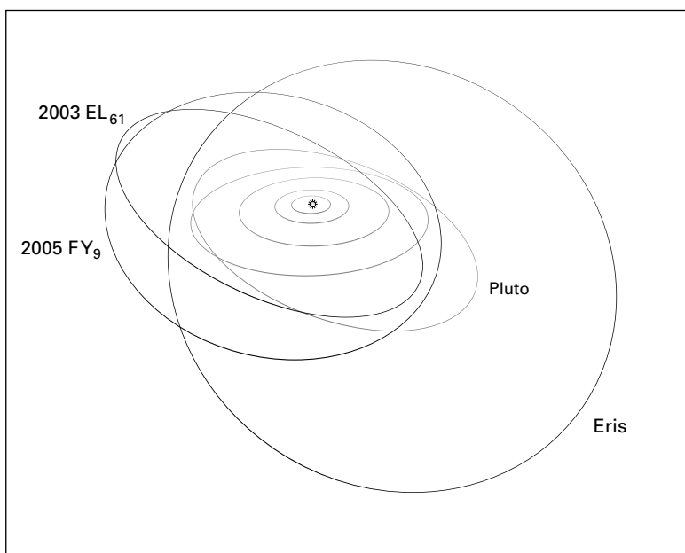
The orbits of Pluto, 'Xena' (now called Eris), 'Santa' (2003 EL 61 ), and 'Easter Bunny' (2005 FY 9 ) (Wil Tirion)
