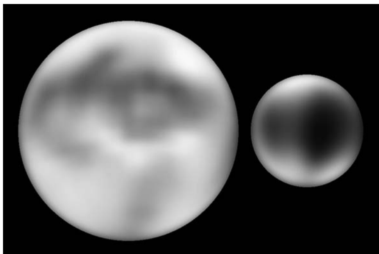
Crude maps of Pluto and Charon, as derived from their mutual eclipses and occultations (Adapted from images by Marc Buie/Lowell Observatory)
