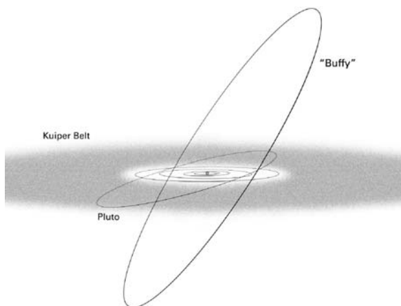
The unusual orbit of 2004 XR 190 ('Buffy') (Wil Tirion)
