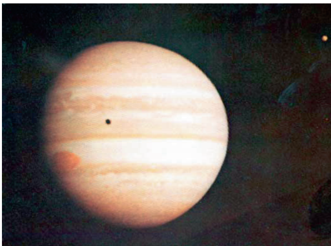
Jupiter, as imaged by Pioneer 10 (NASA/JPL)
