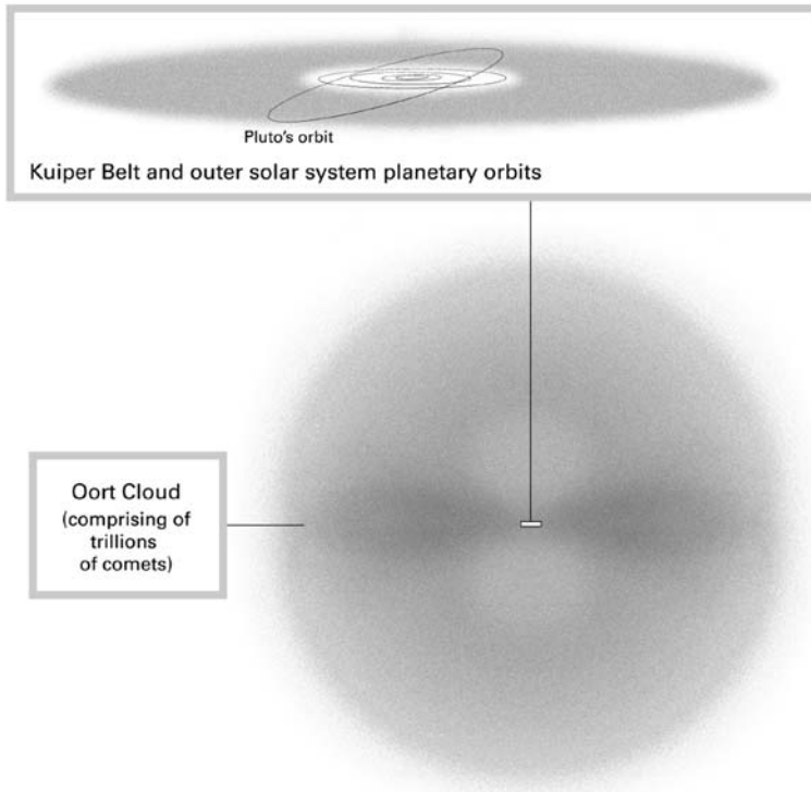
Schematic drawing of the Oort Cloud and the Kuiper Belt (Wil Tirion)
