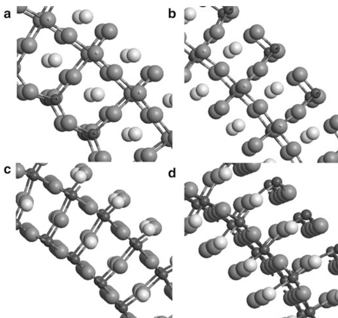
Fig. 13.22 Structure of SrTiO 3 NTs consisting of four atomic layers with different chiralities (view along the tube axis). Chirality (48,0): (a)—type I with SrO outer shell; (b)—type II with TiO 2 outer shell. Chirality (24,24): (c)—type I with SrO outer shell; (d)—type II with TiO 2 outer shell. See Fig. 13.20 for the legend
