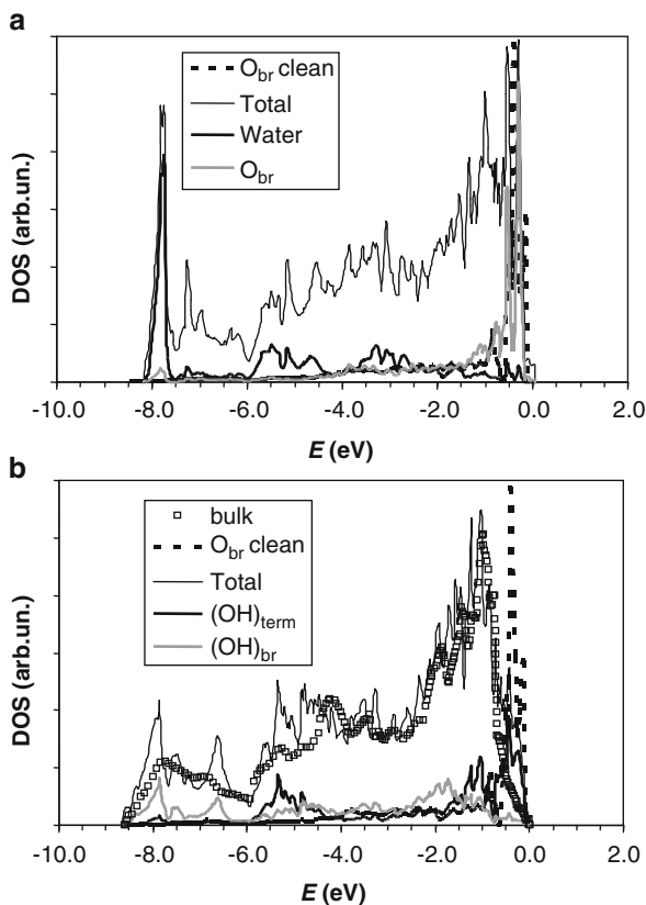
Fig. 11.20 Total and O-projected valence-band DOS in the hydroxylated (100) \text{SnO}_2 surface systems. (a) Molecular adsorption; (b) dissociative adsorption. (The sense of line types and energy scale are the same as in Fig. 11.19.) The projection onto the \text{O}_{\text{br}} states for the clean (100) surface is shown by the dotted lines, and the total bulk DOS is shown in (b) by open circles
