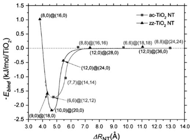
Fig. 13.12 Binding energies E_{bind} versus \Delta R_{NT} for the two sets of DW TiO 2 NTs with ac and zz chiralities. Spline treatment of the curves was performed to make them smooth
