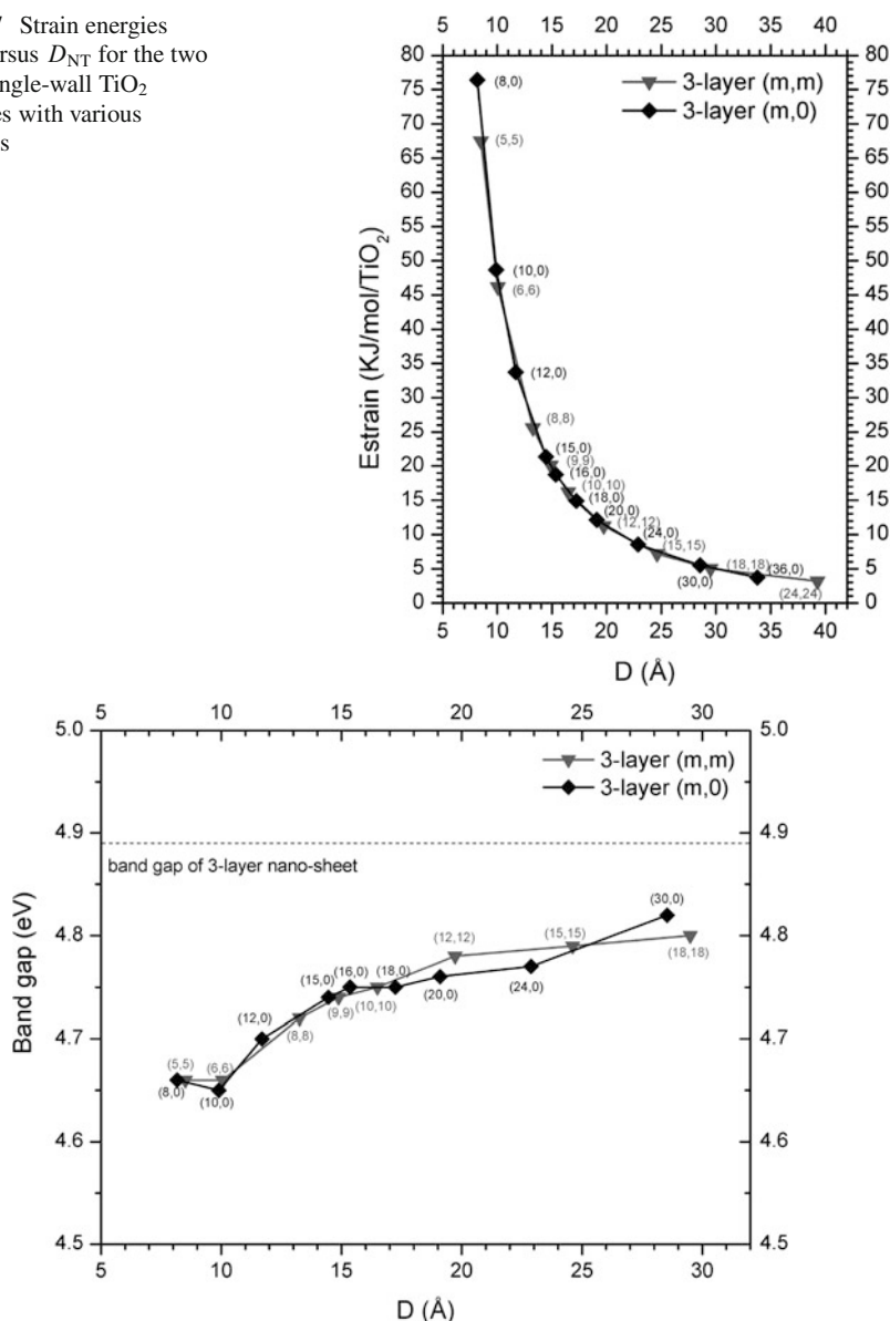
Fig. 13.8 Bandgaps \Delta\epsilon_{\text{gap}} versus D_{\text{NT}} for the two sets of single-wall TiO 2 nanotubes with various chiralities
