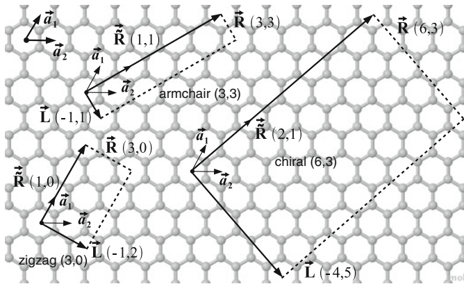
Fig. 13.2 Supercells of graphene layer defining armchair (3,3), zigzag (3,0), and chiral (6,3) nanotubes
