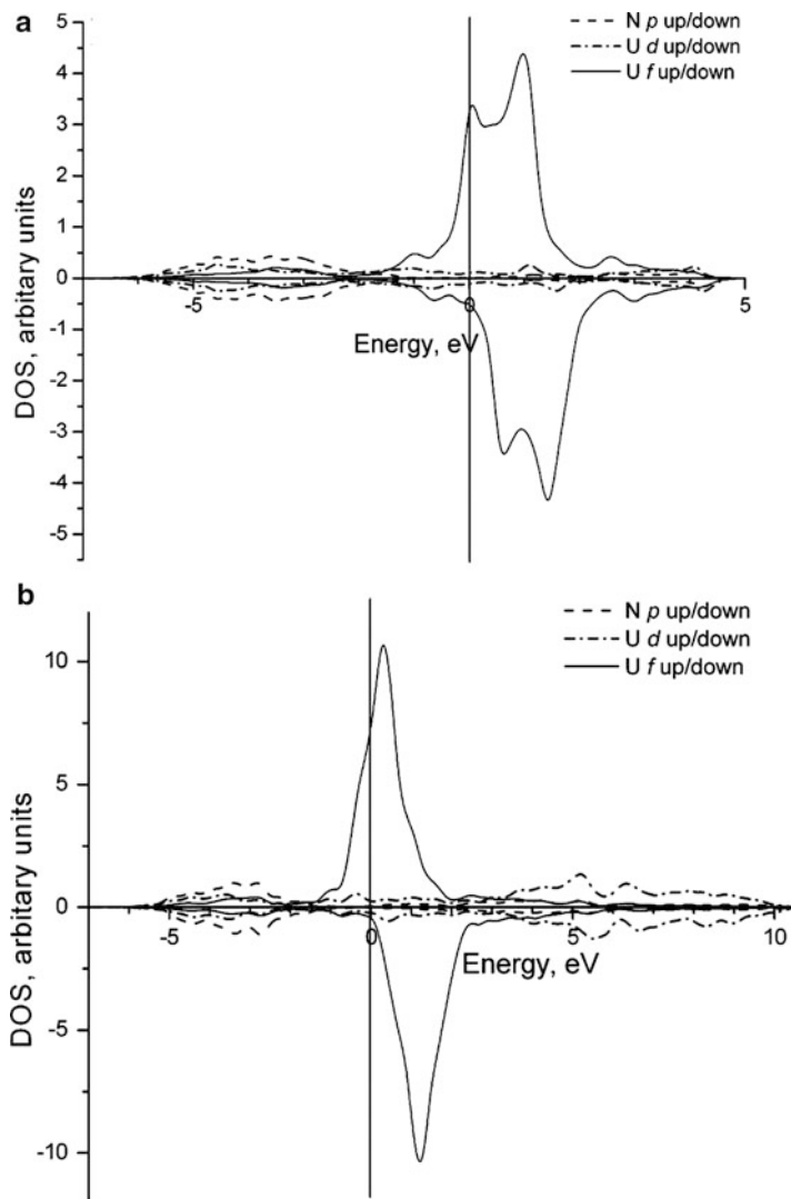
Fig. 12.6 The projected DOS for the bulk (a) and the perfect UN (001) surface (b) in FM states
