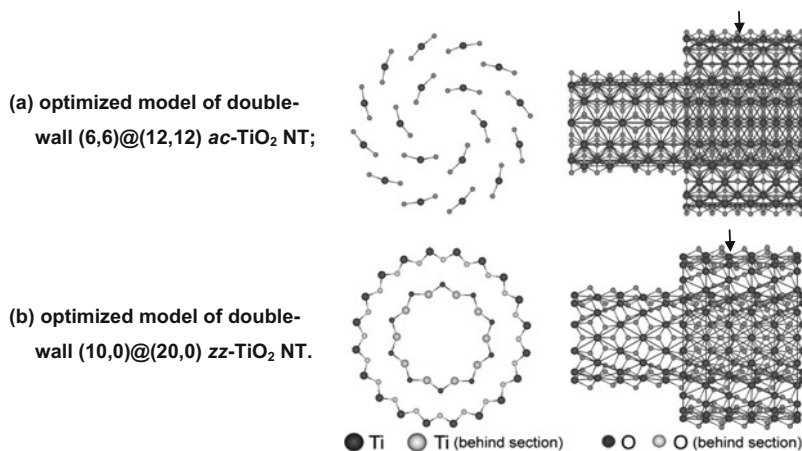
Fig. 13.11 Cross sections and lateral images of hexagonal DW TiO 2 NTs (i.e., left and right parts of models a and b, respectively) corresponding to optimized diameters for armchair and zigzag chiralities. For zz -DW TiO 2 NTs (model b), the atoms of the nearest ring behind the cross section are shown as half-shaded balls . For the description of the graphical details of models, see the clarification in the caption of Fig. 13.9
