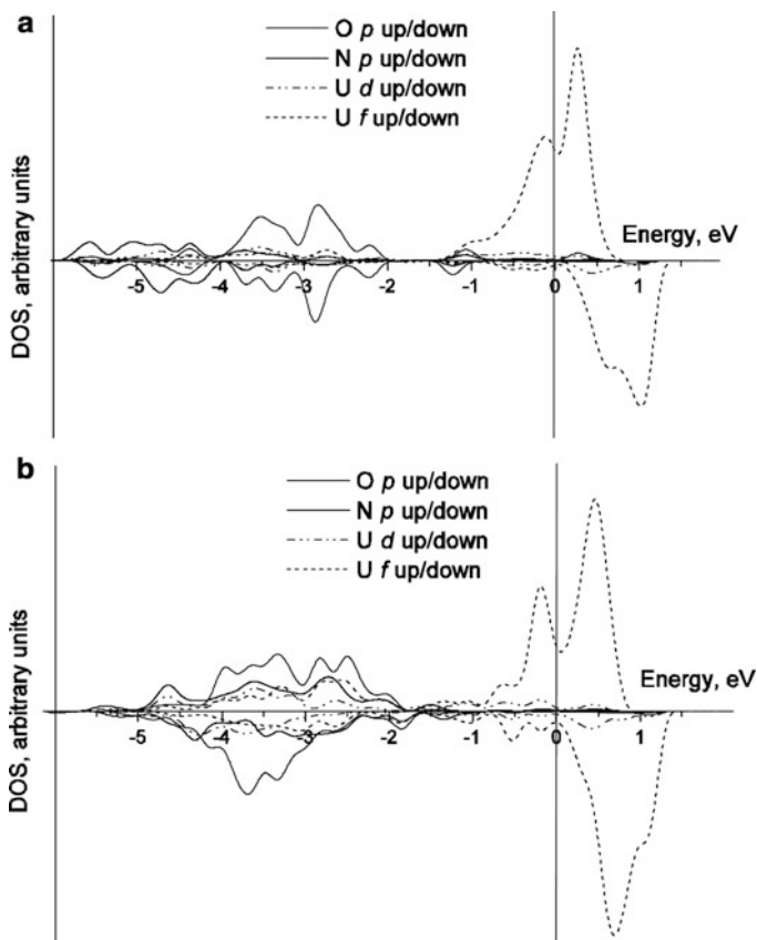
Fig. 12.9 The total and projected densities of states for the O atom adsorption atop the N anion (a) and the U cation (b) obtained using the results of PAW calculations. In the former, we consider the orbital projections of the N anion under the O atom and one of the four nearest neighboring U cations (Fig. 12.8a). Analogously, the lower plot presents the orbital projections of the U cation beneath the adatom and one of the four nearest N anions. The largest peaks were normalized to the same value, whereas the convolution of the individual energy levels was plotted using the Gaussian functions with a halfwidth 0.2 eV. “O” on the energy axis corresponds to the Fermi level
