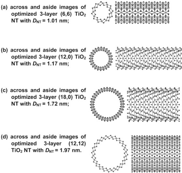
Fig. 13.6 Cross-sectional (across) and lateral (aside) images of hexagonal single-wall TiO 2 nanotubes with different chiralities and diameters
