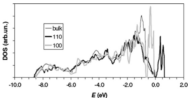
Fig. 11.16 Total valence-band DOS of bulk SnO 2 crystal ( fine line ), its (110) ( bold dark line ) and (100) ( bold gray line ) surfaces calculated using the B3LYP functional (see text for explanation of energy scale)
