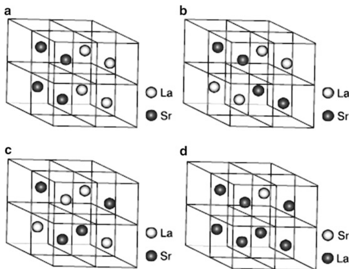
Fig. 10.8 Four structures used in calculations of \text{La}_x\text{Sr}_{1-x}\text{MnO}_3
