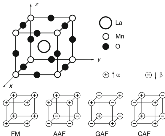
Fig. 9.10 Magnetic ordering in \text{LaMnO}_3 crystal.
