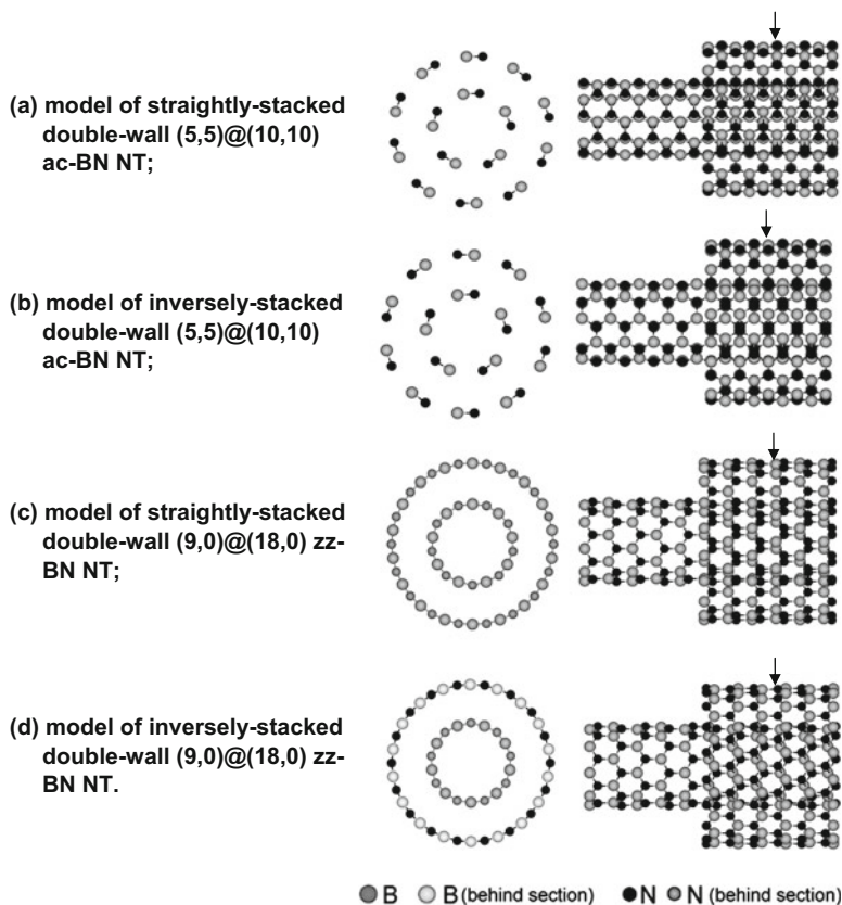
Fig. 13.9 Cross sections and lateral images of hexagonal DWBN NTs (left and right parts of models a–d, respectively) corresponding to optimized diameters for ac and zz chiralities. For zz-DW BN NTs (the models c and d), the atoms of the nearest ring behind the cross section are shown as half-shaded balls. The arrows above each lateral image show the directions of the cross sections. For viewing convenience, the lateral images of the inner shells of the nanotubes are shown as twice as long as those of the outer shells
