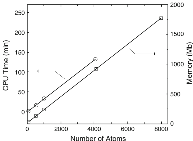
Fig. 7.1 O(N) behavior of the overall CPU time and memory in silicon supercell calculations [387]
