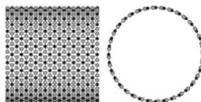
(c) optimized single-wall (18,18) ac -BN NT (aside and across images), D_{NT} = 2.49 nm;
