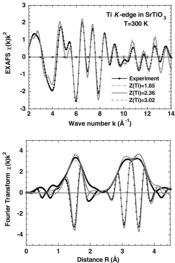
Fig. 9.21 Effect of the titanium ions charge on the calculated EXAFS \chi(k)k^2 signals ( upper panel ) and their Fourier transforms ( lower panel ) for \text{SrTiO}_3 in the range up to the 4th coordination shell. The dash-dotted curve corresponds to Z_{\text{Ti}} = 1.85 , the solid to Z_{\text{Ti}} = 2.36 , and the dashed to Z_{\text{Ti}} = 3.02 . The experimental signals (from [952]) are shown by solid circles. Note that the Fourier transforms are not corrected by the phase shift; therefore, the peaks positions differ from crystallographic values. The error bars for the experimental EXAFS signal are also shown. See text for the calculation details
