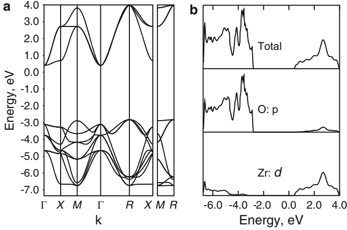
Fig. 9.2 Electronic structure of SrZrO 3 crystal: (a) band structure; (b) total and projected DOS. LCAO DFT calculations [597]
