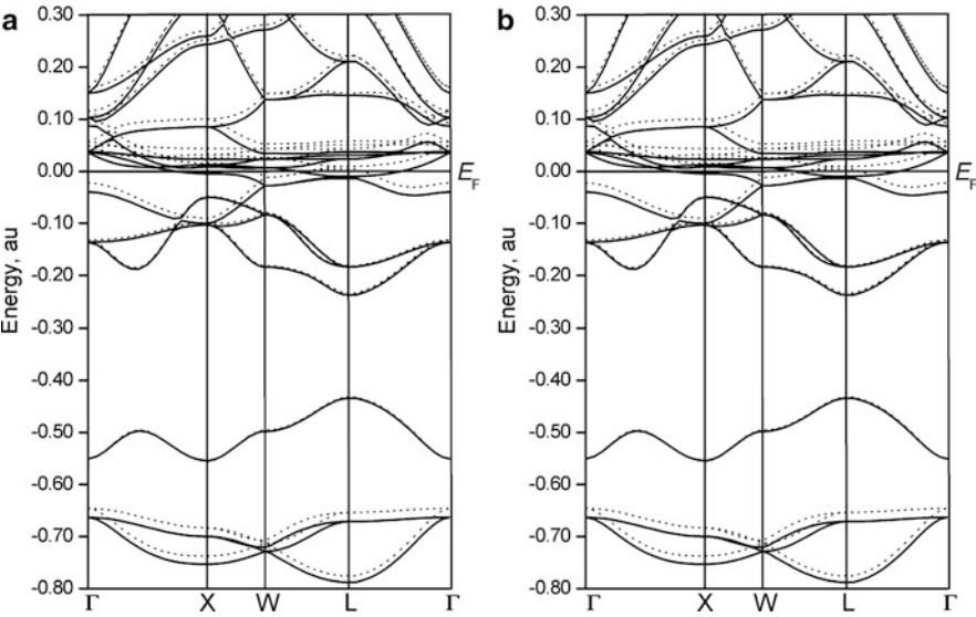
Fig. 12.4 The energy bands of UN crystal constructed for (a) LCAO PW91 (RECP 60) Hamiltonian and (b) PW PW91 (RECP 78) Hamiltonian. The energies are given in a.u., and the solid and dotted lines correspond to the states with spin-up and spin-down, respectively
