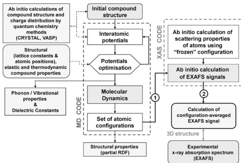
Fig. 9.19 Scheme of the combined quantum mechanics and molecular dynamics (QM-MD) approach to the x-ray absorption spectra simulation
