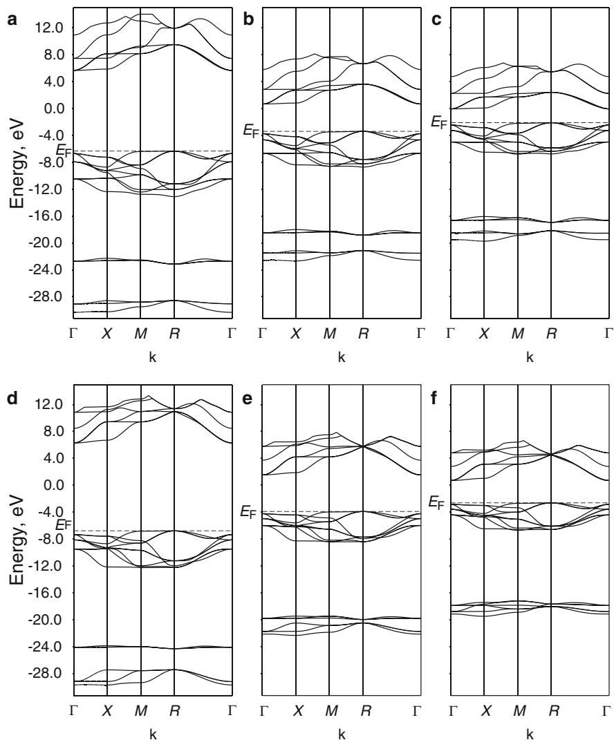
Fig. 9.8 Band structure of cubic crystals: (a),(b),(c)—SrTiO 3 , (d),(e),(f)—SrZrO 3 . HF LCAO method—(a),(d); hybrid HF-DFT(PBE0) LCAO method—(b),(e); DFT(PBE) LCAO method—(c),(f)
