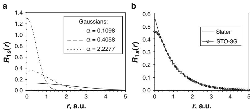
Fig. 8.1 1s orbitals, [444]: (a) Gaussian and (b) Slater and fitted STO-3G
