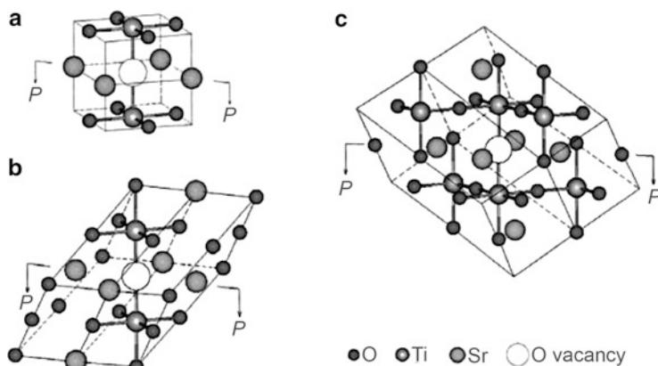
Fig. 10.3 Three types of equidistant crystalline cells with a centered O vacancy for the cubic phase of SrTiO 3 perovskite: (a) simple cubic (sc), (b) face-centered cubic (fcc), and (c) body-centered cubic (bcc). Sticks between the oxygen and titanium ions indicate the partly covalent bonds between them. To construct the difference electron-density plots, each cell is sectioned along the Ti–O–Ti axes by the plane P–P
