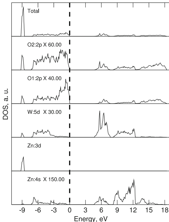
Fig. 9.24 Total/projected density of states for a wolframite-type \text{ZnWO}_4 . The energy zero is set at the Fermi energy level
