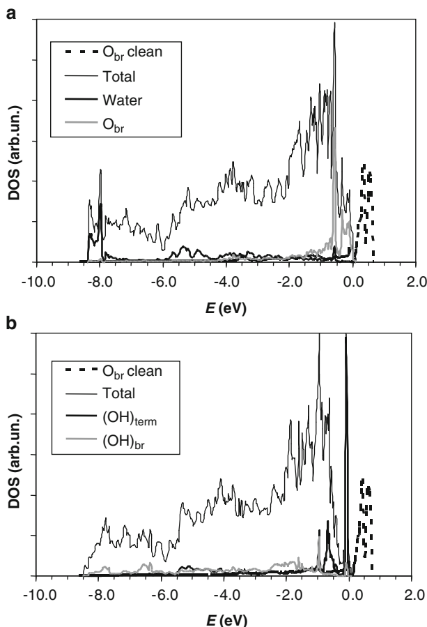
Fig. 11.18 Total and O-projected valence-band DOS in the hydroxylated (110) \text{SnO}_2 surface systems (see text for explanation of energy scale) [799]. (a) Molecular adsorption: total DOS ( fine line ), projection onto the water states ( bold dark line ), projection onto the O_{br} states ( bold gray line ); (b) dissociative adsorption: total DOS ( fine line ), projection onto the (OH)_{term} states ( bold dark line ), projection onto the (OH)_b states ( bold gray line ). The projection onto the O_{br} states in the clean (110) surface is shown by a dotted line
