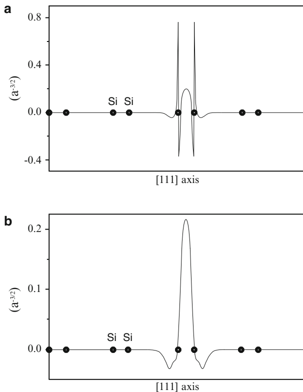
Fig. 3.9 Wannier functions for the silicon upper valence band along the [111] direction: (a) full electron calculation; (b) pseudopotential calculation
