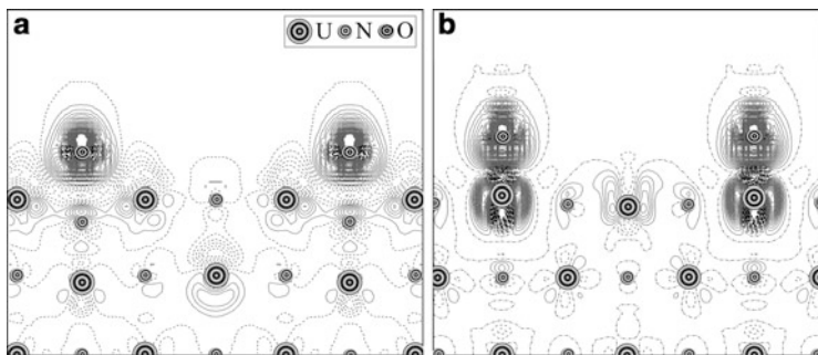
Fig. 12.8 The difference electron-density maps \Delta\rho(r) (the total density of the interface minus the densities of the substrate and adsorbate with optimized interfacial geometry) for the O adatoms atop the surface: (a) N anions and (b) U cations on the UN(001) surface obtained using the results of the PAW calculations. The solid and dashed isolines correspond to positive and negative electron density, respectively. The isodensity increment is 0.003 \text{ e } \text{\AA}^{-3}
