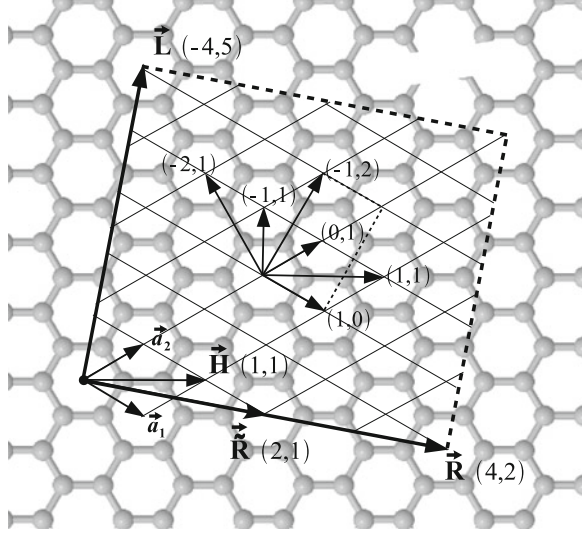
Fig. 13.1 Chirality vectors of the nanotubes from graphene layer
