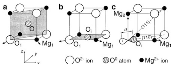
Fig. 10.2 Configurations of the interstitial oxygen atom in MgO
