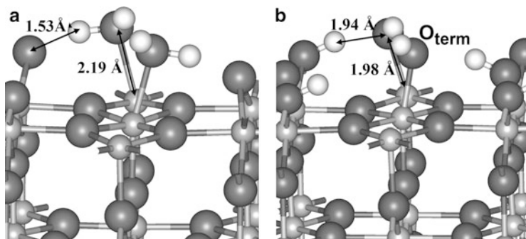
Fig. 11.17 Optimized monolayer structure for the water molecules adsorbed on a (110) SnO 2 surface obtained using the B3LYP functional [799]: (a) stable structure for molecular adsorption and (b) stable structure for dissociative adsorption. Large dark-gray balls are O atoms; light-gray balls are Sn atoms; small white balls are H atoms
