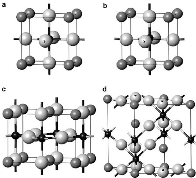
Fig. 9.12 The structure of the conventional unit cells for (a) cubic, (b) tetragonal, (c) orthorhombic, and (d) rhombohedral \text{BaTiO}_3 . Legend: Ti—small balls, Ba—middle balls, O—large balls
