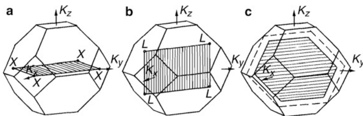
Fig. 11.1 Brillouin zones for a face-centered cubic lattice and surfaces (a) (001), (b) (110), (c) (111)
