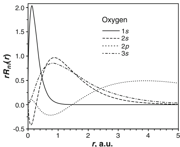
Fig. 8.2 Radial orbitals of oxygen atom in the ground state ( http://www.physik.uni-frankfurt.de/~engel/ncpp.html )
