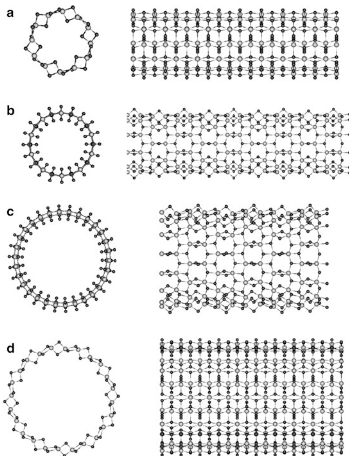
Fig. 13.16 Atop (lateral) and across (cross-section) views of 6-layered anatase-like SW TiO 2 nanotubes for different chiralities: (a)(-3, 3), (b)(10,10),(15,15),(-6, 6)
