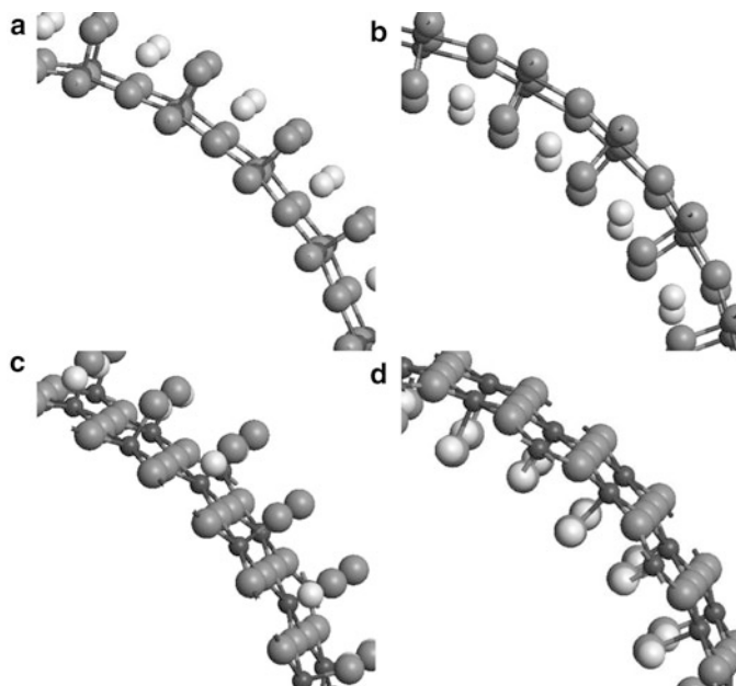
Fig. 13.21 Structure of SrTiO 3 NTs consisting of two atomic layers with different chiralities (view along the tube axis). Chirality (20,0): (a)—type I with SrO outer shell; (b)—type II with TiO 2 outer shell. Chirality (16,16): (c)—type I with SrO outer shell; (d)—type II with TiO 2 outer shell. See Fig. 13.20 for legend
