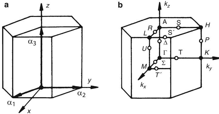
Fig. 3.6 Primitive unit cell and Brillouin zone for hexagonal lattice
