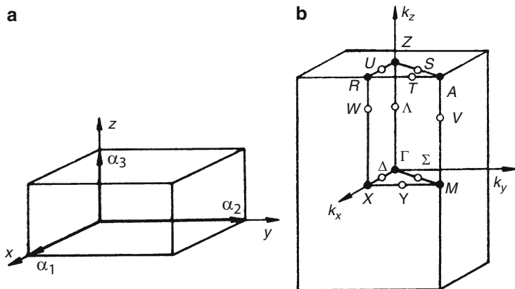
Fig. 3.7 Primitive unit cell and Brillouin zone for simple tetragonal lattice
