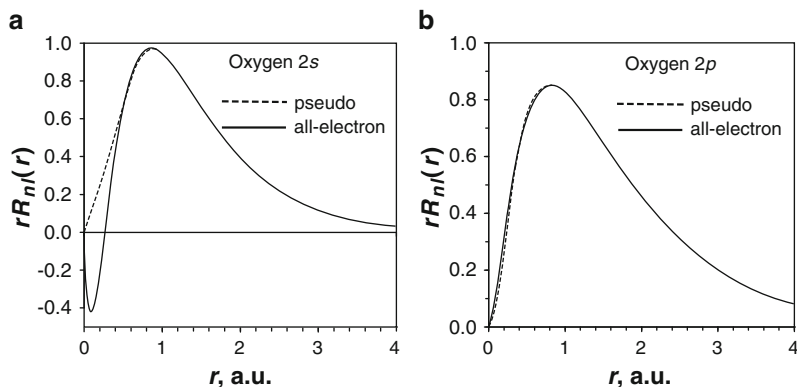
Fig. 8.3 Radial pseudo- versus all-electron orbitals of oxygen: (a) 2s (b) 2p ( http://www.physik.uni-frankfurt.de/~engel/ncpp.html )
