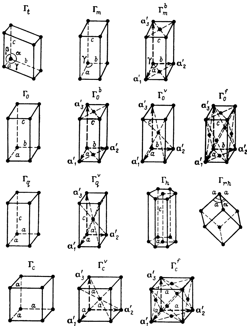
Fig. 2.2 Three-dimensional Bravais lattices
