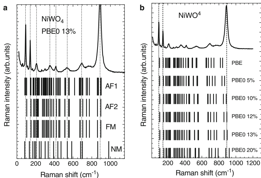
Fig. 9.29 (a) Comparison of the room-temperature experimental Raman spectrum for \text{NiWO}_4 with mode frequencies (vertical lines), calculated by the first-principles LCAO method using hybrid PBE0 13% HF Hamiltonian for AF1, AF2, FM, and NM states. (b) LCAO results for hybrid PBE0-type Hamiltonian with different percentages (0–20%) of HF contribution in the AF2 state)
