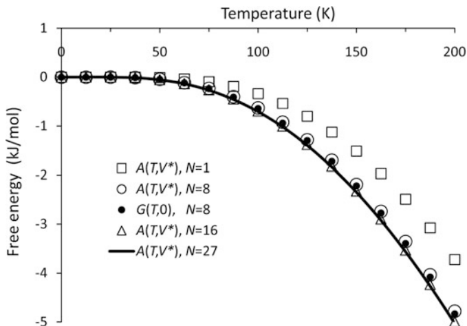
Fig. 9.13 Temperature dependence of the relative change in free energy, calculated using different supercells for the rhombohedral BaTiO 3
