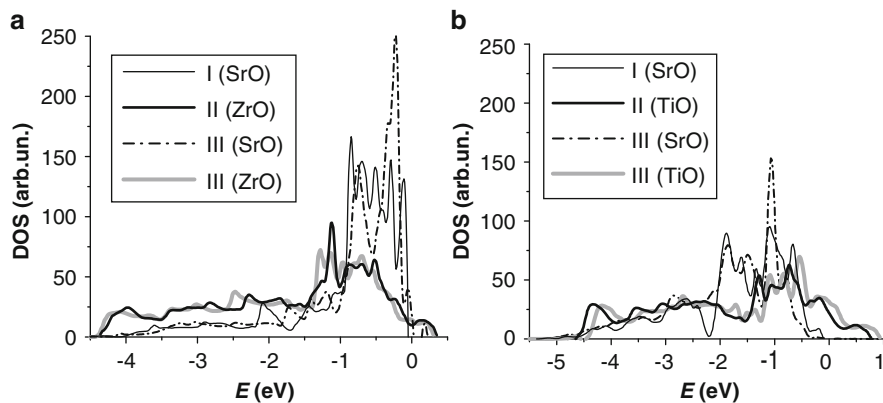
Fig. 11.22 Projected VB DOS for oxygen atom in the first surface layer for all three models (a—SrZrO 3 ; b—SrTiO 3 ). For model III, the first oxygen projection corresponds to the SrO side and the second to the MO 2 side
