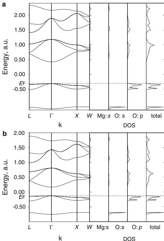
Fig. 9.5 Band structure and DOS of MgO crystal, [607]: (a) HF LCAO method; (b) DFT(LDA) LCAO method
