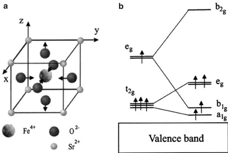
Fig. 10.6 (a) Schematic view of the Fe impurity with asymmetric e_g relaxation of the six nearest O atoms. (b) The relevant energy levels before and after relaxation
