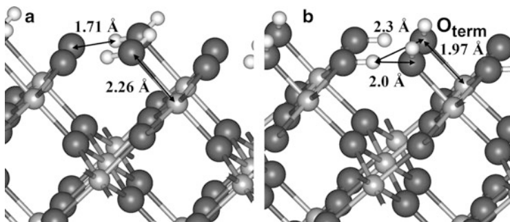
Fig. 11.19 Optimized monolayer structure for the water molecules adsorbed on a (100) \text{SnO}_2 surface obtained using the B3LYP functional [799]: (a) stable structure for molecular adsorption; (b) stable structure for dissociative adsorption. Large dark-gray balls are O atoms, light-gray balls are Sn atoms; small white balls are H atoms
