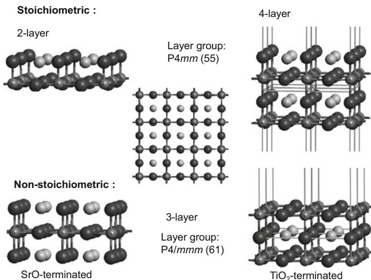
Fig. 13.20 STO slabs consisting of two or four alternating (001) SrO and TiO 2 atomic planes which have been used for nanotubes construction (lateral view). The top view along the [001] direction is shown in the middle. Legend: O—grey balls, Ti—small dark balls, Sr—light balls
