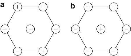
Fig. 9.11 Two local spin configurations in the AFa state in a hexagonal plane; in case (a) the central spin-down Mn ion is surrounded by 4 spin-down and 2 spin-up Mn ions, in (b) the central spin-up Mn ion is surrounded by 6 spin-down Mn ions
