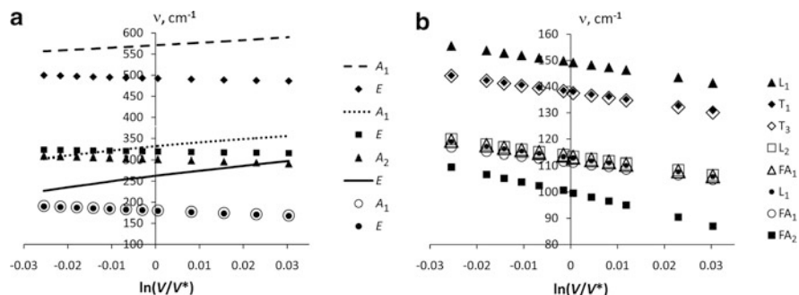
Fig. 9.14 Calculated volume dependence of selected phonon frequencies in BaTiO 3 rhombohedral phase. (a) Zone-center modes. (b) Acoustic modes in L (0 0 1/2), FA (0 1/2 1/2), and T (1/2 1/2 1/2) points of BZ
