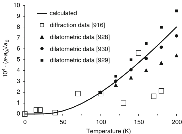
Fig. 9.16 Comparison of experimental and calculated results for the temperature dependence of the relative variation for the pseudocubic lattice parameter in the rhombohedral \text{BaTiO}_3
