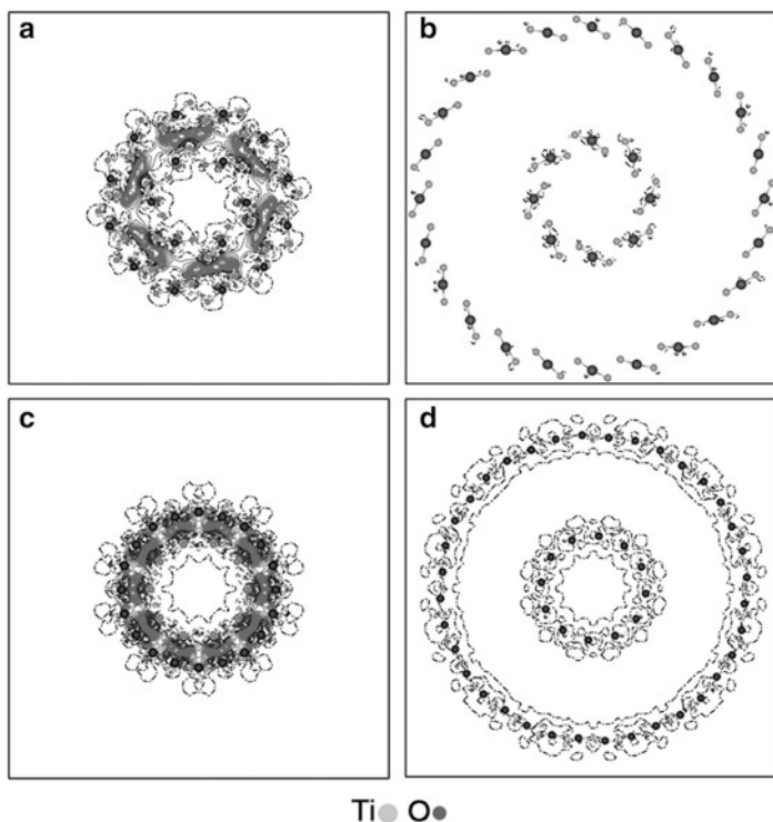
Fig. 13.13 Difference electron density plots \Delta\rho(r) of DW TiO 2 NTs calculated for the cross sections of nanotubes depicted in Fig. 13.11: (a) (6,6)@(12,12), (b) (8,8)@(24,24), (c) (10,0)@(20,0), (d) (12,0)@(36,0). For technical and graphical details, see the caption of Fig. 13.10
