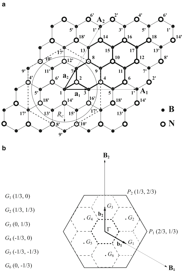
Fig. 6.1 Supercell (a) and small Brillouin zone (b) for hexagonal plane lattice of boron nitride BN. Atoms 1–18 belong to the supercell, the atoms with the primed numbers are supposed to be identical with the corresponding atoms, belonging to the supercell
