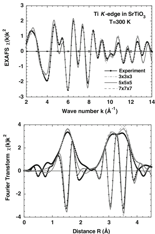
Fig. 9.22 Effect of the supercell size on the calculated EXAFS \chi(k)k^2 signals ( upper panel ) and their Fourier transforms ( lower panel ) for SrTiO 3 in the range up to the 4th coordination shell. The dash-dotted curve corresponds to the supercell size (3×3×3), the solid to (5×5×5), and the dashed to 7×7×7. The experimental signals (from [952]) are shown by solid circles . Note that the Fourier transforms are not corrected by the phase shift; therefore, the peaks positions differ from the crystallographic values. The error bars for the experimental EXAFS signal are also shown in (a)
