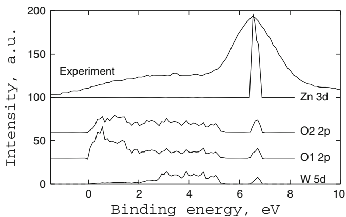
Fig. 9.26 Comparison of XPS spectrum and PDOS curves for the wolframite-type \text{ZnWO}_4 . The curves are vertically shifted for the sake of clarity
