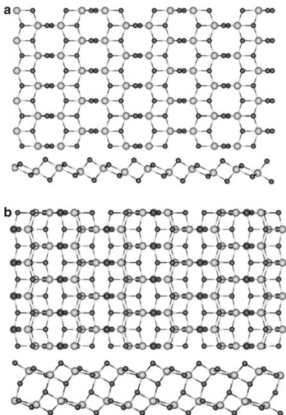
Fig. 13.15 Models of stoichiometric (101) titania sheets of different thickness optimized from the corresponding slabs with initial geometry of bulk anatase (lateral and cross-section images): (a) 6-layer slab (thickness 0.24 nm); (b) 12-layer slab (thickness 0.58 nm)
