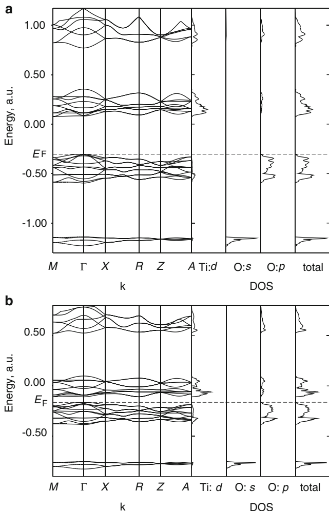
Fig. 9.6 Band structure and DOS of rutile \text{TiO}_2 crystal, [607]: (a) HF LCAO method; (b) DFT(LDA) LCAO method
