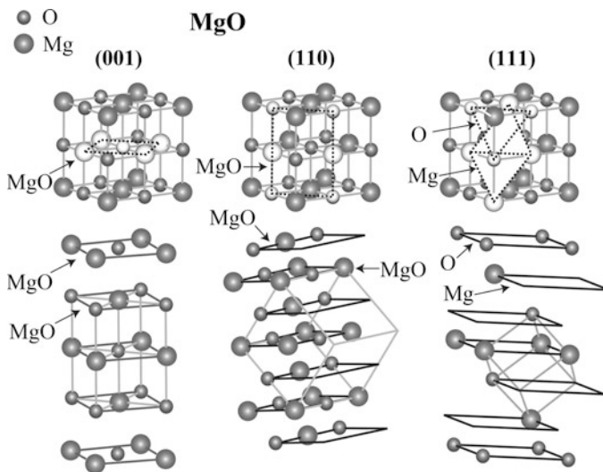
Fig. 11.2 Stacking of atomic planes for MgO surfaces
