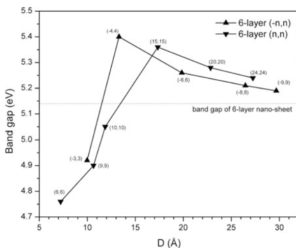
Fig. 13.18 Bandgaps versus D_{\text{NT}} for the two sets of six-layer SW TiO 2 NTs with various chiralities
