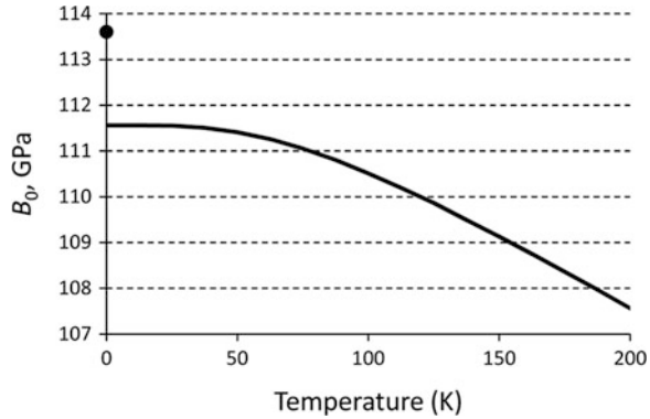
Fig. 9.15 Calculated temperature dependence of the isothermal bulk modulus for the BaTiO 3 rhombohedral phase. A static value is shown by a dot at T = 0 K
