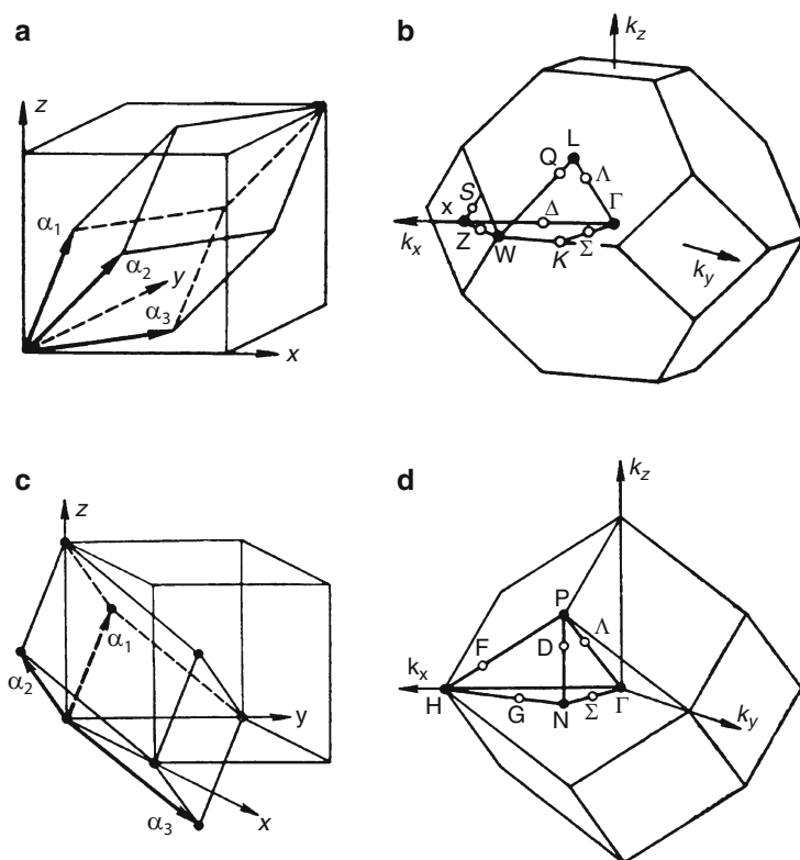
Fig. 3.2 Primitive unit cells (a, c) and Brillouin zones (b, d) for face-centered and body-centered cubic lattices
