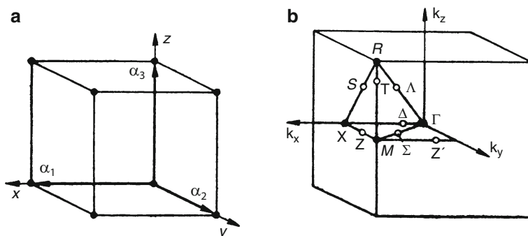
Fig. 3.1 Primitive unit cell and Brillouin zone for simple cubic lattice
