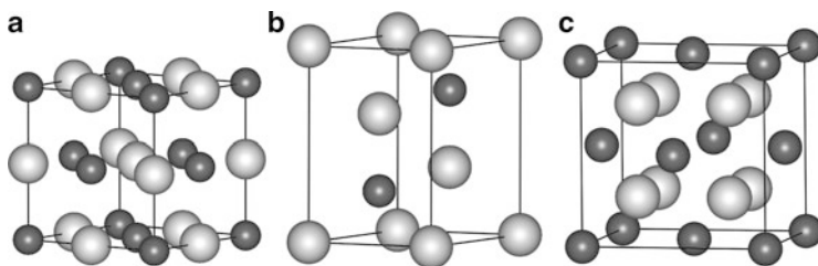
Fig. 12.2 (a) UN, space group Fm\bar{3}m ; (b) U_2N_3 , space group P\bar{3}m1 ; and (c) UN_2 , space group Fm\bar{3}m . U atoms—dark balls and N atoms—light balls
