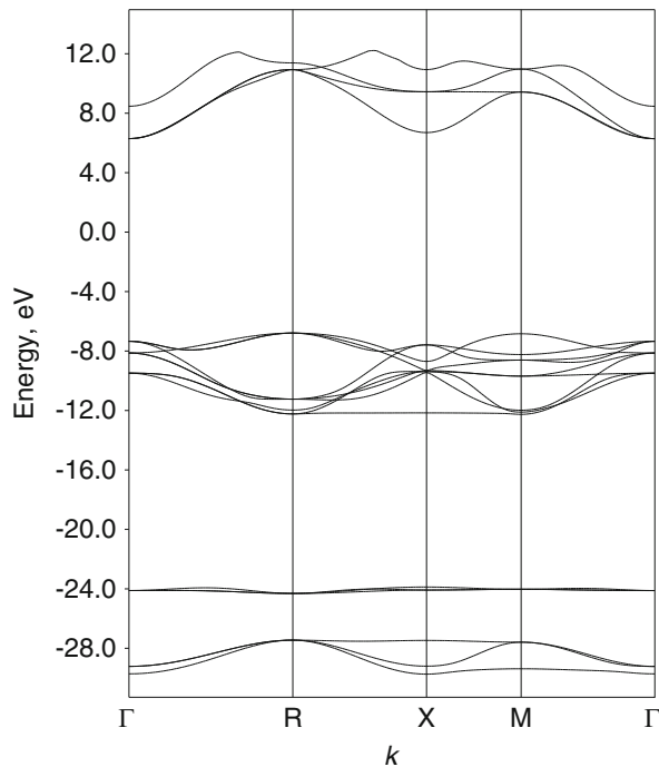
Fig. 3.3 Hartree–Fock energy bands for \text{SrZrO}_3 crystal
