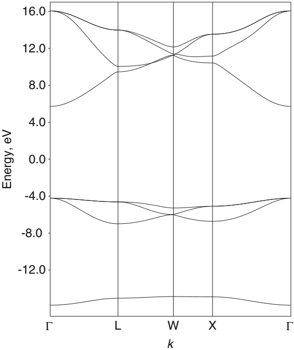
Fig. 3.4 Hartree–Fock energy bands for MgO crystal
