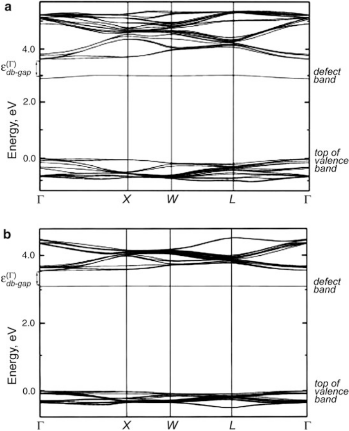
Fig. 10.5 Band structure of unrelaxed \text{SrTiO}_3 crystal with a single F center per fcc supercell containing either 80 atoms ( a ) or 270 atoms ( b ) [715]. Energy bands corresponding to the F center are split off the conduction bands. Their depth (gap) is shown relative to the bottom of the conduction band at the \Gamma point
