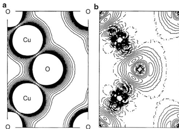
Fig. 9.9 Electron-density maps obtained for Cu 2 O on a (110) plane, [606]. (a) Total electron density. (b) Density difference maps, bulk minus neutral atom superposition. Values corresponding to neighboring isodensity lines differ by 0.01 e/Bohr 3 . The full and broken curves in (b) indicate density increase and decrease, respectively
