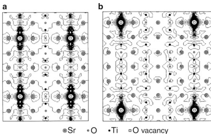
Fig. 10.4 Two-dimensional (2D) difference electron-density maps (the total density in the perfect \text{SrTiO}_3 bulk minus the sum of electron densities of both isolated oxygen atoms and defective \text{SrTiO}_3 ) projected onto the (110) section plane P-P for 80-atom (a) and 270-atom (b) fcc supercells containing a single oxygen vacancy [715]. Dash-dot isolines correspond to the zero level. Solid and dashed isolines describe positive and negative values of electron density, respectively. The isodensity increment is 0.002 \text{ e/\AA}^{-3} .
