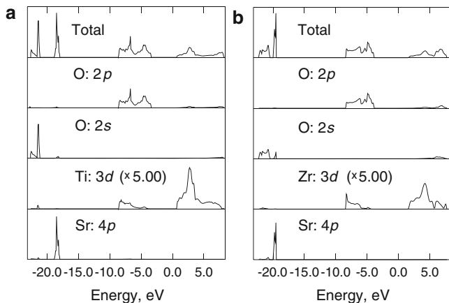
Fig. 9.7 Full and partial DOS in (a) \text{SrTiO}_3 and (b) \text{SrZrO}_3 crystals
