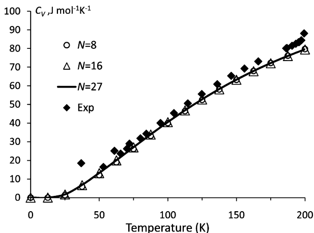
Fig. 9.18 Experimental [932] and theoretical temperature dependence of heat capacity, calculated in the harmonic approximation using different supercells for the rhombohedral BaTiO 3
