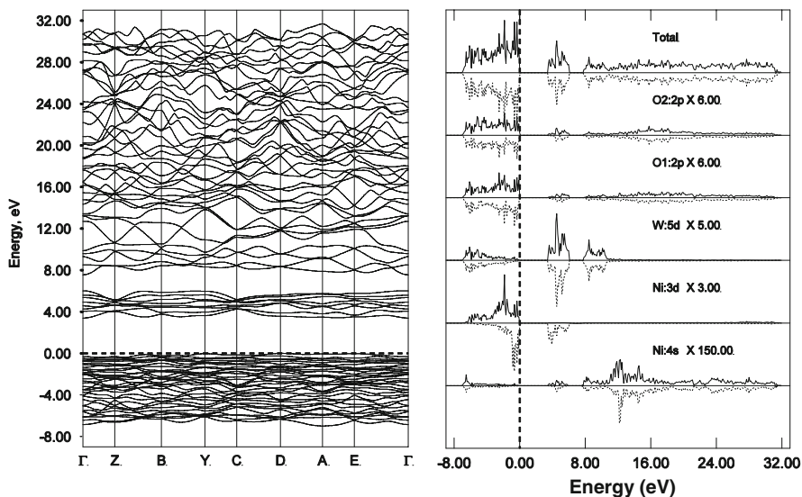
Fig. 9.28 Band-structure diagram ( left panel ) and the spin- dependent total/projected density of states ( right panel ) for the wolframite-type ( P2/c ) \text{NiWO}_4 in the antiferromagnetic AF2 state. The energy zero is set at the Fermi energy level
