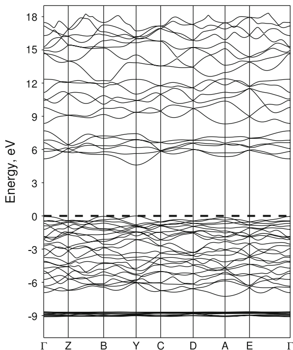
Fig. 9.23 Band-structure diagram for a wolframite-type \text{ZnWO}_4 . The energy zero is set at the Fermi energy level
