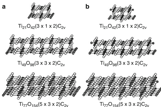
Fig. 11.10 Rutile (110) surfaces of size 3 \times 1 , 3 \times 3 and 5 \times 3 : two-layer clusters of types A and B, [753]. The labels of atoms are the same as in Fig. 11.9
