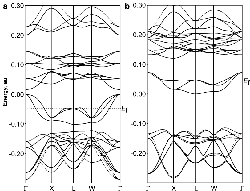
Fig. 12.1 Band structure of the ferromagnetic phase of \text{UO}_2 crystal calculated using (a) nonrelativistic and (b) scalar-relativistic pseudopotentials for the uranium atom
