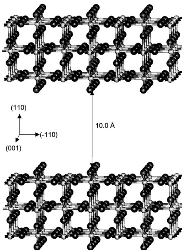
Fig. 11.8 Periodic-slab model of rutile \text{TiO}_2 (110) surface
