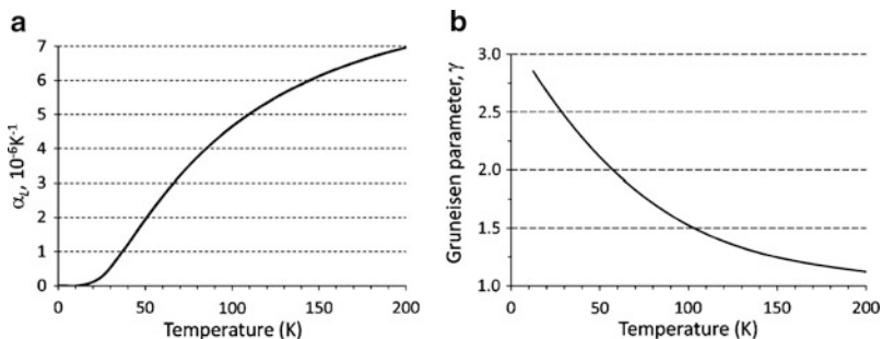
Fig. 9.17 (a) Calculated temperature dependence of the average linear (isotropic) thermal expansion coefficient for the rhombohedral BaTiO 3 at zero pressure. (b) Calculated temperature dependence of the thermal Gruneisen parameter
