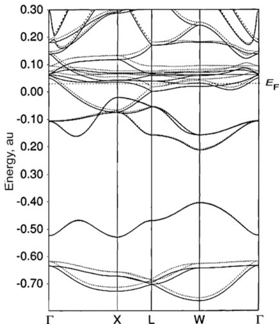
Fig. 12.3 Energy bands of the UN crystal (LCAO DFT/PWGGA calculations, RECP SK60) the energies are given in a.u. and the solid and dotted lines correspond to the states with spin-up and spin-down, respectively
