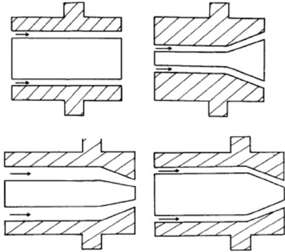
Fig. 8.20 Dies used to study the effect of die geometry on extrudate swell. Clockwise from upper left : annular die, diverging die, 10^\circ converging die, 20^\circ converging die. From Orbey and Dealy [20]
