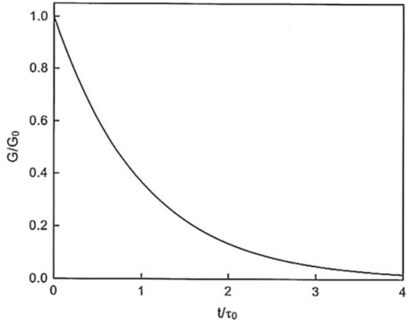
Fig. 3.4 Dimensionless relaxation modulus versus dimensionless time modeled as the exponential function shown as Eq. (3.19)
