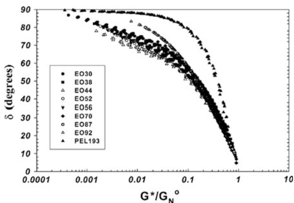
Fig. 7.5 A modified van Gorp and Palmen plot of loss angle versus |G^*|/G_N^0 for eight ethylene/octene copolymers. The number shown is the wt % octene, and the upper data set is for monodisperse, hydrogenated polybutadiene, which is expected to be very similar to monodisperse polyethylene. Normalizing using G_N^0 tends to bring data for all the copolymers close together. From García-Franco et al. [32]
