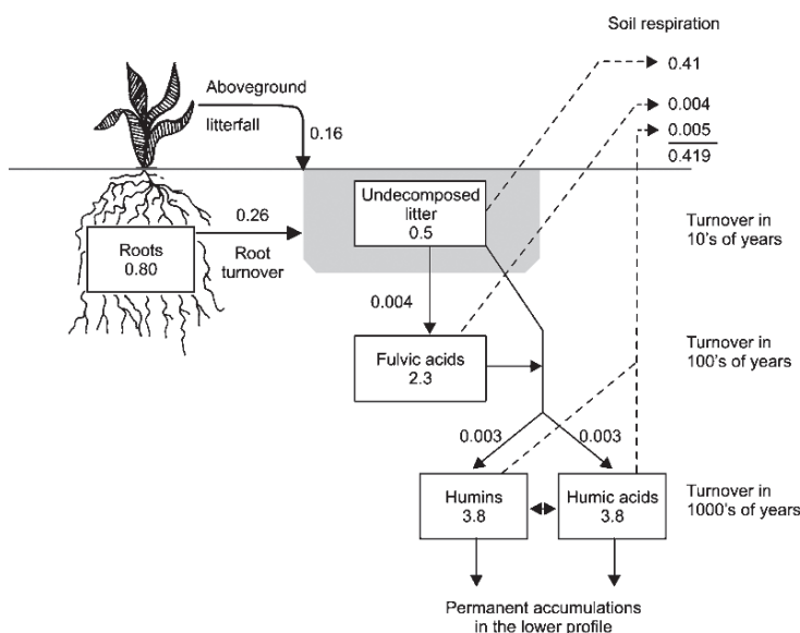
Fig. 2.2 The carbon cycle in upland soils showing the C pools ( \text{kg C m}^{-2} ) and the annual transfers ( \text{kg C m}^{-2} \text{ year}^{-1} ) (Holmen, 2000, p. 296. Reproduced with kind permission from Elsevier)
