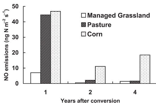
Fig. 8.14 Influence of conversion of natural grassland to cropland on average seasonal NO emission rates during 1st, 2nd and 4th year after conversion (Drawn from Pérez et al., 2007)
