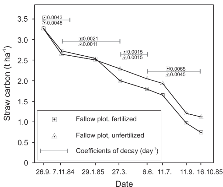
Fig. 5.1 Undecomposed straw carbon and decay coefficients ( \text{day}^{-1} ) for the decomposition phases. The straw ( 8 \text{ t dry matter ha}^{-1} ; C:N: 103) was incorporated into a loess soil (Luvisol near Hannover, North Germany) within litter bags into a 35 cm Ap horizon. The initial C mass in straw was 3.2 \text{ t ha}^{-1} (Nieder & Richter, 1989; p. 417. Reproduced with kind permission from Wiley-VCH)
