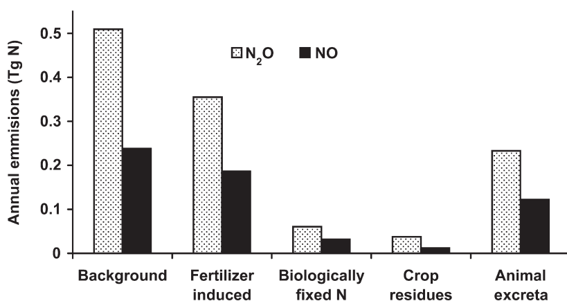
Fig. 8.11 Estimated emissions of \text{N}_2\text{O} and \text{NO} from croplands in East, Southeast and South Asia from different sources (Yan et al., 2003a. Reproduced with kind permission from Springer)
