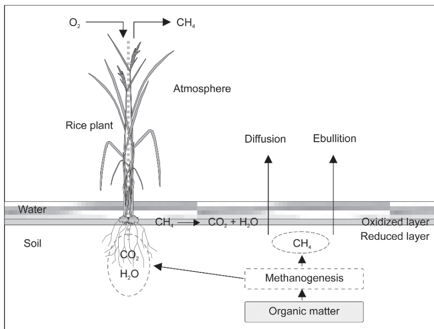
Fig. 8.8 Schematic representation of methane emission from rice fields
