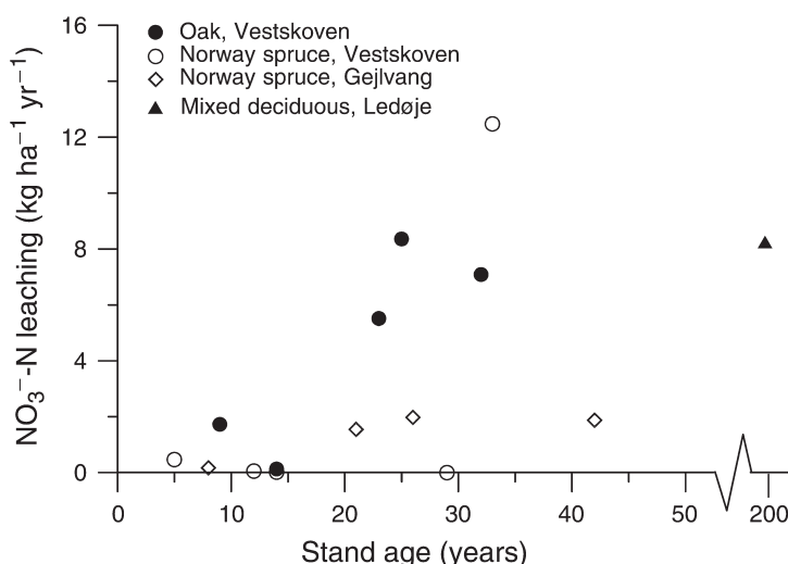
Fig. 7.6 Average annual \text{NO}_3^- -N leaching below the root zone at 90 cm depth as a function of time since afforestation in three chronosequences in Denmark (Hansen et al., 2007; p. 1257. Reproduced with kind permission from Wiley-Blackwell)
