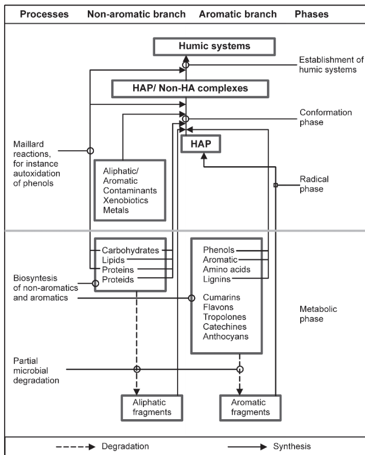
Fig. 3.2 Genesis of humic substances, HAP: humic acid precursors, HA: humic acids (Ziechmann & Müller-Wegener, 1990, p. 39. Reproduced with kind permission from Springer)
