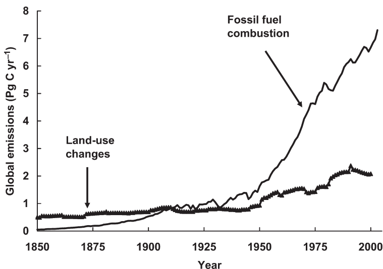
Fig. 8.3 Annual global \text{CO}_2 emission from fossil fuel burning and cement manufacture (1850–2003) and land-use changes (1850–2000) (Using data from CDIAC web site; Houghton & Hackler, 2002; Marland et al., 2006. Reproduced with kind permission from the Carbon Dioxide Information Analysis Center)
