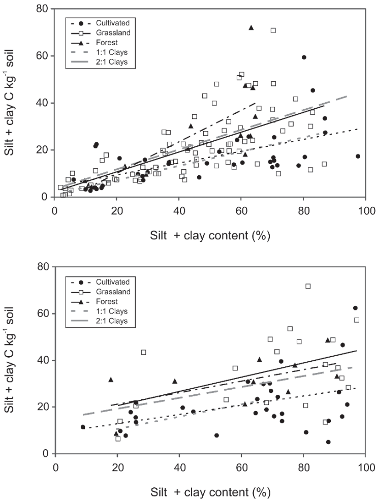
Fig. 3.8 Relationship between silt + clay content (%) and silt + clay associated C (g silt + clay C kg -1 soil) for grassland, forest and cultivated ecosystems. A differentiation between 1:1 and 2:1 clay dominated soils is also made. Figures (A) and (B) are for two silt + clay size boundaries viz. 0–20 μm and 0–50 μm, respectively (Six et al., 2002, p. 158. Reproduced with kind permission from Springer)
