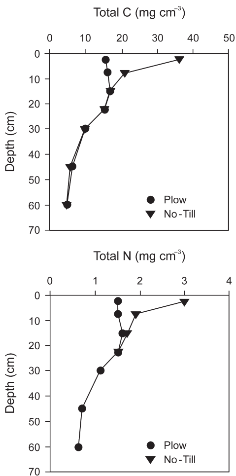
Fig. 6.12 Tillage treatment effects on SOC and SON within the upper 60 cm of a silt loam soil following 12 years of continuous corn (Karlen et al., 1994; p. 323. Reproduced with kind permission from Elsevier)
