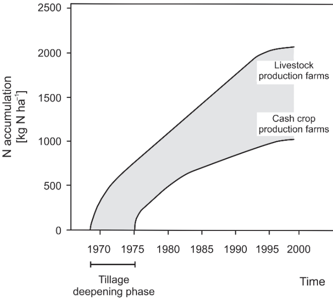
Fig. 6.10 N accumulation after deepening the tillage (16 farms, 120 plots) from <25 to >35 cm around 1970 (Southern Lower Saxony, North Germany) (Nieder et al., 2003c; p. 176. Reproduced with permission from the authors)
