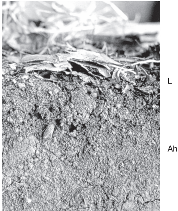
Fig. 3.9 L-Mull under beech ( Fagus sylvatica ) forest, Northrhine-Westphalia, Germany (soil: Calcaric Regosol). In Mull, the organic starting materials (L) are rapidly incorporated into the upper mineral soil horizon. Humified organic matter is homogenized with mineral particles form organo-mineral complexes (Photo: E. von Zezschwitz)
