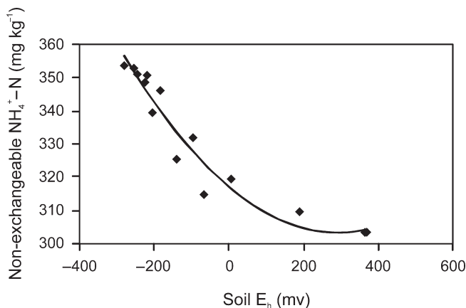
Fig. 5.10 Relationship between soil redox potential ( E_h ) and non-exchangeable NH_4^+-N in soil (Zhang & Scherer 2000; p. 519. Reproduced with kind permission from Springer)
