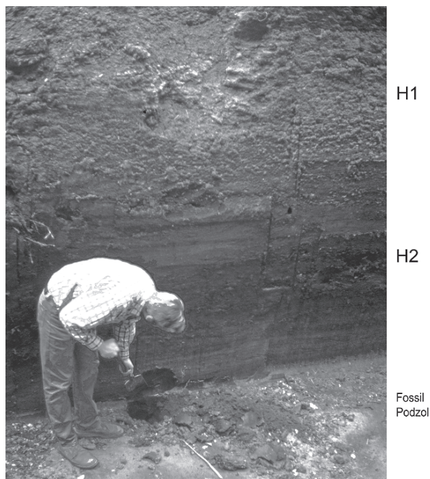
Fig. 1.18 Ombrogenous sphagnum moss peat Histosol (Fibric Histosol) of a raised bog with buried Podzol, Teufelsmoor near Bremen, North Germany. The peat consists mainly of Sphagnum moss which is weakly decomposed in the upper part (H1) and strongly decomposed in the lower part (H2) of the profile (Photo: R. Nieder)
