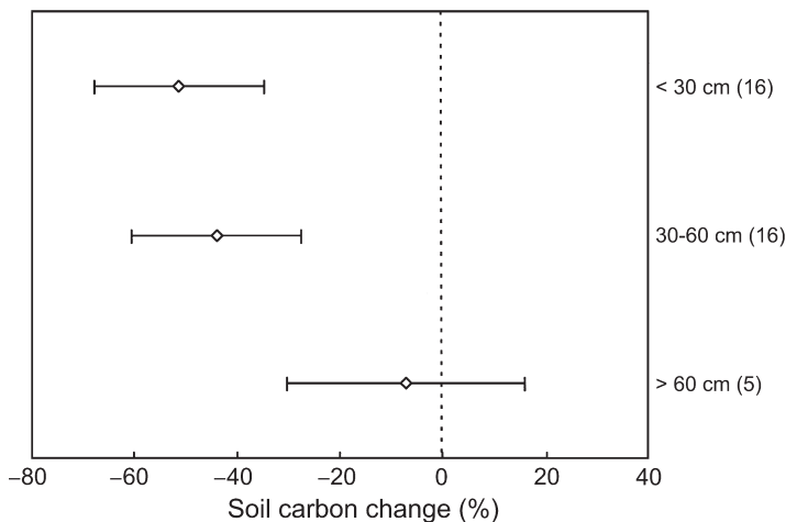
Fig. 6.6 Changes of SOC in different sampling depths after land use change from forest to crop (95% confidence intervals are shown and numbers of observations are in parenthesis) (Guo & Gifford, 2002; p. 351. Reproduced with kind permission from Wiley-Blackwell)
