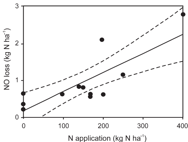
Fig. 8.12 Relationship between NO emission and fertilizer N application. Solid line represents regression ( R^2 = 0.64 ) and dashed lines indicate 95% confidence intervals (Veldkamp & Keller, 1997, p. 74. Reproduced with kind permission from Springer)
