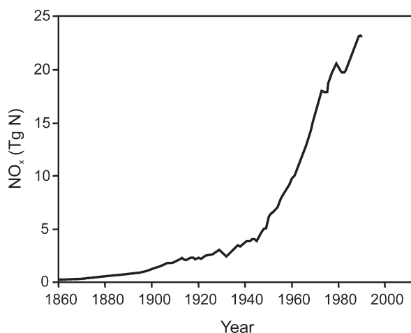
Fig. 8.10 Increase in global NO x emission from fossil fuel combustion since 1860 (Holland & Lamarque, 1997, p. 8. Reproduced with kind permission from Springer)
