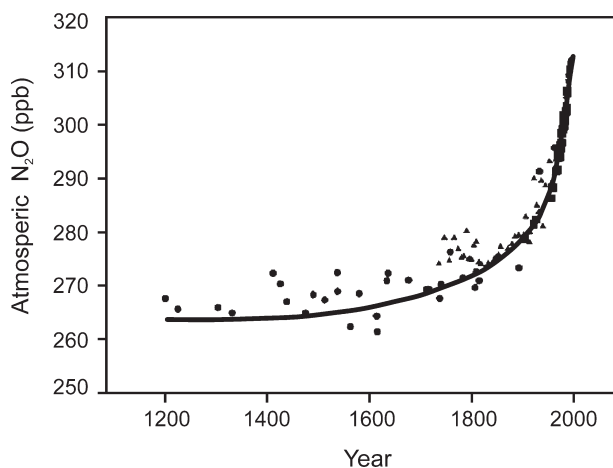
Fig. 8.9 Atmospheric N 2 O abundance trend since the year 1200 (Adapted from IPCC, 2001a. Reproduced with kind permission from Cambridge University Press)
