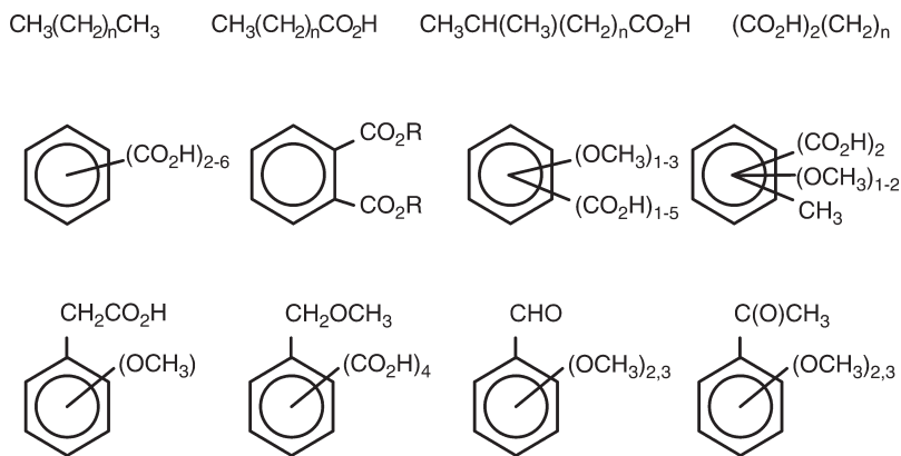
Fig. 3.3 Oxidation degradative products (Hayes, 1991, p. 12. Reproduced with kind permission from Woodhead Publishing Limited)
