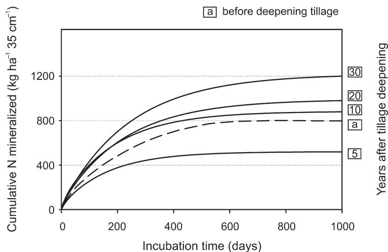
Fig. 6.11 Cumulative N mineralization (from incubation experiments) in Southern Lower Saxonian arable loess soils 5, 10, 20 and 30 years after deepening the tillage (Southern Lower Saxony, North Germany) (Nieder et al., 2003c; p. 176. Reproduced with permission from the authors)
