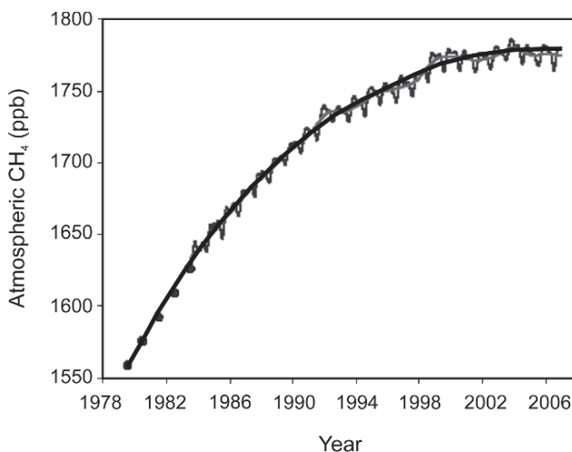
Fig. 8.6 Atmospheric \text{CH}_4 concentration from the NOAA global flask sampling network since 1978 ( http://www.esrl.noaa.gov/gmd/aggi/ ). Reproduced with kind permission from the US National Oceanic and Atmospheric Administration)
