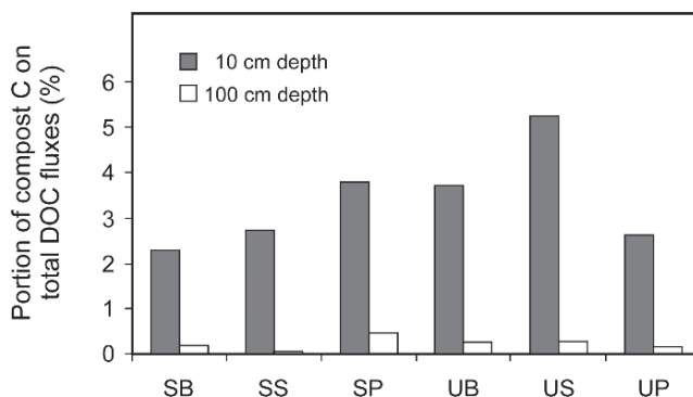
Fig. 7.2 Percent of compost C found in seepage fluxes at 10 and 100 cm depth in the Solling and Unterlüß beech (SB, UB), spruce (SS, US) and pine (SP, UP). (Borken et al., 2004; p. 95. Reproduced with kind permission from American Society of Agronomy, Crop Science Society of America & Soil Science Society of America)
