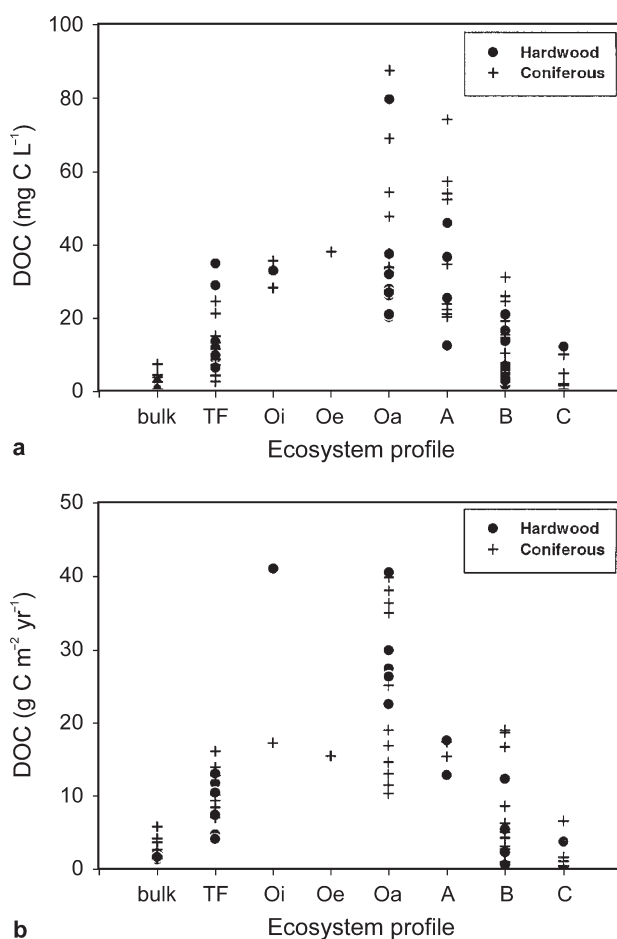
Fig. 7.1 (a) Mean annual concentration of DOC and (b) annual fluxes of DOC along a vertical profile in forest ecosystems [bulk: bulk precipitation; TF: throughfall precipitation; Oi: litter; Oe: fermented; Oa: humic layer (L, Of and Oh, respectively according to AG Boden, 2005); A, B and C: horizons of the mineral soil] (Michalzik et al., 2001; p. 187. Reproduced with kind permission from Springer)
