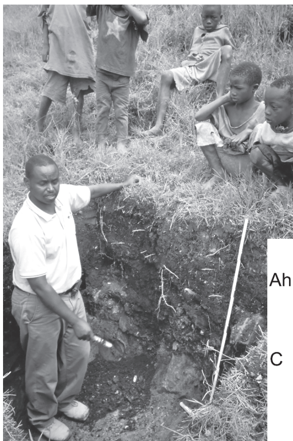
Fig. 1.14 Humic Umbrisol with an umbric Ah horizon overlying palaeozoic sandstone, near Gatumba, Central Rwanda (Photo: R. Nieder)
