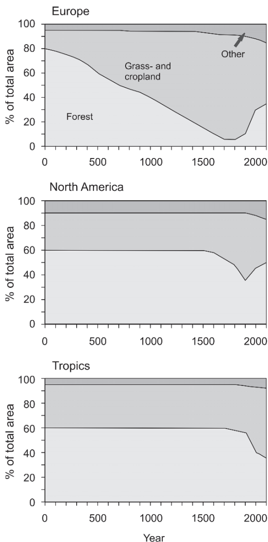
Fig. 6.1 Schematic figure indicating historical changes in land use in three world regions (Apps et al., 2001; p. 310. Reproduced with kind permission from Technical Support Unit Working Group III, IPCC)
