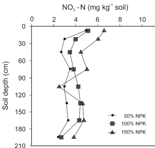
Fig. 7.4 Influence of fertilizer application rates on residual \text{NO}_3^- -N in soil profile after 16 cycles of corn-wheat-cowpea (fodder) cropping (Benbi et al., 1991a; p. 176. Reproduced with kind permission from Springer)
