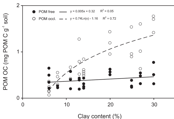
Fig. 3.6 Relationship between organic carbon content for free and occluded POM fractions and clay content (Köbl & Kögel-Knabner, 2004, p. 49. Reproduced with kind permission from Wiley-VCH)
