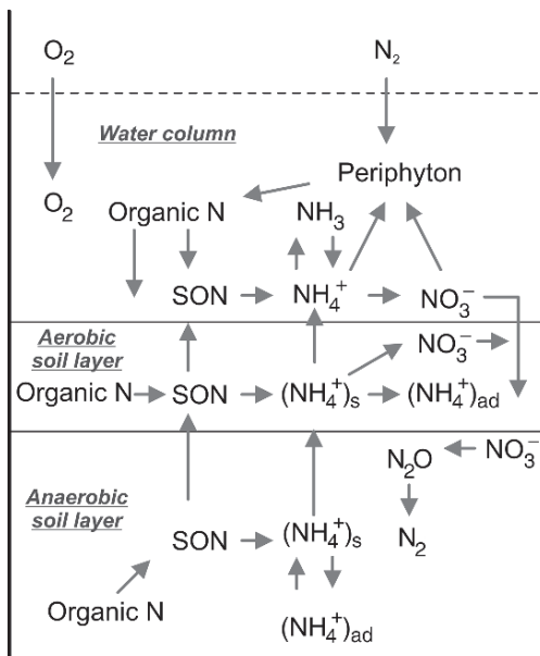
Fig. 2.4 The nitrogen cycle in wetland soils showing the N transformations in aerobic and anaerobic layers (DeBusk et al., 2001, p. 37. Reproduced with kind permission from Taylor & Francis, Copyright Clearance Center)
