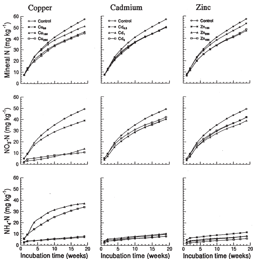
Fig. 5.6 Effect of heavy metal (Cu, Cd and Zn) additions on N mineralization and nitrification in a sandy soil. The numbers as subscripts to the metals indicate the rate of application ( \text{mg kg}^{-1} soil) (Benbi & Richter, 1996; p. 20. Reproduced with kind permission from Springer)
