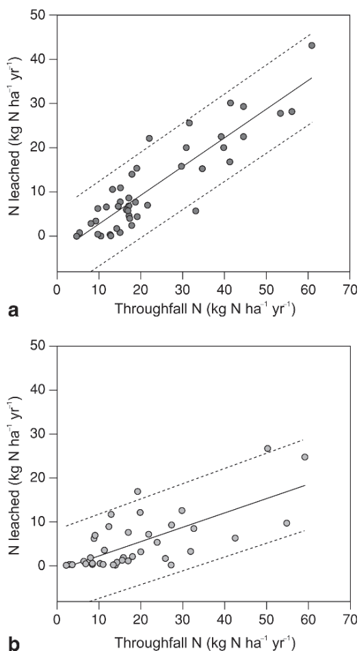
Fig. 7.5 Relationship between N input in throughfall and \text{NO}_3^- -N leached at (a) sites where the organic layer C:N ratio is \leq 25 and (b) sites where the organic layer C:N ratio is > 25 (MacDonald et al., 2002; p. 1031. Reproduced with kind permission from Wiley-Blackwell)
