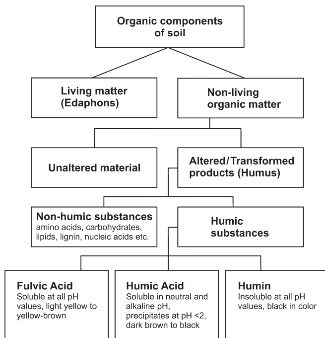
Fig. 3.1 Schematic representation of organic components of soil
