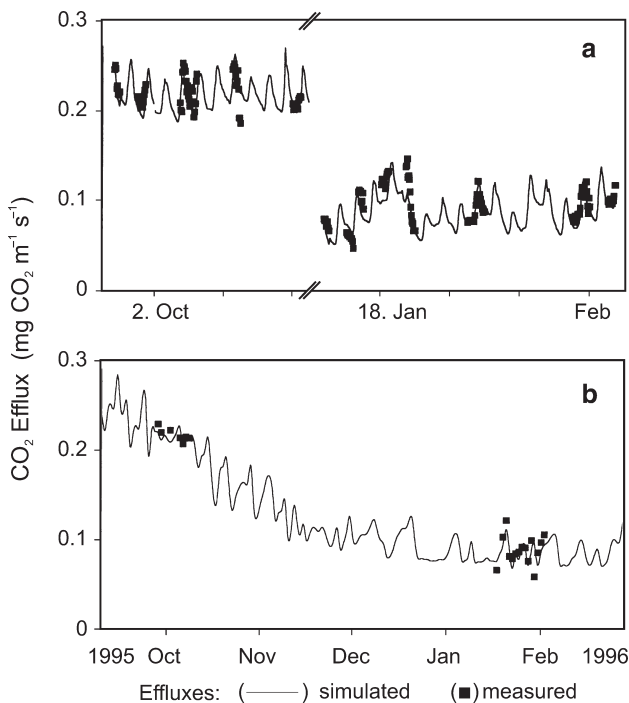
Fig. 9.2 Comparison between measured and simulated hourly (a) and daily average (b) \text{CO}_2 efflux in a slash pine plantation, Florida. Points represent measurements and lines represent simulations (Moncrieff & Fang, 1999, p. 241. Reproduced with kind permission from Elsevier)
