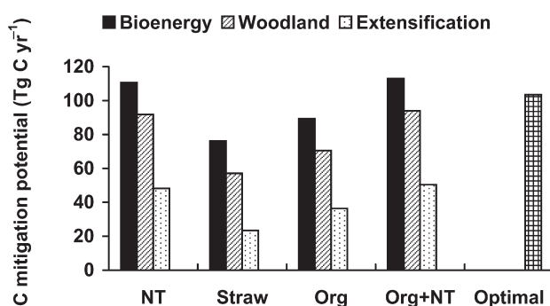
Fig. 8.5 Maximum yearly carbon mitigation potential in Europe through different combinations of land management scenario using 10% surplus arable either for bioenergy production or woodland regeneration or extensification and other management practices viz. no-tillage (NT), straw incorporation (Straw), application of organic amendments (Org). Optimal scenario uses 50% of surplus arable land for bioenergy production and the other 50% for woodland, application of organic amendments at the highest rates allowed and putting the remaining area into no-till (Adapted from Smith et al., 2000b)
