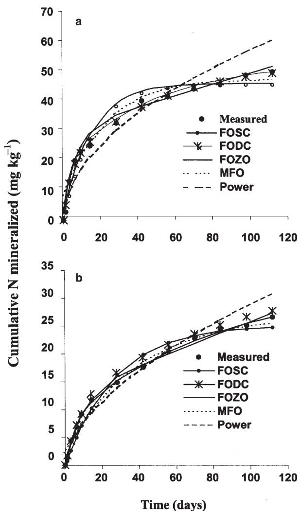
Fig. 9.5 Typical fit of different models to cumulative N mineralization in a sandy loam (a) and a clay loam (b) soil from northwestern India (Haer & Benbi, 2003, p. 163. Reproduced with kind permission from Taylor & Francis, Copyright Clearance Center)
