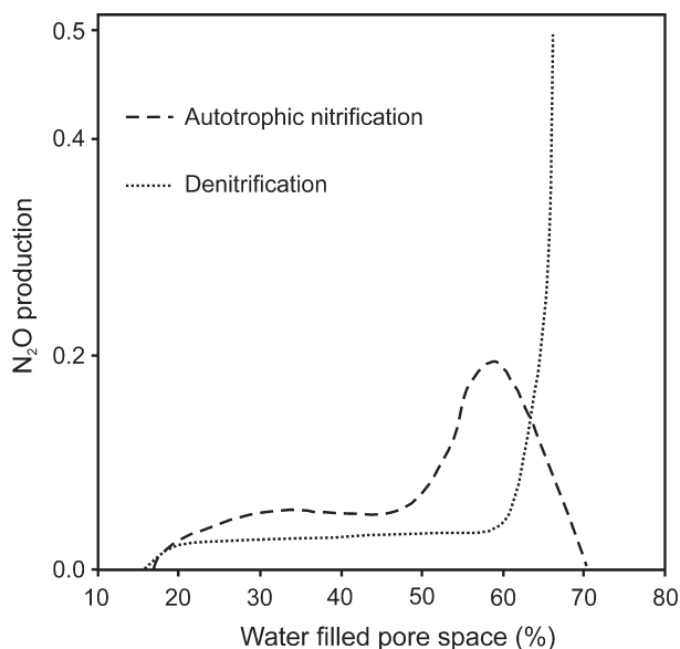
Fig. 8.13 Schematic representation of the influence of water filled pore space on the contribution of nitrification and denitrification towards \text{N}_2\text{O} emissions from soil (Bateman & Baggs, 2005. Reproduced with kind permission from Springer)
