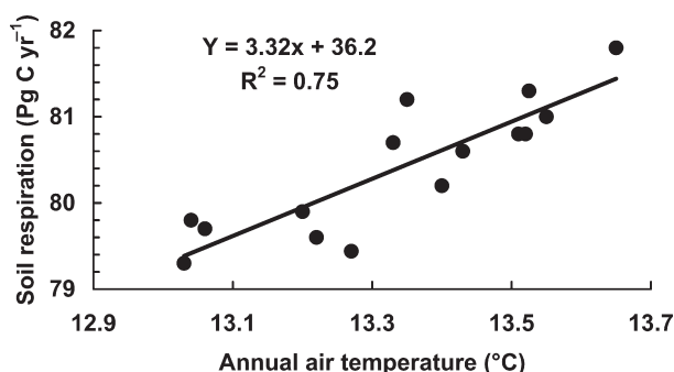
Fig. 9.1 Relationship between estimated global soil respiration and mean annual air temperature over land during 1980 to 1994 (Raich et al., 2002, p. 809. Reproduced with kind permission from Wiley-Blackwell)
