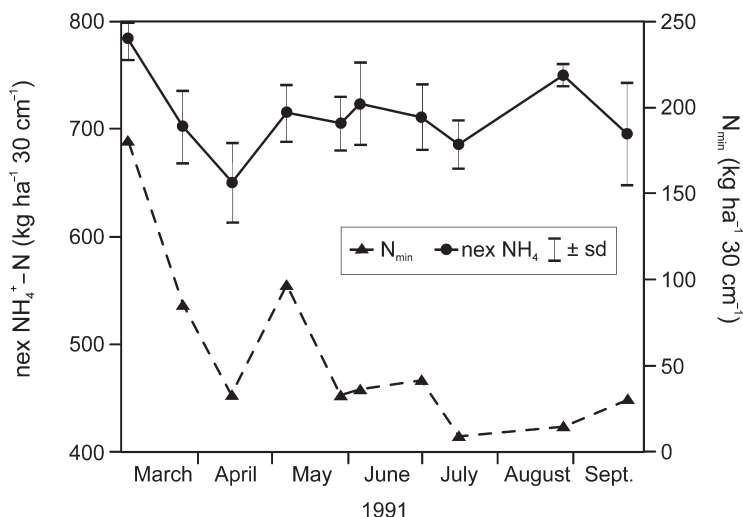
Fig. 5.9 Dynamics of non-exchangeable (nex) \text{NH}_4^+ and mineral N ( \text{N}_{\text{min}} ) in a phaeozem \text{A}_p horizon cultivated to winter wheat with conventional N application (Nieder et al., 1996; p. 182. Reproduced with kind permission from Springer)
