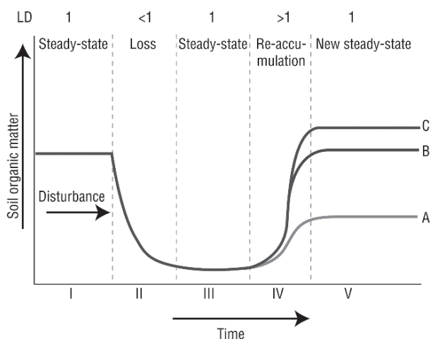
Fig. 6.3 Conceptual scheme of SOM decomposition following disturbance and reaccumulation. Under steady-state conditions (I), C input (“In”) from plant residues equal C losses (“Out”) via SOM decomposition (In/Out = 1). Due to disturbance, “Out” often exceeds “In”, resulting in a loss of SOC (II), until a new but lower steady state is reached (III). Introduction of management systems where “In” exceeds “Out” results in a re-accumulation of SOC (IV) until a new but higher steady state is reached (V). The level of the new steady state (A, B or C) depends on the management that was introduced (Apps et al., 2001; p. 313, adapted from Johnson, 1995; IPCC, 2000c. Reproduced with kind permission from Technical Support Unit Working Group III, IPCC)
