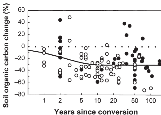
Fig. 6.7 Changes in SOC (% of original C content) after conversion of forest to cultivated soil. Closed circles (•) show data where bulk density effects have been considered by the authors, and open circles (○) show data with remaining uncertainty about the procedures (Murty et al., 2002; p. 108. Reproduced with kind permission from Wiley-Blackwell)
