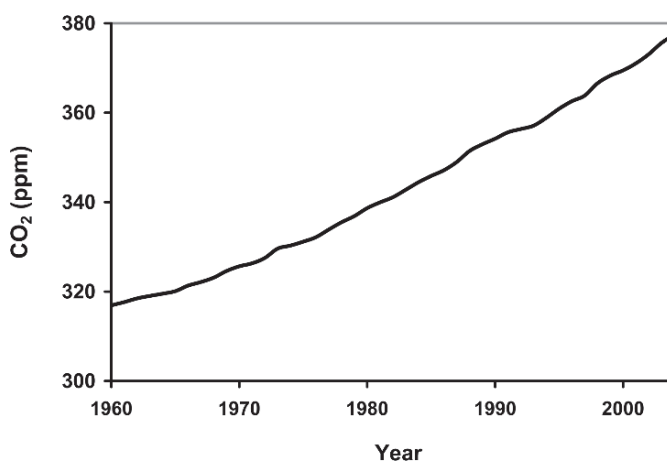
Fig. 8.2 Atmospheric CO_2 concentration derived from in situ air samples collected at Mauna Loa, Hawaii (Using data from Keeling & Whorf, 2005. Reproduced with kind permission from the Carbon Dioxide Information Analysis Center)
