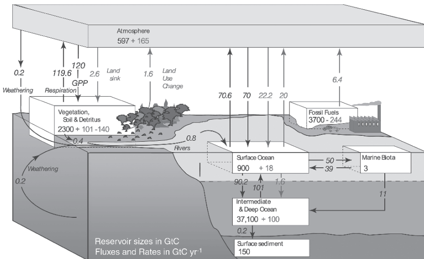
Fig. 2.1 The global carbon cycle for the 1990s showing the main annual fluxes in \text{Pg C year}^{-1} . The preindustrial fluxes are given in black and anthropogenic fluxes in grey (Denman et al., 2007, p. 515. Reproduced with kind permission from Cambridge University Press)
