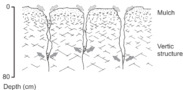
Fig. 1.15 Peloturbation occurring in Vertisols. The drawing shows the shrinking state during the dry season, with soil material (granules or crumbs) falling from the surface mulch layer into the cracks. Subsequent re-wetting generates pressure which results in sliding of soil masses along each other (Adapted from Driessen & Duda, 1991)
