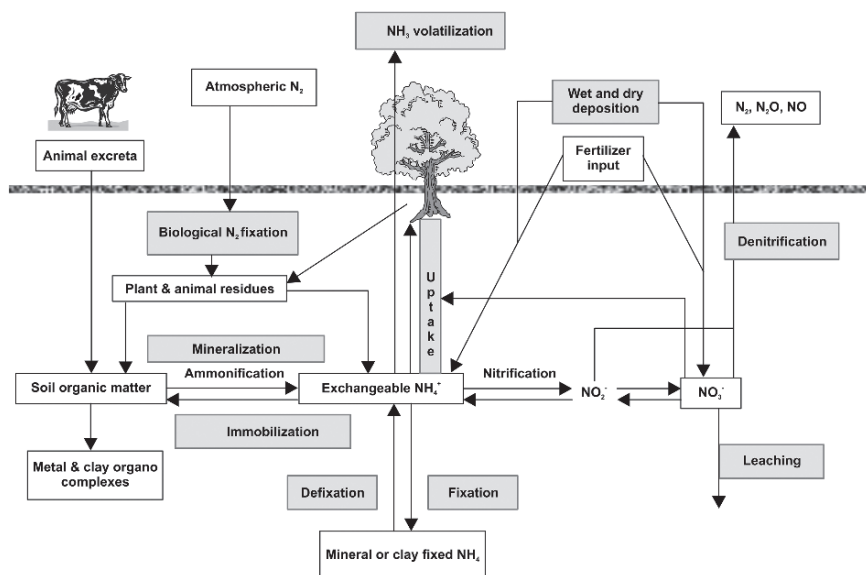
Fig. 2.3 The nitrogen cycle in upland soils (Benbi & Richter, 2003, p. 410. Reproduced with kind permission from Haworth Press)
