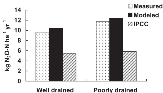
Fig. 9.4 Comparison of measured, modeled and IPCC-calculated annual nitrous oxide emissions from two dairy grazed pasture sites in New Zealand (Adapted from Saggar et al., 2004a)
