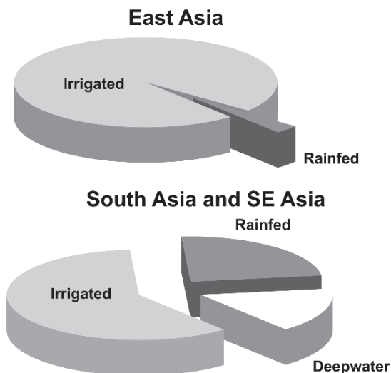
Fig. 8.7 Seasonal emission potential of different rice ecosystems in East, South and Southeast (SE) Asia (Adapted from Wassmann et al., 2000)
