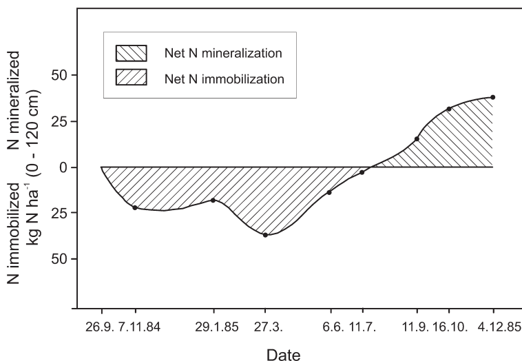
Fig. 5.4 Course of immobilization and remobilization of fertilizer-N and native soil-N in a microplot experiment on a loess soil (Luvisol, near Hannover, Germany) during the vegetation period of winter wheat (Nieder & Richter, 1989; p. 419. Reproduced with kind permission from Wiley-VCH)
