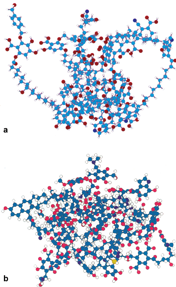
Fig. 3.4 Geometrically optimized three-dimensional structure of (a) soil humic acid and (b) soil organic matter. The element colors are: white H, cyan C, red O, blue N, yellow S (Schulten & Schnitzer, 1997, p. 120; Schulten & Leinweber, 2000, p. 414. Reproduced with kind permission from Wolters Kluwer Health; Lippincott Williams & Wilkins)
