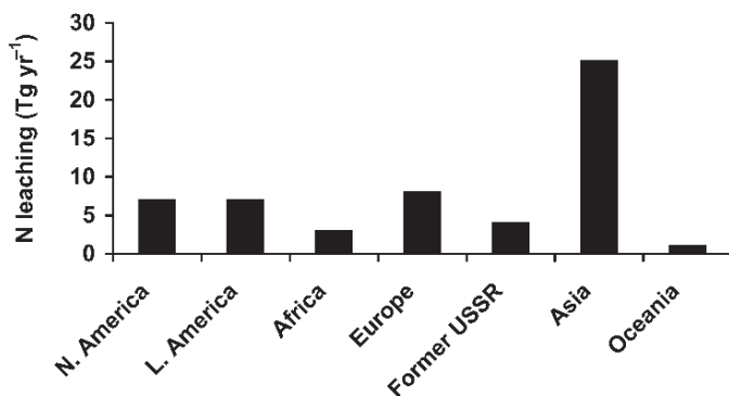
Fig. 7.3 Calculated regional leaching losses of nitrogen from agricultural soils (Drawn from data presented in Van Drecht et al., 2003)
