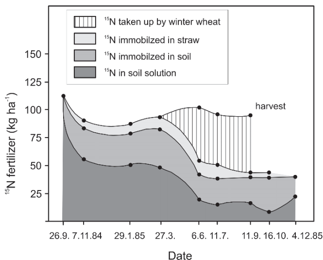
Fig. 5.3 Distribution of ^{15}\text{N} fertilizer in different pools (soil solution, soil matrix, incorporated straw, N uptake by wheat) of a microplot experiment on a loess soil (Luvisol) near Hannover, Germany) during the vegetation period of winter wheat (Nieder et al., 1993; p. 298. Reproduced with kind permission from Wiley-VCH)
