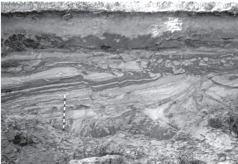
Fig. 1.11 Cryoturbation (relictic) in a Podzol, near Ülzen, North Germany. Freeze-thaw cycles in (ant)arctic regions are responsible for cryoturbation. At the beginning of the frost phase, freezing fronts in the thawed layer move both from the soil surface downwards and from the permafrost table upwards. As a result, unfrozen materials are displaced and soil horizons are contoured and broken (Photo: R. Nieder)
