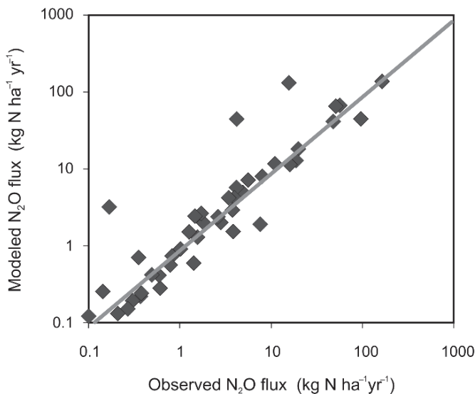
Fig. 9.3 Comparison of modeled and observed \text{N}_2\text{O} fluxes from agricultural sites in the US, Canada, the UK, Germany, China, New Zealand, Costa Rica and Zimbabwe (Saggar et al., 2004b, p. 2. Reproduced with kind permission from The Regional Institute Ltd.)
