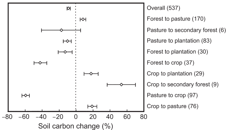
Fig. 6.5 Response of SOC to various land use changes including 537 observations from 74 publications (95% confidence intervals are shown and numbers of observations are in parenthesis) (Guo & Gifford, 2002; p. 374. Reproduced with kind permission from Wiley-Blackwell)
