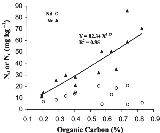
Fig. 9.6 Relationship of nitrogen mineralization potential of easily decomposable ( N_d ) and recalcitrant fraction ( N_r ) estimated from first-order two compartment model (Haer & Benbi, 2003, p. 161. Reproduced with kind permission from Taylor & Francis, Copyright Clearance Center)
