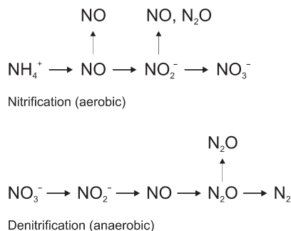
Fig. 5.7 Emission of oxides of nitrogen through nitrification and denitrification processes in soil
