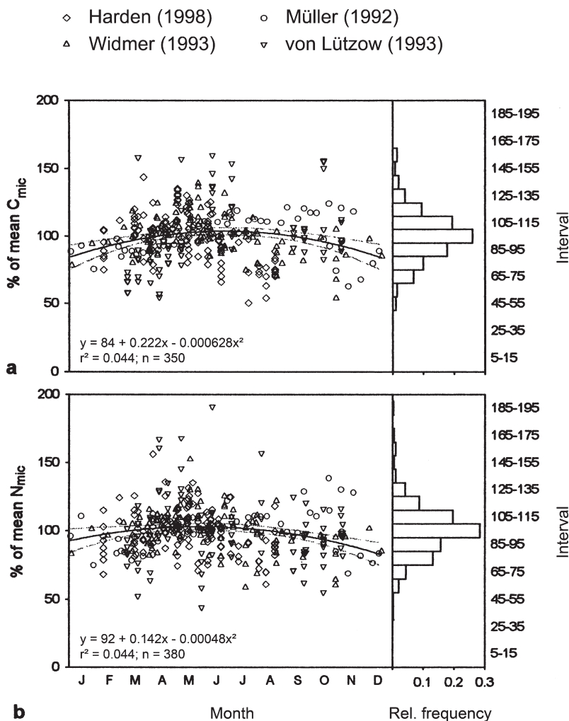
Fig. 5.2 Seasonal microbial biomass (a) C ( C_{mic} ) and (b) N ( N_{mic} ) dynamics drawn from four field studies (15 field plots) in Germany. Single measurements include different sites, replicates and treatments (e.g., different amounts and kinds of N fertilizers). They are given in percent of mean microbial biomass C and N contents. Solid lines indicate the regression line, the dashed line the 95% confidence interval of the regression. Horizontal bars indicate the relative frequency (Nieder et al., in press. Reproduced with kind permission from Wiley-VCH)
