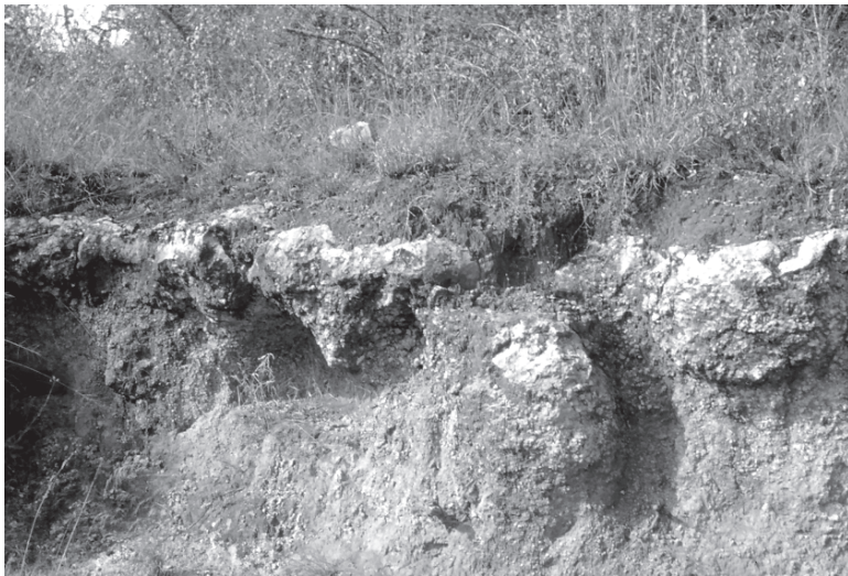
Fig. 5.5 Calcisol exhibiting a compact calcrete horizon (cementation by calcite) (Photo: origin unknown)
