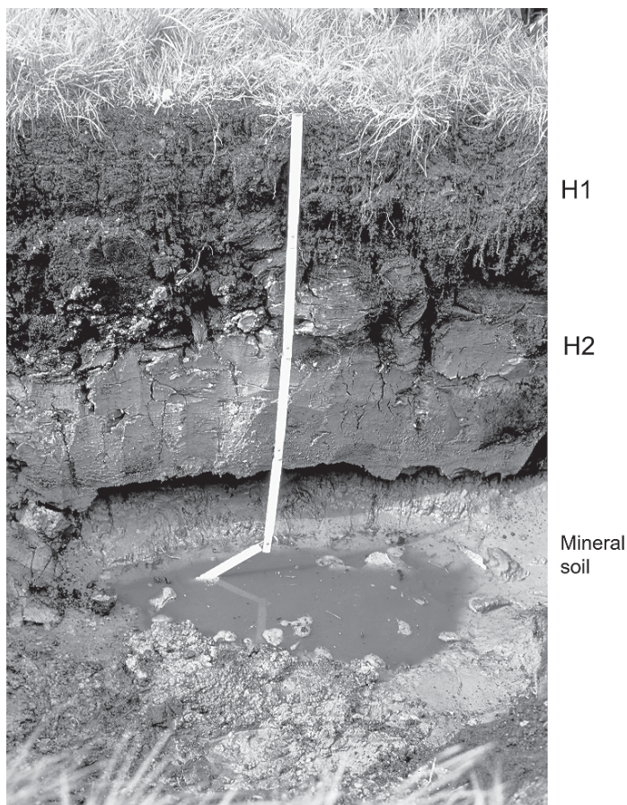
Fig. 1.19 Topogenous low moor peat Histosol (Eutric Histosol) showing a terric H1 and a sapric H2 horizon, Ochsenmoor near Osnabrück, North Germany (Photo: R. Nieder)
