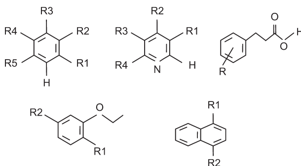
Fig. 3.5 Structural components of humic substances (Piccolo, 2002, p. 99. Reproduced with kind permission from Elsevier)
