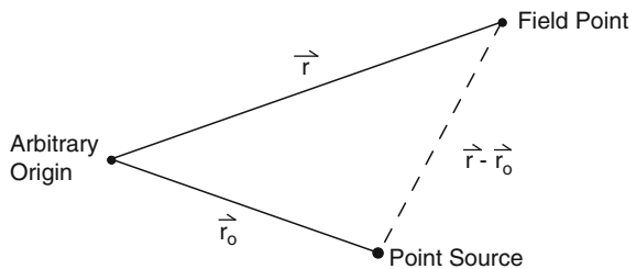
Fig. 11.10 Coordinates for defining Green's functions
