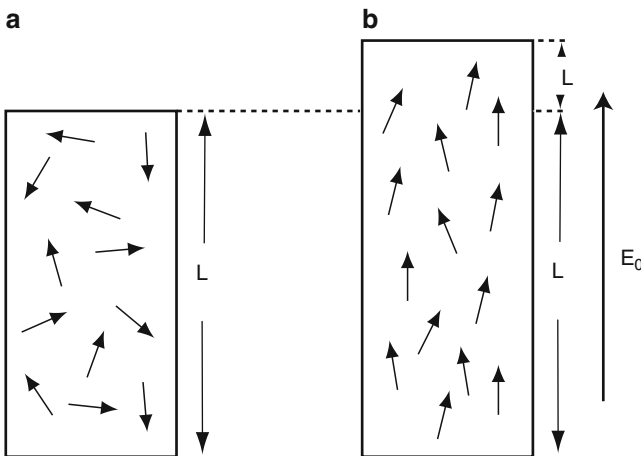
Fig. 2.2 Polarization of a ferroelectric, electrostrictive material occurs when randomly oriented dipole moments (a) are approximately aligned (b) by a strong, steady electric field, E_0 . The material also increases in length in the direction of E_0
