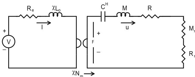
Fig. 3.22 Gyrator circuit representation of Fig. 3.19
