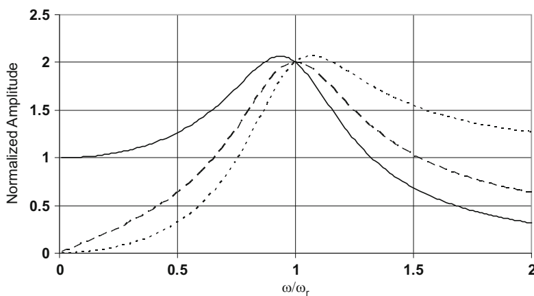
Fig. 4.1 Normalized displacement, x_n , (solid line), velocity, u_n , (dashed line), and acceleration, a_n , (dotted line) vs. normalized frequency for the simple vibrator in Fig. 3.1 for Q_m = 2
