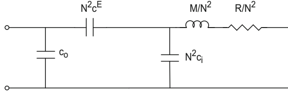
Fig. 4.6 Circuit with glue bond or insulating layer of stiffness K_i = 1/c_i
