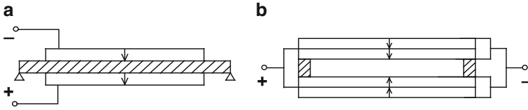
Fig. 5.57 Trilaminar (a) and dual bilaminar (b) bender disc designs
