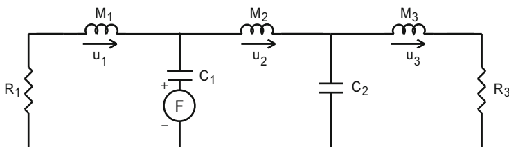
Fig. 3.12 Electrical equivalent circuit of Fig. 3.11
