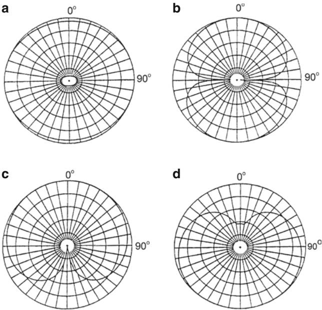
Fig. 5.42 Measured single element 900 Hz radiation patterns operating in the (a) quadrupole mode, (b) dipole mode, (c) directional mode, and (d) directional mode drive leads reversed (10 dB/division) [70]
