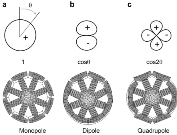
Fig. 5.64 Monopole, dipole, and quadrupole modes with corresponding beam patterns
