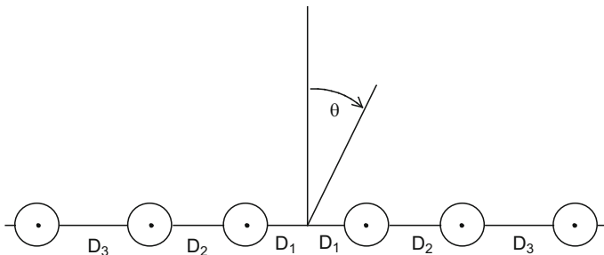
Fig. 7.8 Line array with non-uniform spacing. Geometric spacing with R = 1.5
