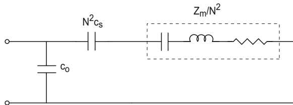
Fig. 4.5 Circuit with stress rod of stiffness K_s = 1/c_s
