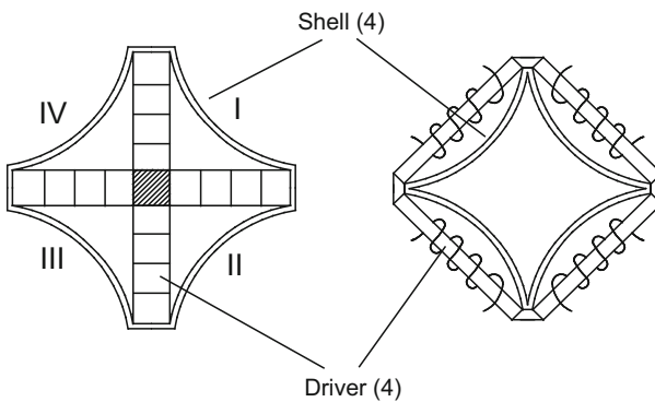
Fig. 5.48 Internally and externally driven Astroid flextensional transducer [71]
