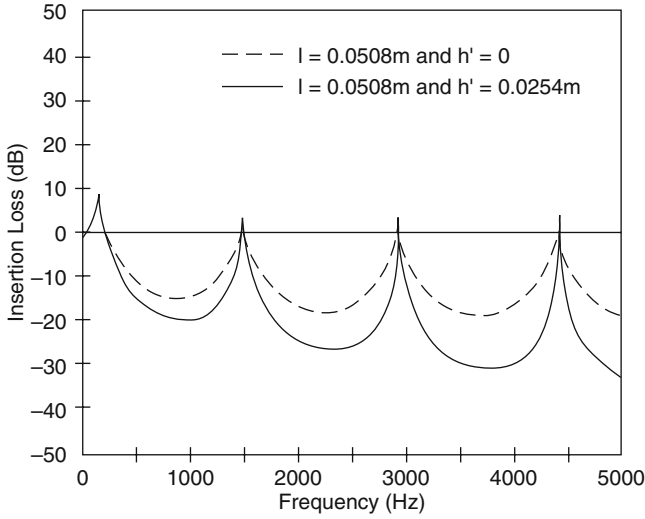
Fig. 8.17 Flexural wave insertion losses for line-force excitation at standoff distance d = 0.0254 m for a steel plate with thickness h = 0.0508 m. E = E' = 1.9 \times 10^{10} , \sigma = \sigma' = 0.28 , \rho_s = \rho_s' = 7700 kg/m 3 , \zeta = \zeta' = 0.1 (material damping factor), \rho_1 = 1000 kg/m 3 , c_1 = 150 m/s, \rho_o = 1000 kg/m 3 , c_o = 1500 m/s [41], with permission from the Acoustical Society of America
