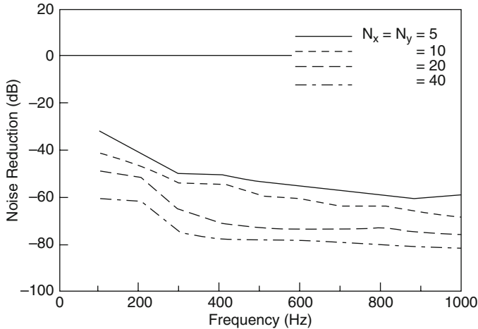
Fig. 8.23 Effect of the number of hydrophones (without inter-hydrophone spacing) embedded within an elastomer layer 2 in. thick, [46], with permission from the Acoustical Society of America
