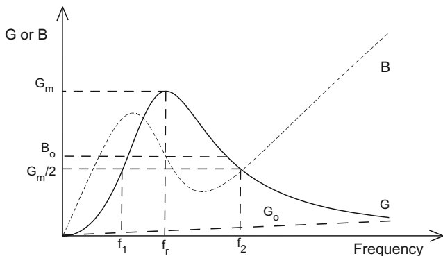
Fig. 9.5 Conductance, G , and susceptance, B , for an electric field transducer
