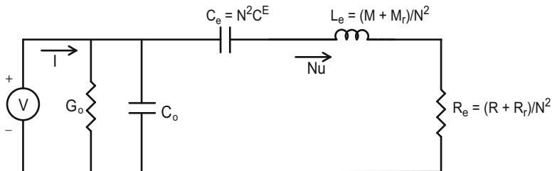
Fig. 3.16 All electric circuit representation of the circuit of Fig. 3.15
