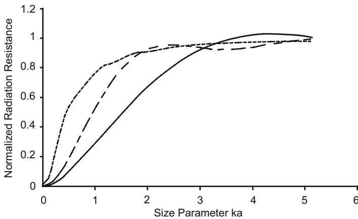
Fig. 11.5 Normalized radiation resistance for uniform motion of the cylinder, mode n=0 , for h/2a = 0.5 (solid line), 1.0 (dash line), and 5.0 (dotted line) [25]
