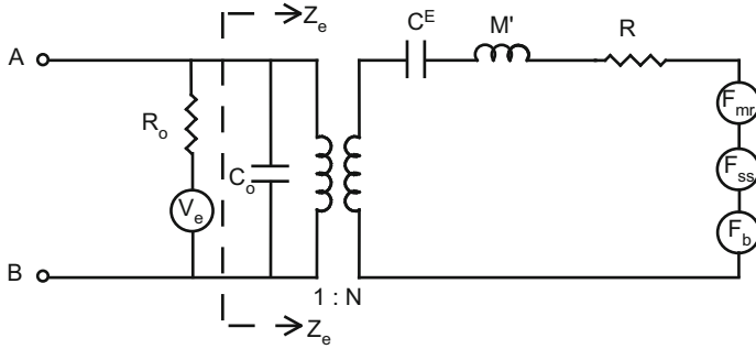
Fig. 13.11 Reduced equivalent circuit where R = R_m + R_r and M' = M_m + M_r
