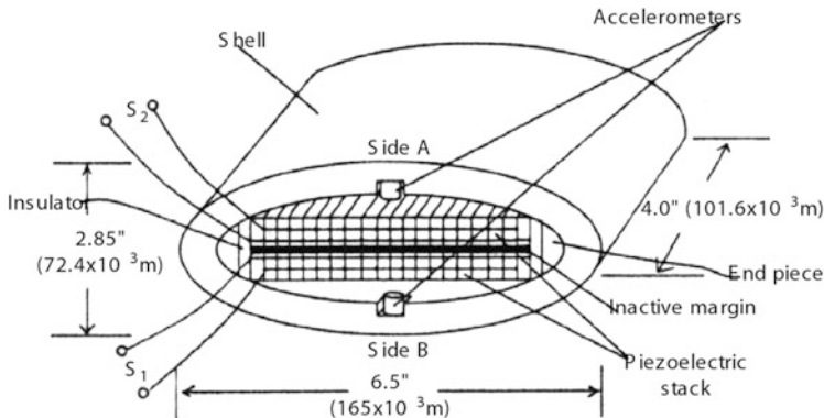
Fig. 1.14 Sketch of a Class IV flextensional transducer with inactive central section for operation in a dipole mode [32]. Shell and interface by John Oswin, British Aerospace England
