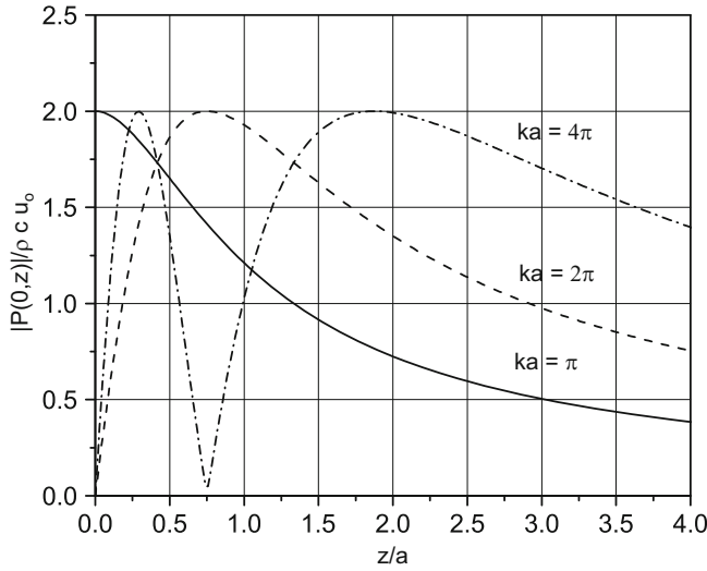
Fig. 10.13 Pressure amplitude on the axis of a circular piston for ka = \pi where the only maximum is on the surface, for ka = 2\pi and ka = 4\pi
