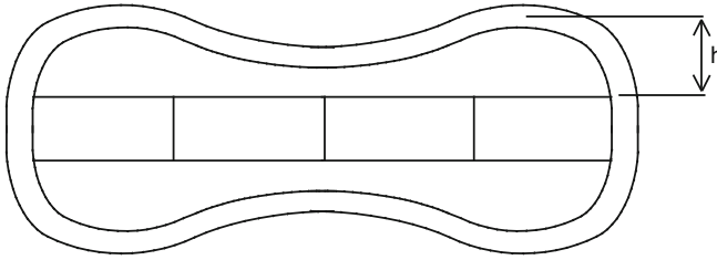
Fig. 5.43 Class VII “dog bone” flextensional transducer
