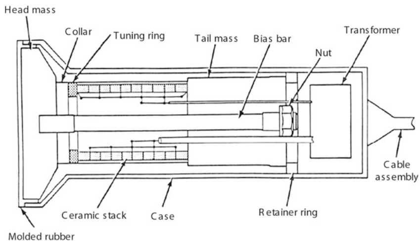
Fig. 1.6 Sketch of high power low frequency Tonpilz transducer with head and tail mounting system and steel housing case
