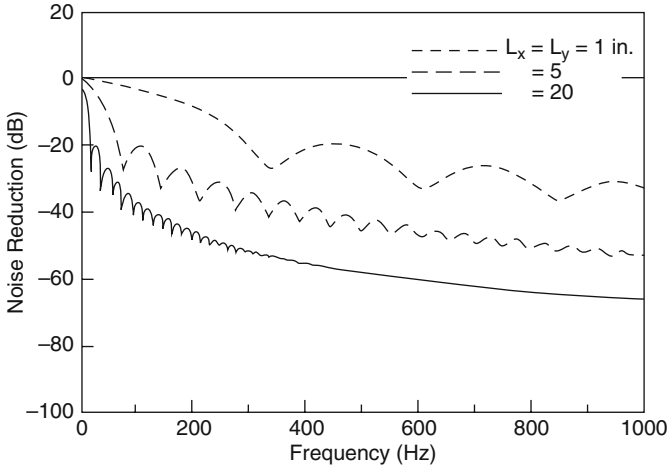
Fig. 8.21 Effect of hydrophone dimensions (flush mounted) on turbulent flow noise reduction [46], with permission from the Acoustical Society of America
