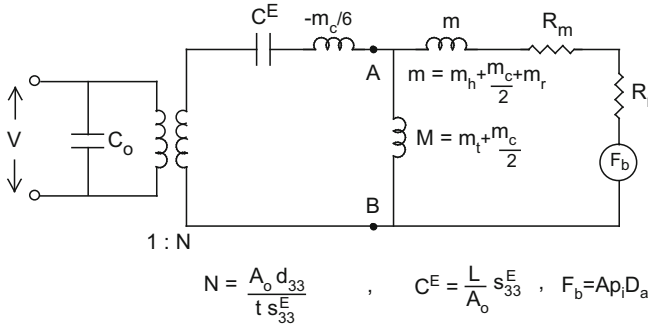
Fig. 6.14 Lumped mass equivalent circuit of Tonpilz hydrophone with t = L/n
