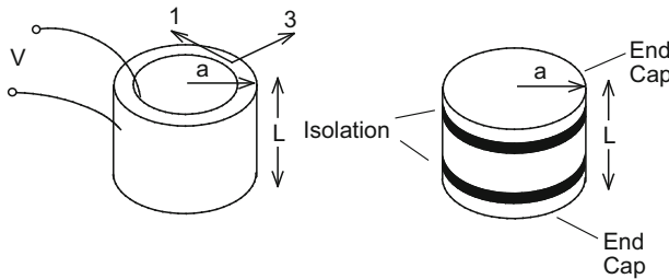
Fig. 6.8 Piezoelectric ring (tube) polarized in the radial (3) direction and operated in the 31-mode with isolated ends caps
