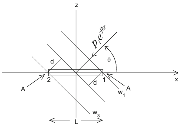
Fig. 6.22 Force on tube of length L and cross-sectional area A
