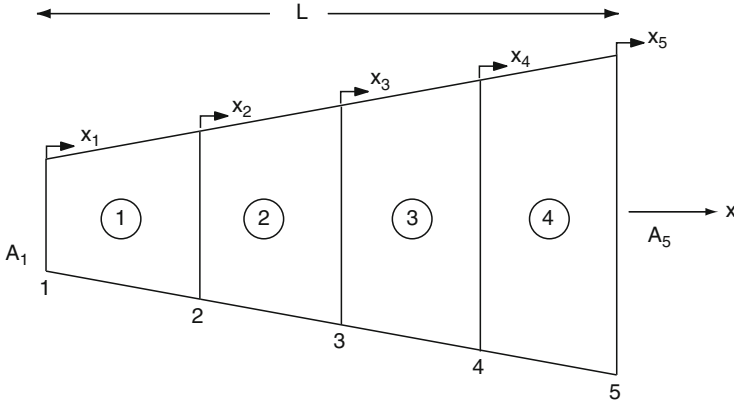
Fig. 3.47 Bar with variable cross-sectional area A_i
