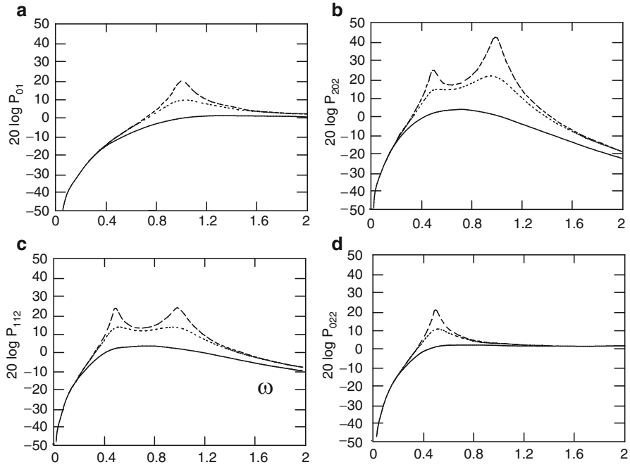
Fig. 12.4 Normalized pressure P (in dB) as a function of the dimensionless frequency, \nu , for the (a) linear fundamental and second harmonics caused by (b) X^2 , (c) X \cos \omega t , and (d) \cos 2\omega t for Q_m = 1 (solid line), 3 (dotted line), and 10 (dashed line) [3]
