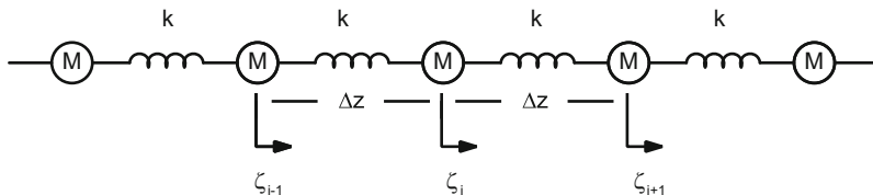
Fig. 3.26 Lumped mode representation of the bar of Fig. 3.25
