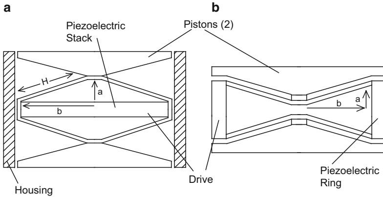
Fig. 5.50 X-spring version of the Class IV (a) and Class VI (b) flextensional transducer [72]
