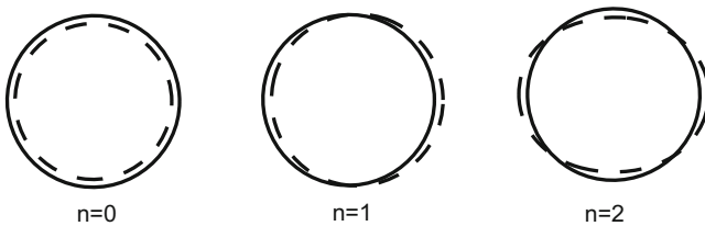
Fig. 5.14 Omni, dipole, and quadrupole ring modes of vibration
