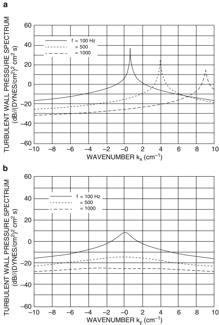
Fig. 8.14 Turbulent wall pressure spectra for flow speed of 20 knots as a function of (a) k_x ( k_y = 0 ) and (b) k_y ( k_x = 0 ) for different frequencies [46], with permission from the Acoustical Society of America. Note use of cgs units on this figure
