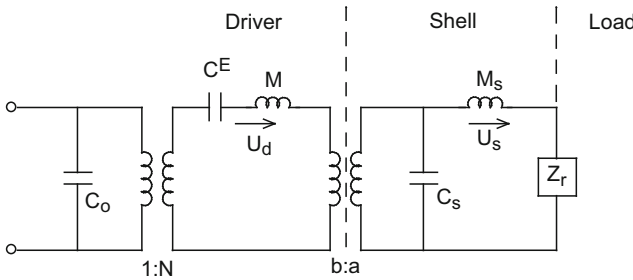
Fig. 5.39 Simplified flextensional equivalent circuit
