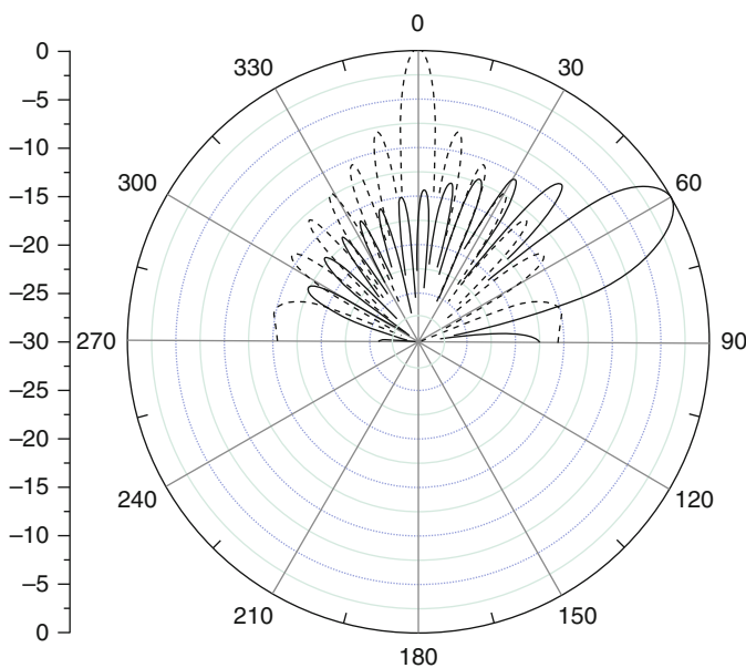
Fig. 8.31 Continuous circular ring ka = 20 without (dashed lines) and with (solid lines) steering to 60^\circ
