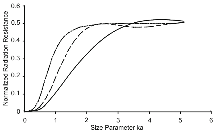
Fig. 11.7 Normalized radiation resistance for dipole motion of the cylinder, mode n=1 , for h/2a=0.5 (solid line), 1.0 (dash line), and 5.0 (dotted line) [25]
