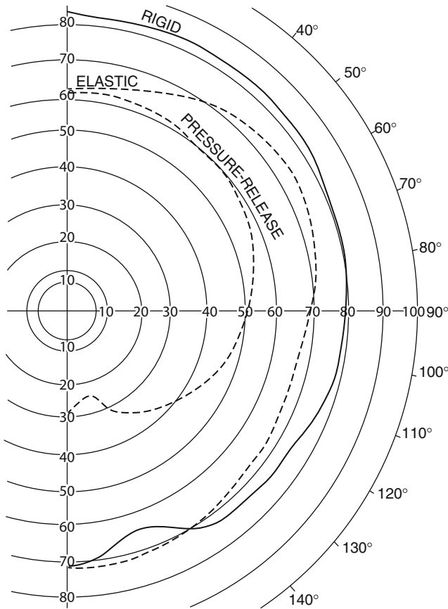
Fig. 11.14 Far-field beam patterns in the horizontal plane of the source in Fig. 11.12 at 1800 Hz for rigid (solid line), elastic (dash line), and pressure-release (dotted line) cylinders [47]
