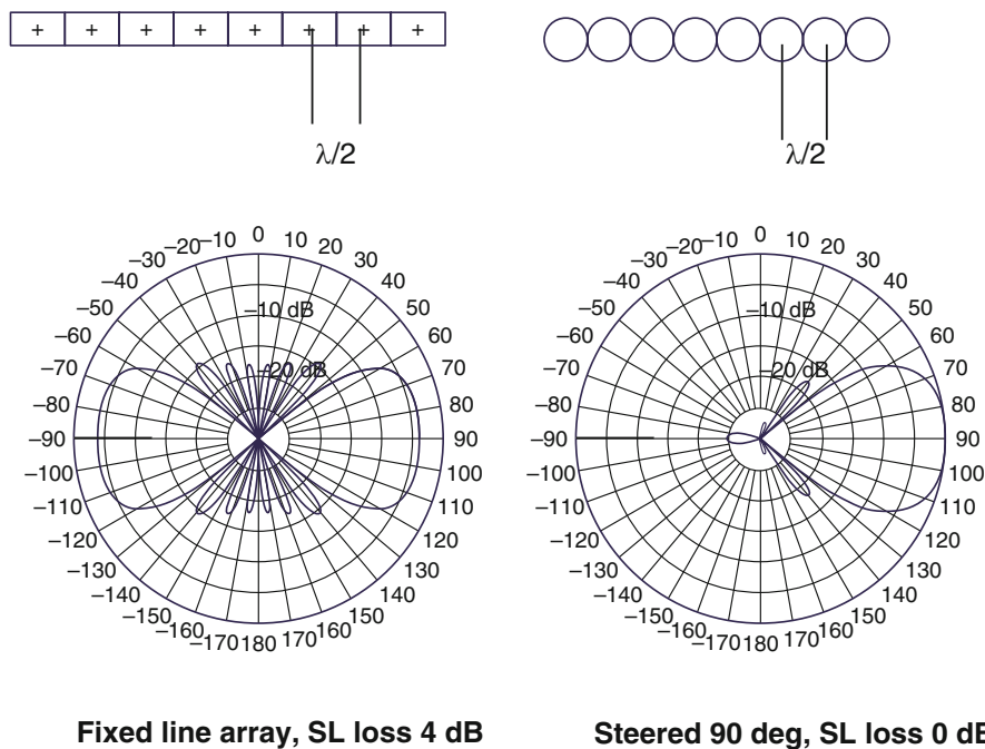
Fig. 7.22 Comparison of leveraged cylindrical transducer end-fire line array beam pattern with conventional line array
