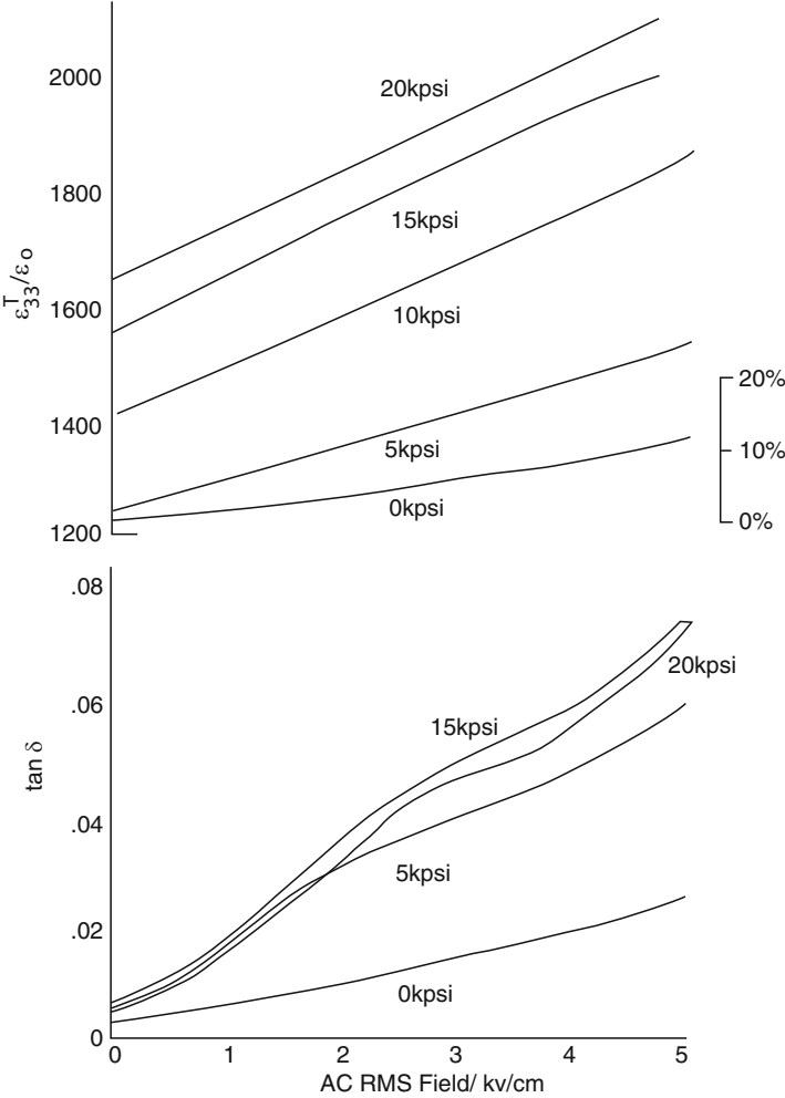
Fig. 13.7 \epsilon_{33}^T/\epsilon_0 and \tan \delta vs. AC field. Parameter; parallel stress ( T_3 ) PZT-4
