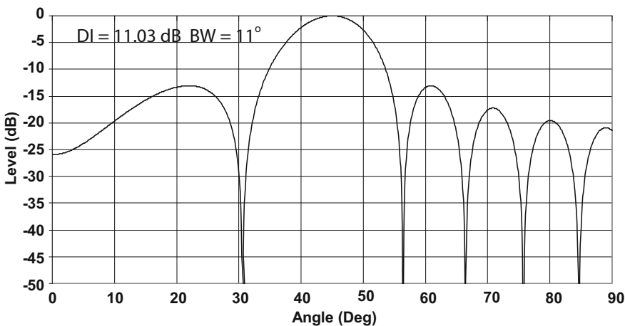
Fig. 8.4 Unshaded 12 element \lambda/2 spaced array steered to 45^\circ
