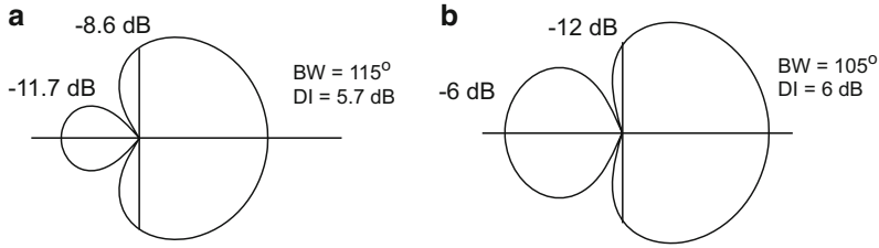
Fig. 6.31 Super cardioid (a) and hyper cardioid (b) beam patterns
