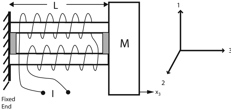
Fig. 2.7 The 33 mode magnetostrictive longitudinal vibrator
