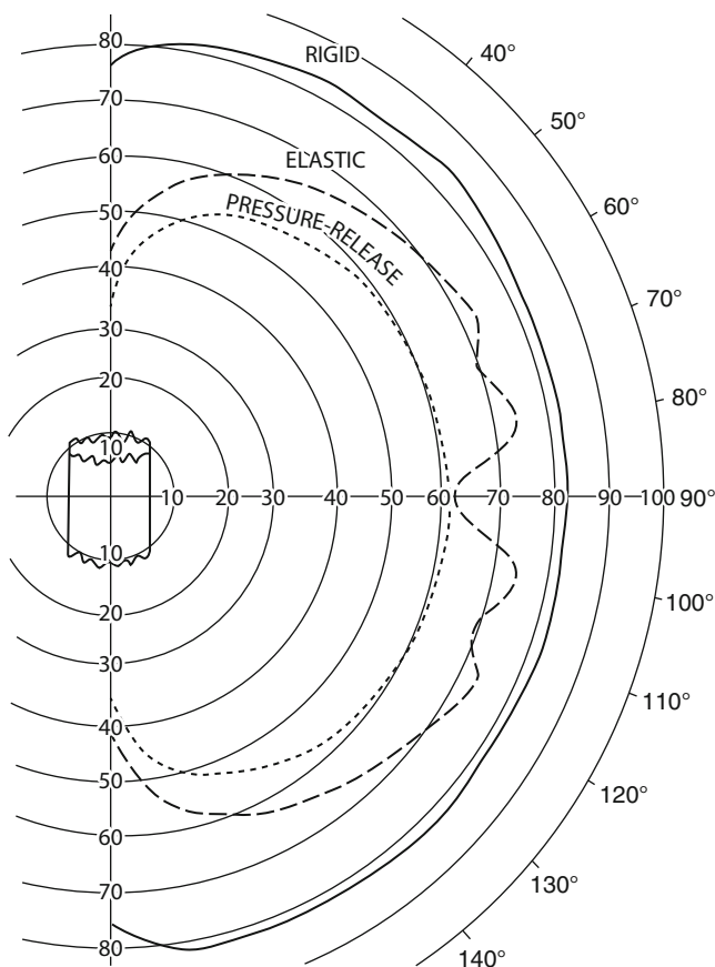
Fig. 11.13 Far-field beam patterns in the vertical plane of the source in Fig. 11.12 at 1800 Hz for rigid (solid line), elastic (dash line), and pressure release (dotted line) cylinders [47]
