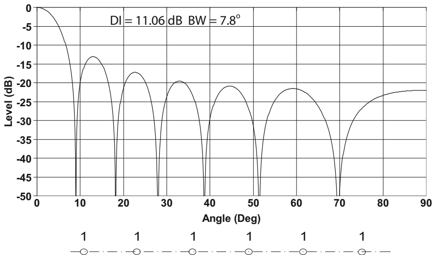
Fig. 8.3 Unshaded 12 element \lambda/2 spaced array
