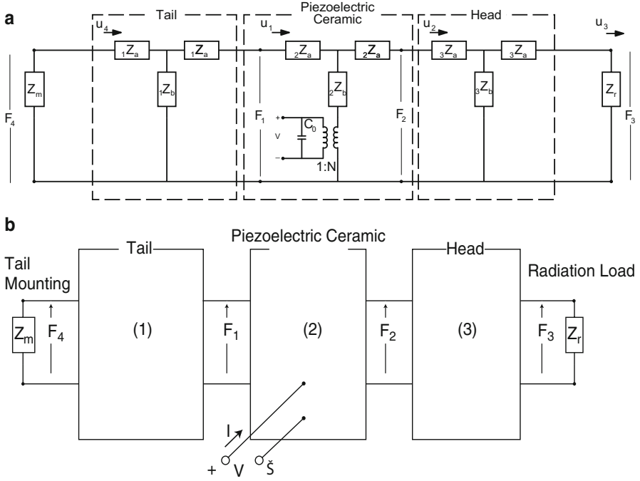
Fig. 3.44 (a) Cascade T network representation of Fig. 3.43. (b) Cascade block matrix representation of Fig. 3.43
