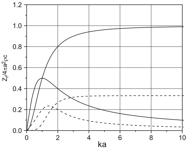
Fig. 10.17 Radiation resistance and reactance for monopole (solid line) and dipole (dashed line) spherical radiators
