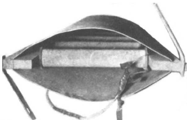
Fig. 1.4 An experimental flextensional transducer built at NRL in May 1929 for in-air operation with magnified shell motion driven by three magnetostrictive tubes [10]
