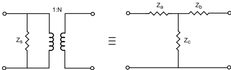
Fig. 13.4 First Norton transformation
