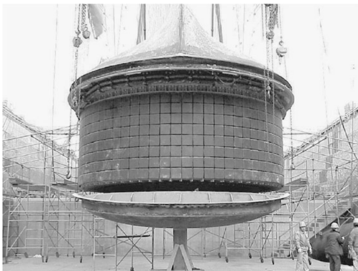
Fig. 1.10 Cylindrical scanning array of Tonpitz transducers
