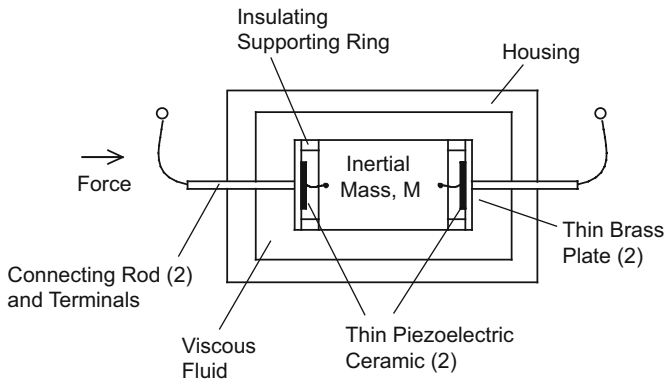
Fig. 6.26 Directional accelerometer based hydrophone with viscous damping for resonance operation [26]
