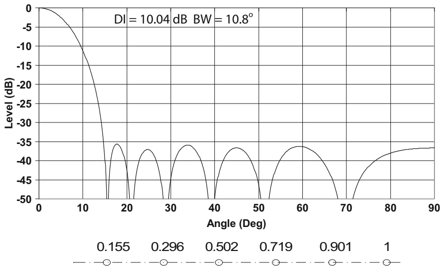
Fig. 8.5 Dolph-Chebyshev shaded 12 element \lambda/2 spaced array, for -37 dB side lobes [10]. Coefficients: 1, 0.901, 0.719, 0.502, 0.296, 0.155
