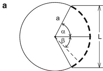
Fig. 7.9 (a) Phasing a cylindrical array of radius a to a plane. L = 2a \sin \alpha is the projected length of the array. A transducer located at angle \beta has the phase ka(1 - \cos \beta) added
