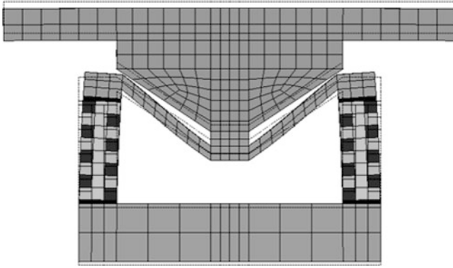
Fig. 5.69 FEA animation of piston for inward bending cantilever
