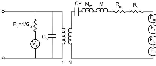
Fig. 13.10 Comprehensive equivalent noise circuit with noise voltage source \langle V_e^2 \rangle and mechanical \langle F_m^2 \rangle , radiation \langle F_r^2 \rangle and sea state \langle F_{ss}^2 \rangle noise forces along with acoustic force signal F_b
