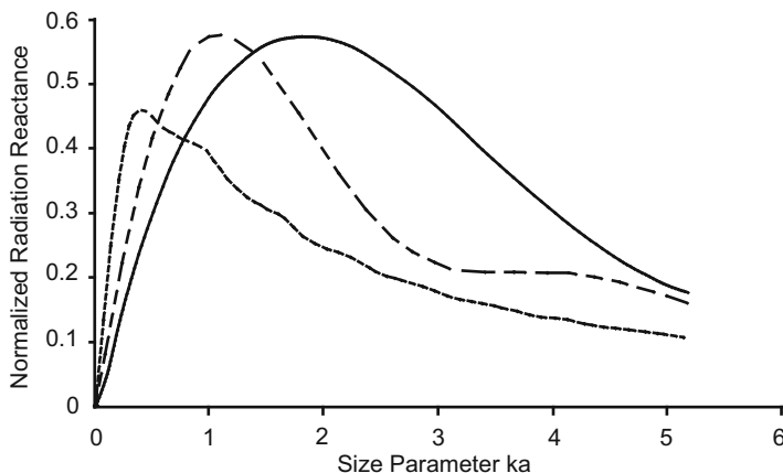
Fig. 11.6 Normalized radiation reactance for uniform motion of the cylinder, mode n=0 , for h/2a=0.5 (solid line), 1.0 (dash line), and 5.0 (dotted line) [25]
