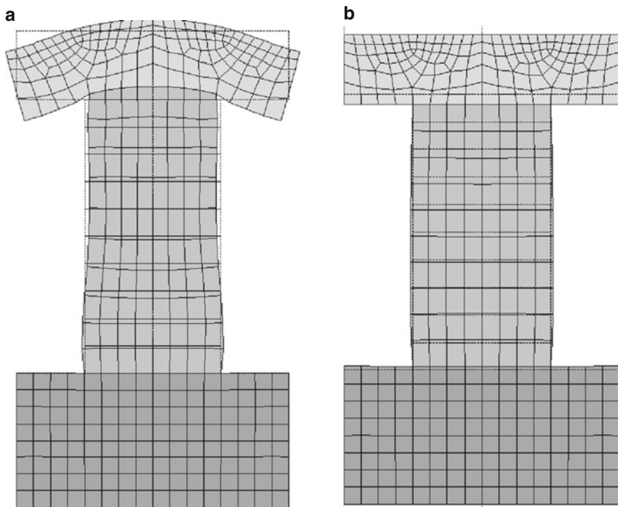
Fig. 3.52 (a) Transducer dynamic motion with flexing head. (b) Transducer dynamic motion with stiffened head
