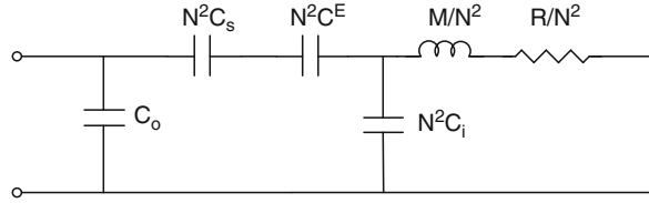
Fig. 4.7 Circuit with both stress rod and glue bond
