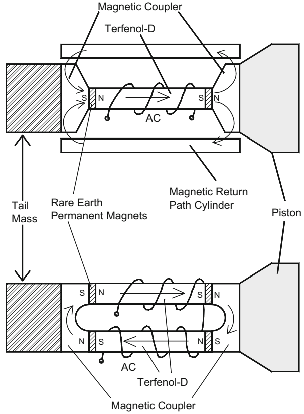
Fig. 5.22 Magnet bias designs for Tonpilz transducer. Arrows indicate magnetic flux directions
