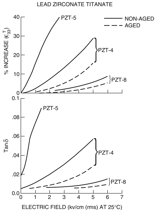
Fig. 13.6 Nonlinear behavior of permittivity and dielectric loss tangent for PZT-4, PZT-5, and PZT-8
