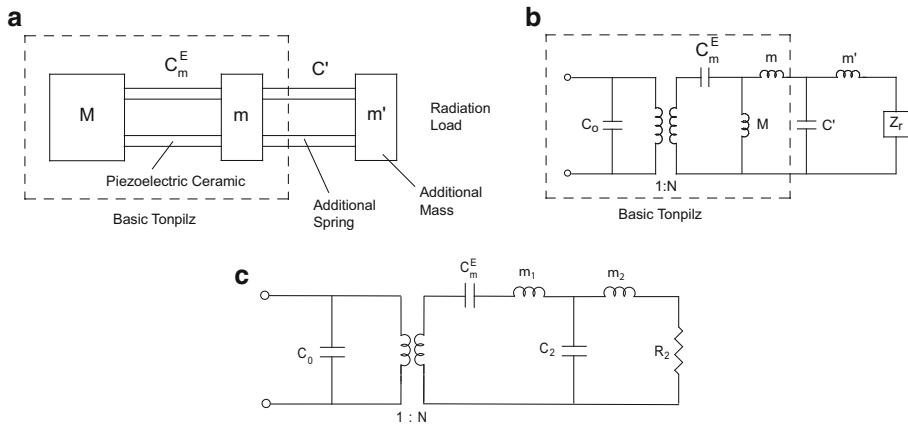
Fig. 5.35 (a) Rodrigo broadband design [45]. (b) Equivalent circuit for Rodrigo design. (c) Approximate circuit representation of Fig. 5.35
