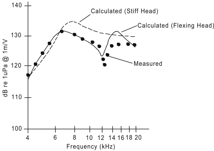
Fig. 5.21 Comparison of the stiff ( dashed line ) and flexing ( solid line ) head calculated responses with the measured ( bulleted line ) constant voltage transmitting response of flexing head Tonpilz transducer [28]
