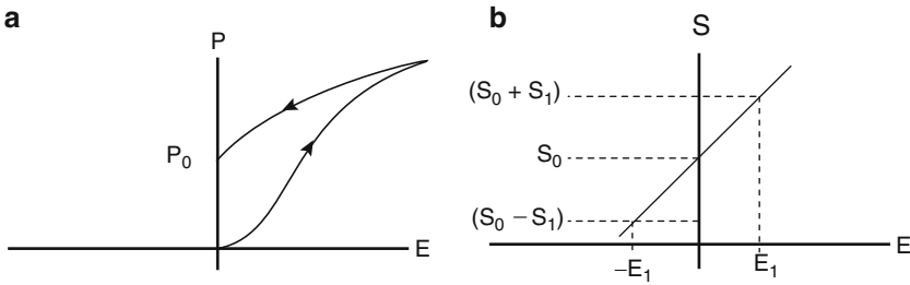
Fig. 2.4 Polarization and strain vs. electric field showing remanent polarization, P_0 (a), and remanent strain, S_0 (b), when the field is removed. Application of the alternating field E_1 then causes alternating strain S_1 about the remanent strain S_0
