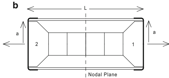
Fig. 5.19 (b) Dual piston transducer
