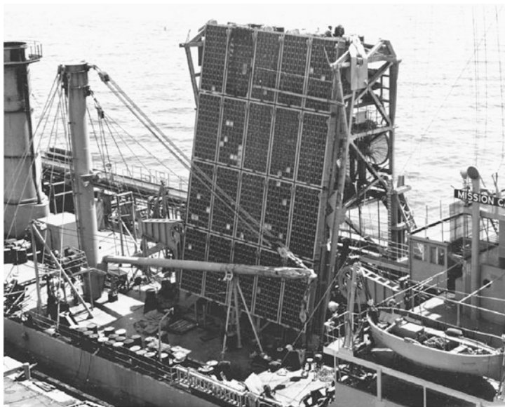
Fig. 1.9 Photograph of large array of very low frequency magnetic variable reluctance dipole “shaker box” transducers ready for deep submergence testing, courtesy of Massa products [30]
