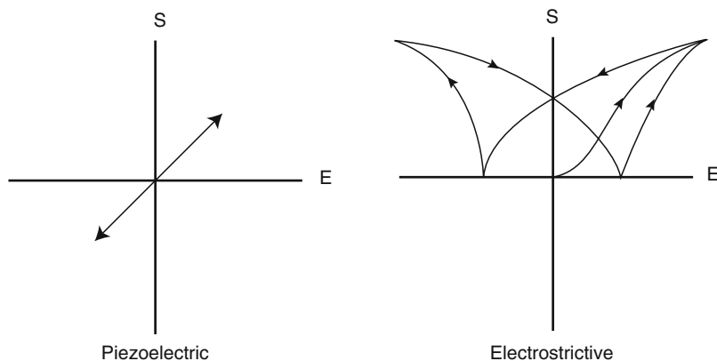
Fig. 2.1 Strain vs. electric field for piezoelectric and electrostrictive materials
