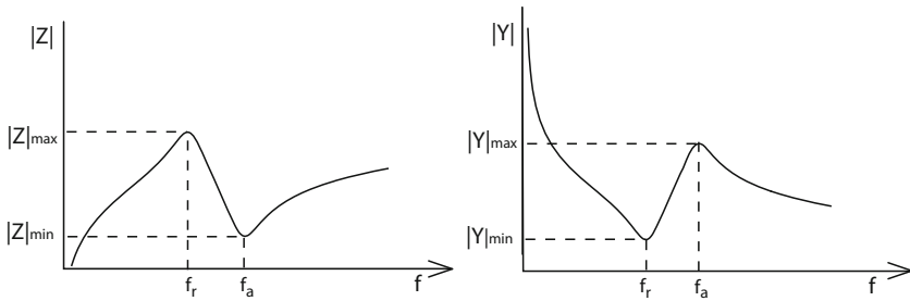
Fig. 9.8 Impedance, Z , and admittance, Y , magnitudes for a magnetic field transducer
