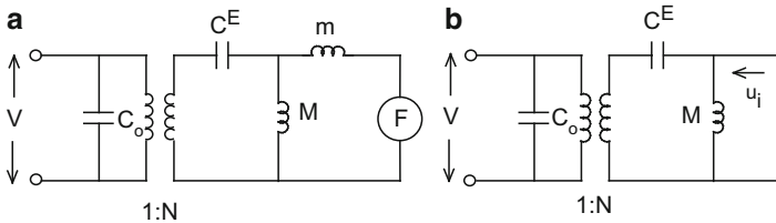
Fig. 6.25 Equivalent circuit of accelerometer for input force (a) and velocity (b)
