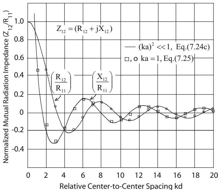
Fig. 7.13 Normalized mutual radiation impedance as a function of relative separation for two rigid circular disks in an infinite rigid plane. Approximate results for small disks and exact results for ka = 1 [23]
