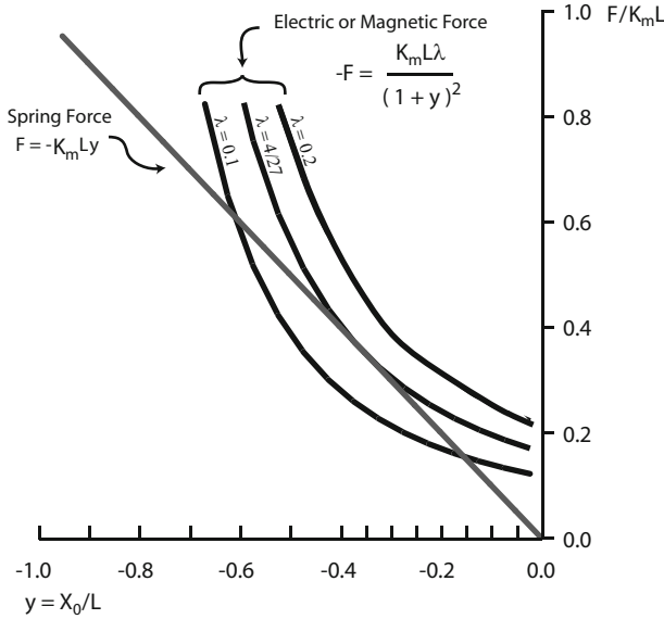
Fig. 12.6 Static equilibrium diagram for electrostatic and variable reluctance transducers. Note the stable equilibrium point at y = -0.16 and the unstable point at y = -0.59 for the case where \lambda = 0.1 . For \lambda = 4/27 there is one equilibrium point at y = -1/3 . For \lambda > 4/27 there are no equilibrium points [21]
