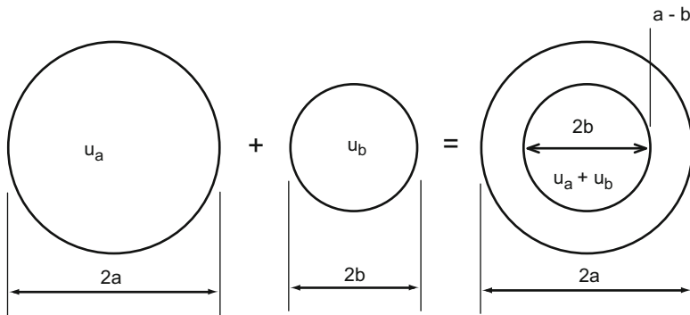
Fig. 10.12 The boundary conditions for two concentric circular pistons combine to give the boundary condition for an annular piston when the velocities are equal and opposite ( u_b = -u_a ). The sound field of the annular piston is the sum of the sound fields of the two pistons
