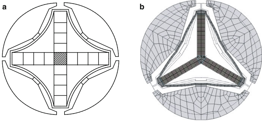
Fig. 5.49 (a) X-spring version of the Astroid flextensional transducer. (b) FEA dynamic in-air motion of the Trioid transducer
