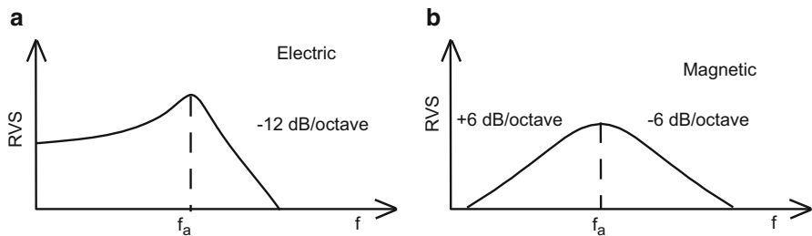
Fig. 9.15 (a) Receiving voltage sensitivity for an electric field transducer. (b) Receiving voltage sensitivity for a magnetic field transducer
