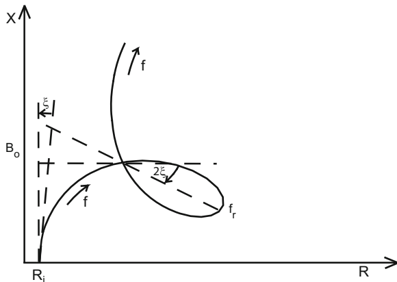
Fig. 9.12 Impedance locus for a magnetic field transducer with eddy current loss angle \xi
