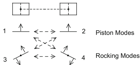
Fig. 7.18 Two transducers each vibrating in a piston mode and a rocking mode. For analysis the two can be considered as four transducers with acoustic interactions between them as shown by the dashed arrows
