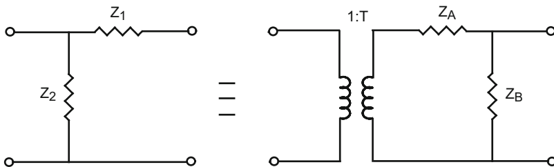
Fig. 13.5 Second Norton transformation
