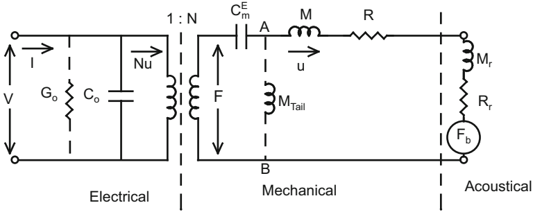
Fig. 2.11 Lumped equivalent circuit. Tail mass inductor between AB is for the case of a finite reaction mass
