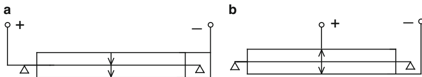
Fig. 5.54 Parallel (a) and series (b) wired bilaminar piezoelectric bars
