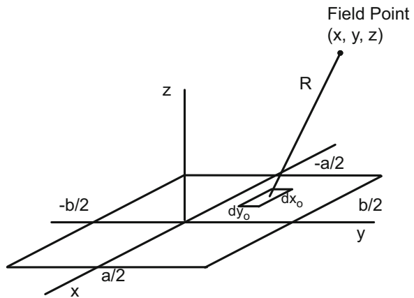
Fig. 10.11 Coordinates for calculating the field of a rectangular piston radiator in an infinite baffle
