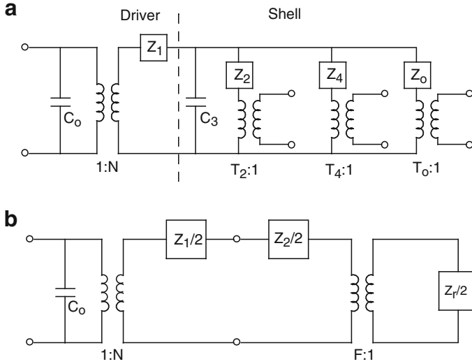
Fig. 5.40 (a) Brigham's flextensional equivalent circuit. (b) Quadrupole mode equivalent circuit
