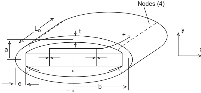
Fig. 5.38 Class IV flextensional transducer [61]
