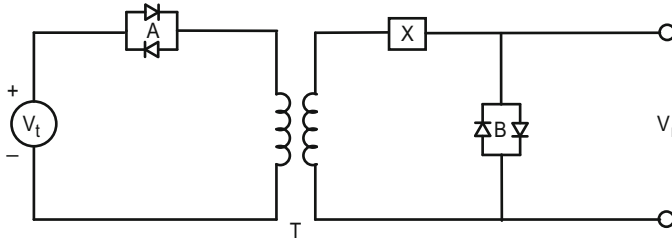
Fig. 9.23 Transmit/receiving, “TR,” circuit with back to back diodes A and B
