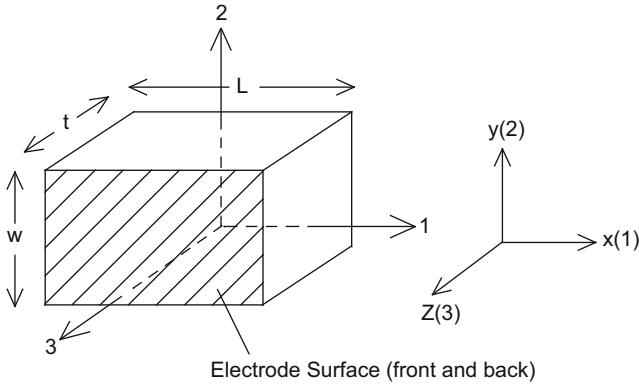
Fig. 6.1 Piezoelectric ceramic with two electrodes perpendicular to the direction of polarization 3 axis
