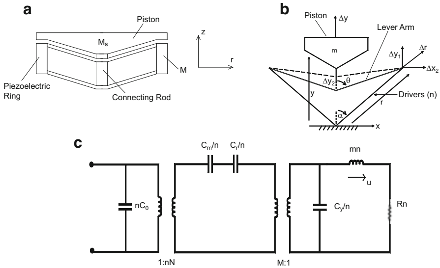
Fig. 5.51 (a) Single piston X-spring transducer. (b) Mechanical model of a symmetry section of an Astroid type Transducer. (c) Equivalent circuit of Astroid ( n = 4 ) type transducers
