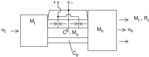
Fig. 5.18 Basic mechanical lumped model
