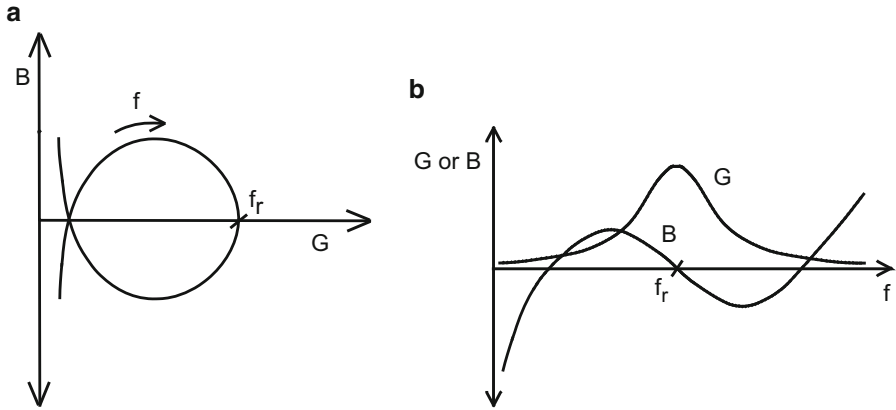
Fig. 9.19 (a) Shunt tuned electric field transducer admittance locus. (b) Shunt tuned electric field transducer conductance, G , and susceptance, B
