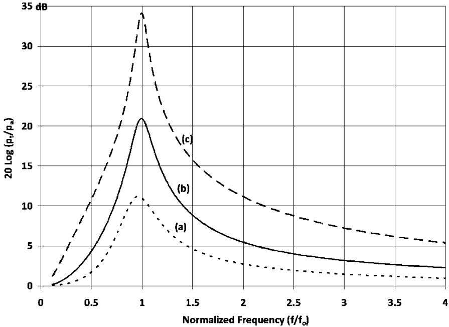
Fig. 10.21 On axis ( \theta=0 ) normalized total pressure level 20\log(p_t/p_a) as a function of ff_o for cases: (a) (dotted line) with k_o d=0.2 , \eta_o=0.1 , and Q_o=2.5 , (b) (solid line) with k_o d=0.1 , \eta_o=0.1 , and Q_o=5.0 , (c) (dashed line) k_o d=0.1 , \eta_o=0.5 , and Q_o=10
