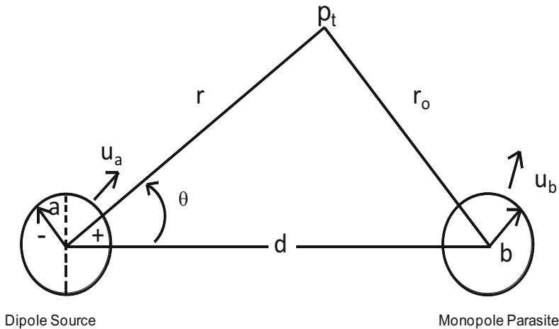
Fig. 10.20 Dipole and monopole spheres of radii a and b and velocities u_a and u_b separated by a center-to-center distance, d , and distances r and r_0 arriving together to form the total pressure p_t(r, \theta) at angle \theta , measured from the axis of symmetry of the dipole
