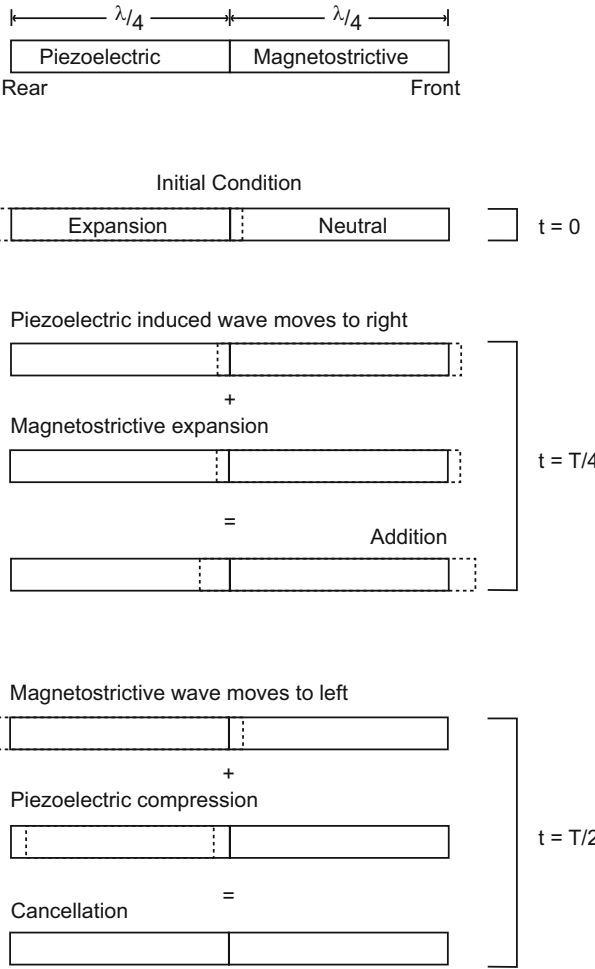
Fig. 5.23 Sequence of events leading to an enhancement at one end and cancellation at the opposite end of the hybrid transducer. Each section is one-quarter-wavelength long. T is the period of one cycle, and \lambda is the wavelength measured in the respective materials [37]
