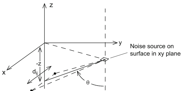
Fig. 8.12 Each small portion of the sea surface in the xy plane is a noise source which radiates into the water with a \cos^2\theta intensity pattern. A pair of hydrophones is shown oriented parallel to the surface at depth z
