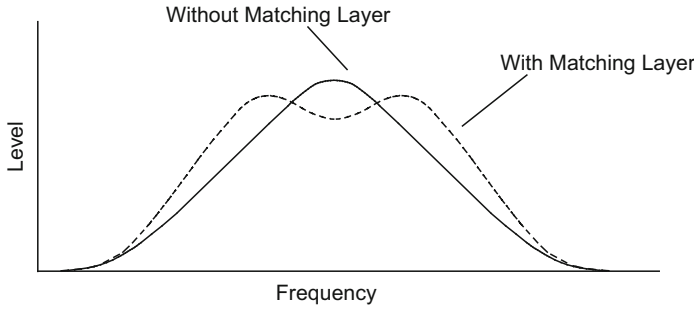
Fig. 5.28 Transmission line transducer response without ( solid line ) and with ( dashed line ) matching layer
