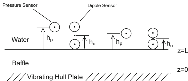
Fig. 8.29 Comparison of pressure sensors and dipole velocity sensors, mounted near a compliant baffle. Both types of sensors have the same standoff distance. Two cases with different standoff distances are shown
