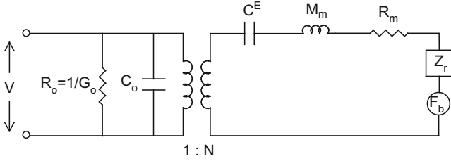
Fig. 6.9 Lumped equivalent circuit of a hydrophone
