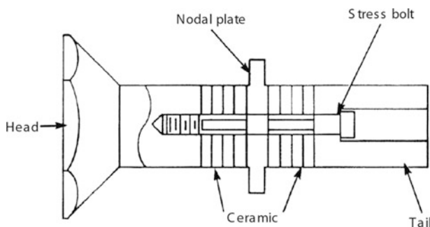
Fig. 1.5 Sketch of a Tonpilz transducer with nodal plate mounting system
