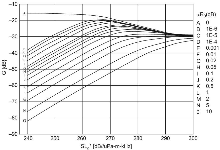
Fig. 7.21 Parametric gain G for scaled primary source level. SL_0^* and down shift ratio of 5 [53]
