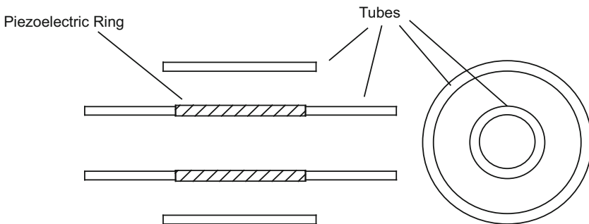
Fig. 5.13 Multiport transducer [19]
