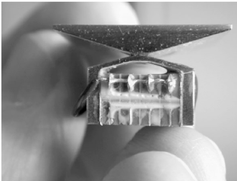
Fig. 1.17 A flexensional amplified single-side one-inch-square piston transducer driven by eight single crystal PMN-PT plates driven into a bending mode. Designed by Image Acoustics and further refined by Northrop Grumman, fabricated by Harris Acoustic Products for Northrop Grumman
