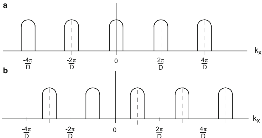
Fig. 8.8 Wave number response of a line array with spacing D between hydrophones. (a) unsteered (b) steered to acoustic end-fire, k_{0x} = \pi/D . The minor lobes between the grating lobes are omitted
