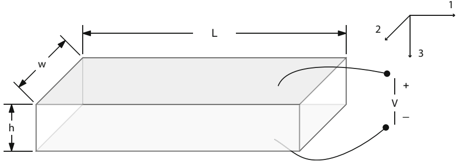
Fig. 3.37 Piezoelectric ceramic side electrode 31 mode bar
