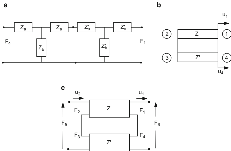
Fig. 3.33 (a) Distributed network representation for the two series bars of Fig. 3.32. (b) Two bars mechanically connected in parallel. (c) Distributed network representation for the two parallel bars of (b)
