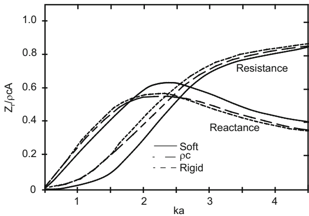
Fig. 11.16 Normalized radiation impedance for the curves of the polar piston on the sphere with the soft, \rho c , and rigid baffle in Fig. 11.15 [54]
