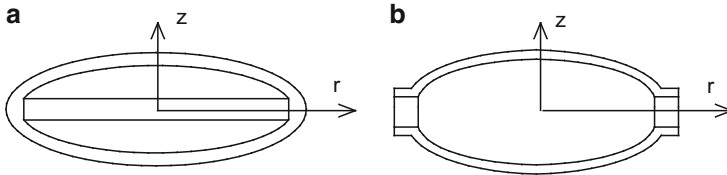
Fig. 5.45 The Class V disc-driven (a) and ring drive (b) flextensional transducer
