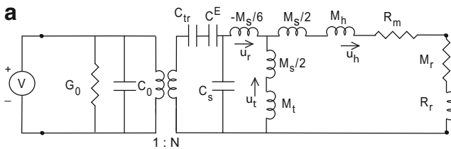
Fig. 5.19 (a) Lumped equivalent circuit for a Tonpilz transducer
