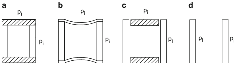
Fig. 6.12 Cylindrical hydrophone with (a) rigid end caps, (b) concave caps, (c) exposed ends, and (d) free-flooding
