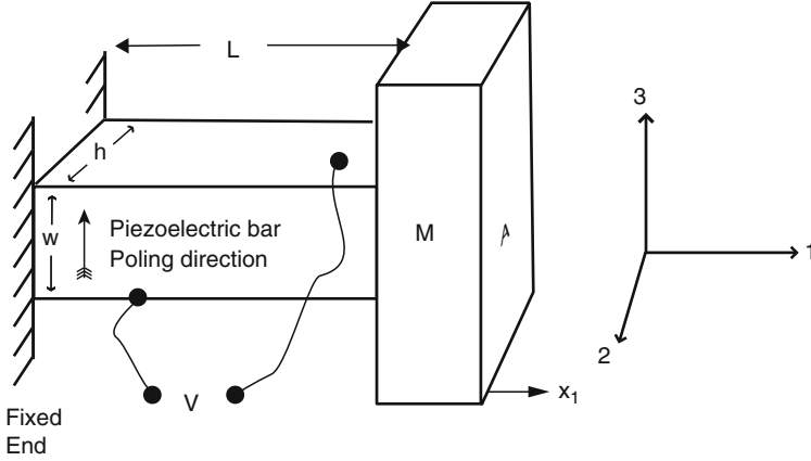
Fig. 2.6 The 31 mode piezoelectric longitudinal vibrator with working strain perpendicular to poling direction and electrodes on the side of the bar
