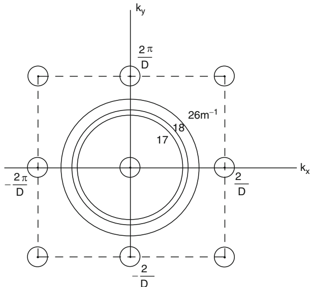
Fig. 8.18 Wavevector response of an unsteered square array with spacing D showing main lobe and first grating lobes. The three circles with radii 17, 18, and 26 \text{ m}^{-1} represent the acoustic wave numbers and free plate wave numbers for 2 in. and 1 in. thick steel plates at 4 kHz
