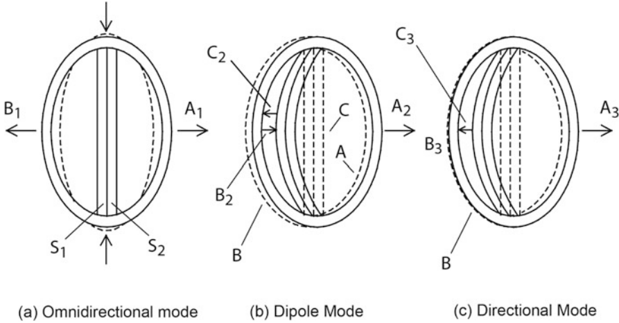
Fig. 5.41 Schematic illustration of a flextensional transducer showing the sequence of events leading to directionality. The neutral state is represented by the dashed lines
