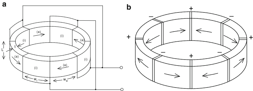
Fig. 5.5 (a) Parallel wired segmented ring with inactive segments (i) interlaced with active piezoelectric segments. The arrows show the direction of remnant polarization [4]. (b) Striped 33-mode piezoelectric ceramic cylinder
