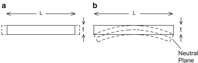
Fig. 5.52 Extensional (a) and inextensional (b) modes of vibration
