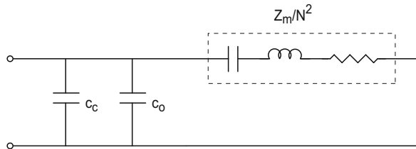
Fig. 4.4 Circuit with cable and/or stray capacitance, c_c
