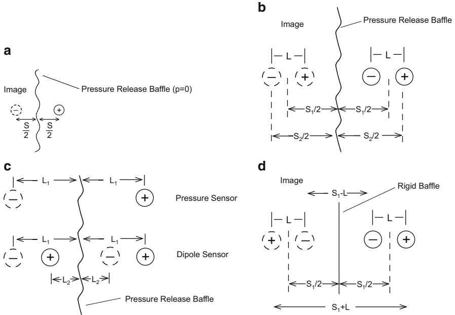
Fig. 6.21 (a) Hydrophone in front of a large planar soft baffle. (b) Dipole sensor near a large planar soft baffle. (c) Comparison of a pressure sensor and a dipole with same stand-off from a soft baffle. (d) Dipole sensor with separation L at a distance S_1/2 in front of a large planar rigid baffle
