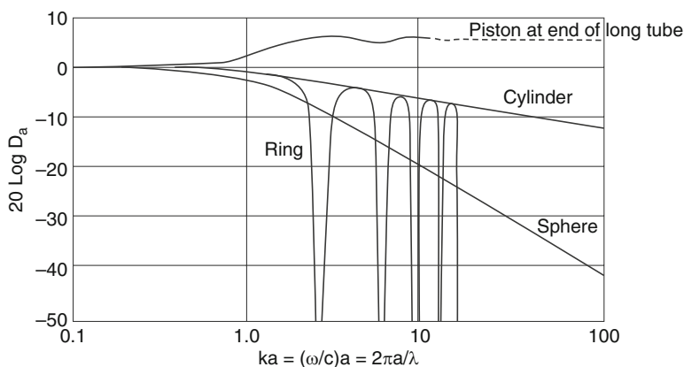
Fig. 6.36 Diffraction constant D_a for a piston, sphere, cylinder, and ring [49]. Note: The cylinder and ring curves should decrease as 20 \log D_a and not 10 \log D_a , as shown. See Z. Milosic [51]. Thus, the dB values for the ring and cylinder curves should be multiplied by 2
