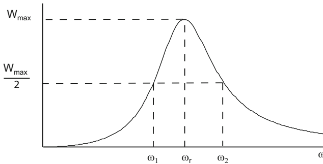
Fig. 4.3 Power vs. frequency showing half power frequencies
