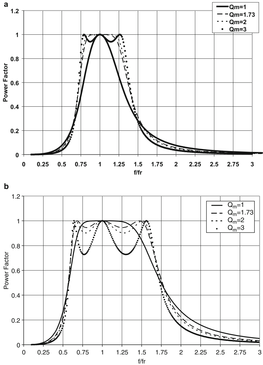
Fig. 2.12 (a) Power factor as a function of frequency, related to resonance, for k=0.5 and Q_m=1, 1.73, 2 , and 3 . (b) Power factor as a function of frequency, relative to resonance, for k=0.7 and Q_m=1, 1.73, 2 , and 3 . (c) Power factor as a function of frequency, relative to resonance, for k=0.9 and Q_m=0.5, 0.7, 1 , and 2
