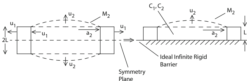
Fig. 5.8 Free-flooded ring with half plane symmetry
