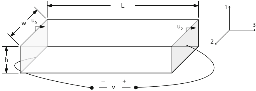
Fig. 3.38 Piezoelectric ceramic end electrode 33 mode bar
