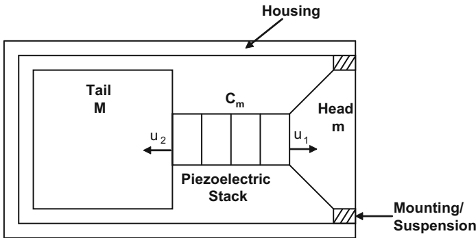
Fig. 2.13 Sketch of a Tonpilz transducer with head and tail velocities, u_1 and u_2 , respectively
