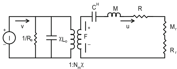
Fig. 3.21 Dual equivalent circuit representation of Fig. 3.20
