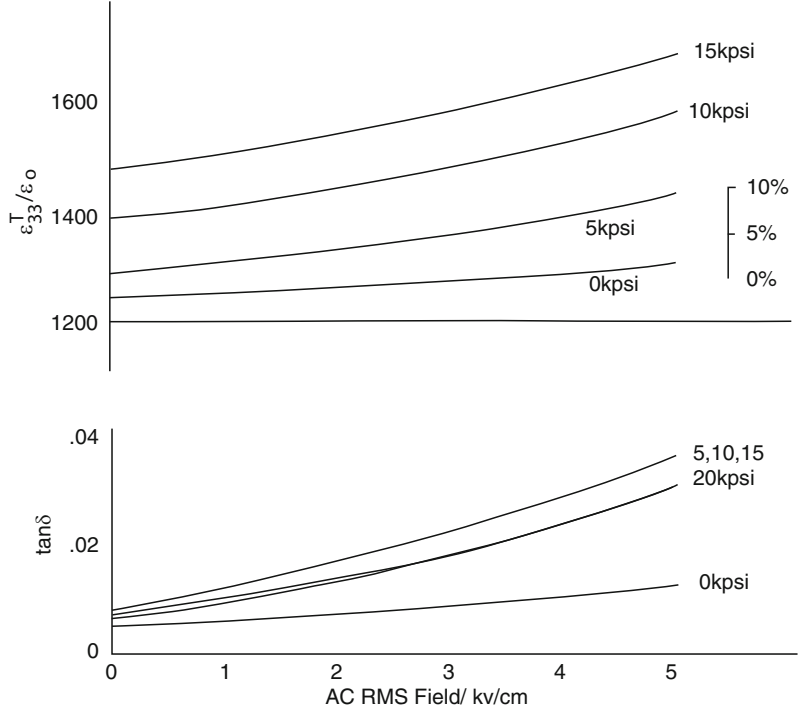
Fig. 13.8 \epsilon_{33}^T/\epsilon_0 and \tan \delta vs. AC field. At various levels of parallel stress ( T_3 ) PZT-8
