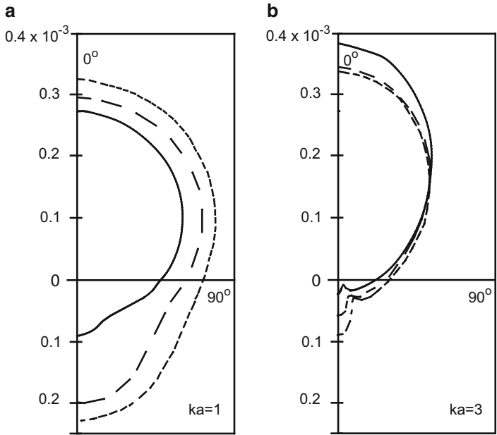
Fig. 11.15 Far-field polar pattern, at kr = 1000 , of the pressure amplitude relative to \rho c for a sphere of radius a vibrating uniformly over the portion from 0^\circ to 60^\circ with a soft, \rho c or rigid baffle from 60^\circ to 180^\circ [54]. (a) ka is equal to unity and (b) ka = 3 . solid line soft; dash line \rho c ; dotted line rigid
