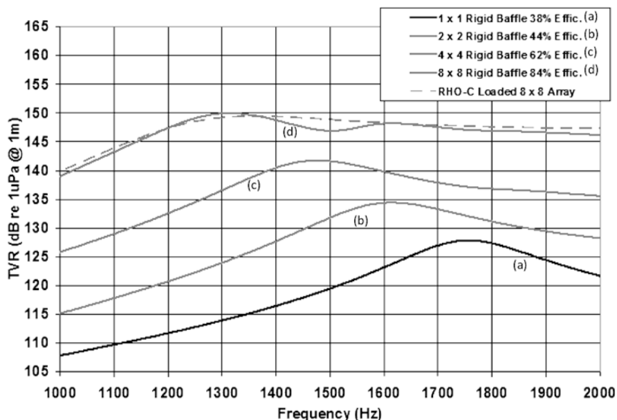
Fig. 5.72 FEA calculated TVR array results for various array configurations of the cantilever mode transducer
