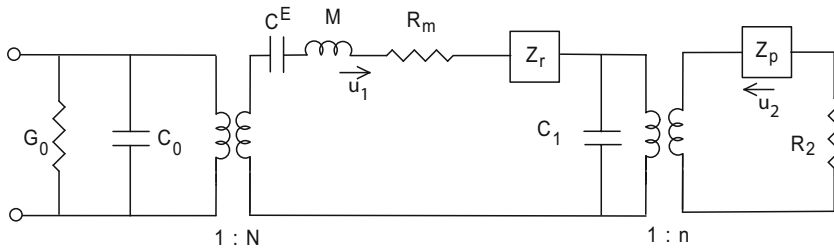
Fig. 5.11 Free-flooded ring equivalent circuit with ring and port radiation impedances Z_r and Z_p
