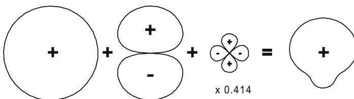
Fig. 5.16 Synthesis of 90° beam [23]
