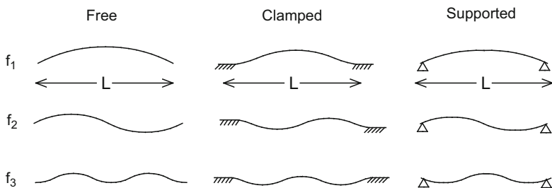
Fig. 5.53 Free, clamped, and simply supported flexural modes of vibration
