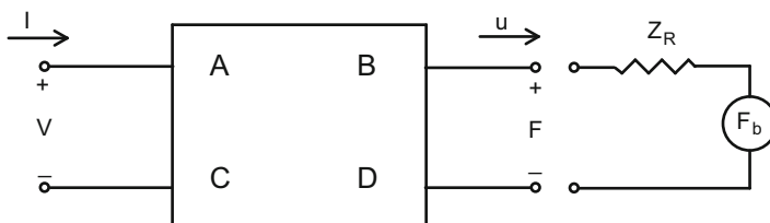
Fig. 9.16 ABCD electromechanical representation
