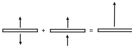
Fig. 10.16 Adding the field of the piston vibrating equally on both sides to the field of the oscillating piston gives the field of the piston vibrating on one side
