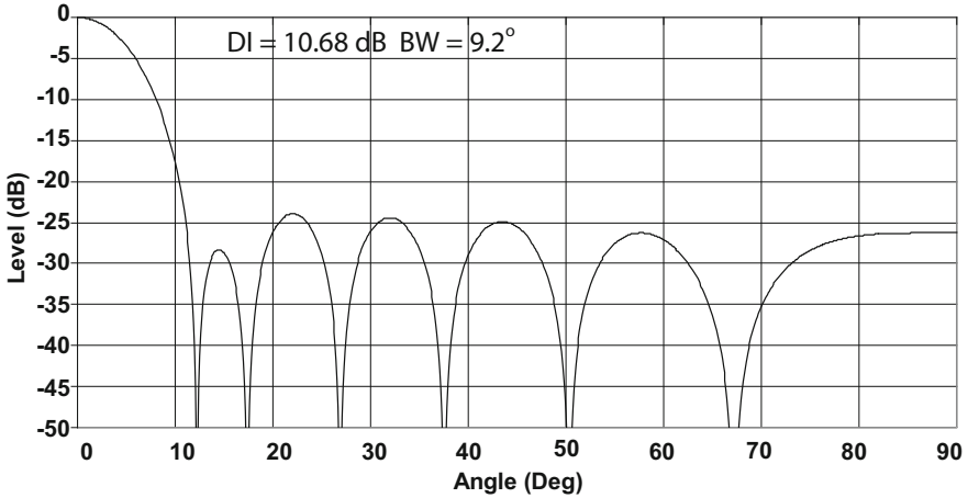
Fig. 8.7 12 element \lambda/2 spaced Taylor shading for 25 dB side lobes. Coefficients: 1, 0.91, 0.77, 0.58, 0.44, 0.40
