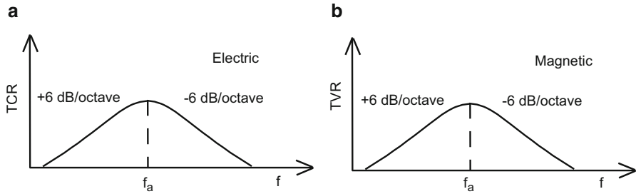
Fig. 9.14 (a) Transmitting current response for an electric field transducer. (b) Transmitting voltage response for a magnetic field transducer
