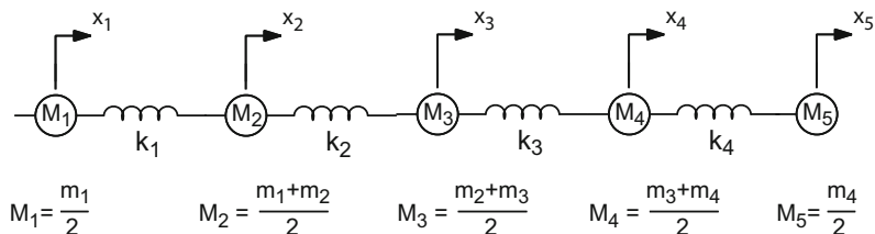
Fig. 3.48 Mechanical lumped mode model of the bar of Fig. 3.47
