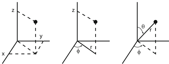
Fig. 10.1 Rectangular (x, y, z) , cylindrical (r, \phi, z) , and spherical (r, \theta, \phi) coordinate systems
