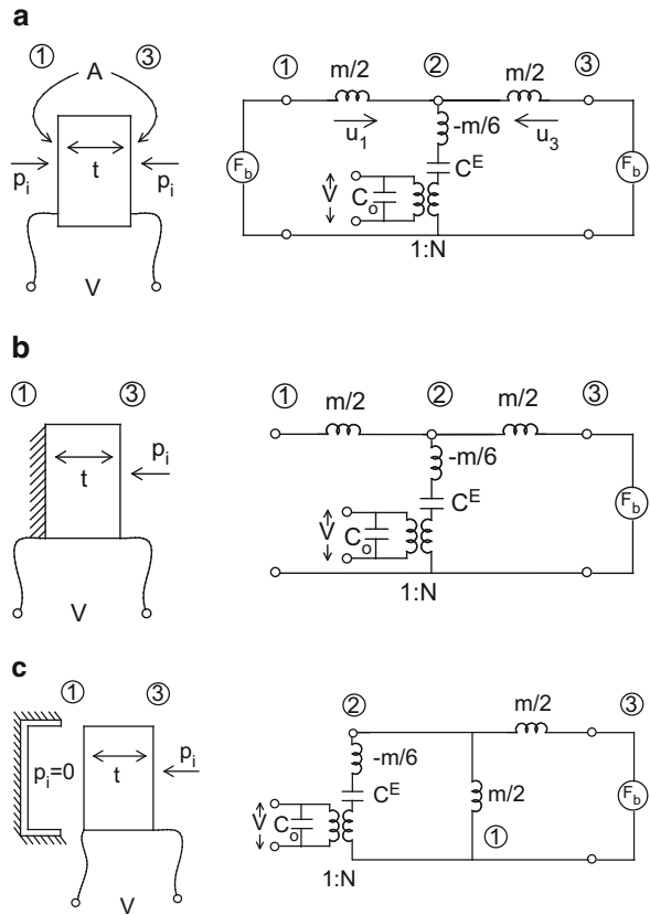
Fig. 6.5 (a) Equal pressure hydrophone. (b) Single pressure but blocked on side 1. (c) Single pressure but free on side 1
