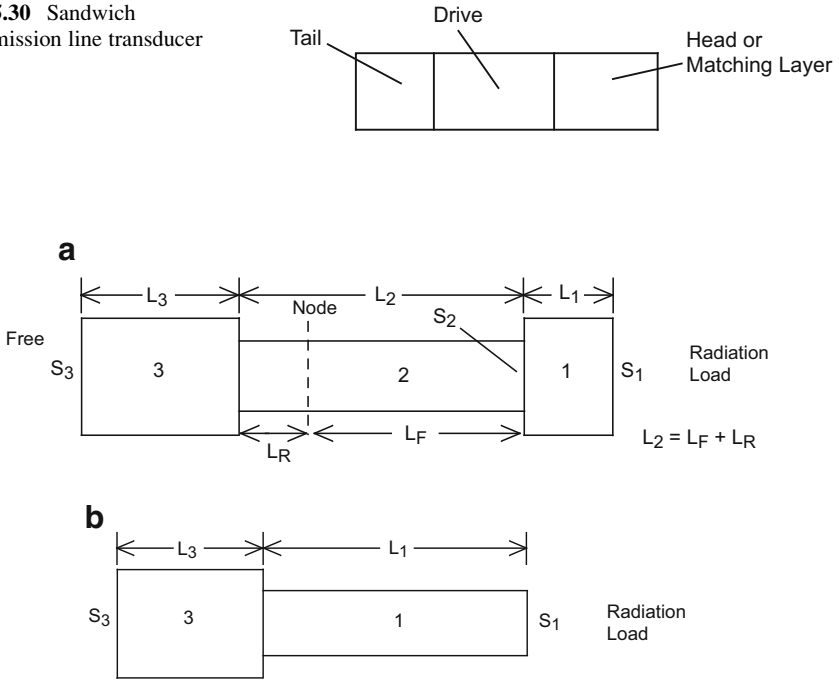
Fig. 5.31 (a) Three part transmission line transducer. (b) Two part transmission line transducer
