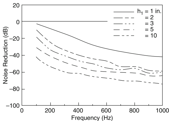
Fig. 8.20 Effect of rubber outer decoupler thickness ( h_1 ) on reduction of TBL noise for point hydrophone [46], with permission from the Acoustical Society of America
