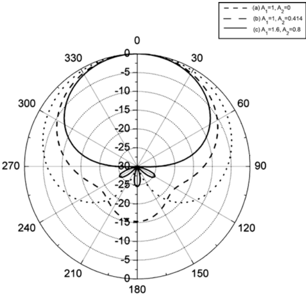
Fig. 5.63 Three modal projector beam patterns with weighting factors: (a) A_1 = 1, A_2 = 0 (b) A_1 = 1, A_2 = 0.414 ; and (c) A_1 = 1.6, A_2 = 0.8
