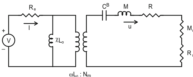
Fig. 3.23 Impedance circuit representation of Fig. 3.19
