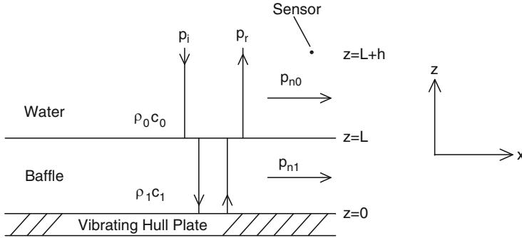
Fig. 8.28 A vibrating plate produces evanescent flexural noise waves traveling parallel to the plate in the baffle and in the water. An acoustic signal arrives at normal incidence and is reflected. An acoustic sensor is located at z = L + h
