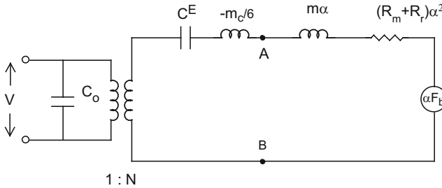
Fig. 6.15 Equivalent circuit of Fig. 6.14 for (R_r + R_m) \ll \omega M_t and \alpha = M_t / (m + M_t)
