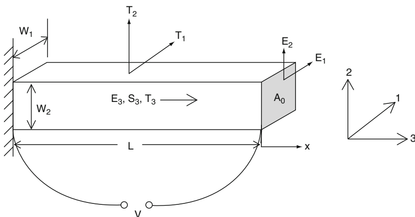
Fig. 3.13 End electroded piezoelectric ceramic bar rigidly mounted on one end
