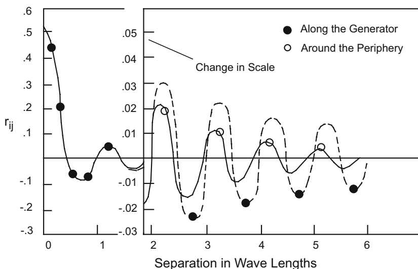
Fig. 7.15 Illustration of dependence of mutual radiation resistance on curvature of the baffle. The dashed curve is for pistons in a plane, the solid dots for square pistons with the same angular position on a cylinder. The solid curve is for circular pistons with the same axial position on a cylinder. The cylinder radius is 6 wavelengths, r_{ij} = R_{ij}/\rho c A [34]
