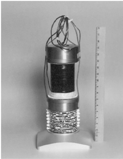
Fig. 1.16 A high power magnetostrictive/piezoelectric hybrid transducer with square piston, piezoelectric ceramic drive, centermass, magnetostrictive drive, and tail mass along with water-tight housing and electrical connector [34]
