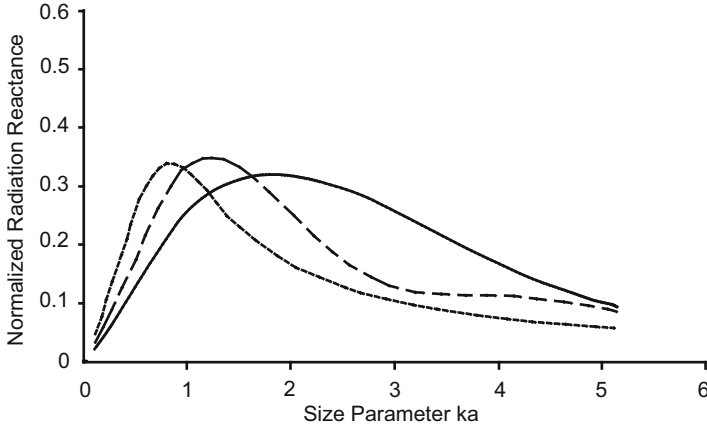
Fig. 11.8 Normalized radiation reactance for dipole motion of the cylinder, mode n=1 , for h/2a=0.5 (solid line), 1.0 (dash line), and 5.0 (dotted line) [25]
