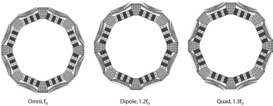
Fig. 5.67 Monopole (omni), dipole, and quadrupole modes of vibration
