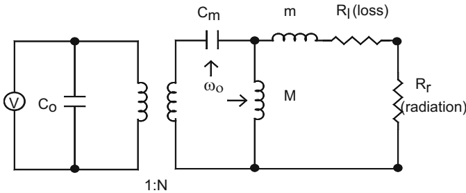
Fig. 5.70 Equivalent circuit representation of a cantilever mode transducer
