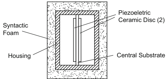
Fig. 6.27 Directional accelerometer based hydrophone with trilaminar bender and syntactic foam buoyancy
