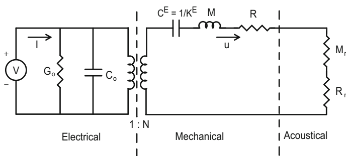
Fig. 3.15 Electrical equivalent circuit of the single degree of freedom piezoelectric vibrator shown in Fig. 3.14
