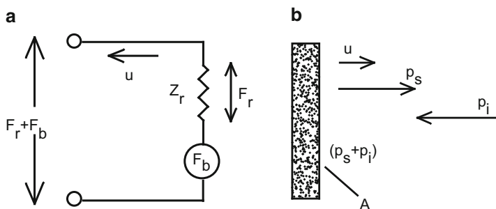
Fig. 6.35 (a) Clamped (blocked) force F_b and radiation force F_r . (b) Incident pressure, p_i , and scattered pressure, p_s
