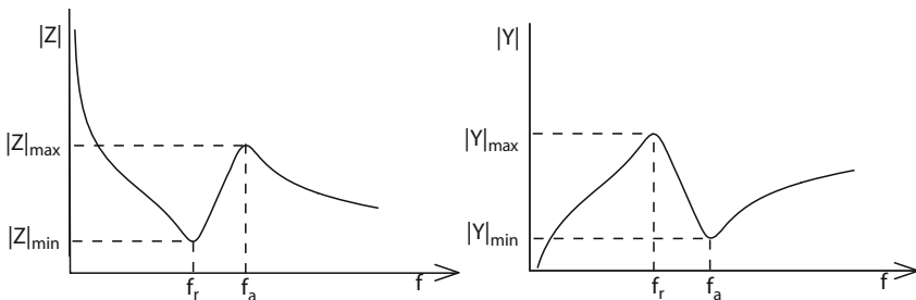
Fig. 9.2 Impedance, Z , and admittance, Y , magnitudes for an electric field transducer
