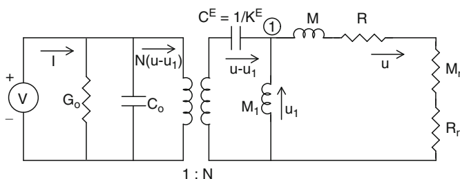
Fig. 3.18 Electrical equivalent circuit of the two-degree of freedom piezoelectric vibrator shown in Fig. 3.17
