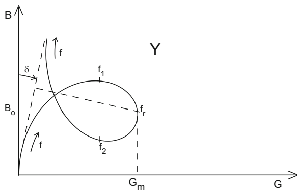
Fig. 9.5 Conductance, G , and susceptance, B , for an electric field transducer
