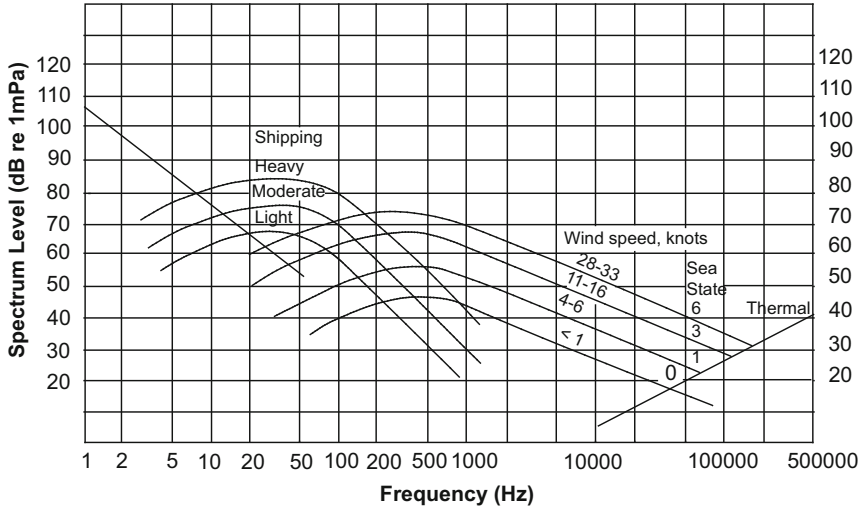
Fig. 8.10 Average deep-water ambient-noise spectra. From [14] (Fig. 7.5) with permission from Peninsula Publishing, Westport, CT 06880. Note: mPa is microPa in this figure
