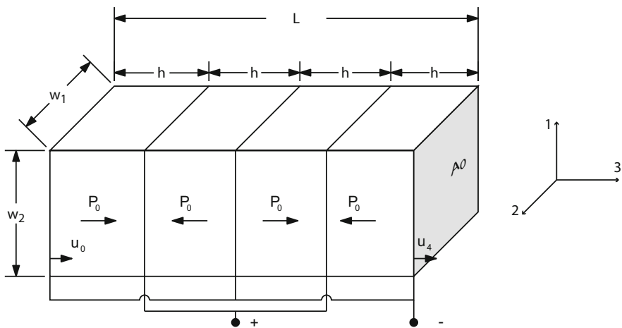
Fig. 3.34 Four piezoelectric bars stacked mechanically in series and wired in parallel
