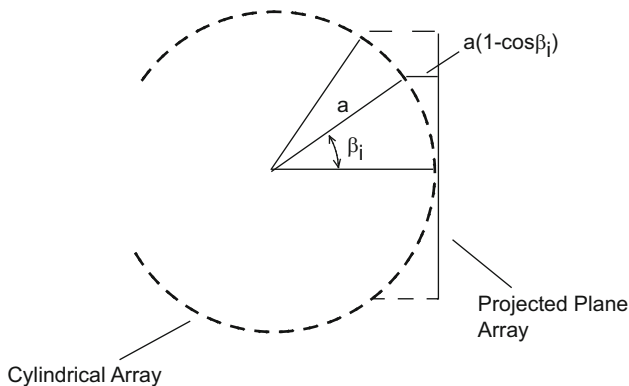
Fig. 8.2 Top view of cylindrical array with 13 staves being phased to a plane to form a beam
