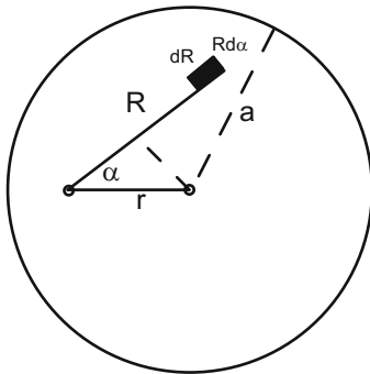
Fig. 10.18 Coordinates for calculating the pressure at an arbitrary point on the surface of a circular piston. The integration over R goes from 0 to r \cos \alpha + (a^2 - r^2 \sin^2 \alpha)^{1/2} , the integration over \alpha goes from 0 to 2\pi
