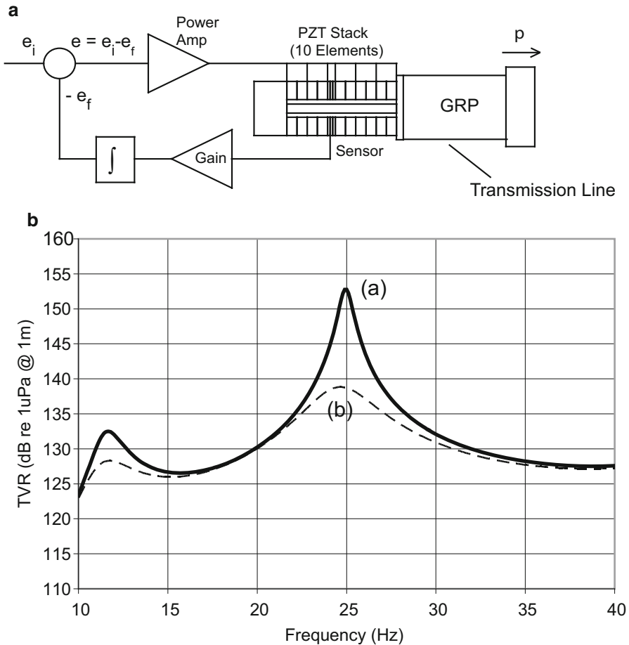
Fig. 5.34 (a) Multiply resonant transducer with feedback. (b) Calculated transmitting voltage response without (a) and with (b) feedback [44]
