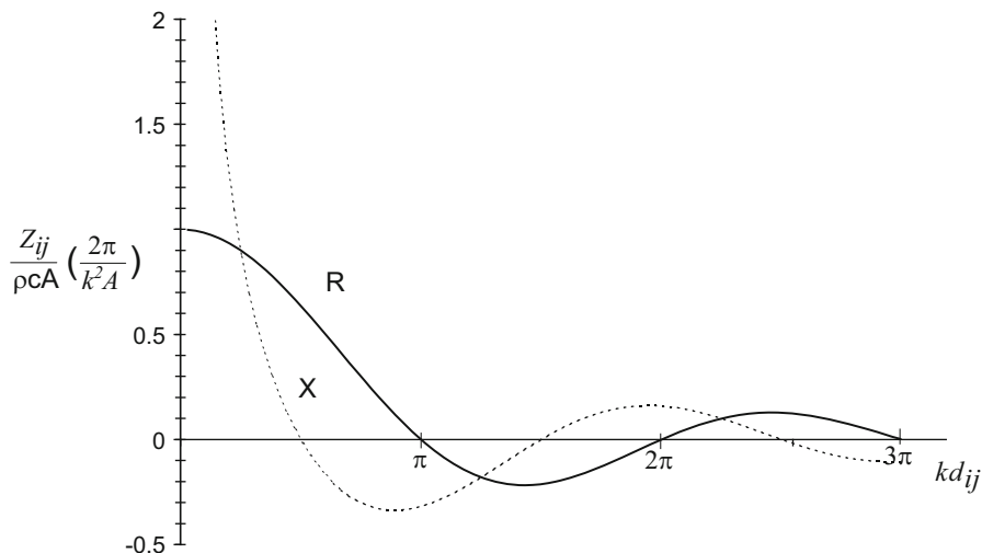
Fig. 7.12 Mutual radiation resistance and reactance for two small piston transducers of area, A , in a plane from Eq. (7.24b)
