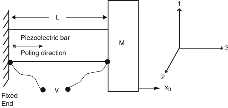
Fig. 2.5 The 33 mode piezoelectric longitudinal vibrator with working strain parallel to poling direction and electrodes on the ends of the bar
