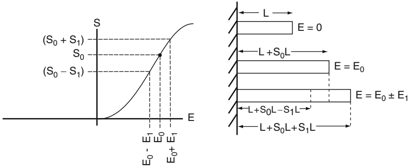
Fig. 2.3 Electrostrictive material with maintained static bias field E_0 and static strain S_0 . An alternating field E_1 follows a minor hysteresis loop and causes an alternating strain S_1 . If E_1 \ll E_0 the variations are approximately linear
