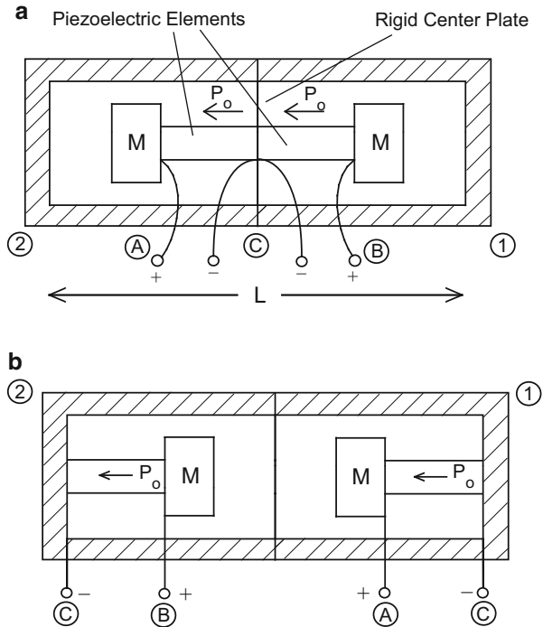
Fig. 6.23 (a) Central accelerometers for net force detection. (b) End mounted accelerometers
