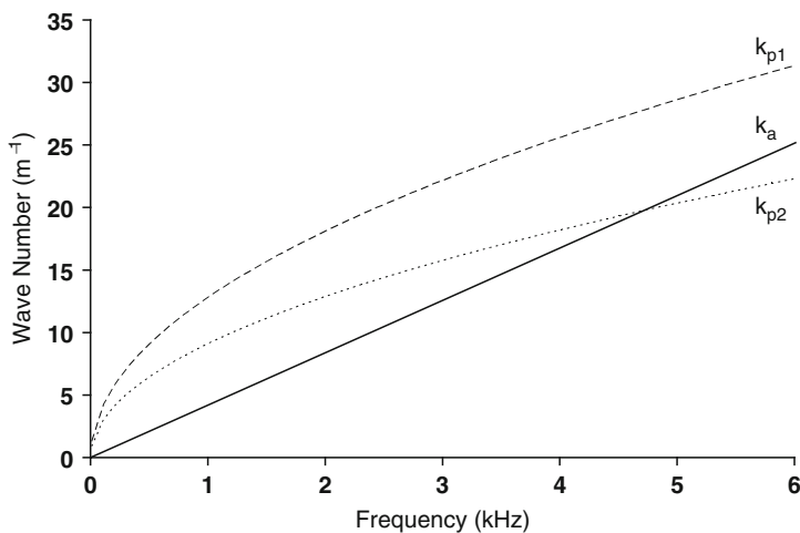
Fig. 8.19 Frequency dependence of wave numbers: k_a for acoustic, k_{p1} for 1 in. thick steel plate, k_{p2} for 2 in. thick steel plate
