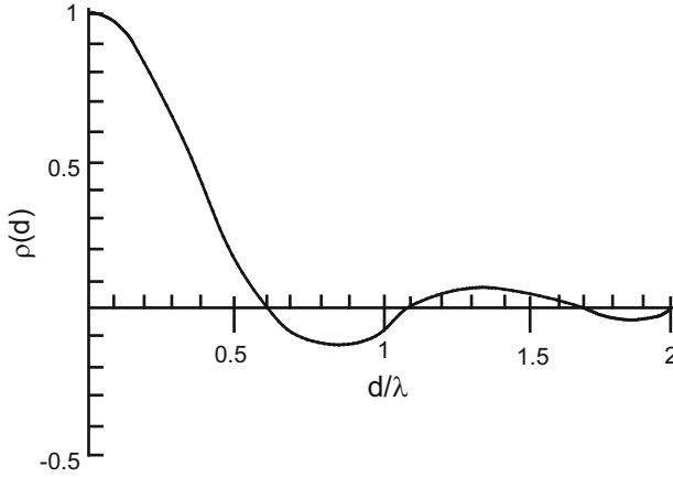
Fig. 8.13 Spatial correlation for surface noise with \cos^2\theta directionality and with the hydrophones oriented parallel to the surface [30]
