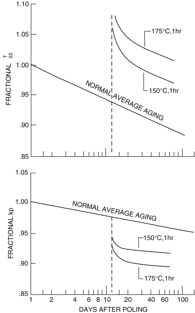
Fig. 13.9 Typical aging of permittivity and planar coupling coefficient of piezoelectric ceramic showing the effects of heat treatments applied 12 days after polarizing
