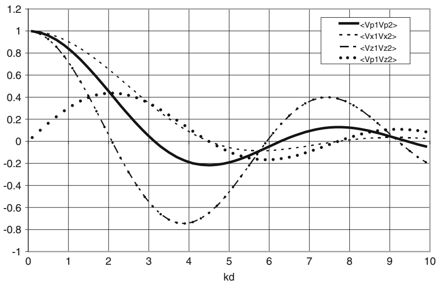
Fig. 8.26 Normalized spatial correlation functions between acoustic pressure and particle velocity components
