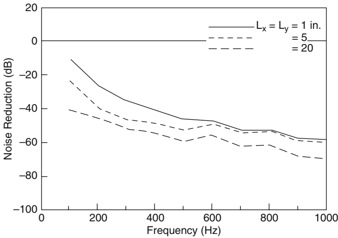
Fig. 8.22 Effect of dimensions of a hydrophone embedded in an elastomer layer 2 in. thick [46], with permission from the Acoustical Society of America
