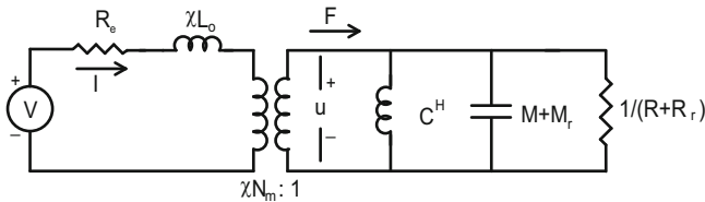
Fig. 3.20 Mobility equivalent circuit of Fig. 3.19
