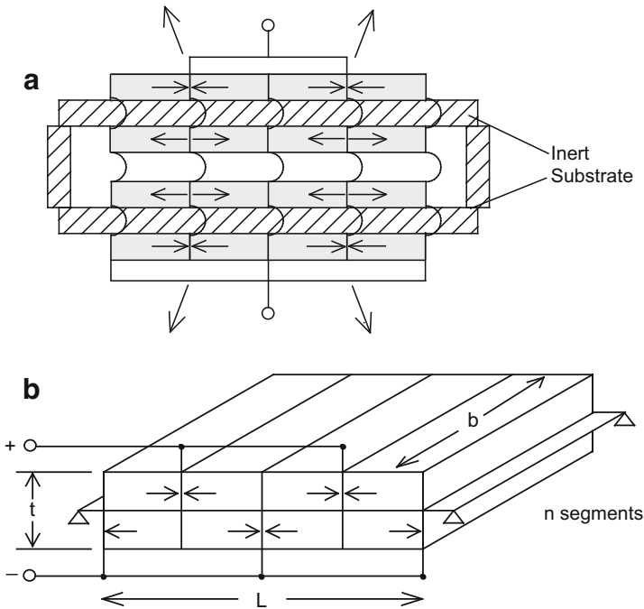
Fig. 5.56 (a) A dual trilaminar bender 33-mode piezoelectric bar transducer. (b) The 33-mode bender with length L , thickness t , width b , and n segments. Arrows show direction of polarization
