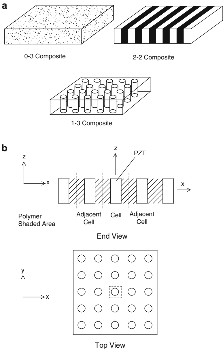
Fig. 5.37 (a) Three piezocomposite configurations in current use for transducers. (b) Model for 1-3 composite
