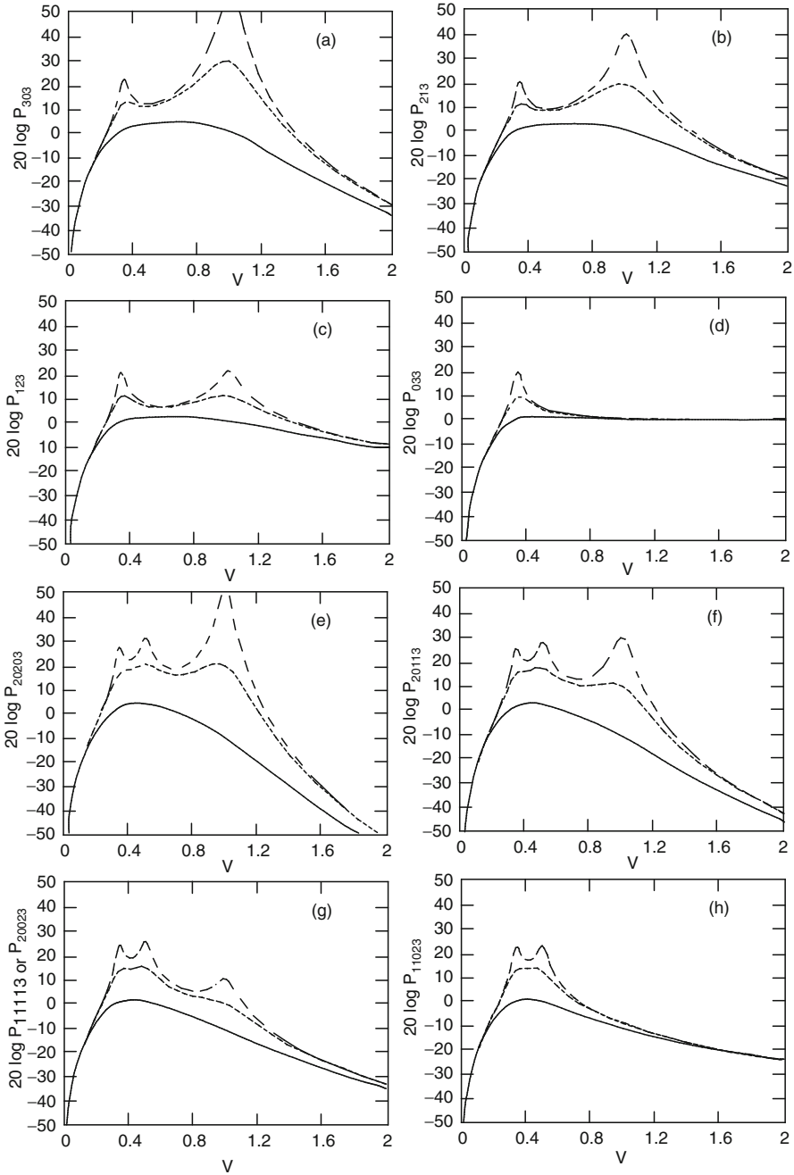
Fig. 12.5 Normalized pressure P (in dB) as a function of the dimensionless frequency \nu for the third harmonics caused by (a) X^3 , (b) X^2 \cos \omega t , (c) X \cos 2\omega t , (d) \cos 3\omega t (e) X^2 , (f) X^2 and X \cos \omega t , (g) X \cos \omega t or X^2 and \cos 2\omega t , (h) X \cos \omega t and \cos 2\omega t for Q_m = 1 (solid line), 3 (dotted line), and 10 (dash line) [3]
