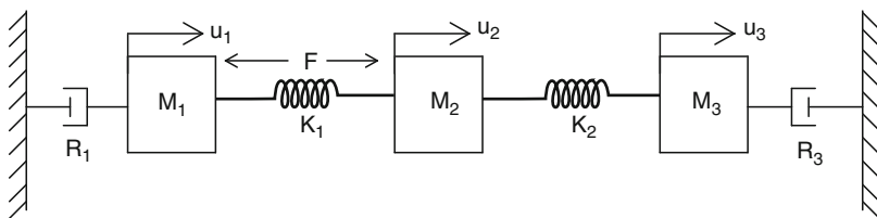
Fig. 3.11 Three degree of freedom mechanical vibrator
