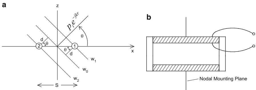
Fig. 6.20 (a) Two omni scalar sensors, 1 and 2, receiving plane wave fronts w_1 and w_2 . (b) End-capped 31 mode cylinder pressure sensor mounted at nodal plane
