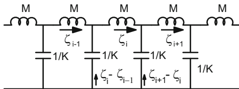
Fig. 3.26 Lumped mode representation of the bar of Fig. 3.25
