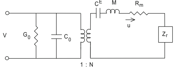
Fig. 5.4 Equivalent circuit for piezoelectric ring
