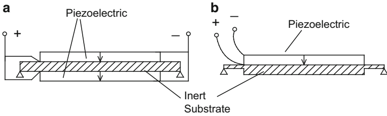
Fig. 5.55 Bilaminar and trilaminar benders
