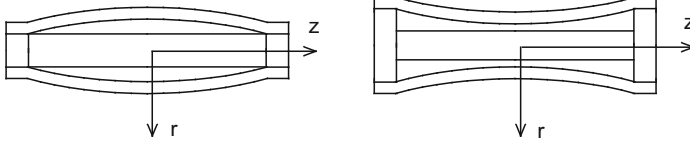
Fig. 5.44 The Class I convex and concave barrel stave flextensional transducer
