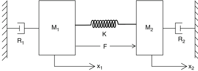
Fig. 3.6 Dual mass two-degree of freedom vibrator
