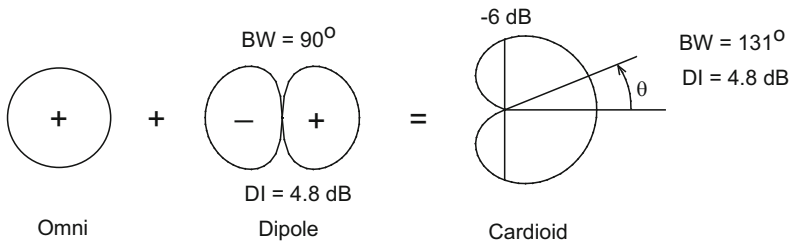
Fig. 6.30 Synthesis of a cardioid pattern
