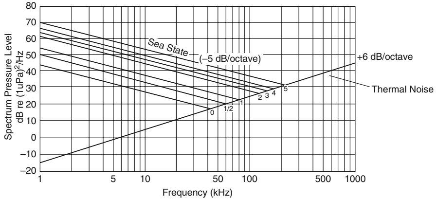
Fig. 6.37 Sea state and thermal noise [54]
