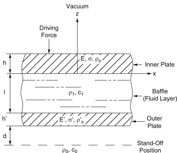
Fig. 8.16 Geometry of the model used for flexural wave baffling [43], with permission from the Acoustical Society of America. ( E is Young's modulus, \sigma is Poisson's ratio, and \rho is the density)
