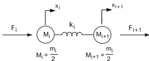
Fig. 3.48 Mechanical lumped mode model of the bar of Fig. 3.47
