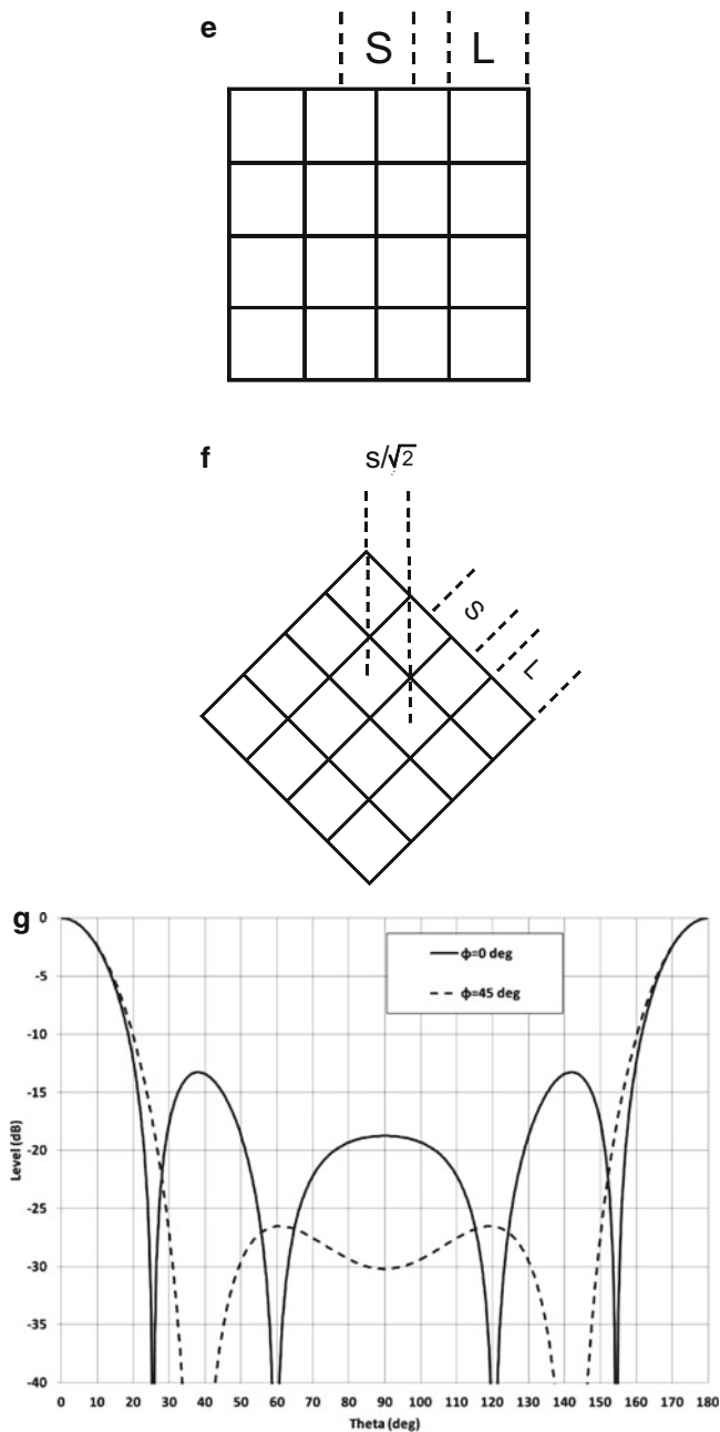
Fig. 7.9 (e) Square array with center-to-center separation S . (f) Diamond array with center-to-center separation S/\sqrt{2} . (g) Normalized patterns for \phi = 0^\circ (solid line) and (dashed line) \phi = 45^\circ
