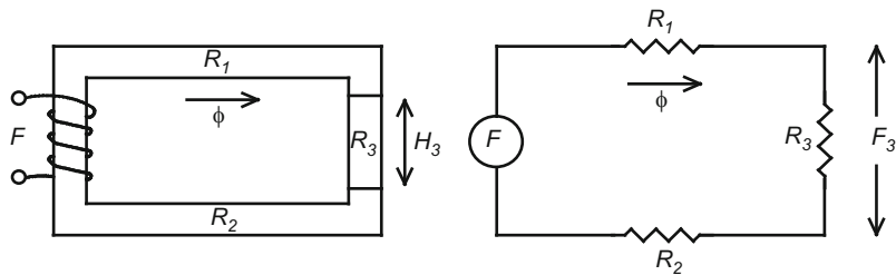
Fig. 13.3 Magnetic equivalent circuit
