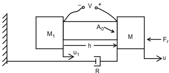
Fig. 3.17 Two-degree of freedom system driven by a piezoelectric ceramic bar with voltage V applied
