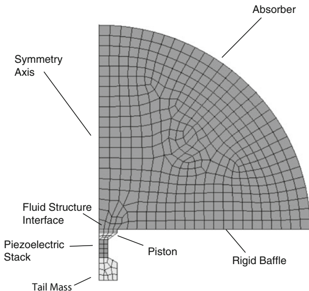
Fig. 3.54 Axi-symmetric finite element model of a Tonpilz transducer set in a rigid baffle with fluid field and absorbers
