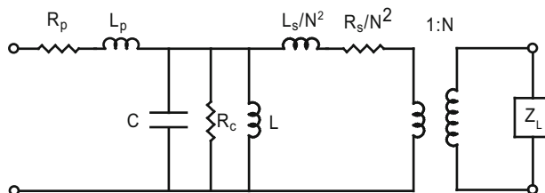
Fig. 13.16 Equivalent circuit for a transformer
