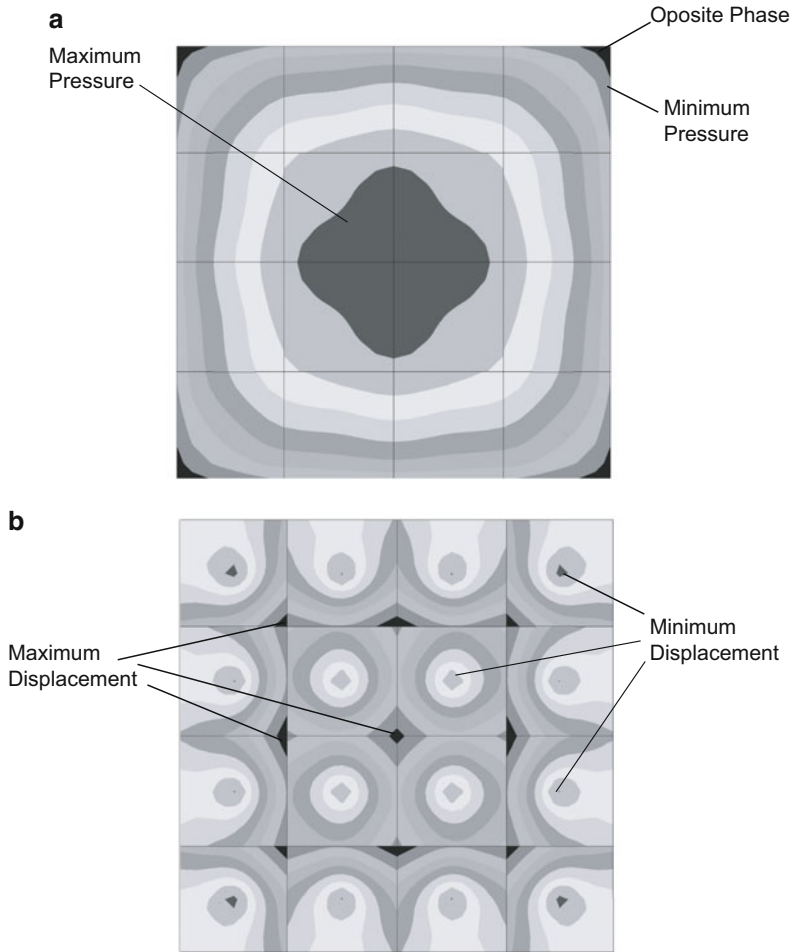
Fig. 7.17 (a) Pressure contours on a 16 element array. (b) Displacement contours on the 16 element array
