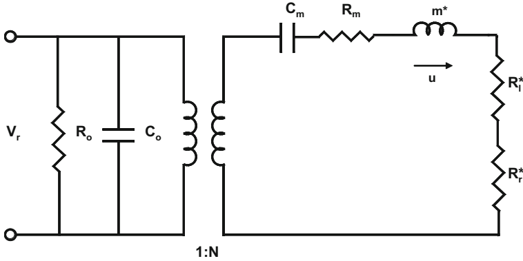
Fig. 2.14 Lumped 1 degree of freedom equivalent circuit \omega_r M \gg R_l + R_r with R_o the clamped shunt resistance, R_m the equivalent-stack mechanical series-loss resistance, R_l^* the equivalent mechanical mounting loss resistance, and R_r^* the equivalent radiation resistance
