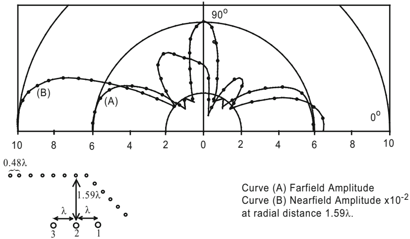
Fig. 9.34 Exact (—) and predicted (···) far-field (a) and near-field (b) pressure amplitude polar beam patterns for three sources with amplitude ratios 3:2:1 and one wavelength separation with the 13-element hydrophone arrangement [22]
