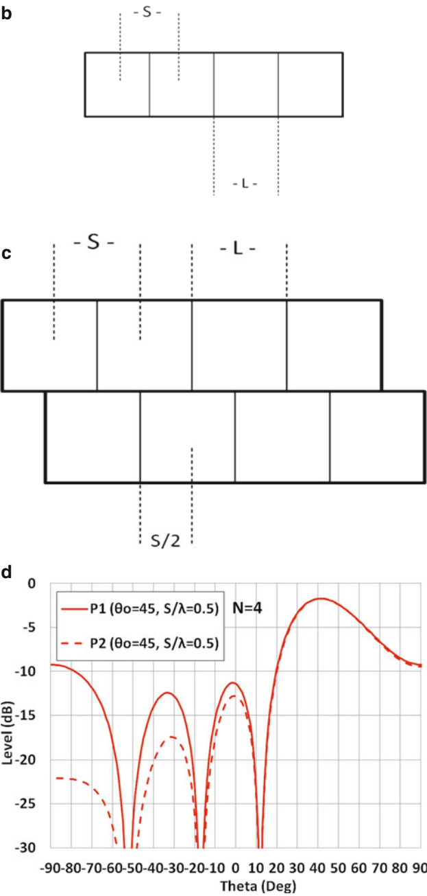
Fig. 7.9 (b) Four element line array, with center-to-center separation S . (c) Staggered four element line array, with center-to-center separation S/2 . (d) Side lobe comparison of in-line, P_1 , and staggered, P_2 , results for 45^\circ steering.
