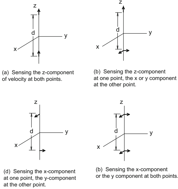
Fig. 8.25 Diagrams for calculating the spatial correlation between two uniaxial dipole sensors separated by a distance, d , sensing different velocity components (each solid arrow represents a dipole sensor)
