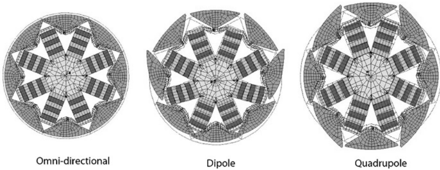
Fig. 5.65 FEA of first three modes of vibration for 6 in. octoid
