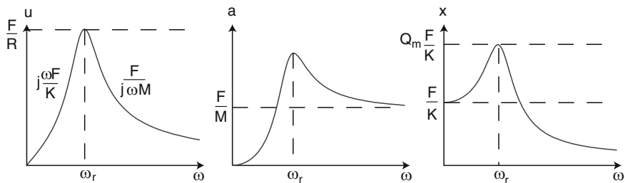
Fig. 3.2 Velocity, u , acceleration, a , and displacement, x , response for the lumped-parameter vibrator of Fig. 3.1
