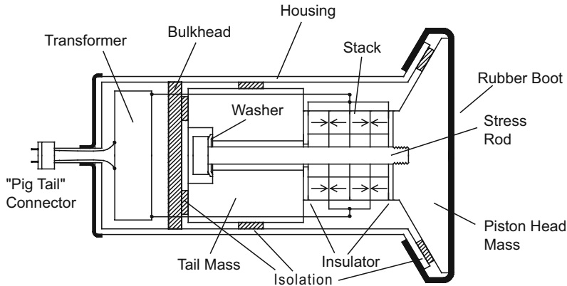
Fig. 5.17 Cross section of typical Tonpilz transducer
