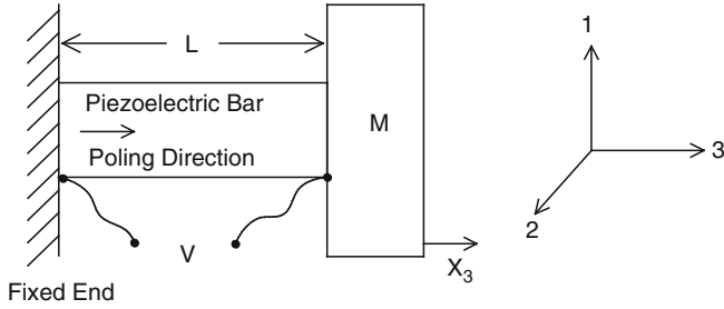
Fig. 12.1 The 33-mode piezoelectric longitudinal vibrator with working strain parallel to poling direction and electrodes on the ends of the bar
