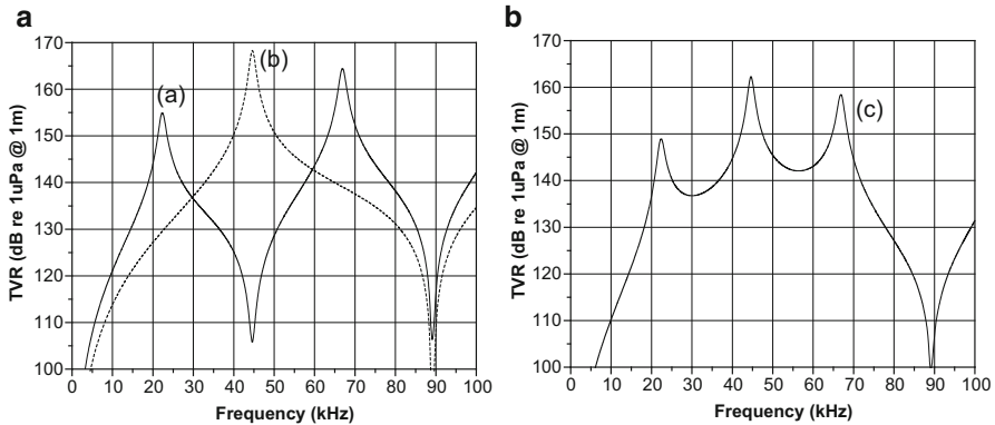
Fig. 5.33 Even (a), odd (b), and combined (c) mode excitations [44]
