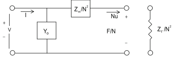
Fig. 3.46 Alternative electrical representation of equivalent circuit of Fig. 3.15
