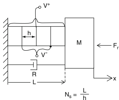
Fig. 3.52 (a) Transducer dynamic motion with flexing head. (b) Transducer dynamic motion with stiffened head
