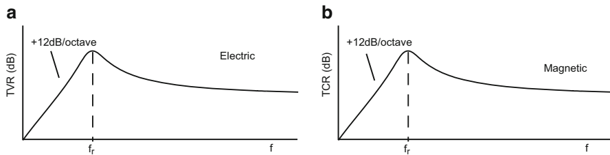
Fig. 9.13 (a) Transmitting voltage response for electric field transducer. (b) Transmitting current response for magnetic field transducer
