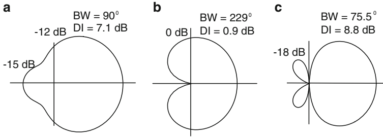
Fig. 6.32 Addition of the quadrupole mode with omni, dipole, and quadrupole ratios (a) 1:1:0.414, (b) 1:2/3:−1/3, and (c) 1:2:1
