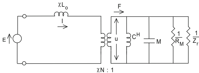
Fig. 5.7 Mobility circuit representation of the mechanical portion
