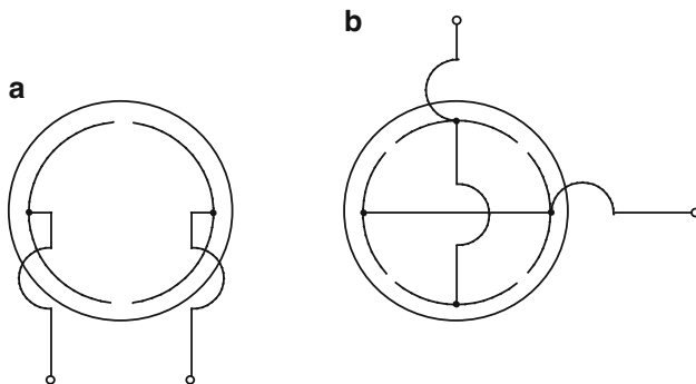
Fig. 5.15 Wiring scheme excitation of the dipole (a) and quadrupole (b) modes
