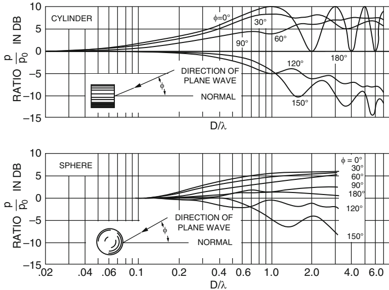
Fig. 9.35 Diffraction of a sound wave by cylinder and sphere
