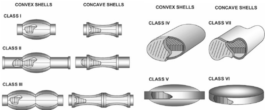
Fig. 1.13 Sketch of various classes of flextensional transducers [31]
