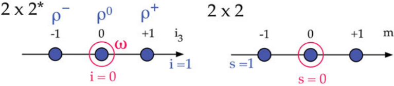
Fig. 6.3 Weight diagram of SU(2) \times SU(2) for isospin \frac{1}{2} (left) and for spin \frac{1}{2} (right). The states i_3 = 0 and m = 0 are doubly occupied
