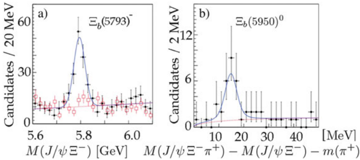
Fig. 17.12 (a) J/\psi(\rightarrow \mu^+\mu^-)\Xi^- invariant mass distribution in pp collisions at 7 TeV with the \Xi_b(5793)^- signal. The open (red) squares show the background from events associated with a wrong charge (positive) pion from \Xi^- decay; (b) observation of the \Xi_b(5950)^0 decaying into \Xi^-\pi^+ . The dotted curve shows the background [16]
