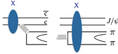
Fig. 16.5 The X(3872) as a charmonium meson (left) or a tetraquark (right)
