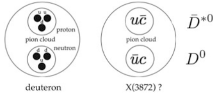
Fig. 16.6 The X(3872) as a loosely bound D^0 \bar{D}^{*0} system similar to the deuteron
