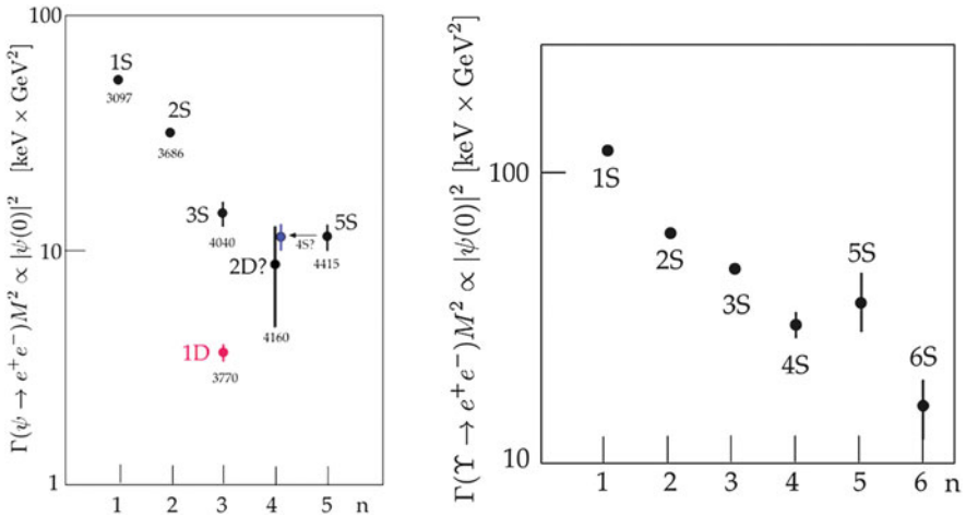
Fig. 8.5 Left: e^+e^- partial widths of 1^{--} c\bar{c} mesons. The \psi(3770) , and possibly the \psi(4160) , are 1^3D_1 and 2^3D_1 orbital excitations. Right: e^+e^- partial widths of the 1^{--} b\bar{b} mesons
