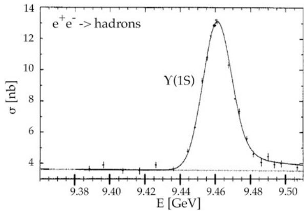
Fig. F.1 The \Upsilon(1S) in e^+e^- \rightarrow \Upsilon(1S) \rightarrow \text{hadrons} , after Kobel, M., et al.: Z. Phys. C 53, 193 (1992)
