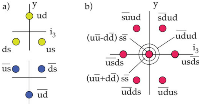
Fig. 16.1 (a) Weight diagrams of the 3^* and 3 representations of \text{SU}(3)_f for diquarks and antidiquarks, respectively; (b) scalar nonet of the lightest tetraquark configuration (see the text)
