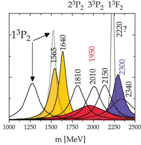
Fig. 11.10 The tensor mesons that have been observed so far, normalized to unit area. The f_2(1270) and f_2'(1565) (arrows) are firmly established as the ground state n\bar{n} and s\bar{s} tensor mesons, respectively. The quantum numbers of the narrow state at 2220 MeV are not well established
