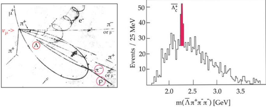
Fig. 17.4 Left: bubble chamber picture of the reaction \nu_\mu p \rightarrow \mu^- \Lambda \pi^+ \pi^+ \pi^- \pi^+ with \Lambda \rightarrow \pi^- p (adapted from [3]). One of the two tracks labelled \pi^- or \mu^- is the negative muon induced by the \nu_\mu . The loop is due to the decay chain \pi^+ \rightarrow \mu^+ \rightarrow e^+ . Right: observation of the (\bar{u}dc) \bar{\Lambda}_c^+ decaying into \bar{\Lambda} \pi^+ \pi^- \pi^- in a broadband photon beam [4]
