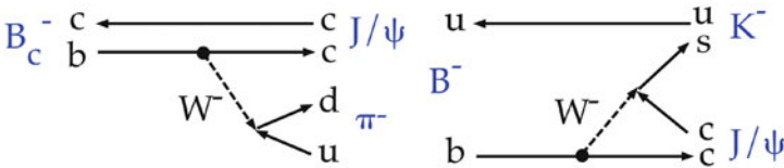
Fig. 8.9 Top: J/\psi \pi^\pm mass distribution (left) and enhanced region around the B_c^\pm signal (right). The peak around 5.2 GeV is due to the background channel B^\pm \rightarrow J/\psi K^\pm with the pion mass incorrectly attributed to the kaon [16]. Bottom: Cabibbo favoured decays of the B_c^- and B^-
