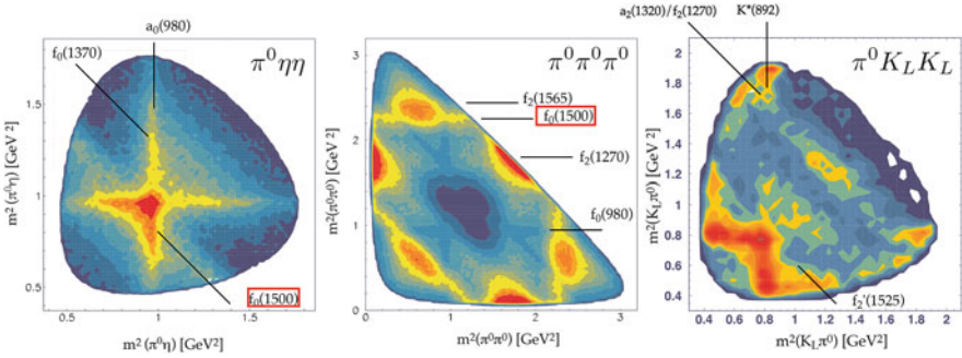
Fig. 11.3 \pi^0 \eta \eta ( 2.0 \times 10^5 events) and \pi^0 \pi^0 \pi^0 Dalitz plots ( 7.1 \times 10^5 events) in \bar{p}p annihilation at rest into 6\gamma ; \pi^0 K_L K_L Dalitz plot [10] ( 3.7 \times 10^4 events) (colour pictures from [8])
