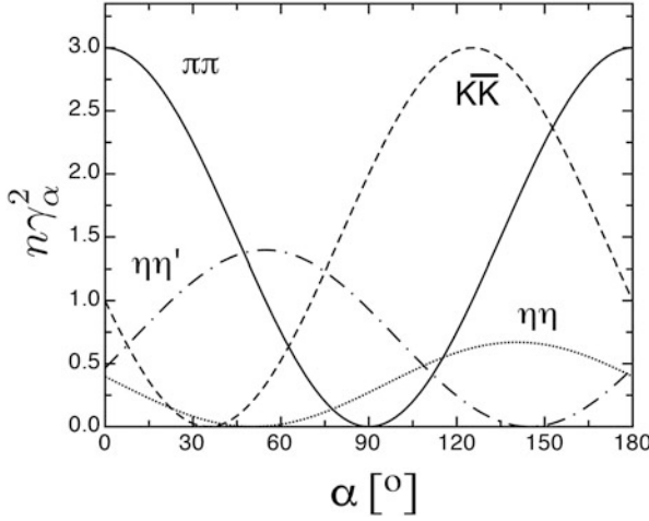
Fig. 11.6 SU(3) predictions for isoscalar q\bar{q} scalar (or tensor) mesons decaying into pseudoscalar pairs, assuming \theta = -17.3^\circ and \rho = 1 [14]
