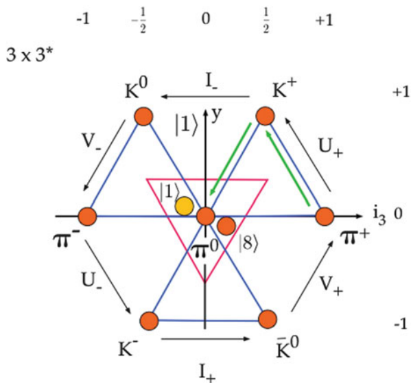
Fig. 7.3 The nonet of the 0^{-+} mesons ( 3 \times 3^* representation) decomposes into an octet and a singlet
