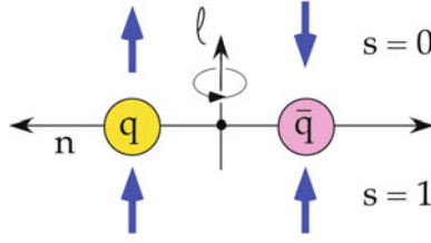
Fig. 2.1 A q\bar{q} meson is in a spin-singlet state ( s = 0 , antiparallel quark spins) or in a spin-triplet state ( s = 1 , parallel quark spins). Excited states are obtained by switching angular momentum \ell > 0 within the pair (orbital excitation) or by inducing vibrations n > 1 (radial excitations)
