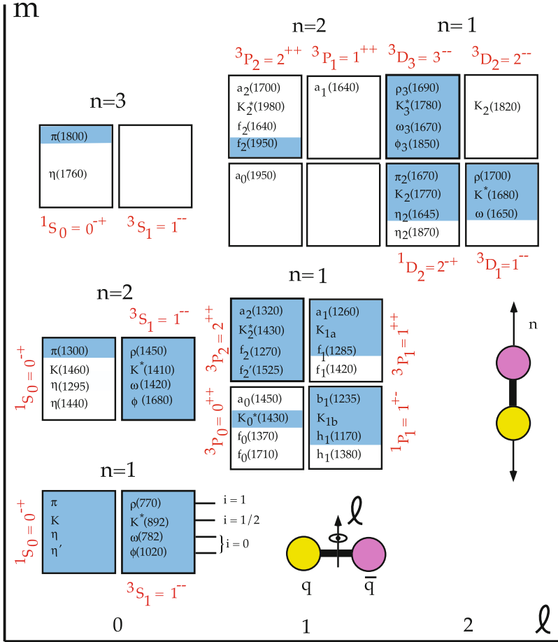
Fig. 5.1 The mesons made of the u , d , and s light quarks are organised in n^{2s+1}\ell_j nonets (or J^{PC} ). The well established mesons are shown in the dark (blue) areas. Strong evidence has been reported for those in the white areas, but their classification is tentative. The vertical mass scale is approximate. Many orbital and radial excitations have not been identified yet (see the text and also Fig. 1.1 for further candidates)
