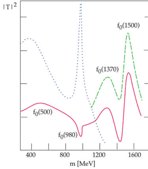
Fig. 12.3 \pi^0\pi^0 and \eta\eta mass distributions (in arbitrary units). Full red curve: \pi^0\pi^0\pi^0 ; dotted blue curve: \pi^0\pi^0\eta ; dashed green curve \pi^0\eta\eta (compiled from [5])
