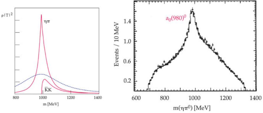
Fig. 12.2 Left: predicted \eta\pi and K\bar{K} mass distributions (in arbitrary units, full red curves) for a_0(980) resonance production in \bar{p}p annihilation into a_0\pi , according to the Flatté formalism with g_1 = 324 MeV, g_2 = 329 MeV ( \Gamma'_0 = 462 MeV). The observed width is about 54 MeV. The dashed blue line shows the \eta\pi mass distribution for the same width \Gamma'_0 in the absence of K\bar{K} decay ( g_2 = 0 ). The observed width increases to 300 MeV. Right: the a_0(980) \rightarrow \eta\pi^0 resonance in proton-antiproton annihilation at rest into \eta\pi^0 [4]
