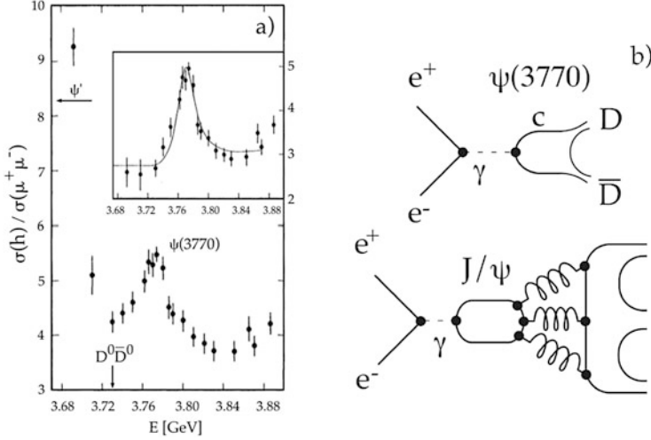
Fig. 8.4 (a) Observation of the \psi(3770) in the cross section for e^+e^- \rightarrow \text{hadrons} just above D^0\bar{D}^0 production threshold (see the text, adapted from [6]). The inset shows the fitted signal after subtracting the radiative processes from the \psi' ; (b) excitation and decay of the \psi(3770) resonance into D\bar{D} ( D^0\bar{D}^0 or D^+D^- ). D decay contributes to (and dominates) the hadronic final state. The J/\psi and \psi' lie below threshold and decay hadronically through OZI-suppressed decays (or through electromagnetic processes such as e^+e^- , \mu^+\mu^- , or \gamma + \text{hadrons} )
