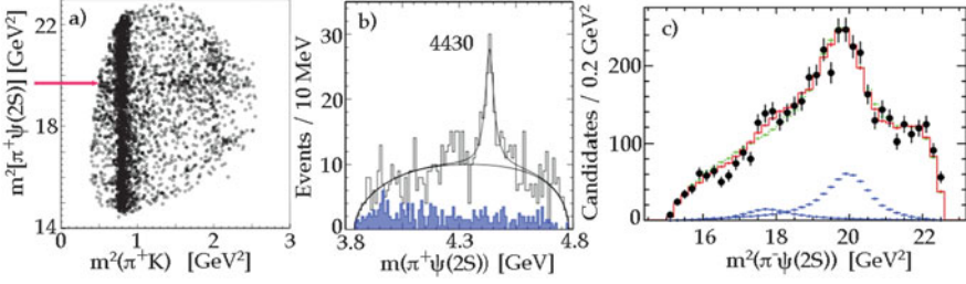
Fig. 16.7 Observation of the Z_{c1}(4430)^{\pm} ; (a) \pi^+\psi(2S) vs. \pi^+K Dalitz plot in B \rightarrow K\pi^+\psi(2S) from Belle [19]; (b) \pi^+\psi(2S) mass projection with fit excluding the K^* band. The dark (blue) area shows the excluded K^* contribution; (c) m^2(\pi^-\psi(2S)) projection in B^0 \rightarrow K^+\pi^-\psi(2S) from LHCb. The strong peak around 20 \text{ GeV}^2 (with contribution shown by the blue bottom distribution) is due to the Z_{c1}^-(4430) . A possible additional resonance around 4200 \text{ MeV} is also suggested [20]
