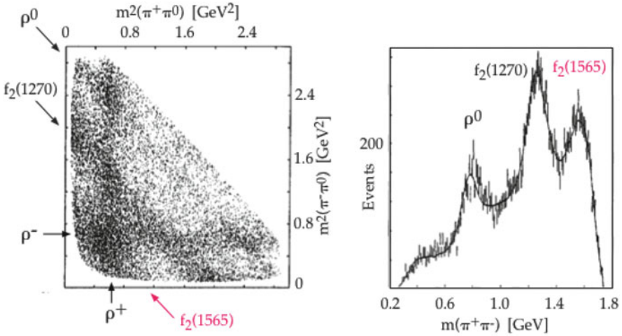
Fig. 11.11 Left: \pi^+\pi^-\pi^0 Dalitz plot in \bar{p}p annihilation at rest in gaseous hydrogen. Right: \pi^+\pi^-\pi^0 invariant mass projection. The curve shows the Dalitz plot fit (adapted from [31])
