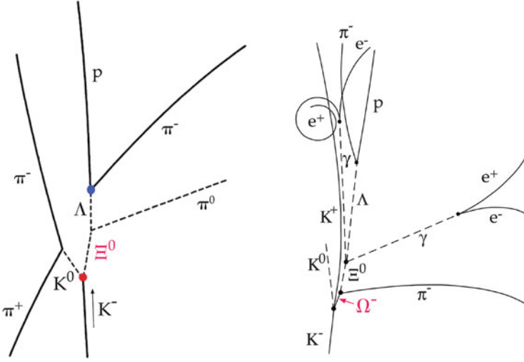
Fig. 13.3 Left: production and decay of the first \Xi^0 hyperon observed in a bubble chamber [1]. The trajectories of the invisible neutral particles are shown by dashed lines (see the text). Right: bubble chamber photograph showing the production and decay of the \Omega^- [2]
