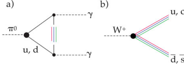
Fig. 10.2 (a) \pi^0 decay into 2\gamma . The quark colours increase the amplitude of the triangular diagram by a factor of 3; (b) the W^+ boson decays into u\bar{d} and c\bar{s} with a probability of 2 \times 3 (colour) \times 0.11 \simeq 66\% . The decays into e^+\bar{\nu}_e , \mu^+\bar{\nu}_\mu and \tau^+\bar{\nu}_\tau account for the remaining 34%
