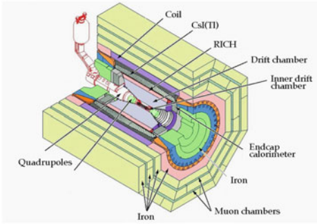
Fig. 9.7 Left: the CLEO III / CLEO-c detector at the Cornell electron-positron collider CESR [16]. Right: radiative transitions from the \Upsilon(2S) and \Upsilon(3S) states [17] (see the text and Fig. 9.6)
