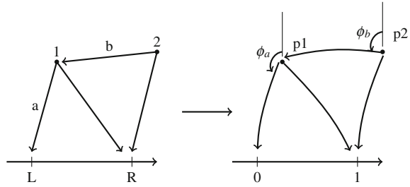
Fig. 4.4 Representation of \Gamma on \mathbb{R}^2
