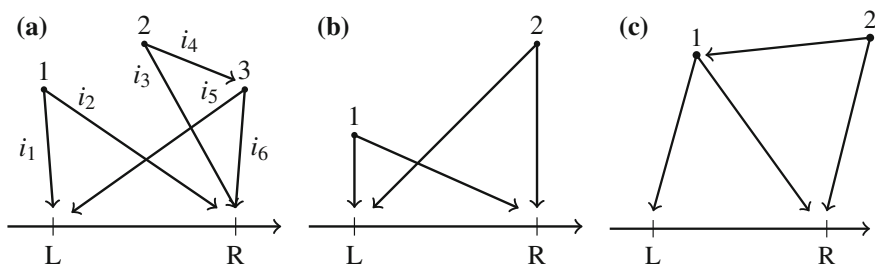
Fig. 4.1 Admissible graphs
