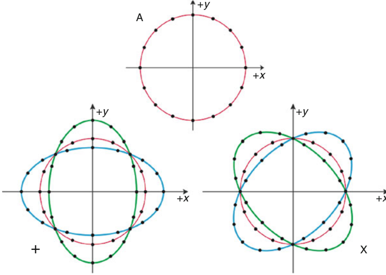
Fig. 1.2 The plus and cross polarizations of a gravitational wave. A represents a circle of test masses at rest, in the absence of a GW. the lower left image is the response to a “+” polarized GW, and the lower right image is the response to a “x” polarized GW. This is the characteristic stretching and squashing of spacetime, due to a GW. Imagine reproduced from Larson and Wheeler (2013)
