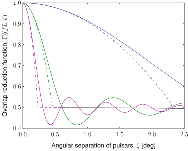
Fig. 3.4 The small angle approximation of the isotropic ORF compared to the full ORF. Moving from right to left: the solid line is the full ORF and the dashed line is the approximation given by Eq. (3.15) for fL = 10 (online blue), fL = 51.2 (green), and fL = 100 (magenta). Empirically, we find that the approximation holds for \zeta \lesssim 2.3^\circ (fL/10) , Eq. (3.16). Afterward the ORF reverts to the Earth-term only solution which, due to its slowly varying initial slope, appears to be flat over 0^\circ \leq \zeta \leq 3^\circ . Figure reproduced from Mingarelli et al. (2014)
