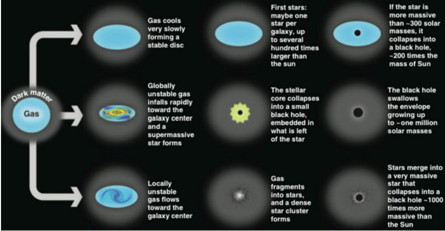
Fig. 1.3 The three principal black hole seed theories, from Volonteri (2012)
