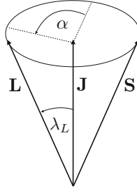
Fig. 4.1 Precession geometry for a spinning binary: here \lambda_L is the angle of the precession cone, \alpha is the precession angle, and the total spin \mathbf{S} = \mathbf{S}_1 + \mathbf{S}_2 and the orbital angular momentum \mathbf{L} precess around the (essentially) constant direction of the total angular momentum, \mathbf{J} = \mathbf{S} + \mathbf{L} at a rate d\alpha/dt , given by Eq. (4.6)
