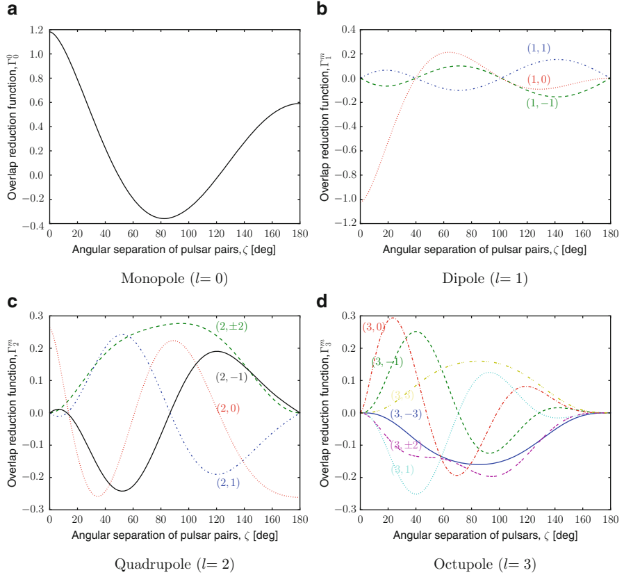
Fig. 2.2 The Earth-term only, generalized overlap reduction functions \Gamma_l^m in the computational frame for l = 0, 1, 2, 3 as a function of the angular separation of pulsar pairs. In the computational frame, \Gamma_l^{-m} = (-1)^m \Gamma_l^m . For the l = 0 case, \Gamma_0^0 is the Hellings and Downs curve up to the multiplicative constant 4\sqrt{\pi}/3 . Figure reproduced from Mingarelli et al. (2013)
