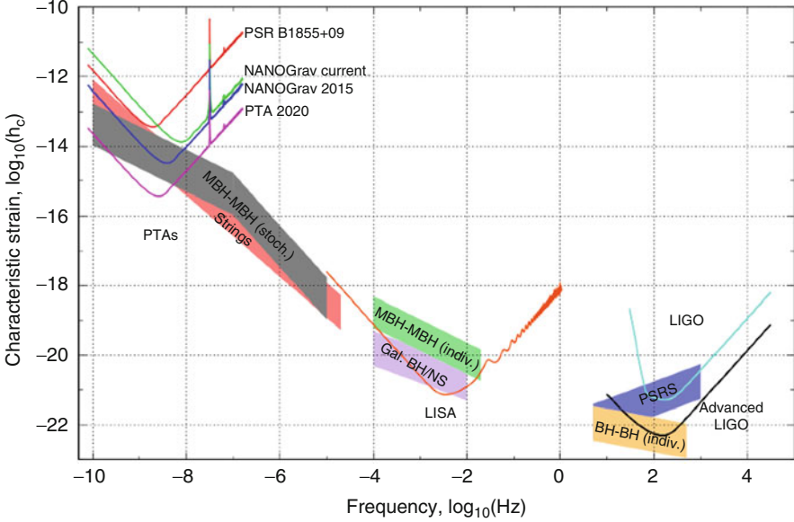
Fig. 1.5 The GW strain spectrum from PTAs in the nHz band to ground-based laser interferometers in the kHz band. Note the lack of sensitivity in the PTA band to frequencies of 1/year—this is due to solar system ephemeris errors. Pulsar TOA fitting processes remove low-frequency information, making PTAs less sensitive to the lower frequency limit of the PTA band. Image reproduced from Demorest et al. (2009)
