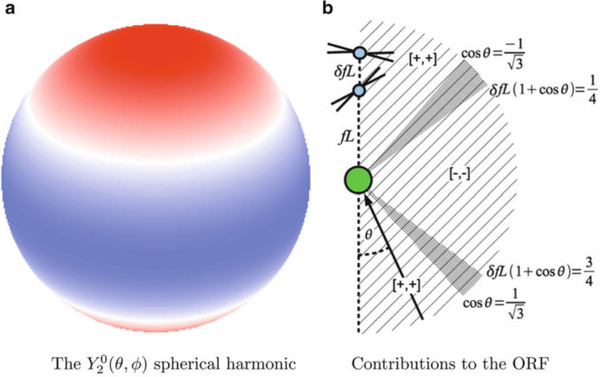
Fig. B.1 (a) The energy density distribution for Y_2^0(\theta, \phi) . The red and blue regions are positive and negative, respectively. (b) The Earth (green, equivalently the SSB) is at the centre with the two pulsars above. The magnitude of the ^{(ab)}\Gamma_2^0(fL, \zeta) ORF is enhanced by small 0 < \delta fL \lesssim 1 pulsar b displacements, over the \delta fL = 0 case. The arrow shows the direction of a GW propagating with incoming angle \theta . The lighter shaded regions of the diagram show the regions of the sky from which the signal will contribute positively to the ORF. The darker shaded regions will contribute negatively to the ORF, though their size depends on \delta fL . The brackets indicate the [sign of the pulsar term correlation, sign of the background energy density]. Figure reproduced from Mingarelli and Sideri (2014)
