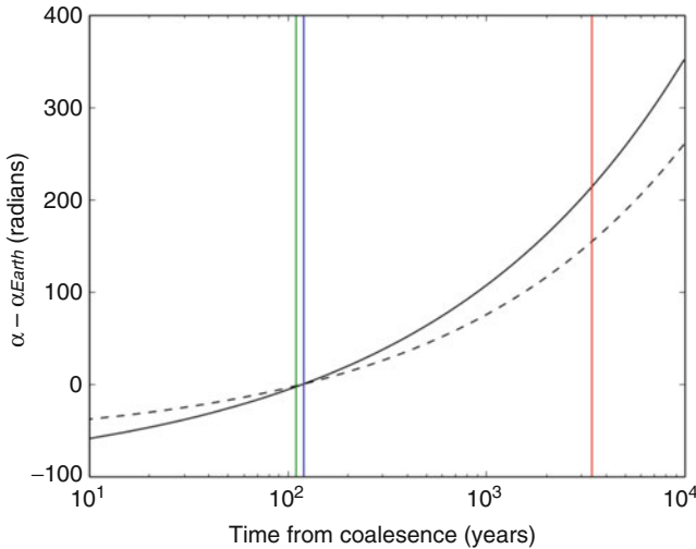
Fig. 4.2 The precession angle \alpha = 0 at the Earth, as a reference. The red line highlights a distance of 1 kpc, the blue line is the beginning of the observation at the Earth and the green line is after a 10 year observation, hence is closer to coalescence. For the a dimensionless spin parameter a = 0.98 ( a = 0.10 ), the solid (dashed) line is the change in \alpha for a 10^9 M_\odot SMBHB. Over 10 years, \Delta\alpha \sim -3 \text{ rads} ( -2 \text{ rads} ), however, over 1 kpc, \Delta\alpha \sim 213 \text{ rads} ( 154 \text{ rads} )
