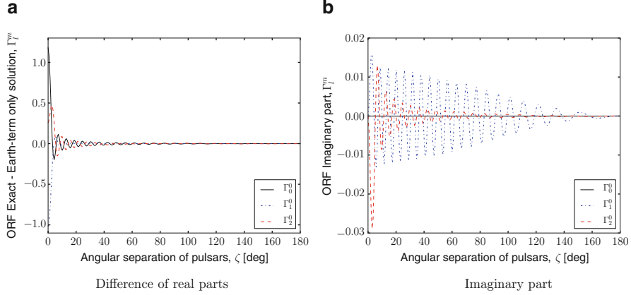
Fig. 2.3 Generalized overlap reduction functions (ORF) with the pulsar term. (a) The difference between the exact solution and the Earth term-only solution for fL = 10 in the computational frame. These oscillations are already quite small for \zeta = 60^\circ and rapidly converge to zero for larger values of \zeta . (b) The value of the complex component of the pulsar term for fL = 10 in the computational frame. Recall that the Earth-term only solution is always real, but introducing the pulsar term gives rise to complex-valued overlap reduction functions, even in the computational frame. Notice that these oscillations induced by the pulsar term are at least an order of magnitude smaller than the real part but do not, however, converge as quickly as the real component. The \Gamma_0^0 function has no imaginary component. Figure reproduced from Mingarelli et al. (2013)
