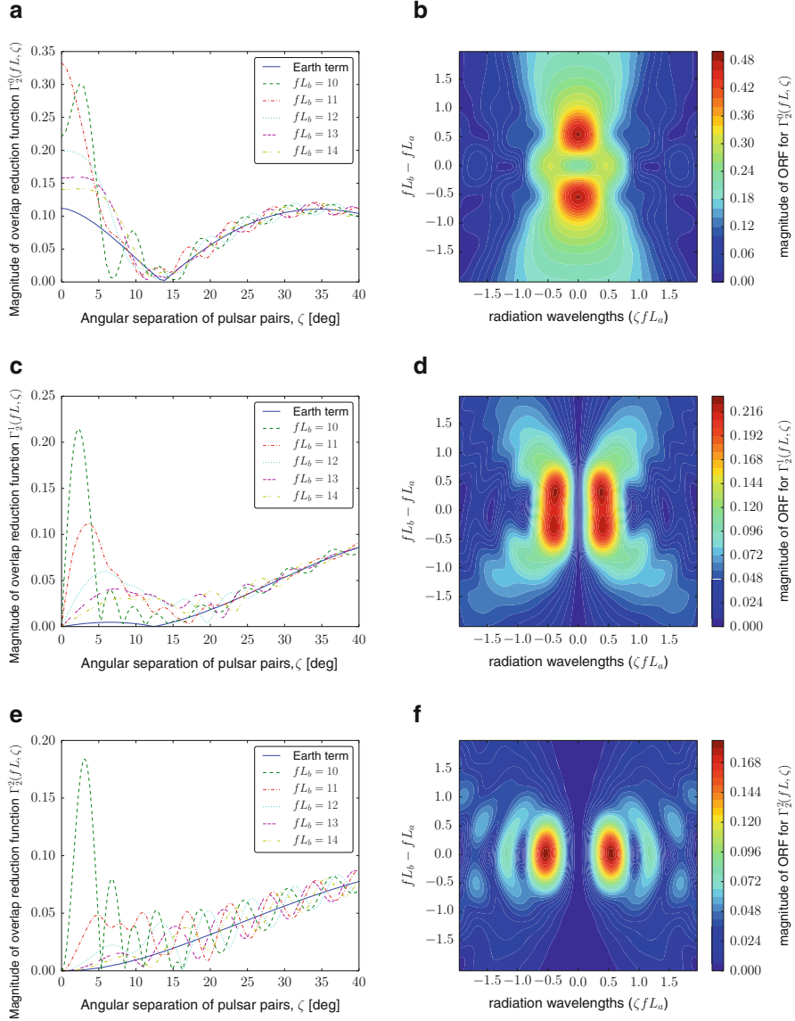
Fig. 3.3 The effect of pulsar distance variations on the magnitude of the quadrupole overlap reduction functions, with fL_a = 10 fixed. Panels on the left hand side are truncated at 40^\circ since error bars on each point are expected to be of the order of 10–20 %. Moreover it is clear that the pulsar term oscillations rapidly converge to zero. Note that the maximum value of some ORFs is achieved for small, but non-zero, angular separations between pulsar pairs. (a) Magnitude of the ^{(ab)}\Gamma_2^0(fL, \zeta) ORF. (b) Strong pulsar term regime of ^{(ab)}\Gamma_2^0(fL, \zeta) . (c) Magnitude of the ^{(ab)}\Gamma_2^1(fL, \zeta) ORF. (d) Strong pulsar term regime of ^{(ab)}\Gamma_2^1(fL, \zeta) . (e) Magnitude of the ^{(ab)}\Gamma_2^2(fL, \zeta) ORF. (f) Strong pulsar term regime of ^{(ab)}\Gamma_2^2(fL, \zeta) . Figure reproduced from Mingarelli et al. (2014)
