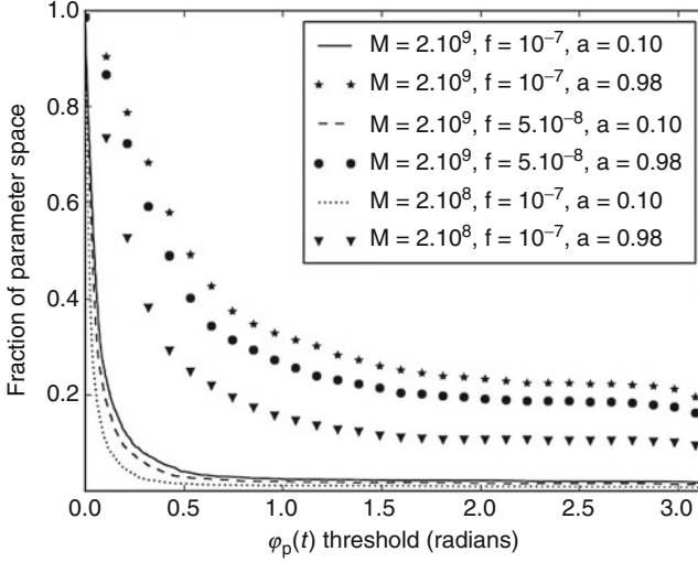
Fig. 4.3 The fraction of parameter space in \hat{\Omega} and \hat{\mathbf{p}} for which the maximum excursion of \varphi_p over the time L_p(1 + \hat{\Omega} \cdot \hat{\mathbf{p}}) for L_p = 1 kpc exceeds a certain value, shown on the horizontal axis. Several values of m_{1,2} , a and f_{\text{GW,E}} are considered (see legend). Figure reproduced from Mingarelli et al. (2012)
