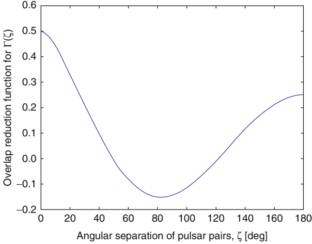
Fig. 1.8 The overlap reduction function for an isotropic stochastic GW background, called the Hellings and Downs curve
