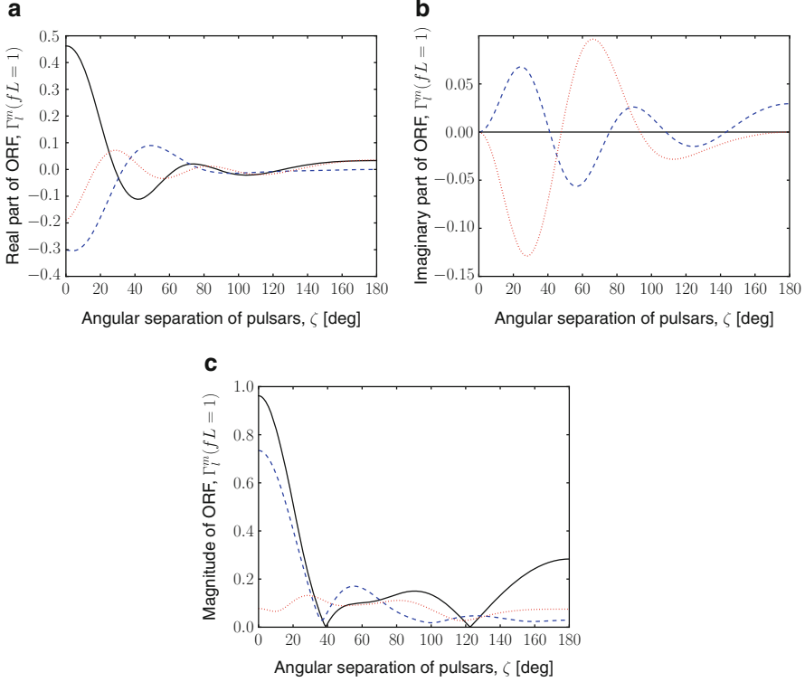
Fig. 3.5 In both panels ^{(ab)}\Gamma_0^0(fL, \zeta) is the solid curve, ^{(ab)}\Gamma_1^0(fL, \zeta) is the dashed curve (blue) and ^{(ab)}\Gamma_2^0(fL, \zeta) is the dotted curve (red). These functions are the most sensitive to the pulsar term, as they have non-zero values at \zeta = 0 . (a) The behaviour of the pulsar term only for ^{(ab)}\Gamma_0^0(fL, \zeta) , ^{(ab)}\Gamma_1^0(fL, \zeta) and ^{(ab)}\Gamma_2^0(fL, \zeta) when L_a = L_b = L and fL = 1 . This is found by subtracting the Earth term from the numerically integrated overlap reduction function. (b) The imaginary part only of ^{(ab)}\Gamma_0^0(fL, \zeta) , ^{(ab)}\Gamma_1^0(fL, \zeta) and ^{(ab)}\Gamma_2^0(fL, \zeta) when fL = 1 . As there is no imaginary part in the computational frame where the Earth term is calculated, we cannot display the difference as done in (a) . Note that these imaginary values are only a factor a few smaller than their real counterparts, with the exception of ^{(ab)}\Gamma_0^0(fL, \zeta) where the imaginary part is zero. Moreover, they do not quickly converge to zero as in previous cases for fL \geq 10 . (a) Real part, Pulsar term—Earth term ORF. (b) Imaginary part of the ORFs. (c) Magnitude of the overlap reduction functions. Figure reproduced from Mingarelli et al. (2014)
