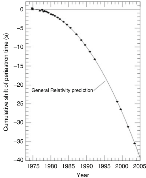
Fig. 1.1 Evidence for GWs form the change in the periastron of PSR 1913 + 16, updated in Weisberg and Taylor (2005). Experimental data are the filled circles , error bars are half a percent, and the solid line is the change in periastron according to the gravitational wave emission model proposed by general relativity
