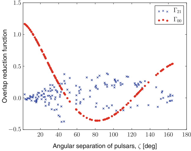
Fig. 2.1 The real-value overlap reduction functions \Gamma_{00} and \Gamma_{21} for 18 EPTA pulsars in the cosmic rest-frame. Note that for illustrative purposes, we have not included the autocorrelation term ( \zeta = 0 ). Figure reproduced from Mingarelli et al. (2013)
