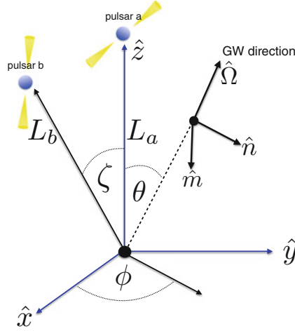
Fig. 1.7 The “computational” reference frame: pulsar a is on the z -axis at a distance L_a from the origin, pulsar b is in the x - z plane at a distance L_b from the origin making an angle \zeta with pulsar a , \hat{\Omega} is the direction of GW propagation and \hat{m} \times \hat{n} = \hat{\Omega} . The polar and azimuthal angles are given by \theta and \phi , respectively. This figure was reproduced from Mingarelli and Sidery (2014)
