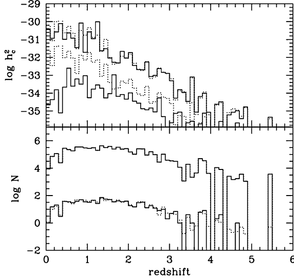
Fig. 1.4 Contribution of different redshift intervals to the build-up of the GW signal at two different frequencies, f = 8 \times 10^{-9} Hz and 10^{-7} Hz, computed using Monte Carlo sampling ( solid lines ) and a semi-analytical approach ( dotted lines ). In each panel, the upper histograms refer to f = 8 \times 10^{-9} Hz and the lower histograms refer to f = 10^{-7} Hz. Figure and caption reproduced from Sesana et al. (2008)’s Fig. 4
