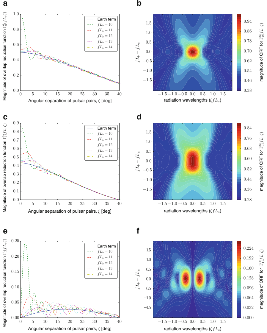
Fig. 3.2 The effect of pulsar distance variations on the magnitude of the isotropic and dipole overlap reduction functions, with fL_a = 10 fixed. Panels on the left hand side are truncated at 40^\circ , as pulsar term oscillations rapidly converge to zero. (a) Magnitude of the ^{(ab)}\Gamma_0^{(ab)}(fL, \zeta) ORF. (b) Strong pulsar term regime of ^{(ab)}\Gamma_0^{(ab)}(fL, \zeta) . (c) Magnitude of dipole ^{(ab)}\Gamma_1^{(ab)}(fL, \zeta) ORF. (d) Strong pulsar term regime of ^{(ab)}\Gamma_1^{(ab)}(fL, \zeta) . (e) Magnitude of the ^{(ab)}\Gamma_1^{(ab)}(fL, \zeta) ORF. (f) Strong pulsar term regime of ^{(ab)}\Gamma_1^{(ab)}(fL, \zeta) . Figure reproduced from Mingarelli et al. (2014)
