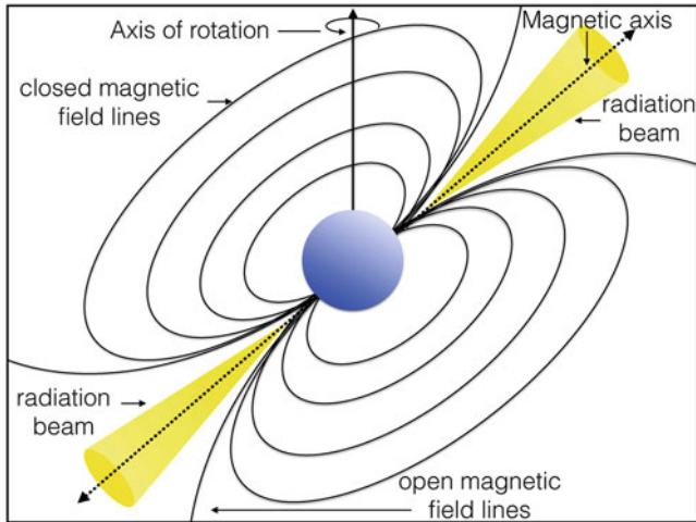
Fig. 1.6 A rotating neutron star with its spin axis misaligned with its magnetic field axis, called a pulsar. Electromagnetic radiation centred on the magnetic field axis is produced above the surface of the pulsar. Due to the misalignment of the magnetic and rotational axes, pulsars are often referred to as cosmic lighthouses, since the received light appears to pulse as the beam crosses our line of sight
