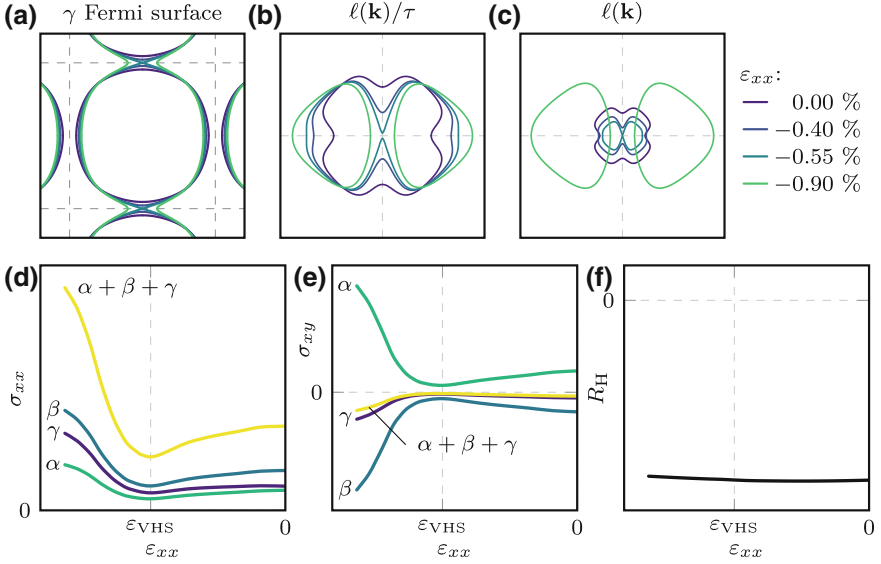
Fig. 3.41 Isotropic- \tau analysis of the Hall effect. Using the measured \rho_{xx} resistivity from Fig. 3.34 an isotropic \tau can be calculated and then used with the geometric interpretation by Ong to calculate the Hall effect. Panel a shows the \gamma Fermi surface at a series of strains and the area swept out by the scattering length \ell(\mathbf{k}) around the Fermi surface at each strain is shown in panels b and c , where in b the data has been scaled by \tau at each strain. The \alpha and \beta Fermi surfaces are much less affected by uniaxial pressure and there is little change to the shape of the \ell(\mathbf{k}) curves. The contributions of all three bands to the conductivities \sigma_{xx} and \sigma_{xy} , within the isotropic- \tau approximation, are shown in panels d and e . The calculated weak-field Hall coefficient is shown in panel f and shows very little change with strain within the isotropic- \tau approximation
