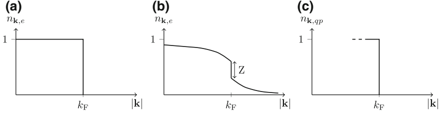
Fig. 1.4 Particle probability distributions. a The probability that any given energy state is occupied by an electron at T = 0 in a Fermi gas, the Fermi-Dirac distribution. b The probability distribution of electrons at T = 0 in a Fermi liquid, the discontinuity at k_F remains. c The probability distribution of quasiparticles in the Fermi liquid recovers the Fermi-Dirac distribution
