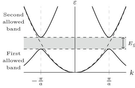
Fig. 1.2 Nearly-free electron dispersion. The free electron dispersion, dashed line, transforms into a set of discrete bands with energy gaps in between when a periodic potential with lattice constant a is weakly introduced
