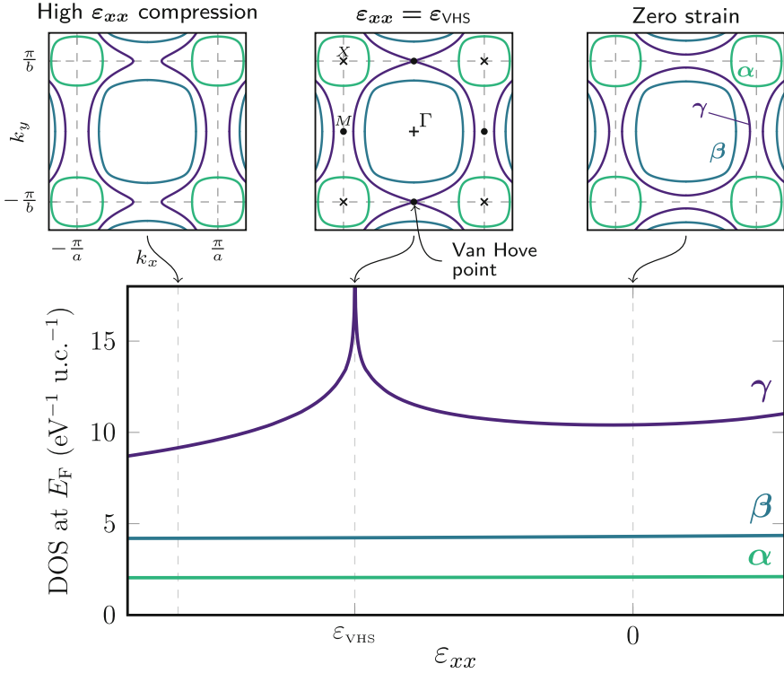
Fig. 3.26 Density of states and Fermi surface calculations. The density of states at the Fermi energy as a function of applied anisotropic strain as calculated from a tight-binding model including strain dependent hopping terms, see main text for details. Three representative Fermi surfaces show the effects of applied strain on the band structure and highlight the Lifshitz transition as the \gamma -band reaches the Van Hove point
