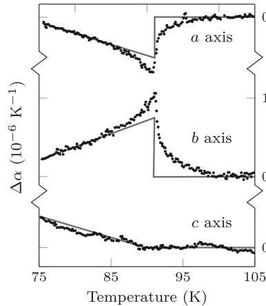
Fig. 2.4 Temperature dependence of thermal expansivities. Change in expansivities for \text{YBa}_2\text{Cu}_3\text{O}_{7-\delta} near the superconducting transition temperature. Based on original data from [21]
