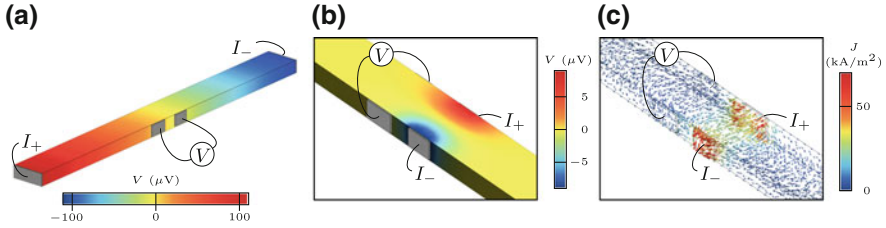
Fig. 4.20 Finite element electrical resistivity simulations. a Finite element simulation of the longitudinal resistivity setup. Real sample dimensions from Fig. 4.18 were used and the room temperature resistivity tensor. At zero field the components are \rho_{aa} = \rho_{bb} = 232 \mu\Omega \text{ cm} and \rho_{cc} \approx 8.5 \text{ m}\Omega \text{ cm} [13]. The simulations are with an applied current of 1 mA. b and c A simulation of the transverse resistivity setup showing the electric potential and current density stream lines
