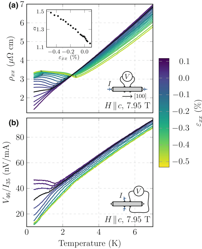
Fig. 4.34 Resistivity against temperature. a Longitudinal resistivity against temperature at 7.95 T for a series of applied strains. The upturn in resistivity marks the onset of the anomalous phase. The transition temperature is identified by the maximum in d^2\rho/dT^2 and is shown by the dashed line. A second transition is seen at lower temperatures for compressions above \sim -0.1\% and the second dashed line follows the corresponding extremum in the second derivative. The inset shows the resistivity temperature exponent at high temperatures calculated from a fit of the form \rho = \rho_0 + AT^\alpha above 3 K. b Transverse resistivity measurement against temperature at 7.95 T for a series of applied strains. See Fig. 4.24 for the measurement configuration. The dashed line marks the maximum in the second derivative with temperature
