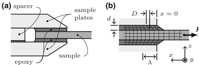
Fig. 2.14 Model for the effective sample length. a Schematic of the symmetric sample mounting. b When a force F is applied to the sample, the load is transferred through the epoxy to the sample plates over a characteristic length scale \lambda . See text for further details
