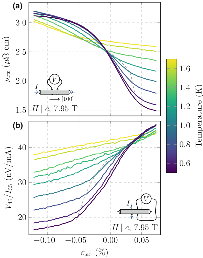
Fig. 4.35 Resistivity against strain. a Longitudinal resistivity against strain at 7.95 T for a series of fixed temperatures. The resistivity is largest in the anomalous phase and the transition is identified by the maximum in d^2\rho/d\epsilon_{xx}^2 . The dashed line follows this maximum in the second derivative. b Transverse resistivity measurement against strain at 7.95 T for a series of fixed temperatures. The transition to the high resistivity phase is identified in the same manner
