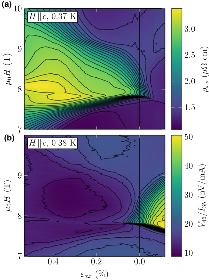
Fig. 4.25 Magnetoresistance contour plots. Contour plots of the longitudinal (a) and transverse (b) resistivities from Fig. 4.24 as a function of c -axis magnetic field and applied strain
