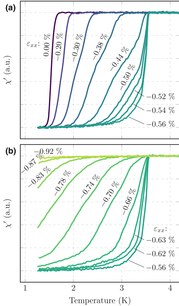
Fig. 3.24 Susceptibility against temperature.
