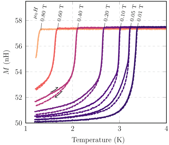
Fig. 3.27 Susceptibility measured at the peak in T_c at various applied fields H \parallel c . Real part of the susceptibility \chi measured as the temperature is swept up and down for sample 1. The y axis is the mutual inductance between the two coils of the susceptibility sensor. The field was incremented at the bottom of each temperature ramp, in the superconducting phase. This disrupts the vortex lattice and is responsible for the apparent hysteresis
