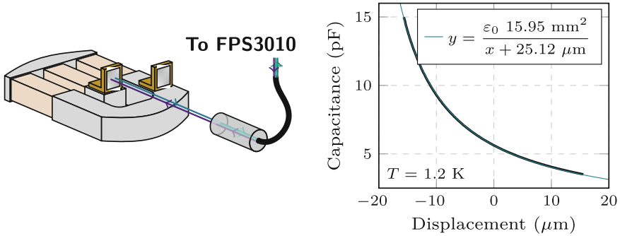
Fig. 2.12 Capacitor calibration. A hermetic feedthrough at the top of the cryostat brings the fibre heads of the attocube FPS3010 interferometer down to low temperatures. The FPS3010 interferometer is a Fabry-Pérot type and takes the first reflection from the sensor head itself and the second from mirrors attached to the uniaxial stress device. By using multiple fibres and mirrors placed at different points on the device an accurate calibration of the capacitive displacement sensor was achieved
