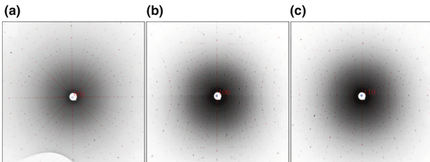
Fig. 4.17 Sample alignment. Pictures of X-ray back-reflection Laue diffraction patterns with simulated fits from OrientExpress [64] overlaid in red. a c -axis aligned with the X-ray beam, b [100] direction and c the [110] direction of the tetragonal unit cell
