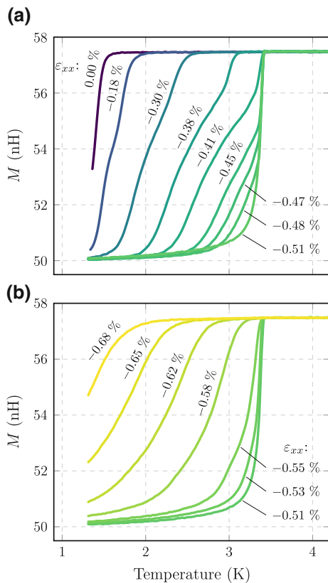
Fig. B.1 Susceptibility against temperature. Real part of the susceptibility \chi for sample 1 against temperature. a Strains below the peak T_c , b above the peak. No normalisation or offsets are applied to the curves. The y axis is the mutual inductance between the two coils of the susceptibility sensor
