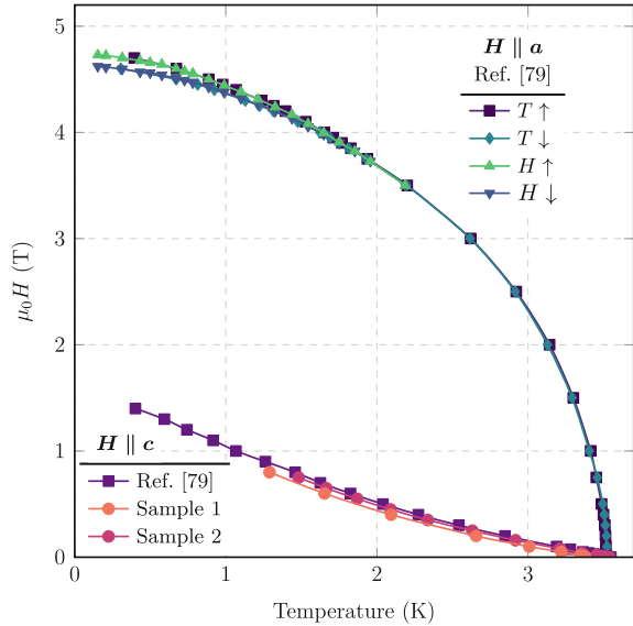
Fig. 3.28 H_{c2} against temperature at the peak in T_c . H_{c2\parallel c} against temperature for samples 1 and 2 compressed to the peak in T_c together with H_{c2\parallel a} at the peak in T_c with compressive strain applied along a measured by Steppke [79]
