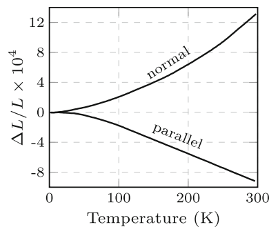
Fig. 2.8 PZT thermal expansion. The thermal expansion of PZT measured both parallel and normal to the poling direction. Based on original data from [37]
