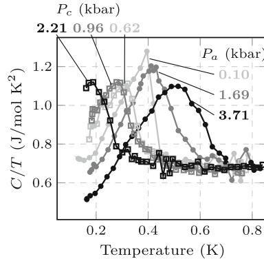
Fig. 2.7 Heat capacity for \text{CeIrIn}_5 under a - and c -axis uniaxial pressure. Uniaxial pressure causes a linear change in T_c with opposite slope for a - and c -axis pressures. Based on original data from [28]
