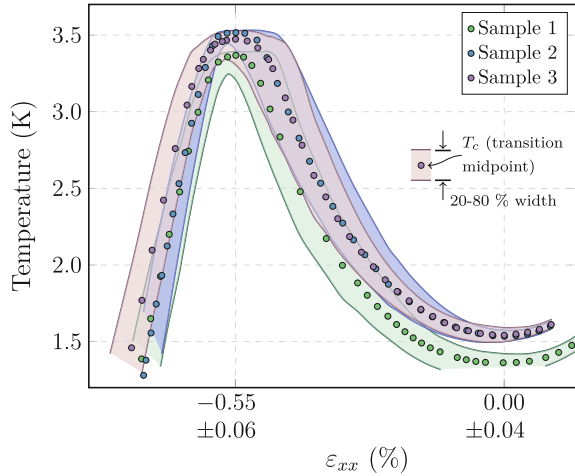
Fig. 3.25 T_c against strain for all three samples. The points are the midpoints (50% levels) of the transitions shown in Figs. B.1, B.2 and 3.24. The 20 and 80% levels of the transitions are shown as lines to give a measure of the transition width. Here the strain scales have been normalised so the peaks in T_c coincide at their average value of (-0.55 \pm 0.06)\%
