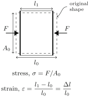
Fig. 2.1 Stress and Strain. Definitions of engineering normal stress and strain, and engineering shear stress and strain
