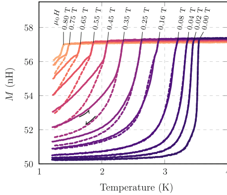
Fig. B.3 Susceptibility measured at the peak in T_c at various applied fields H \parallel c . Real part of the susceptibility \chi measured as the temperature is swept up and down for sample 2. The y axis is the mutual inductance between the two coils of the susceptibility sensor. The field was incremented at the bottom of each temperature ramp, in the superconducting phase. This disrupts the vortex lattice and is responsible for the apparent hysteresis
