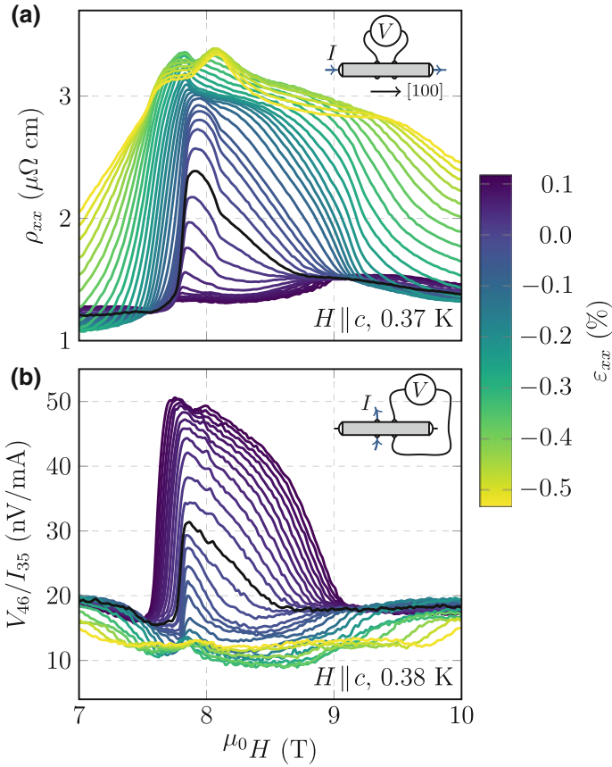
Fig. 4.24 Magnetoresistance. a Longitudinal resistivity \rho_{xx} against c -axis magnetic field for a series of applied strains at 370 mK. b Transverse resistivity measurement against c -axis magnetic field for the same sample and strains. The measurement configuration is depicted in the upper right corner, contact numbers are as per Fig. 4.19. V_{46} is the voltage difference between contacts 4 and 6 when current I_{35} is passed between contacts 3 and 5. The transverse measurements were at 380 mK. The black curves in both panels are the measurements closest to zero strain
