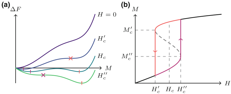
Fig. 4.6 Exchange-enhanced metamagnetism. a Free energy density against magnetisation at several applied fields for an exchange-enhanced Pauli paramagnet with a peak in the density of states close to the Fermi energy. Vertical bars mark minima in the free energy and crosses mark inflection points. b Magnetisation curve in applied field showing the first order metamagnetic jumps at H'_c for increasing field sweeps and H''_c for decreasing field sweeps.
