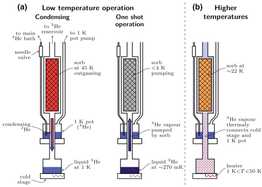
Fig. 4.22 Principle of operation of the ^3\text{He} refrigerator. a and b To reach temperatures below 1 K the condensing cycle begins by warming up the sorb to 45 K, outgassing the adsorbed helium-3 which then condenses through the 1 K pot into the lower helium-3 pot. Once the sorb is cooled back down it also acts as a pump, evaporatively cooling the ^3\text{He} pot by readsorbing the helium-3 gas. c To operate at higher temperatures the sorb is held at 22–25 K maintaining a small pressure of helium-3 gas which provides a heat link between the 1 K pot and the sample stage which is heated using a resistive heater. See text for further details
