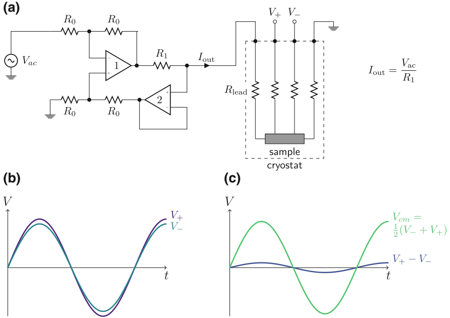
Fig. A.1 A modified Howland bipolarity current source-sink. a Circuit diagram for a single ended voltage to current converter for driving a grounded load. b and c In a four point resistance measurement with long resistive wires in the cryostat, the large lead resistance to ground produces a large common-mode voltage in addition to the normal sample voltage drop
