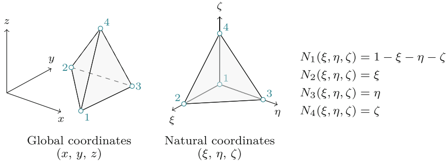
Fig. 2.3 Natural coordinates and shape functions. Natural coordinates of a linear tetrahedral element and the shape functions for this element
