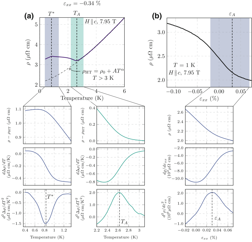
Fig. C.2 Phase boundaries from temperature and strain ramps. a The transition into the A phase through the roof with temperature, T_a , was identified from the point at which the slope of the resistivity deviates from a high temperature power law fit, i.e. a peak in the second derivative. A second feature, T^* , was observed at lower temperatures and high strains and was also identified by an extremum in the second derivative. b The entry into the phase with strain is the least sharp of all the observed features in the data, but it could also be identified from a change in slope of \rho versus \epsilon_{xx} ; a peak in the second derivative of \rho with respect to \epsilon_{xx}
