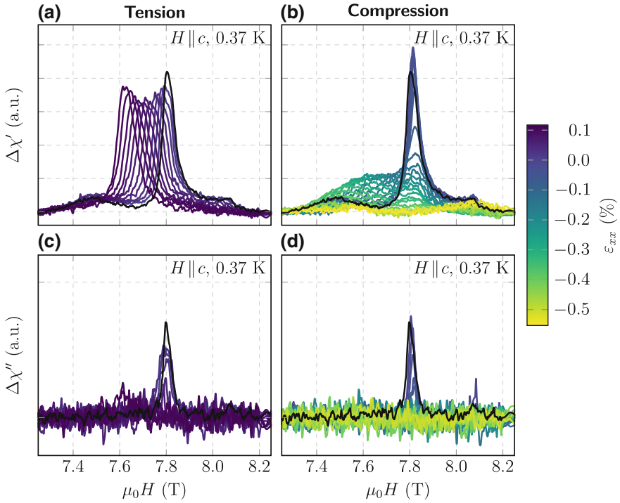
Fig. 4.28 Susceptibility against field. a and b Real part of the AC susceptibility \chi against c -axis magnetic field for a series of applied strains at 370 mK. The black curves are the measurement closest to zero strain. a shows measurements under tensioned and b compression. All measurements are of increasing field sweeps and are quoted as \Delta\chi because of a background subtraction procedure detailed in the text. c and d The imaginary part of the susceptibility for the same measurements. The susceptibility is expressed in arbitrary units but the scale divisions for the real and imaginary susceptibilities are the same
