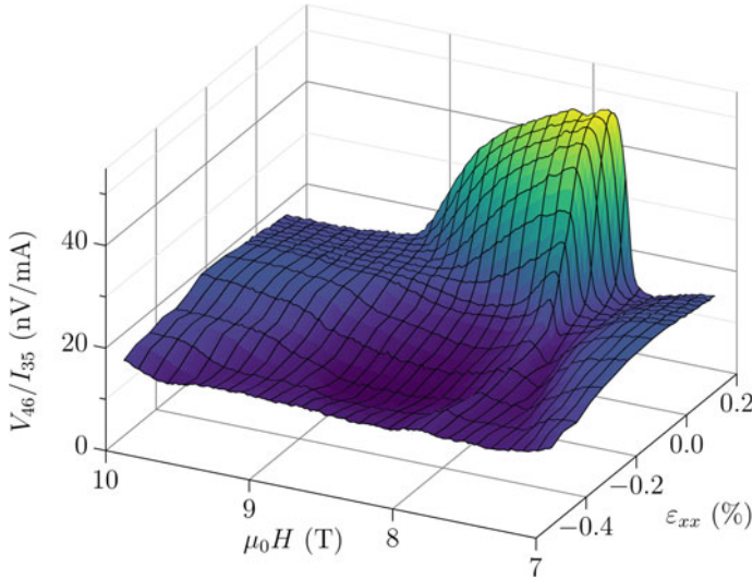
Fig. 4.27 Transverse magnetoresistance. Surface plot of the transverse resistivity against c -axis magnetic field and applied strain at 380 mK. See Fig. 4.24 for the measurement configuration
