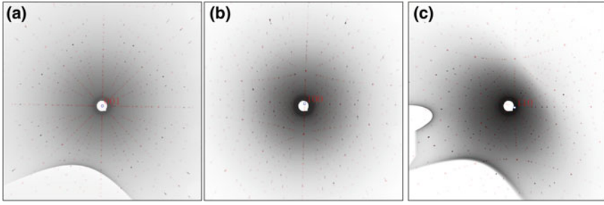
Fig. 3.20 Sample alignment. Pictures of X-ray back-reflection Laue diffraction patterns with simulated fits from OrientExpress [75] overlaid in red. a c -axis aligned with the X-ray beam, b a -axis and c the [110] direction
