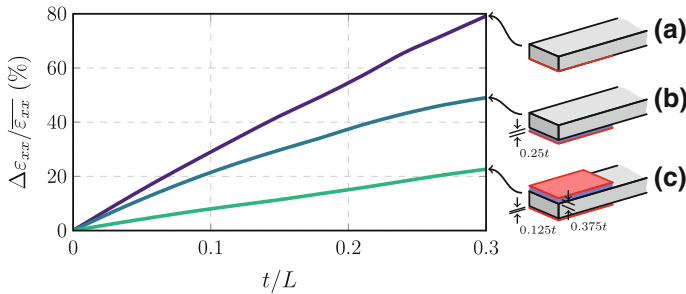
Fig. 2.20 Bending induced strain inhomogeneity. The difference in strain between the top and bottom of a bent sample at the centre divided by the average strain across the central plane of the sample plotted against the sample's aspect ratio. The three cases from top to bottom are: a rigid epoxy holding only the lower sample face; b soft epoxy on the under side of the sample with a thickness equal to 0.25t ; c a sample mounted asymmetrically between top and bottom sample plates. The sample is off centre by 0.125t and the total space between the two plates is 1.5t
