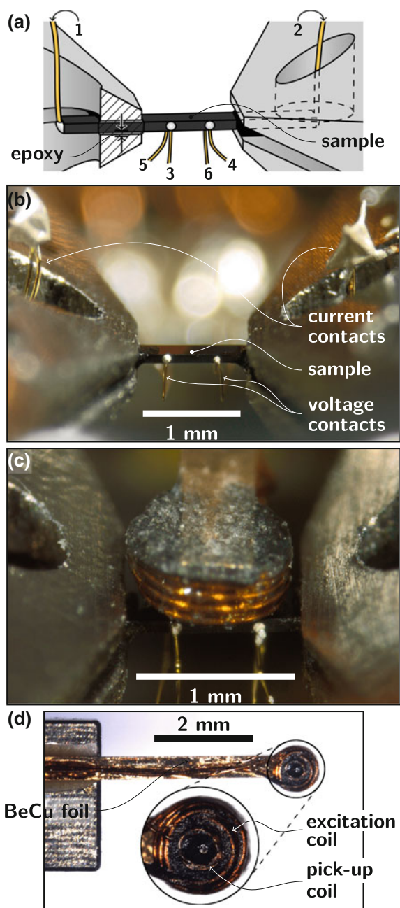
Fig. 3.22 Mounted Sample. a Mounting schematic showing the epoxy holding the sample between the sample plates and the numbering of electrical contacts. b Electrical resistivity setup for sample 3. c and d AC magnetic susceptibility setup. Concentric coils of diameter \sim 300 and \sim 600 \mu\text{m} are mounted on a flexible cantilever and positioned above the sample
