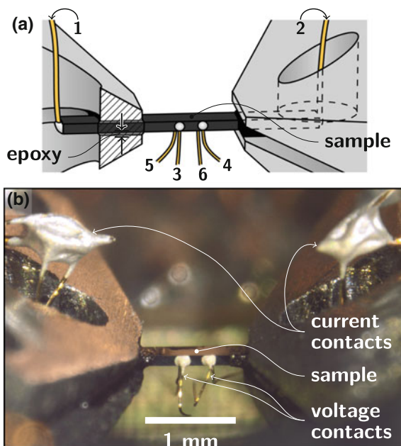
Fig. 4.19 Mounted Sample. a Mounting schematic showing the epoxy holding the sample between the sample plates. The schematic is the same as that given in Chap. 3 but it is included here because it defines the resistivity contact numbering. b Mounted sample showing the electrical resistivity setup. The gap between the two sample plates was set to 1.1 mm and the epoxy was 25 \mu\text{m} thick giving a strain transmission of \sim 70\%
