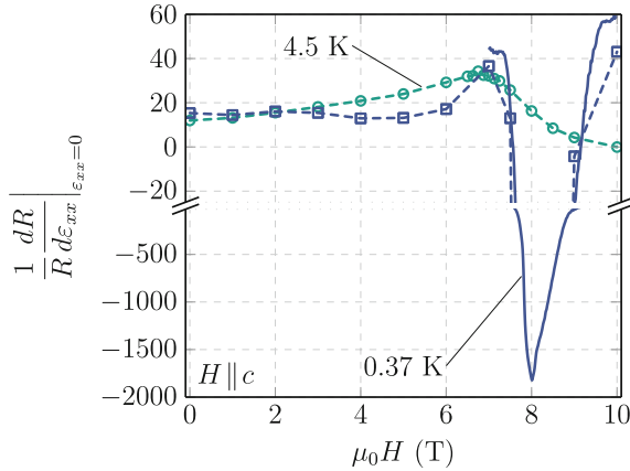
Fig. 4.33 Elastoresistance. Gauge factor against c -axis magnetic field at 4.5 K and 370 mK. The gauge factor is highly nonlinear with strain and is evaluated at zero strain from the derivative of the elastoresistance (1/R)dR/d\varepsilon_{xx}|_{\varepsilon_{xx}=0} . The circle and square points are calculated from short strain sweeps through zero strain at fixed field and temperature. The solid line is calculated by interpolating between different field sweeps at fixed strain and temperature but at fine enough strain spacing to accurately capture the slope at zero strain
