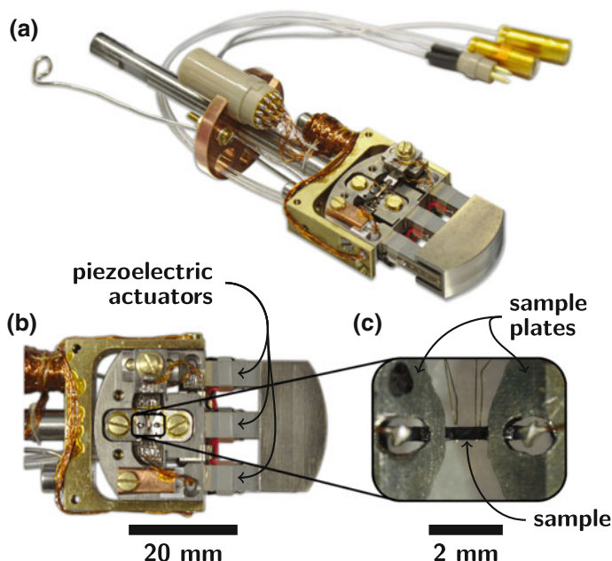
Fig. 2.13 Uniaxial stress cell. a Overview of the whole device including frame and wiring. b Detailed section of the main body of the device. c A typical sample mounted for electrical resistivity measurements
