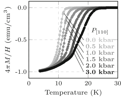
Fig. 2.5 \text{La}_{1.64}\text{Eu}_{0.2}\text{Sr}_{0.16}\text{CuO}_4 temperature dependence of magnetization under [110] uniaxial pressures. [110] oriented pressure destabilises stipe order relieving the competition with superconductivity and a strong T_c enhancement is seen. Based on original data from [26]
