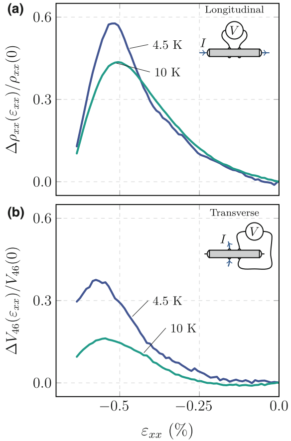
Fig. 3.34 Longitudinal and transverse resistivity against strain.
