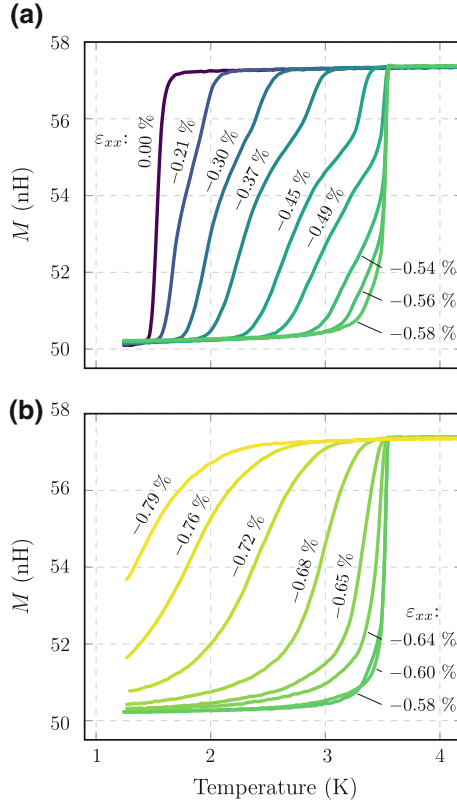
Fig. B.2 Susceptibility against temperature. Real part of the susceptibility \chi for sample 2 against temperature. a Strains below the peak T_c , b above the peak. No normalisation or offsets are applied to the curves. The y axis is the mutual inductance between the two coils of the susceptibility sensor
