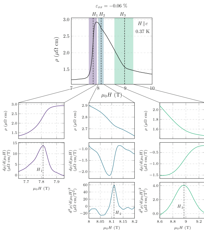
Fig. C.1 Phase boundaries from field ramps. A method for identifying the boundaries of the A and B phases from magnetoresistance measurements. H_1 , the entrance to the A phase, is identified with the maximum slope of the magnetoresistance, i.e. a peak in the first derivative as introduced by Grigera et al. [4]. Transitions H_2 and H_3 are identified by changes in slope of the magnetoresistance, i.e. a peak in the second derivative
