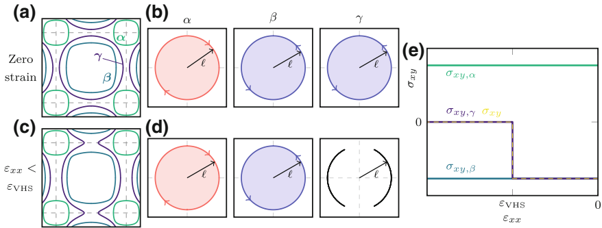
Fig. 3.40 Isotropic- \ell analysis of the Hall effect. Using the geometric interpretation of the Hall conductivity by Ong the area swept out by the scattering length \ell(\mathbf{k}) as \mathbf{k} is moved around the Fermi surface defines the Hall conductivity. Panel b shows this area for each of the three Fermi surfaces of \text{Sr}_2\text{RuO}_4 at zero strain in the isotropic- \ell approximation. The circulation of the \alpha band is in the opposite direction to the other two bands and adds to the overall conductivity with the opposite sign. Above the Lifshitz transition the \gamma band no longer contributes to the Hall conductivity and the Hall coefficient is expected to fall to zero
