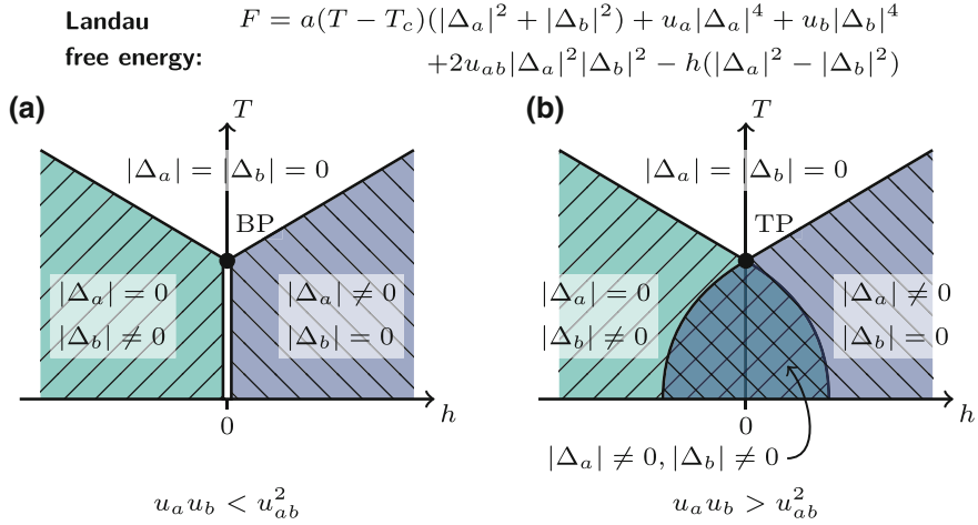
Fig. 4.38 Phase diagram of a two-component vector order parameter. The Landau free energy for a two-component order parameter, where each component is C_2 symmetric. The phase diagram of temperature ( T ) against h , a C_2 symmetric field, shows a a bicritical point (BP) when u_a u_b < u_{ab}^2 and b a tetracritical point (TP) when u_a u_b > u_{ab}^2 . The double line marks a first-order transition, all other transition lines are second-order.
