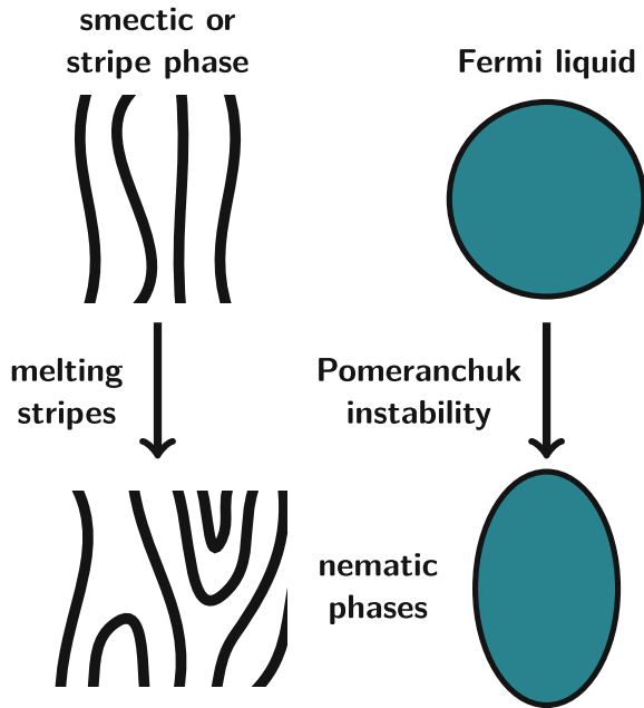
Fig. 4.15 Electron nematics. Two different mechanisms for producing electron nematic phases, see text for details.
