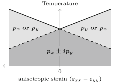
Fig. 2.10 Hypothesis for p_x \pm ip_y superconductivity. General phase diagram expected for p_x \pm ip_y superconductivity in a tetragonal crystal subject to a small, volume-preserving, but symmetry-breaking strain \varepsilon_{xx} - \varepsilon_{yy}
