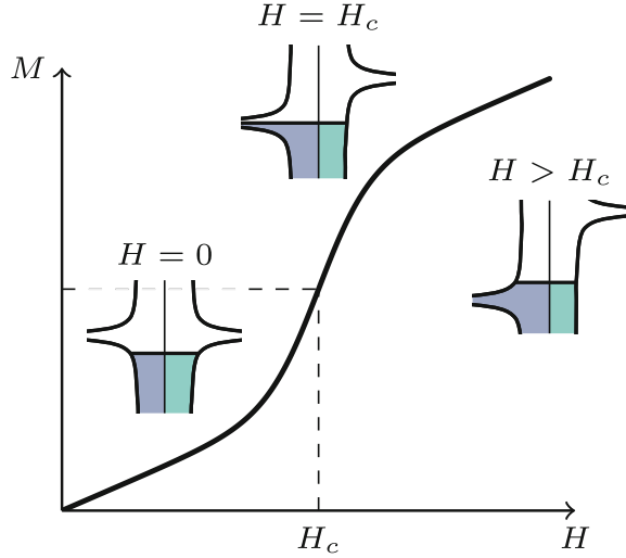
Fig. 4.5 Metamagnetism caused by a peak in the density of states.
