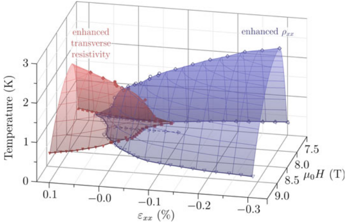
Fig. 4.37 Boundaries of enhanced \rho_{xx} and transverse resistivity. An empirical phase diagram for the bounding surfaces of enhanced longitudinal and transverse resistivity, in blue and red respectively, based on the resistivity and susceptibility measurements presented in Figs. 4.24, 4.28, 4.34 and 4.35. The symbols are the loci of peaks in susceptibility or maxima in derivatives of the resistivities with respect to temperature, field or strain as follows: \Delta d\rho/dH , \nabla d^2\rho/dH^2 , \square and \circ d^2\rho/d\varepsilon_{xx}^2 , \diamond d^2\rho/dT^2 and \triangleleft peaks in \chi' . Open symbols are from measurements of the longitudinal resistivity and closed symbols the transverse resistivity. The shaded surfaces are guides to the eye only. The region encloses both the A and B phases with the boundary between them H_2 drawn with \triangleright symbols only while it can be identified from the corresponding feature in d^2\rho/dH^2 . The solid lower bounding lines are H_1 and H_3
