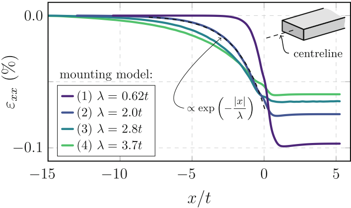
Fig. 2.19 Strain along the centreline of the sample. Strain \varepsilon_{xx} along the centreline of the sample for the mounting models in Fig. 2.17. The legend includes the load transfer lengths, \lambda , from fits to the portion of the sample inside the mounts. Negative x/t corresponds to where there is epoxy, the scale is the same as in Fig. 2.18
