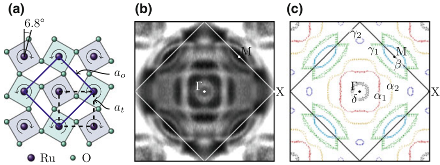
Fig. 4.2 Fermi surfaces of \text{Sr}_3\text{Ru}_2\text{O}_7 . a Cooperative rotation of the \text{RuO}_4 octahedra within the plane about the c -axis leads to a doubling of the unit cell and a \sqrt{2} \times \sqrt{2} reconstruction of the Fermi surfaces. b In-plane Fermi surface cross sections obtained in an ARPES study by Tamai et al. [25]. Data was taken in the first quadrant of the larger tetragonal Brillouin zone and the Fermi surface reconstruction can be clearly seen. c Fermi surface contours extracted from the ARPES data and the naming scheme used throughout this thesis
