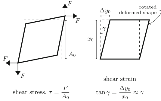
Shear stress and strain
