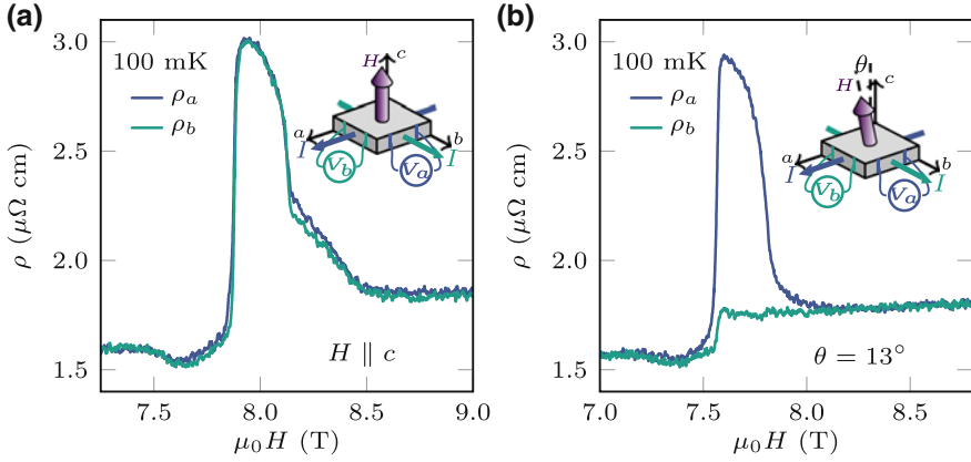
Fig. 4.14 Electron nematic transport. The two in-plane principle resistivity components, \rho_a and \rho_b , measured with different angles between the applied field and crystal axis. a For field applied along the c -axis there is almost no anisotropy. b With the field 13^\circ from the c -axis tilted towards a a pronounced anisotropy is seen. The easy direction for current is along b , and the hard direction along a . Tilting the field towards b rather than a reverses the hard and easy directions. Based on original data from [6]
