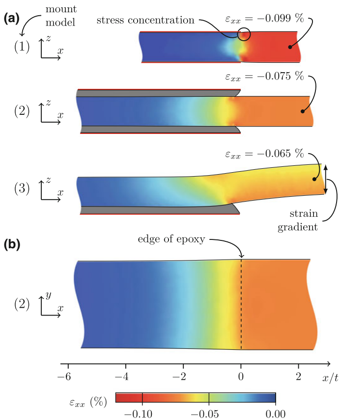
Fig. 2.18 FEA simulations. Strain \epsilon_{xx} for samples mounted as in the models of Fig. 2.17. In all the models the sample plates, represented by the thick red lines, were moved towards each other by 0.1% of L . The deformations have been exaggerated 200 times. a Cuts through the centre xz -plane of the sample. b Cut through the centre xy -plane of the sample for mounting model 2
