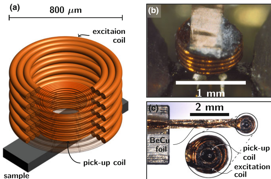
Fig. 4.21 Susceptibility Coils. a Model of the susceptibility coils used in the simulation. The excitation coil has 15 turns of 50\text{ }\mu\text{m} wire wound in three layers with diameters 550 , 650 and 750\text{ }\mu\text{m} . The pick-up coil fits within the excitation coil and consists of 50 turns of 15\text{ }\mu\text{m} wire in five layers with diameters from 315 to 435\text{ }\mu\text{m} . The pick-up coil rests on the surface of the sample which is 250\text{ }\mu\text{m} wide and 80\text{ }\mu\text{m} thick. b and c The actual susceptibility setup. The coils are mounted on a flexible cantilever so they can be easily positioned above the sample
