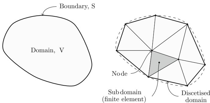
Fig. 2.2 Discretisation of a domain. The domain V is discretised by tessellating triangular elements
