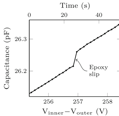
Fig. 2.16 Epoxy slippage. With the strain increasing steadily a jump in the capacitance is observed whenever the epoxy slips
