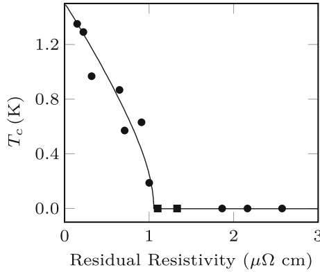
Fig. 3.8 Impurity effect on superconductivity in \text{Sr}_2\text{RuO}_4 . The superconducting transition temperature as function of residual resistivity for a variety of samples with different purity levels. The solid line is a fit of the Abrikosov-Gor'kov pair-breaking function to the data. Superconductivity is destroyed when the mean free path becomes similar to the superconducting coherence length. The extreme sensitivity of the superconductivity to non-magnetic impurities is expected only for unconventional pairing. Based on original data from [27]
