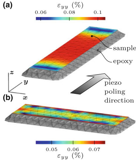
Fig. 2.9 Sample on piezo stack finite element simulations. Finite element simulations of the strain transmitted to samples mounted parallel and perpendicular to the poling direction of the piezo stack. Samples are 800 \times 200 \times 20 \mu\text{m} with a Young's modulus of 50 GPa and Poisson's ratio of 0.35. The epoxy is 20 \mu\text{m} thick and has a Young's modulus and Poisson's ratio of 10 GPa and 0.3, respectively. The stack is strained to +0.1\% and has a Poisson's ratio of 0.45. Deformations are exaggerated 200
