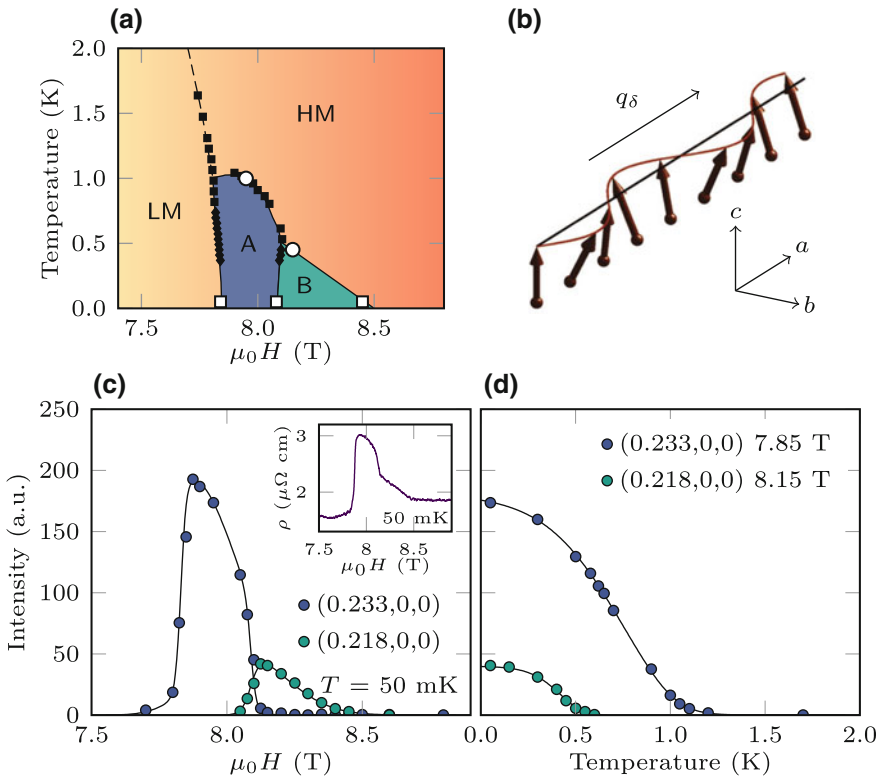
Fig. 4.16 Spin density wave ordering in \text{Sr}_3\text{Ru}_2\text{O}_7 . a Phase diagram determined from neutron scattering measurements. Open symbols are the boundaries determined from the scattering measurements whereas the solid symbols are from resistivity and susceptibility measurements. The two blue shaded regions mark the regions with SDWs of different wavevectors. b Proposed structure of the spin density wave within a single domain. c and d Magnetic field and temperature dependence of the SDW Bragg peak intensities. Adapted from [5]
