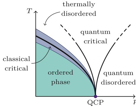
Fig. 4.9 Quantum critical point. Schematic phase diagram of a second-order phase transition giving rise to a quantum critical point. p is a non-thermal tuning parameter that suppress a second-order phase transition, thick black line, to absolute zero at the quantum critical point. At finite temperature and sufficiently close to the transition a classical critical region exists where the critical fluctuations are much lower in energy than the temperature and the thermal phase transition is universal. The effect of the quantum critical fluctuations, however, can be observed over a much larger region of phase space, see text for further details
