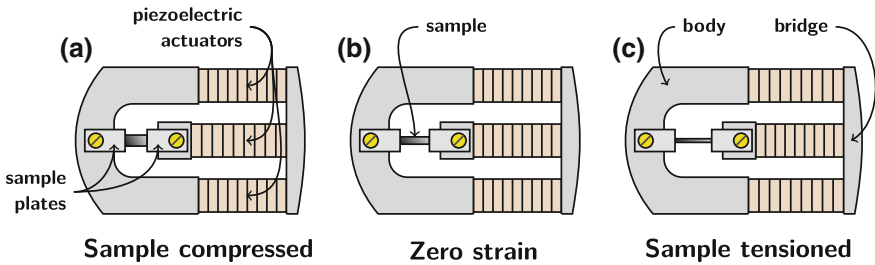
Fig. 2.11 Principle of operation. a The sample is compressed by extending the middle piezoelectric actuator. b Sample at zero strain. c The sample is tensioned by extending both outer actuators and pushing the bridge piece out
