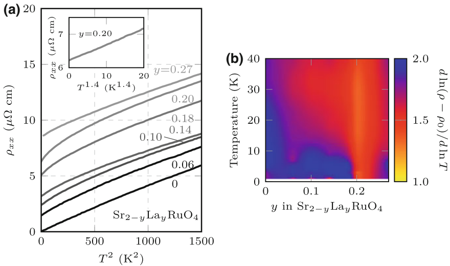
Fig. 3.18 Resistivity of \text{Sr}_{2-y}\text{La}_y\text{RuO}_4 . a In-plane resistivity against T^2 for y = 0 to 0.27 . The inset shows \rho versus T^{1.4} for y = 0.20 , the doping closest to the Van Hove singularity. b Resistivity temperature exponent, \alpha , for a nominal temperature dependence \rho = \rho_0 + AT^\alpha calculated from the logarithmic derivative of the resistivity. Based on original data from [4]
