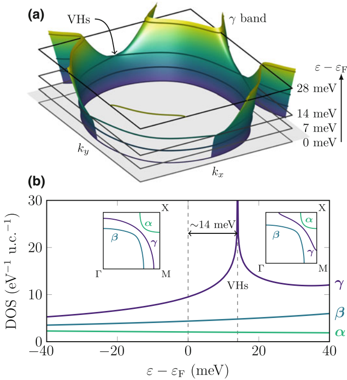
Fig. 3.16 Van Hove singularities in \text{Sr}_2\text{RuO}_4 . The \gamma band in \text{Sr}_2\text{RuO}_4 lies very close to a saddle point Van Hove singularity. a Tight binding model of the band structure at energies close to the Fermi level. The tight-binding parametrisation is from a fit to the experimentally determined band structure by Bergemann et al. [2] with the correct many-body renormalization from Shen et al. [5]. b With this tight-binding description the density of states peaks at \sim 14 meV above the Fermi energy where the \gamma band changes character from electron like to hole like
