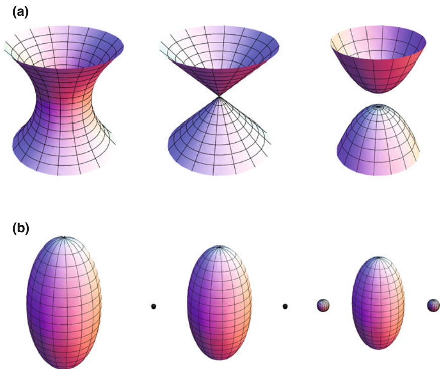
Fig. 3.17 Lifshitz transitions. a The collapse of a neck in a Fermi surface. b Appearance/disappearance of a new detached region of Fermi surface
