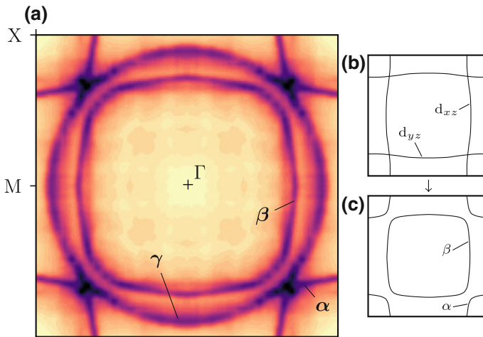
Fig. 3.2 Fermi surfaces of \text{Sr}_2\text{RuO}_4 . a In-plane Fermi surface cross sections obtained from an \varepsilon_F intensity map in an ARPES study by Damascelli et al. [10]. The first Brillouin zone is shown and the naming of the three surfaces \alpha , \beta and \gamma . b and c The d_{xz} and d_{yz} bands hybridise to form the \alpha and \beta surfaces
