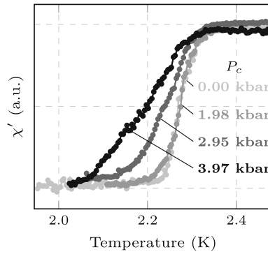
Fig. 2.6 Susceptibility against temperature for \text{CeCoIn}_5 under c -axis uniaxial pressure. The transition width \Delta T_c is strongly pressure dependent, whereas the onset temperature T_c is not. Based on original data from [27]
