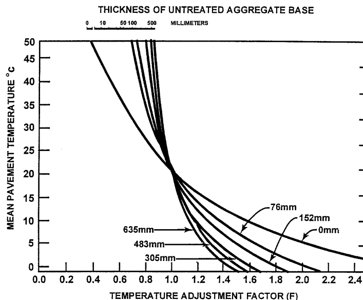
Figure 4.1 (from Ref. 15): Temperature Adjustment Factor for Benkelman Beam Deflections
