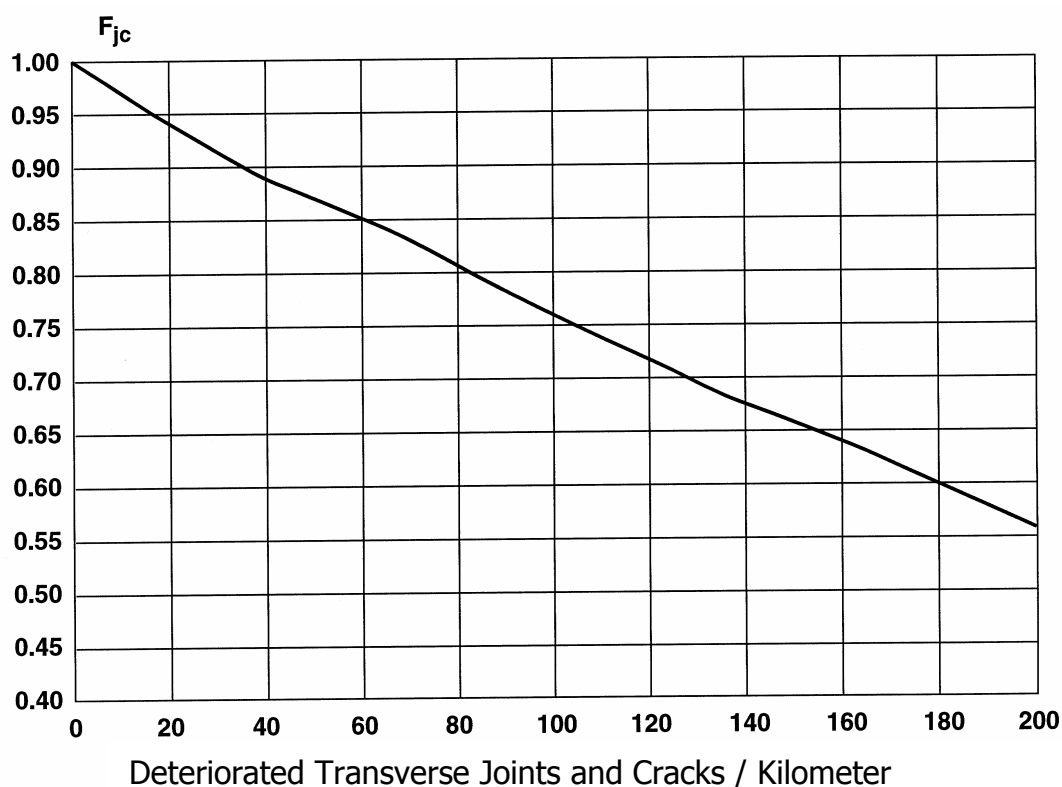
Figure 4.4 F_{jc} Adjustment Factor
