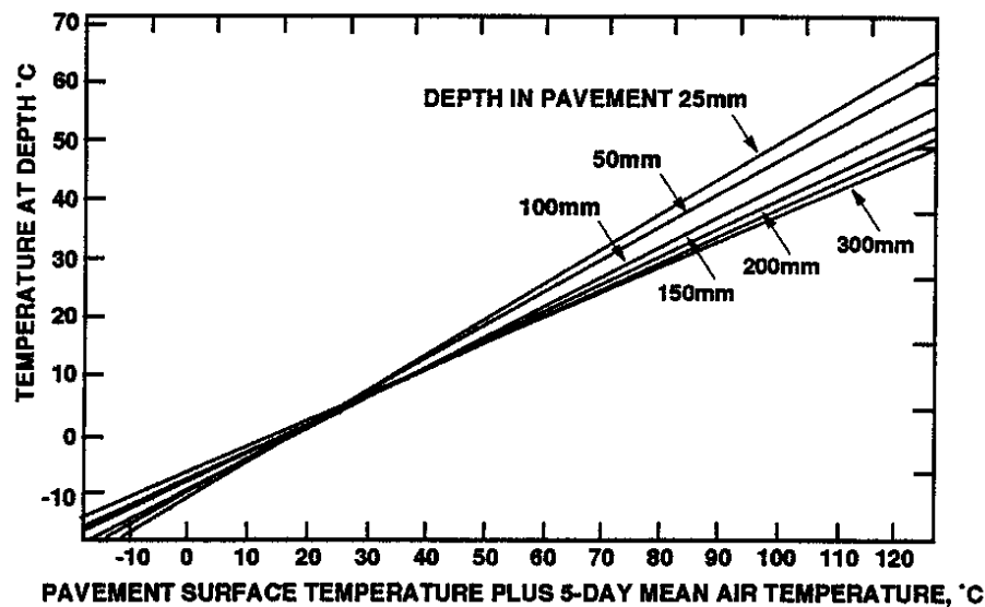
Figure D.1 Predicted Pavement Temperature
