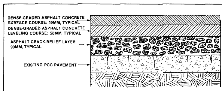
Figure 4.5 (from Ref.11) Crack-Relief Layer in an Overlay System, Cross-Section
