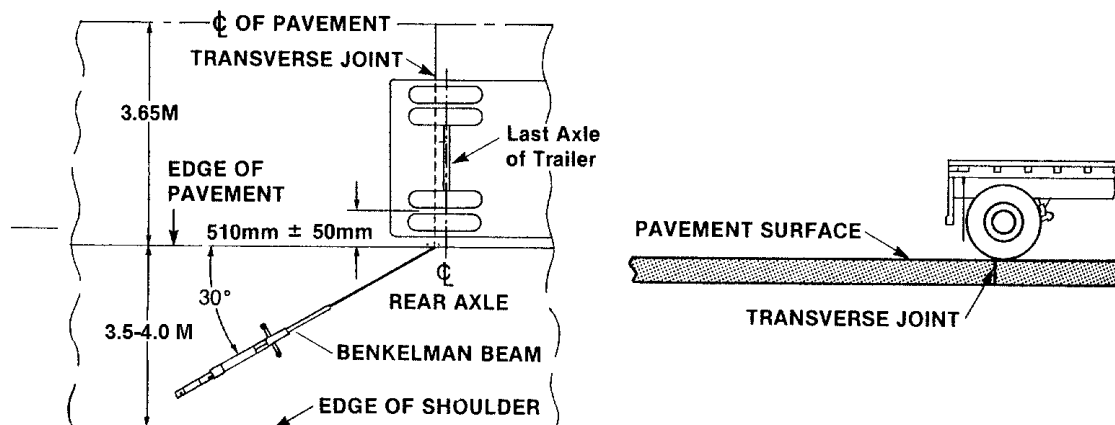
Figure B.4 (after Ref. 11) Position of vehicle and Benkelman Beam for making static rebound deflection measurements on rigid pavements.
