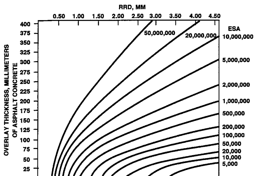
Figure 4.2 (from Ref. 15): Overlay Thickness Design Chart
