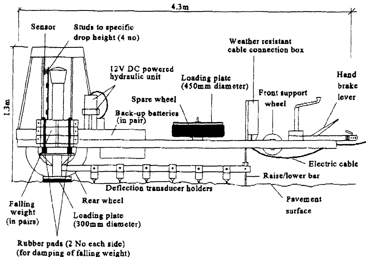
Figure B.5 Falling Weight Deflectometer
