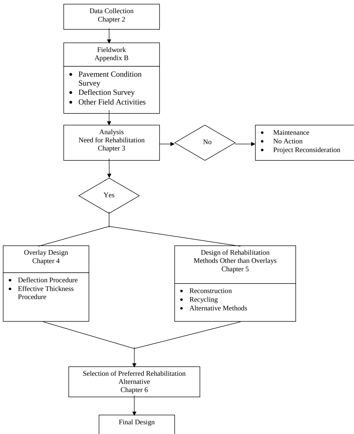
Figure 1.1 Rehabilitation Design Procedure and Organization of the Manual – Flow Diagram
