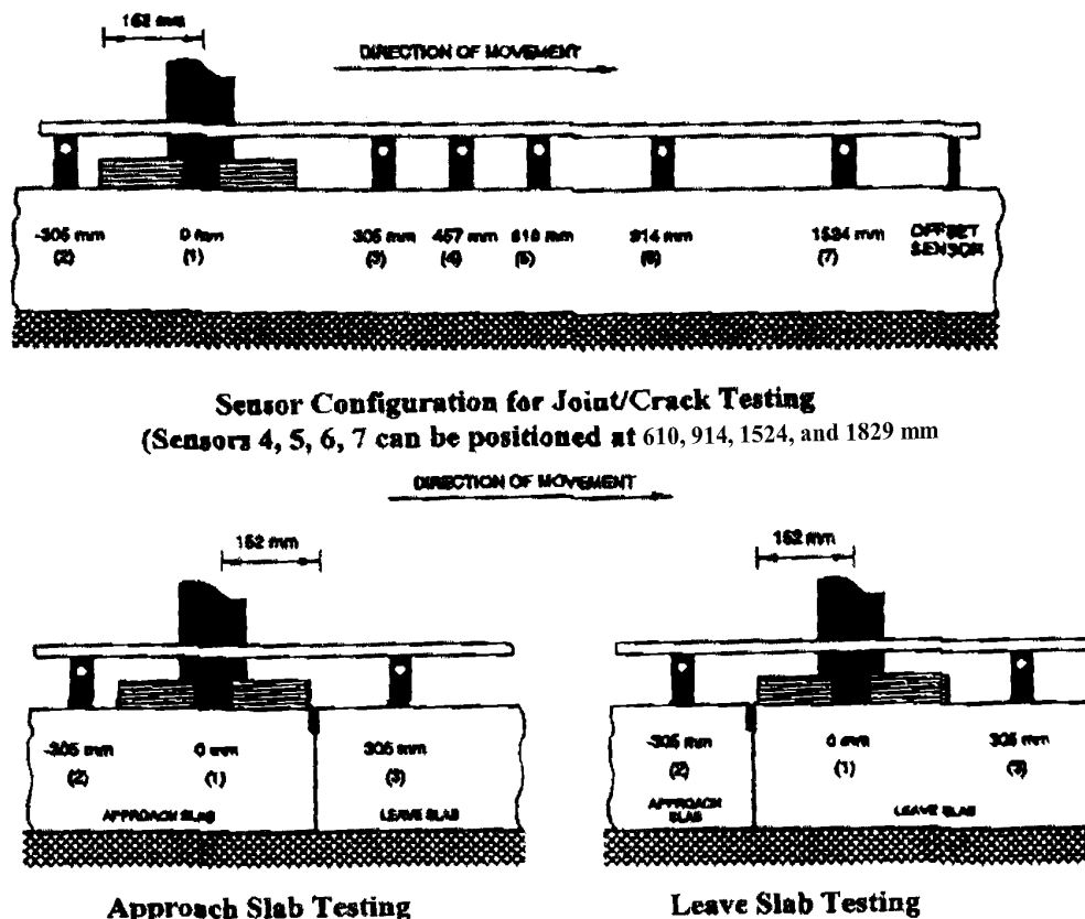
Figure B.8 Deflection Sensors Configuration (Rigid Pavements)
