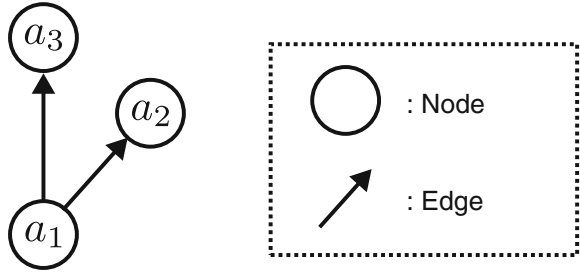
Fig. 5.1 An example of a directed graph
