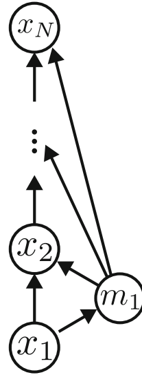
Fig. 5.3 Examples of causal networks. Example 1 Markov chain. Example 2 Feedback control with a single measurement
