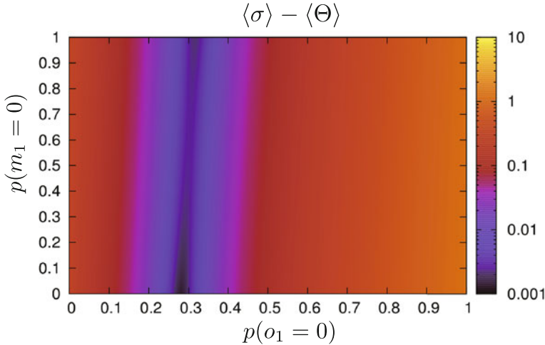
Fig. 6.11 Numerical illustration of the nonnegativity of \langle \sigma \rangle - \langle \Theta \rangle = -\langle \beta^O \Delta F^O \rangle + \langle \ln p(o_1, m_1, m_2) \rangle - \langle \ln p(o_2, m_1, m_2) \rangle . We here assume that o_1 and m_1 are independent, i.e., p(o_1, m_1) = p(o_1)p(m_1) . We set the parameters as follows: \Delta t = 0.5 , \beta^O = \beta^M = 0.01 , \tau^O = \tau^M = 0.001 , D_{01}^O = D_{01}^M = 100 , F_0^M(x_1 = 0) = F_0^M(x_1 = 1) = 100 , F_1^M(x_1 = 0) = 10 , F_1^M(x_1 = 1) = 30 , F_0^O(m_1 = 0, m_2 = 0) = F_0^O(m_1 = 1, m_2 = 0) = F_0^O(m_1 = 0, m_2 = 1) = F_0^O(m_1 = 1, m_2 = 1) = 100 , F_1^O(m_1 = 0, m_2 = 0) = 30 , F_1^O(m_1 = 1, m_2 = 0) = 10 , F_1^O(m_1 = 0, m_2 = 1) = 20 , and F_1^O(m_1 = 1, m_2 = 1) = 5
