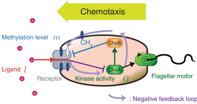
Fig. 7.2 Schematic of the E. coli bacterial chemotaxis
