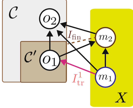
Fig. 6.9 The generalized second law in M on the causal network corresponding to the coupled chemical reaction model with a time-delayed feedback loop
