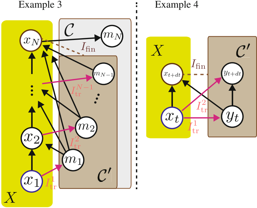
Fig. 6.5 Examples of the generalized second law on causal networks. Example 3 Repeated feedback control with multiple measurements. Example 4 Coupled Langevin equations
