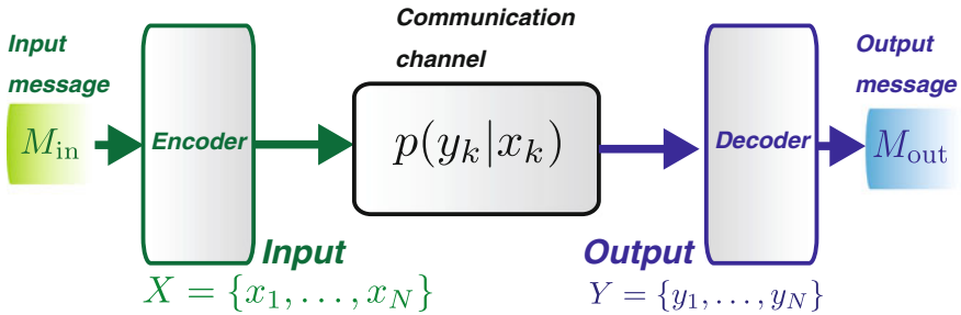
Fig. 2.2 Schematic of the communication system. To send an input message M_{\text{in}} through a noisy artificial communication channel, the input message should be encoded in a redundant sequence of bits by a channel coding protocol, and the encoded bits sequence X is transmitted through a noisy communication channel p(y_k|x_k) (e.g., a Gaussian channel). The output sequence Y does not necessary coincide with the input sequence X , because of the noise in the communication channel. However, if the redundancy N of the encoded bit sequence is sufficiently large, one can recover the original input message M_{\text{out}} = M_{\text{in}} correctly from the output sequence Y . This is a sketch of the channel coding
