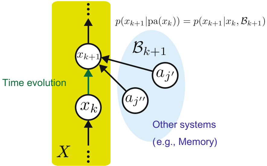
Fig. 6.1 A schematic of X and \mathcal{B}_{k+1} on causal networks. \mathcal{B}_{k+1} represents a set of random variables which can affects the time evolution in X from time k to k + 1
