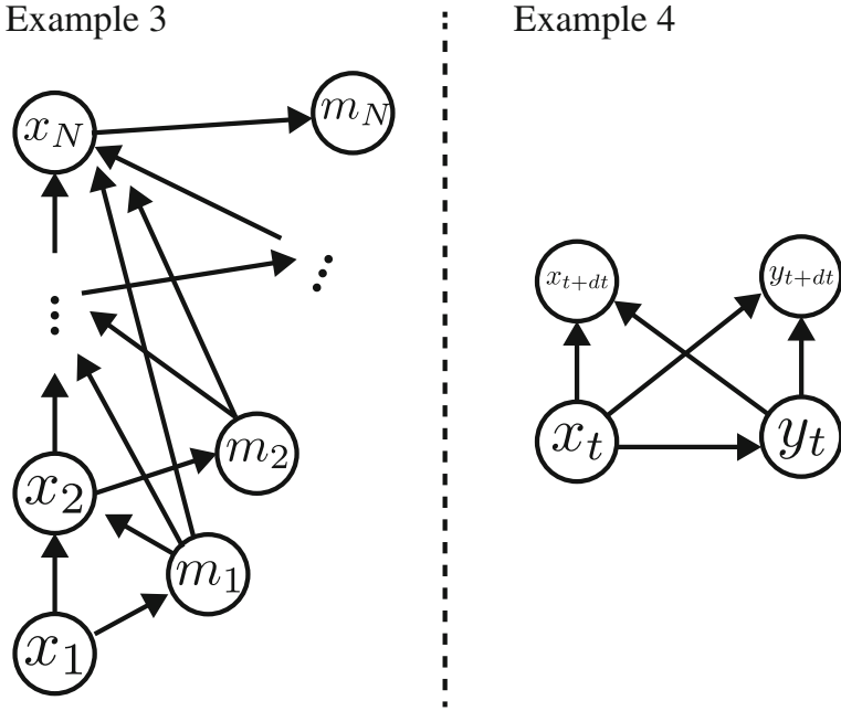
Fig. 5.4 Examples of causal networks. Example 3 Repeated feedback control with multiple measurements. Example 4 Coupled Langevin equations
