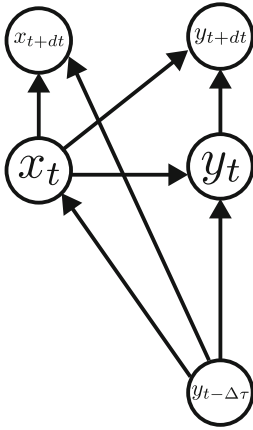
Fig. 5.5 Examples of causal networks. Example 5 Coupled dynamics with a time delay. Example 6 Complex dynamics
