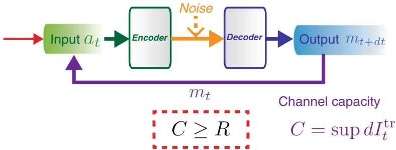
Fig. 7.8 Analogy and difference between our approach and Shannon's noisy channel coding theorem. a , Information thermodynamics for biochemical signal transduction. The robustness J_t^a is bounded by the information flow dI_t^{\text{tr}} in stationary states, which is a consequence of the second law of information thermodynamics. b , Information theory for artificial communication. The achievable information rate R , given by the redundancy of the channel coding, is bounded by the channel capacity C = \max dI_t^{\text{tr}} , which is a consequence of the Shannon's second theorem. If the noise is Gaussian as is the case for E. coli chemotaxis, both of the transfer entropy and the channel capacity are given by the power-to-noise ratio C = dI_t^{\text{tr}} = (2)^{-1} \ln(1 + dP_t/N_t) , under the condition that the initial distribution is Gaussian
