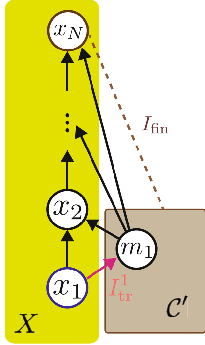
Fig. 6.4 Examples of the generalized second law on causal networks. Example 1 Markov chain. Example 2 Feedback control with a single measurement
