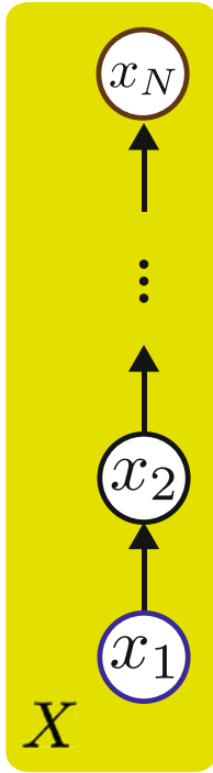
Fig. 6.4 Examples of the generalized second law on causal networks. Example 1 Markov chain. Example 2 Feedback control with a single measurement
