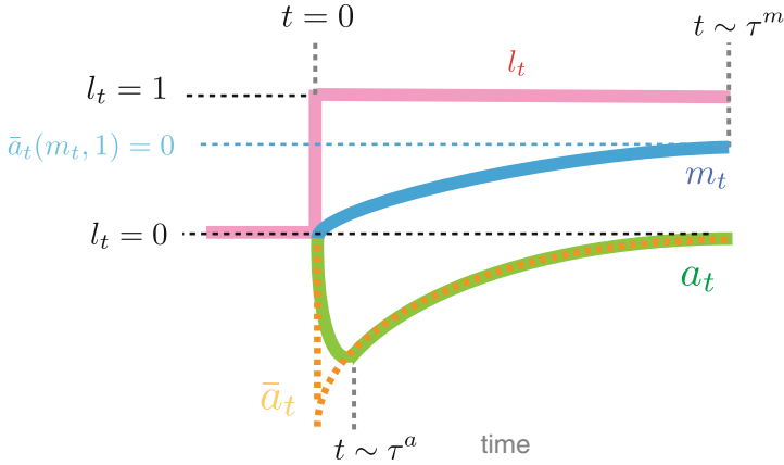
Fig. 7.4 Typical dynamics of adaptation with the ensemble average. Suppose that l_t changes as a step function (red solid line). Then, a_t suddenly responds (green solid line), followed by the gradual response of m_t (blue solid line). The adaptation is achieved by the relaxation of a_t to \bar{a}_t (orange dashed line). The methylation level m_t gradually changes to \bar{a}_t(m_t, 1) = 0 (blue dashed line)
