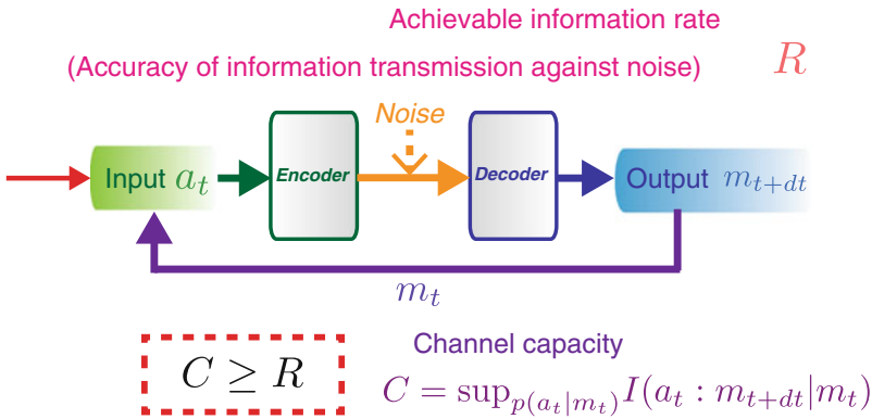
Fig. 7.3 The noisy channel coding theorem in a feedback loop. The transfer entropy I(a_t : m_{t+dt}|m_t) is related to the achievable information rate R in case of a feedback loop
