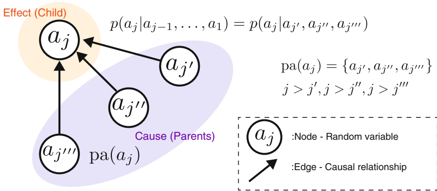
Fig. 5.2 A schematic of Bayesian network. The edge represents the causal relationship between random variables (i.e., nodes). The transition probability p(a_j|a_{j'}, a_{j''}, a_{j'''}) is given by the topology (edges) of the network
