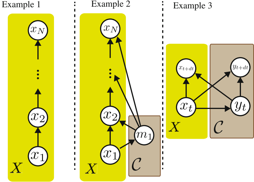
Fig. 6.2 Examples of X and C on causal networks. Example 1 Markov chain. Example 2 Feedback control with a single measurement. Example 3 Coupled Langevin equations.
