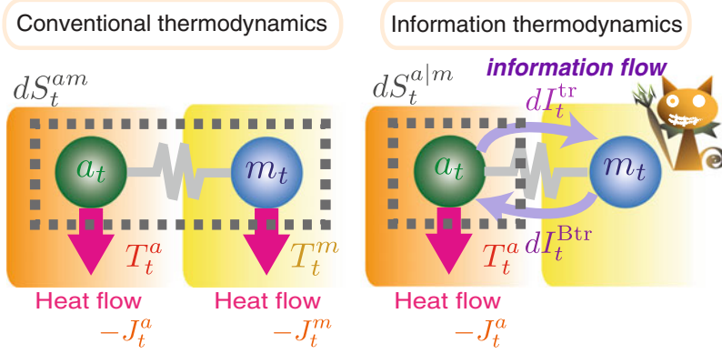
Fig. 7.6 Information thermodynamics and conventional thermodynamics. The second law of information thermodynamics characterizes the entropy change in a subsystem in terms of the information flow between the subsystem and the outside world (i.e., dI_t^{tr} + dS_t^{a|m} \geq dI_t^{tr} - dI_t^{Btr} + dS_t^{a|m} \geq -J_t^a dt/T_t^a ). In contrast, the conventional second law of thermodynamics states that the entropy change in a subsystem is compensated for by the entropy change in the outside world (i.e., -J_t^m dt/T_t^m + dS_t^{am} \geq J_t^a dt/T_t^a ).
