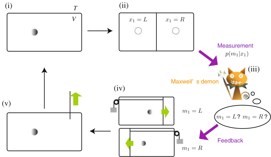
Fig. 4.1 The schematic of the Szilard's engine. Maxwell's demon measure a state of the position of a single particle x_1 , and performs feedback control using the measurement outcome m_1 . In a cycle, Maxwell's demon can extract the work from the heat bath attached to the box. That fact is the apparent violation of the second law of thermodynamics
