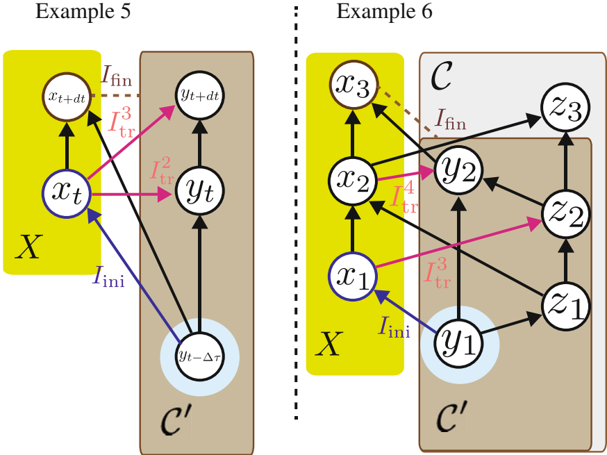
Fig. 6.6 Examples of the generalized second law on causal networks. Example 5 Coupled dynamics with a time delay. Example 6 Complex dynamics
