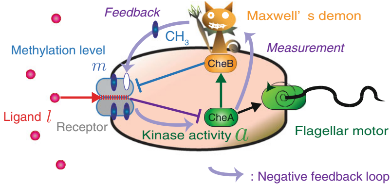
Fig. 7.5 Maxwell's demon in E. coli chemotaxis. From the viewpoint of thermodynamics, the methylation level m plays a similar role to the memory of Maxwell's demon, which reduces the effect of the environmental noise on the kinase activity
