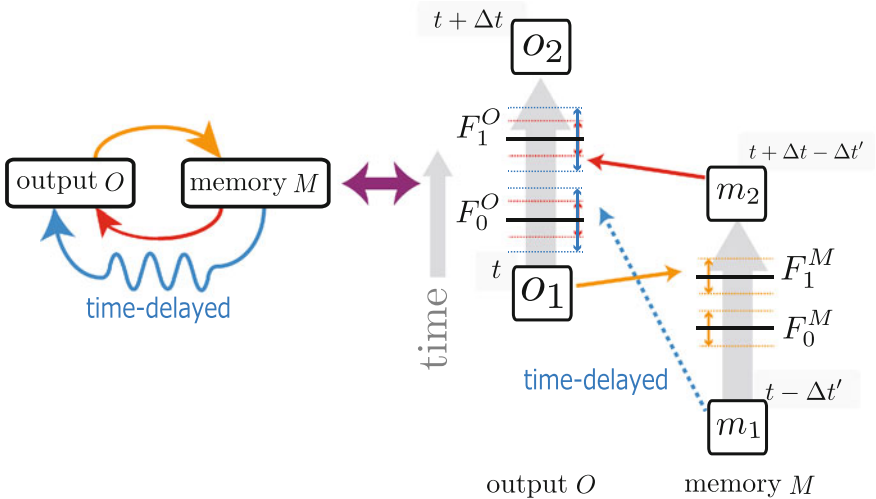
Fig. 6.7 Schematic of the coupled chemical reaction model with a time-delayed feedback loop. The previous states of O and M determine the effective free energy landscapes F^O or F^M . A blue directed arrow indicates the effect of time-delayed feedback loop. This time-delayed effect is introduced by m_1 -dependence of F^O
