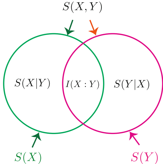
Fig. 2.1 The Venn's diagram which represents the nature of the mutual information (i.e., Eq. 2.17). The mutual information between X and Y represents the correlation between them in the sense of the Shannon entropy
