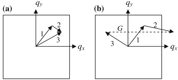
Fig. 3.8 Representation in two dimensions of a N-processes and b U-processes
