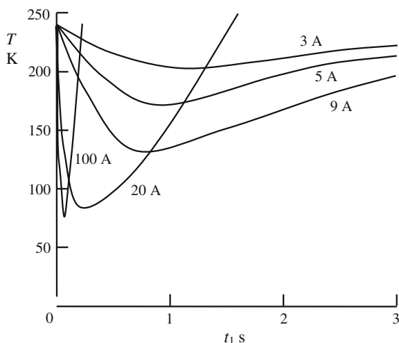
Fig. 10.10 Plot of cold junction temperature against pulse length for different values of the pulse current. The pulses are superimposed on a steady current of 5 A. Data obtained for a bismuth telluride couple by Landecker and Finlay [26]
