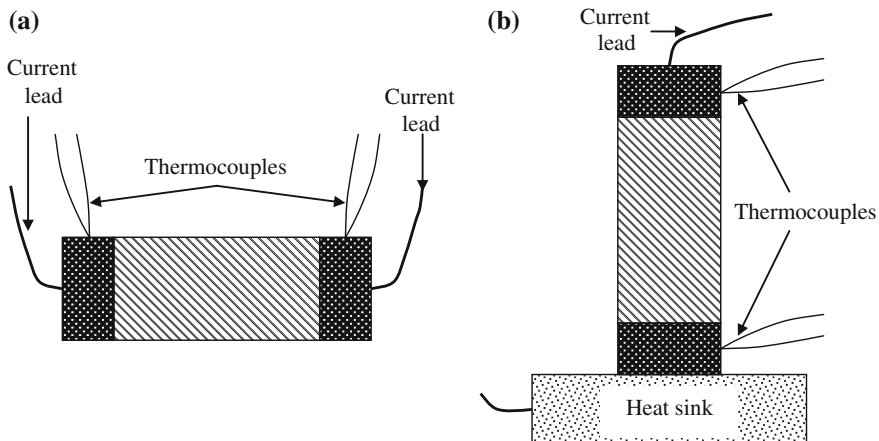
Fig. 8.13 Experimental arrangements for the direct measurement of the figure of merit. In a the sample is suspended in vacuum and in b one end of the sample is attached to a heat sink
