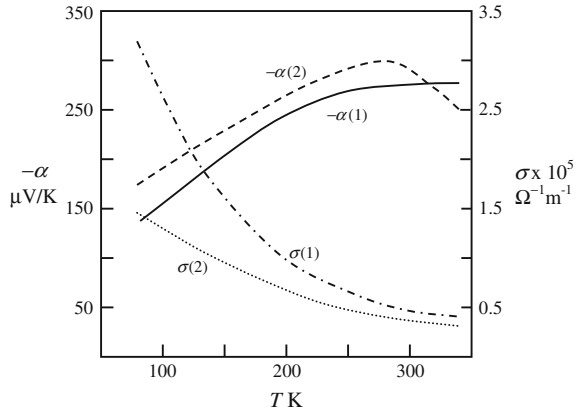
Fig. 6.9 Seebeck coefficient and electrical conductivity plotted against temperature for n-type alloys of bismuth telluride. A schematic plot based on the data of Kutasov et al. [35]. Sample 1 is suitable for use at ordinary temperatures while Sample 2 is a low temperature material
