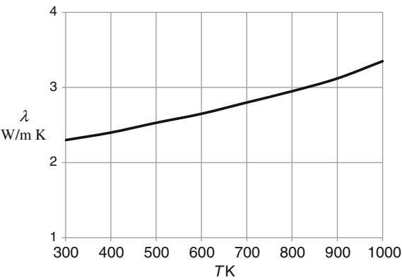
Fig. 9.31 The temperature dependence of the thermal conductivity of complex-doped HMS (based on the data of Fedorov and Zaitsev)
