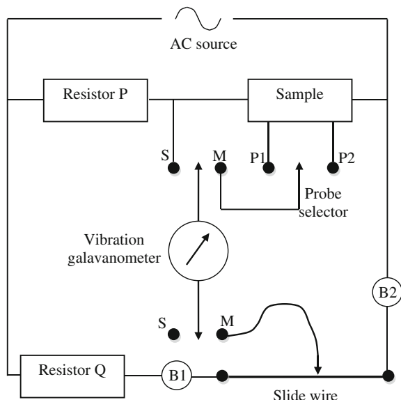
Fig. 8.2 Alternating current bridge for measurement of electrical conductivity of thermoelectric materials. B1 and B2 are the balancing resistors
