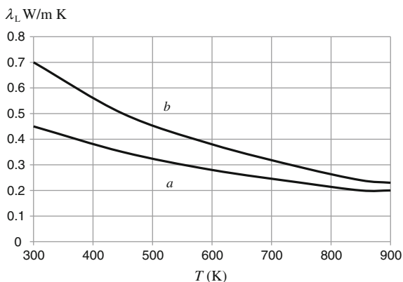
Fig. 9.15 Lattice conductivity plotted against temperature for SnSe in the b - and a -directions. Based on the data of Zhao et al. [40]
