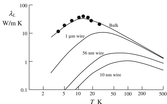
Fig. 12.7 Schematic plot of lattice conductivity against temperature for PbTe. The experimental points indicated by the dots are based on the data of Greig [16] for a bulk crystal and the curves represent the theoretical calculations of Dames and Chen [12]
