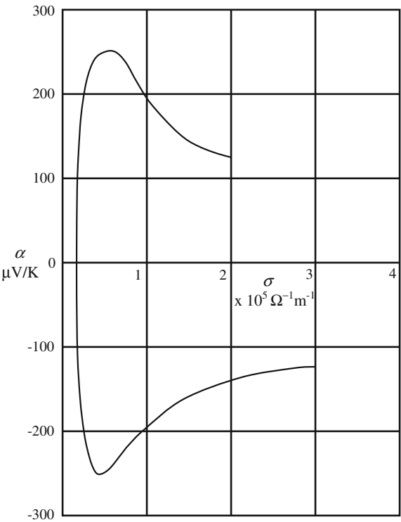
Fig. 6.1 Seebeck coefficient plotted against electrical conductivity for p-type and n-type bismuth telluride at 300 K
