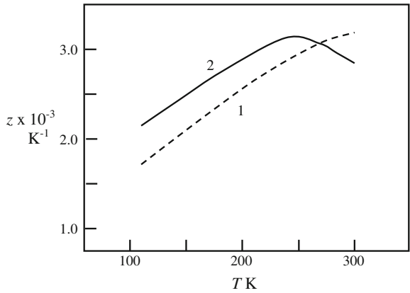
Fig. 6.10 Figure of merit plotted against temperature for two bismuth telluride alloys. Samples 1 and 2 are similar to those in Fig. 6.9. A schematic plot based on the data of Vedernikov et al. [38]
