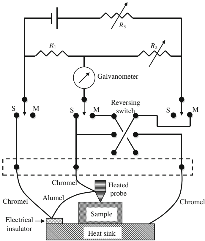
Fig. 8.7 Measurement of the Seebeck coefficient using the technique devised by Cowles and Dauncey [6]. The chromel wires are connected to copper wires in an enclosure at a constant temperature
