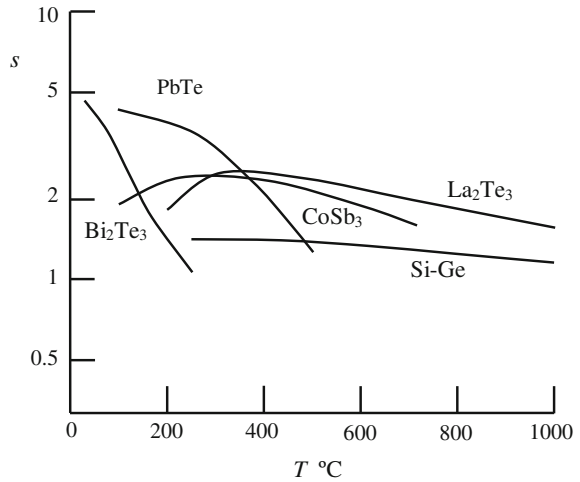
Fig. 10.15 Compatibility factor of n-type generator materials. Schematic plot based on data of Snyder [42]
