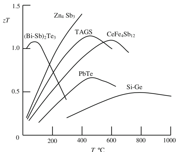
Fig. 10.12 Dimensionless figure of merit of p-type generator materials. Schematic plot based on data of Snyder [42]
