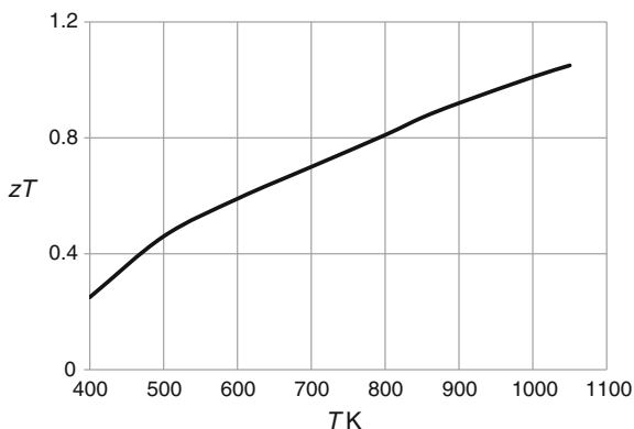
Fig. 9.28 Plot of zT against temperature for optimised \text{Mg}_2\text{Si}_{0.7}\text{Sn}_{0.3} . This is a theoretical plot based on assumption (3) (see text). Optimisation of the Seebeck coefficient is most evident at the highest temperatures
