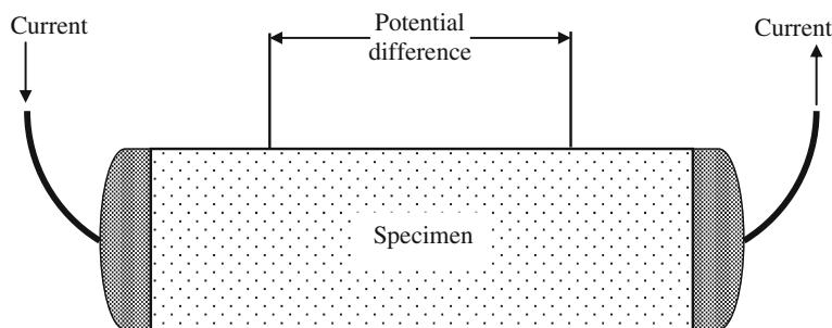
Fig. 8.1 Arrangement of sample with inset probes for measurement of the electrical conductivity
