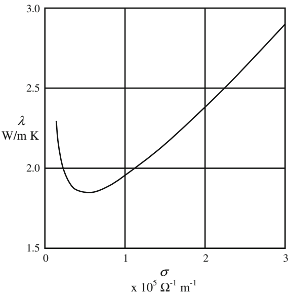
Fig. 6.2 Plot of thermal conductivity against electrical conductivity for bismuth telluride at 300
