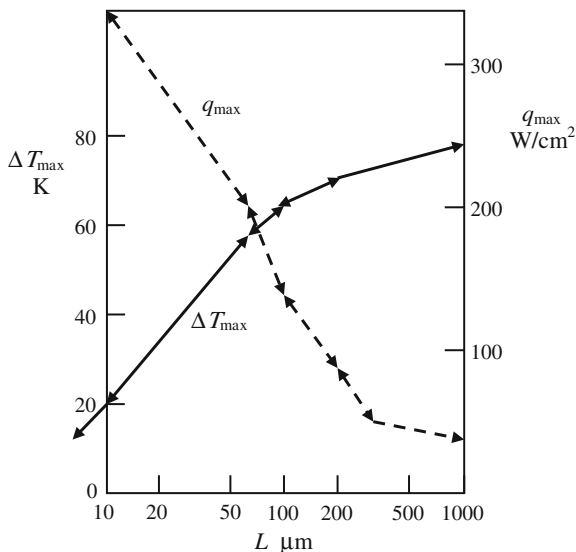
Fig. 10.8 Maximum temperature difference and maximum cooling power plotted against the length of the thermoelements. This is a representation of Semenyuk's data on thermoelectric modules for cooling optoelectronic components
