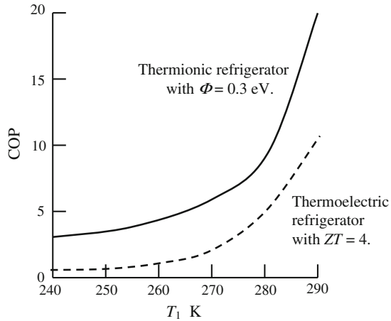
Fig. 13.7 Coefficient of performance plotted against source temperature for thermionic and thermoelectric refrigerators. The heat sink is at 300 K
