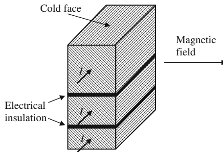
Fig. 2.10 3-stage Ettinghausen cooler. The same current, I , passes through each stage but the stages are of different thickness
