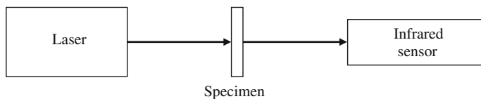
Fig. 8.12 Essential features of the laser flash method for determining the thermal diffusivity
