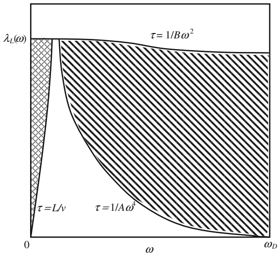
Fig. 5.4 Contribution to the lattice conductivity of phonons of angular frequency \omega plotted against \omega . The upper curve is applicable when only phonon–phonon scattering occurs. The single-hatched region on the right indicates the contribution removed by point-defect scattering. The double-hatched region on the left shows the contribution removed by boundary scattering
