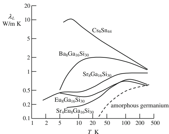
Fig. 9.21 Lattice conductivity plotted against temperature for selected Type I clathrates. A schematic plot based on the data of Cohn et al. [72]
