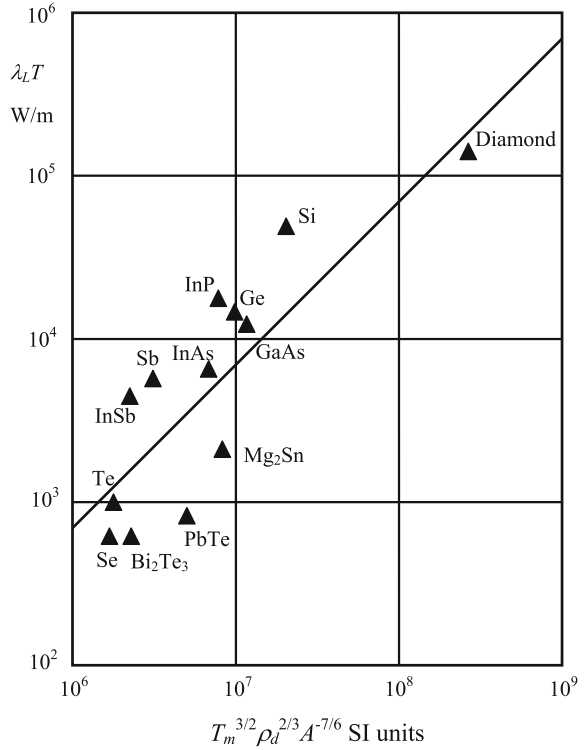
Fig. 4.4 Plot of \lambda_L T against T_m^{3/2} \rho_d^{2/3} A^{-7/6} for a number of semiconductors. The line represents (4.12) with the parameter B_K = 6 \times 10^{-4} SI units
