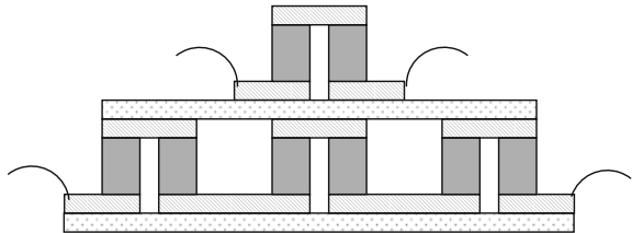
Fig. 2.7 Schematic arrangement of a 2-stage thermoelectric cascade. The stages are electrically insulated from one another but in good thermal contact
