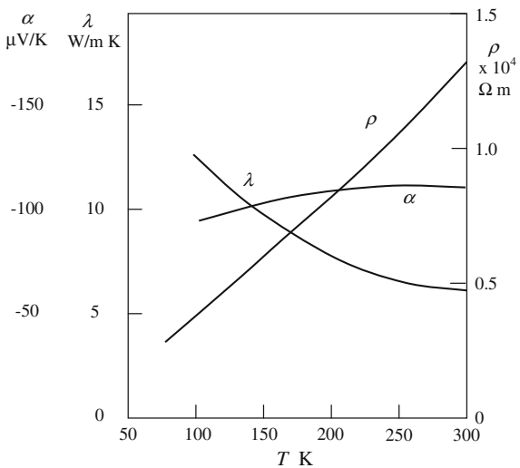
Fig. 9.3 Thermoelectric properties of bismuth parallel to the trigonal axis
