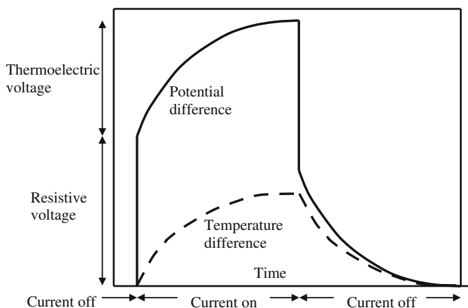
Fig. 8.14 Schematic variation of potential and temperature differences with time when the current is switched on and off in a Harman-type measurement
