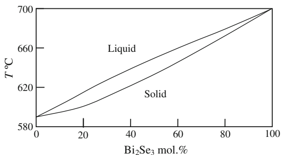
Fig. 7.7 Schematic phase diagram for the \text{Bi}_2\text{Te}_3\text{--Bi}_2\text{Se}_3 alloy system
