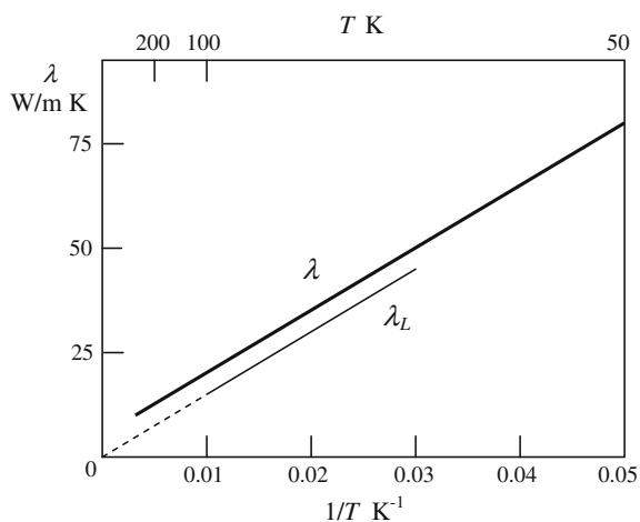
Fig. 9.5 Total and lattice thermal conductivity of bismuth plotted against the reciprocal of the absolute temperature
