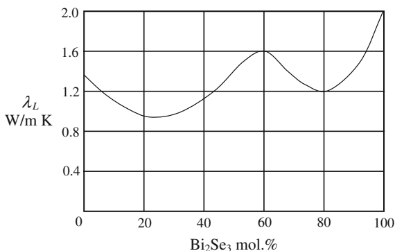
Fig. 6.7 Lattice thermal conductivity at 300 K plotted against concentration of \text{Bi}_2\text{Se}_3 in (\text{Bi-Sb})_2\text{Te}_3 solid solutions (based on the data of Rosi et al. [23])
