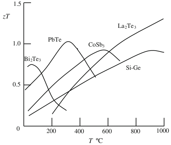
Fig. 10.14 Dimensionless figure of merit of n-type generator materials. Schematic plot based on data of Snyder [42]
