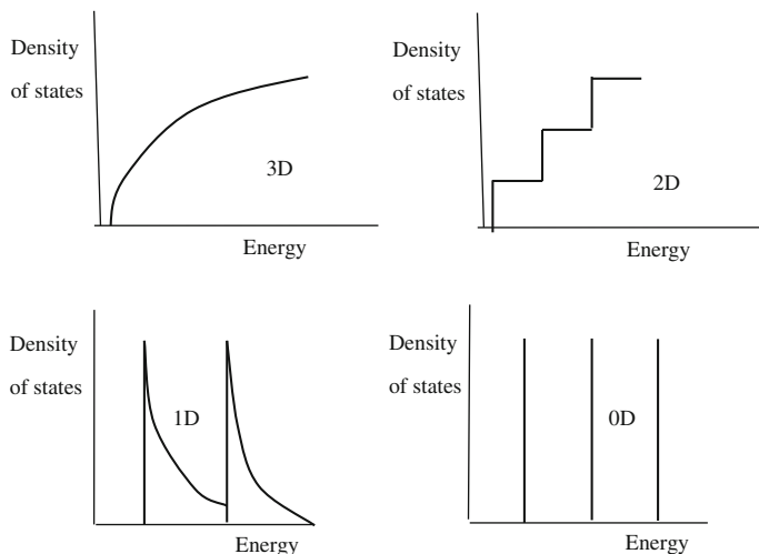
Fig. 12.4 Schematic diagrams for the density of states as a function of energy in bulk (3D), 2D, nanowires (1D) and quantum dot (0D) configurations. Based on the review by Dresselhaus and Heremans [4]
