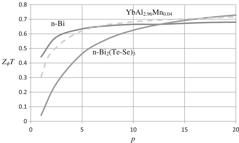
Fig. 11.5 Plot of optimum dimensionless transverse figure of merit against the porosity factor of the positive component (\text{Bi-Sb})_2\text{Te}_3 . For the solid curves , the negative component is either \text{Bi}_2(\text{Te-Se})_3 or Bi. For the broken curve , the negative component is \text{YbAl}_{2.96}\text{Mn}_{0.04}
