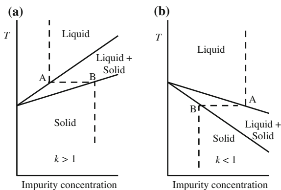
Fig. 7.1 Equilibrium phase diagrams showing the liquidus and solidus lines for different values of the segregation coefficient k . a k > 1 and b k < 1
