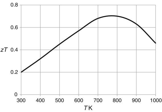
Fig. 9.32 The dimensionless figure of merit of complex-doped HMS
