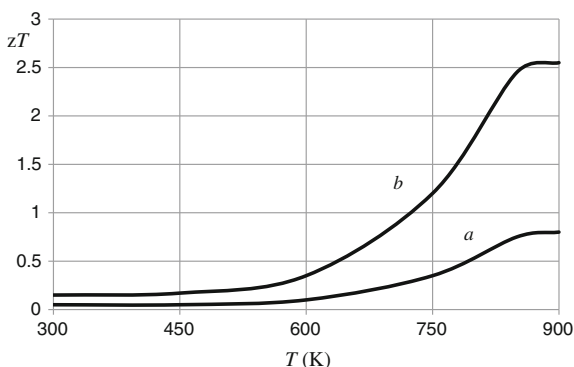
Fig. 9.14 zT plotted against temperature for SnSe for transport along the b and a axes. Based on the data of Zhao et al. [40]
