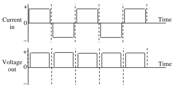
Fig. 8.3 Measurement of electrical conductivity of a sample of thermoelectric material using a DC potentiometer and a mechanical chopper
