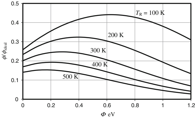
Fig. 13.8 Ratio of coefficient of performance to its value for a Carnot cycle plotted against barrier height. The parameter T_R represents the losses and is proportional to the square root of the thermal conductance of the barrier
