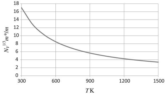
Fig. 5.7 The requirement for improvement in the figure of merit on the transition from the crystalline to the amorphous state. An improvement is likely if the parameter N_V^{1/3}m^*/m lies above the curve
