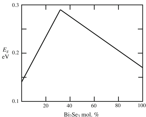
Fig. 6.12 Variation of energy gap with concentration of \text{Bi}_2\text{Se}_3 in \text{Bi}_2(\text{Te}-\text{Se})_3 alloys based on the observations of Greenaway and Harbeke [17]
