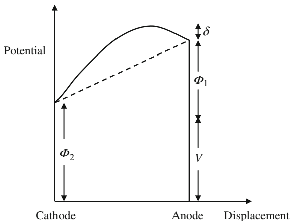
Fig. 13.1 Schematic plot showing potential as a function of displacement in a thermionic diode
