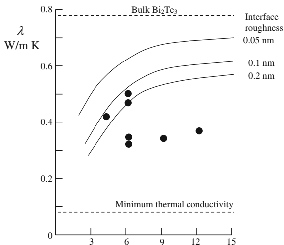
Fig. 12.5 Thermal conductivity of a \text{Bi}_2\text{Te}_3/\text{Sb}_2\text{Te}_3 superlattice plotted against the superlattice period. Schematic diagram based on the data of Touzelbaev et al. [9]. The three curves represent calculated values using the Boltzmann equation for different degrees of roughness at the interfaces. The broken lines show the thermal conductivities of bulk bismuth telluride and the minimum value predicted by Cahill's theory [10]. The dots are the experimental data
