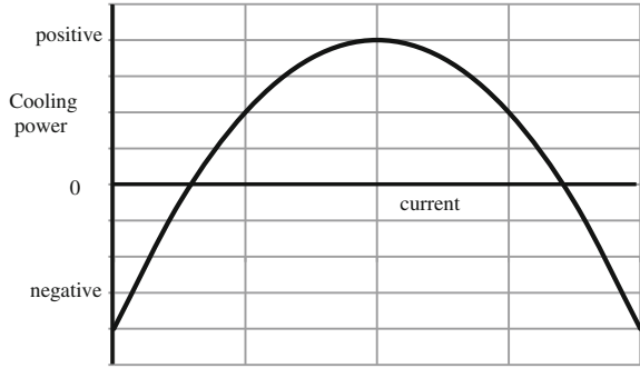
Fig. 2.2 Schematic plot of cooling power against current for a thermoelectric cooler. The cooling power is negative until the Peltier effect is great enough to counteract both heat conduction and Joule heating
