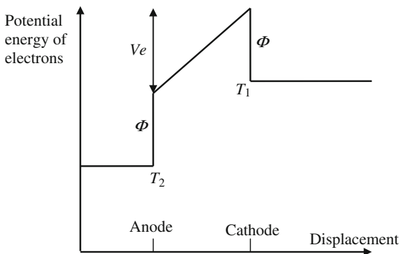
Fig. 13.2 Schematic plot of the potential energy of the electrons against displacement in a thermionic diode with \Phi_1 = \Phi_2
