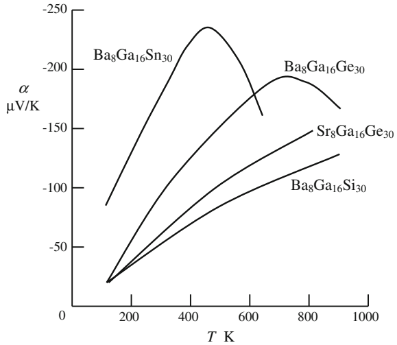
Fig. 9.22 Seebeck coefficient plotted against temperature for some Type I clathrates. Schematic representation of the data of Kuznetsov et al. [74]
