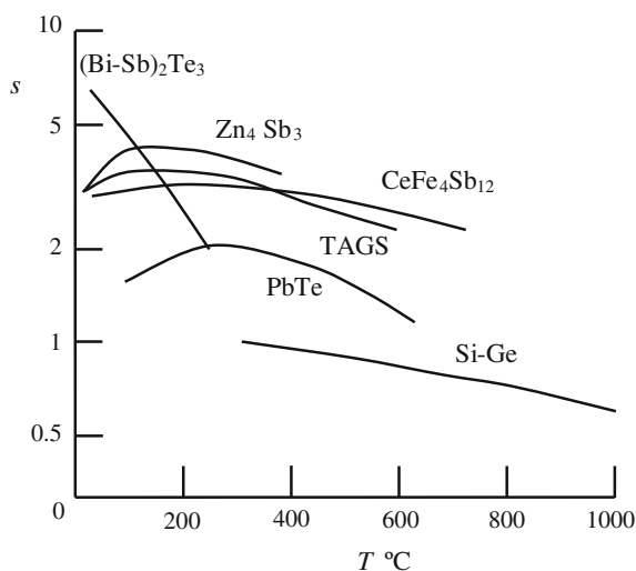
Fig. 10.13 Compatibility factor of p-type generator materials. Schematic plot based on data of Snyder [42]
