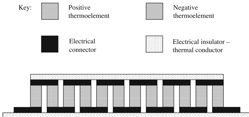
Fig. 10.1 Schematic diagram of a thermoelectric module
