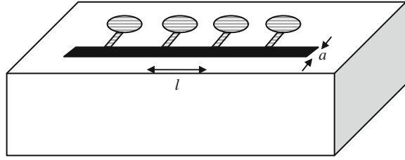
Fig. 8.11 Arrangement of the metal strip and side arms on the sample in the 3\omega method
