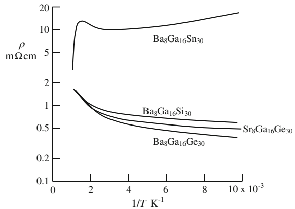
Fig. 9.23 Electrical resistivity plotted against inverse temperature for some Type I clathrates. Schematic representation of the data of Kuznetsov et al. [74]
