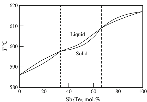
Fig. 7.6 Schematic phase diagram for the \text{Bi}_2\text{Te}_3 – \text{Sb}_2\text{Te}_3 alloy system. The meeting of the liquidus and solidus curves at \text{Sb}_2\text{Te}_3 concentrations of one-third and two-thirds suggests that there may be some measure of ordering at these compositions
