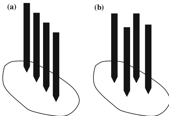
Fig. 8.5 4-point probe configurations; a probes regularly spaced in line and b probes at the corners of a square. The probes are usually spring-loaded and pressed against the plane surface of a semiconductor
