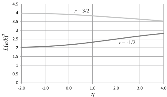
Fig. 3.6 Plot of Lorenz number in units of (k/e)^2 against reduced Fermi energy
