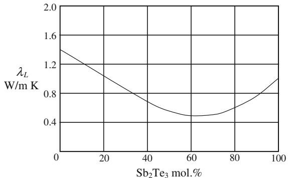
Fig. 6.6 Lattice thermal conductivity at 300 K plotted against concentration of \text{Sb}_2\text{Te}_3 in (\text{Bi-Sb})_2\text{Te}_3 solid solutions (based on the data of Rosi et al. [23])
