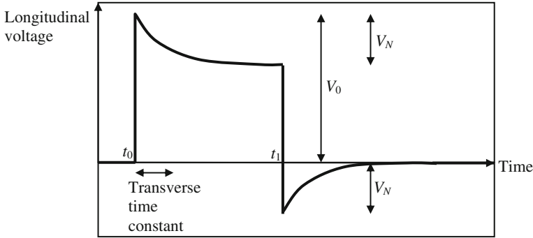
Fig. 8.17 Schematic plot of longitudinal voltage against time in the measurement of the thermomagnetic figure of merit using the technique of Guthrie and Palmer [31]
