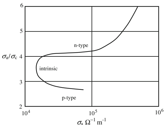
Fig. 6.3 Ratio of electrical conductivity in the a -direction to that in the c -direction plotted against \sigma_a for single crystal bismuth telluride at 300 K
