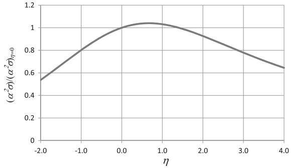
Fig. 4.1 Plot of power factor against reduced Fermi energy for r = -1/2
