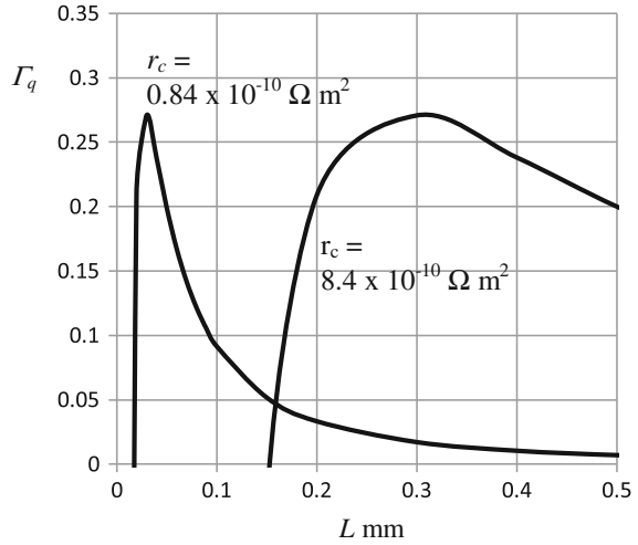
Fig. 10.6 Plot of Parrott and Penn's function \Gamma_q against length of thermoelements for a contact resistance r_c equal to 0.84 \times 10^{-10} \Omega \text{ m}^2 and 8.4 \times 10^{-10} \Omega \text{ m}^2 . ZT = 1 and \Delta T/T = 1/15
