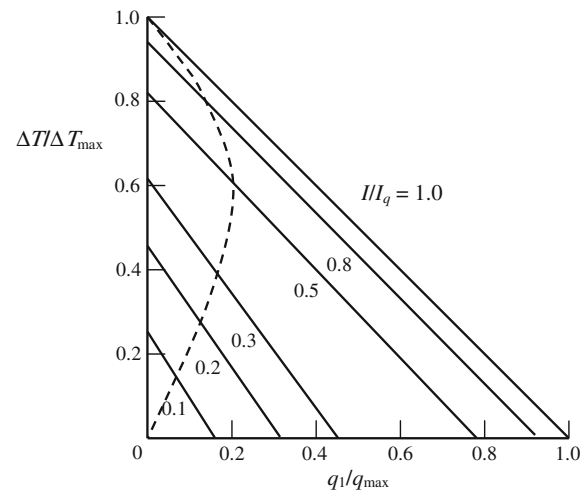
Fig. 10.3 Plots of \Delta T/\Delta T_{\max} against ratio of cooling power to maximum cooling power for modules in Table 10.1. Each solid line represents a different ratio of the current to the current for maximum cooling power. The broken curve corresponds to the conditions for optimum coefficient of performance
