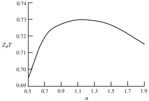
Fig. 11.7 Dimensionless transverse figure of merit plotted against ratio of layer thicknesses for a (Bi–Sb) 2 Te 3 –Bi 2 (Te–Se) 3 composite. The porosity factor for the p-type component is 20 and the angle of orientation of the layers is 18.4°
