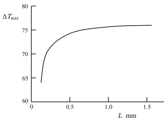
Fig. 10.7 Dependence of maximum temperature depression on length of thermoelements in a module made from extruded bismuth telluride alloys, according to Semenyuk [9]. The heat sink was at 30 °C
