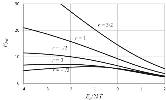
Fig. 4.8 Plot of the function F_{NE} against E_g/2kT for different values of the scattering parameter r . The Nernst–Ettingshausen figure of merit is proportional to F_{NE} . F_{NE} is defined as the function on the right hand side of the relation (4.40)
