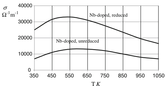
Fig. 9.24 Electrical conductivity plotted against temperature for strontium titanate. The lower curve is for Nb-doped \text{SrTiO}_3 and the upper curve for Nb-doped material that has also been oxygen-deficiency doped. The curves represent the data of Backhaus-Ricoult et al. [89]
