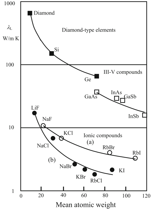
Fig. 4.3 Plot of lattice conductivity against mean atomic weight for certain covalent and ionic crystals. The plot is based on the observations of Ioffe and Ioffe [12]. The ionic compounds are divided into those (a) with the atomic weight ratio less than 1.5 and those (b) with the atomic weight ratio greater than 1.5
