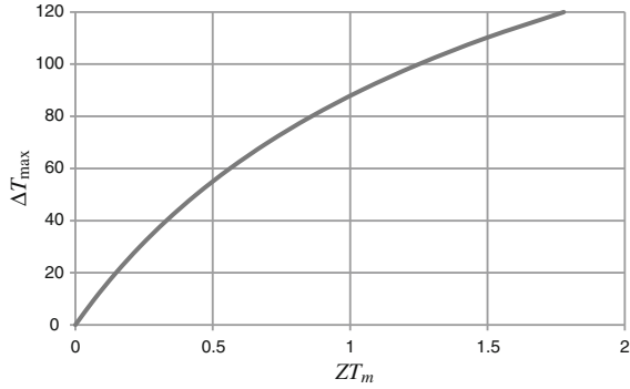
Fig. 2.3 Plot of maximum temperature depression against ZT_m for the heat sink at 300 K
