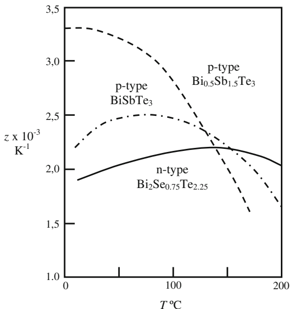
Fig. 6.13 Figure of merit for p-type and n-type bismuth telluride alloys above ambient temperature. Data selected by Matsuura and Rowe [41]
