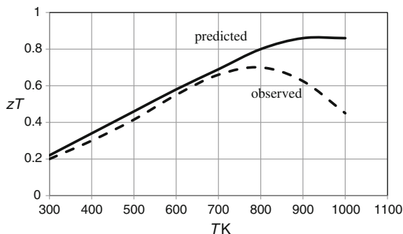
Fig. 9.33 Optimised zT plotted against temperature for complex-doped HMS. The upper curve is the maximum value predicted from the variation of \beta with temperature together with the energy gap as estimated from the maximum Seebeck coefficient. The lower curve represents the observations of Fedorov and Zaitsev [118] as displayed in Fig. 9.32
