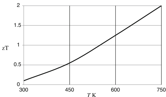
Fig. 9.16 Plot of zT against temperature for (\text{PbTe})_{0.86}(\text{PbSe})_{0.07}(\text{PbS})_{0.07} doped with 2 % Na. Based on observations of Korkosz et al. [44]
