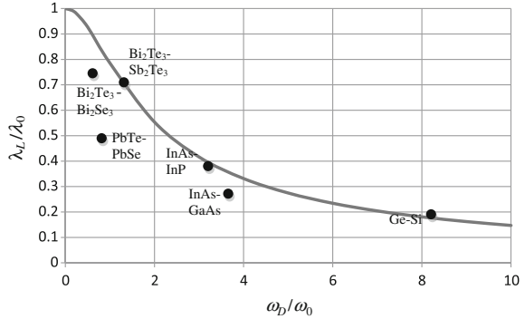
Fig. 5.3 Plot of lattice conductivity against \omega_D/\omega_0 according to (5.20) assuming mass-defect scattering from (5.21). The data points represent thermal conductivity data for semiconductor solid solutions
