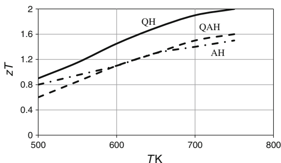
Fig. 12.10 Plots of zT against temperature for nanostructured Na-doped PbTe. The labels refer to the preparation techniques. QH is quenched and hot-pressed AH is annealed and hot-pressed and QAH is quenched, annealed and hot-pressed. The QH material has a mean particle size of less than 4 nm and a mean particle spacing of 5.4 nm. These are schematic plots based on the data of Wang et al. [52]
