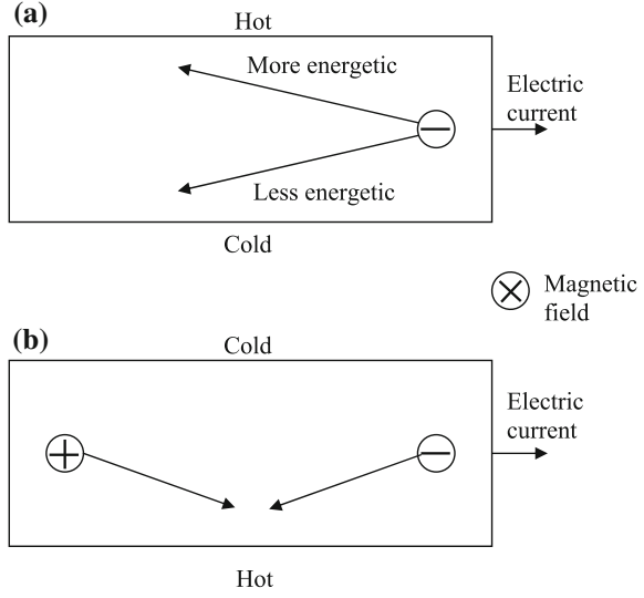
Fig. 4.7 Origin of the Ettingshausen effect in a an extrinsic conductor and b an intrinsic conductor
