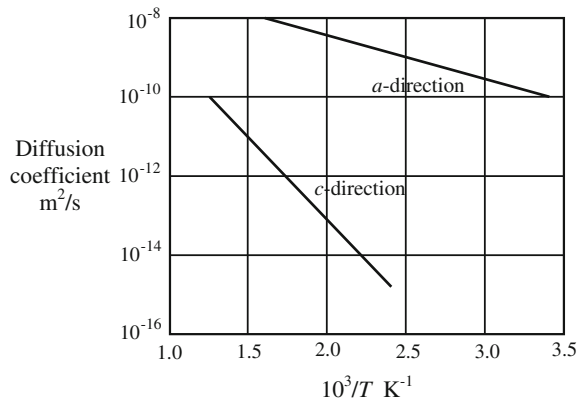
Fig. 6.5 Diffusion coefficient of copper in bismuth telluride in the c -direction and along the plane of the a -axes
