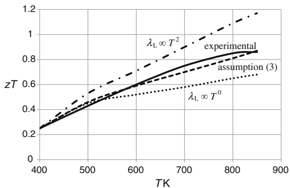
Fig. 9.27 Plots of zT against temperature for \text{Mg}_2\text{Si}_{0.7}\text{Sn}_{0.3} . The theoretical plots correspond to the 3 different assumptions regarding the variation of \beta with temperature. The experimental plot is based on the data from Zaitsev et al. [119]
