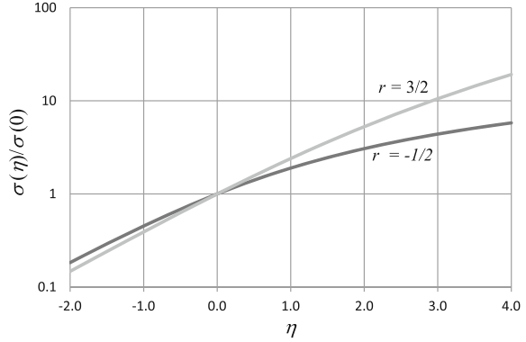
Fig. 3.4 Plot of electrical conductivity against reduced Fermi energy for r equal to -1/2 and 3/2 . The electrical conductivity is given as a fraction of its value at \eta = 0
