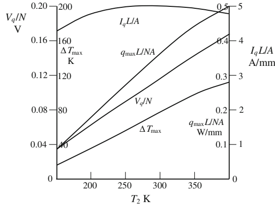
Fig. 10.2 Maximum design parameters plotted against temperature of hot junctions for modules [1] in Table 10.1
