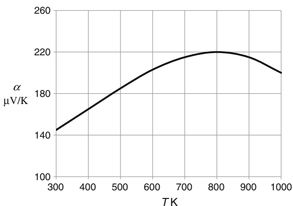
Fig. 9.29 The Seebeck coefficient of complex-doped HMS plotted against temperature (based on the data of Fedorov and Zaitsev [118])
