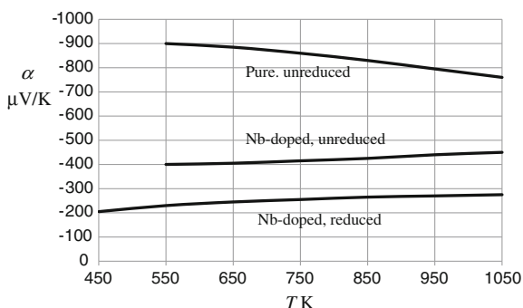
Fig. 9.25 Seebeck coefficient plotted against temperature for \text{SrTiO}_3 . The curves are based on the data of Backhaus-Ricoult et al. [89]
