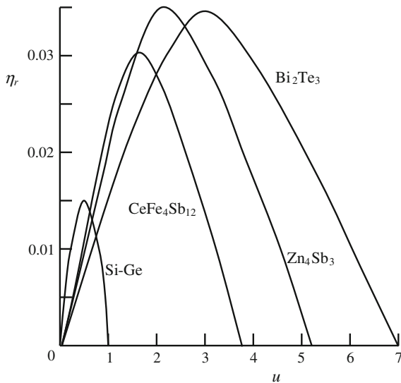
Fig. 10.11 Reduced efficiency as a function of the ratio of electric current density to heat flux density. Schematic plot based on the data of Ursell and Snyder [41]
