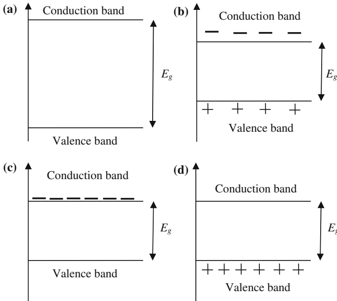
Fig. 3.3 Energy band diagrams for a an insulator, b an intrinsic semiconductor, c an n-type semiconductor and d a p-type semiconductor
