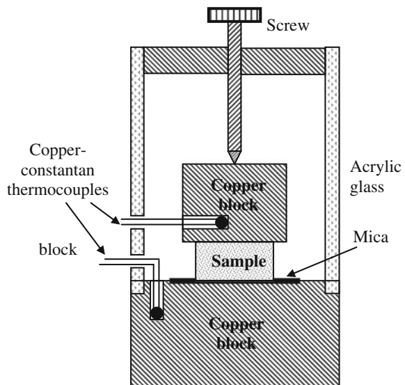
Fig. 8.8 Ioffe and Ioffe's apparatus for the dynamic measurement of thermal conductivity
