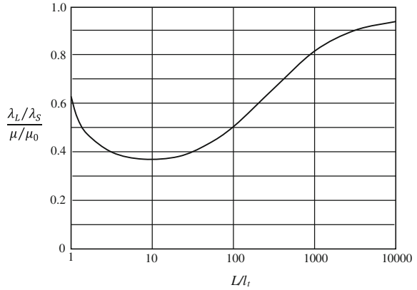
Fig. 5.6 Calculated values of (\lambda_L/\lambda_S)/(\mu/\mu_0) plotted against ratio of effective grain size to phonon mean free path in a Si–Ge alloy at 300 K
