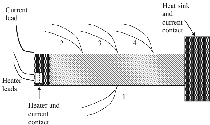
Fig. 8.16 Arrangement of contacts for thermogalvanomagnetic measurements. 1, 2, 3 and 4 are thermocouples, one lead of each also serving as a potential probe. The magnetic field is directed perpendicular to the diagram
