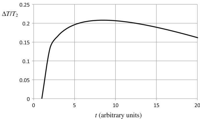
Fig. 10.9 Temperature depression in the transient mode. \Delta T/T_2 is plotted against time in arbitrary units. zT_2 is equal to unity
