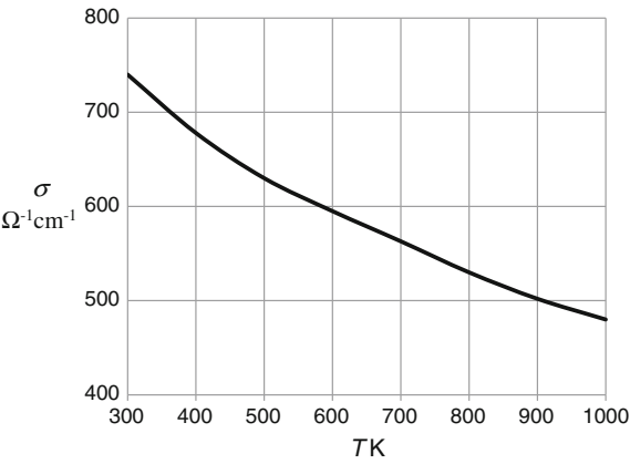
Fig. 9.30 The electrical conductivity of complex-doped HMS as a function of temperature (based on the data of Fedorov and Zaitsev)
