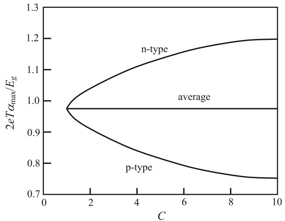
Fig. 4.5 2eT\alpha_{\max}/E_g plotted against the parameter C for n-type and p-type material with \eta_g = 10 . The central line represents the average for the maximum Seebeck coefficients of both types
