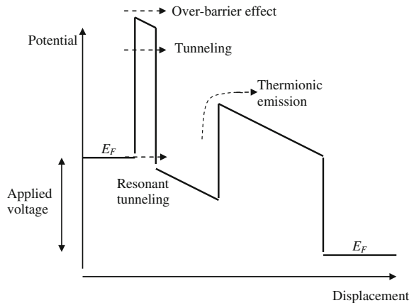
Fig. 13.11 Schematic potential diagram for a heterojunction refrigerator
