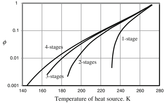
Fig. 2.8 Overall coefficient of performance plotted against heat source temperature for 1, 2, 3 and 4 stage coolers. The heat sink is at 300 K and ZT = 0.7
