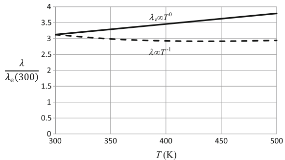
Fig. 6.11 Plot of relative total thermal conductivity against temperature for a typical thermoelectric material with \lambda_L independent of temperature ( upper plot ) and inversely proportional to temperature ( lower plot )
