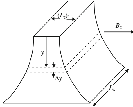
Fig. 2.11 Exponentially-shaped Ettingshausen cascade. Heat is extracted from the source at the upper face
