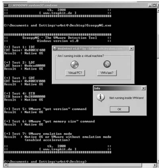
Exhibit 4-26 ScoobyNG and VmDetect after applying VME detection prevention configuration.
