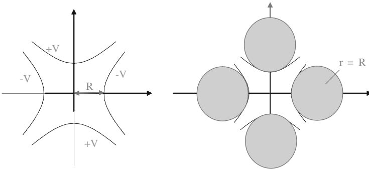
Fig. 6.22 Electric field quadrupole, ideal pole profile ( left ), and an example of a practical approach with cylindrical metallic tubes ( right )
