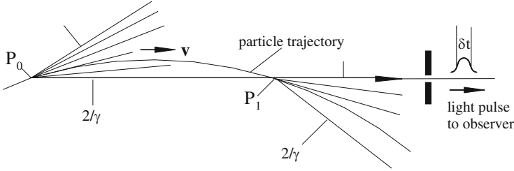
Fig. 24.11 Temporal pulse formation of synchrotron radiation
