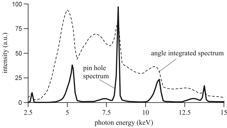
Fig. 26.6 Actual radiation spectra from an undulator with a maximum field of 0.2 T and a beam energy of 7.1 GeV through a pin hole and angle-integrated after removal of the pin hole [7]
