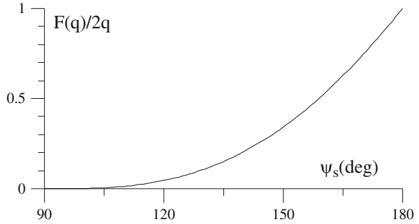
Fig. 9.13 Reduction factor of the momentum acceptance F(q)/2q as a function of the synchronous phase
