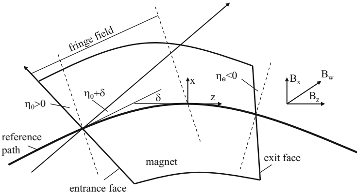
Fig. 7.10 Fringe field focusing in wedge magnets
