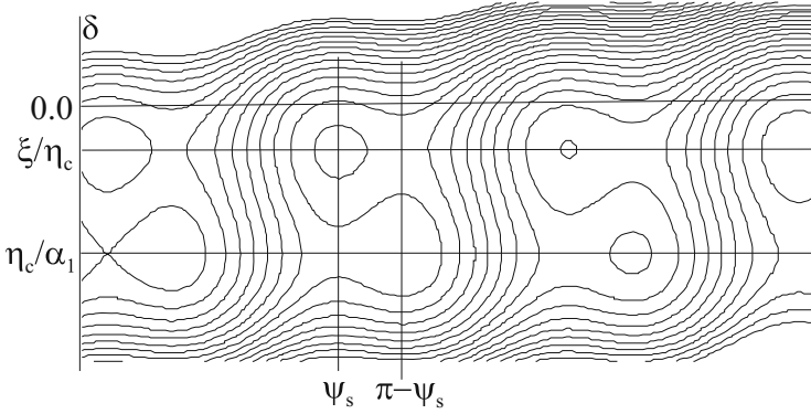
Fig. 9.22 Higher-order longitudinal phase space diagrams for \psi_s = 0.7 , 2\xi/\eta_c = -0.125 and a weak perturbation \alpha_1/\eta_c = -3.0
