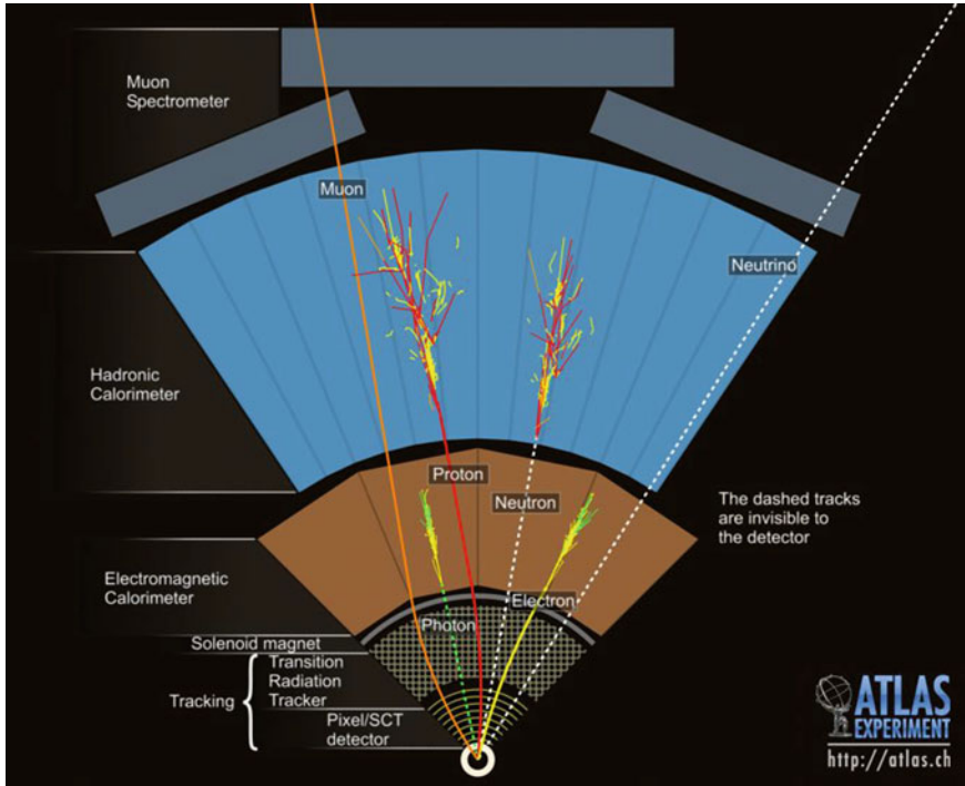
Fig. 4.1 Schematic cut-away of the ATLAS detector. The different signatures of particles traversing the detector are shown
