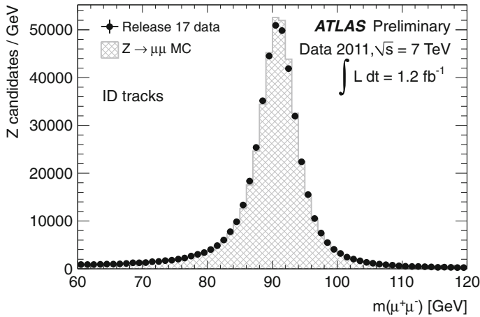
Fig. 5.19 Reconstructed invariant mass using ID track for Z \rightarrow \mu\mu events. The data after detector alignment is shown in black. The expectation from a perfectly aligned detector is shown in gray
