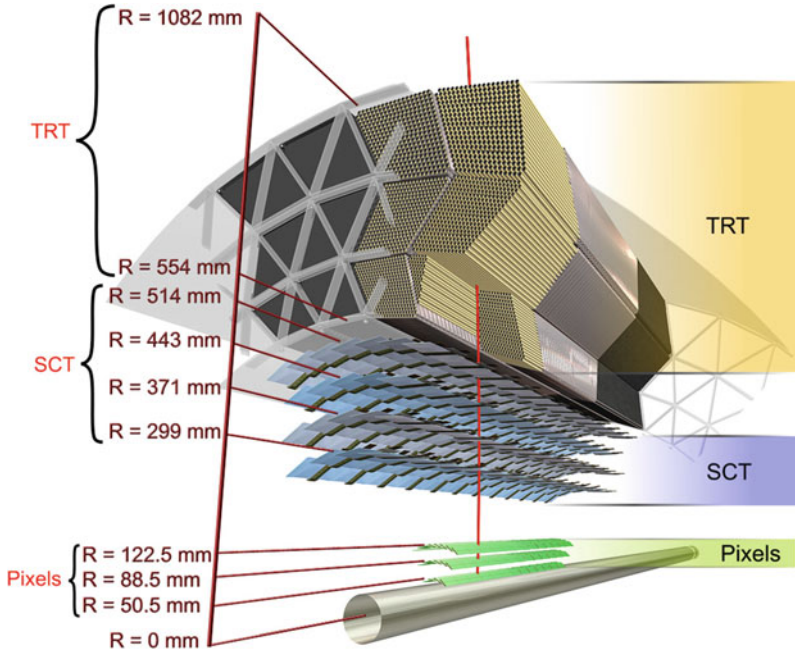
Fig. 3.2 Drawing showing the detector elements crossed by a charged particle with 10 GeV P_T in the barrel of the Inner Detector. The particle emerges from the interaction point and traverses the beam-pipe, three pixel layers, four double layers of SCT sensors, and around 35 TRT straws
