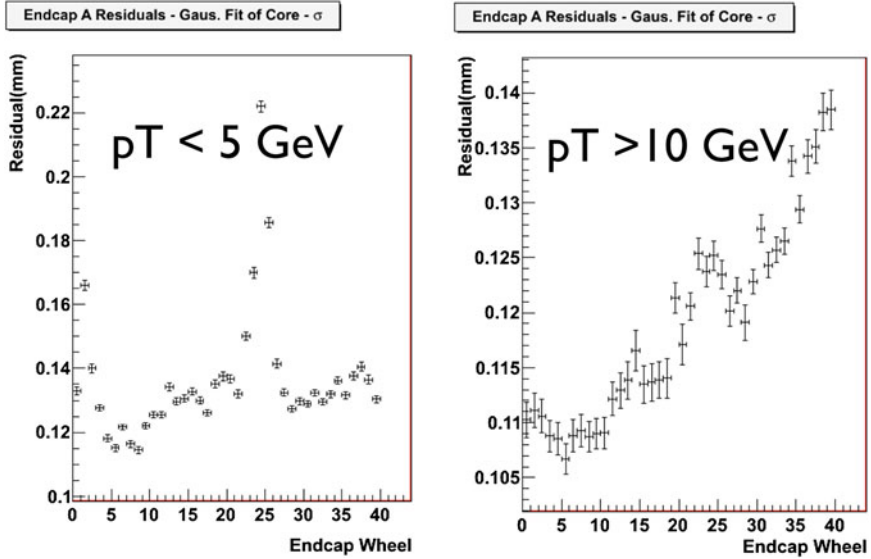
Fig. 6.46 TRT resolution in end-cap A as a function of 4-plane wheel [7]. Left-hand plot uses tracks with p_T below 5 GeV. Right-hand plot is with tracks with p_T above 10 GeV. Note the scale difference
