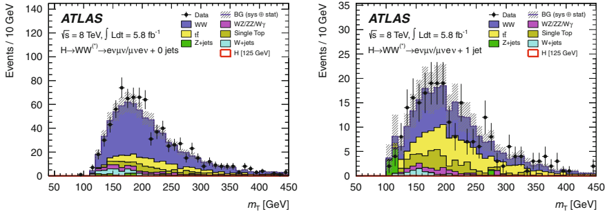
Fig. 11.10 m_T distribution in the WW control region for the 0-jet 2012 analysis (left-hand side) and the 1-jet 2012 analysis (right-hand side). The points show the observed data and the stacked histograms represent the signal and background expectation
