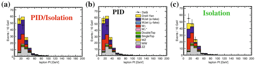
Fig. 9.30 Test of W +jet modeling in the “Medium-Not-Tight” validation region defined in Table 9.9. Sub-leading p_T distribution is shown for events in the \mu e -channel. The fake predictions are made with the fake factor procedure using: a the “Pid-And-Iso”-denominator definition, b The “Pid”-denominator definition c the “Isolation”-denominator definition. Results are from the 5.8 \text{ fb}^{-1} 7 \text{ TeV} data set
