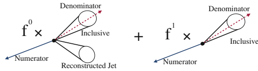
Fig. 9.26 Schematic of background modeling in a one jet signal region. The left-hand term predicts background when the jet does not overlap the misidentified lepton. The right-hand term predicts background when the jet overlaps the misidentified lepton
