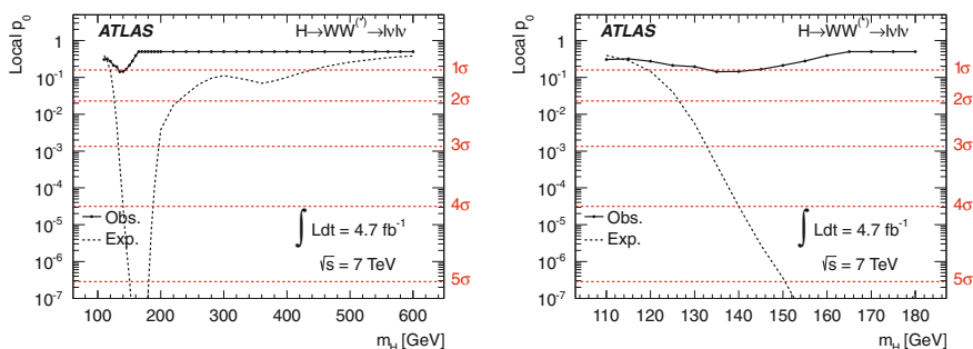
Fig. 11.16 Probabilities for the background-only hypothesis, p_0 , as a function of m_h , for the 2011 analysis. The left-hand plot shows m_h in the range 110–600 GeV, the right-hand plot focuses on m_h between 110 and 180 GeV. The solid line shows the observed probability. The dashed line shows the corresponding expectation for the signal + background hypothesis at the given value of m_h . The red, horizontal dashed lines indicate the corresponding significance
