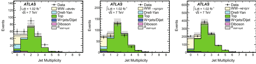
Fig. 10.3 Jet multiplicity distributions for the ee -channel (left-hand side), the \mu\mu -channel (middle) and e\mu -channel (right-hand side) before the jet veto. The points show the observed data and the stacked histograms represent the signal and background expectation. Scale factors as described in Sect. 10.2 are applied to MC
