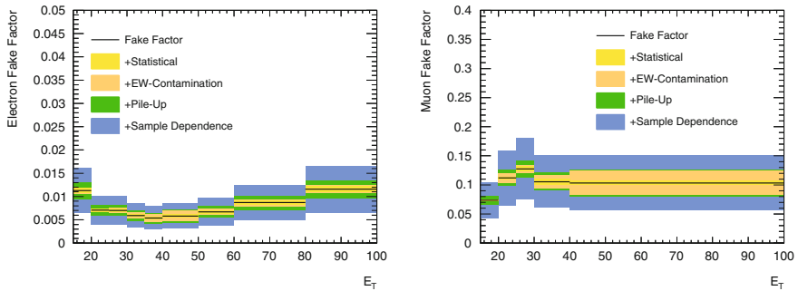
Fig. 11.13 Measured electron ( left ) and muon ( right ) fake factors for the 2011 analysis. The systematic uncertainties are included in the error bands
