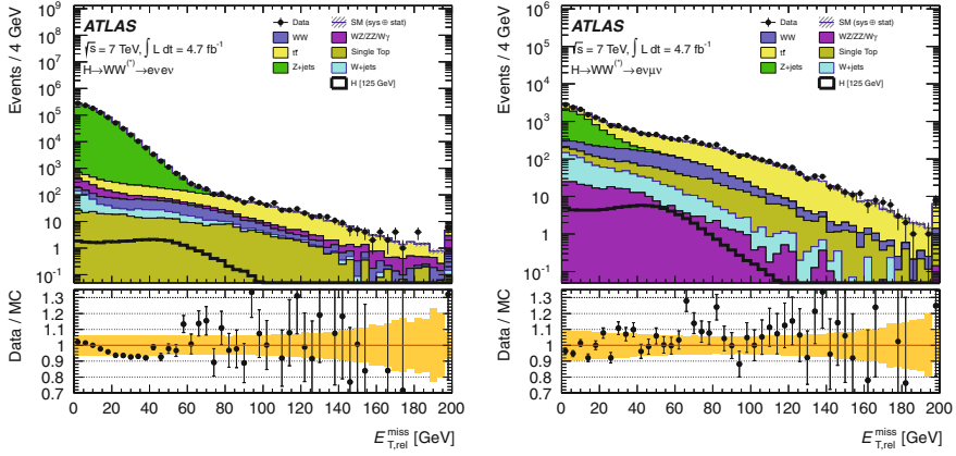
Fig. 11.1 E_T^{\text{miss,Rel}} distributions after the di-lepton pre-selection in the 2011 analysis. The same-flavor ( ee ) channel is shown on the left . The opposite-flavor channel is shown on the right . The points show the observed data and the stacked histograms represent the signal and background expectation
