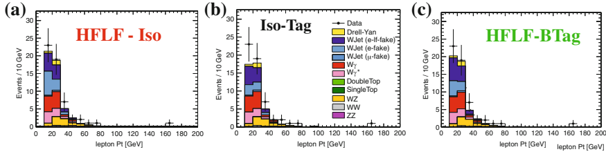
Fig. 9.34 Test of the W +jet modeling in same sign events using separate light-flavor and heavy-flavor predictions. Sub-leading p_T distribution is shown for events in the \mu e -channel with a same sign requirement. The fake predictions are made with the fake factor procedure using: a the “Pid” light-flavor denominator definition and the “Isolation” heavy-flavor denominator definition. b The “Pid” light-flavor denominator definition and the “Isolation” heavy-flavor denominator definition. c The “Pid-And-Iso” light-flavor denominator definition and the “BTag” heavy-flavor denominator definition. Results are from the 5.8 \text{ fb}^{-1} 7 \text{ TeV} data set
