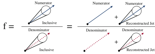
Fig. 9.23 Schematic of the separation of the standard fake factor measurement into terms extrapolating to background with and without overlapping jets. f^0 extrapolates to fake background without overlapping jets. f^1 extrapolates to fake background with overlapping jets
