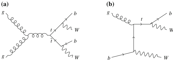
Fig. 8.5 The dominant Feynman diagrams for a t\bar{t} and b Wt production. t\bar{t} production also includes a t -channel top quark exchange diagrams, which is not pictured. Wt production includes an s -channel b-quark exchange diagram which is not shown
