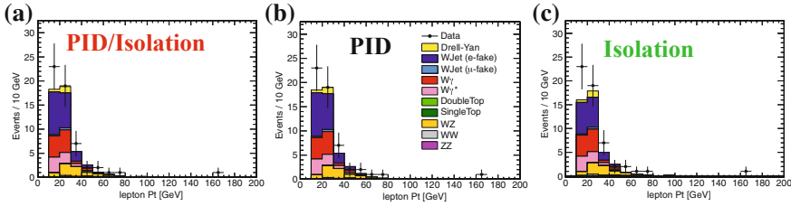
Fig. 9.27 Test of W +jet modeling in same sign events. Sub-leading p_T distribution is shown for events in the \mu e -channel with a same sign requirement. The fake predictions are made with the fake factor procedure using: a the “Pid-And-Iso”-denominator definition. b The “Pid”-denominator definition c the “Isolation”-denominator definition. Results are from the 5.8 \text{ fb}^{-1} TeV data set
