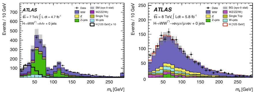
Fig. 11.5 m_{ll} distribution before the p_{Tll} requirement for the 2011 analysis ( left-hand side ) and after the p_{Tll} requirement for 2012 analysis ( right-hand side ). The 2011 analysis is shown before the p_{Tll} because in that analysis the m_{ll} cut is made before the p_{Tll} requirement. The points show the observed data and the stacked histograms represent the signal and background expectation. The signal distribution in the left-hand plot has been scale up by a factor of 10 for clarity
