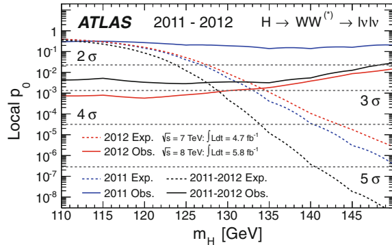
Fig. 12.11 The observed p_0 as a function of m_h for the H \rightarrow WW^{(*)} channel. The dashed line shows the corresponding expectation for the signal+background hypothesis at the given value of m_h . Results are shown separately for the \sqrt{s} = 7 TeV data (dark, blue), the \sqrt{s} = 8 TeV data (light, red), and their combination (black)
