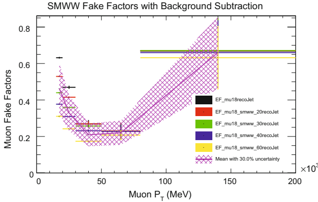
Fig. 10.8 Muon fake factors measured in the di-jet sub-samples. The purple line shows the weighted average of the fake factors and the hashing indicates the \pm 30\% band. The statistical and the systematic error from electro-weak MC subtraction are included in the error bars
