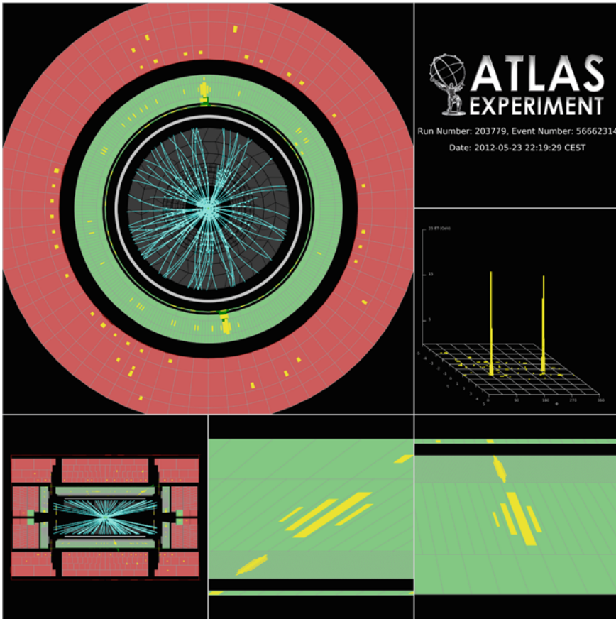
Fig. 12.5 Event display of a selected H \rightarrow \gamma\gamma event. The photons are shown in yellow and correspond to localized high energy deposits in the calorimeter not matched to tracks in the inner detector. The photons have a combined invariant mass of 126.9 GeV. The upper-left panel shows the projection of the detector in the plane perpendicular to the beam line. The lower-left panel shows the projection of the detector along the beam line, running left to right in the panel. The lower-middle and lower-right panels are zoom-ins of interesting regions. The middle-right panel depicts the energy deposited in the calorimeters as a function of \phi and \eta
