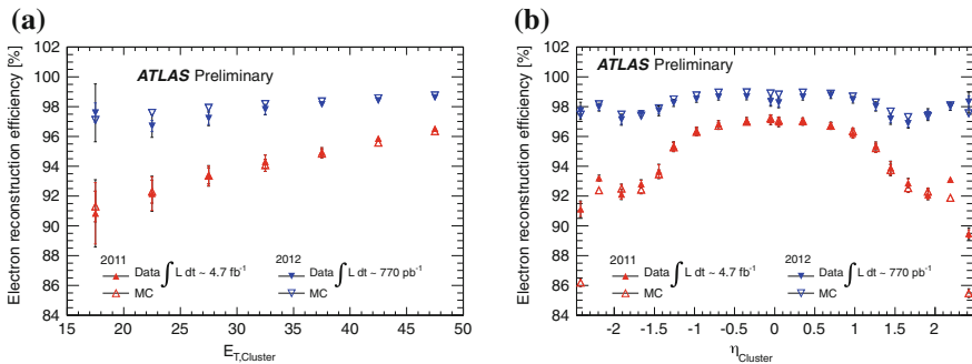
Fig. 7.2 Electron reconstruction efficiency, including the requirements on the track quality, ( N_{\text{pix}} \geq 1 and N_{\text{Si}} \geq 7 ) as a function of a E_T and b \eta . The plot versus \eta is shown for electrons with E_T between 30 and 50 GeV
