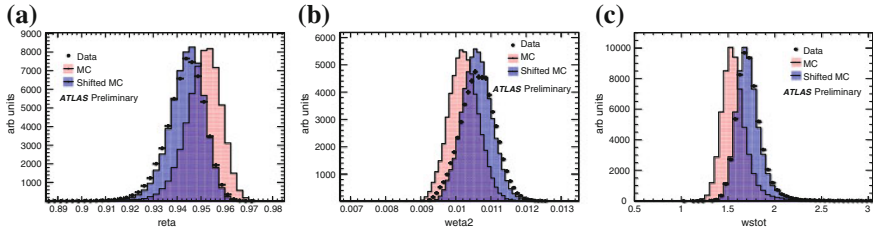
Fig. 7.14 MC correction procedure using the high statistics 2011 data sample. The R_\eta , w_{\eta^2} , and w_{s,\text{tot}} distributions are shown for data (black), the uncorrected MC (red), and the corrected MC (blue). The results are shown for the bin with E_T between 30 and 40 GeV, and |\eta| between 1.15 and 1.37
