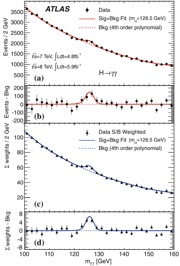
Fig. 12.6 The distributions of the invariant mass of di-photon candidates after all selections for the combined 7 and 8 TeV data sample. The inclusive sample is shown in upper figure, marked (a). The distribution weighted according to the event categories is shown in the lower figure marked (c). The result of a fit using a m_h = 126.5 GeV signal component and the background component is superimposed. The excess of data with respect to the background fit are displayed in panels marked (b) and (d)
