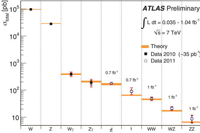
Fig. 1.2 Summary of several Standard Model total production cross section measurements compared to the corresponding theoretical expectations. The dark error bar represents the statistical uncertainty. The red error bar represents the full uncertainty, including systematics and luminosity uncertainties. The W and Z vector-boson inclusive cross sections were measured with 35\text{pb}^{-1} of integrated luminosity. All other measurements were performed using the 2011 data-set. The top quark pair production cross-section is based on a statistical combination of measurements in the single-lepton, di-lepton and all-hadronic channels using up to 0.7\text{fb}^{-1} of data. The single-top measurement uses 0.7\text{fb}^{-1} of data. The WW and WZ and ZZ measurements were made using 1.02\text{fb}^{-1} .
