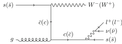
Fig. 9.28 Feynman diagram for W +charm production where the charm quark decays semi-leptonically. The charge of the W is opposite that of the lepton from the charm quark decay
