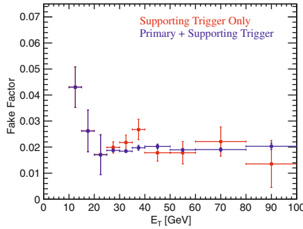
Fig. 9.7 Comparison of electron fake factor using only the supporting triggered sample, in red , and using a combination of primary electron and supporting triggers, in blue . Using the combination of triggers reduces the statistical uncertainty on the fake factor. The “PID”-denominator definition is used the fake factor calculation
