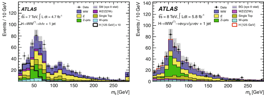
Fig. 11.8 m_{||} distribution after the Z \rightarrow \tau\tau veto for the 2011 analysis ( left-hand side ) and the 2012 analysis ( right-hand side ). The points show the observed data and the stacked histograms represent the signal and background expectation. The signal distribution in the left-hand plot has been scale up by a factor of 10 for clarity
