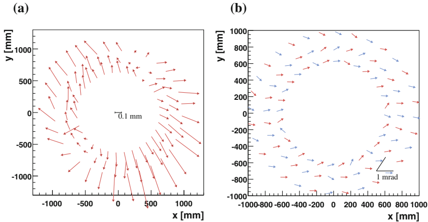
Fig. 6.22 L2 Alignment Parameters when using silicon Information. a Visual representation of the translation alignment parameters. Each arrow represents a barrel module. The tail of the arrow is the nominal module position. The arrow length and direction represent the global x and y alignment parameters. The arrow lengths are enlarged by a factor of 1,000 relative to the axes. A scale is provided for reference. b Visual representation of the rotations about z. Each arrow represents a barrel module. The size of the rotation is given as the angle the arrows make with respect to the positive x-axis. The arrow lengths has no meaning. The size of the rotations are enlarged by a factor of 1,000. A scale is provided for reference
