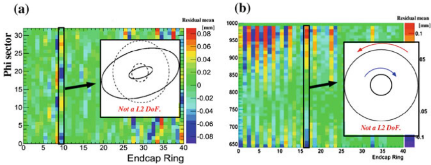
Fig. 6.37 Sketches of 4-plane wheel deformations indicated by systematic residual bias after the L2 alignment. The residual map of \phi versus 4-plane wheel ( left ) shows signs of elliptical deformation. The residual map of r versus 4-plane wheel ( right ) shows signs of twist-like deformation
