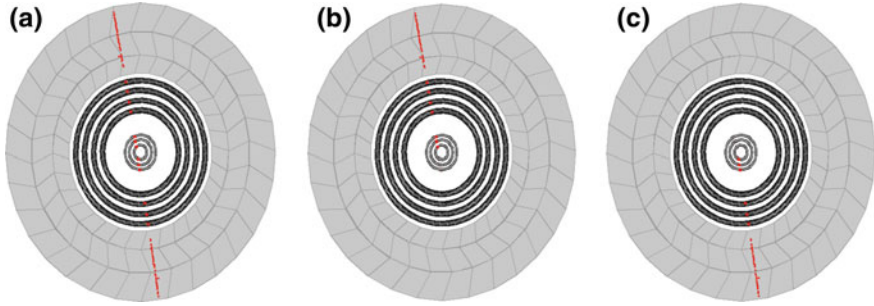
Fig. 5.11 Illustration of track-splitting in cosmic-ray events. Cosmic-ray muons with low impact parameters crossing both halves of the ID (a), can be split and reconstructed as two collision-like tracks (b) and (c). The upper and lower track halves are from the same charged particle and should thus have the same track parameters
