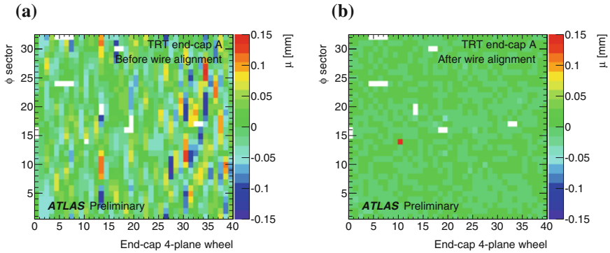
Fig. 6.39 Mean of a Gaussian fit to TRT residuals versus \phi -sector and wheel before, (a), and after, (b), the wire-level alignment. The plots illustrate the results for end-cap A. The white bins are due to dead channels
