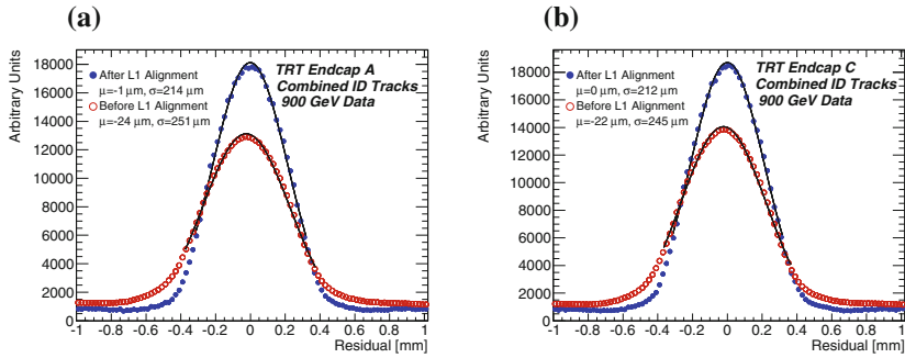
Fig. 6.13 The TRT end-cap residual distributions before and after the L1 end-cap alignment for end-cap A (a) and end-cap C (b)
