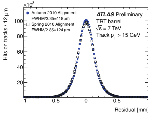
Fig. 6.43 TRT residual distributions in the barrel before and after the L3 barrel alignment. The “Autumn 2010 Alignment” includes the L3 alignment, the “Spring 2010 Alignment” uses the TRT geometry before the L3 alignment
