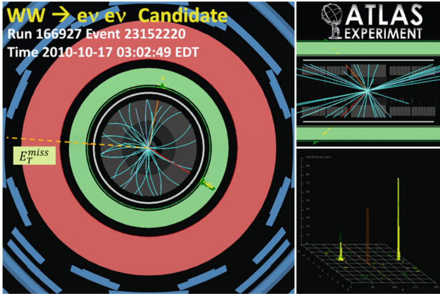
Fig. 12.9 Event display of a WW event in the eev channel. The electrons are shown in yellow and correspond to localized high energy deposits in the calorimeter matched to tracks in the inner detector, indicated by the red and orange lines. The dashed line, label E_T^{\text{miss}} , indicates the direction of the measured momentum imbalance. The left panel shows the projection of the detector in the plane perpendicular to the beam line. The upper-right panel shows the projection of the detector along the beam line, running left to right in the panel. The lower-right panel depicts the energy deposited in the calorimeters and the direction of the E_T^{\text{miss}} , as a function of \phi and \eta
