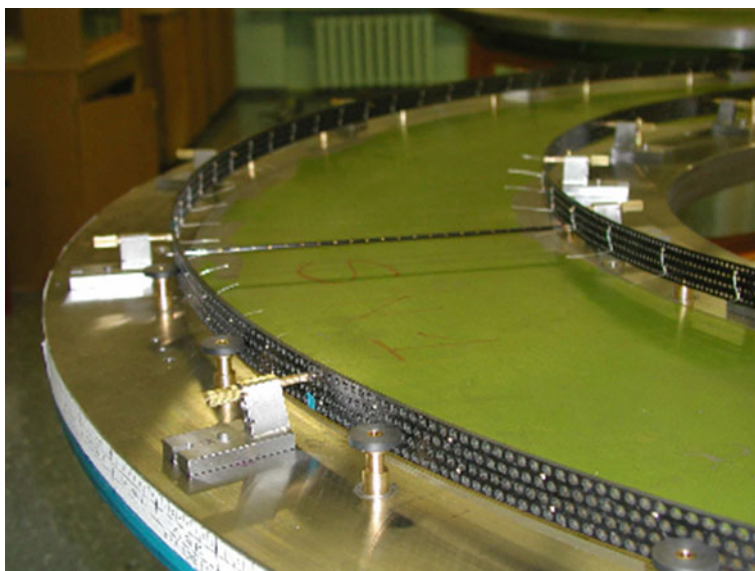
Fig. 6.6 A picture of a TRT end-cap 4-plane wheel during construction. The inner and outer supporting rings are visible. One straw is shown connecting the rings.
