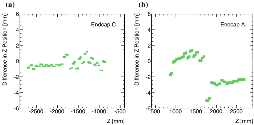
Fig. 6.50 Measured misalignment in z as a function of z , for end-cap C ( left ) and end-cap A ( right ). The division between A and B-wheels occurs around |z| of 1,700 mm
