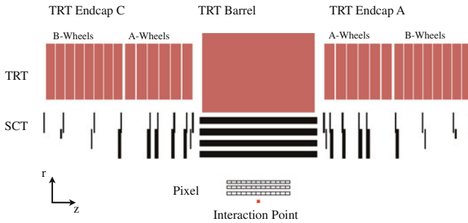
Fig. 6.1 Schematic of TRT in the r - z plane. The TRT is composed of barrel and end-cap detectors. The division of the end-caps into A-wheels and B-wheels can be seen
