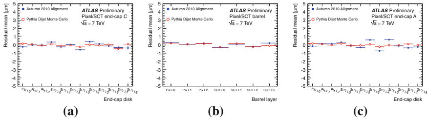
Fig. 5.15 Average of the residual distribution as a function of Pixel or SCT barrel layer or end-cap disk for: end-cap C (a), barrel (b), and end-cap A (c). The result from data after the L3 alignment is shown in blue. The expectation from a perfectly aligned detector in MC is shown in red
