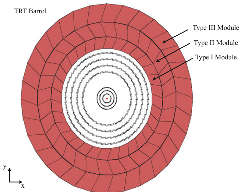
Fig. 6.5 Schematic of the Inner Detector barrel, x-y view. The TRT barrel modules are the red shaded trapezoids . The three layers of module types are indicated
