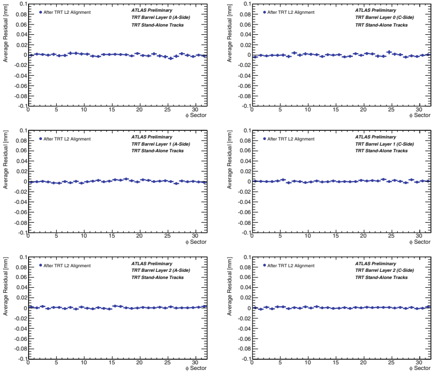
Fig. 6.27 Average residual as a function of \phi -sector for hits in barrel modules on sides A ( left plots ) and C ( right plots ) separately. Modules in the first barrel layer are in the top row , those in the second layer are shown in the middle , and barrel modules in the third layer are shown in the bottom row . For the residuals in side-A (side-C), the geometry after the L2 alignment with only the A-side (C-side) hits was used
