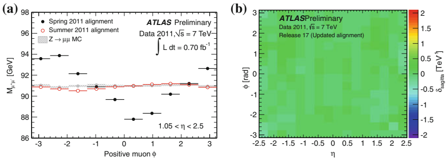
Fig. 5.18 Evidence for the removal of detector weak modes with the constrained alignment. a shows the mean of the reconstructed Z invariant mass using ID tracks in Z \rightarrow \mu\mu events as a function of the \phi of the positive muon, for tracks in end-cap A. The data before the constrained alignment is shown in black. The data after the constrained alignment is shown in red. The expectation from a perfectly aligned detector is shown in gray. b shows the measured sagitta bias using W \rightarrow e\nu events as a function of the electron \eta and \phi after the constrained alignment. No bias is seen after the constrained alignment
