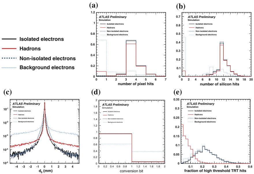
Fig. 7.6 Electron identification variables in the ID, shown separately for signal and the various background types. The variables shown are a number of hits in the Pixel detector, b combined number of hits in the Pixel and SCT detectors, c transverse impact parameter d_0 , d conversion flag, or “conversion bit”, and e fraction of high-threshold hits in the TRT
