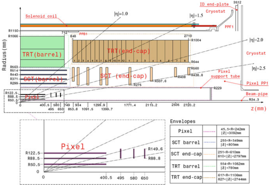
Fig. 5.4 Layout of the Inner Detector. The division into barrel and end-caps can be seen. The further division of the barrels, into layers, and the end-caps, into disks is also shown. The full detector granularity is not given
