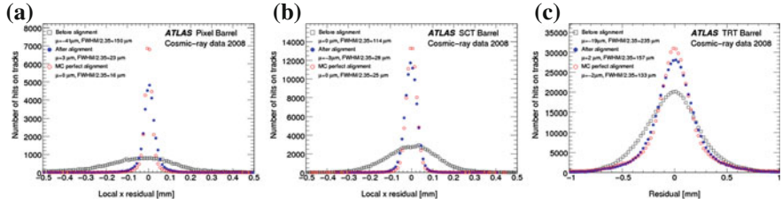
Fig. 5.12 Residual distributions from cosmic-ray muon tracks in the Pixel (a), SCT (b), and TRT (c) barrels. Distributions are shown before and after the alignment from cosmic-rays. The result of using a perfectly aligned detector in MC is shown for comparison
