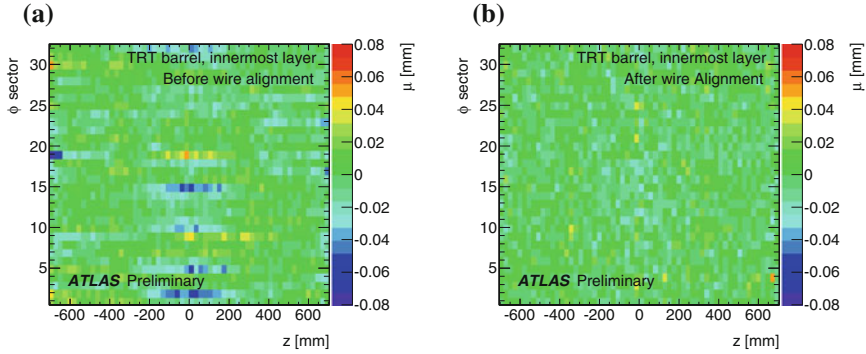
Fig. 6.44 Mean of a Gaussian fit to TRT residuals versus \phi -sector and z for the first TRT barrel layer before (a) and after (b), the wire-by-wire alignment
