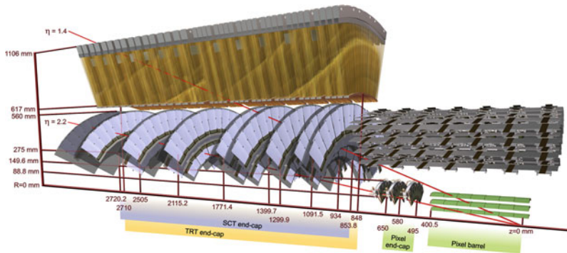
Fig. 3.3 Drawing showing the detector elements crossed by two charged particles of 10 GeV P_T in the end-cap of the Inner Detector. A particle at |\eta| = 1.4 traverses the beam-pipe, three pixel layers, four SCT disks with double layers of sensors, and approximately 40 straws in the TRT end-cap. A particle at |\eta| = 2.2 traverses the beam-pipe, only the first layer of the pixel detector, two end-cap pixel disks and the last four disks of the SCT end-cap. The coverage of the end-cap TRT does not extend beyond |\eta| = 2
