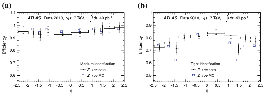
Fig. 7.12 Efficiencies of the medium and tight requirements in the “robust” isEM menu. The efficiencies are measured using Z \rightarrow ee events and are shown for electrons with E_T between 20 and 50 GeV. The error bars provide the statistical ( inner ) and total ( outer ) uncertainties on the measured efficiencies
