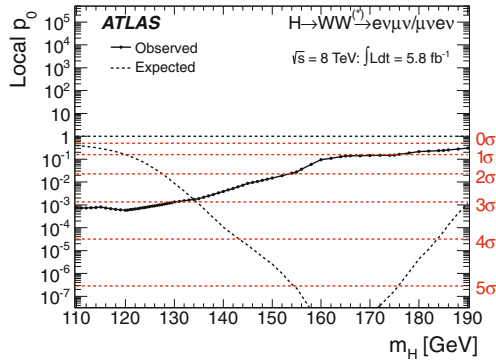
Fig. 11.19 Probabilities for background-only hypothesis, p_0 , as a function of m_h , for the 2012 analysis. The solid line shows the observed probability. The dashed line shows the corresponding expectation for the signal + background hypothesis at the given value of m_h . The red, horizontal dashed lines indicate the corresponding significance
