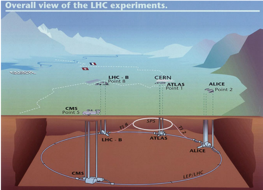
Fig. 2.1 Diagram of the locations of the four main experiments (ALICE, ATLAS, CMS and LHCb) at the LHC. Located between 50 and 150 m underground, huge caverns have been excavated to house the giant detectors. The SPS, the final link in the pre-acceleration chain, and its connection tunnels to the LHC are also shown
