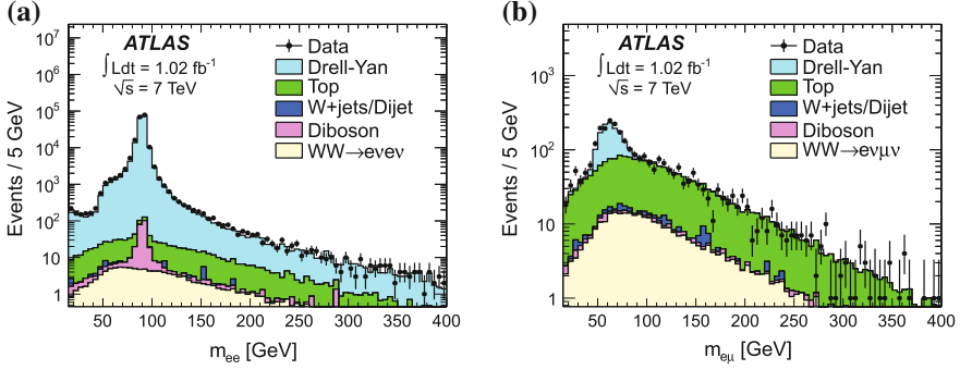
Fig. 8.6 m_{\ell\ell} distributions for same-flavor and opposite-flavor di-leptons before a missing energy requirement. a Shows the ee -channel, b Shows the e\mu -channel. The events are required to have one lepton with p_T above 25 GeV and one lepton with a p_T above 20 GeV
