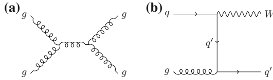
Fig. 9.4 Leading order Feynman diagrams for a di-jet production and b W +jet production. The jets in the di-jet sample are gluon initiated, whereas jets in the W +jet sample are quark initiated
