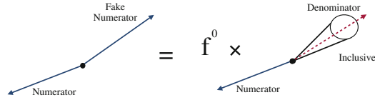
Fig. 9.25 Schematic of corrected fake factor procedure for predicting background to events in which a jet veto is applied. The left-hand side represents the background in the signal region, the right-hand side represents the updated fake factor modeling of the background. The W +jet control region with the inclusive denominator sample is scaled by fake factor for no overlapping jets
