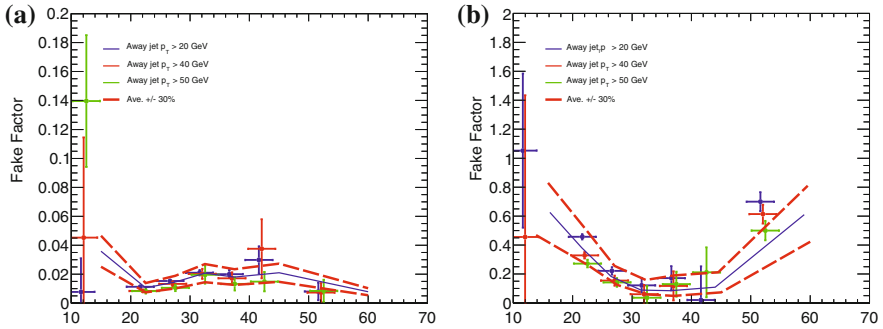
Fig. 10.9 a Extracted light-flavor f_{l.f.} ( left ), b Heavy-flavor f_{h.f.} ( right ) fake factors
