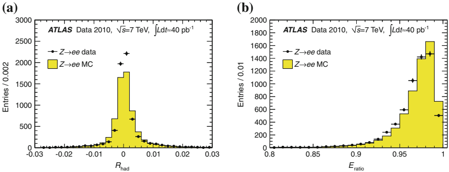
Fig. 7.11 Comparison of the shower shapes, R_{\text{had}} and E_{\text{ratio}} , of electrons from Z \rightarrow ee events in data and MC. The electrons are required to have E_T between 40 and 50 GeV. The data distributions are shown after background subtraction. The uncertainties on the data include the systematic uncertainty from the background subtraction. The MC is normalized to the number of entries in data
