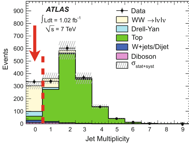
Fig. 8.9 Distribution of the number of reconstructed jets after the E_T^{\text{miss, Rel}} requirement. The plot combines the same-flavor and opposite-flavor channels. The jet veto of the WW signal selects events in the first bin, indicated by the arrow
