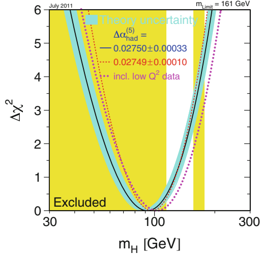
Fig. 1.5 Standard Model prediction of the Higgs mass. The line is the result of the fit using data at the Z pole, and the direct determinations of m_t, m_W, \Gamma_W . The band represents an estimate of the theoretical error due to missing higher order corrections. The vertical band shows the 95 % CL exclusion limit on m_h from the direct searches at LEP-II (up to 114 GeV) and the Tevatron (158–175 GeV). The dashed curve shows the result of using a different values of \Delta\alpha_{\text{had}}^{(5)} . The dotted curve corresponds to a fit including lower energy data
