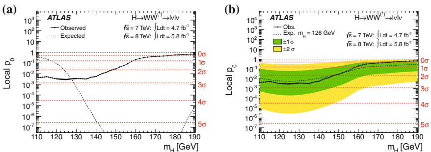
Fig. 11.22 Probabilities for background-only hypothesis, p_0 , as a function of m_h , for the combined 2011 and 2012 analysis. The solid lines show the observed probability. The dashed line in the left-hand plot shows the corresponding expectation for the signal + background hypothesis at the given value of m_h . In the right-hand plot, the dashed line shows the corresponding expectation for the m_h = 126 \text{ GeV} hypothesis. The green and yellow regions indicate the 1\sigma and 2\sigma uncertainty bands on the expected p_0 . The red, horizontal dashed lines indicate the corresponding significance
