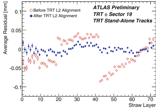
Fig. 6.20 Average residual as a function of straw-layer for hits in \phi -sector 19. The discontinuities in the distribution before L2 alignment are removed with the L2 alignment
