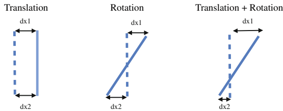
Fig. 6.7 Wire-level DoF used in the L3 alignment. The plane of the page represents the straw plane. The direction of charged particles is into the page. The sensitive displacements in the straw plane can be represented by two DoF: a translation and a rotation
