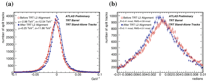
Fig. 6.21 Validation of the L2 alignment with split tracks. Comparison of the \frac{q_T}{p_T} (a) and the \phi_0 (b), difference of split tracks before and after the L2 barrel alignment
