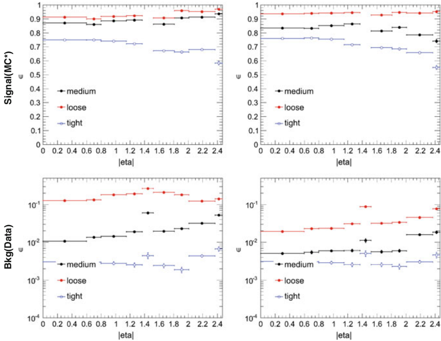
Fig. 7.16 Comparison of the isEM and isEM++ menus. Signal efficiency and background rejection of the isEM menu is given on the left . The results for the isEM++ menu is given on the right . The upper two plots give the signal efficiency, as determined from the corrected MC. The lower plots show the background rejection with respect to reconstructed electrons. The results are shown for electrons candidates with 20 < E_T < 30 GeV
