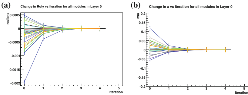
Fig. 6.17 Examples of convergence of the L2 alignment parameters. Changes in the rotations around y (a) and translations along x (b), as a function of alignment iteration for all modules in the first barrel layer. Each curve represents a different barrel module
