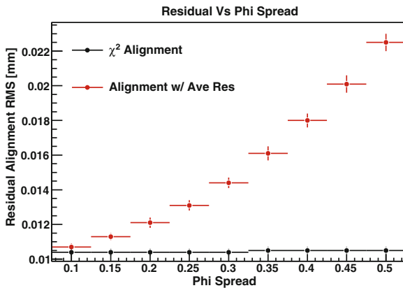
Fig. A.9 RMS of residual misalignments as a function of phi spread of tracks used in alignment
