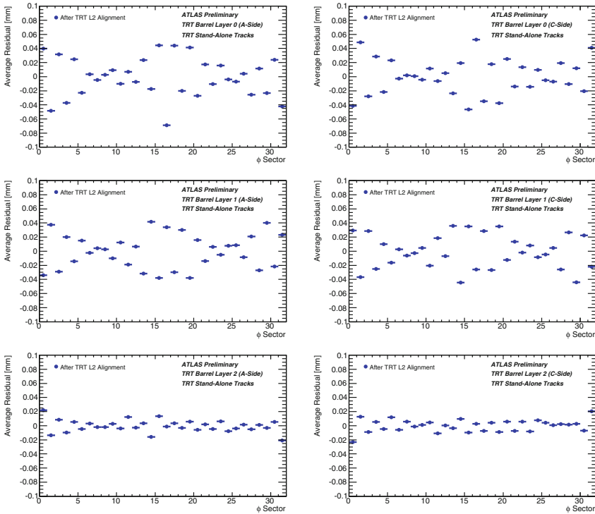
Fig. 6.26 Average residual as a function of \phi -sector for hits in barrel modules on side A ( left plots ) and C ( right plots ) separately. Modules in the first barrel layer are shown in the top row , those in the second are shown in the middle , and barrel modules in the third layer are shown in the bottom row
