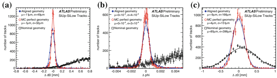
Fig. 5.13 Difference in track parameters: d_0 (a), \phi_0 (b), and z_0 (c), for split cosmic-ray tracks in the Pixel and SCT barrel. Distributions are shown before and after the alignment from cosmic-rays. The result of using a perfectly aligned detector in MC is shown for comparison
