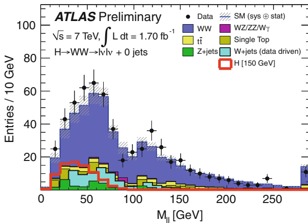
Fig. 8.12 m_{ll} distribution after the WW selection. The distribution from the Higgs signal with a mass of 150 GeV is indicated in the figure
