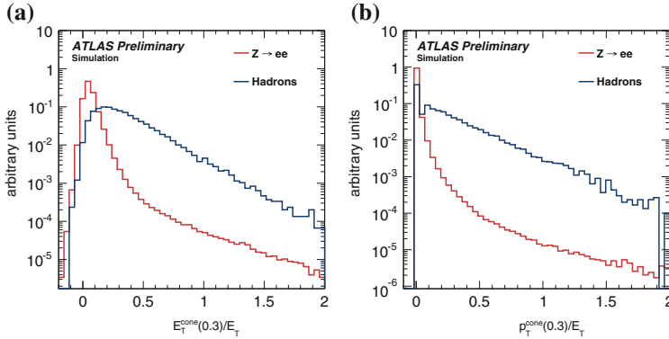
Fig. 7.9 Examples of electron isolation variables a relative calorimeter isolation in a cone of \Delta R < 0.3 b relative track isolation in a cone of \Delta R < 0.3 . Signal electrons and hadron background are shown separately
