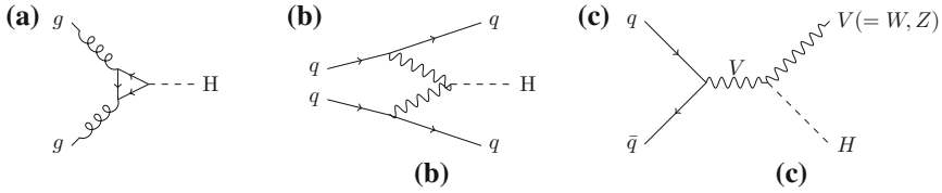
Fig. 1.6 Leading order Feynman diagrams for Higgs production at the LHC. a The gluon fusion diagram proceeds via top-quark loop. b The vector-boson fusion diagram results in a final state with the Higgs and two jets. c The associated production diagram results in a final state with the Higgs and a W or Z boson. The relative size of the cross-sections of the different processes is shown in Fig. 1.7
