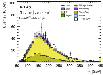
Fig. 11.11 m_T distribution in the Top control region for the 1-jet 2011 analysis. The distribution for the 2-jet analysis is not shown as the statistics are too poor to make a meaningful shape comparison. The points show the observed data and the stacked histograms represent the signal and background expectation
