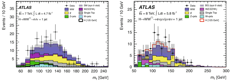
Fig. 11.9 m_T distribution after the full 1-jet selection for the 2011 analysis ( left-hand side ) and the 2012 analysis ( right-hand side ). The points show the observed data and the stacked histograms represent the signal and background expectation. The signal distribution in the left-hand plot has not been scale up
