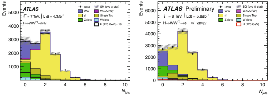
Fig. 11.3 Jet multiplicity distributions after the E_T^{\text{miss, Rel}} requirement for 2011 analysis ( left-hand side ) and the 2012 analysis ( right-hand side ). The points show the observed data and the stacked histograms represent the signal and background expectation. The signal distribution in the left-hand plot has been scale up by a factor of 10 for clarity
