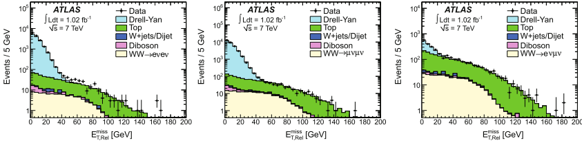
Fig. 10.2 E_T^{\text{miss,Rel}} distributions for ee (left), \mu\mu (middle) and e\mu channels after the Z-veto cut. The points show the observed data and the stacked histograms represent the signal and background expectation. Scale factors as outlined in Sect. 10.2 are applied to MC
