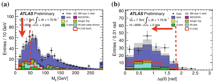
Fig. 8.14 Kinematic variables used to separate SM WW production from H \rightarrow WW^{(*)} production. a m_{\ell\ell} distribution after the WW selection. The cut value used in the low-mass Higgs search is indicated in the figure. b \Delta\phi_{\ell\ell} distribution after the low m_{\ell\ell} requirement. The cut value used in the low-mass Higgs search is indicated in the figure
