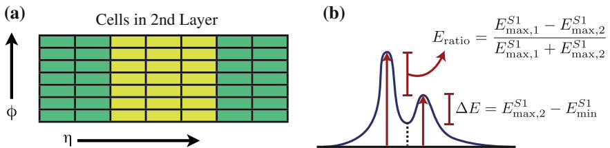
Fig. 7.5 Schematic diagrams of R_\eta and E_{\text{ratio}} . a R_\eta is calculated as the ratio of the sum of energy in the yellow cells to the sum of energy in the yellow and green cells. The yellow cells are centered on the reconstructed electron. b E_{\text{ratio}} is calculated as the ratio of the difference in energy of the two highest cells, to the sum the energy in the two highest cells [8]. E_{\text{ratio}} is calculated from the cells in the first layer of the calorimeter
