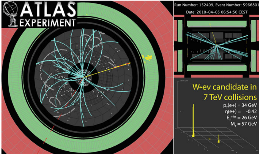
Fig. 7.1 Event display of a reconstructed electron from a candidate W decay. The reconstructed electron track is indicated in yellow . The electron cluster is shown in yellow , in the green EM calorimeter. The red points along the electron track indicate detection of transition radiation. The red dashed line indicates the direction of the momentum imbalance
