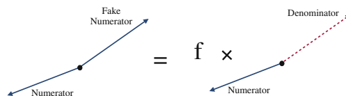
Fig. 9.22 Schematic of the standard fake factor procedure for predicting background to events in which a jet veto is applied. The left-hand side represents the background in the signal region, the right-hand side represents the fake factor modeling of the background: W +jetcontrol region times fake factor. None of the objects in the picture overlap with reconstructed jets
