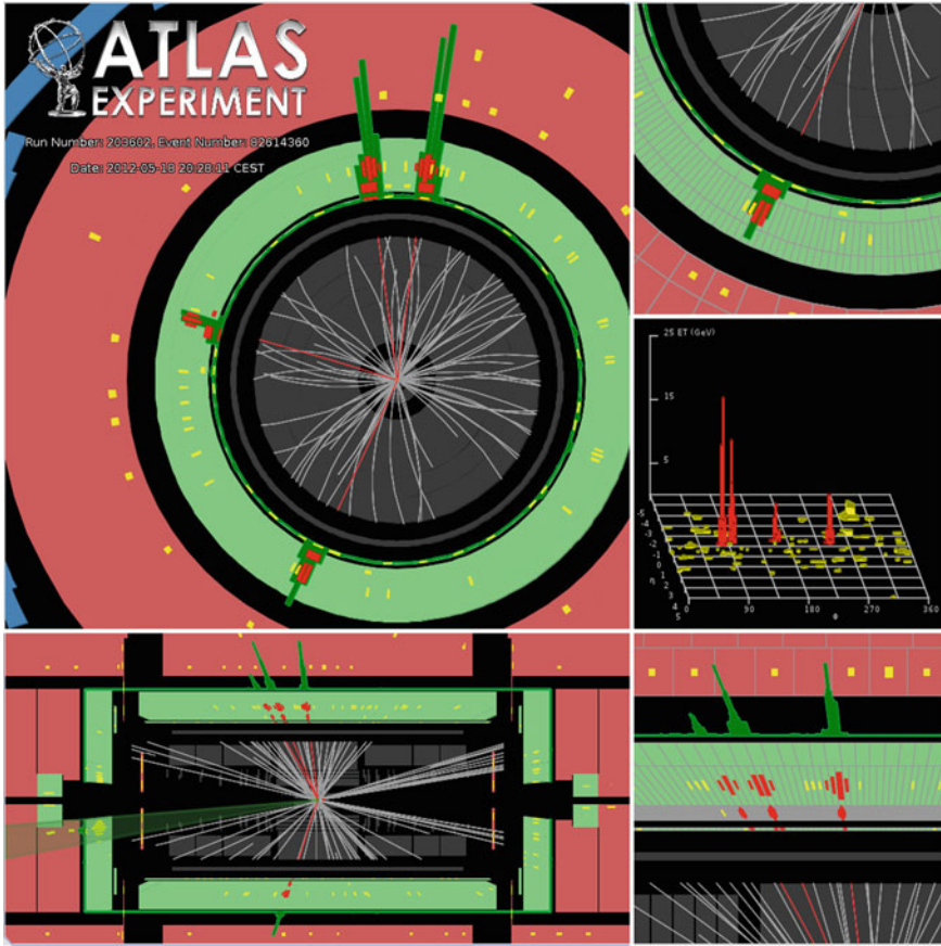
Fig. 12.1 Event display of a selected H \rightarrow ZZ^{(*)} \rightarrow llll event with four identified electrons. The electrons are shown in red and correspond to localized high energy deposits in the calorimeter matched to tracks in the inner detector, indicated by the red lines . The electrons have a combined invariant mass of 124.6 GeV. The upper-left panel shows the projection of the detector in the plane perpendicular to the beam line. The lower-left panel shows the projection of the detector along the beam line, running left to right in the panel. The upper-right and lower-right panels are zoom-ins of interesting regions. The middle-right panel depicts the energy deposited in the calorimeters as a function of \phi and \eta
