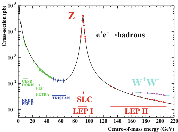
Fig. 1.1 The hadronic cross-section in electron-positron collisions as a function of center-of-mass energy. The solid line is the prediction of the SM, and the points are the experimental measurements. Also indicated are the energy ranges of various e^+e^- accelerators. The cross-sections have been corrected for the effects of photon radiation
