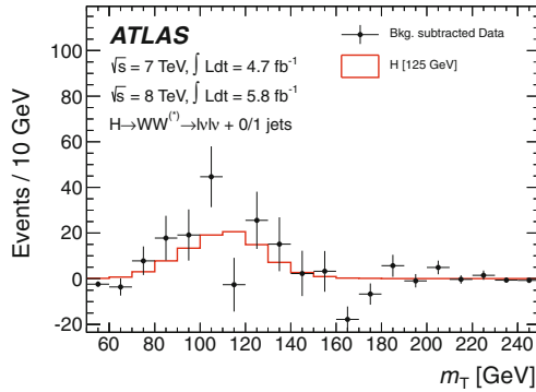
Fig. 11.23 The m_T distribution in data with the estimated background subtracted, overlaid with the predicted signal for m_h = 125 GeV. The distributions are summed for the 0-jet and 1-jet analyses and for the 2011 and 2012 analyses. The statistical errors of both the data and the subtracted background are reflected in the data points. The systematic uncertainty on the background estimate is not included
