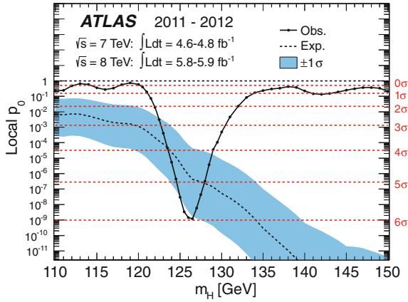
Fig. 12.14 The observed and expected p_0 as a function of m_h in the low mass range for the combined Higgs search. The dashed curve shows the corresponding expectation for p_0 for the signal+background hypothesis at the given values of m_h ; the blue band gives the \pm 1 one sigma region. The horizontal dashed lines indicate the p -values corresponding to 1 to 6 sigma
