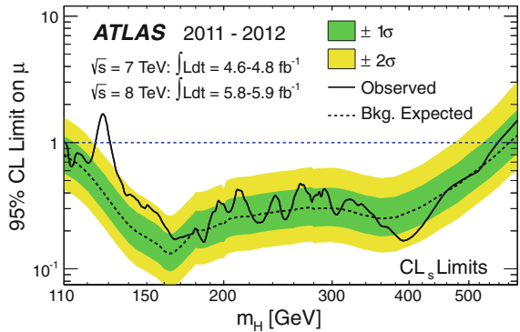
Fig. 12.17 The observed (solid) 95 % CL upper limit on the signal strength as a function of m_h . The dashed line gives the expected exclusion under the background-only hypothesis. The green and yellow shaded bands give the one and two sigma uncertainties on the expected exclusion
