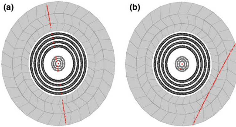
Fig. 5.9 Examples of tracks from cosmic-ray muons with track topologies different from that seen in collision events. a Shows an example of a cosmic-ray muon which correlates the upper and lower parts of the ID barrel. b Shows an example of a cosmic-ray muon which correlates detector elements in the TRT that are not correlated by tracks from collision events
