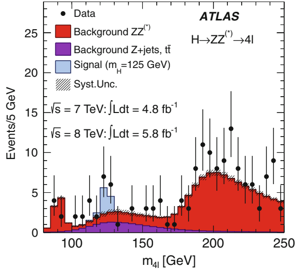
Fig. 12.2 The four-lepton invariant mass distribution, m_{4l} , for selected events in the H \rightarrow ZZ^{(*)} \rightarrow llll analysis using the combined 7 and 8 TeV data sets. The observed data is compared to the background expectation. The signal expectation for a SM Higgs with m_H = 125 GeV is shown
