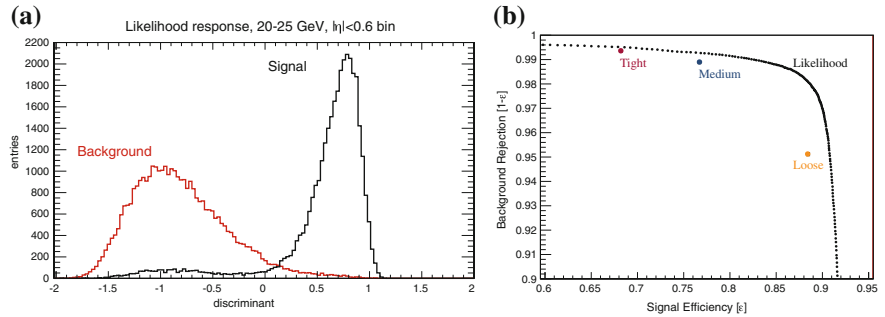
Fig. 7.19 Preliminary results from an implementation of a likelihood for electron selection. Left-hand plot shows the likelihood discriminate for signal and background electrons. Right-hand plot shows the performance of the likelihood with respect to the isEM++ operating points
