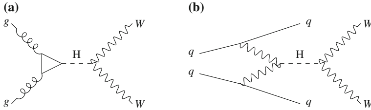
Fig. 8.1 Leading-order Feynman diagrams for H \rightarrow WW production. a The gluon-fusion diagram proceeds via top-quark loop. b The vector-boson fusion diagram results in a final state with WW+2 jets
