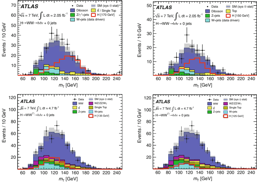
Fig. 8.15 Transverse mass distribution after H \rightarrow WW^{(*)} signal selection, for various values of Higgs mass. The result for a Higgs mass of 170 GeV is shown in the top left , 150 GeV in the top right , 135 GeV in the bottom left , and 125 GeV in the bottom right
