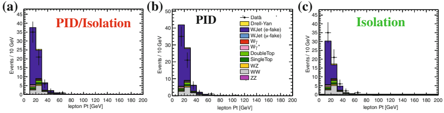
Fig. 9.29 Test of W +jet modeling in the “Tight-Inter-Iso” validation region defined in Table 9.9. Sub-leading p_T distribution is shown for events in the \mu e -channel. The W +jet predictions are made with the fake factor procedure using: a the “Pid-And-Iso”-denominator definition, b the “Pid”-denominator definition, and c the “Isolation”-denominator definition. Results are from the 5.8 \text{ fb}^{-1} 7 \text{ TeV} data set
