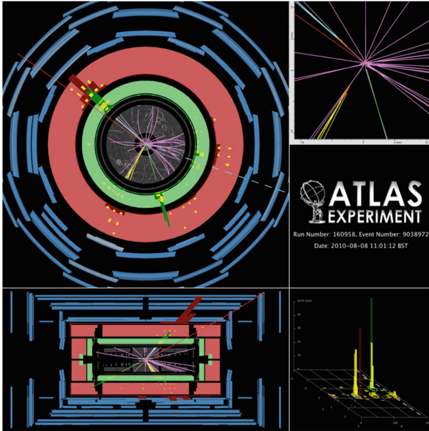
Fig. 4.2 Event display of a t\bar{t} -di-lepton candidate in the e\mu -channel with two b-tagged jets. The electron is shown by the green track pointing to a calorimeter cluster, the muon by the long red track intersecting the muon chambers, and the E_T^{\text{miss}} direction is indicated by the blue dotted line in the x-y view. The secondary vertices of the two b-tagged jets are indicated by the orange ellipses in the upper right
