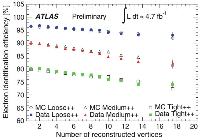
Fig. 7.17 Efficiency of the isEM++ operating points as a function of the number of primary vertices. The efficiency was determined using the tag-and-probe technique in Z \rightarrow ee events. Error bars include statistical and systematic uncertainties
