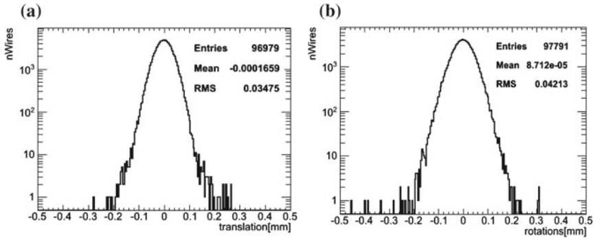
Fig. 6.45 Distribution of measured wire misalignment in the TRT Barrel. The measured translation displacements are given in the left . The measured rotation displacements, defined as \frac{dx_1 - dx_2}{2} , are given on the right
