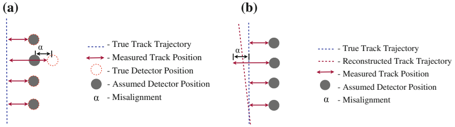
Fig. 5.2 Schematic of track reconstruction in the presence of detector misalignment. a Shows the measurements caused by the trajectory of a charged particle with detector misalignment indicated by \alpha . b Shows the reconstructed trajectory using those measurements and assuming no misalignment. The reconstructed trajectory differs from the charged particle trajectory
