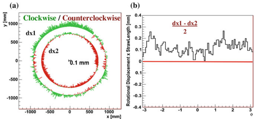
Fig. 6.42 Visual representation of wire-level misalignment in a 4-plane wheel with twist-deformation-like biases in the residual map. a Gives the measured alignment of each wire with respect to position in the wheel. b Shows the measured rotation of each wire as a function of \phi position in the wheel. A correlation in the wire-level alignment indicative of an twist deformation is seen
