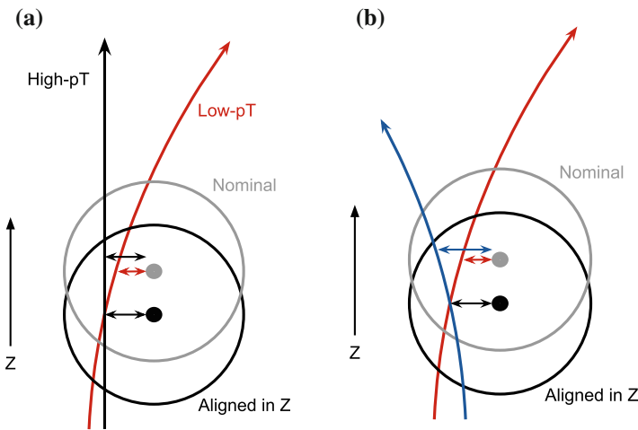
Fig. 6.49 Sketches of the effect of a z-misalignment in the end-caps [9]. The misalignment effects low p_T tracks (a) and positively and negatively charged tracks in the opposite direction (b)
