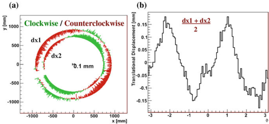
Fig. 6.41 Visual representation of wire-level misalignment in a 4-plane wheel with elliptical-deformation-like biases in the residual map. a Gives the measured alignment of each wire with respect to position in the wheel. b Shows the measured displacement of each wire as a function of \phi position in the wheel. A correlation in the wire-level alignment indicative of an elliptical deformation is seen
