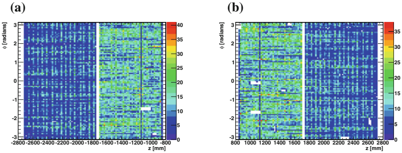
Fig. 6.12 Map of the TRT hits from combined ID tracks in collision data. The figures show the number of hits on track as a function of z and \phi , for end-cap C (a) and end-cap A (b)
