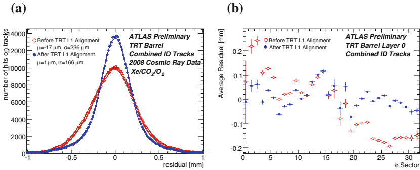
Fig. 6.9 a Comparison of the TRT residual for combined tracks before and after the L1 alignment. b Comparison of the average residual of combined tracks versus \phi -sector for barrel modules in the first layer, before and after the L1 alignment
