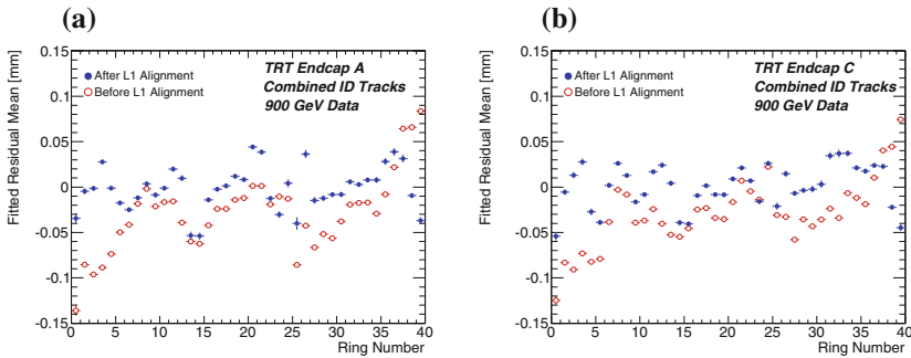
Fig. 6.14 Mean of the fitted TRT residual distribution as a function of end-cap 4-plane wheel (denoted ring in the figures) before and after the L1 alignment. End-cap A is shown in (a) and end-cap C is shown in (b)
