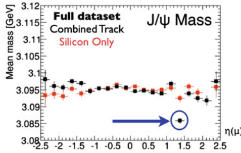
Fig. 6.48 Reconstructed J/\psi mass as a function \eta from tracks with only Pixel and SCT measurements (“Silicon Only”) and including TRT measurements (“Combined Tracks”) [8]
