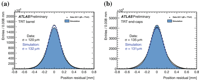
Fig. 6.54 TRT residual distribution after the alignment presented in this chapter for hits the barrel ( left ) and end-cap ( right ). The expectation from a perfectly aligned detector in simulation is provided
