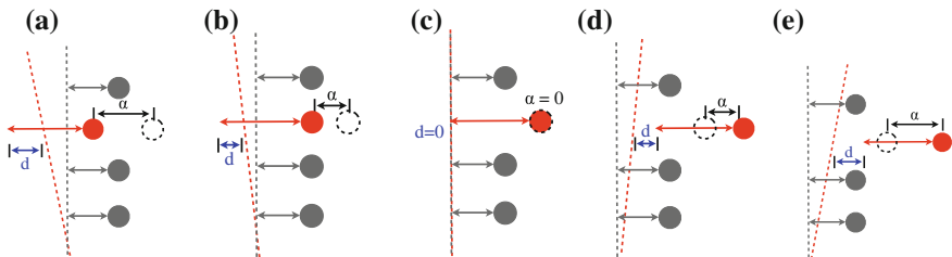
Fig. 5.5 Sketch of how track quality is effected by detector misalignment. a–e Show various alignments of the second detector element and the resulting track fits, indicated by the dashed red line . When the detector misalignment, indicated by \alpha , is larger, the distance of the track fit to the hits, indicated by d for the second hit, is correspondingly larger
