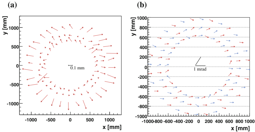
Fig. 6.18 Visual representation of the result of the L2 barrel alignment. a Visual representation of the translation alignment parameters. Each arrow represents a barrel module. The tail of the arrow is the nominal module position. The arrow length and direction represent the measured x and y alignment parameters. The arrow lengths are enlarged by a factor of 1,000 relative to the axes. A scale is provided for reference. b Visual representation of the rotations about z . Each arrow represents a barrel module. The size of the rotation is given as the angle the arrows make with respect to the positive x -axis. The arrow length has no meaning. The size of the rotations are enlarged by a factor of 1,000. A scale is provided for reference
