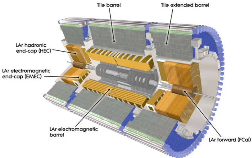
Fig. 3.4 Cut-away view of the ATLAS calorimeter system
