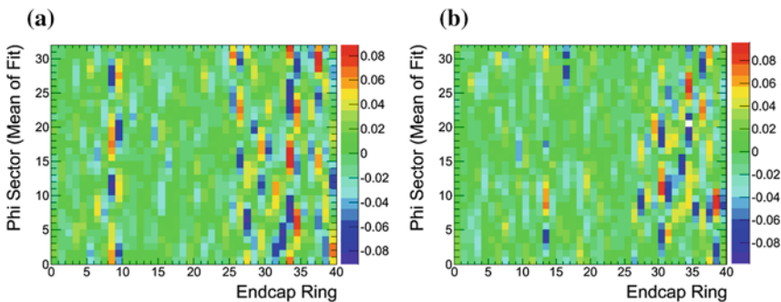
Fig. 6.35 Mean of the fitted residual distribution (in [mm] indicated by the color) versus end-cap 4-plane wheel (x-axis) and \phi (y-axis). The results for end-cap C are shown on the left , whereas those for end-cap A are presented in the right
