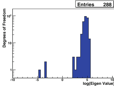
Fig. 6.16 The eigenvalue spectrum of the second derivative matrix for the L2 alignment with TRT-Only tracks. The three trivially unconstrained DoF are identified as orders of magnitude smaller than the others
