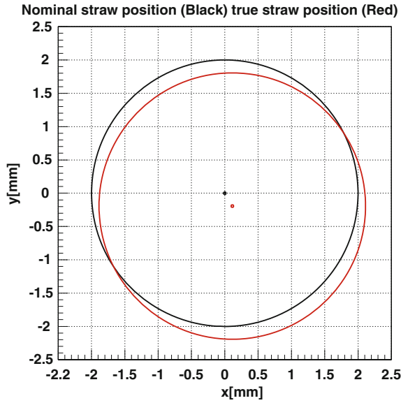
Fig. A.1 Description of a straw. The nominal position is at the origin, misalignment is seen in red
