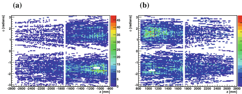
Fig. 6.11 Map of the TRT hits from combined ID tracks in cosmic-ray data. The figures show the number of hits on track as a function of z and \phi , for end-cap C (a) and end-cap A (b)
