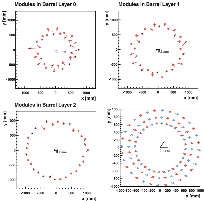
Fig. 6.28 Visual representation of the differences in translation alignment parameters when aligning A-side only and C-side only. Each arrow represents a barrel module. For the upper two plots and for the one on the lower left , the tails of the arrows are the module position after alignment with C-side only. The arrow-heads are the module positions after alignment with A-side only. The arrow lengths are enlarged by a factor of 1,000 relative to the axes. The modules in each layer are shown separately for clarity. Scales are provided for reference. The plot in the lower right is a visual representation of the differences in rotations. Each arrow represents a barrel module. The difference in the rotation is given as the angle the arrows make with respect to the positive x-axis. The arrow length has no meaning. The size of the rotations are enlarged by a factor of 1,000. A scale is provided for reference
