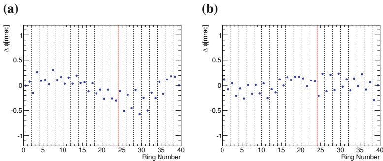
Fig. 6.29 Visualization of measured rotations about z with the alignment using cosmic-rays. The measured misalignment in \phi is plotted as a function of 4-plane wheel number. The solid red lines give the separation of the Type-A and Type-B wheels, and the dashed vertical black lines give the separation of the 8-plane Type-A and Type-B type wheels. The results for end-cap C are shown on the left, whereas those for end-cap A are presented in the right
