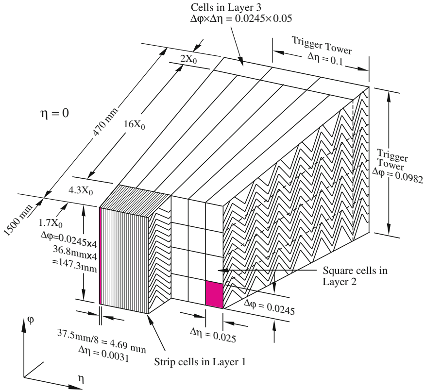
Fig. 3.5 Sketch of section of the LAr EM barrel where the different layers are clearly visible. The granularity in \eta and \phi of the cells of each of the three layers is shown
