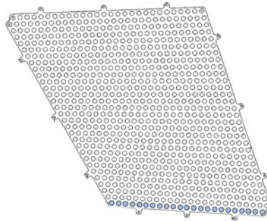
Fig. 6.2 Schematic of a Type II TRT barrel module. The circles represent individual straws, which are all oriented parallel to the beam line. The z -axis (beam pipe) is in the direction coming out of the page. The first layer of straws is highlighted in blue at the bottom
