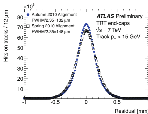
Fig. 6.38 TRT residual distributions in the end-cap before and after the L3 end-cap alignment. The “Autumn 2010 Alignment” includes the L3 alignment, the “Spring 2010 Alignment” uses the TRT geometry before the L3 alignment
