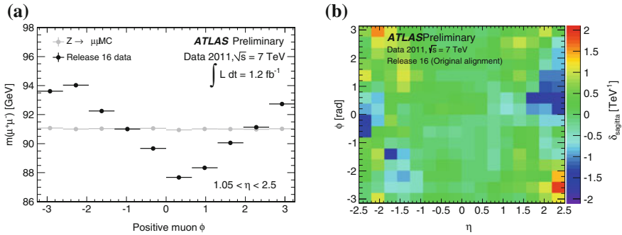
Fig. 5.17 Evidence for the presence of detector weak modes after alignment. a Shows the mean of the reconstructed Z invariant mass using ID tracks in Z \rightarrow \mu\mu events as a function of the \phi of the positive muon, for tracks in end-cap A. b Shows the measured sagitta bias using W \rightarrow e\nu events as a function of the electron \eta and \phi . No bias is expected from a properly aligned detector
