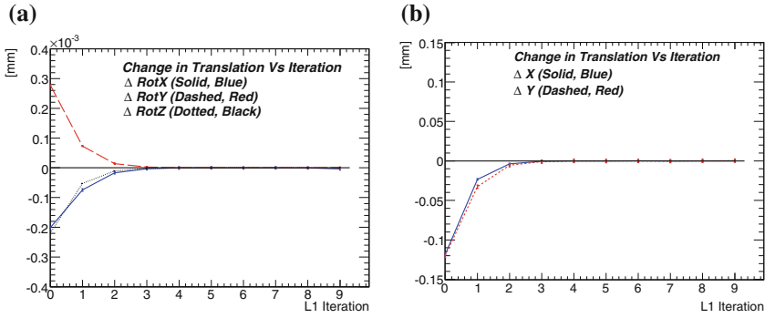
Fig. 6.8 Convergence of the L1 barrel alignment parameters. The changes in the alignment DoF versus iteration: a shows the convergence of the rotational DoF and b shows the convergence of the translation DoF
