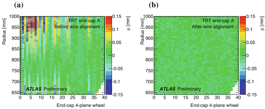
Fig. 6.40 Mean of a Gaussian fit to the TRT residuals versus radius and wheel before (a) and after (b), the wire-level alignment. The plots illustrate the results for end-cap A. The white area in the lower right corner is due to acceptance effects
