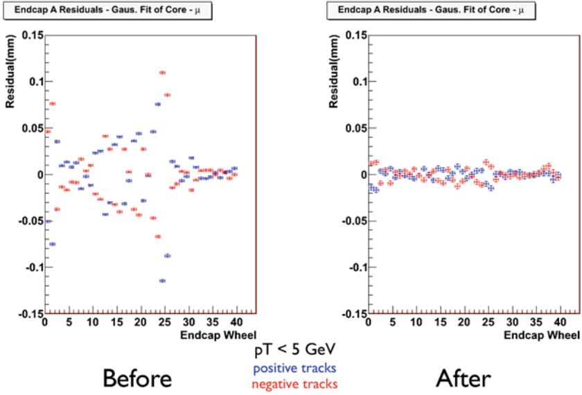
Fig. 6.52 Average residual versus wheel in end-cap A [7]. Positively and negatively charged tracks are shown separately and are required to have p_T below 5 GeV. The result before the end-cap z-alignment are shown on the left , whereas, the result after the z-alignment is shown in the right
