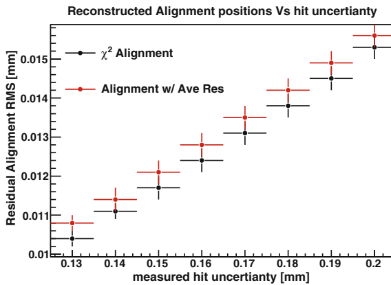
Fig. A.8 RMS of residual misalignments as a function of the hit resolution used
