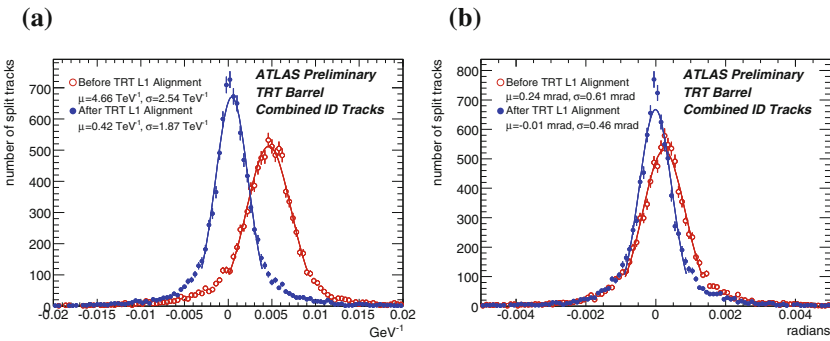
Fig. 6.10 Validation of the L1 alignment with split tracks. Comparison of the \frac{q_T}{p_T} (a) and the \phi_0 (b), difference of split tracks before and after the L1 alignment
