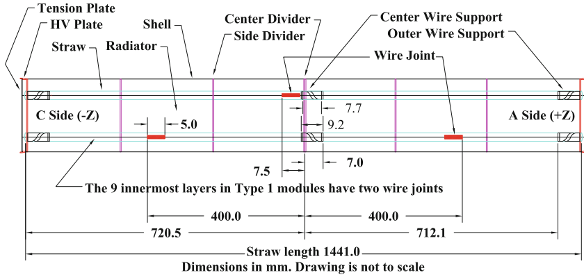
Fig. 6.3 Schematic of a TRT barrel module along z . The wires are connected, but electronically split in the center of the barrel modules
