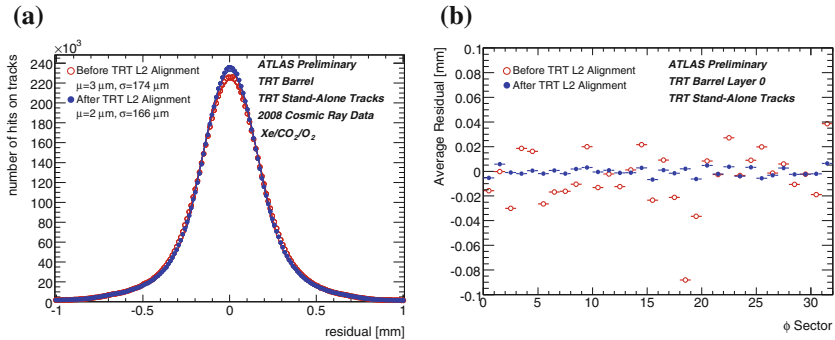
Fig. 6.19 TRT residuals before and after L2 alignment. a Comparison of TRT residual for TRT stand-alone tracks before and after L2 alignment. b Comparison of the average residual of TRT stand-alone tracks versus \phi -sector for barrel modules in the first module layer, before and after L2 alignment
