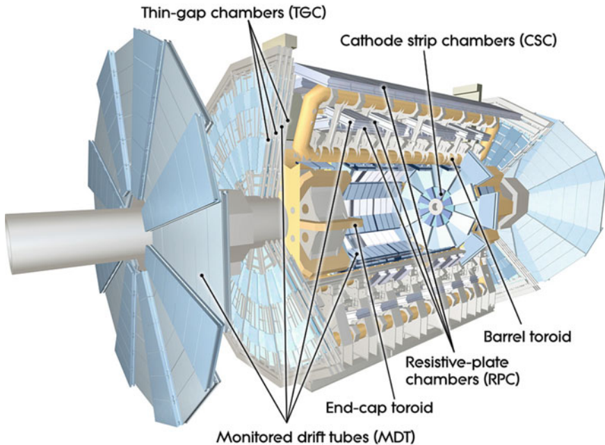
Fig. 3.6 Cut-away view of the ATLAS muon system
