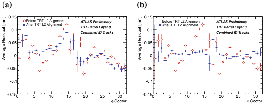
Fig. 6.25 Comparison of the average residual of combined tracks versus \phi -sector for barrel modules in layer zero before and after the TRT stand-alone L2 barrel alignment (a), and before and after the L2 barrel alignment including silicon information (b)
