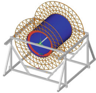
Fig. 6.3 Schematic of a TRT barrel module along z . The wires are connected, but electronically split in the center of the barrel modules
