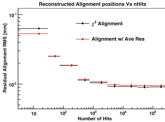
Fig. A.7 RMS of residual misalignments as a function of number of hits used in alignment
