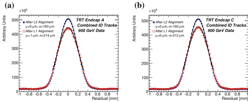
Fig. 6.34 TRT residual distributions before and after the L2 end-cap alignment for end-cap A (a) and end-cap-C (b)
