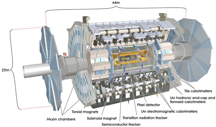
Fig. 3.1 Cut-away view of the ATLAS detector
