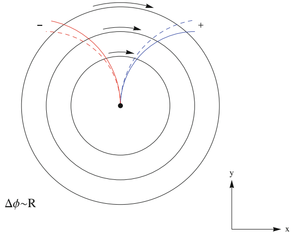
Fig. 5.7 Sketch of the curl deformation, a weak mode that biases the reconstructed track p_T . The detector elements are misaligned in \phi with a magnitude that is proportional the radial position, as indicated by the arrows. The effect on the curvature for a positively and negatively charged track are shown
