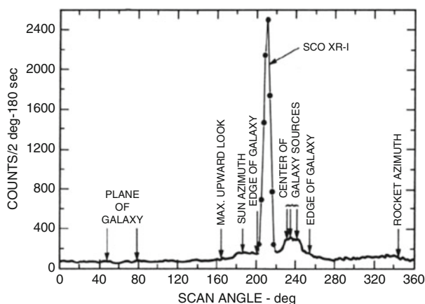
Fig. 9.3 Three minutes of a scan from a rocket-borne X-ray detector made in 1967 showing how the source Sco X-1 stands out above the emission from the Milky Way. ©American Astronomical Society, from ApJ 154, 655 (1968)
