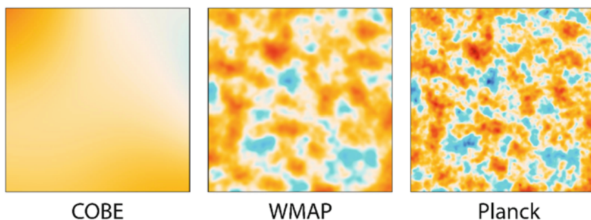
Fig. 7.12 The same 10 square degree patch of sky as seen by the COBE, WMAP, and Planck satellites. Image credit: ESA/NASA/JPL-Caltech
