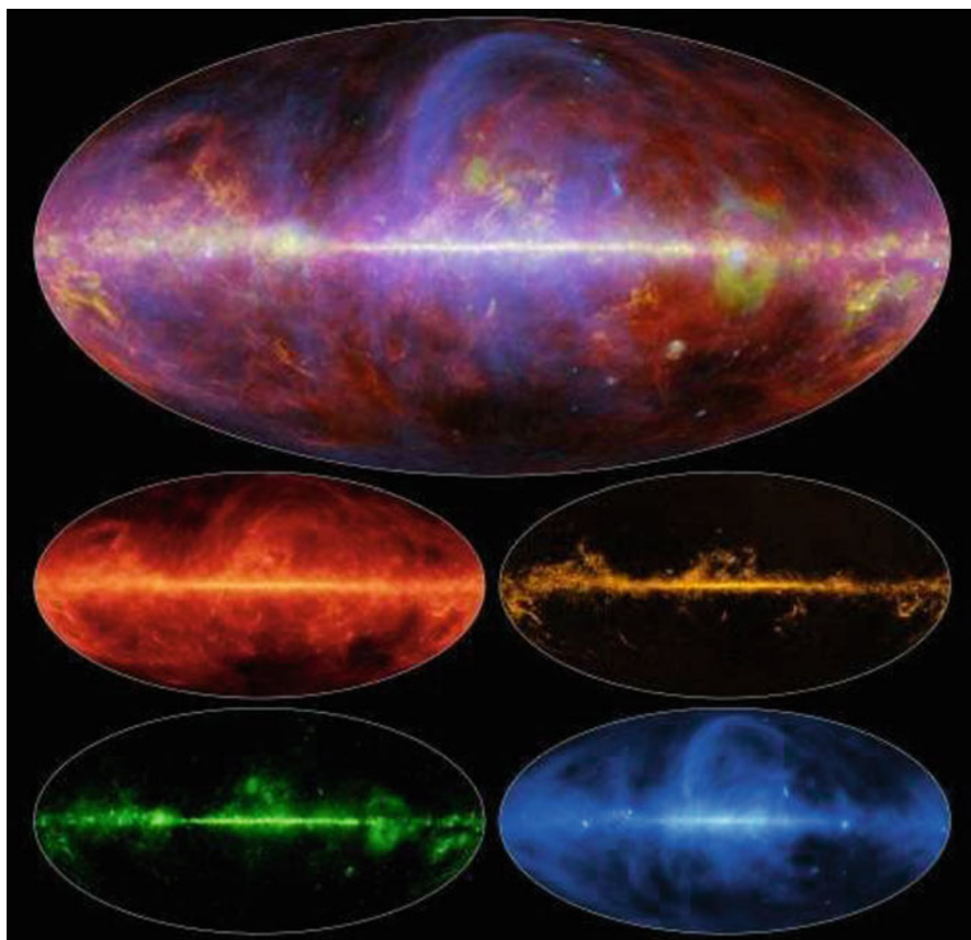
Fig. 7.10 Emission from the Milky Way galaxy as measured by the Planck spacecraft. Red color indicates emission from warm dust grains, yellow shows carbon monoxide gas, blue represents synchrotron radiation, and green is radiation from hot ionized gases such as those in the Orion Nebula. The top map is a combination of these radiation sources. Image credit: ESA/NASA/JPL-Caltech
