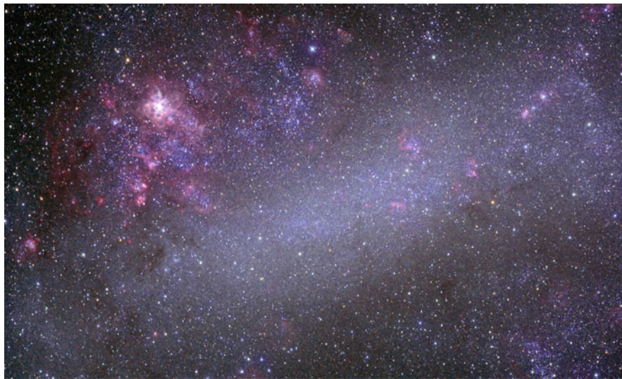
Fig. 13.9 The Large Magellanic Cloud. Image credit: Axel Mellinger, Central Michigan University
