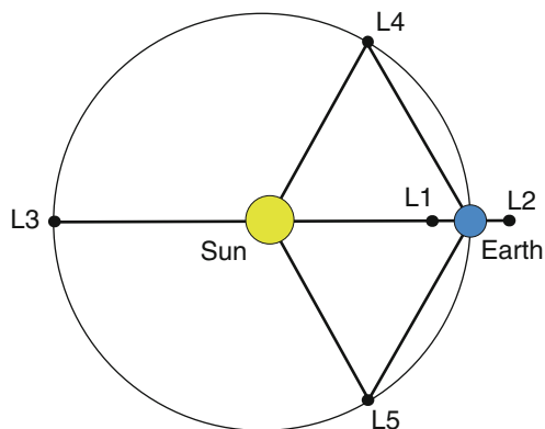
Fig. 7.7 The five Lagrangian points of the Sun-Earth system
