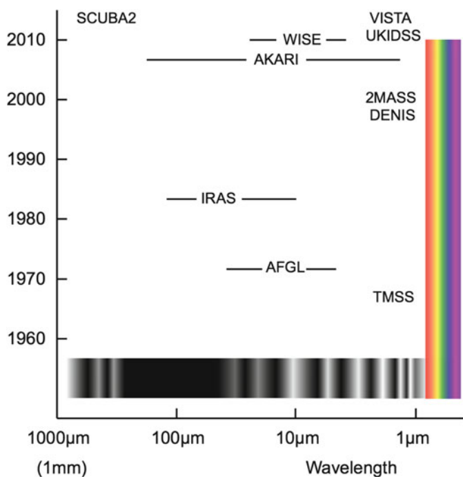
Fig. 6.1 Major infrared surveys sorted by approximate dates and wavelength ranges. The shaded bar near the bottom of the figure shows how the transparency of the atmosphere changes with wavelength: black means the atmosphere is opaque: white or gray indicates at least some transparency
