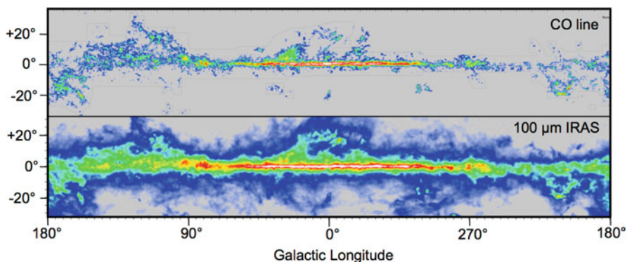
Fig. 5.15 Map of the 2.6-mm carbon monoxide emission from the plane of the Milky Way galaxy compared with a map of the 100-micron hot dust emission obtained by the IRAS infrared survey. Image ©American Astronomical Society, modified by author
