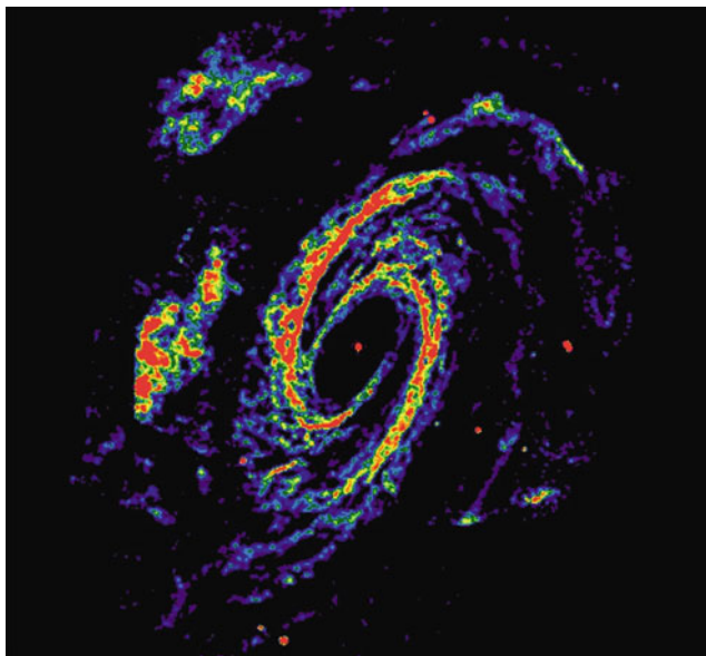
Fig. 5.12 21-cm line emission from the spiral galaxy M81. See Figure 8.3 for an image of the same galaxy at visible and ultraviolet wavelengths. Image credit: NRAO/AUI
