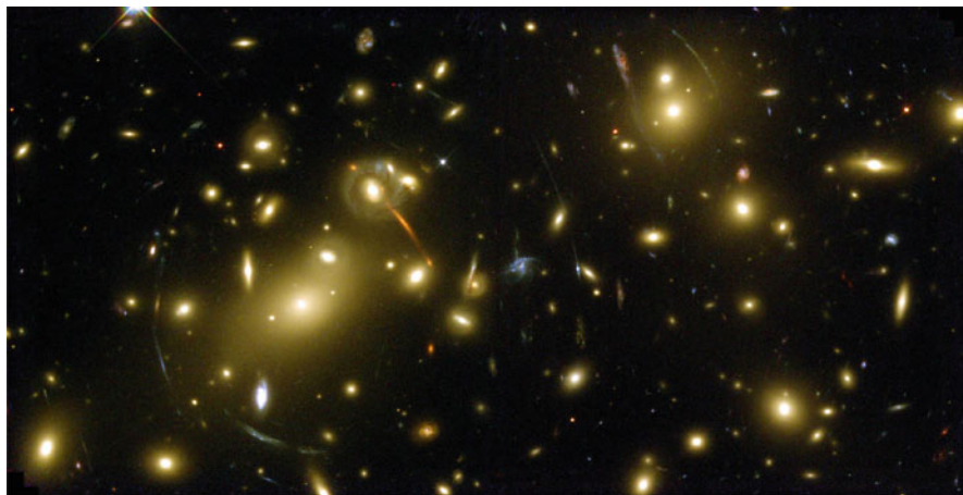
Fig. 13.7 Gravitational lensing of distant galaxies by a foreground galaxy cluster. Image credit NASA/ESA
