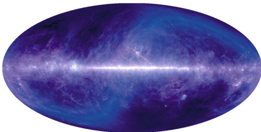
Fig. 6.8 Map of the sky by AKARI in galactic coordinates. Emission at 140\mu\text{m} is in blue and at 90\mu\text{m} is in cyan. The bright area in the galactic plane to the left of center is the Cygnus X star formation region. Infrared “cirrus” emission covers most of the sky. Image credit: Japanese Aerospace Exploration Agency and European Space Agency
