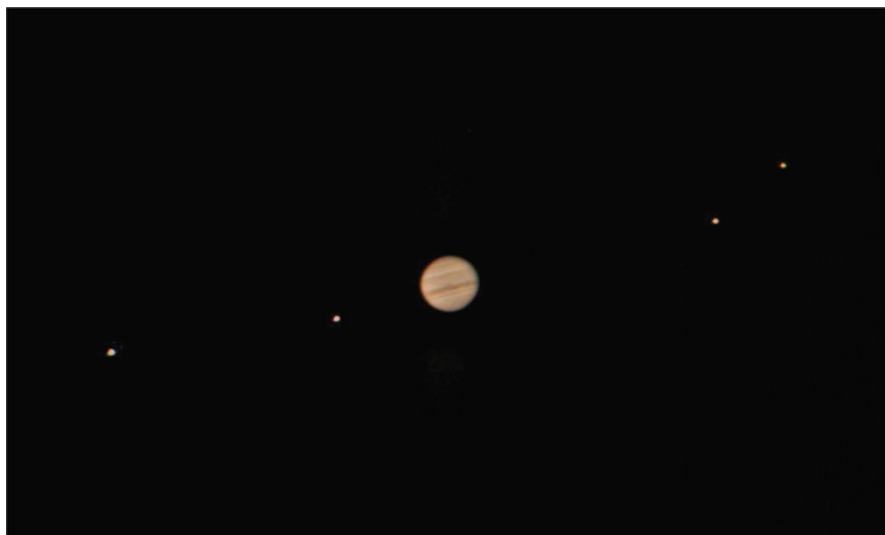
Fig. 3.3 Jupiter and its major moons as seen through a modern 25-cm telescope. Image credit: Jan Sandberg
