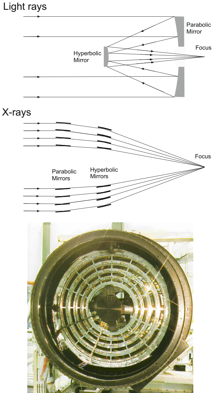
Fig. 9.7 Comparison between the optics of a conventional Cassegrain optical telescope ( top ) and a Wolter X-ray telescope ( middle ). The bottom image shows a face-on view of the 83-cm diameter concentric parabolic mirrors in ROSAT. Bottom image credit: Max-Planck-Institut für Extraterrestrische Physik
