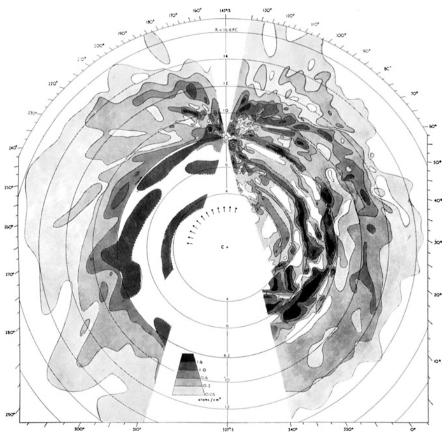
Fig. 5.11 The distribution of neutral hydrogen in the Milky Way galaxy as determined from 21-cm line observations in Netherlands and Australia in 1958. The V-shaped areas centered above and below the location of the Sun are left blank because the Doppler shifts of the line are too small to use. Image ©Royal Astronomical Society/Oxford University Press
