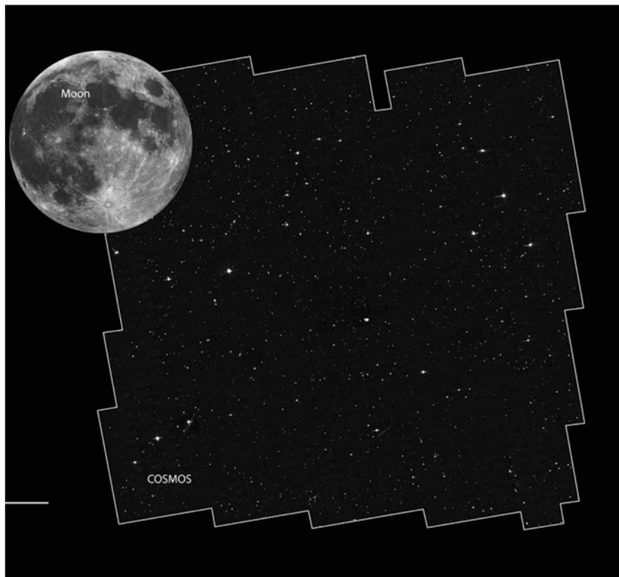
Fig. 13.5 The COSMOS field as observed by the Hubble Space telescope at a wavelength of 0.8\mu\text{m} in 2003–2004, with the size of the full moon for comparison. On this scale the Hubble Deep Field image (Figure 13.2) would be about 3 millimeters across. Image credit: NASA, ESA and Z. Levay (STScI)
