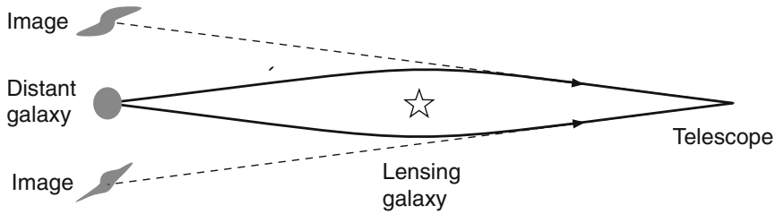
Fig. 13.6 Gravitational lensing of a distant galaxy by an intervening one
