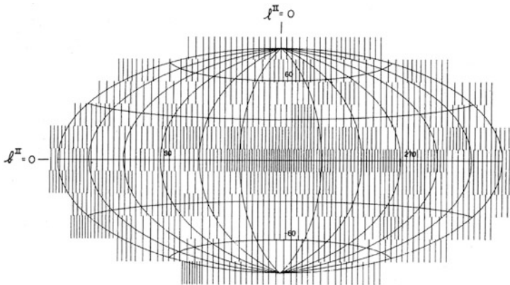
Fig. 10.2 OSO-3 map of the sky in galactic coordinates. The number of vertical bars indicates the strength of the emission in that direction ©American Astronomical Society, from ApJ 177, 341 (1972)
