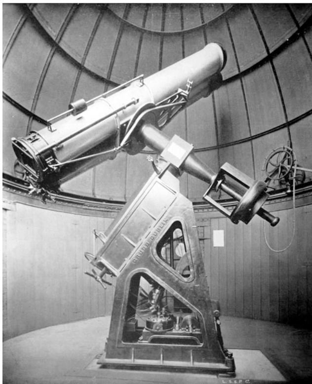
Fig. 4.3 One of the telescopes used to make the Carte du Ciel —the 13-inch astrograph at Greenwich Observatory, London in about 1900. Image credit: Graham Dolan
