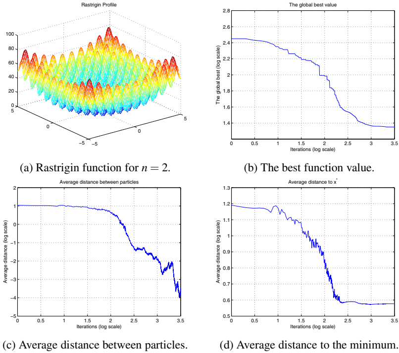
Fig. 12.11. Simulations for the Rastrigin benchmark function.
