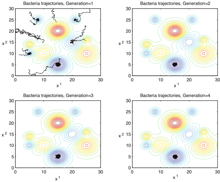
Fig. 11.5. Bacteria motion trajectories, generations 1–4, on contour plots, after an elimination-dispersal event.
