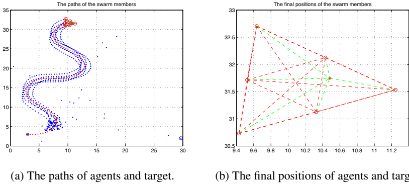
Fig. 6.7. A swarm of N = 6 agents with non-holonomic vehicle dynamics subject to external disturbances and model uncertainty tracking a moving target and forming an equilateral triangle formation.
