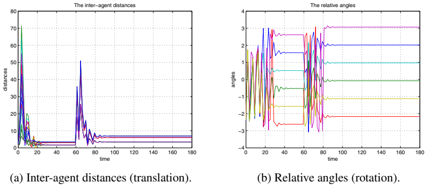
Fig. 7.9. Agent trajectories for a translation and relative angles for a rotation maneuvers.
