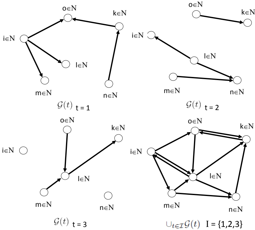
Fig. 12.6. Directed graph representation of Assumption 20
