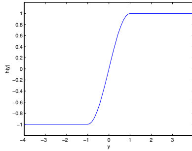
Fig. 6.2. Function h(\cdot) with \varepsilon = 1 .
