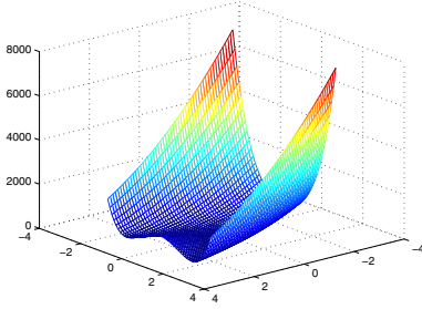
(a) Rosenbrock function for n = 2 .
