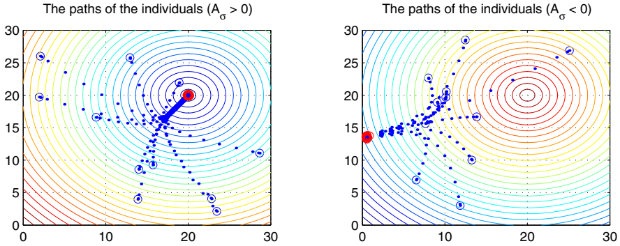
Fig. 3.5. Response for quadratic resource profile.
