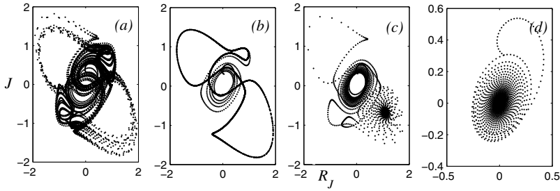
Fig. 1 Attractors of system (2) for q_1 = q_2 = q_3 = q_4 = \theta with the same parameters and initial conditions as in Fig.1: (a) \theta = 0.99 ;(b) \theta = 0.98 ;(c) \theta = 0.97 ;(d) \theta = 0.96 .
