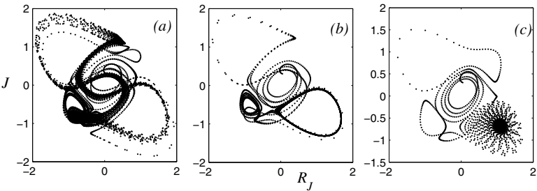
Fig. 2 Attractors of system (2) for q_2 = q_3 = q_4 = 1.0, q_1 = \theta with the same parameters and initial conditions as in Fig.1: (a) \theta = 0.99 ;(b) \theta = 0.985 ;(c) \theta = 0.98 .
