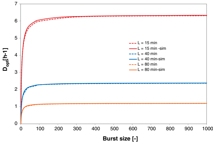
Figure 12.11 Effect of burst size ( b ) and latent period ( L ) on optimal dilution rate ( D_{\text{opt}} ). Comparison of results calculated from Equations 12.14 and 12.17.
