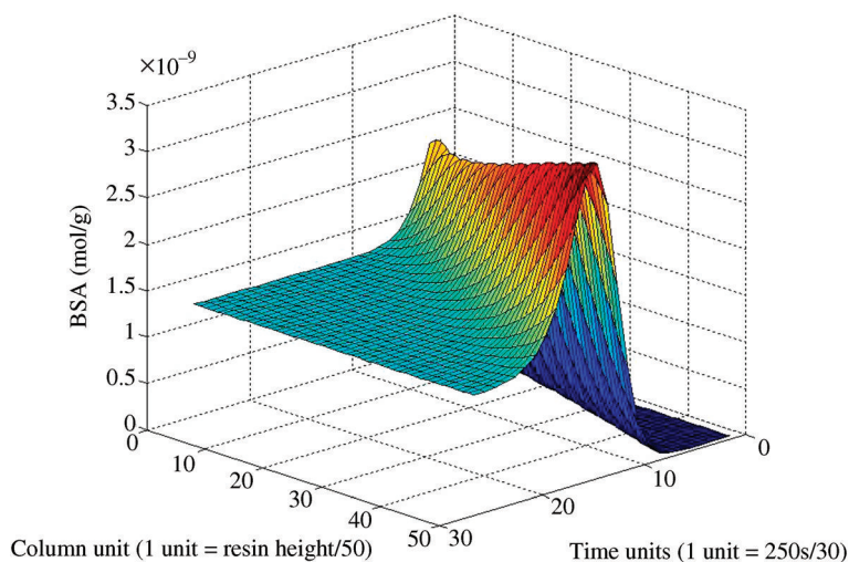
Figure 5.8 BSA distribution in column during binding.
