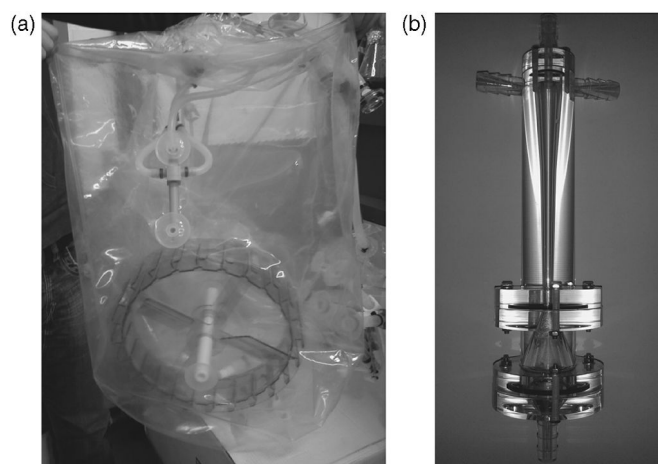
Figure 6.7 (a) Customized bag of an Air Wheel® bioreactor (PBS Biotech) incorporating a hydrocyclone (Sartorius); (b) Plexiglas® prototype of a hydrocyclone of novel geometry currently under development at LECC/Federal University of Rio de Janeiro.
