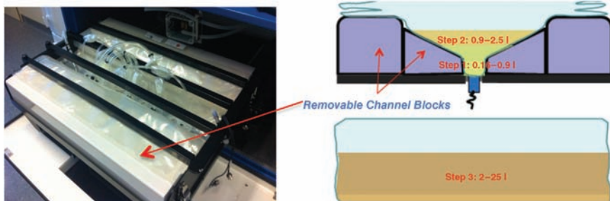
Figure 7.6 Expansion set CELL-tainer®.
