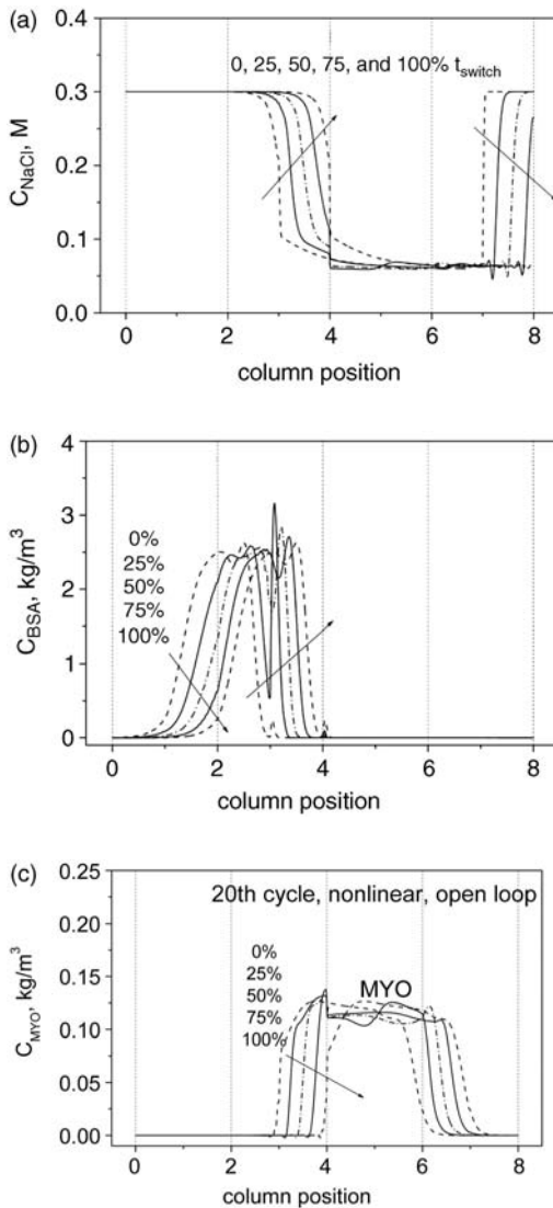
Figure 1.12 Cyclic steady state internal concentration profiles during a switch interval in salt gradient IE-SMB with open loop when C_S^F = 0.05 M NaCl and C_S^D = 0.3 M NaCl for BSA and myoglobin separation at nonlinear equilibrium isotherm.
