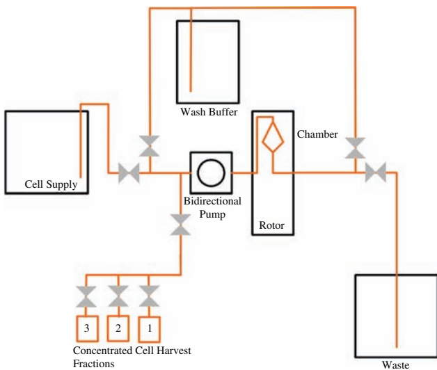
Figure 15.12 Automated concentration, media replacement, and harvest process.
