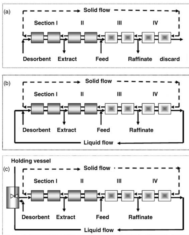
Figure 1.9 Operation modes for gradient IE-SMB: (a) gradient IE-SMB with open loop; (b) gradient IE-SMB with closed loop; (c) gradient IE-SMB with closed loop and a
