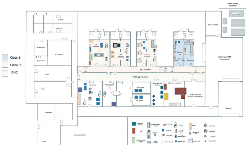
Figure 16.8 Process platform design for a 1000 l mAb facility (courtesy of G-CON LLC).
