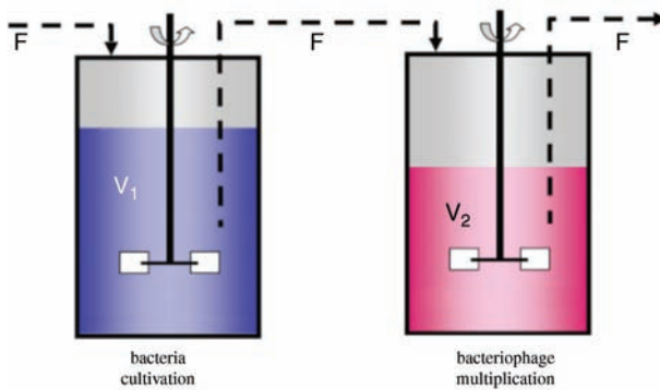
Figure 12.6 Schematic drawing of continuous system consisting of two bioreactors connected in series. While flow rate through the system is constant, volume in the second
