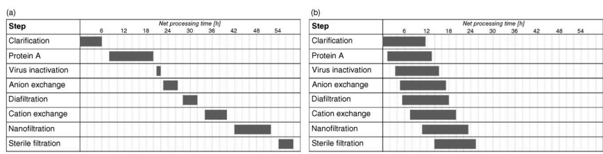
Figure 2.1 Typical DSP manufacturing schedules for (a) a cascade of batch-wise operated unit operations, and (b) an integrated continuous downstream process.
