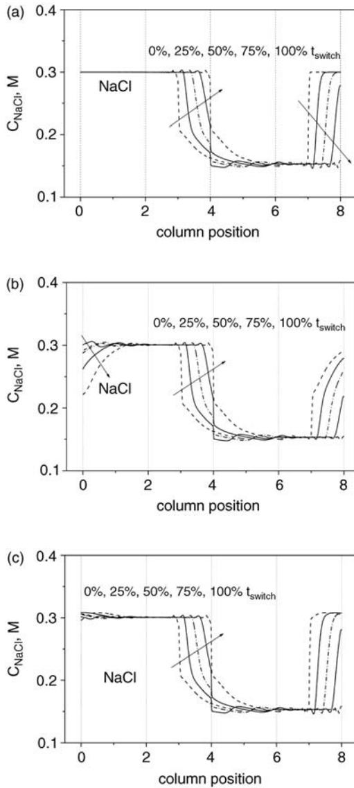
Figure 1.10 Salt gradient formations in IE-SMB chromatography with (a) open loop, (b) closed loop, and (c) closed loop with a holding vessel ( V_h = 10 ml). Reprinted from Ref. [121] with permission from John Wiley & Sons.
