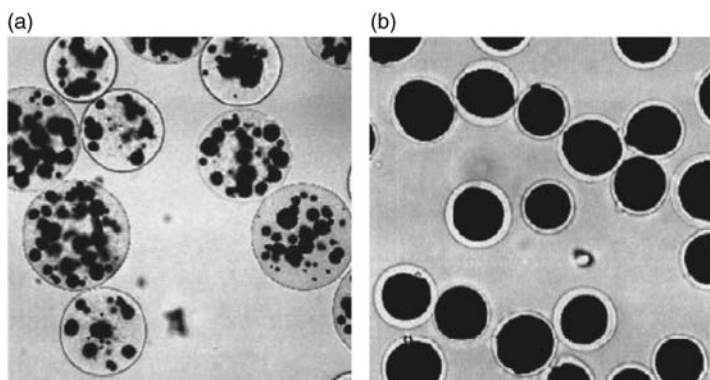
Figure 1.2 Adsorbents with a high-density matrix used in expanded bed. (a) Streamline DEAE/Streamline Direct CST I. (b) Pellicular adsorbent/inert core adsorbent.
