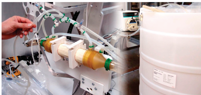
Figure 9.2 Single-use, continuous bioproduction with a single-use Thermo Scientific HyClone BioProcess Container and Drum (right) supporting culture in a FiberCell Systems LS-HFBR reactor (left).
