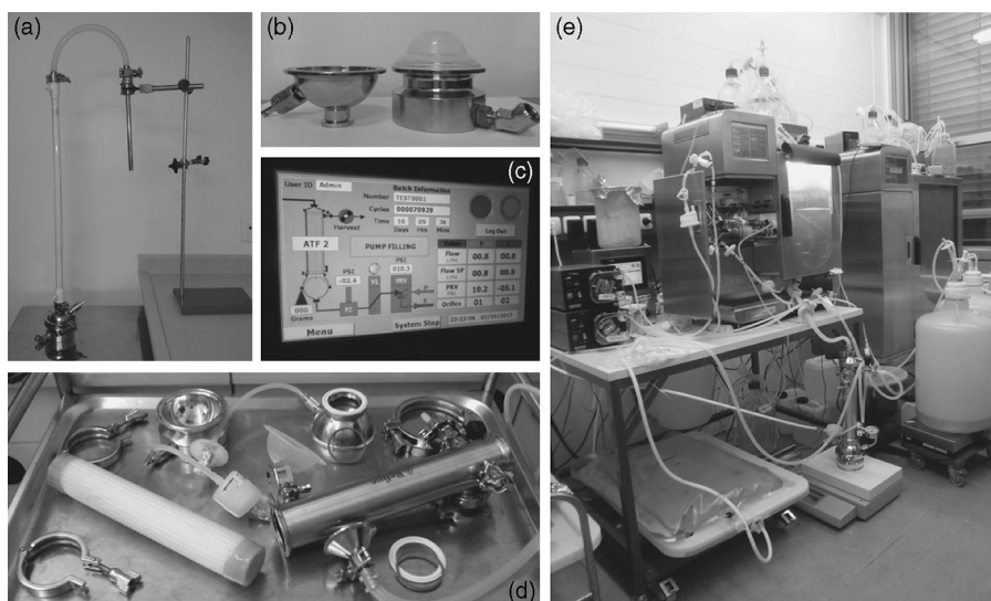
Figure 6.8 (a) ATF-2 system (Refine Technology); (b) detail of the diaphragm placed in the bottom part of the ATF-2 unit; (c) screen of ATF controller unit; (d) dismantled ATF-4 system showing its hollow-fiber cartridge; (e) ATF-4 system connected to a disposable Air-Wheel ® bioreactor (PBS Biotech). Photos taken by our group at the Federal University of Rio de Janeiro and at the University of Bielefeld.
