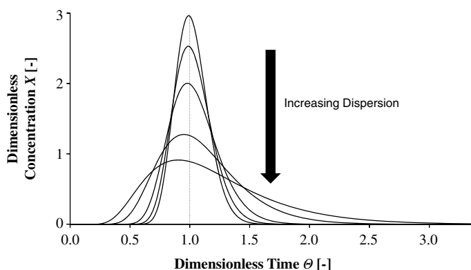
Figure 11.16 Simulated effluent curves from pulse tracer injections using the equation with increasing dispersion in the tube where \theta is dimensionless time ( \theta = t/\tau_{VL} = tv/L_{VL} ), v is the superficial fluid velocity, X is the dimensionless concentration ( X = C/C_0 ), and c_0 is the
