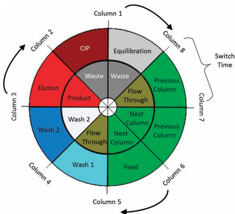
Figure 11.6 Circular chronogram example for bind and elute step with eight columns. The outer ring shows the feed solution of each column with columns 6, 7, and 8 in the loading zone (green) and columns 4 and 5 are in the wash zone and so on. The inner ring shows where the effluent of a column is directed.
