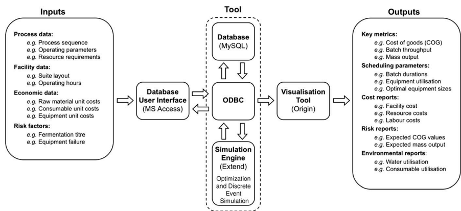
Figure 17.1 Overview of simulation tool structure highlighting key communication directionality and content with respect to key inputs and outputs. ODBC; open data base connectivity.
