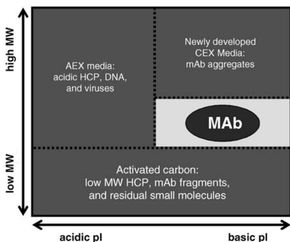
Figure 4.5 A schematic analysis of the various mAb process impurities based on their molecular weight and isoelectric point with examples of media types that can be employed for their selective removal.
