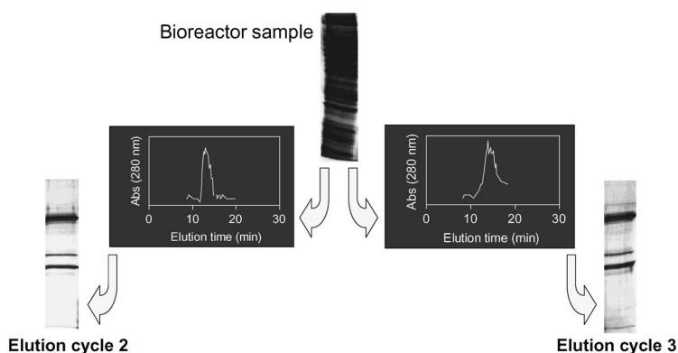
Figure 6.11 SDS-PAGE analysis under reducing conditions of eluates obtained in different elution cycles carried out during perfusion cultivation of CHO cells using a rotating disc filter
