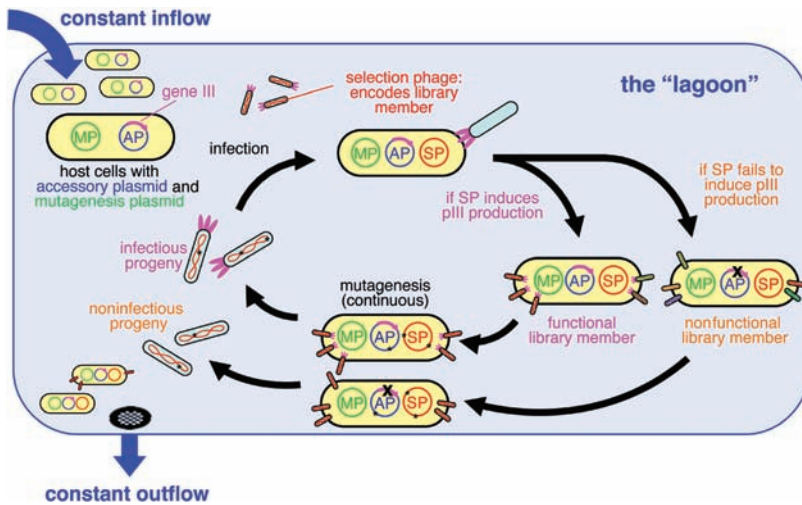
Figure 12.8 Schematic presentation of the system for continuous directed evolution of biomolecules. Bacterial cells continuously flow into bioreactor where they are infected with selection phase (SP) encoding library members. Functional library members induce production of pIII from the accessory plasmid (AP)
