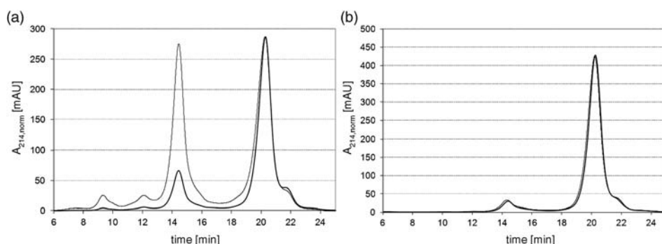
Figure 10.10 mAb isoform separation capabilities of MCSGP visualized for the case of Herceptin® using analytical cation exchange chromatograms. (a) Overlay of original Herceptin® (blue) and Herceptin® spiked with
