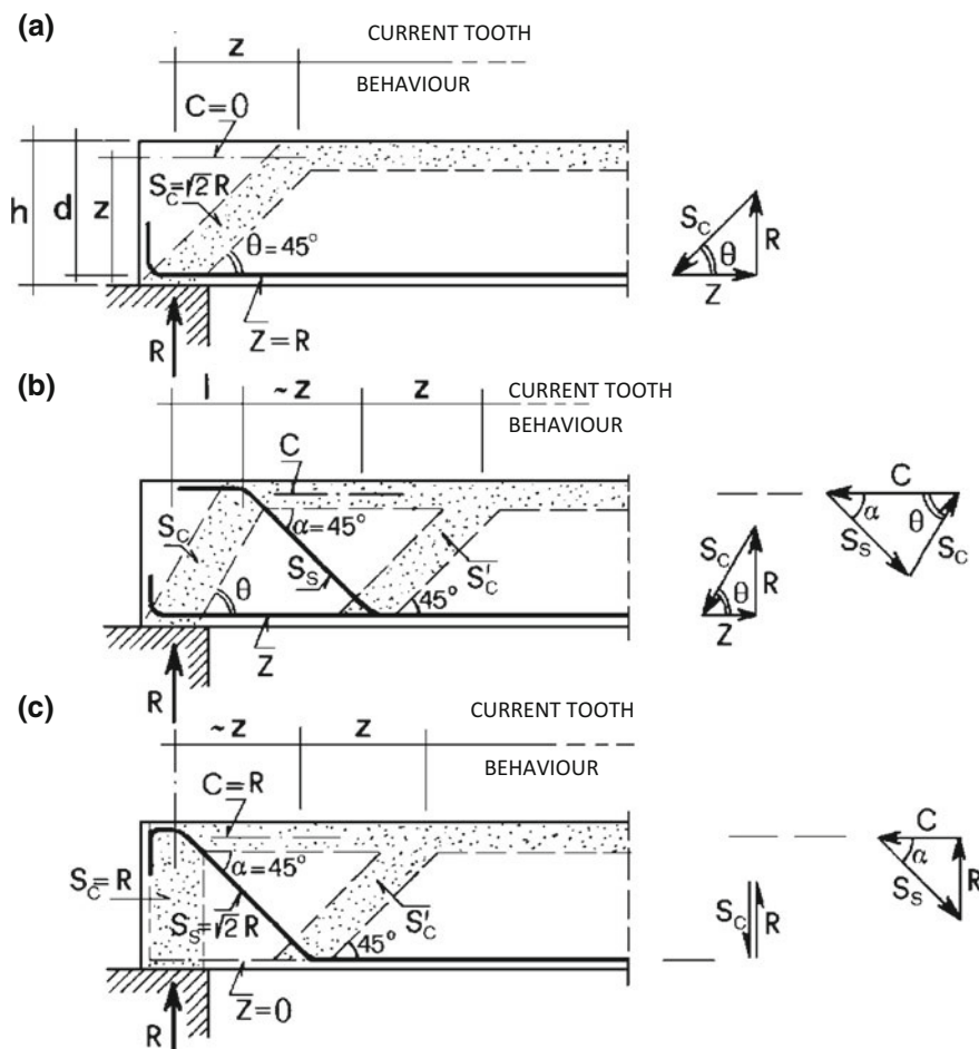
Fig. 5.17 Possible different details over the end support
