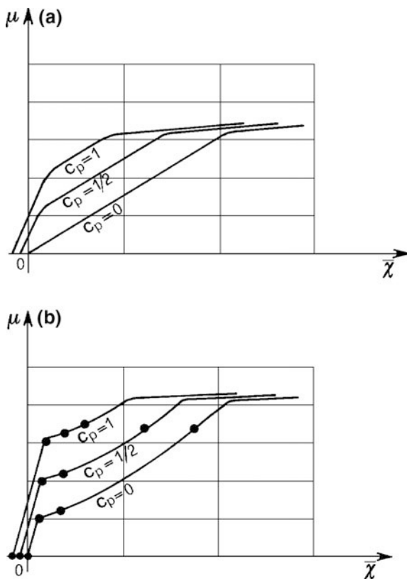
Fig. 3.39 Resistance (a) and deformation (b) diagrams with precompression
