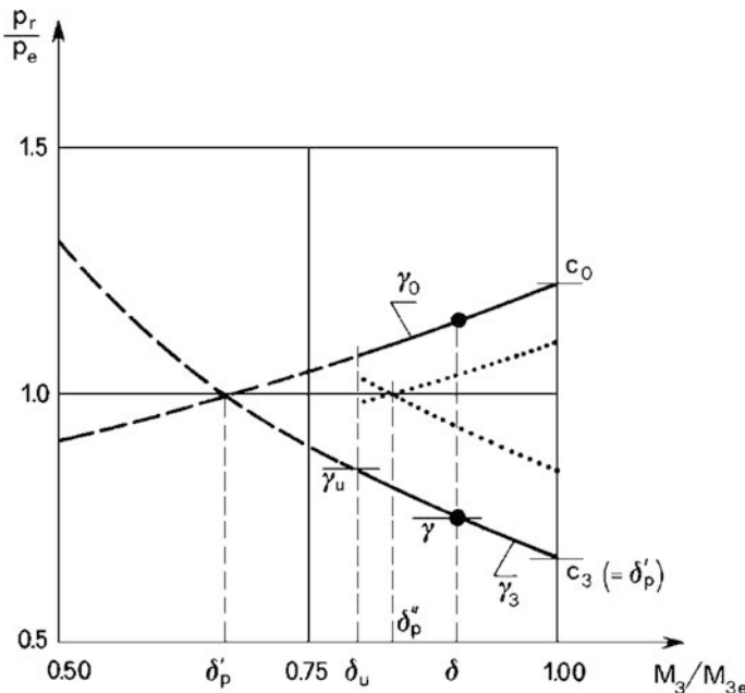
Fig. 5.46 Collapse factor \gamma for different moment redistributions
