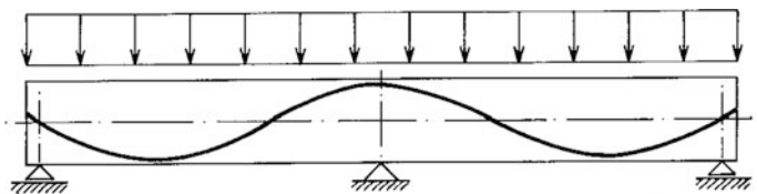
Fig. 10.22 Consistent tendon profile
