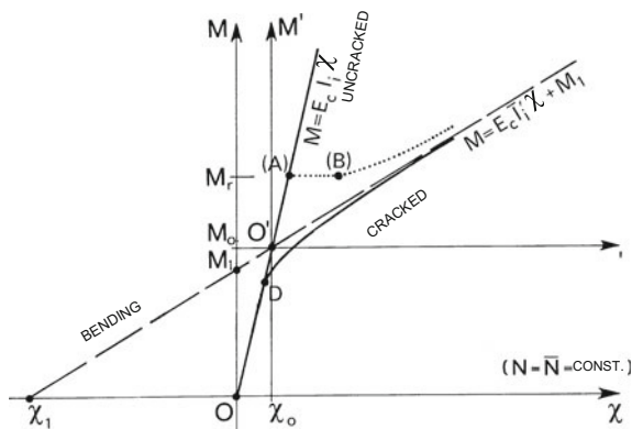
Fig. 6.30 Moment-curvature diagram for N = \text{const}
