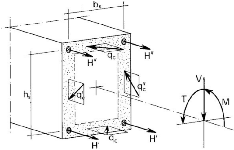
Fig. 8.14 Stress distribution under M, V, T interaction
