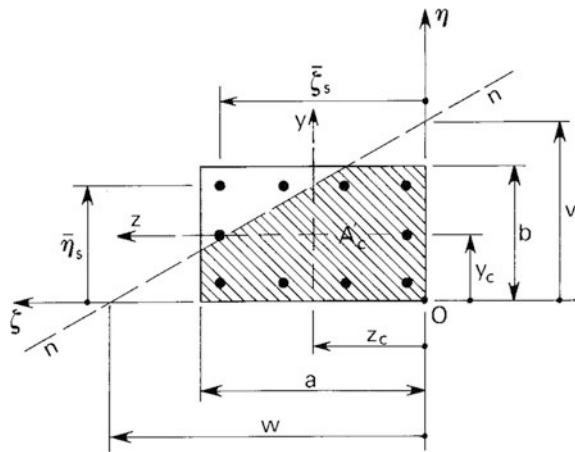
Fig. 6.23 Cracked section under axial action and biaxial bending
