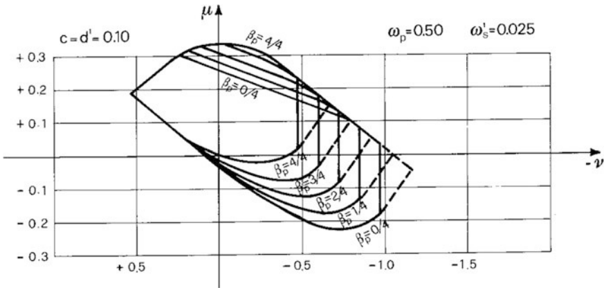
Fig. 6.17 Prestressing effects on the interaction curves
