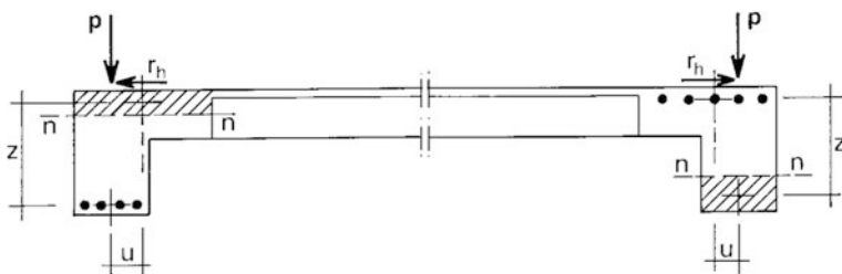
Fig. 6.9 Sections with horizontally restrained deformation
