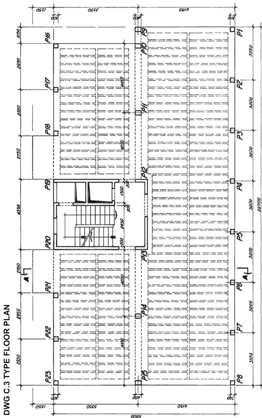
Fig. 2.19 Multistorey building—plan
