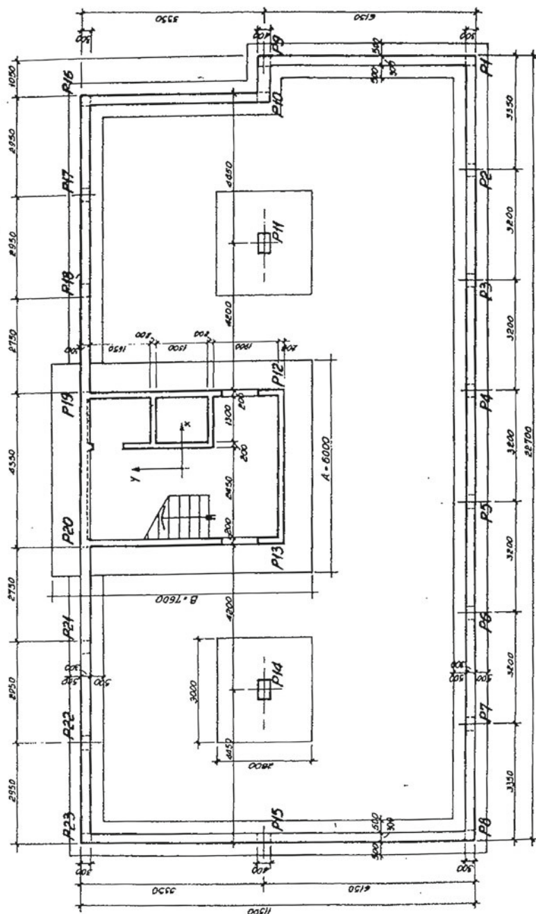
Fig. 9.50 Foundation layout
