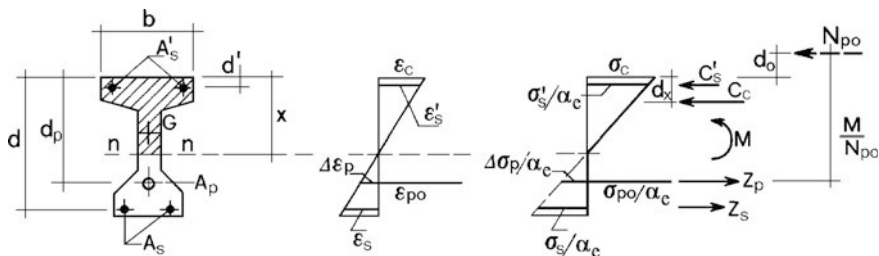
Fig. 3.14 Prestressed section in cracked phase
