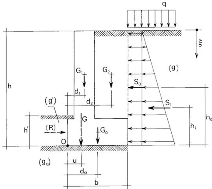
Fig. 9.37 Force components acting on the retaining wall
