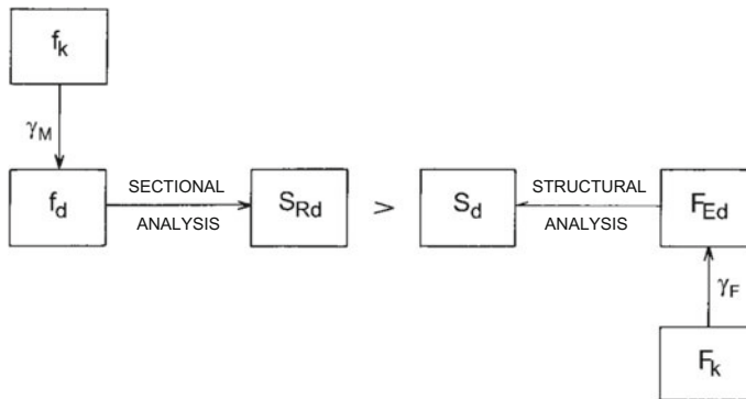
Fig. 7.15 Verification procedure of the stability of RC frames
