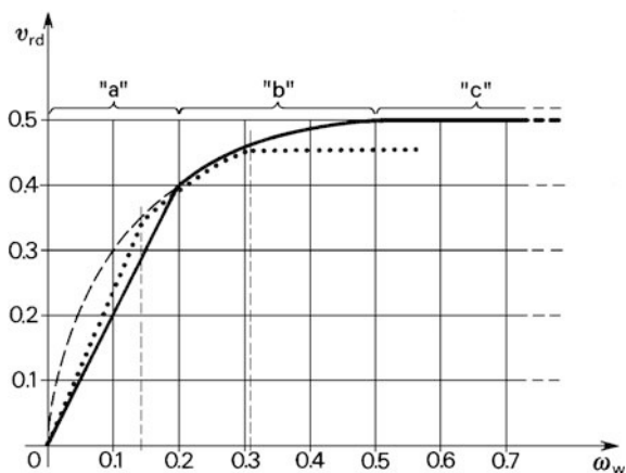
Fig. 4.37 Fields of low (a), medium (b) and high (c) reinforcement ratios
