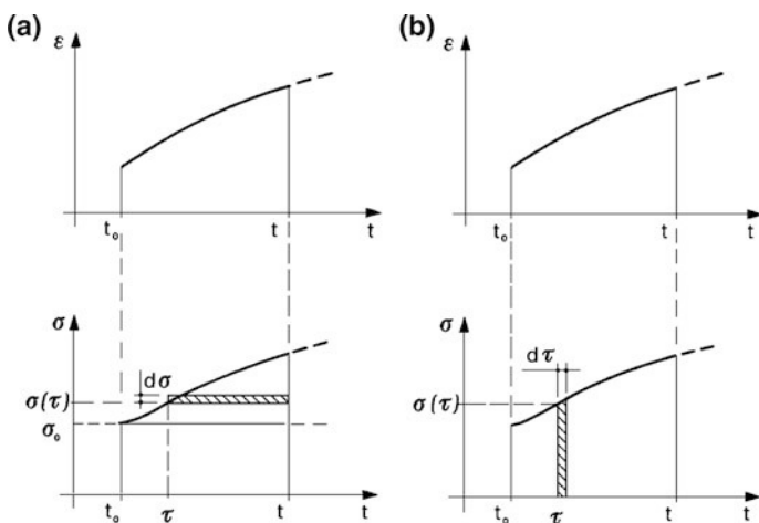
Fig. 1.18 Creep with variable stresses—superposition modes
