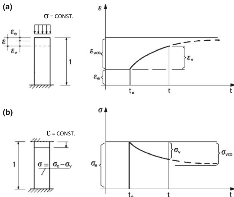
Fig. 1.16 Creep of concrete: creep (a) and relaxation (b)
