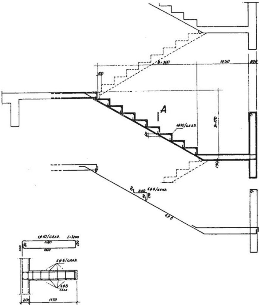
Fig. 8.31 Stair reinforcement
