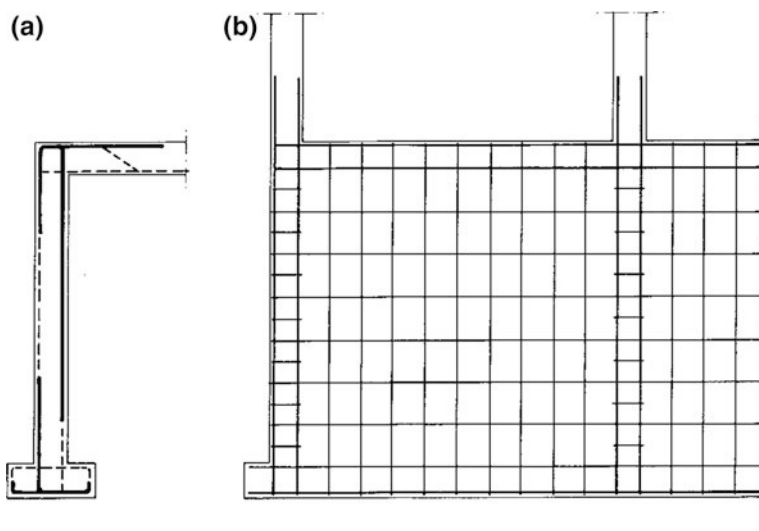
Fig. 9.42 Scheme of flexural (a) and general layout (b) of reinforcement
