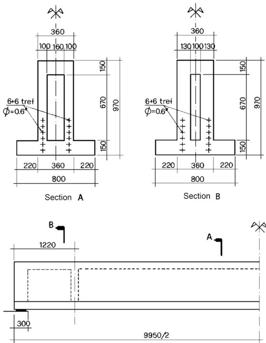
Fig. 5.36 Example of prestressed beam
