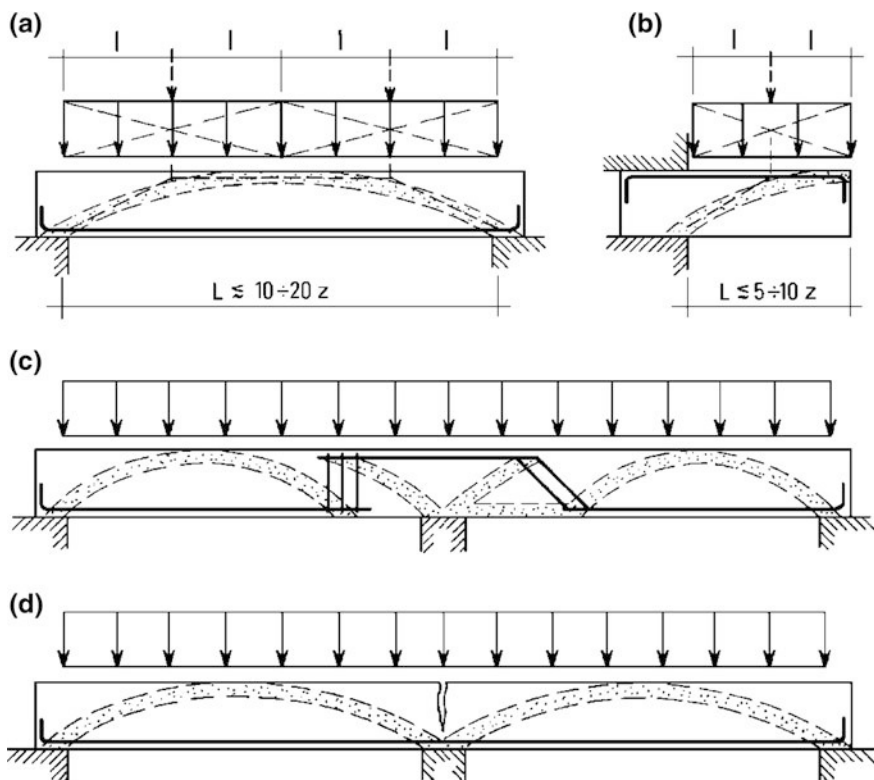
Fig. 5.6 Arch mechanisms for different beam arrangements
