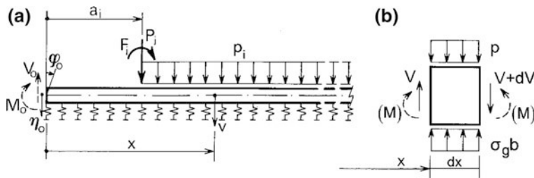
Fig. 9.20 Beam on elastic soil—model (a) and equilibrium of beam segment (b)
