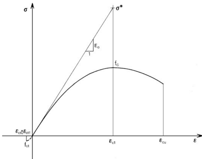
Fig. 1.4 Mathematical model for stress–strain curve
