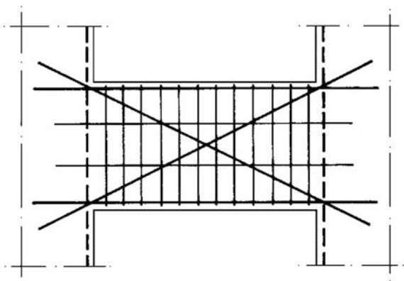
Fig. 5.27 Overall reinforcement layout of the lintel
