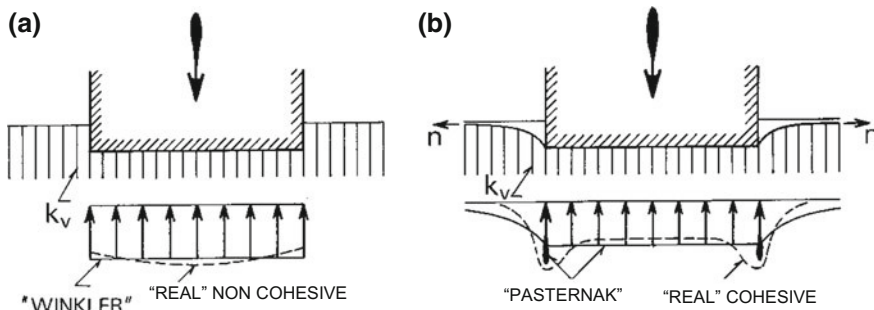
Fig. 9.3 Soil models of Winkler (a) and Pasternak (b)
