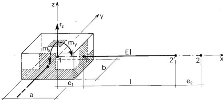
Fig. 9.30 Case of finite dimensions of a node
