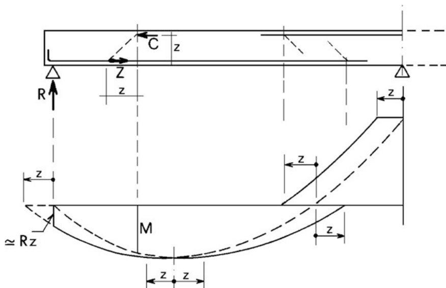
Fig. 4.23 Beam without shear reinforcement—"moment shifting" effect
