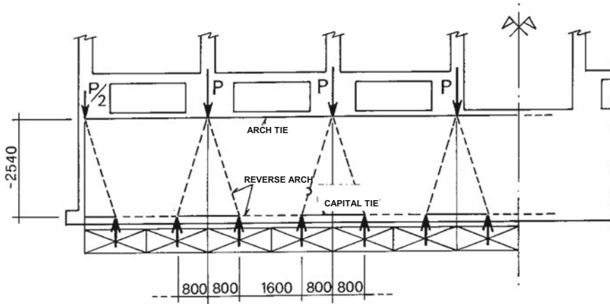
Fig. 9.54 Strut and tie balanced scheme for the foundation wall
