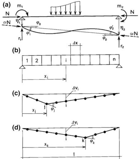
Fig. 7.19 Discretized procedure for second analysis
