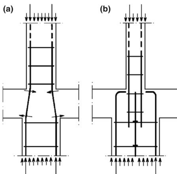
Fig. 2.30 Details of bars overlapping in column joints
