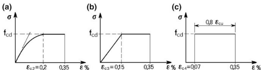
Fig. 1.28 Simplified \sigma - \varepsilon models for concrete in compression
