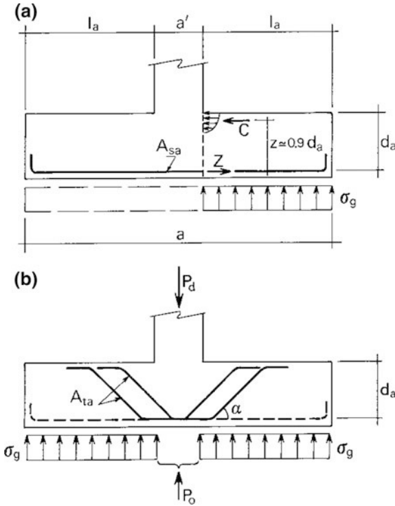
Fig. 9.12 Slender footing— bending (a) and ) and punching shear (b) reinforcement
