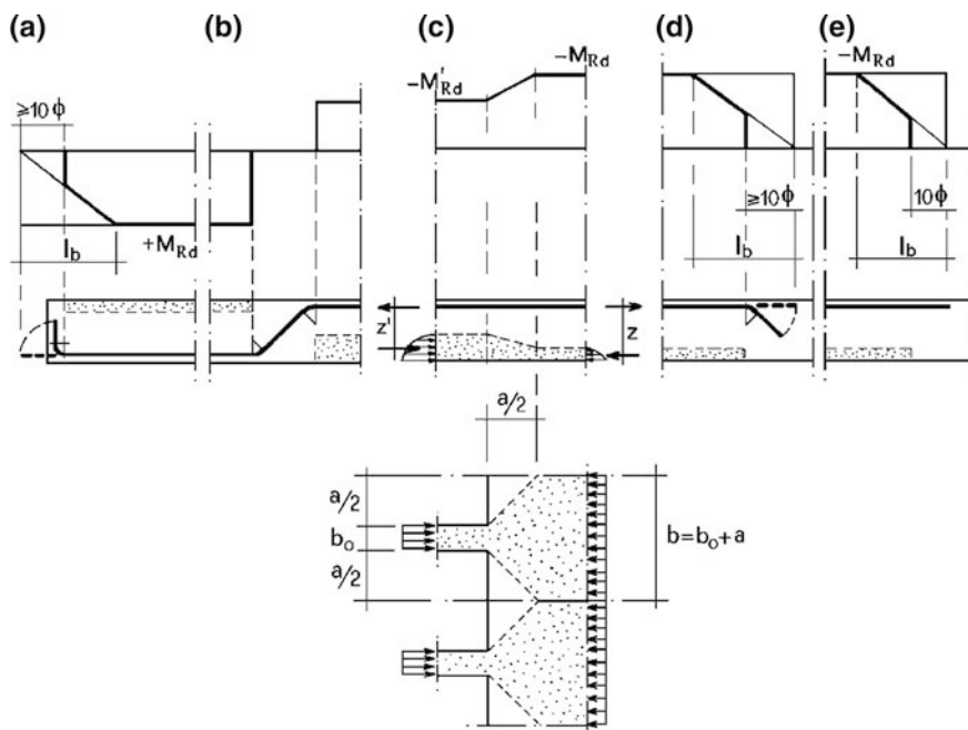
Fig. 3.47 End and internal discontinuity zones of the floor rib
