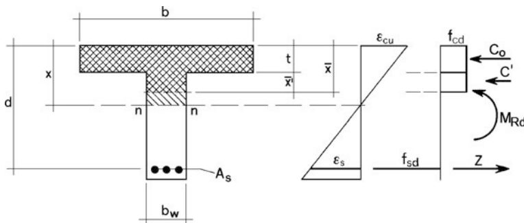
Fig. 3.11 T-section at ultimate limit state of bending
