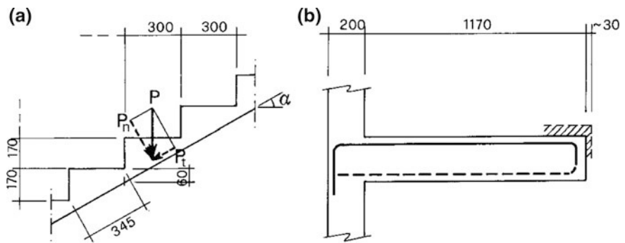
Fig. 8.29 Geometric details of stairs
