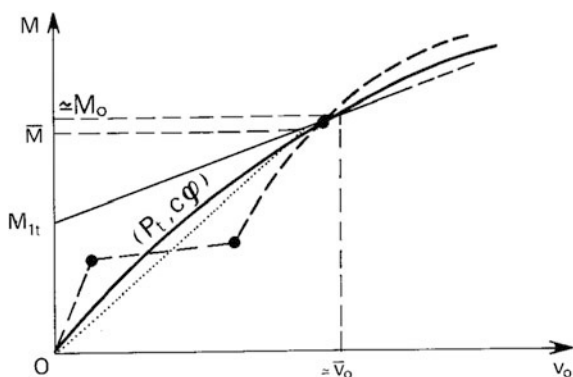
Fig. 7.12 Delayed instability cases due to creep
