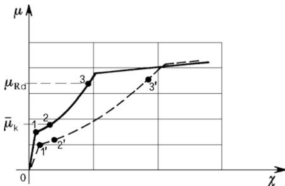
Fig. 3.38 Moment-curvature deformation diagrams
