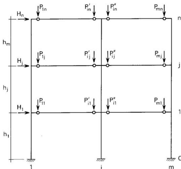
Fig. 7.17 Multistorey precast frame
