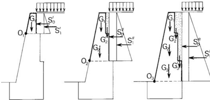
Fig. 9.39 Verification levels of a massive gravity wall
