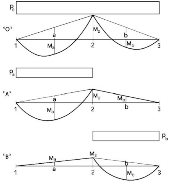
Fig. 3.42 Permanent “O” and variable elementary “A”, “B” load conditions
