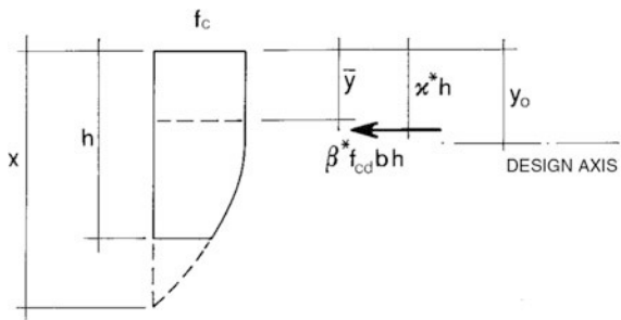
Fig. 6.12 Stress distribution in an entirely compressed section
