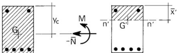
Fig. 6.31 Uncracked section and cracked section in simple bending
