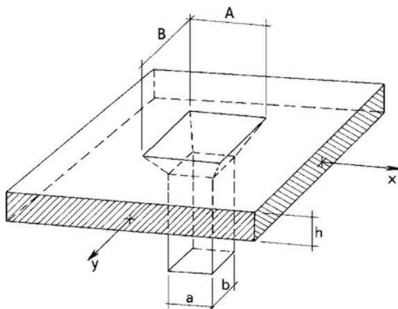
Fig. 5.28 Scheme of the resisting surface in punching shear
