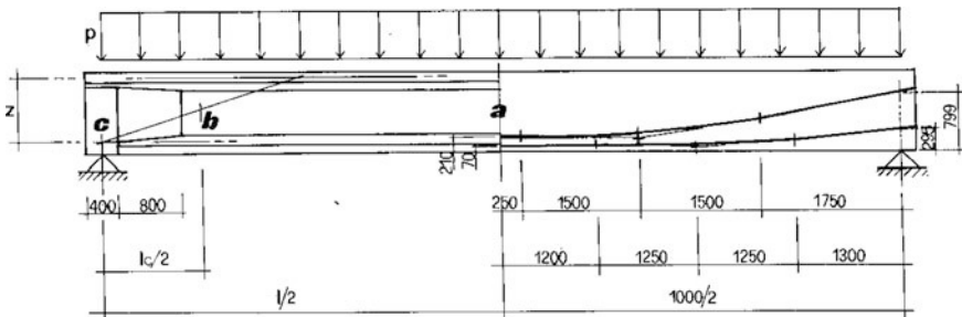
Fig. 10.46 Post-tensioned concrete beam
