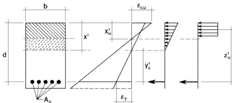
Fig. 3.29 Equilibrium conditions of the section
