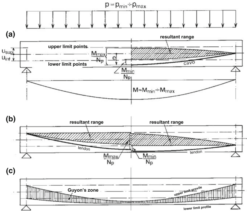
Fig. 10.20 Allowable tendon profile (Guyon's zone)
