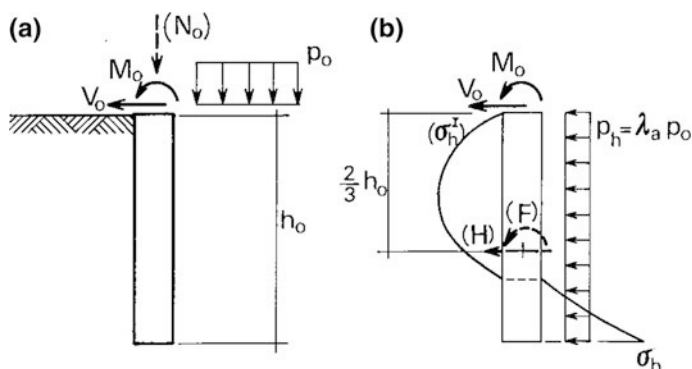
Fig. 9.45 Equilibrium of the embedded wall segment
