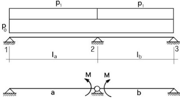
Fig. 3.41 Calculation schemes of the continuous beam
