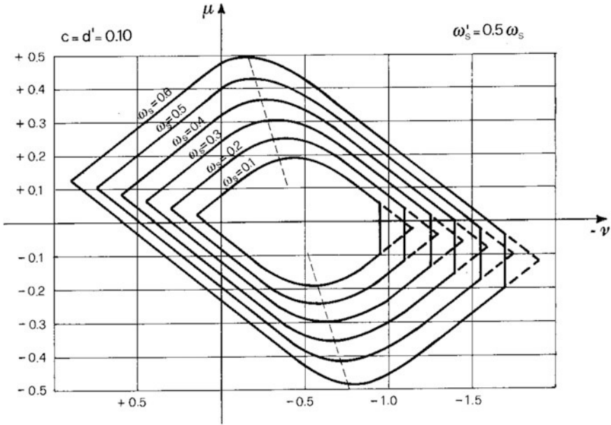
Fig. 6.16 Family of interaction curves for non-symmetric section
