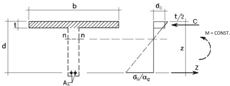
Fig. 3.26 Equilibrium condition of the ideal T-section
