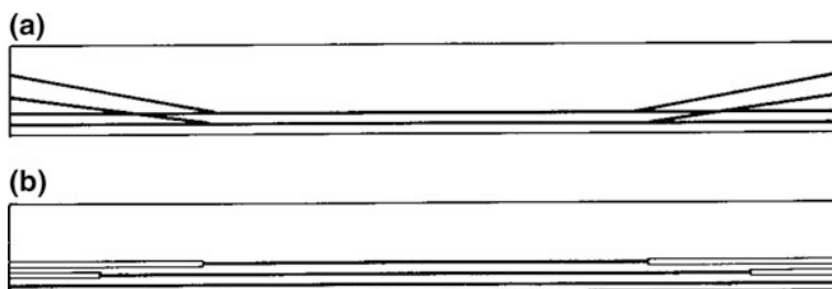
Fig. 10.14 Deviation (a) and sheathing (b) of pretensioned tendons
