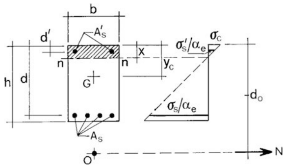
Fig. 6.8 Cracked section under tension and uniaxial bending
