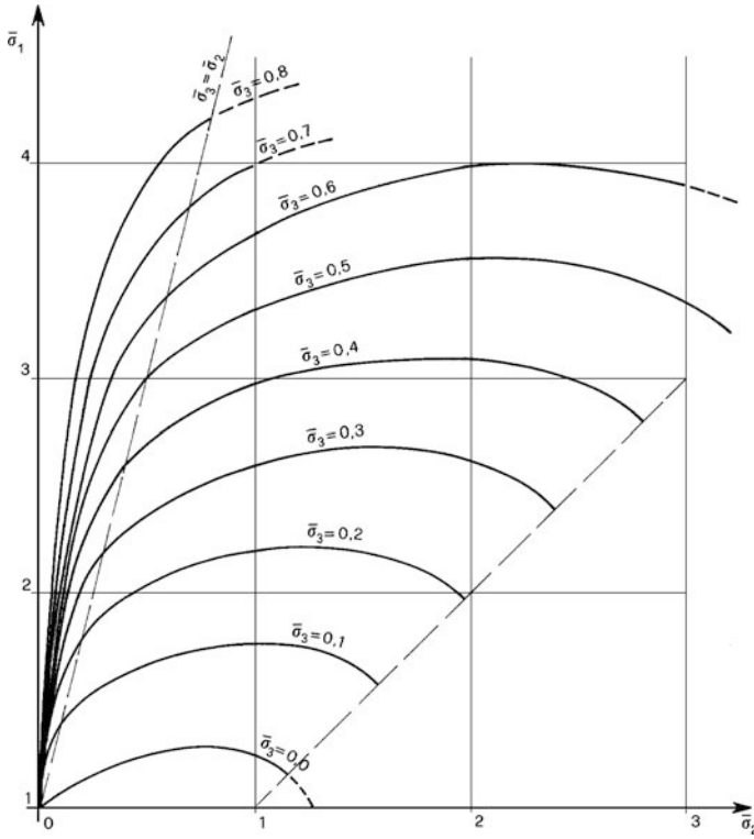
Fig. 1.15 Failure limit curves for triaxial stress states
