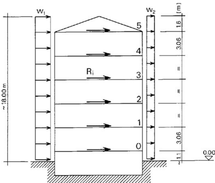
Fig. 8.22 Scheme of wind pressure on the building
