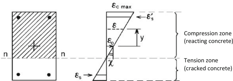
Fig. 1.27 Deformation model of RC section
