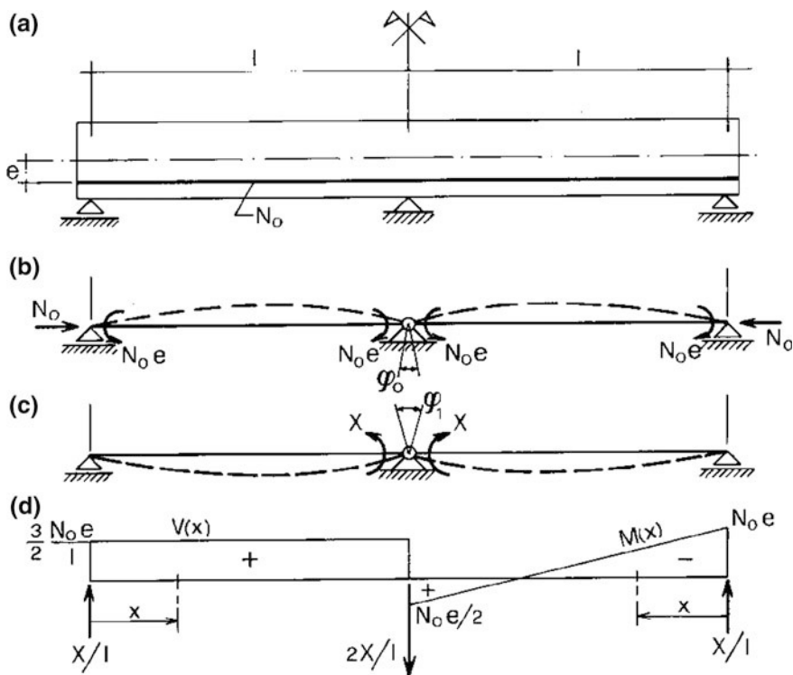
Fig. 10.21 Solution of the hyperstatic beam
