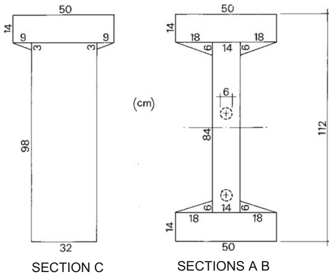
Fig. 10.47 Geometric dimensions of the sections
