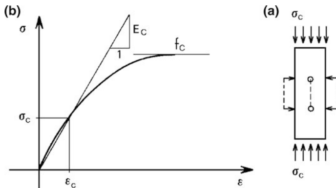
Fig. 1.10 Tests for the modulus of elasticity
