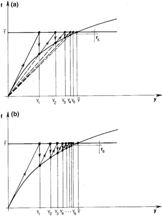
Fig. 6.37 Secant (a) and residual redistribution (b) methods
