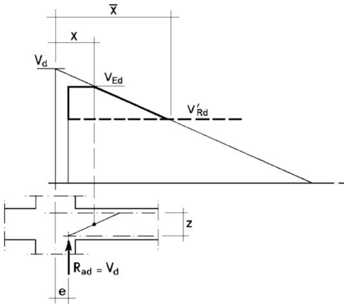
Fig. 5.51 Distribution of shear action between stirrups and bent bars
