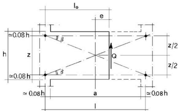
Fig. 5.24 Geometrical parameters of the lintel model
