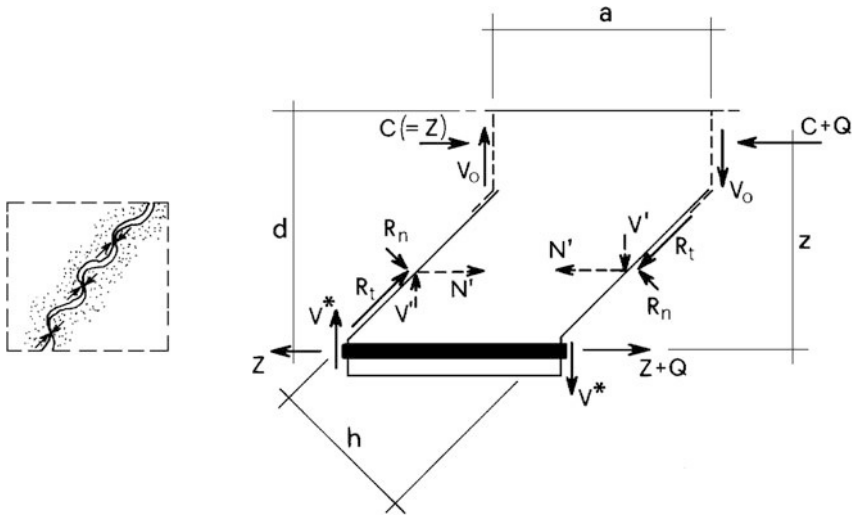
Fig. 4.22 Aggregate interlock in the concrete web
