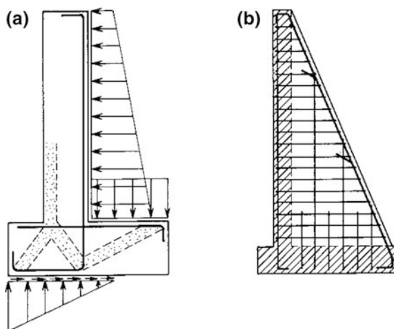
Fig. 9.40 Cantilever (a) and buttressed (b) retaining walls
