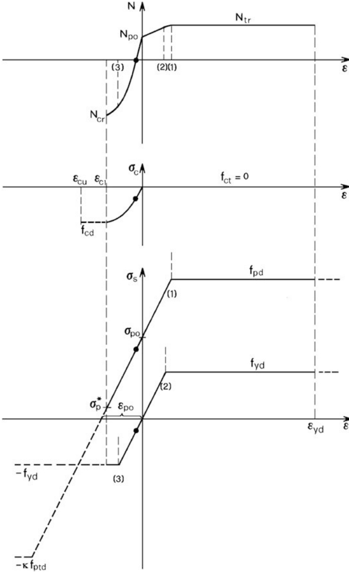
Fig. 2.10 Stress-strain diagrams of a prestressed tie
