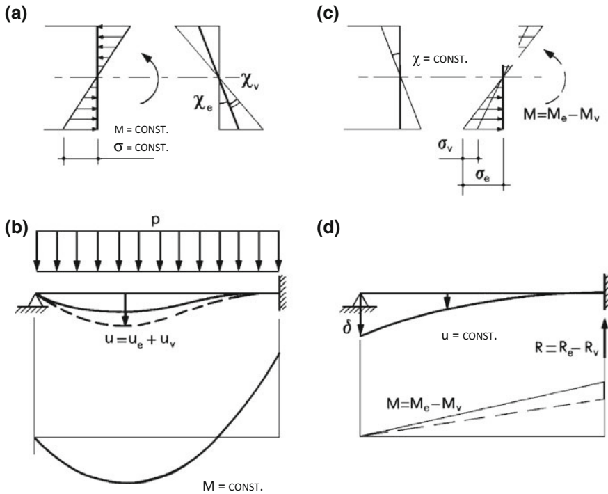
Fig. 1.21 Structural effects of creep
