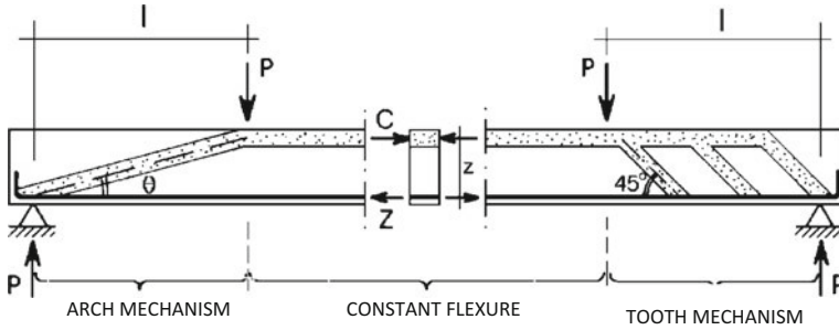
Fig. 5.3 Arch (left) and tooth (right) mechanisms
