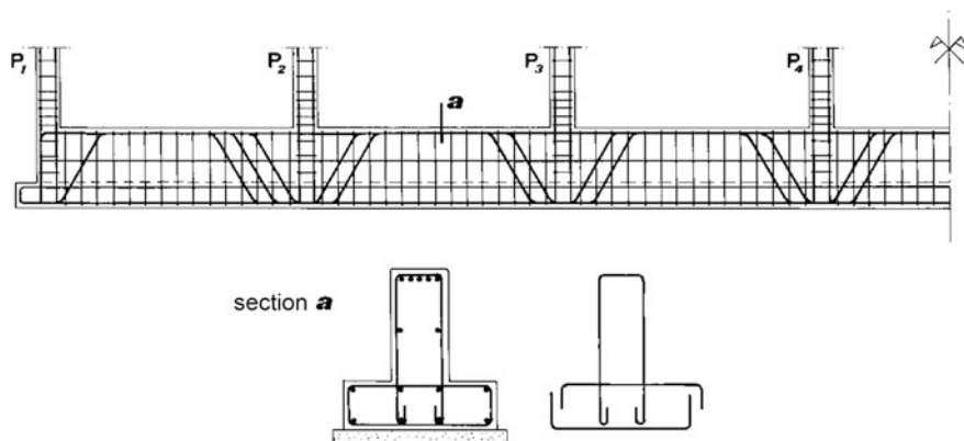
Fig. 9.25 Reinforcement details of the foundation beam
