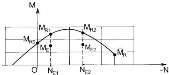
Fig. 6.18 Representation of analytical verification
