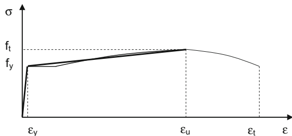
Fig. 1.29 Bilinear model for reinforcing steel
