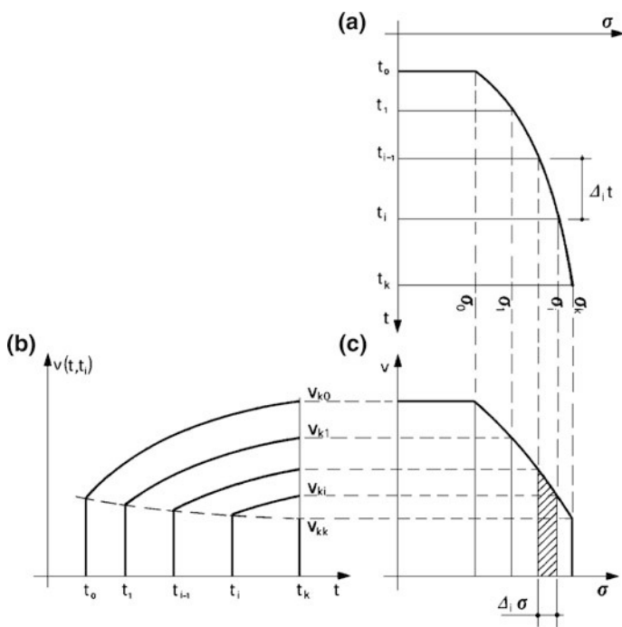
Fig. 1.22 Graphical representation of the numerical procedure
