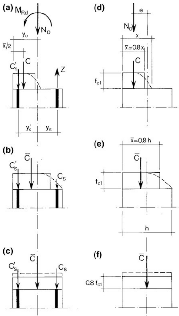
Fig. 6.21 Compression and uniaxial bending in an unreinforced section
