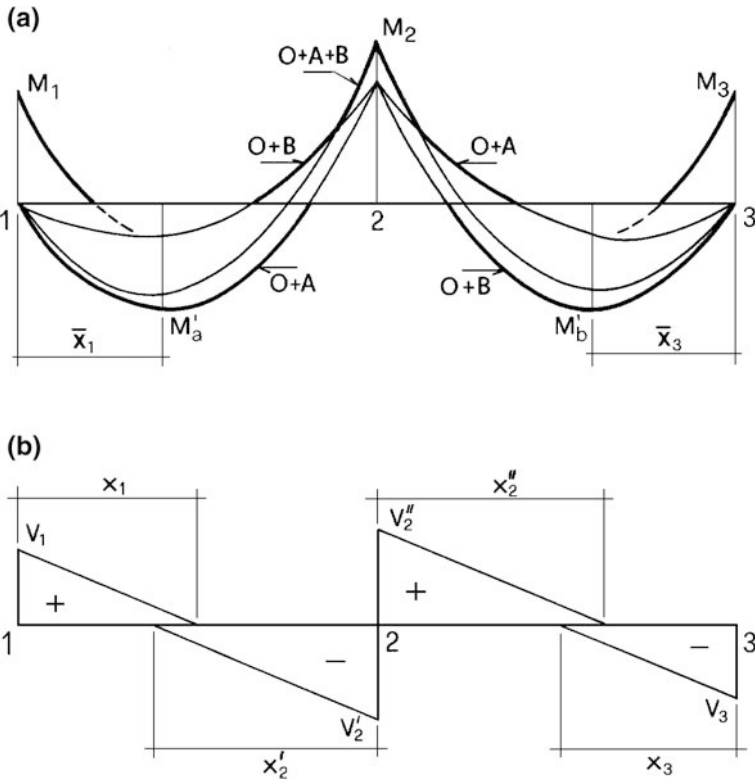
Fig. 4.42 Envelope diagrams for moment (a) and shear (b)
