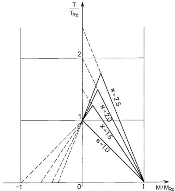
Fig. 8.16 Resistance limit curves for M - T interaction
