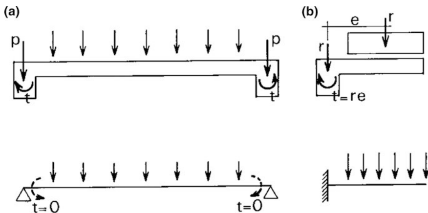
Fig. 8.2 Calculation schemes for compatibility (a) and equilibrium (b) torsion
