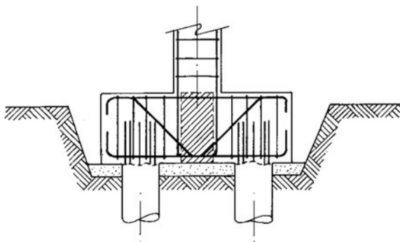
Fig. 9.18 Reinforcement details of a double cantilever
