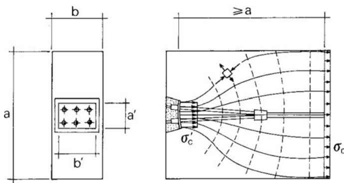
Fig. 10.31 End anchorage of a post-tensioned tendon and stress diffusion
