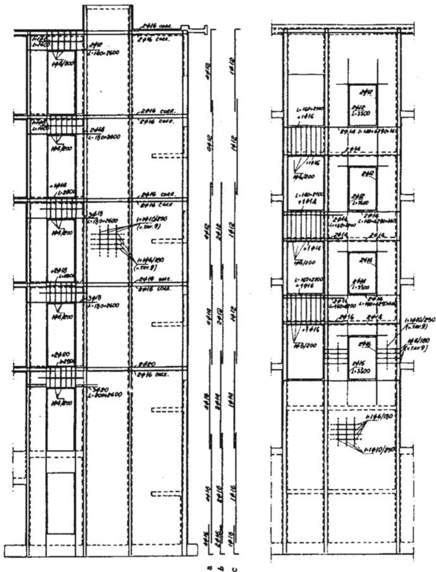
Fig. 8.27 Corewall reinforcement—walls
