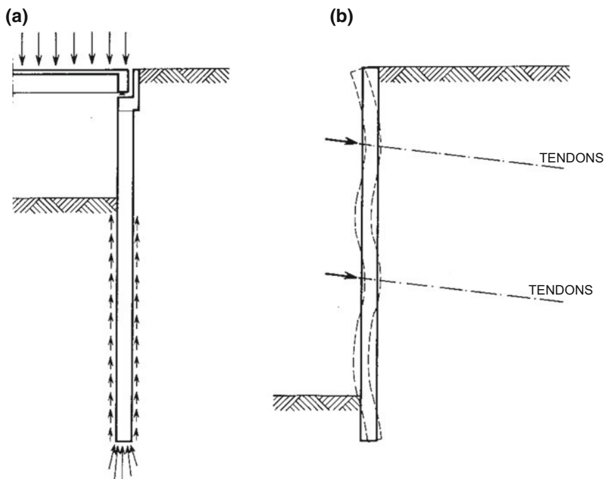
Fig. 9.47 Deep foundation wall (a) and diaphragm with prestressed tendons (b)
