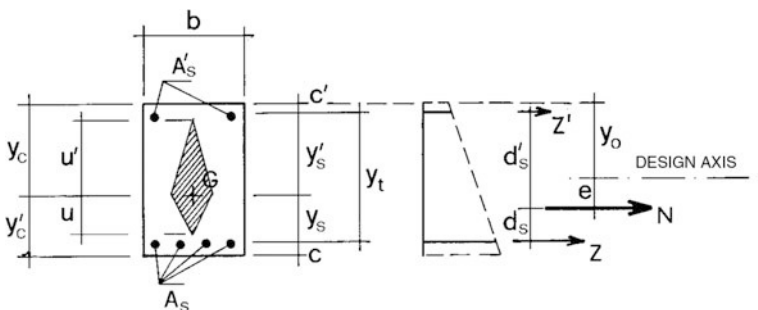
Fig. 6.7 Entirely cracked section under tension and uniaxial bending
