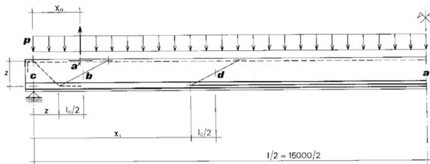
Fig. 10.43 Lateral view of the pretensioned element
