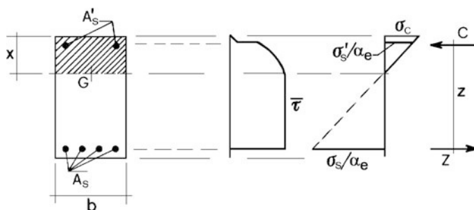
Fig. 4.2 Cracked section—stresses distribution for shear and moment
