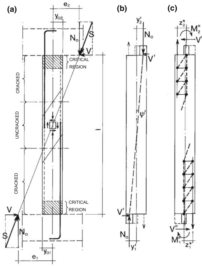
Fig. 6.27 Typical column (a) and its model with two mechanisms (b) + (c)
