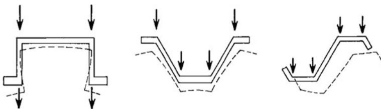
Fig. 8.21 Deformation warping effects in folded plates systems
