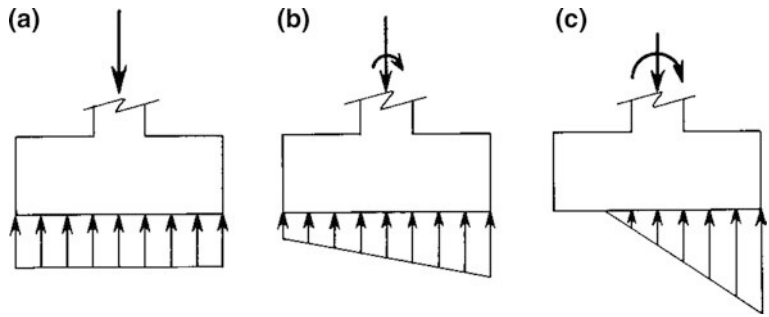
Fig. 9.8 Pressure distributions rendered by the soil
