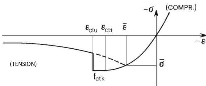
Fig. 3.31 Stress-strain model in tension
