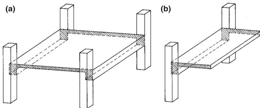
Fig. 8.1 Example of compatibility (a) and equilibrium (b) torsion
