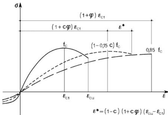
Fig. 3.32 Creep effects on stress–strain diagram
