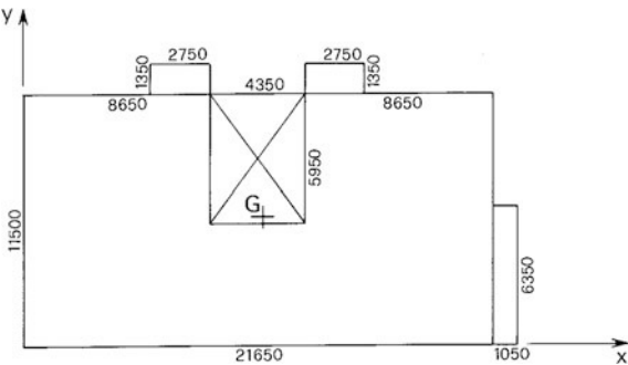
Fig. 8.23 Overall dimensions of the type floor
