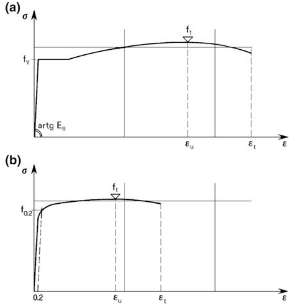
Fig. 1.24 Stress–strain curves of reinforcing steel
