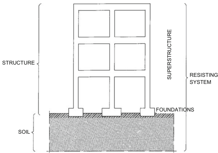
Fig. 9.1 Resisting system of the building
