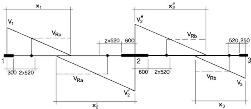
Fig. 4.39 Shear diagram along a floor strip
