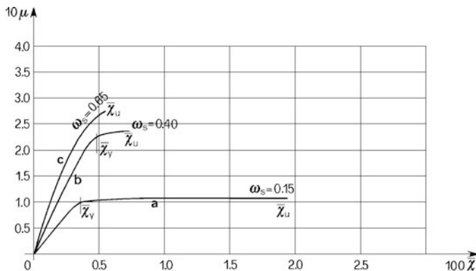
Fig. 3.36 Resistance constitutive laws
