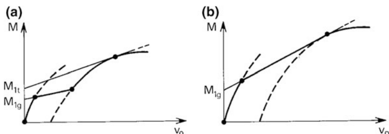
Fig. 7.12 Delayed instability cases due to creep
