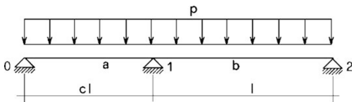
Fig. 5.41 Example of continuous beam
