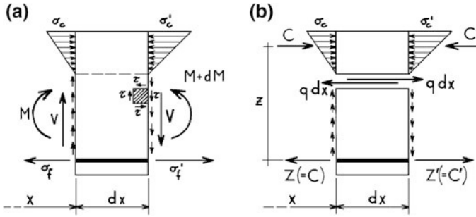
Fig. 4.5 Equilibrium condition of a beam segment
