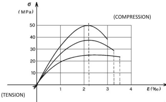
Fig. 1.1 Concrete stress–strain diagrams
