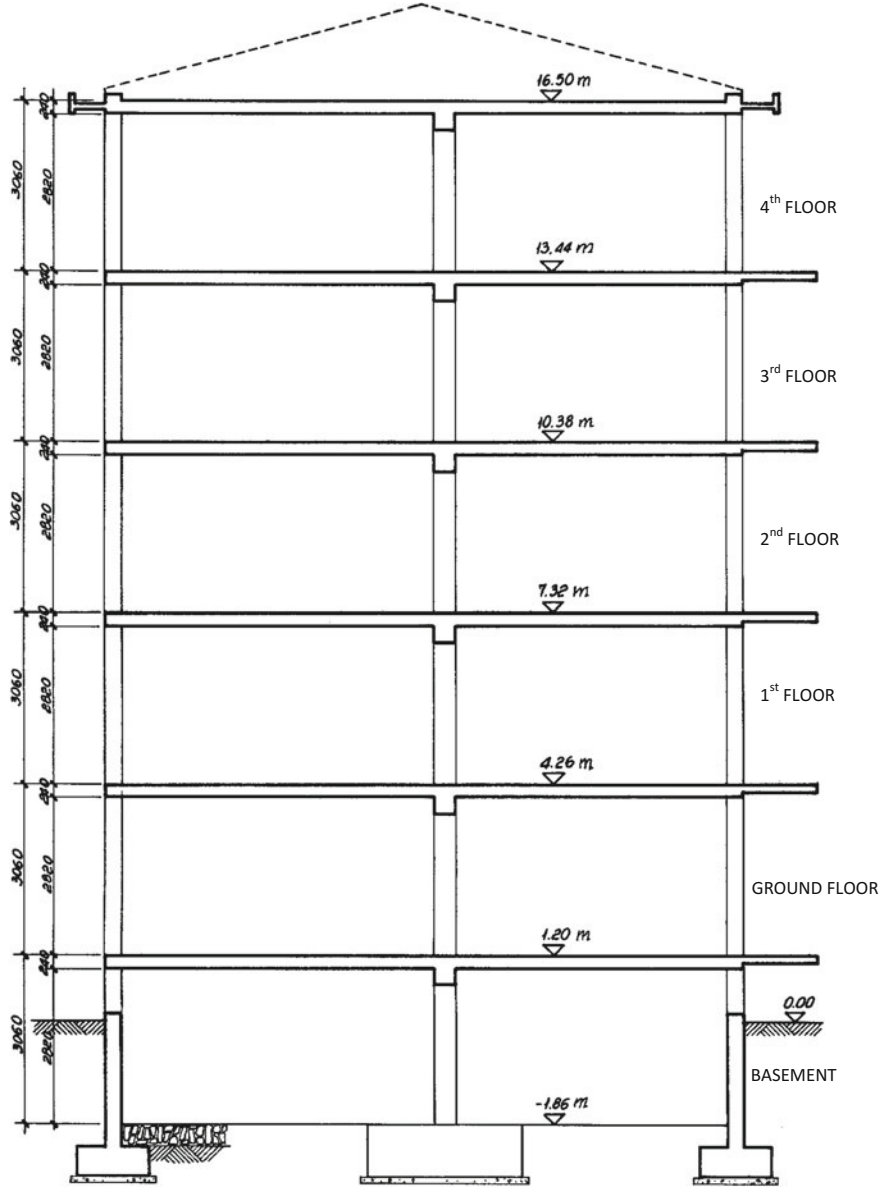
Fig. 2.20 Multistorey building—elevation
