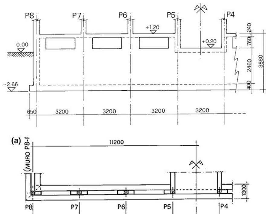
Fig. 9.52 Dimensions of the foundation wall
