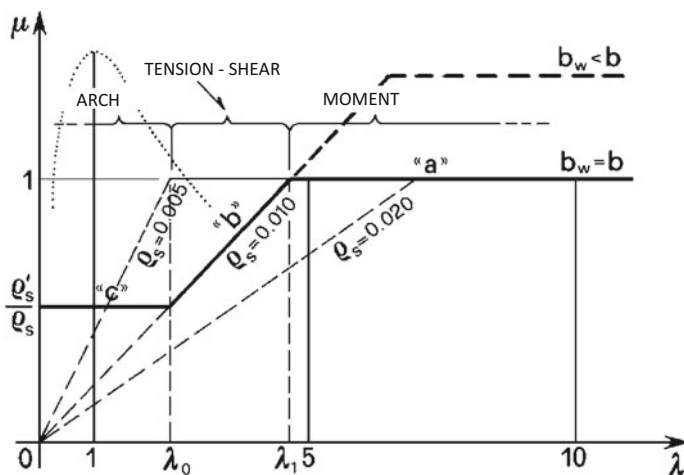
Fig. 5.10 Different domains of rupture of the beam
