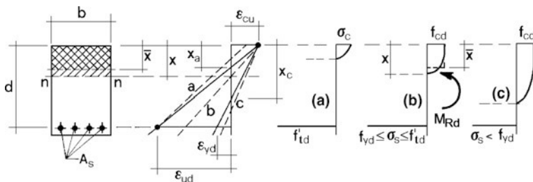
Fig. 3.10 Strain and stress distributions at the ultimate limit state
