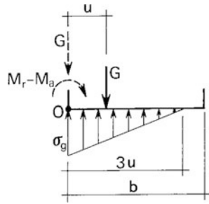
Fig. 9.38 Elastic response of the foundation soil
