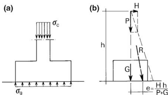
Fig. 9.2 Equilibrium conditions under centred (a) and eccentric (b) loads
