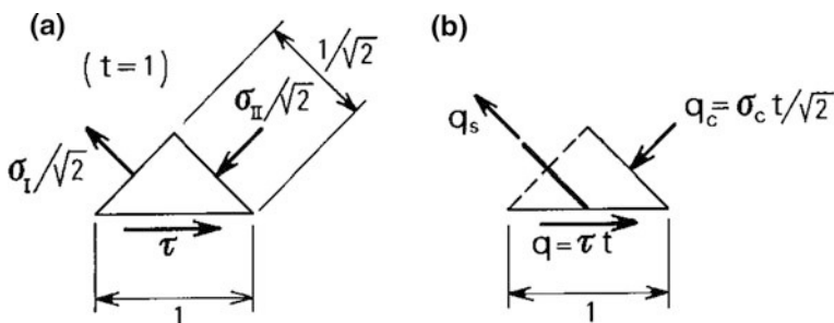
Fig. 8.12 Stress equilibrium before (a) and after (b) torsional cracking
