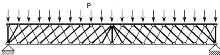
Fig. 4.27 Diffuse truss model
