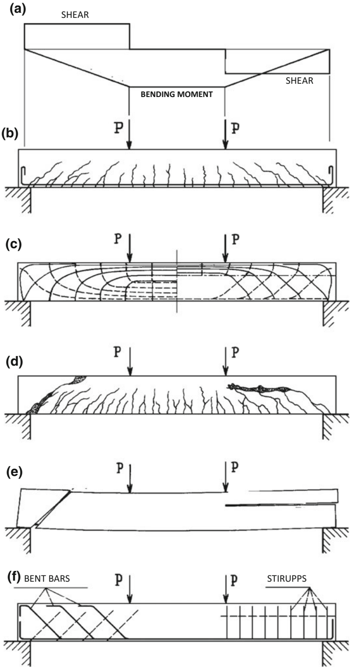
Fig. 4.3 Cracking process and shear failure mechanisms
