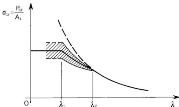
Fig. 7.2 Critical stress curve
