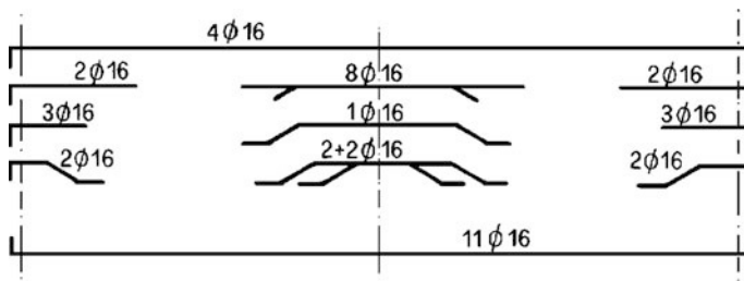
Fig. 5.47 General layout of longitudinal reinforcement
