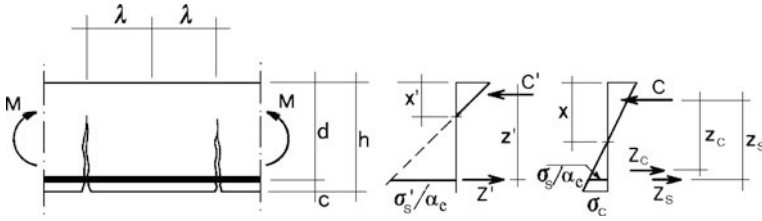
Fig. 3.18 Equilibrium conditions along the beam
