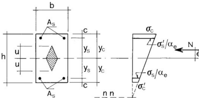
Fig. 6.2 Stress distribution in an entirely compressed section
