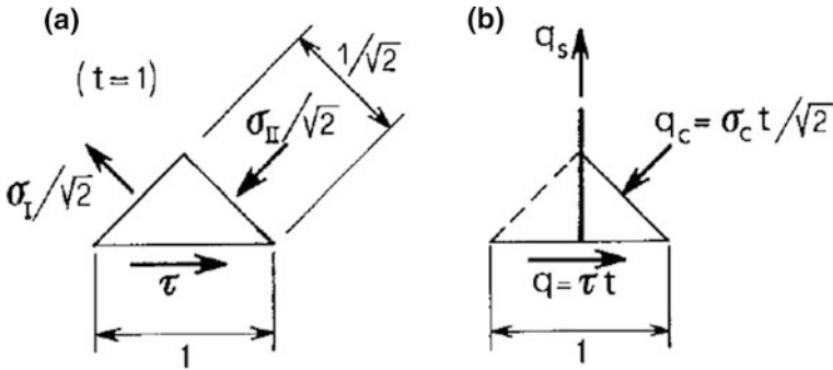
Fig. 8.10 Stress equilibrium before (a) and after (b) cracking
