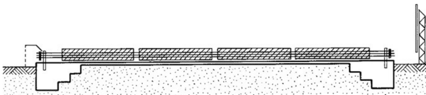
Fig. 10.4 Production line of pre-tensioned precast beams
