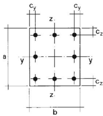
Graph 6.6: Combined Biaxial Bending—Section with 8 Bars
