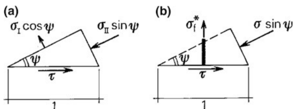
Fig. 10.34 Local equilibrium of stresses
