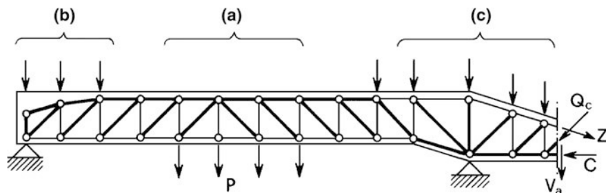
Fig. 4.30 Hung loads (a), inclined compressions (b), variable depth (c)
