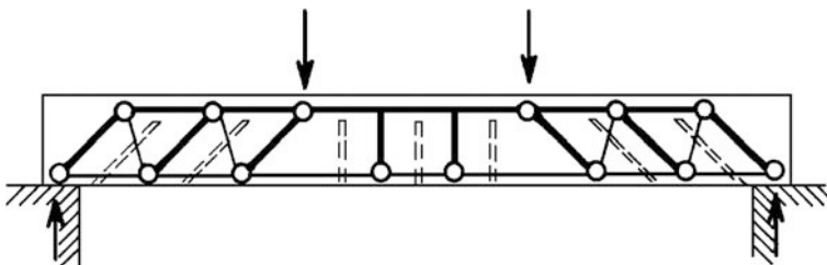
Fig. 4.9 Mörsch truss model
