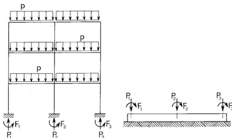
Fig. 9.26 Separate calculation models for superstructure and foundations
