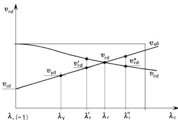
Fig. 4.36 Ultimate limit state of shear resistance
