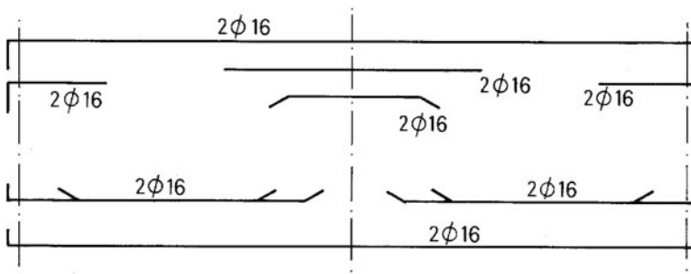
Fig. 4.44 General layout of the reinforcement bars
