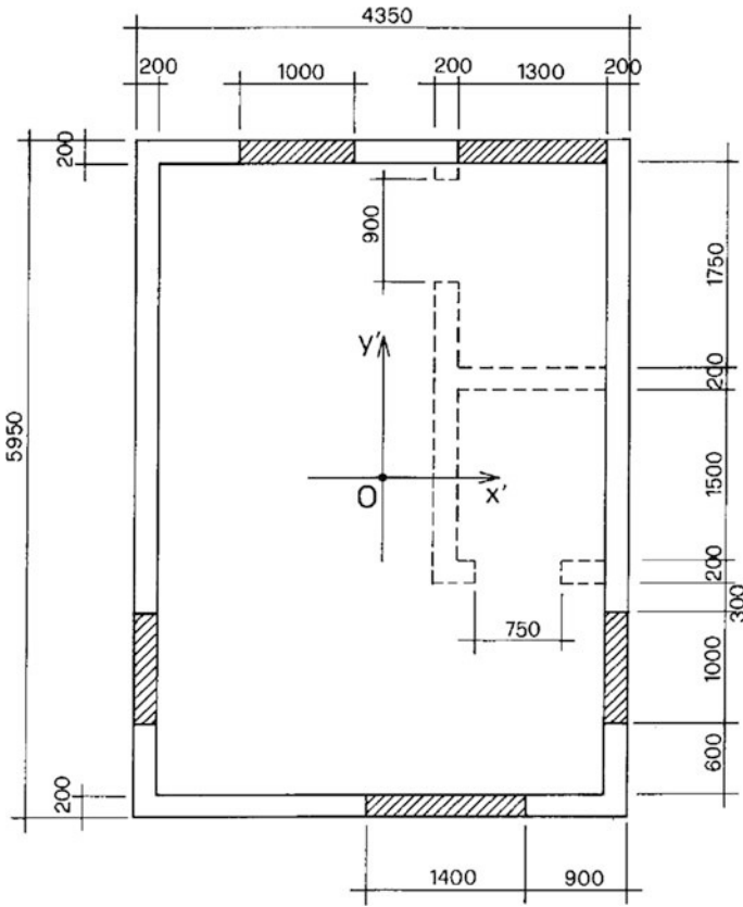
Fig. 8.24 Section of the stability core
