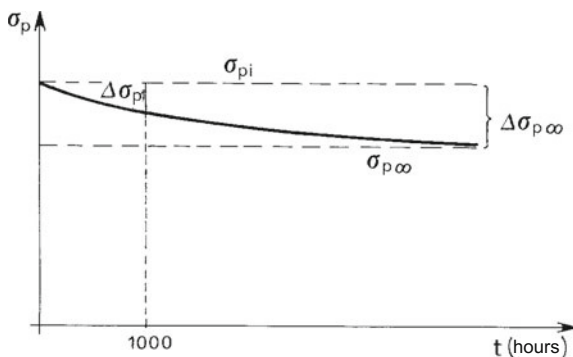
Fig. 10.12 Progressive stress losses due to relaxation
