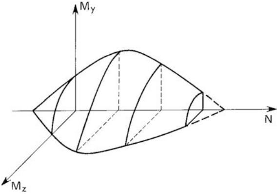
Fig. 6.24 Interaction limit surface for doubly symmetric section
