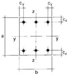
Graph 6.8: Combined Biaxial Bending—Section with 6 Bars
