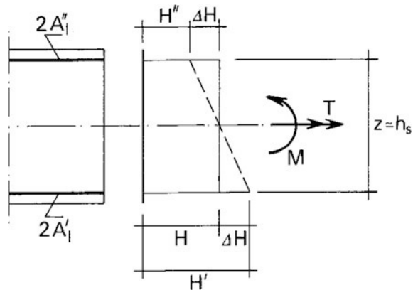
Fig. 8.15 Bending moment and torsion interaction
