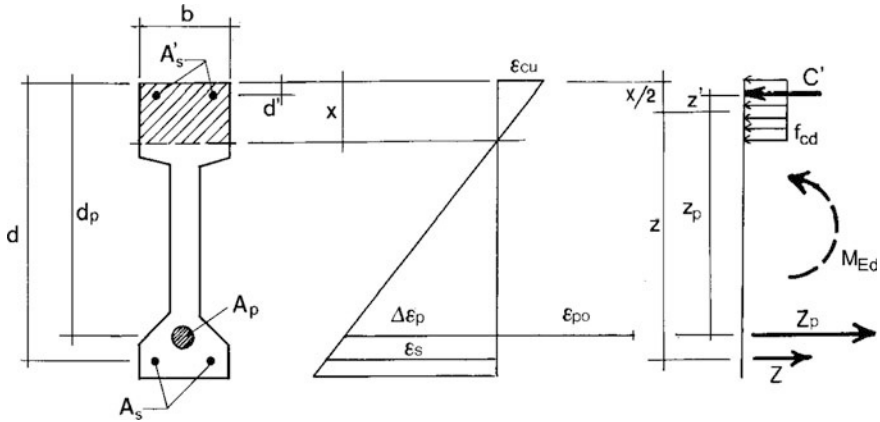
Fig. 10.25 Strain and stress distribution in a post-tensioned section
