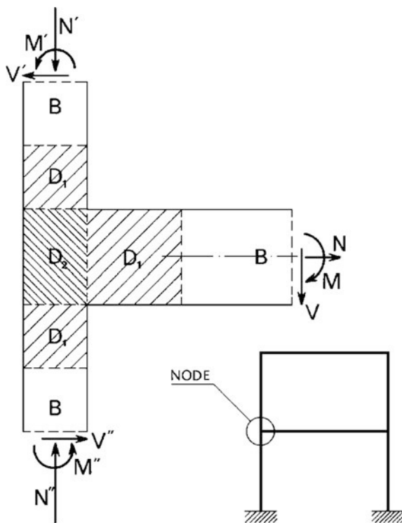
Fig. 5.13 Transition ( D_1 ) and discontinuity ( D_2 ) zones
