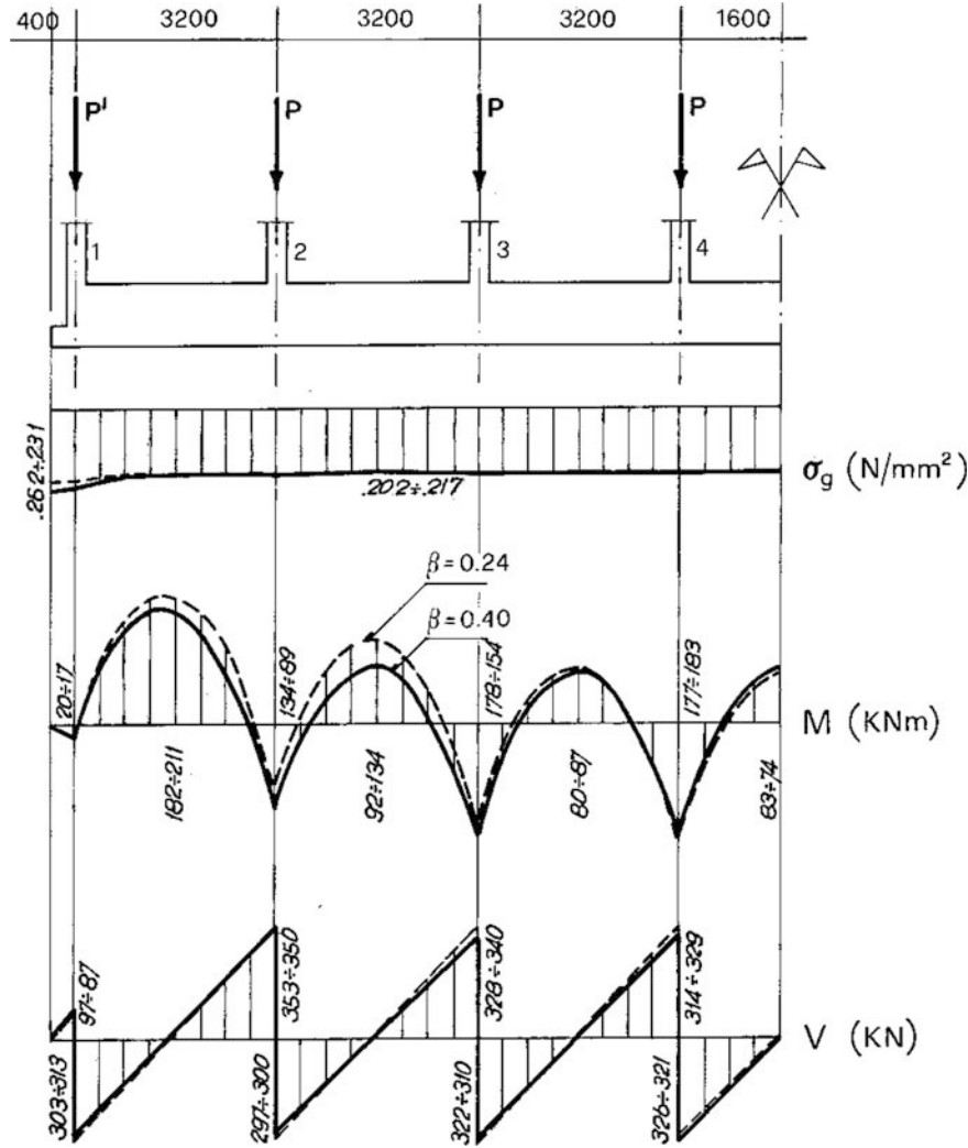
Fig. 9.23 Distributions of soil pressure and internal forces
