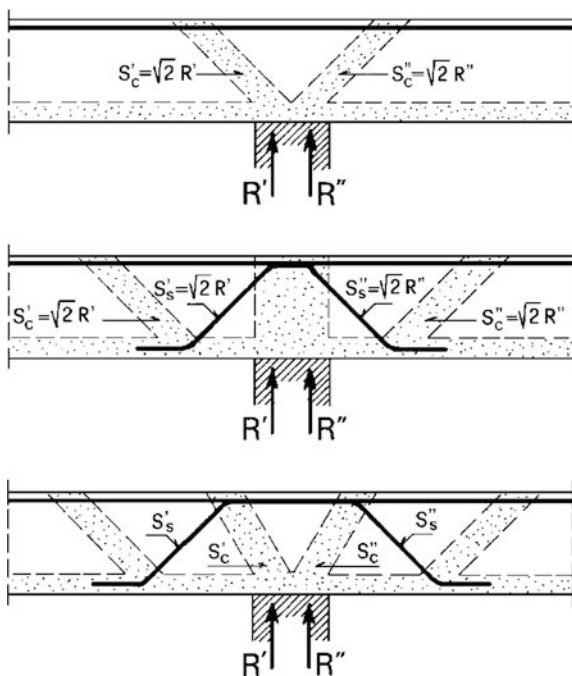
Fig. 5.18 Possible different details over the internal support
