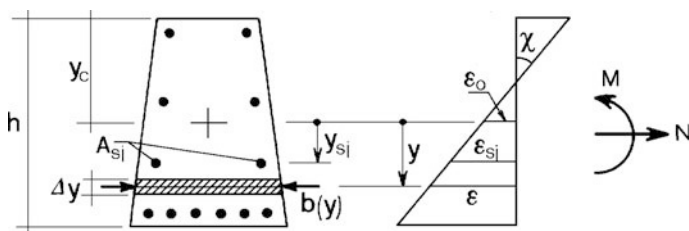
Fig. 3.30 Integration of the stresses over the section
