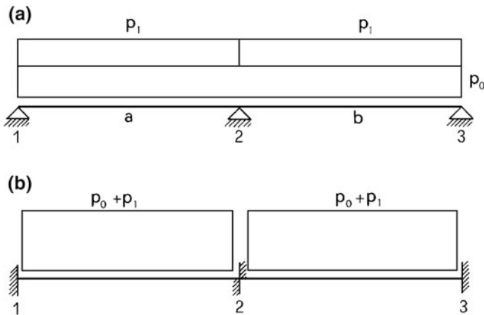
Fig. 4.41 Partial calculation schemes
