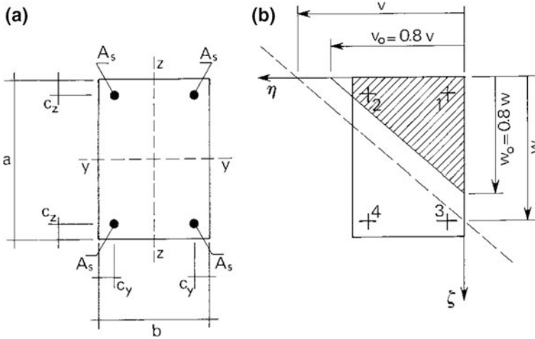
Fig. 6.26 Case of rectangular section with doubly symmetric reinforcement
