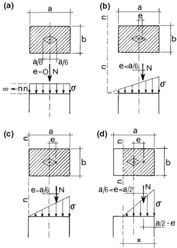
Fig. 6.3 Stress distribution in an unreinforced section
