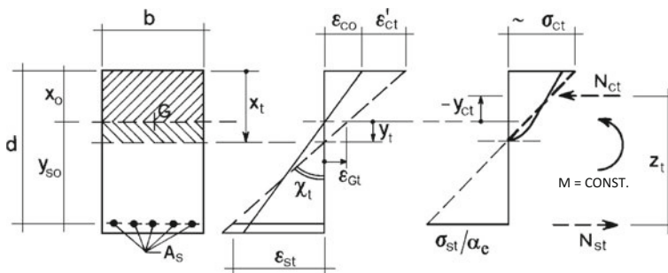
Fig. 3.24 Creep effects on the section in bending
