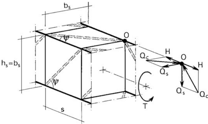
Fig. 8.9 Model of the resisting peripheral truss
