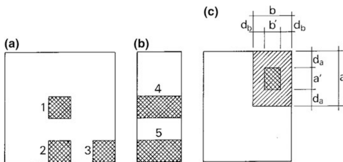
Fig. 10.32 Localised pressure—positions of the poaded print
