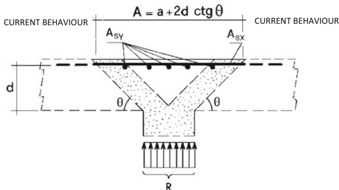
Fig. 5.29 Detail of the diffusion zone
