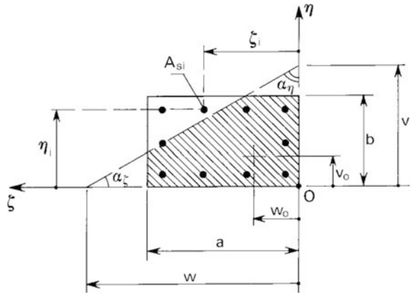
Fig. 6.10 Cracked section under axial force and biaxial bending
