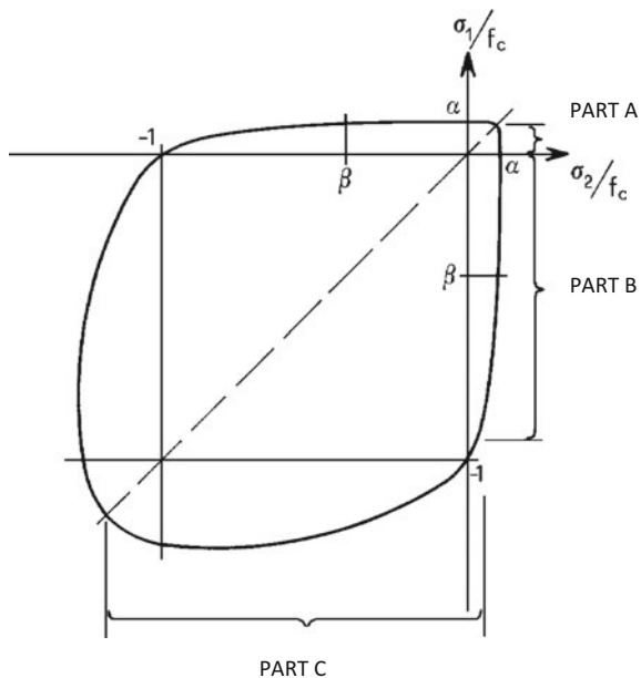
Fig. 1.14 Failure limit curve for biaxial stress states
