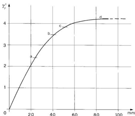
Fig. 6.40 Progressive formation of plastic hinges
