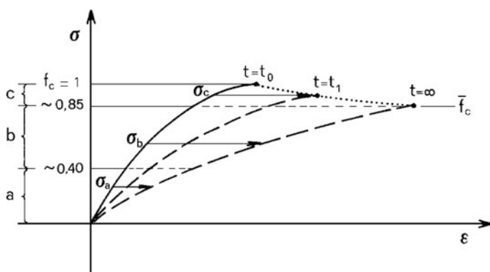
Fig. 1.2 Concrete stress-strain diagrams under long-term loading
