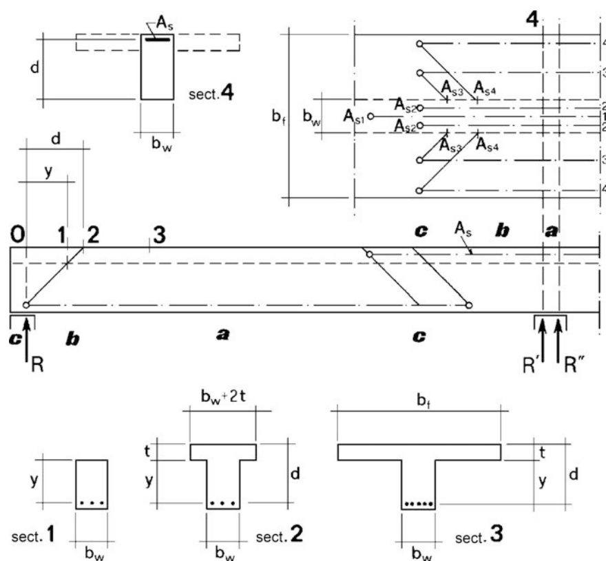
Fig. 5.15 Conventional model of stress diffusion
