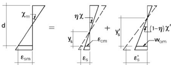
Fig. 3.20 Deduction of the average curvature
