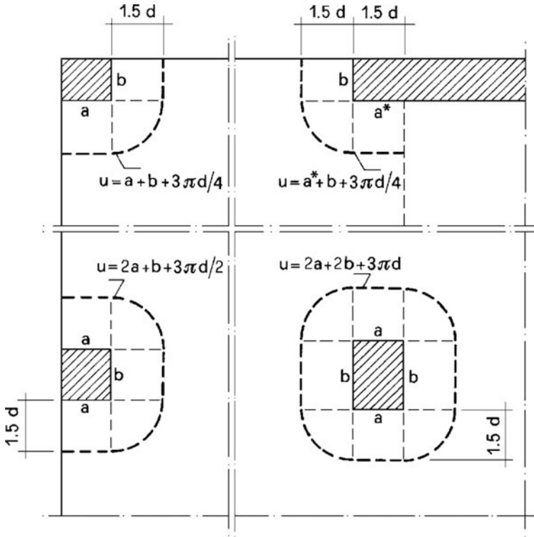
Fig. 5.30 Perimeter of the diffusion zone for the different positions
