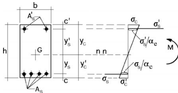
Fig. 3.5 Stress distribution in an uncracked section
