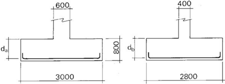
Fig. 9.49 Footing to column P14
