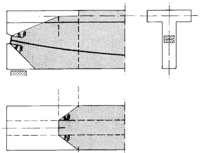
Fig. 10.41 Post-tensioned tendon—model of prestressing diffusion
