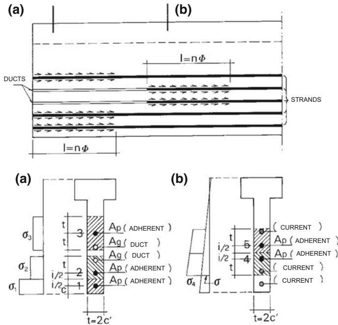
Fig. 10.38 Application example of the conventional procedure
