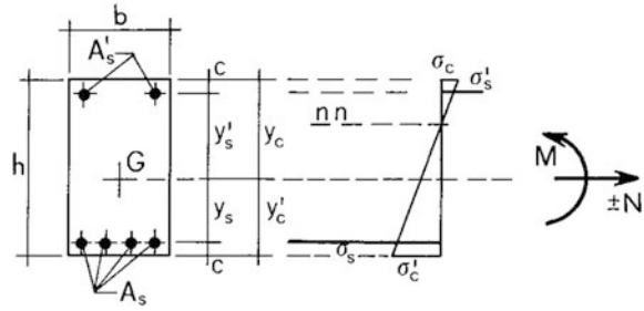
Fig. 6.1 Stress distribution in elastic uncracked section
