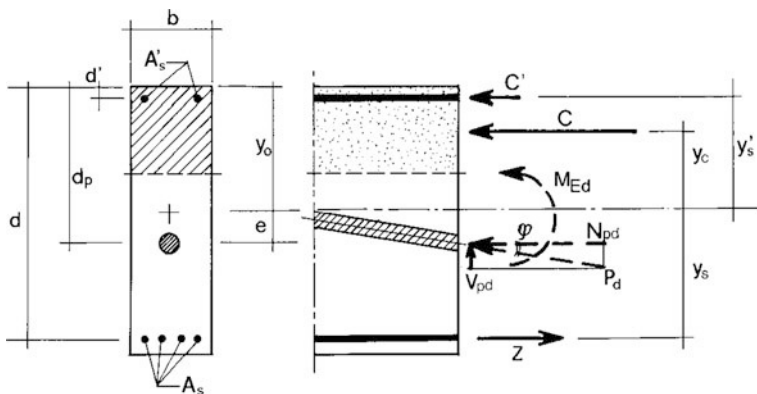
Fig. 10.26 Force representation of the precompression
