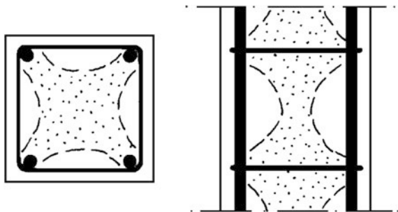
Fig. 2.6 Confining action on the concrete core
