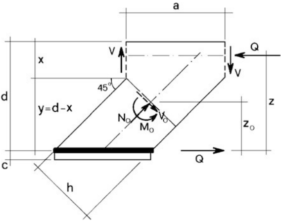
Fig. 4.18 Equilibrium condition of a beam segment
