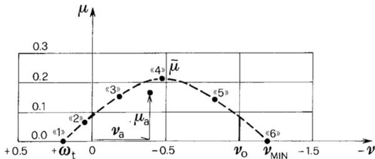
Fig. 6.14 Interaction limit curve
