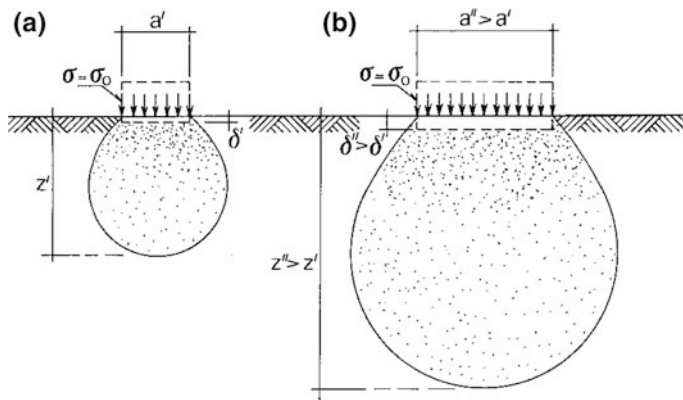
Fig. 9.48 Soil volume involved in settlement
