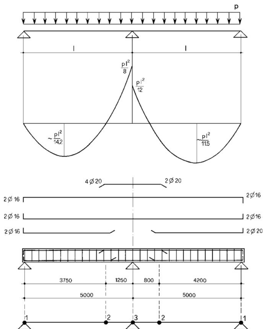
Fig. 5.42 Example of nonlinear calculation up to collapse
