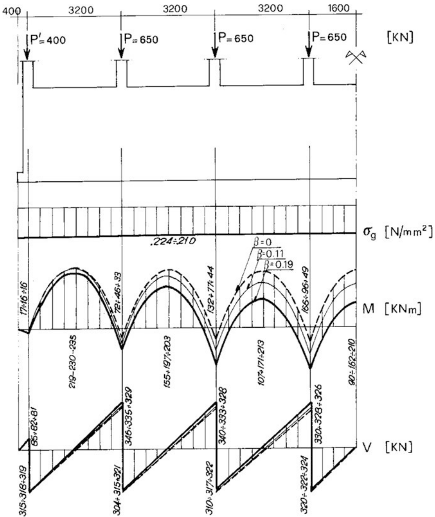
Fig. 9.43 Soil pressure and internal forces on foundation wall-beam
