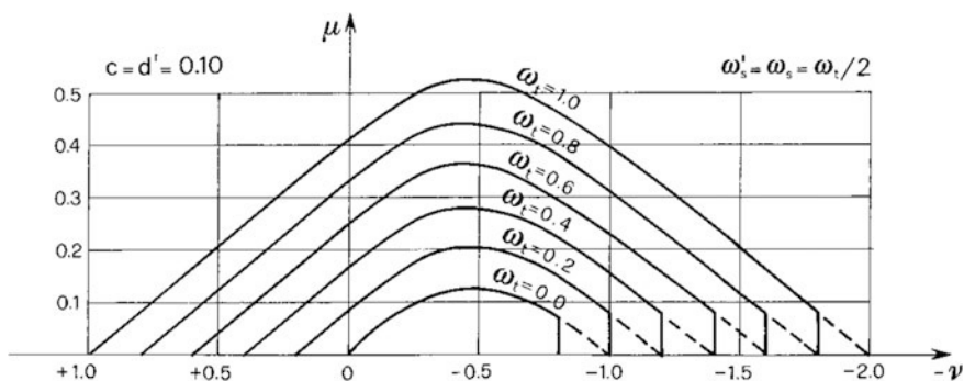
Fig. 6.15 Family of interaction curves for symmetric section
