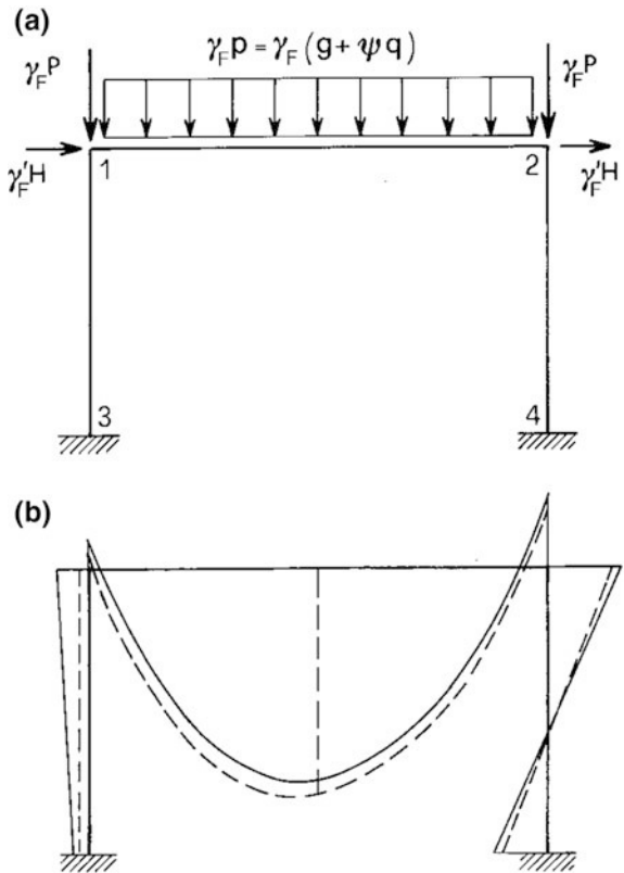
Fig. 6.38 Example of reinforced concrete frame
