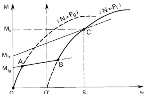
Fig. 7.10 Limit collapse situations for eccentric and centred axial compression
