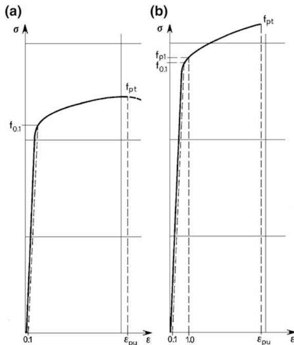
Fig. 1.25 Stress-strain curves of pre-stressing steel
