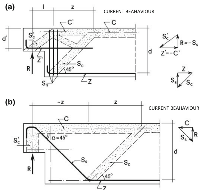
Fig. 5.19 Possible different details of half joints
