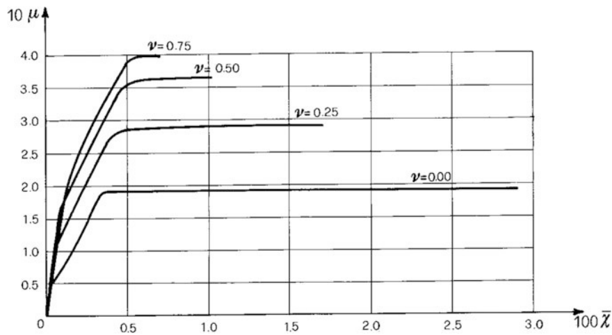
Fig. 6.33 Deformation moment-curvature curves
