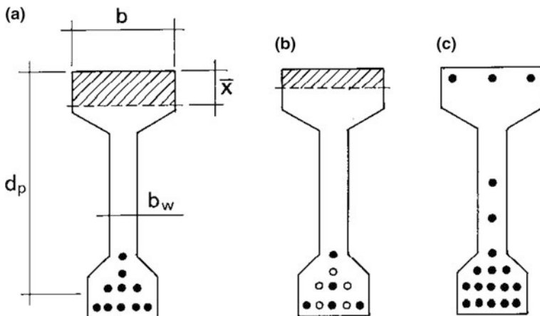
Fig. 10.27 Section prestressed with pretensioned tendons
