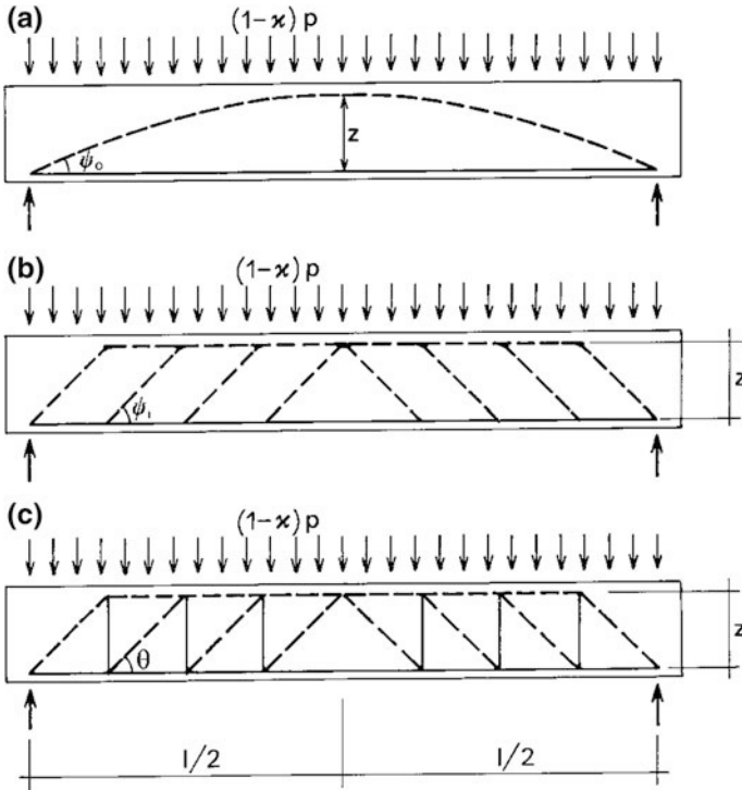
Fig. 10.29 Arch (a), tooth (b) and truss (c) models of the prestressed beam
