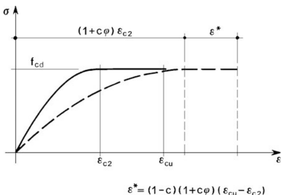
Fig. 3.33 Parabola-rectangle \sigma - \varepsilon with creep effects
