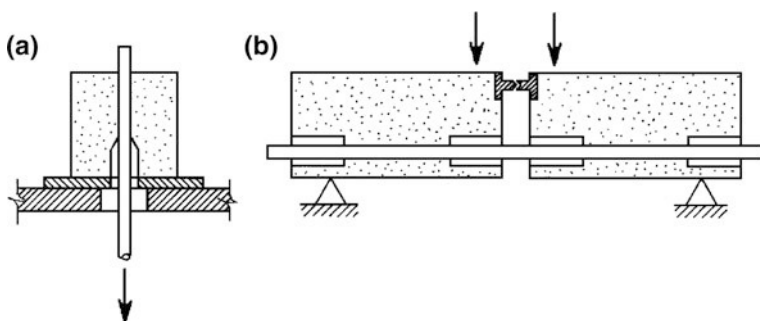
Fig. 1.36 Pull-out (a) and beam (b) tests for bond measurement
