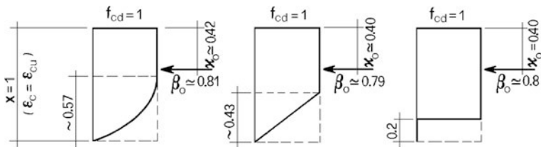
Fig. 3.3 Models of stresses in compression zone
