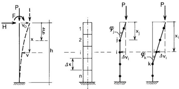
Fig. 7.3 Column deflection and discretization procedure
