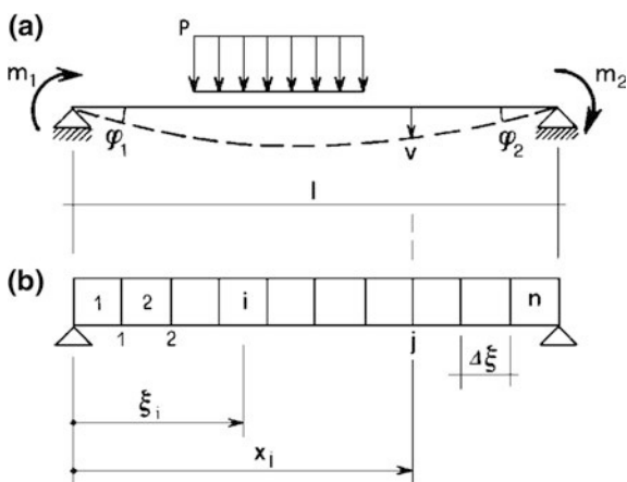
Fig. 5.34 Discretized model for deformation calculation
