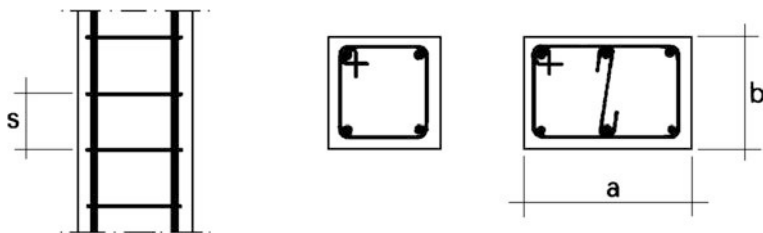
Fig. 2.1 Details of RC column—view and sections
