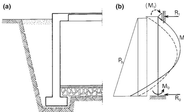
Fig. 9.41 Example of laterally braced retaining wall
