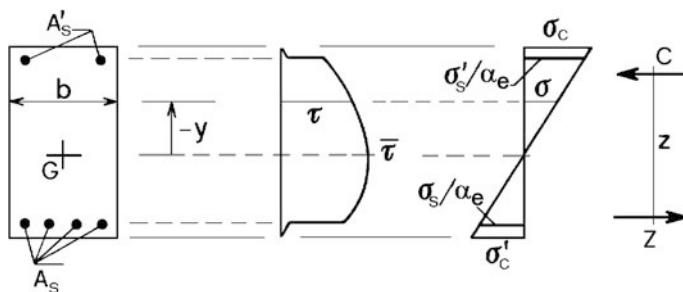
Fig. 4.1 Uncracked section—stresses distribution for shear and moment
