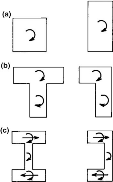
Fig. 8.19 Cases of circulatory (a and b) and warping (c) torsion
