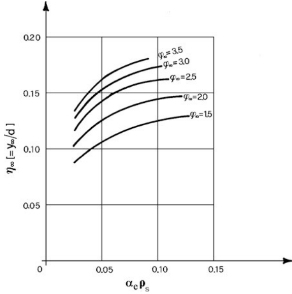
Fig. 3.25 Lowering of the neutral axis
