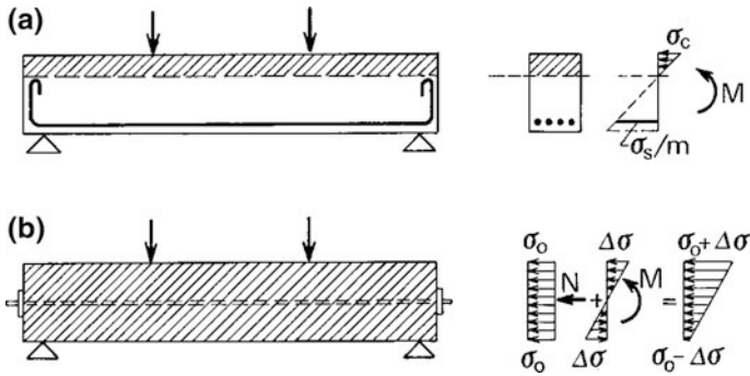
Fig. 10.1 Original concept of “fully utilize the entire section” in bending
