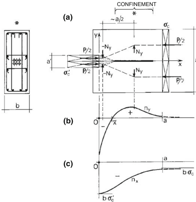
Fig. 10.35 Transverse splitting action due to stress diffusion
