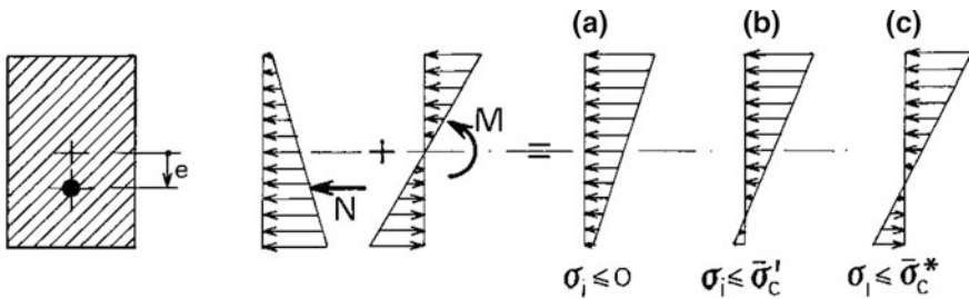
Fig. 10.2 Optimization of the tendon position
