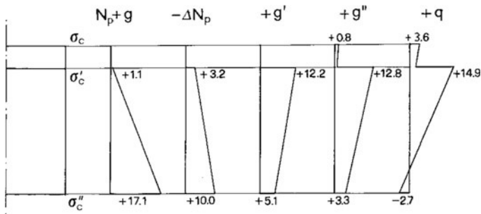
Fig. 10.51 Stress distribution at the different construction stages
