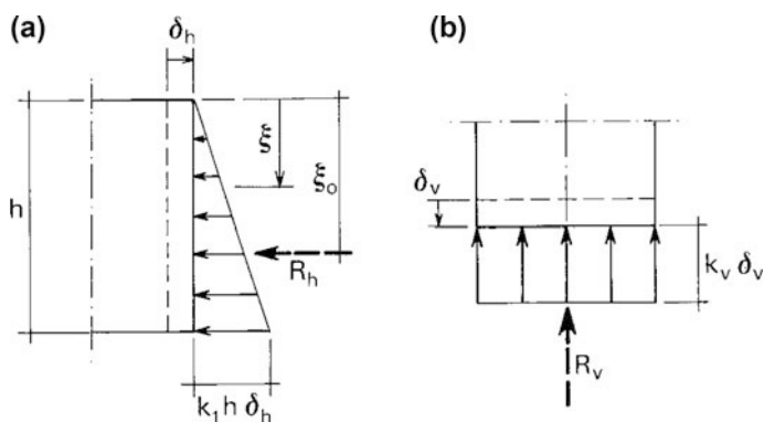
Fig. 9.5 Soil pressure response for horizontal (a) and vertical (b) displacements
