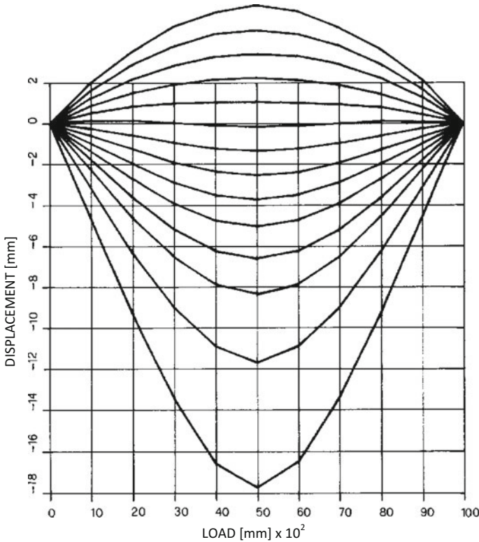
Fig. 5.38 Beam deformation for increasing loads
