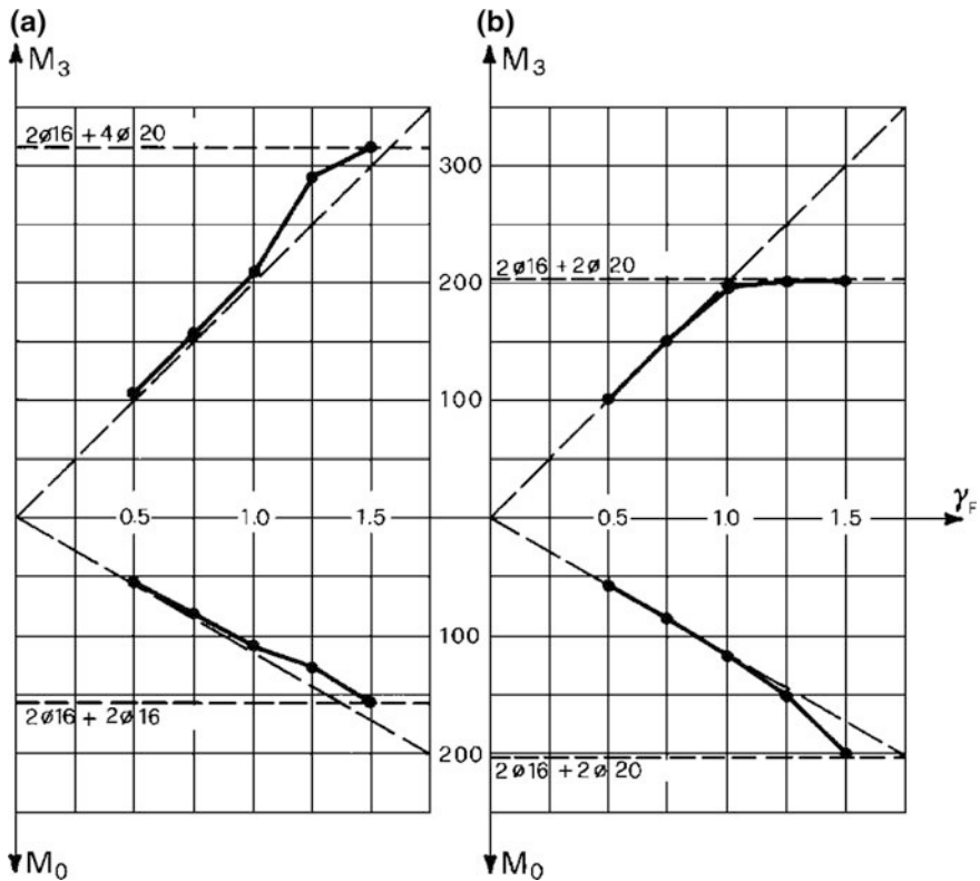
Fig. 5.43 Ways to collapse for consistent (a) and redistributed (b) steel proportioning
