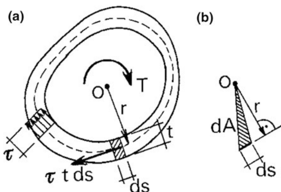
Fig. 8.4 Stress distribution in thin-walled hollow section
