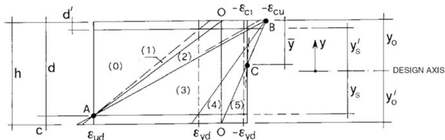
Fig. 6.11 Resistance ultimate states of the section
