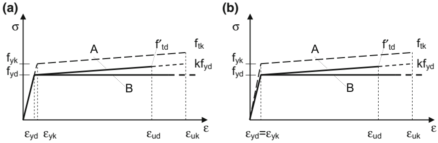
Fig. 1.30 Reinforcing steel \sigma - \varepsilon models for strength calculations
