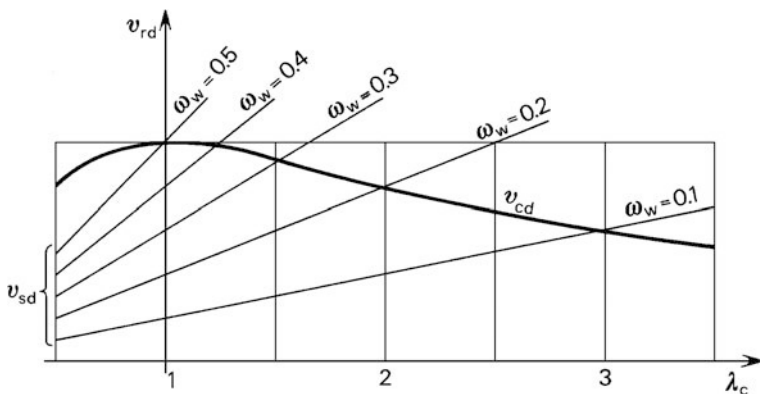
Fig. 4.35 Adimensional compression and tensile shear strengths
