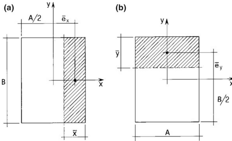
Fig. 9.56 Limit allowable eccentricities for action along x (a) and along y (b)
