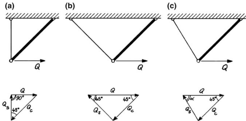
Fig. 4.10 Equilibrium conditions for a single transverse reinforcement
