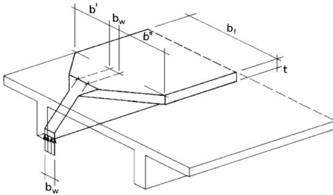
Fig. 5.14 Diffusion of stresses on web and flange
