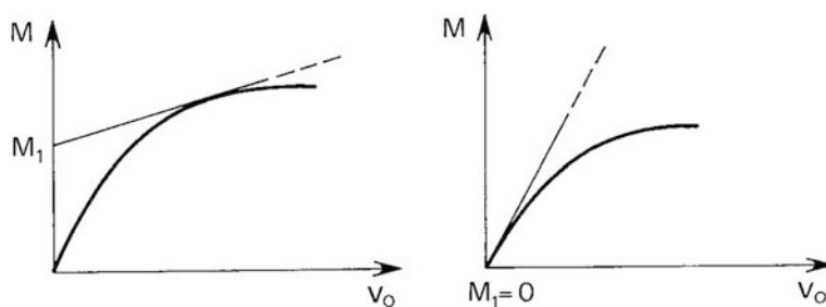
Fig. 7.10 Limit collapse situations for eccentric and centred axial compression
