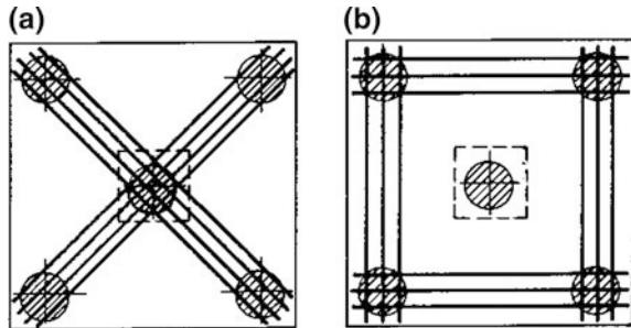
Fig. 9.17 Possible layouts of reinforcement
