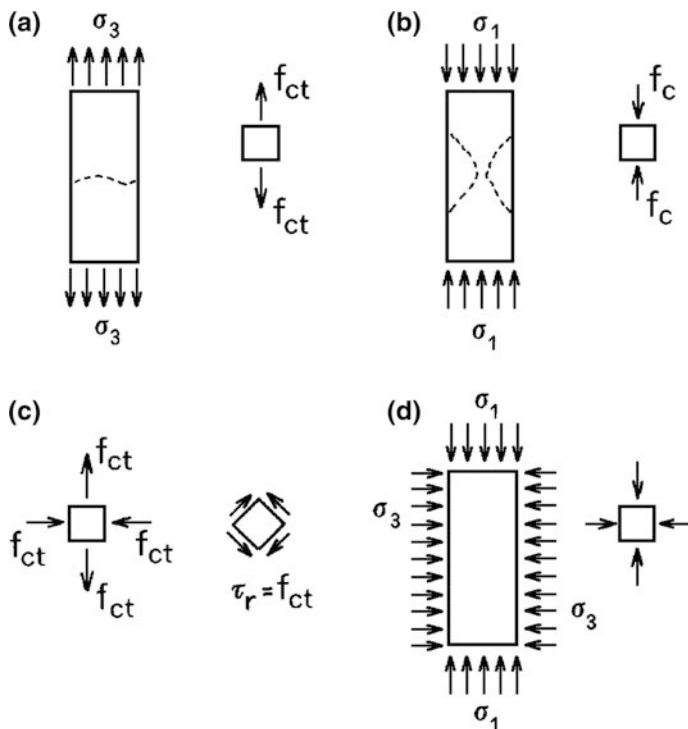
Fig. 1.13 Tests and failure limit situations
