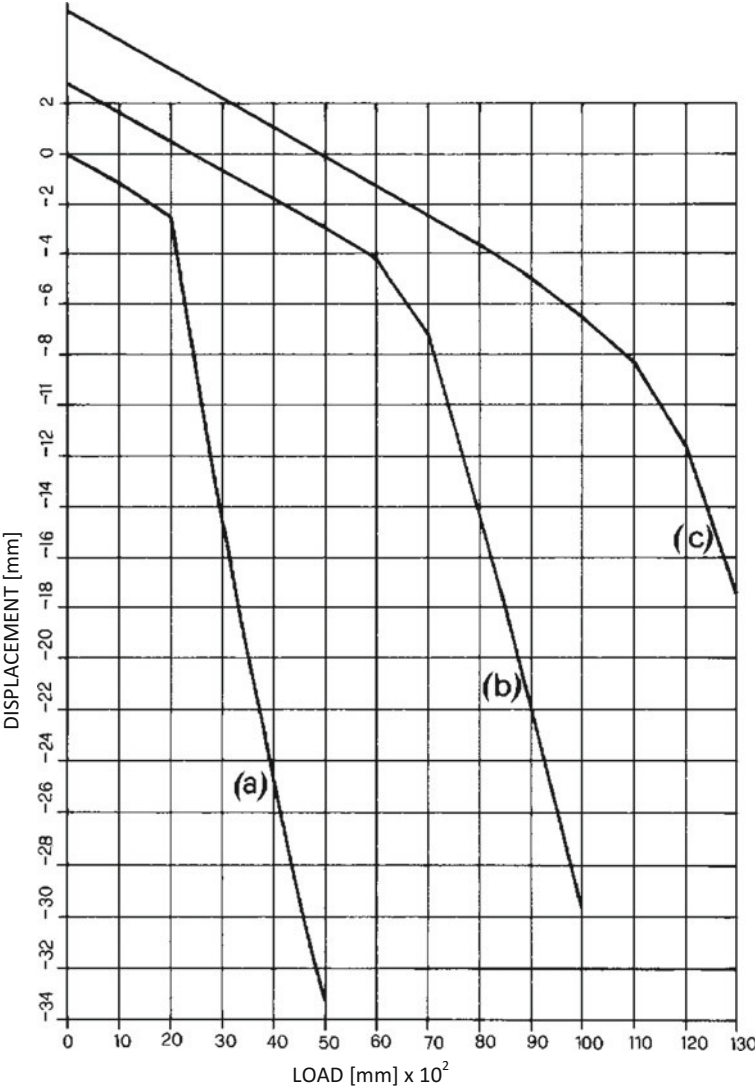
Fig. 5.37 Mid-span deflection curves
