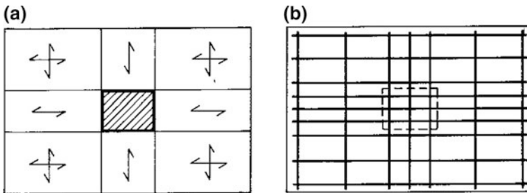
Fig. 9.11 Base reinforcement of the footing
