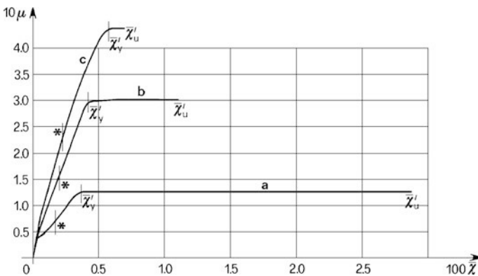
Fig. 3.37 Deformation constitutive laws
