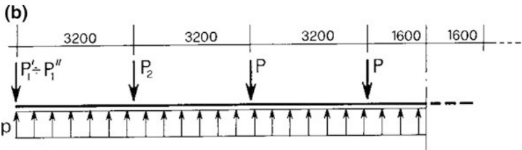
Fig. 9.53 Isolated static scheme of the foundation wall
