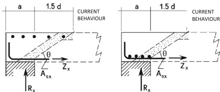
Fig. 5.31 Details on edge ( left ) and corner ( right ) supports
