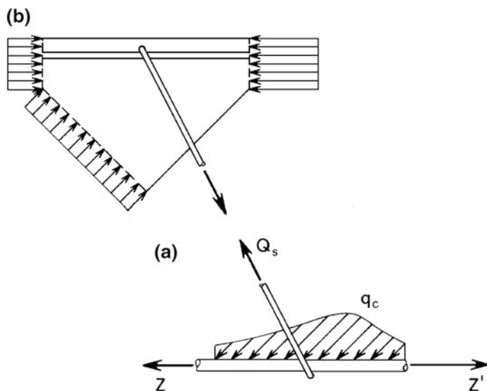
Fig. 4.13 Anchorages of stirrups
