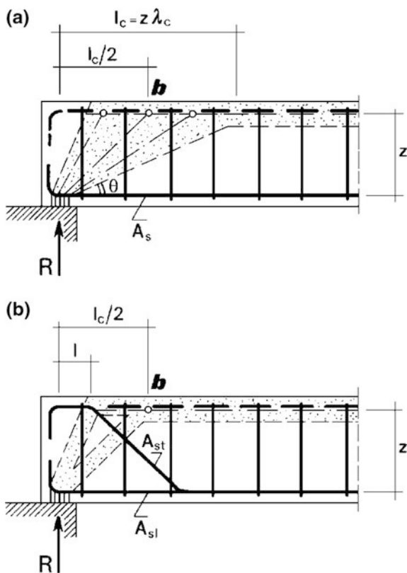
Fig. 5.20 Possible different details over the end support
