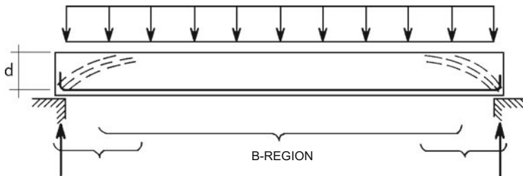
Fig. 4.16 Current “B” flexural behaviour and discontinuity “D” regions
