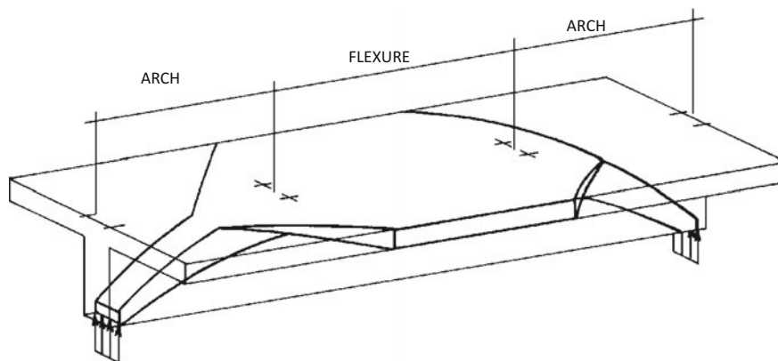
Fig. 5.16 Lateral arch behaviour in the beam web
