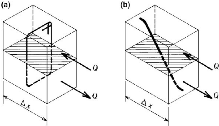
Fig. 4.7 Shear reinforcement—stirrup (a) and bent bar (b)
