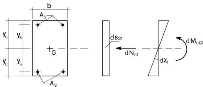
Fig. 3.23 Elementary deformation contributions
