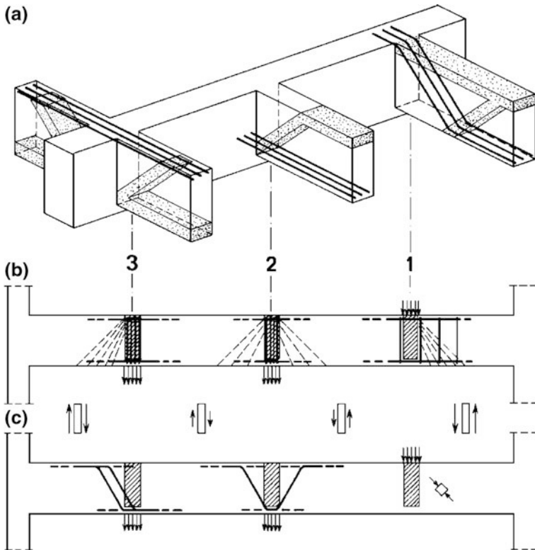
Fig. 5.21 Details of indirect supports
