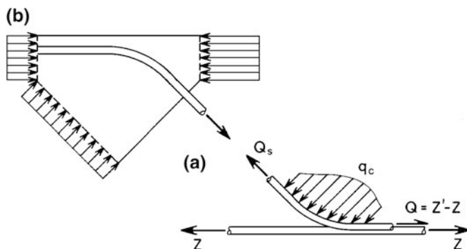
Fig. 4.14 Anchorage of bent bars
