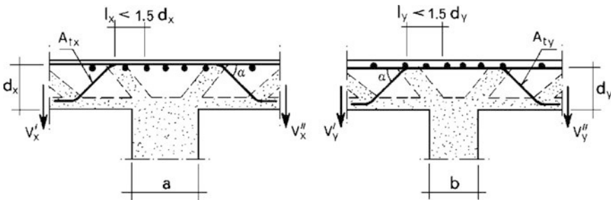
Fig. 5.32 Reinforcement layout over an internal column
