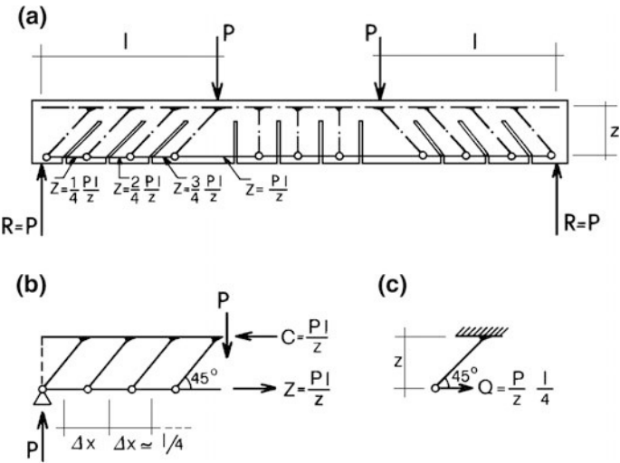
Fig. 4.17 Tooth model for beams without shear reinforcement
