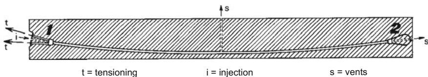
Fig. 10.6 Scheme of the tendon post-tensioning in a beam
