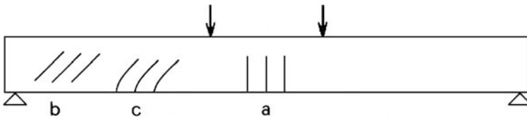
Fig. 4.15 Possible cracking patterns of the beam
