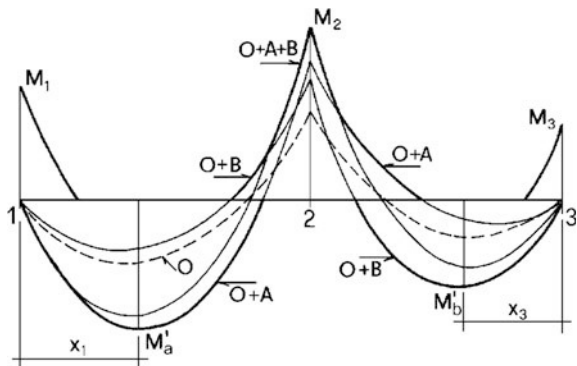
Fig. 3.43 Envelope diagram of bending moment
