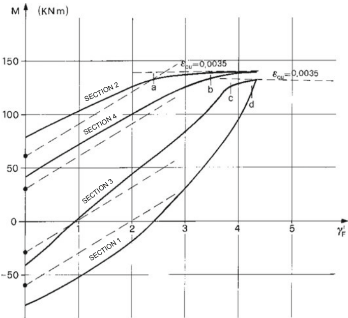
Fig. 6.42 Growth of bending moments up to collapse
