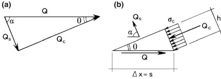
Fig. 4.34 Equilibrium conditions of the web truss
