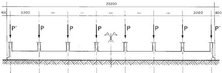
Fig. 9.21 Example of continuous foundation beam
