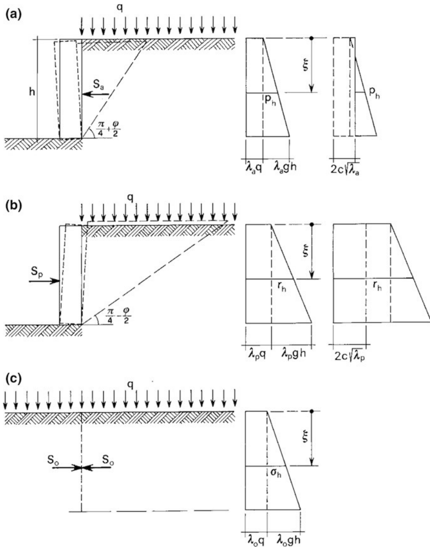
Fig. 9.32 Models of active (a), passive (b) and at rest (c) soil pressure
