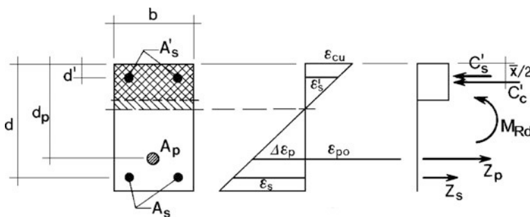
Fig. 3.16 Section with double reinforcement
