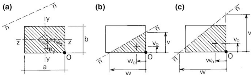
Fig. 6.4 Section with combined compression and biaxial bending
