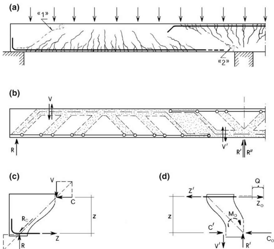
Fig. 4.25 Cracking pattern, tooth model and critical regions
