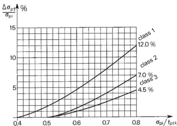
Fig. 10.13 Curves of reference relaxation losses
