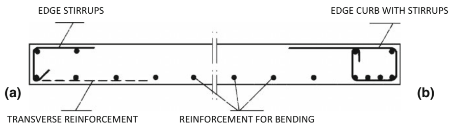
Fig. 4.26 Plate element and edge reinforcement
