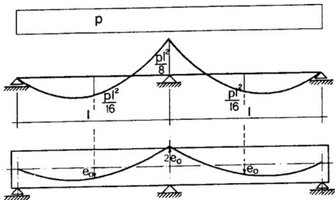
Fig. 10.23 Theoretical complying tendon
