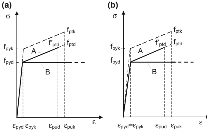
Fig. 1.32 Pre-stressing steel \sigma - \epsilon models for strength calculations
