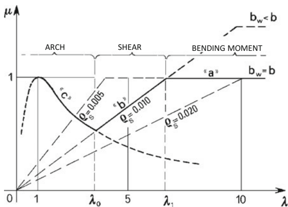
Fig. 5.4 Different domains of rupture of the beam
