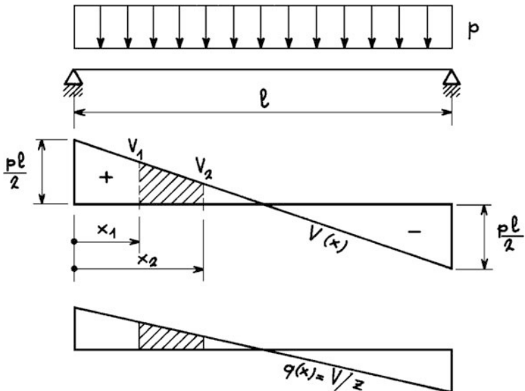
Fig. 4.8 Shear and unit longitudinal shear diagrams
