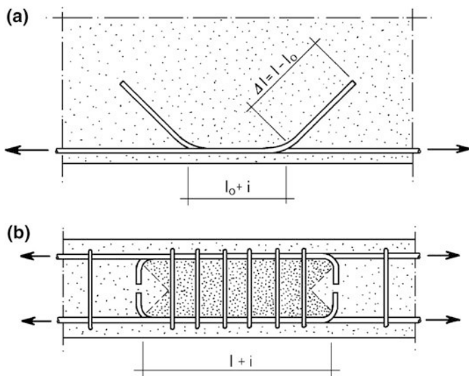
Fig. 2.29 Bars overlapping tension zones of beams (a) and ties (b)
