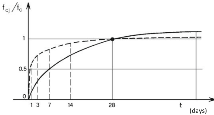
Fig. 1.3 Concrete-hardening curves
