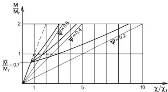
Fig. 3.21 Adimensional moment-curvature diagrams
