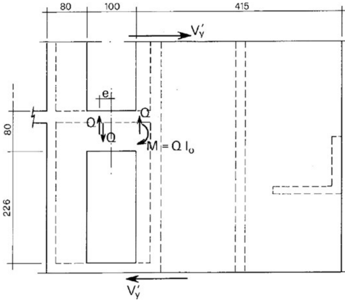
Fig. 8.28 Action acting on lintels
