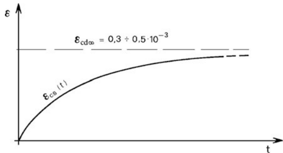
Fig. 1.5 Drying shrinkage curve
