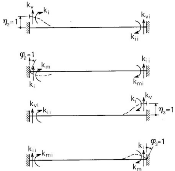
Fig. 9.28 Stiffness parameters of the beam on elastic soil
