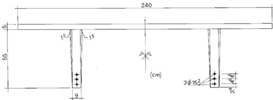
Fig. 10.44 Cross section of the element
