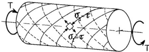
Fig. 8.5 Orientation of principal stresses under pure torsion
