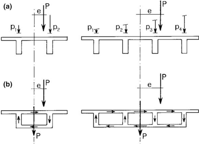
Fig. 8.20 Multiflexural (a) and circulatory (b) behaviour of a multi-rib deck
