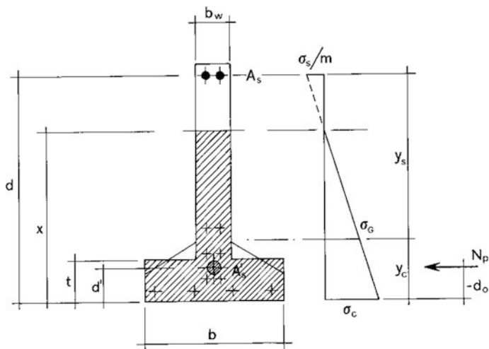
Fig. 10.52 Cracked resisting section in lifting stage
