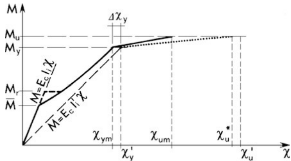
Fig. 3.28 Moment-curvature model
