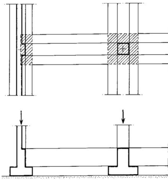
Fig. 9.29 Finite dimensions of nodes
