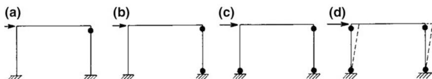
Fig. 6.40 Progressive formation of plastic hinges
