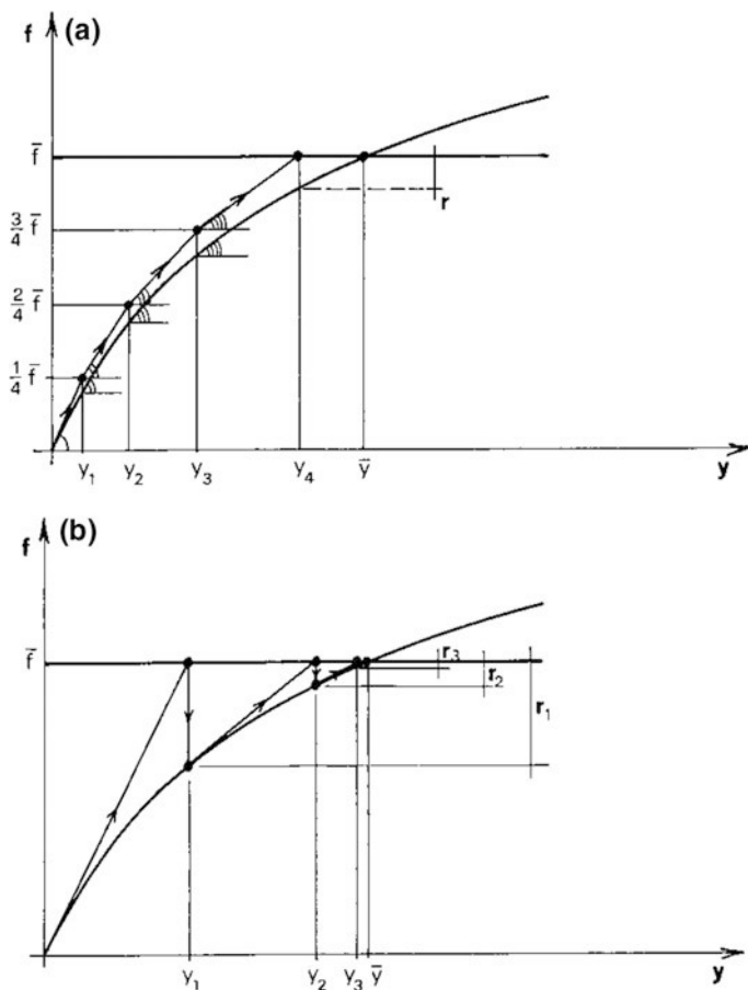
Fig. 6.36 Representations of step-by-step (a) and tangent (b) methods
