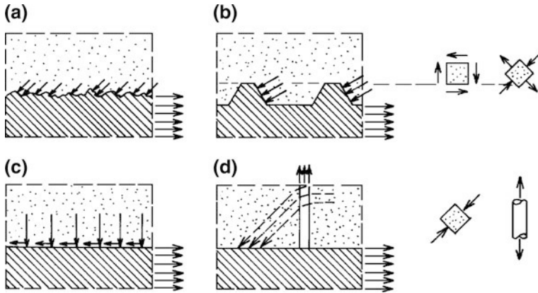
Fig. 1.35 Types of bond of steel bars
