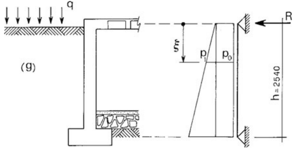
Fig. 9.55 Lateral earth pressure on the foundation wall
