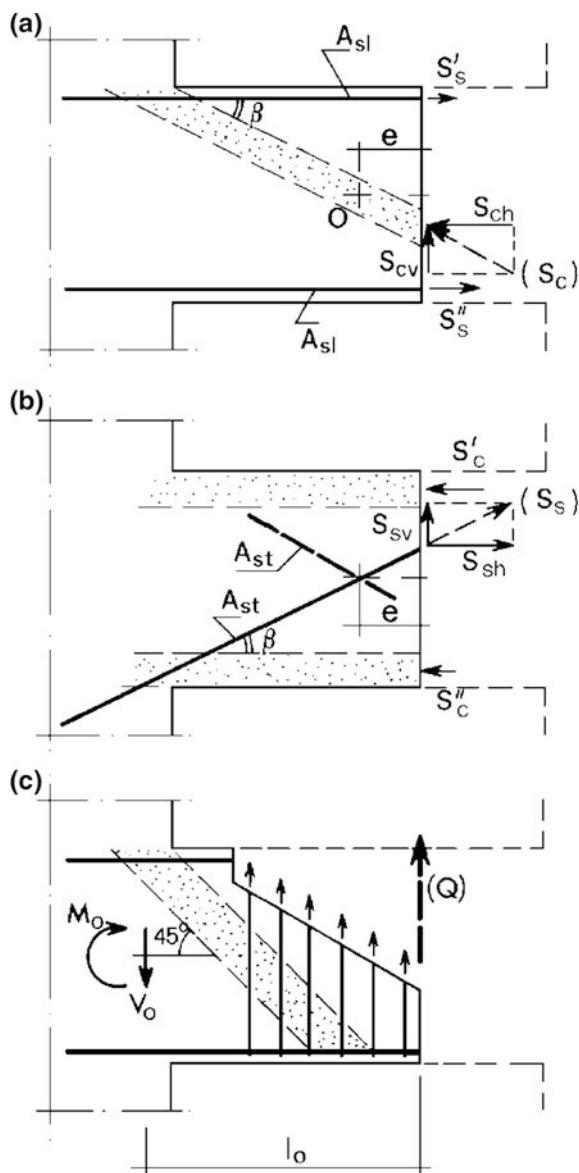
Fig. 5.25 Resisting schemes of the lintel
