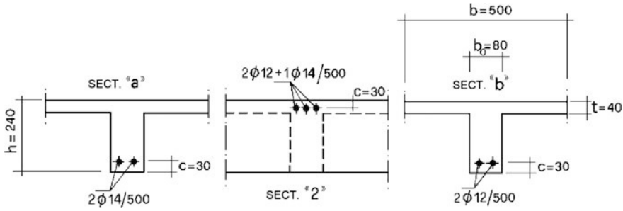
Fig. 3.45 Mid-span left, central support and mid-span right sections
