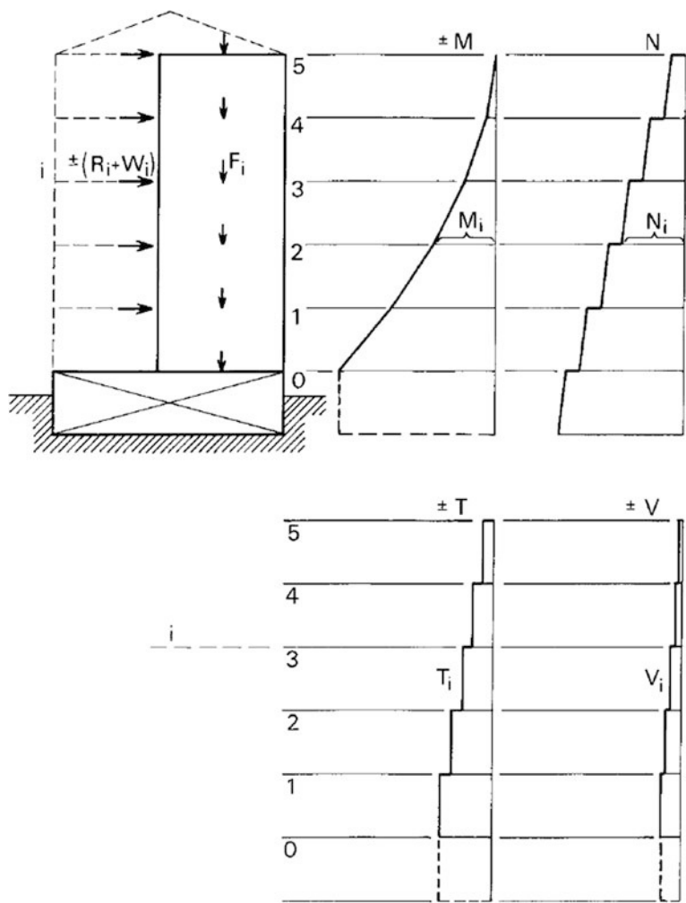
Fig. 8.25 Internal forces distribution in the corewall
