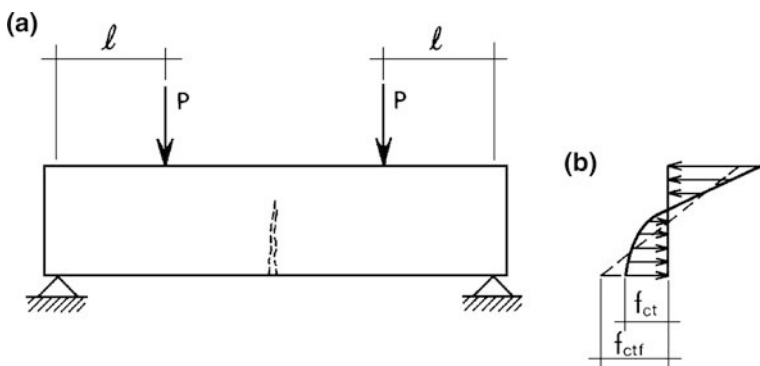
Fig. 1.9 Test for flexural strength
