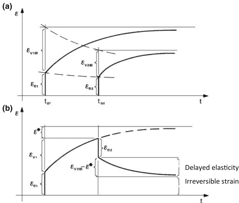
Fig. 1.17 Loading and unloading curves of concrete
