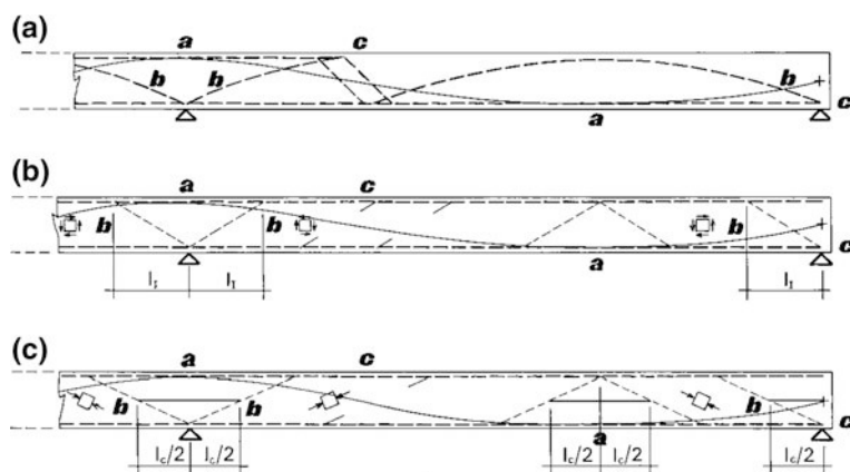
Fig. 10.30 Critical sections of the calculation procedure
