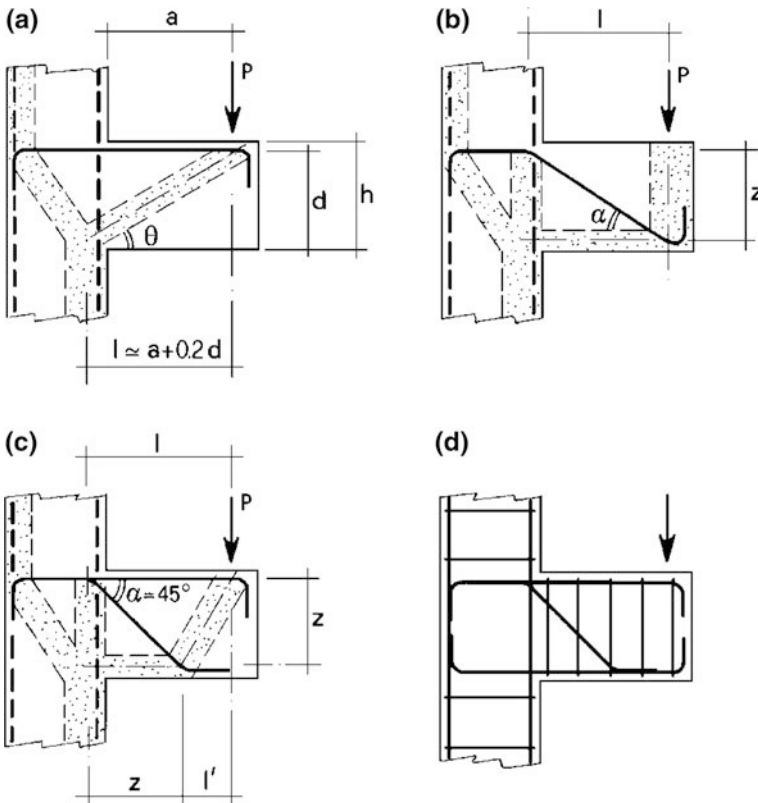
Fig. 5.22 Possible different details of corbels
