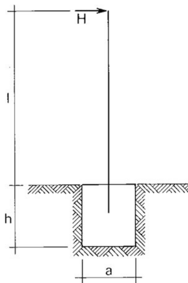
Fig. 9.4 Scheme of massive foundation
