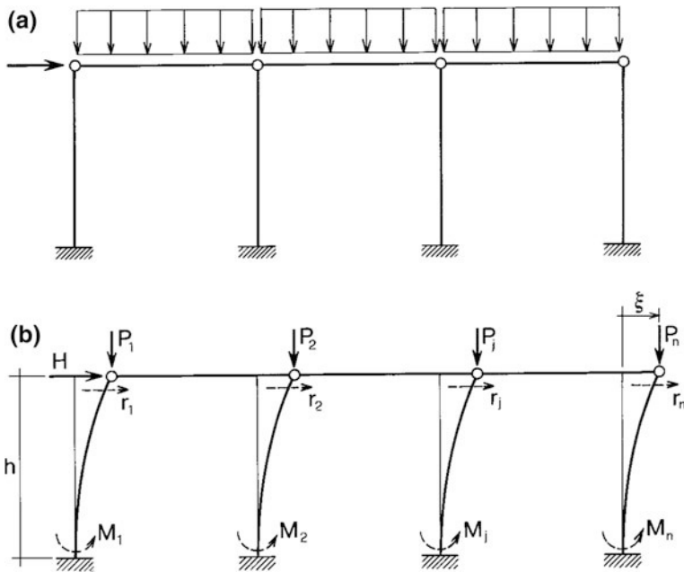
Fig. 7.16 Second-order analysis of one-storey precast frame
