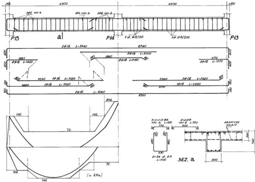
D.6 REINFORCEMENT BEAM P15-14-13
