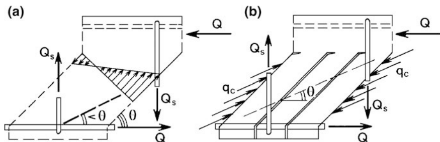
Fig. 4.32 Original (a) and improved (b) models of stress diffusion
