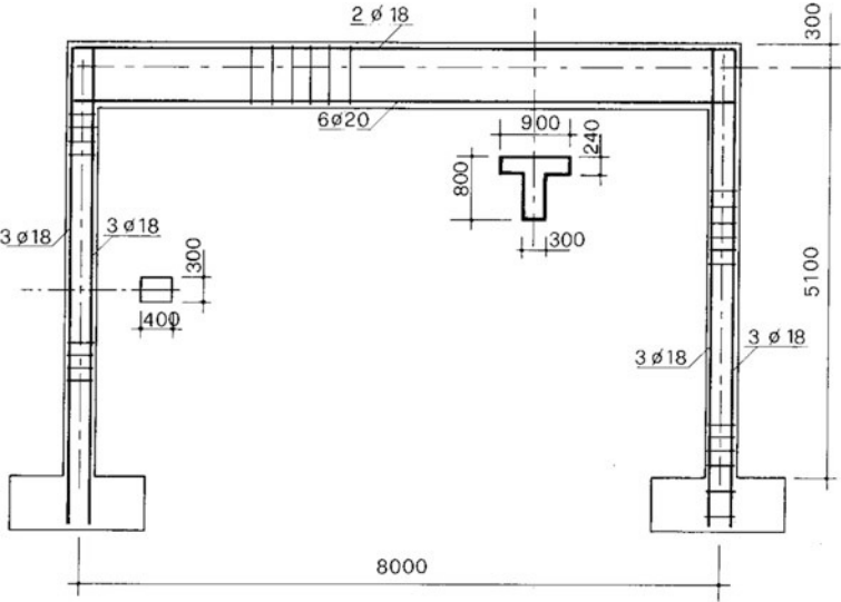
Fig. 6.38 Example of reinforced concrete frame
