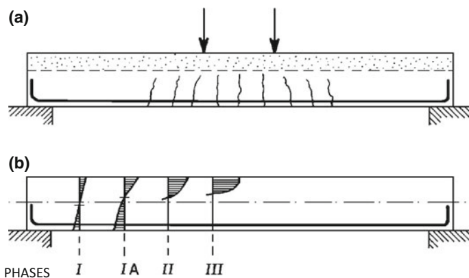
Fig. 3.1 Behaviour phases of a beam in bending
