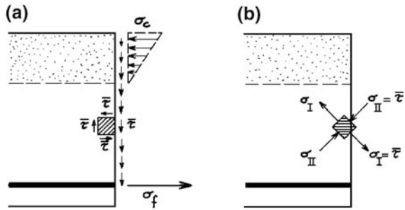
Fig. 4.4 Cracked section— theoretical distribution of stresses
