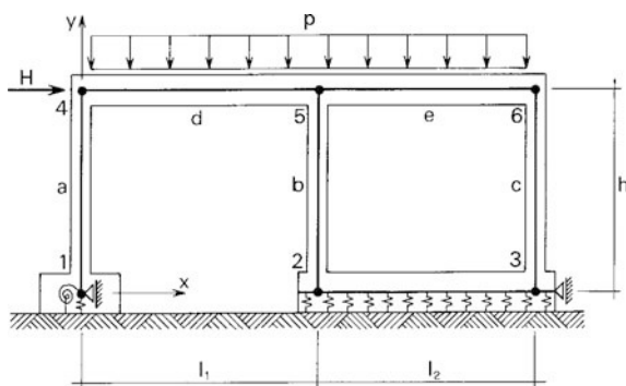
Fig. 9.26 Separate calculation models for superstructure and foundations
