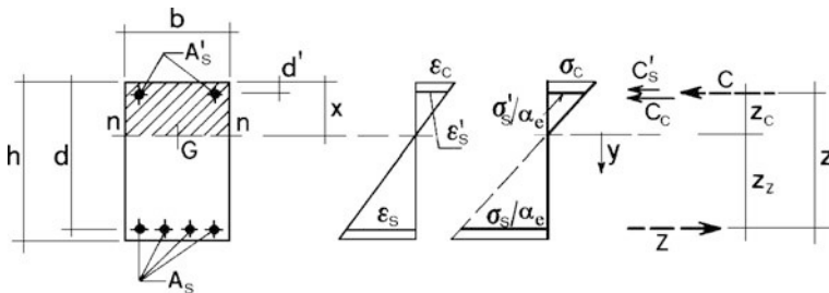
Fig. 3.7 Strain and stress distribution in a section with double reinforcement
