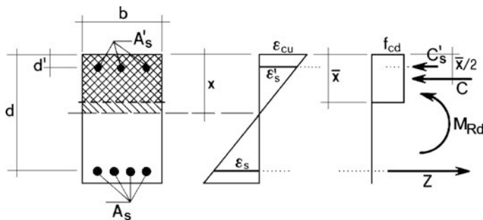
Fig. 3.12 Section with double reinforcement at ultimate limit state of bending
