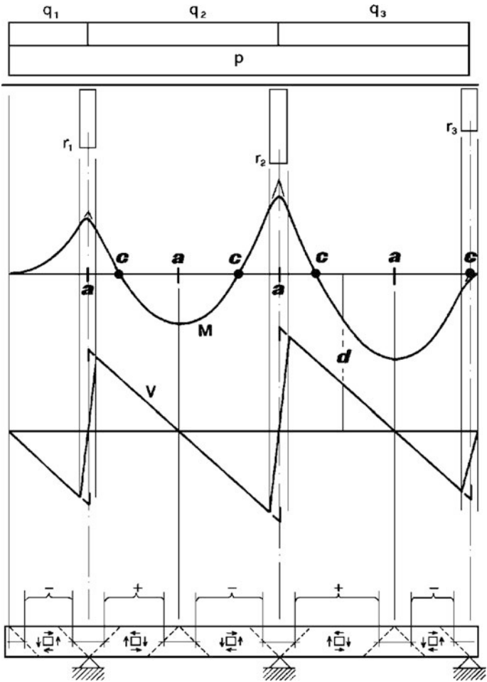
Fig. 5.1 Global model of a beam in bending
