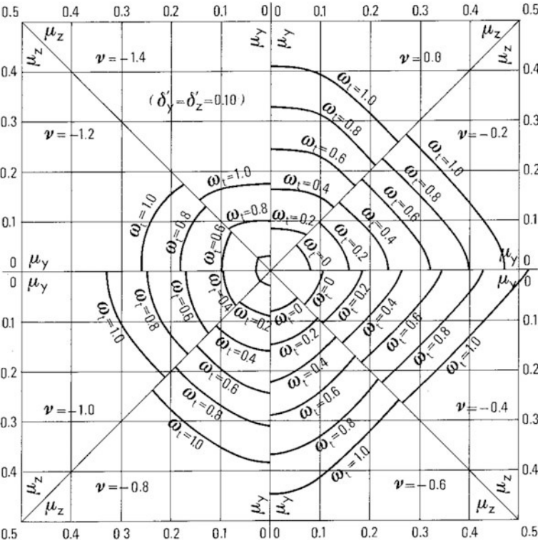
Fig. 6.25 Plane representation of the interaction surface with isolines
