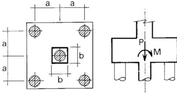
Fig. 9.15 Action applied on the piles
