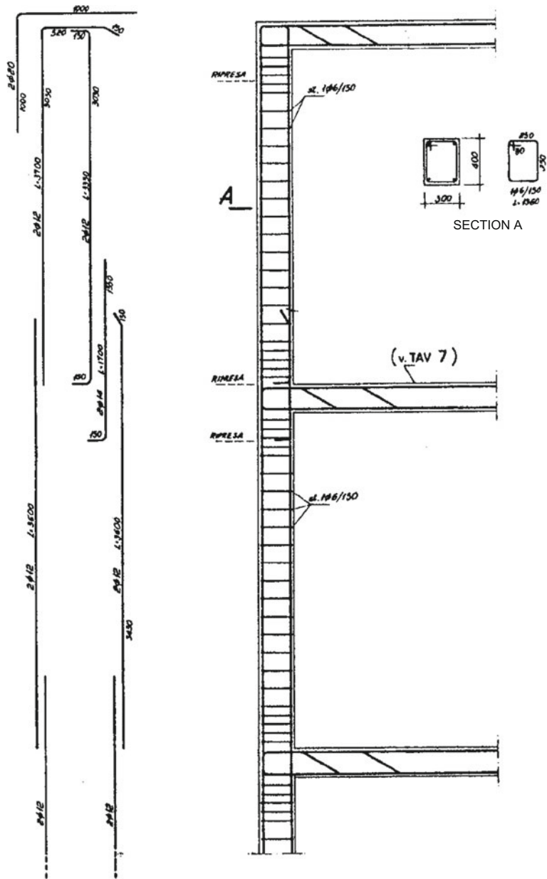
Fig. 6.45 Reinforcement details of edge column
