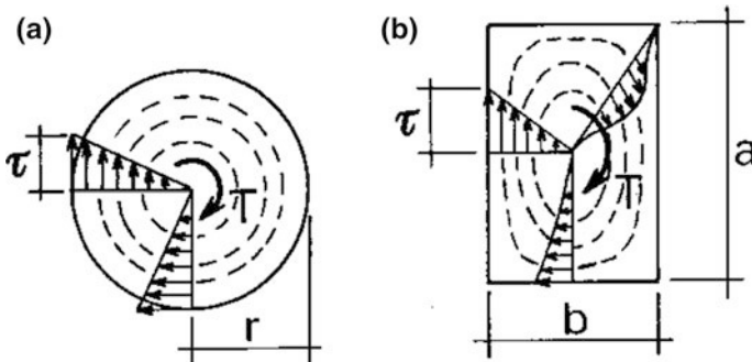
Fig. 8.3 Stress distribution in circular (a) and rectangular (b) sections
