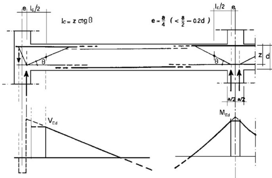
Fig. 5.12 Location of the critical sections for shear (left) and moment (right)
