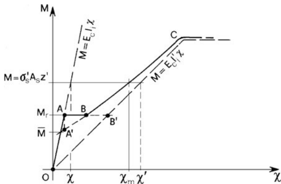
Fig. 3.19 Moment-curvature cracking model
