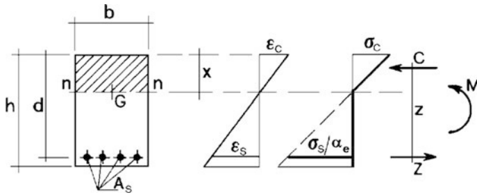
Fig. 3.6 Strain and stress distribution in a cracked section
