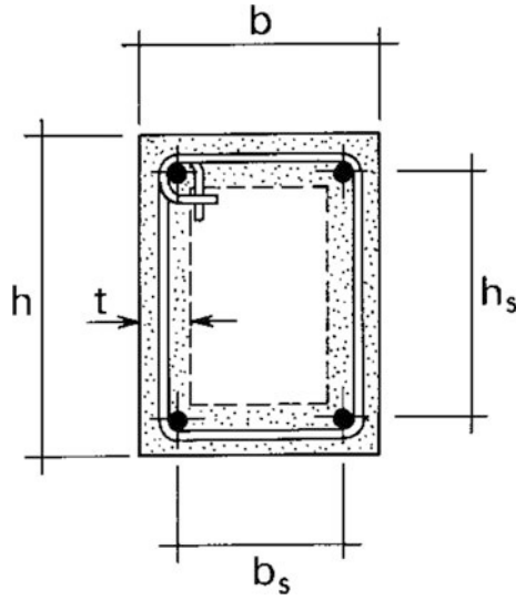
Fig. 8.8 Peripheral position of the resisting mechanism
