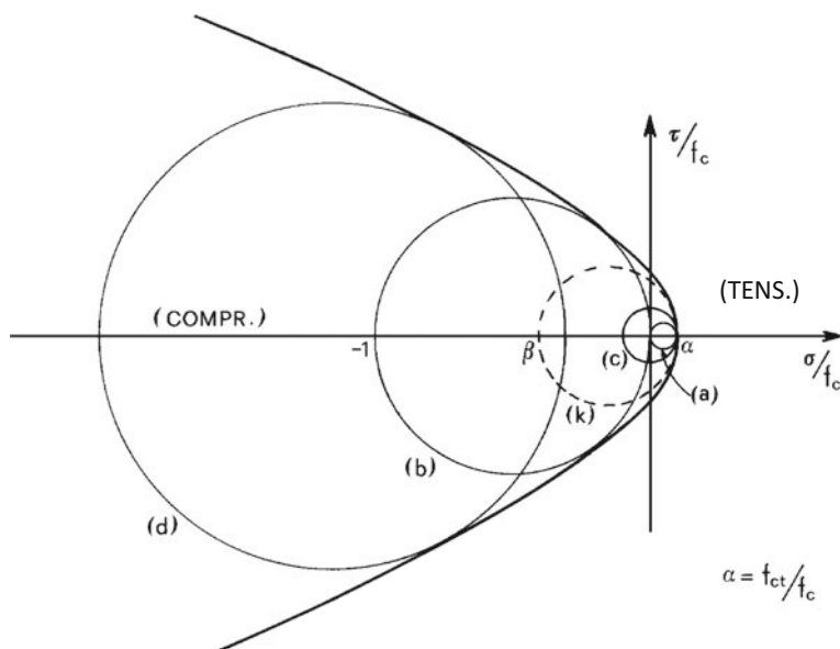
Fig. 1.12 Representation of Mohr's envelope curve for concrete failure
