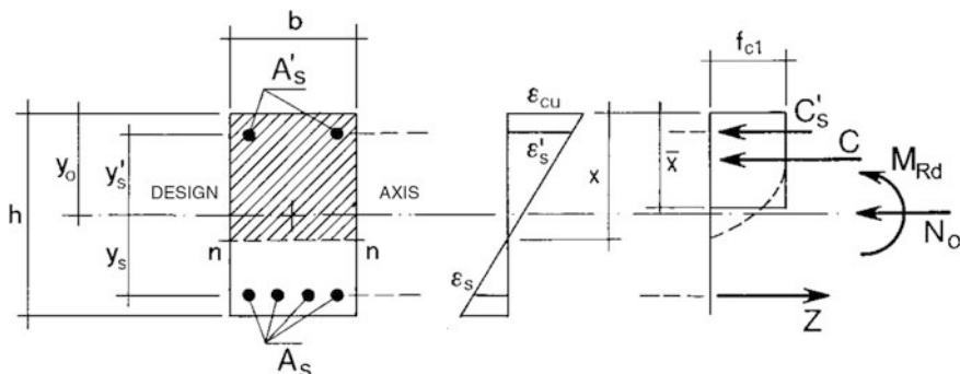
Fig. 6.20 Resistance limit state under compression and uniaxial bending
