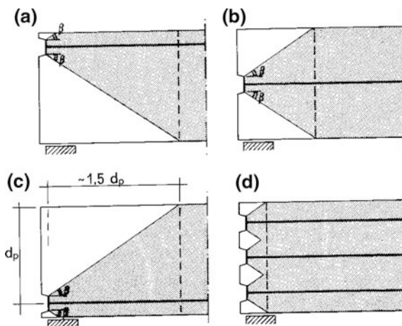
Fig. 10.39 Post-tensioned tendons—model of prestressing diffusion
