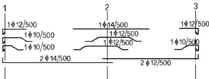
Fig. 3.46 General layout of reinforcing bars
