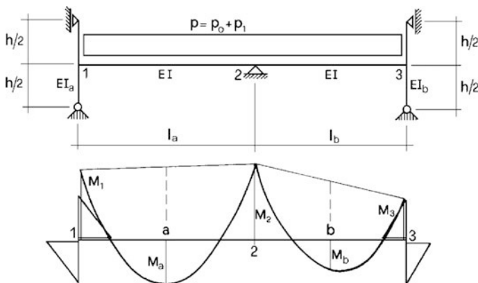
Fig. 3.44 Calculation scheme for the end moments
