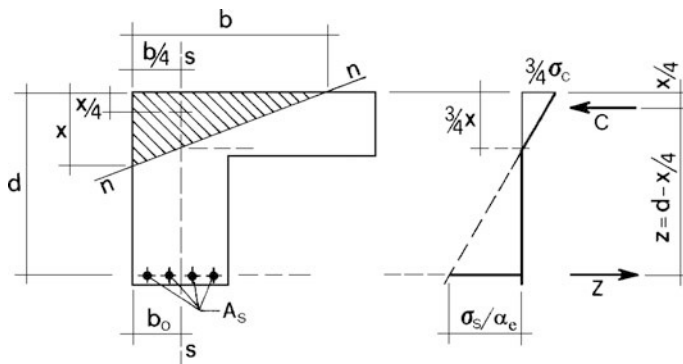
Fig. 3.8 Section under biaxial bending
