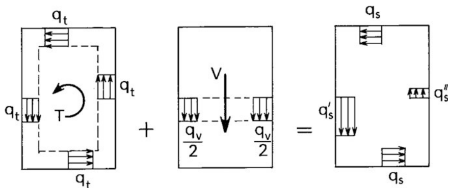
Fig. 8.17 Sum of fluxes in V-T interaction
