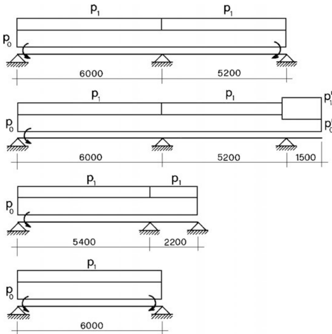
Fig. 3.40 Calculation schemes of the different floor strips
