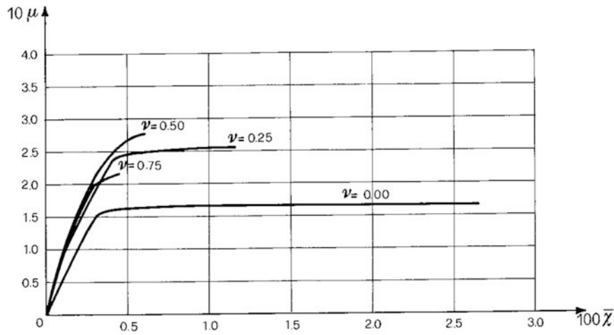
Fig. 6.32 Resistance moment-curvature curves
