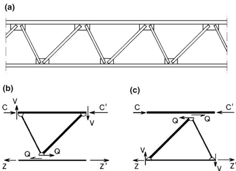
Fig. 4.12 Joint connections of the truss model
