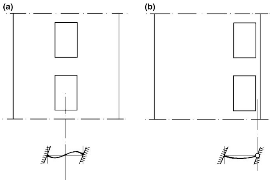
Fig. 5.26 Different structural situations of the lintel
